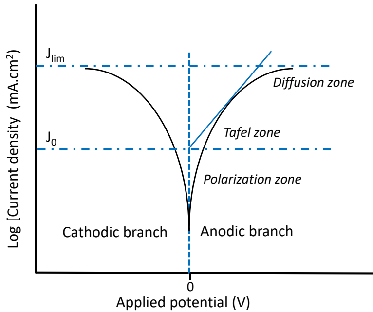
Figure 2.15: Diagram illustrating a Tafel polarization plot of a DSSC.
