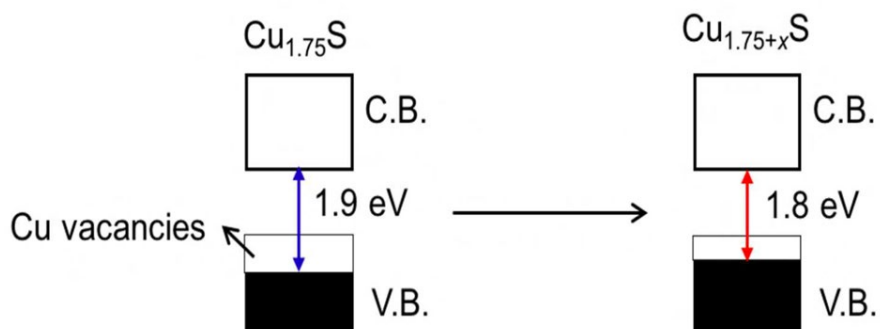
Figure 4.15: Diagram showing the change in bandgap due to copper vacancies [17].
