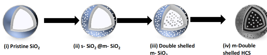
Figure 3.4: Schematic diagram depicting the synthesis of double-shelled mesoporous hollow carbon spheres.
