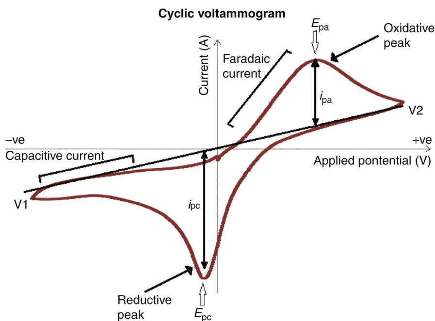
Figure 2.13: Diagram illustrating a cyclic voltammetry plot showing the cathodic potential ( E_{pc} ) and current ( I_{pc} ) [136].
