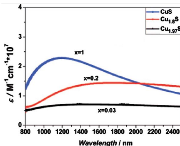
Figure 4.6: Near-infrared spectra of \text{Cu}_{2-x}\text{S} nanostructures, showing absorption energy with relation to increasing copper deficiency [31].
