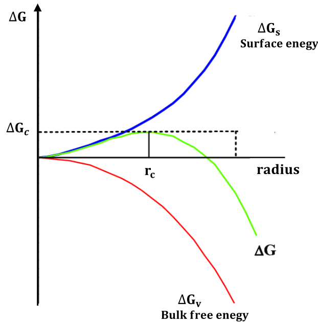
Figure 2.10: Graph shows the change in Gibbs free energy for clusters depending on their radius r_c .
