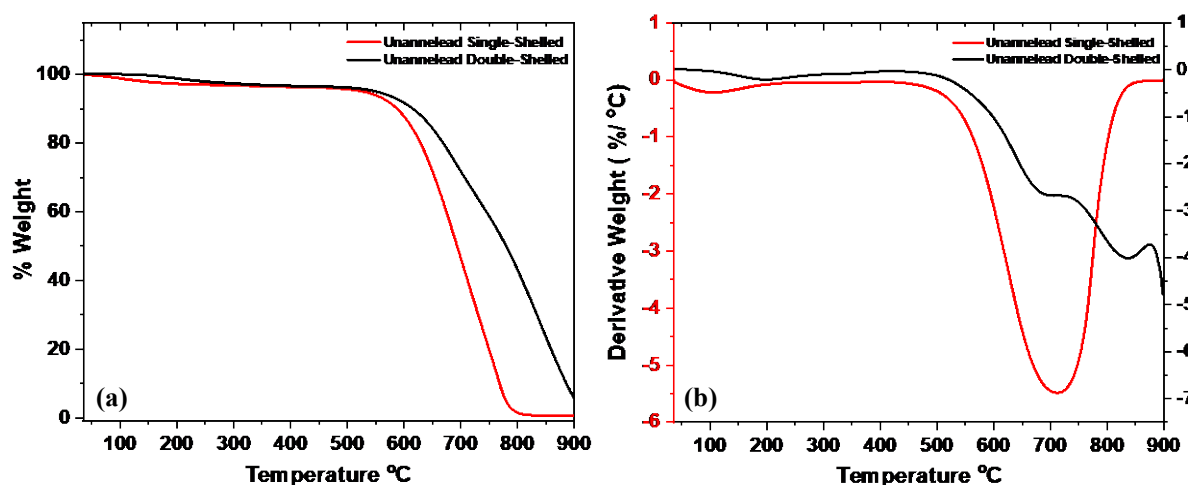
Figure 3.15: (a) Thermograms and (b) corresponding derivative profiles of unannealed single and double-shelled mesoporous hollow carbon spheres.
