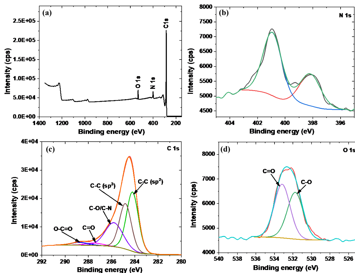
Figure 3.18: (a) XPS survey spectrum of N-doped single-shelled HCS and (b)-(d) high-resolution spectra of nitrogen, carbon, and oxygen, respectively.
