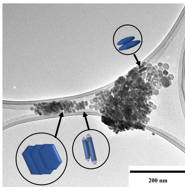
Figure 4.10: TEM micrograph of different orientations for synthesized \text{Cu}_{2-x}\text{S} at 60 min reaction time.
