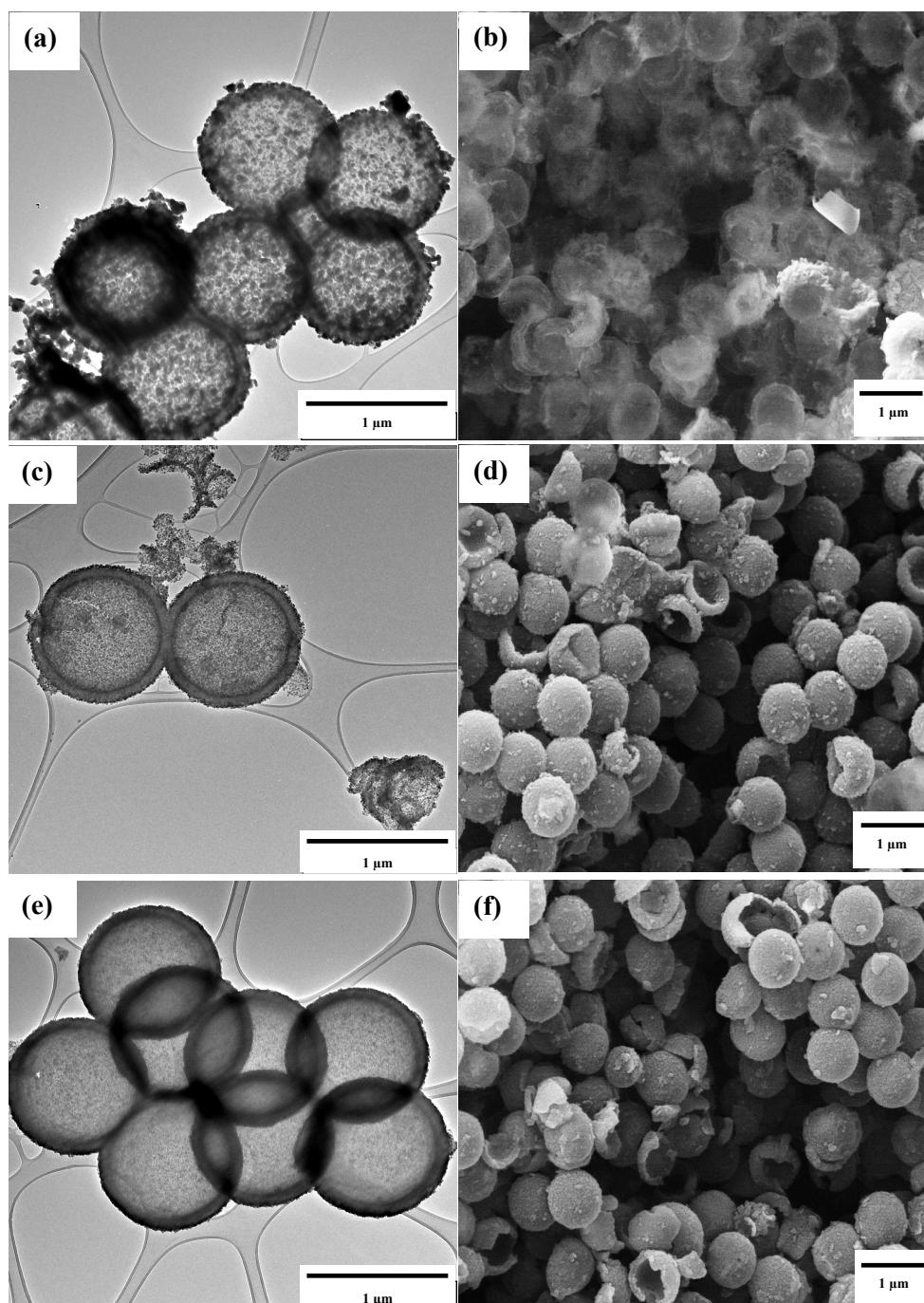
Figure 5.4: TEM micrographs of (a) 25 wt% N-HCS, (c) 50 wt% N-HCS and (e) 75 wt% N-HCS with their corresponding SEM micrographs (b, d, and f).
