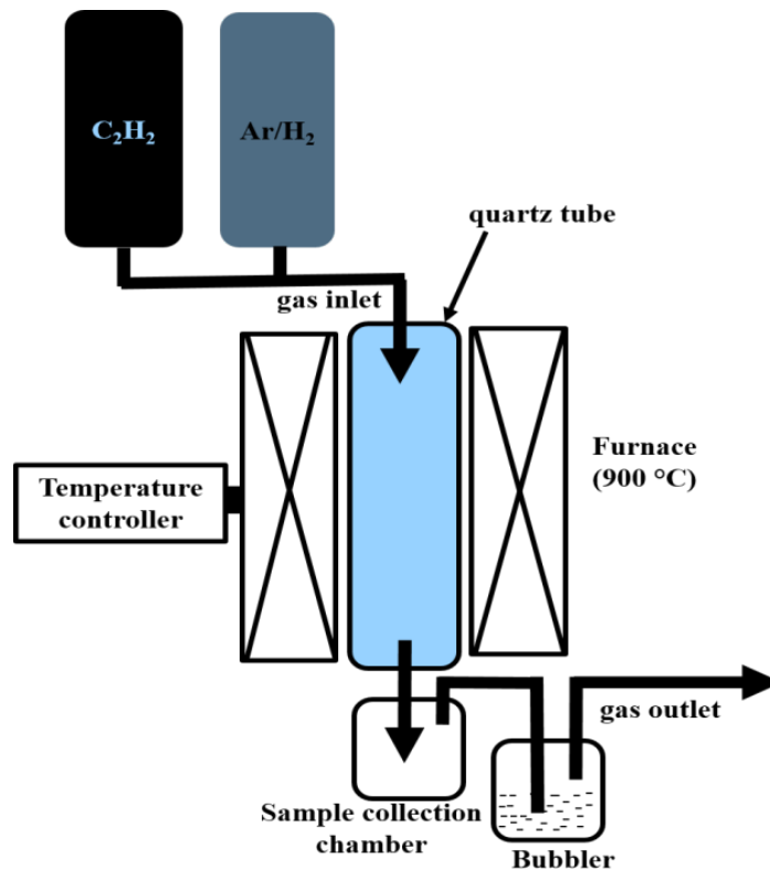
Figure 2.2: Schematic diagram showing the arrangement of a vertical CVD reactor [44].
