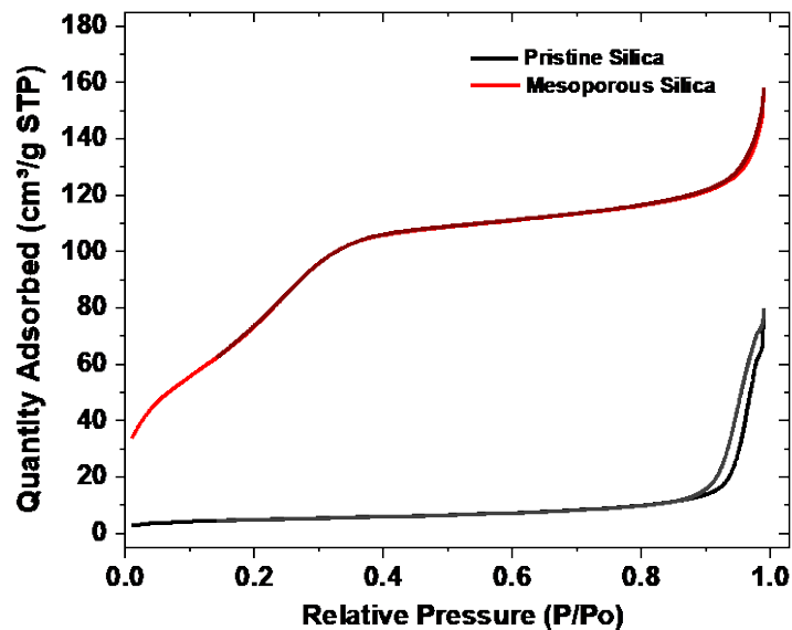
Figure 3.7: BET surface area analysis of pristine and mesoporous silica spheres.
