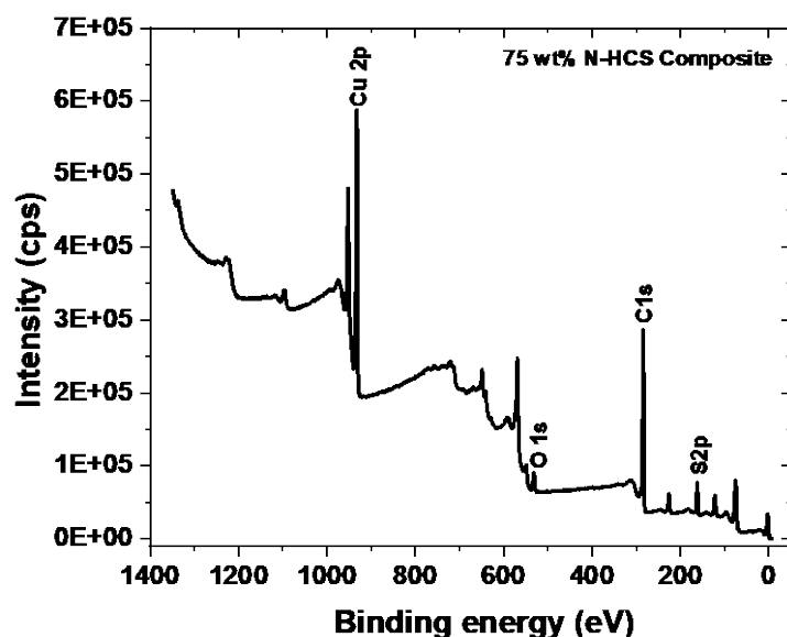
Figure 5.5: XPS survey spectrum for the 75 wt% N- HCS composite.
