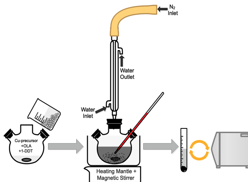
Figure 4.2: Simplified schematic diagram showing the synthesis sequence for Cu 2-x S nanoparticles.
