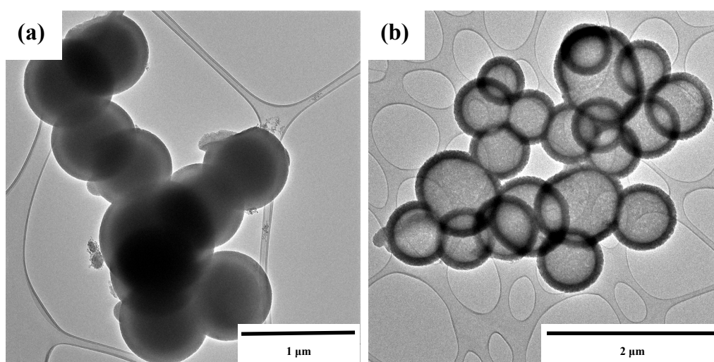
Figure 3.11: TEM micrographs of (a) \text{SiO}_2@m\text{-SiO}_2 , (b) double-shelled m\text{-SiO}_2 .
