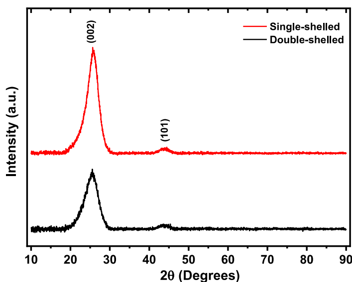
Figure 3.13: Powder X-ray diffraction patterns of single and double-shelled mesoporous hollow carbon spheres.
