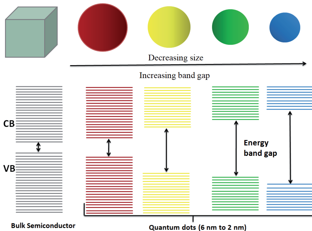
Figure 2.8: Descriptive diagram showing the relationship between bandgap energy and size of particles [100].
