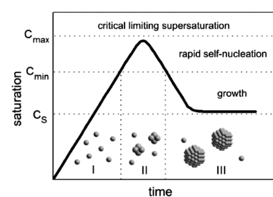
Figure 2.11: Diagram showing LaMer plot for the generation of nuclei, nucleation, supersaturation and the successive growth of colloidal systems [110].
