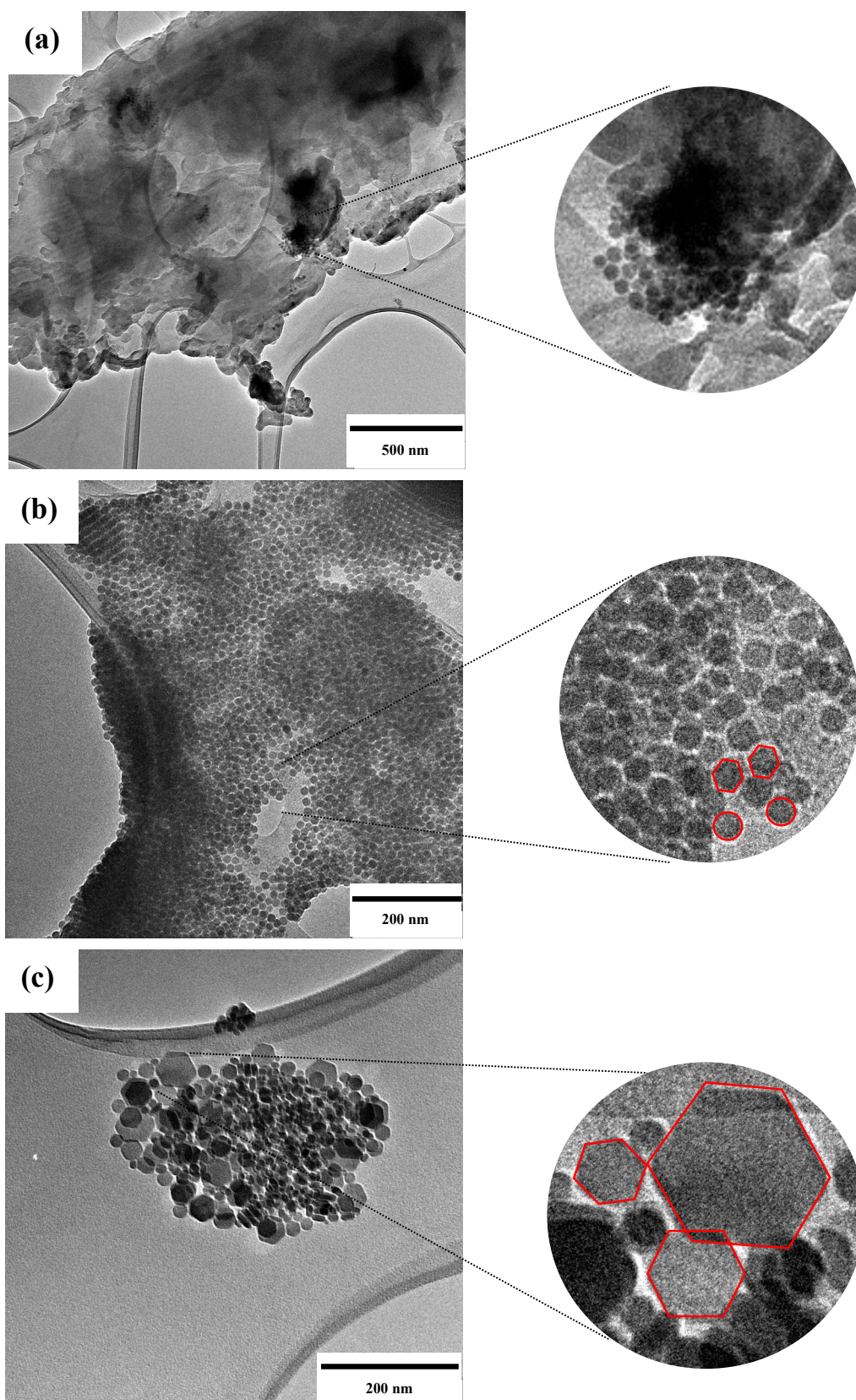
Figure 4.8: Synthesized \text{Cu}_{2-x}\text{S} TEM micrographs (a)-(c) and (d)-(e) particle size distribution for particles at 30 and 60 min reaction time using \text{Cu}(\text{acac})_2 as a precursor.
