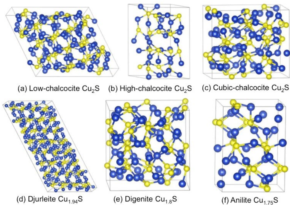
Figure 2.6: Crystal structures of (a) the low-chalcocite), (b) high chalcocite (hexagonal), (c) cubic-chalcocite (cubic), (d) djurleite, (e) digenite, and (f) anilite. Blue and yellow represent copper and sulfur atoms respectively [97].
