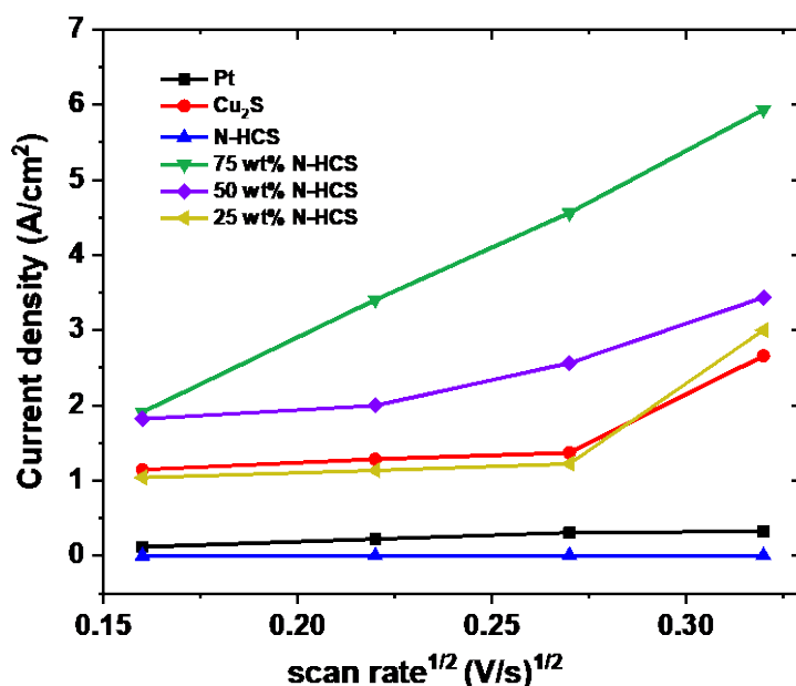
Figure 5.9: Capacitive current versus scan rate for the prepared composites, Pt, Cu 2 S, and N-HCS electrocatalysts.
