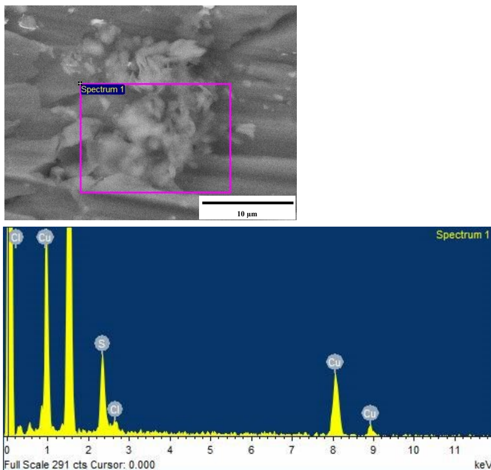
Figure 4.7: EDX spectrum and corresponding SEM micrograph of synthesized \text{Cu}_{2-x}\text{S} at 60 min.
