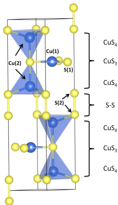
Figure 2.7: Hexagonal unit cell showing the Cu-S system of triangular and tetrahedron coordination for copper (blue) and sulfur (yellow) [92].
