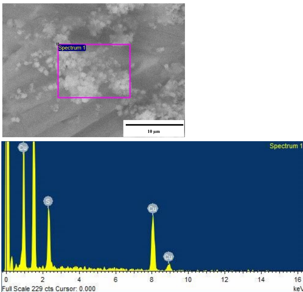
Figure 4.13: EDX spectrum and corresponding SEM micrograph of synthesized \text{Cu}_{2-x}\text{S} at 60 min.
