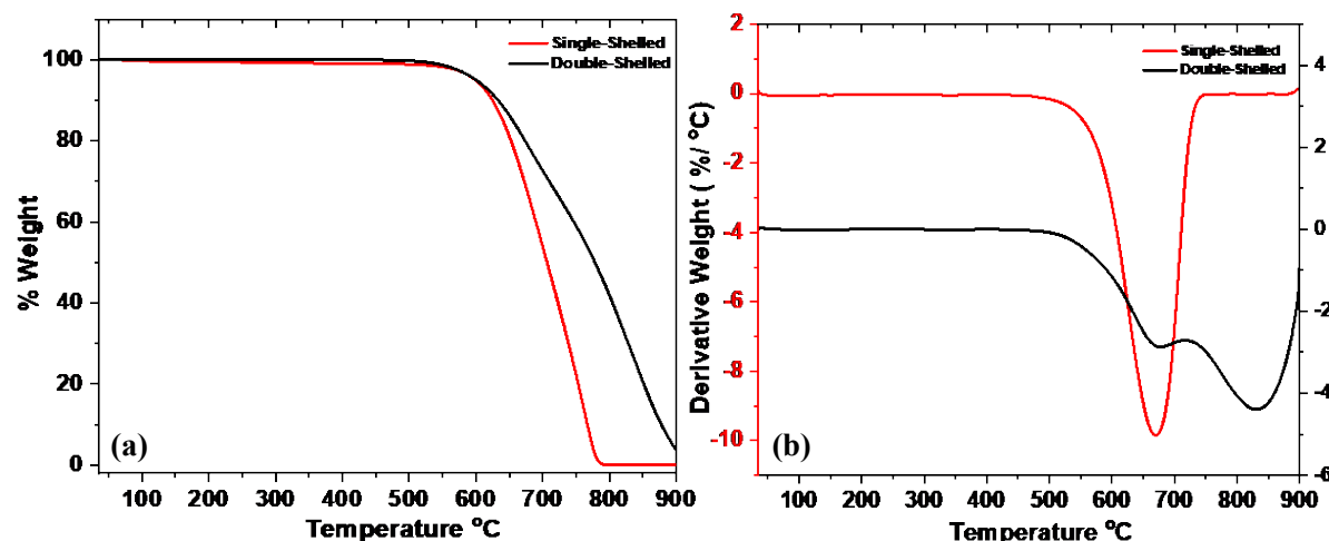
Figure 3.16: a) Thermograms and (b) corresponding derivative profiles of annealed single and double-shelled mesoporous hollow carbon spheres.
