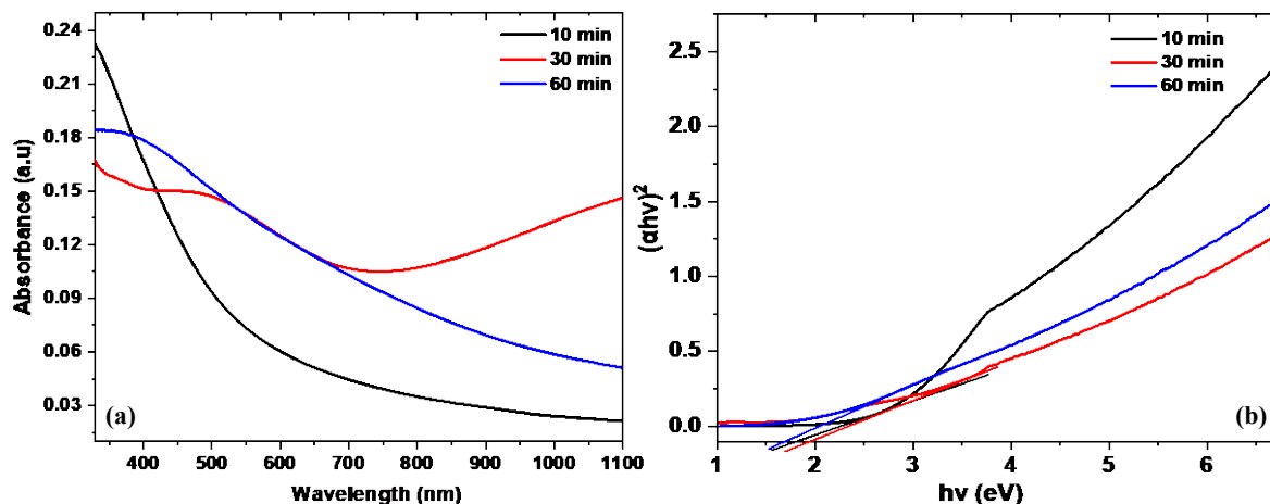
Figure 4.12: a) UV-Vis absorption spectra of synthesized \text{Cu}_{2-x}\text{S} particles at different reaction times, using \text{Cu}(\text{acac})_2 as a Cu precursor and (b) their corresponding Tauc plots.
