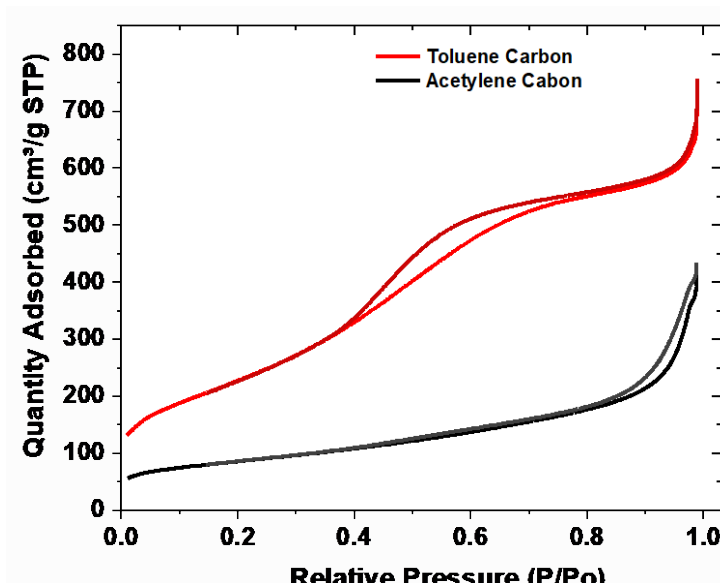
Figure 3.10: BET surface area analysis of mesoporous hollow carbon spheres carbonized by toluene (red) and acetylene (black).
