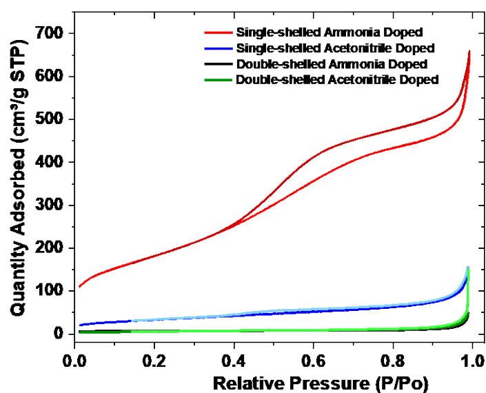
Figure 3.17: BET surface area analysis of nitrogen-doped mesoporous hollow carbon spheres.
