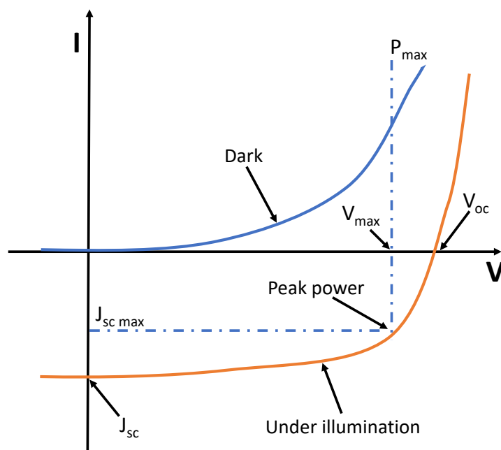
Figure 2.16: Plot of the current-voltage (I-V) curves of a solar cell in the dark and under illumination.
