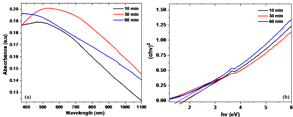
Figure 4.5: (a) UV-vis absorption spectra of synthesized \text{Cu}_{2-x}\text{S} particles at different reaction times, using CuCl as a Cu precursor and (b) their corresponding Tauc plots.
