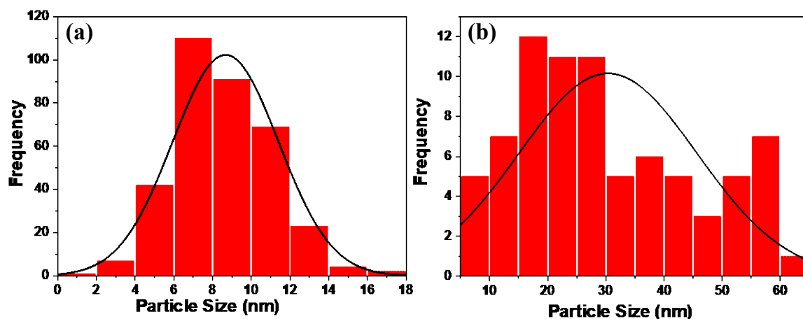
Figure 4.9: Particle size distribution for synthesized \text{Cu}_{2-x}\text{S} particles at 30 and 60 min reaction time using \text{Cu}(\text{acac})_2 as a precursor.
