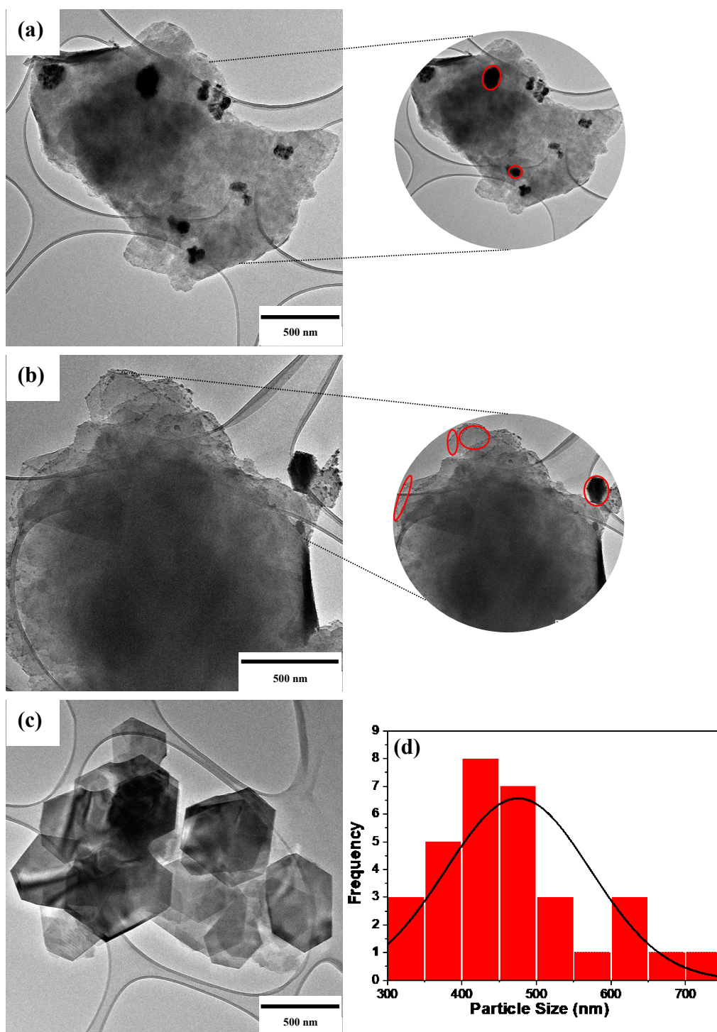
Figure 4.3: Synthesized \text{Cu}_{2-x}\text{S} TEM micrographs at different reaction times (a) 10 min (b) 30 min, and (c) 60 min. The particle size distribution for the synthesized particles at 60 min reaction time.
