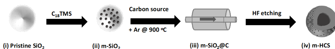
Figure 3.3: Schematic diagram depicting the synthesis of single-shelled mesoporous hollow carbon spheres.
