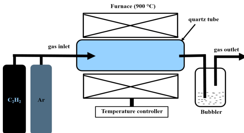
Figure 2.3: Schematic diagram showing the arrangement of a horizontal CVD reactor [44].
