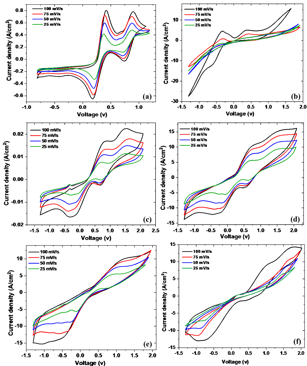
Figure 5.8: Cyclic voltammograms for (a) Pt-CE, (b) Cu 2 S (c) N-HCS, (d) 75wt% N-HCS, (e) 50wt% N-HCS and (f) 25 wt% N-HCS counter electrode at various scan rate after 10 scans.
