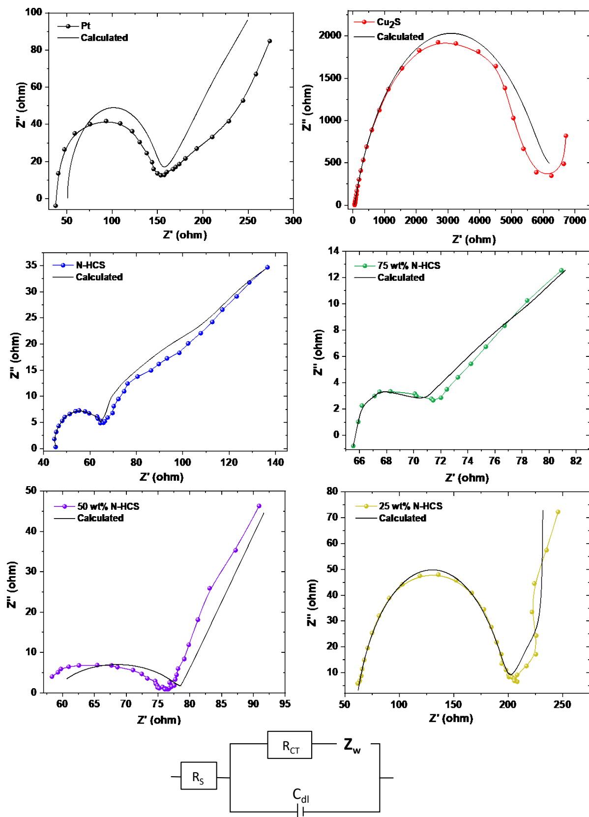
Figure 5.10: Nyquist plots of EIS for the symmetric cells with their electrochemical equivalent circuit for Pt, \text{Cu}_2\text{S} , N-HCS, 75 wt% N-HCS, 50 wt% N-HCS, and 25 wt% N-HCS.
