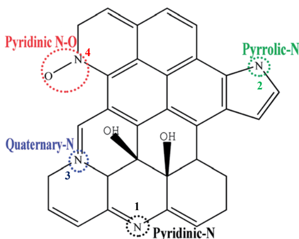
Figure 3.2: Nitrogen atom configurations in carbon materials: (1) pyridinic-N, (2) pyrrolic-N, and (3) quaternary-N [31].
