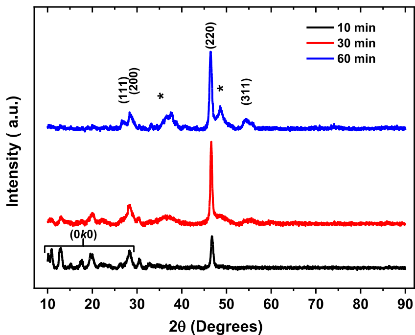
Figure S4.2: XRD pattern of as-synthesized copper sulfide particles at various reaction times of 10, 30, and 60 min using Cu(acac) 2 as a Cu precursor.
