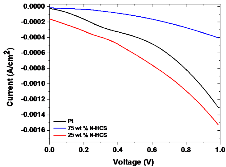
Figure 5.12: Current-voltage characteristic curves for the DSSCs of Pt, 75 wt% N-HCS, and 25 wt% N-HCS.
