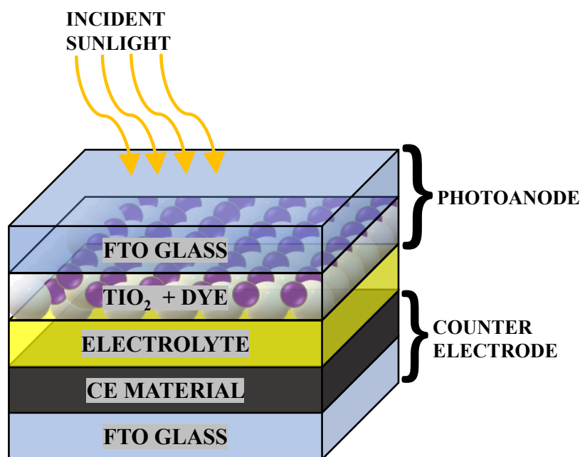
Figure 5.3: Structure of an assembled DSSC for current-voltage analysis of solar cell.
