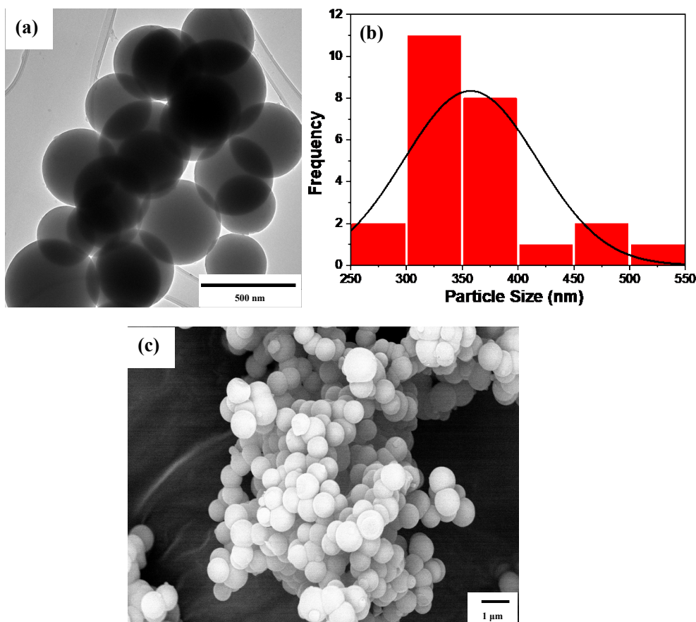
Figure 3.5: Pristine silica (a) TEM micrograph, (b) particle size distribution (extracted from a low magnification image) and (c) SEM micrograph.
