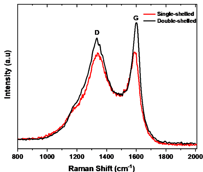
Figure 3.14: Raman spectra of single and double-shelled mesoporous hollow carbon spheres.
