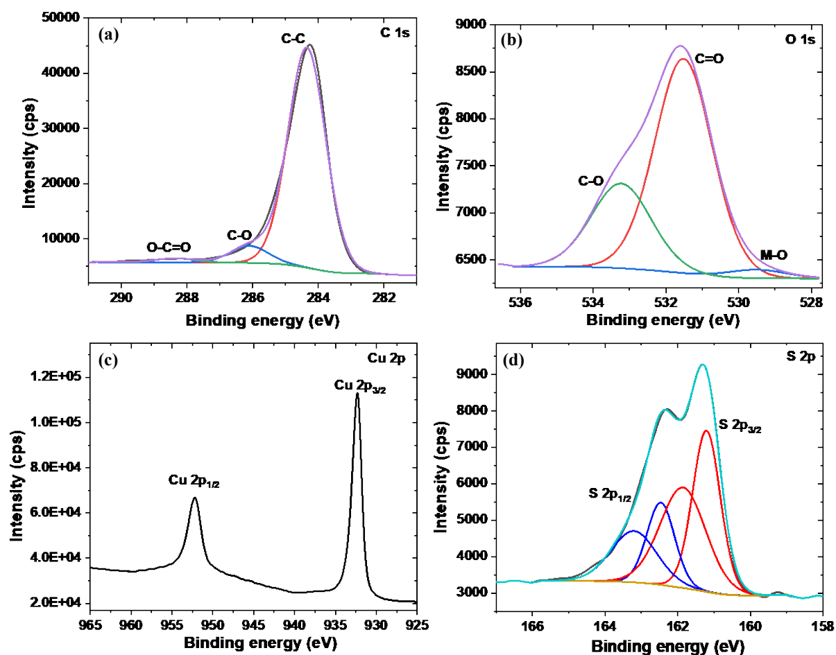
Figure 5.7: High resolution XPS spectra of (a) C 1s, (b) O 1s, (c) Cu 2p and (d) S 2p for the 75 wt% N-HCS composite.
