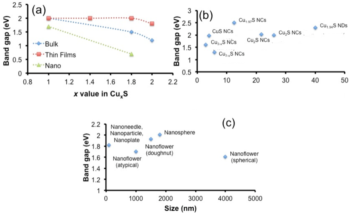
Figure 2.9: Graphs (a-c) show bandgap dependence of copper sulfides with composition, size, and shape of nanostructures [104].
