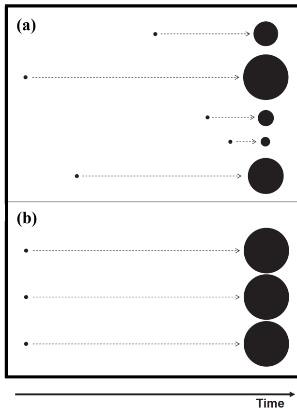
Figure 4.14: Diagram illustrating different reaction systems when nucleation occurs (a) at random and (b) all at once, and how the nuclei (•) grows with increased reaction time [48].
