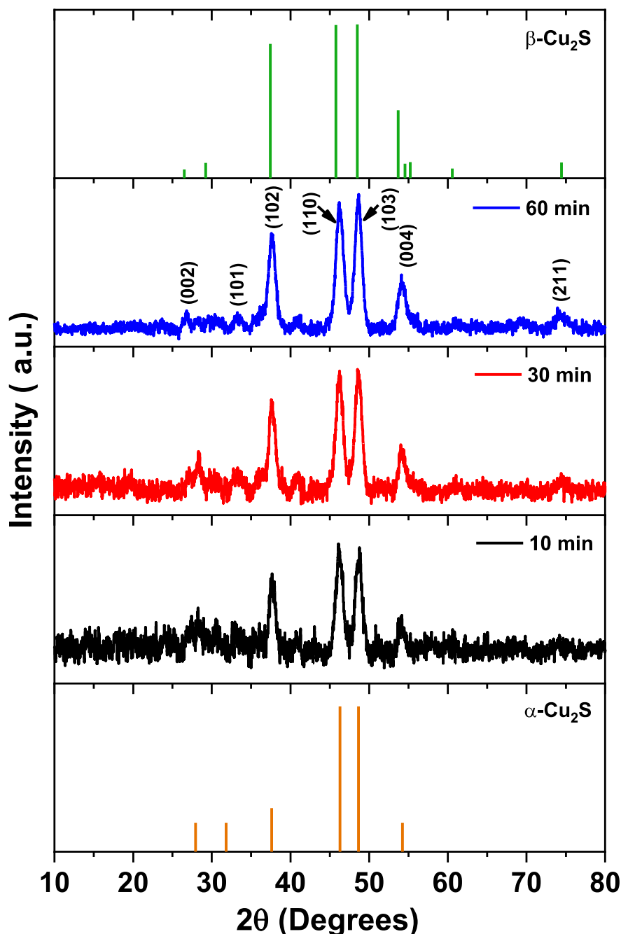
Figure 4.11: Powder X-ray diffraction patterns for as-synthesized \text{Cu}_{2-x}\text{S} particles at different reactions times and the corresponding peak matching PXRD spectra for \alpha and \beta \text{Cu}_2\text{S} .
