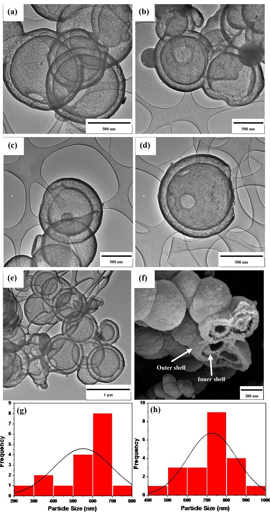
Figure 3.12: Double-shell mesoporous hollow carbon spheres micrographs (a-e) TEM, (f) SEM, and (g-h) the particle size.
