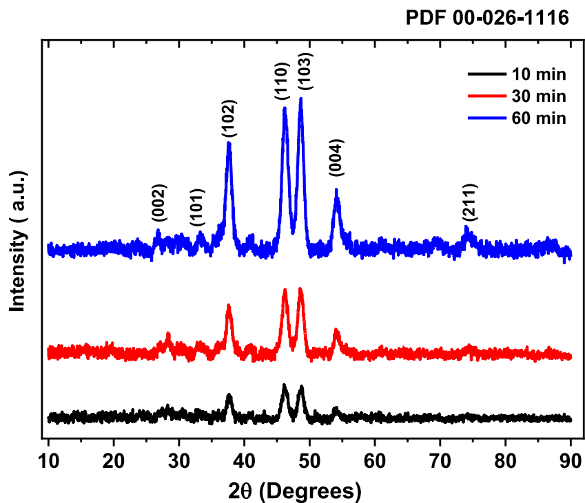
Figure S4.1: XRD pattern of as-synthesized copper sulfide particles at various reaction times of 10, 30, and 60 min using CuCl as a Cu precursor.
