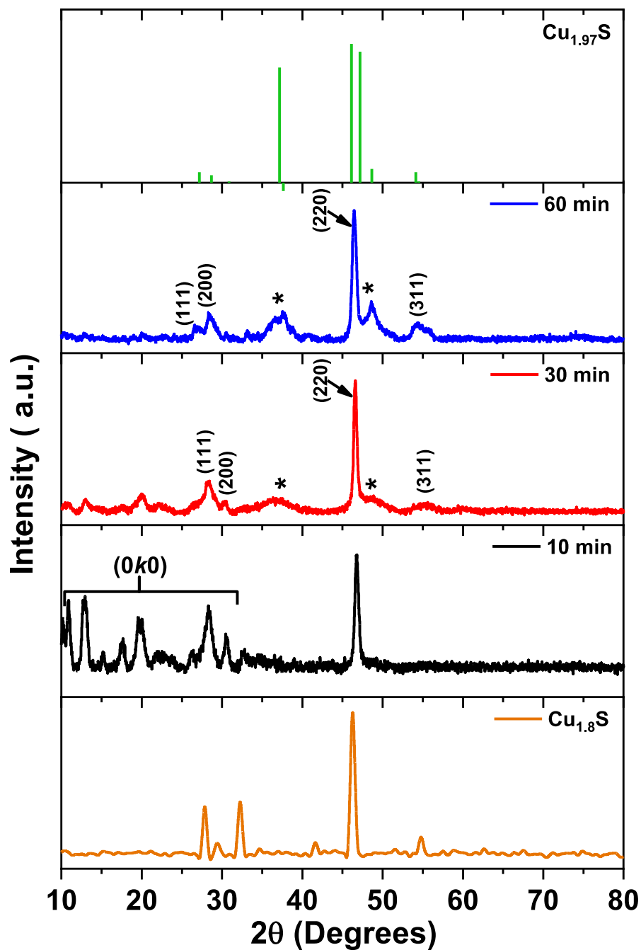
Figure 4.4: Powder X-ray diffractogram patterns for synthesized \text{Cu}_{2-x}\text{S} particles at different reaction times (10, 30, and 60 min) with the corresponding peak matching PXRD spectra for \text{Cu}_{1.97}\text{S} and from the XRD database, \text{Cu}_{1.8}\text{S} (JCPDS 622980).
