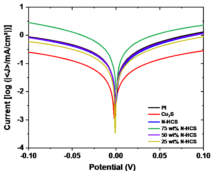
Figure 5.11: Tafel plot of the Pt and the synthesized materials: Cu_2S , N-HCS, 75 wt% N-HCS, 50 wt% N-HCS, and 25 wt% N-HCS.
