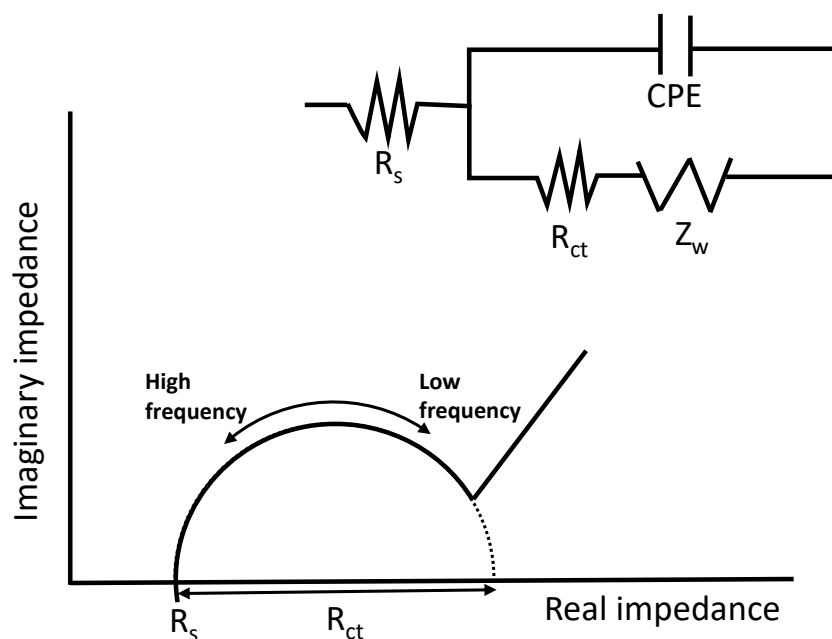
Figure 2.14: An example of a Nyquist plot with an inset of the equivalent circuit for fitting the electrochemical impedance spectroscopy (EIS) data.
