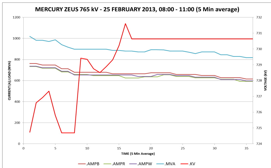
Figure 6.4: Mercury – Zeus 765 kV transmission line system parameters – 25/2/2013
