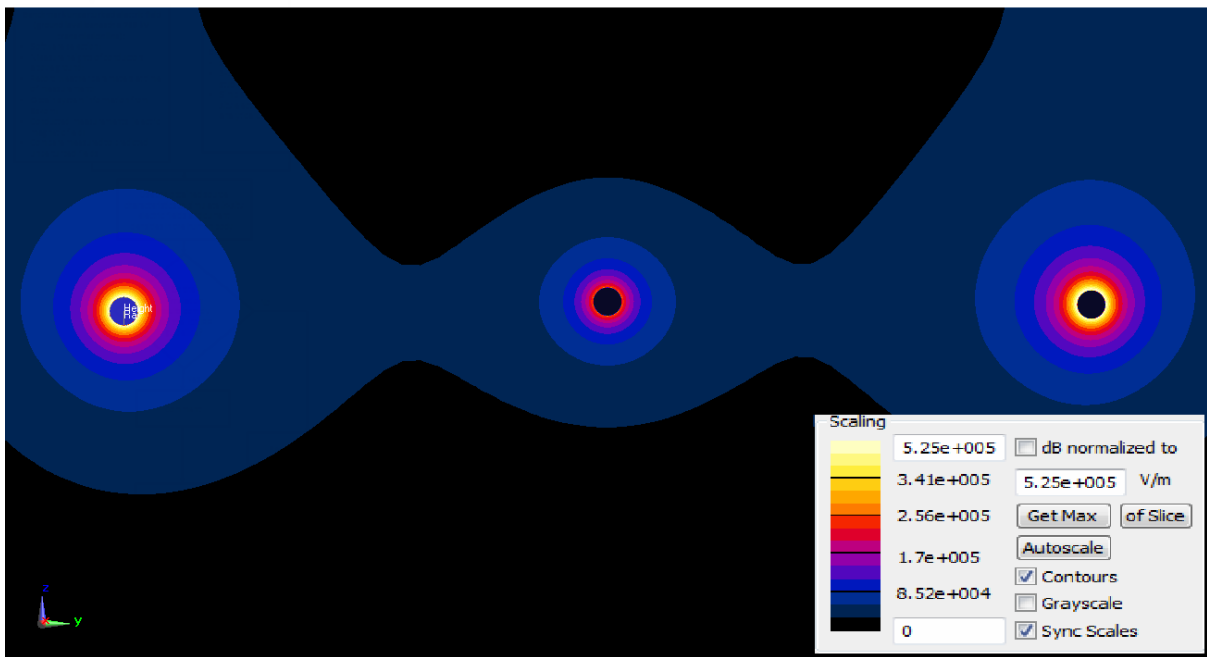
Figure 5.5: Sliced electric field plot of a 765 kV line displayed in electric field strength referenced to 5.25 \times 10^5 V/m
