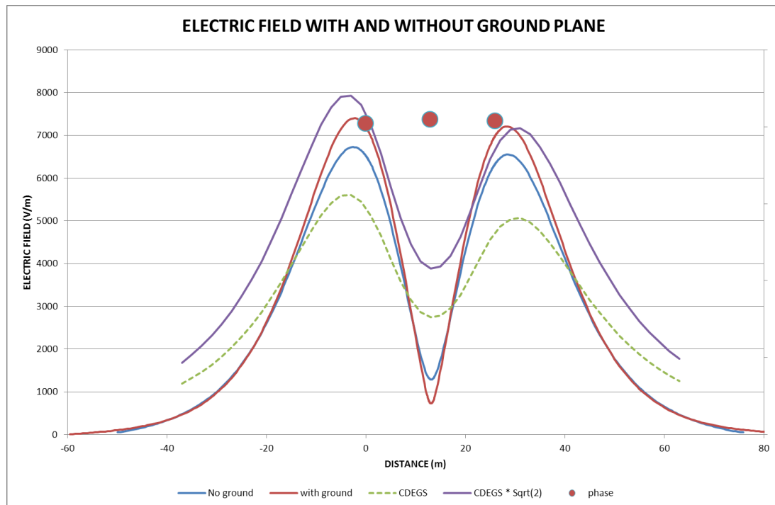
Figure 5.8: Electric field comparison with CDEGS
