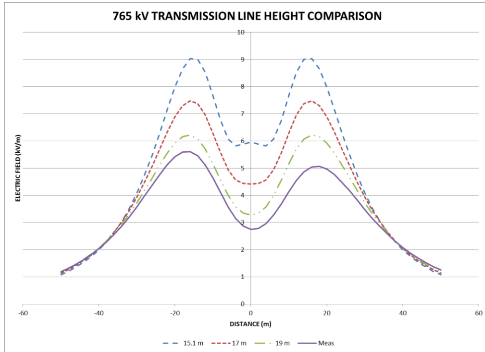
Figure 7.7: Electric field comparison with varied height comparisons
