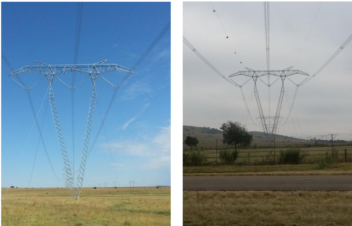
Figure 6.1: Typical tower geometry for the Mercury – Zeus 765 kV transmission line
