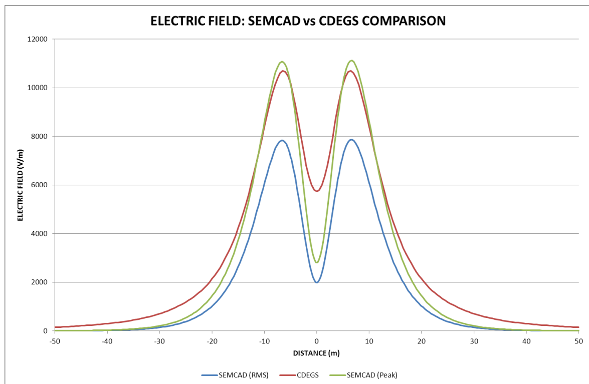
Figure 5.2: Electric field comparison of CDEGS and SEMCAD X
