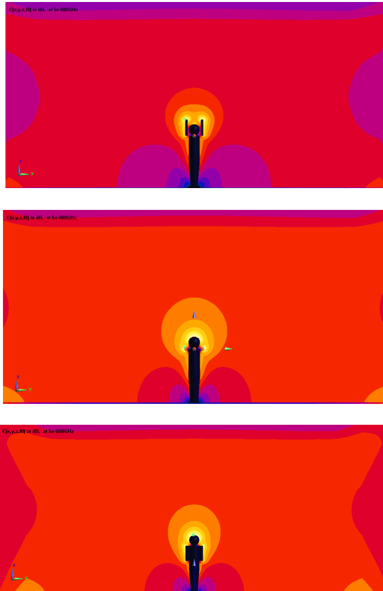
Figure 5.11: Electric field comparison (Top: Arms raised above the head; Middle: Hands raised in-front of the body; Bottom: Arms at the side of the body)
