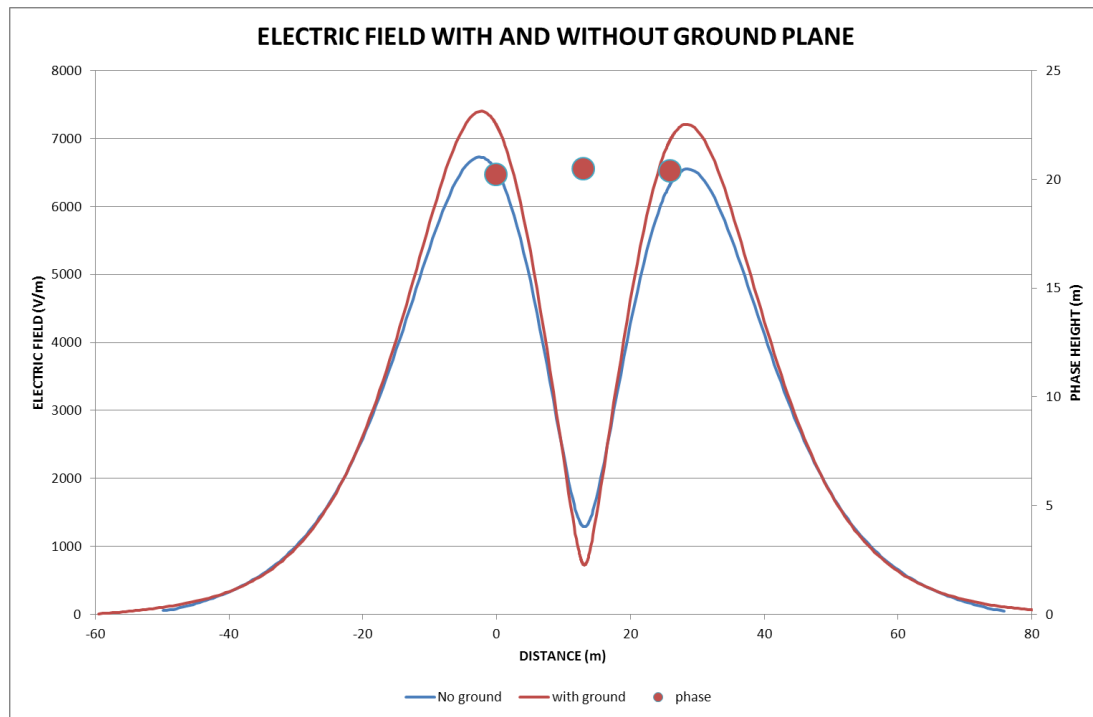
Figure 5.7: Electric field comparison with and without ground plane
