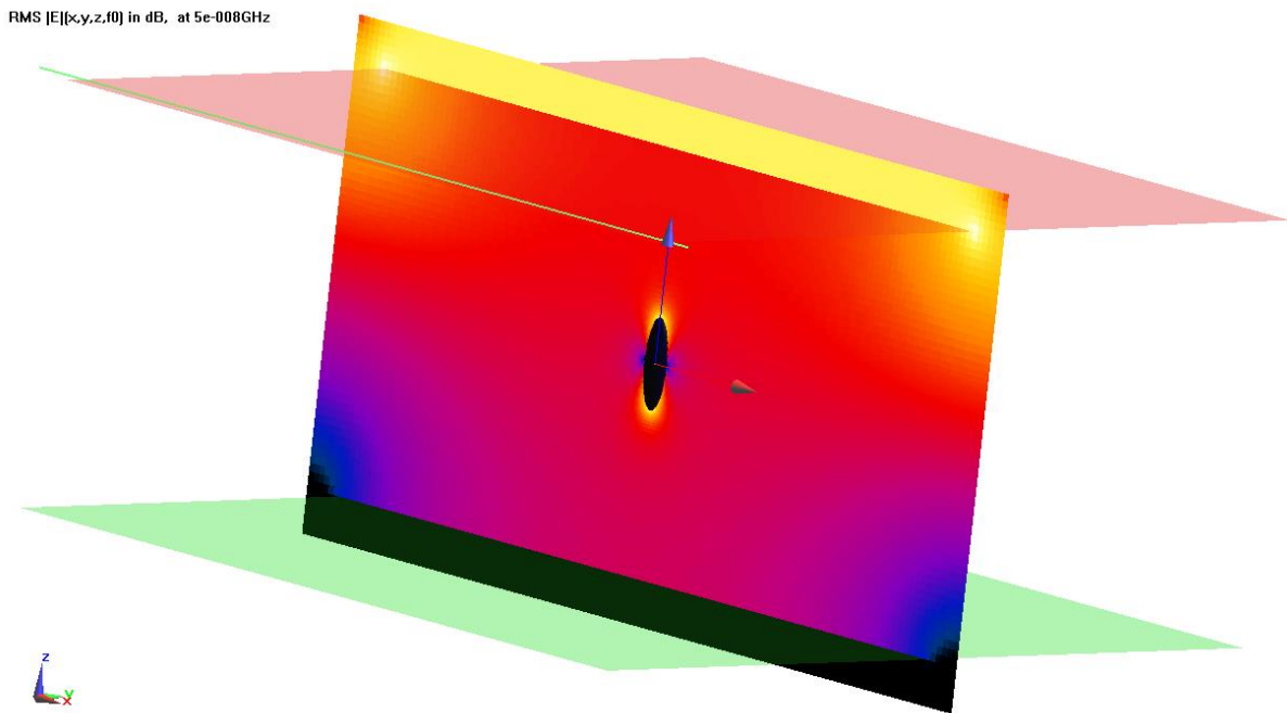
Figure 5.4: Electric field plot of the model with the ellipsoid inserted in the centre of the parallel plates along the X-axis.
