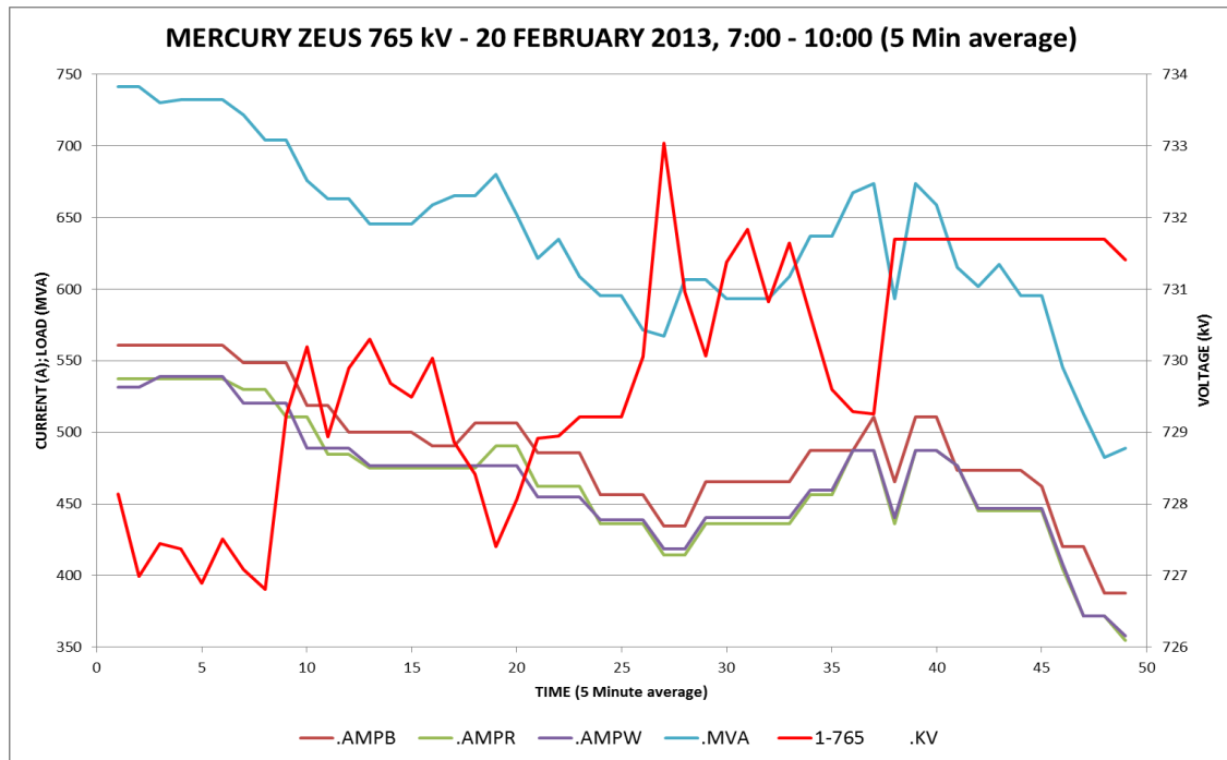
Figure 6.3: Mercury – Zeus 765 kV transmission line system parameters – 20/2/2013
