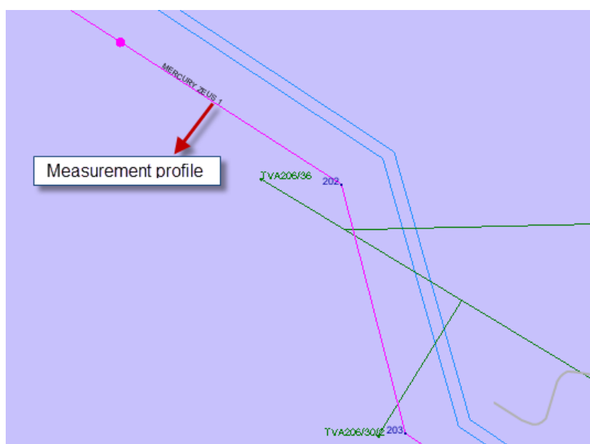
Figure 6.2: Lateral half profile (red arrow) indicating area of measurement beneath the Mercury – Zeus 765 kV transmission line (TXSIS)
