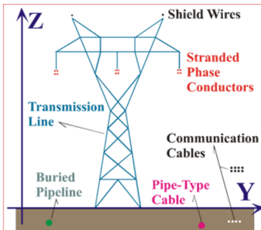
Figure 4.1: Cross-section of transmission line used in SES-EnviroPlus
