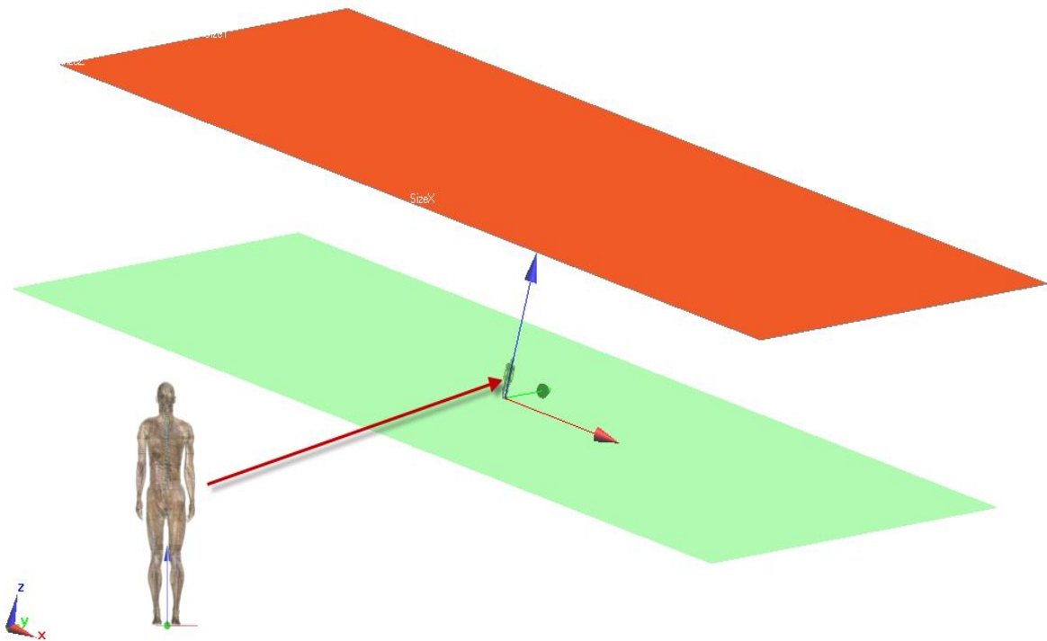
FIGURE C1: Human Exposure Model Used to Calculate the In-situ Electric Field and Current Densities
