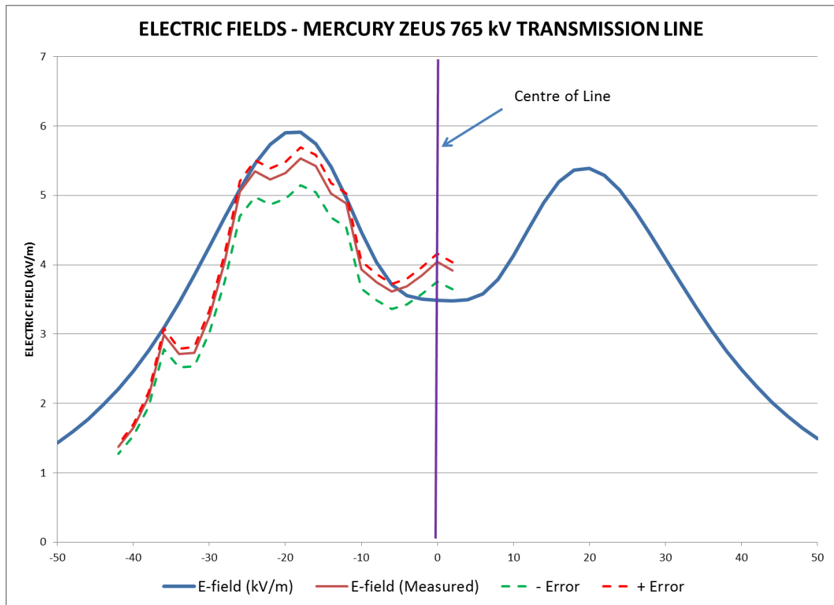
Figure 6.5: Electric fields: Mercury – Zeus 765 kV transmission line (25/2/2013) (computed vs measured)
