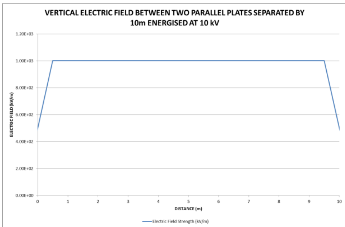
FIGURE C2: Distribution of the Electric Field between the Parallel Plates, Without the Human Body Present. Top: Three Dimensional Model, Bottom: Vertical Electric Field Strength between the Plates
