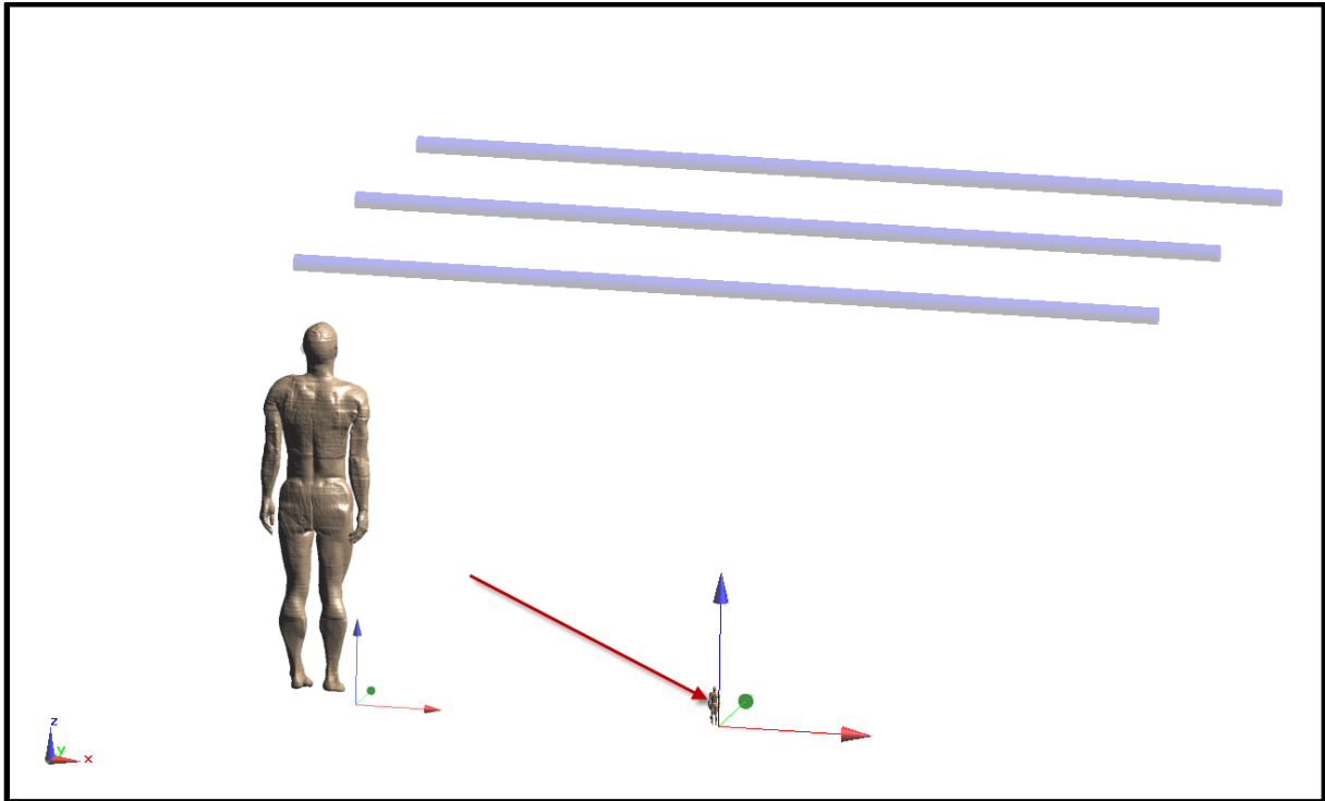
Figure 7.4: Model set-up used for the anatomical modelling of human exposed to 765 kV transmission line
