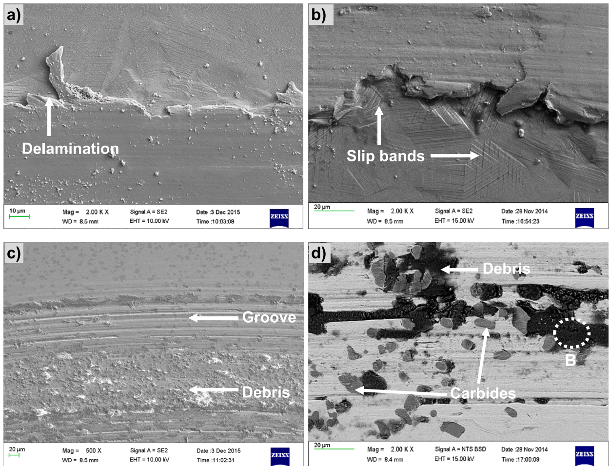
Fig. 11. SEM-SE micrographs of: a) and b) ULTIMET™, showing delamination, slip bands on the surface near the wear track and debris smeared over the grooves, c) SEM-SE and d) SEM-BSE micrographs of STELLITE™ 6B, showing debris (position B), and the matrix phase removed, leaving carbides above the surface [33].
