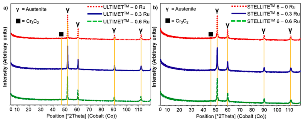
Fig. 3. XRD patterns of: a) ULTIMET™, and b) STELLITE™ 6 powders with 0, 0.3 and 0.6 wt% Ru, showing mainly \gamma and \text{Cr}_3\text{C}_2 .
