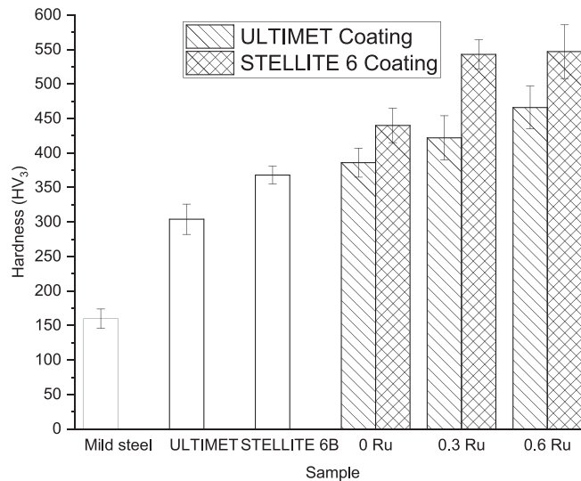
Fig. 6. Hardnesses (HV 3 ) of mild steel substrate, ULTIMET TM and STELLITE TM 6B bulk alloys, and nominal 0, 0.3 and 0.6 wt% Ru ULTIMET TM and STELLITE TM 6 coatings.
