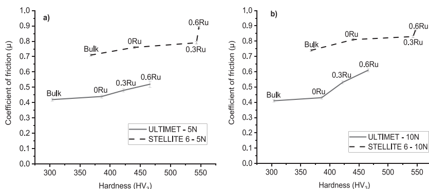
Fig. 16. Relationship between coefficient of friction and hardness of ULTIMET™ and STELLITE™ 6B bulk alloys, ULTIMET™ and STELLITE™ 6 coatings with ruthenium under sliding wear conditions under: a) 5 N and b) 10 N.
