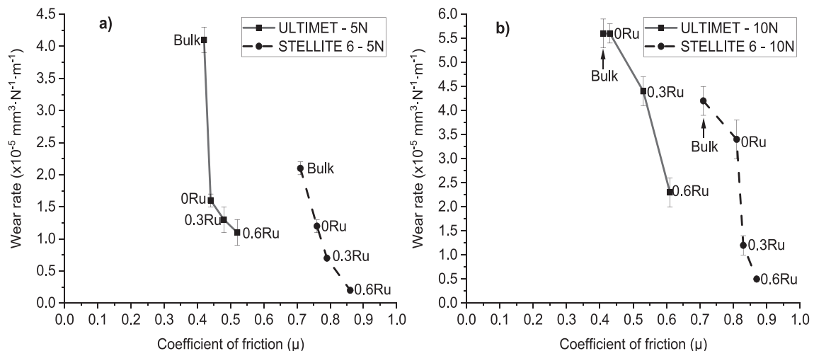
Fig. 14. Relationship between wear rate and coefficient of friction of ULTIMET™ and STELLITE™ 6B bulk alloys, ULTIMET™ and STELLITE™ 6 coatings with ruthenium under sliding wear conditions under: a) 5 N and b) 10 N.
