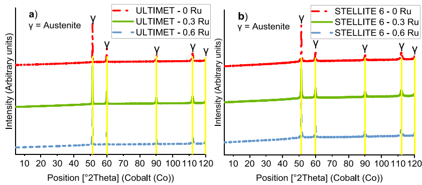
Fig. 5. XRD patterns of: a) ULTIMET TM , and b) STELLITE TM 6 coatings, with 0, nominal 0.3 wt% Ru and nominal 0.6 wt% Ru, showing only fcc ( \gamma ).
