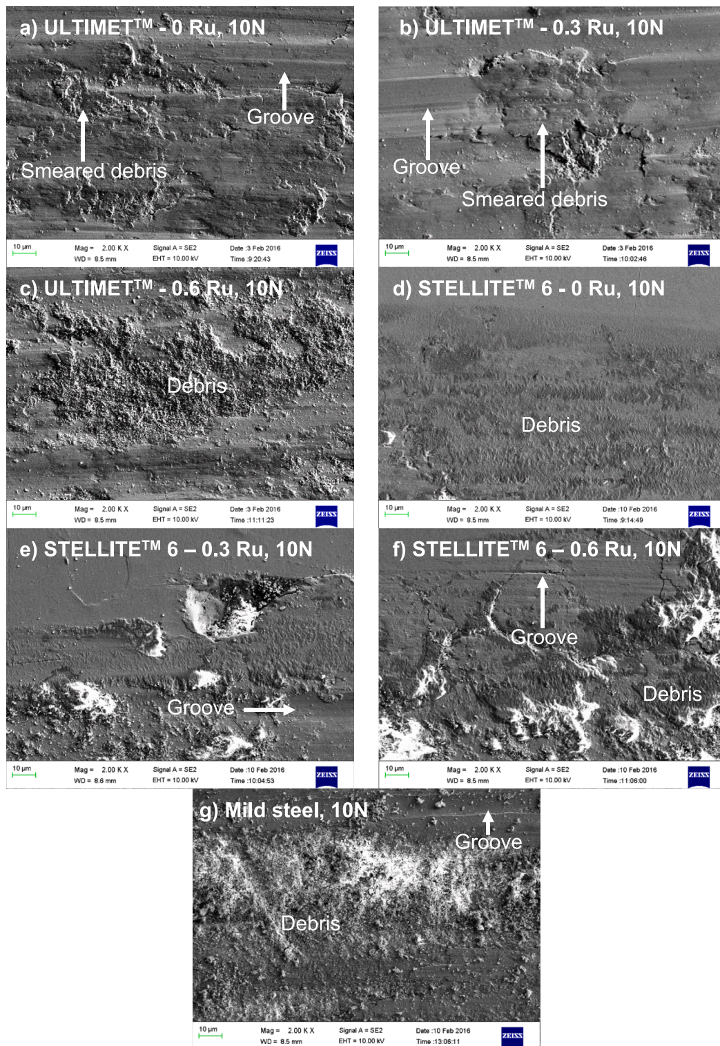
Fig. 13. SEM-SE micrographs of: a)–c) ULTIMET™ and d)–f) STELLITE™ 6 coatings, and after dry sliding wear conditions against 100Cr6 steel balls at 10 N [33].
