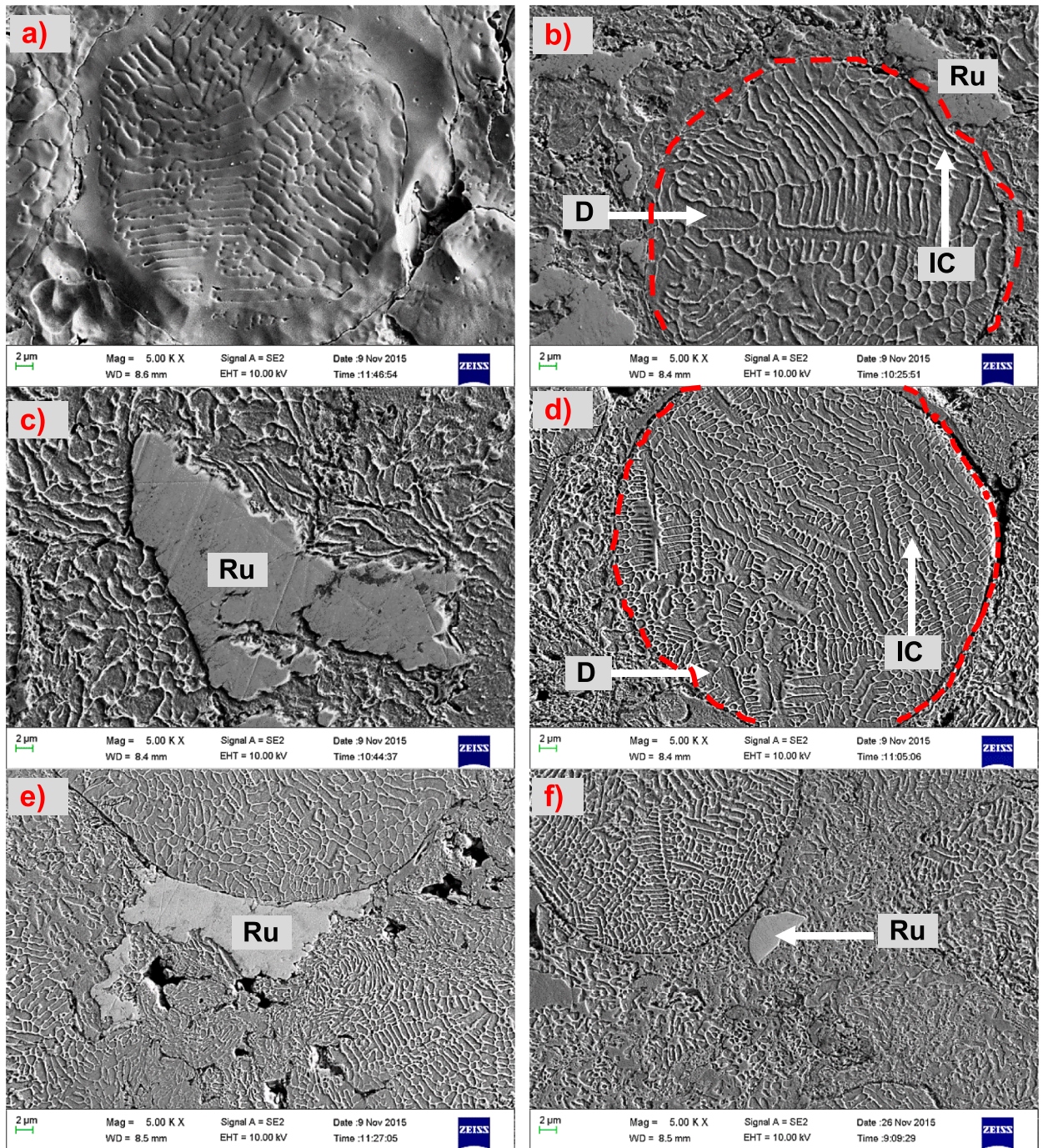
Fig. 4. SEM-SE micrographs showing the top surfaces of ULTIMET™ coatings with: a) 0 Ru, b) 0.3 wt% Ru, and c) 0.6 wt% Ru and STELLITE™ 6 coatings with: d) 0 Ru, e) 0.3 wt% Ru [33], and f) 0.6 wt% Ru, all with dendrites (D) and interdendritic carbides (IC).
