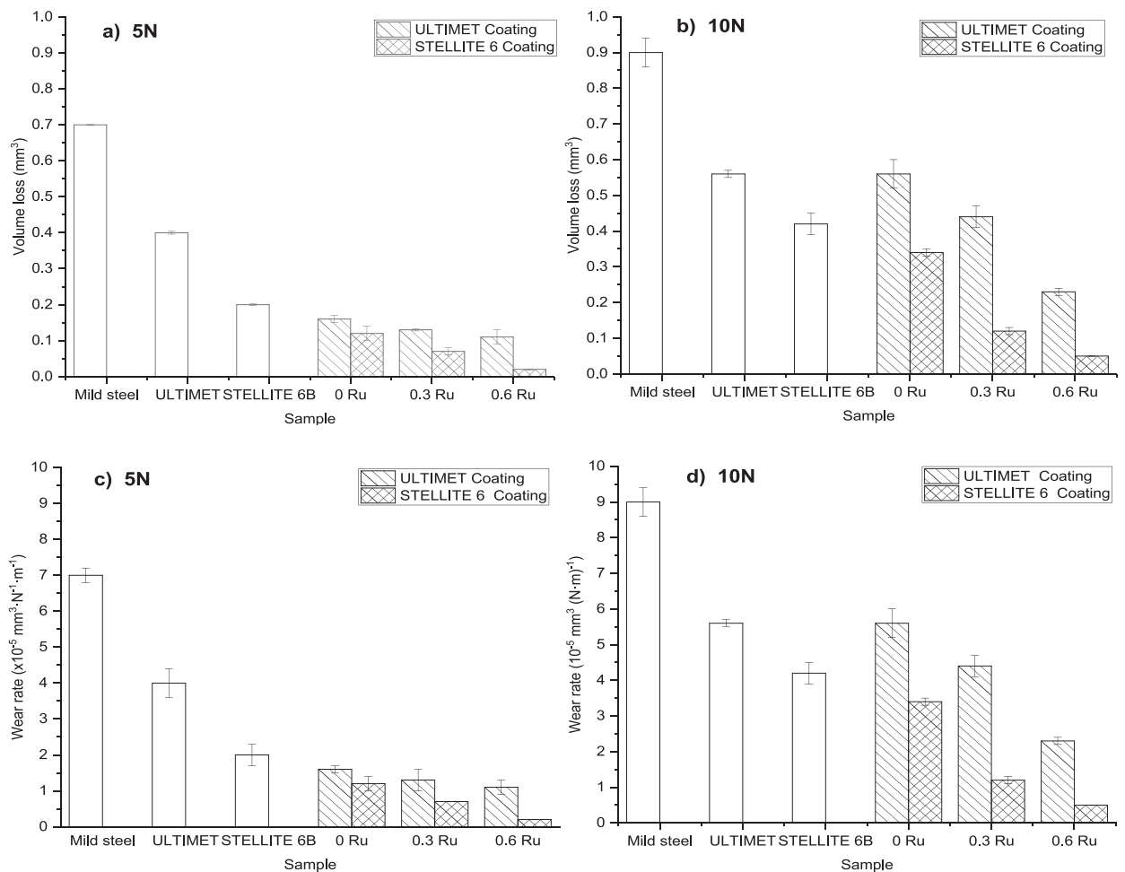
Fig. 9. Wear results for mild steel, ULTIMET™ and STELLITE™ 6B bulk alloys, and ULTIMET™ and STELLITE™ 6 coatings under sliding wear conditions: a) volume loss for 5 N load, b) volume loss for 10 N load, and c) wear rates for 5 N load, and d) wear rates for 10 N load.
