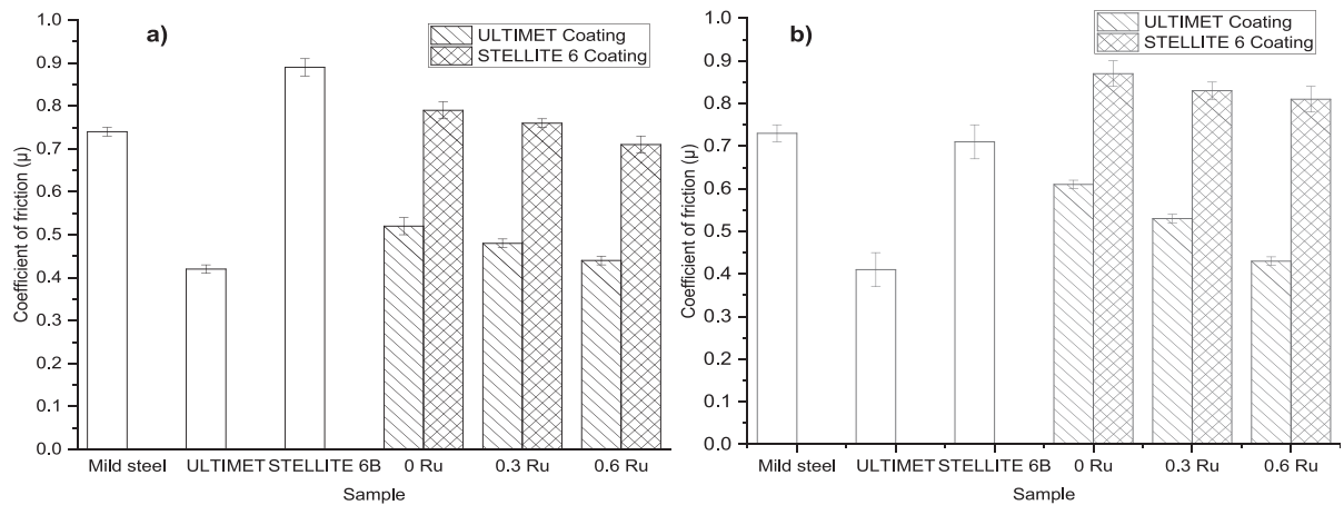
Fig. 8. Average coefficients of friction of mild steel, ULTIMET™ and STELLITE™ 6B bulk alloys, and ULTIMET™ and STELLITE™ 6 coatings at: a) 5 N, and b) 10 N loads [33].
