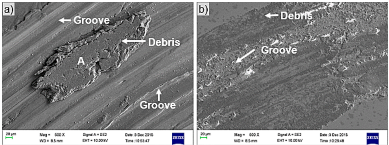
Fig. 10. SEM-SE micrographs after ball-on-disc sliding wear of: a) ULTIMET™, showing fairly long continuous grooves, and debris smeared on the surface (position A), and b) STELLITE™ 6B, showing much debris on the wear track [33].
