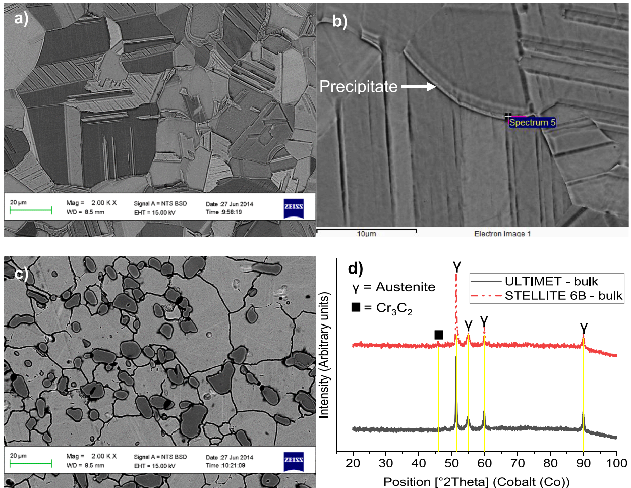
Fig. 1. SEM-BSE micrographs of the alloys: a) ULTIMET™, showing γ grains and twins, b) a higher magnification micrograph of ULTIMET™, showing narrow grain boundary precipitates [33], c) STELLITE™ 6B, showing twins in the γ grains and carbides in the matrix and at the grain boundaries, and d) XRD patterns of the alloys, showing γ-austenite and Cr 3 C 2 phases [33].
