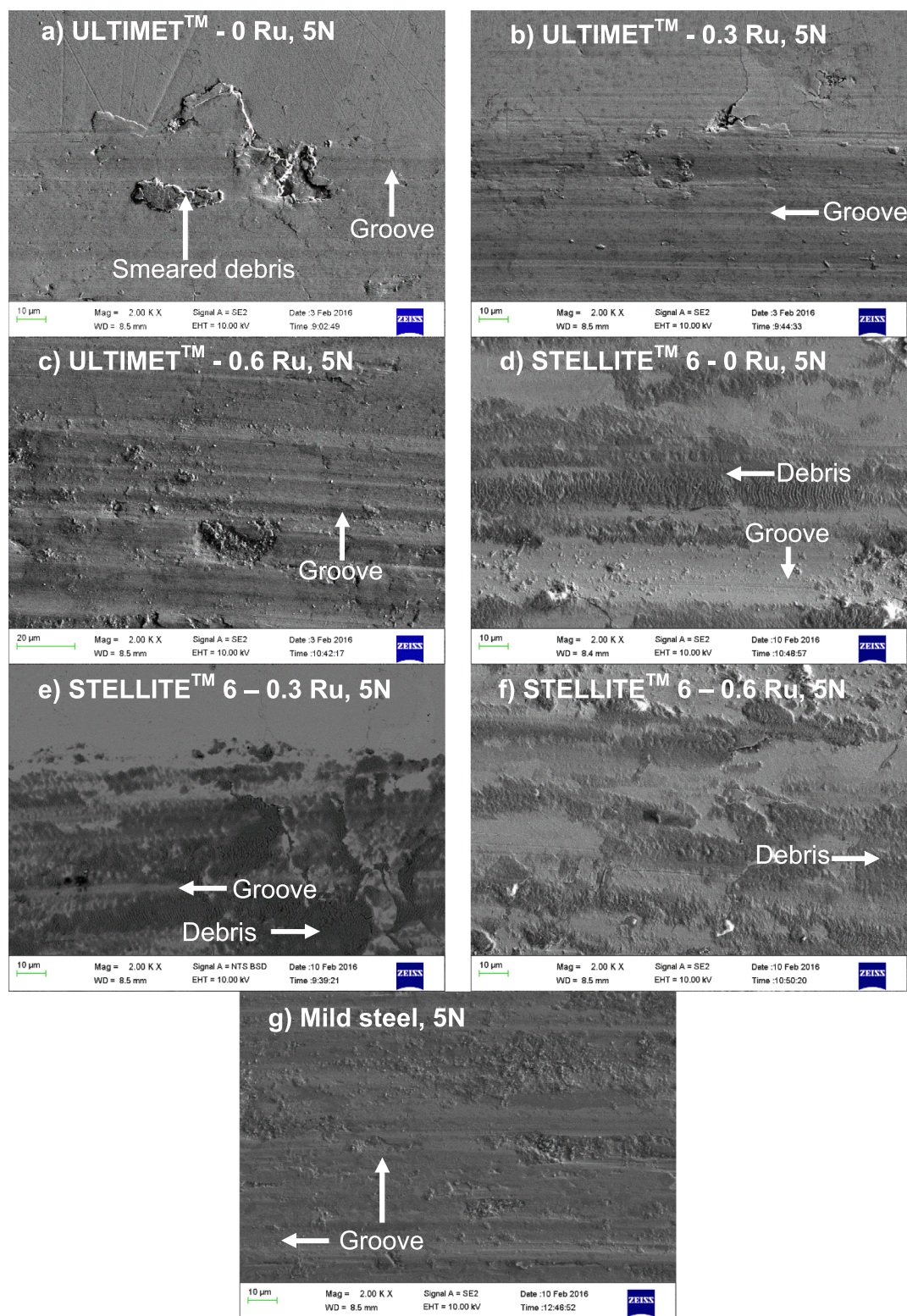
Fig. 12. SEM-SE micrographs of: a)–c) ULTIMET™ and d)–f) STELLITE™ 6 coatings and g) mild steel after dry sliding wear conditions against 100Cr6 steel balls at 5 N [33].
