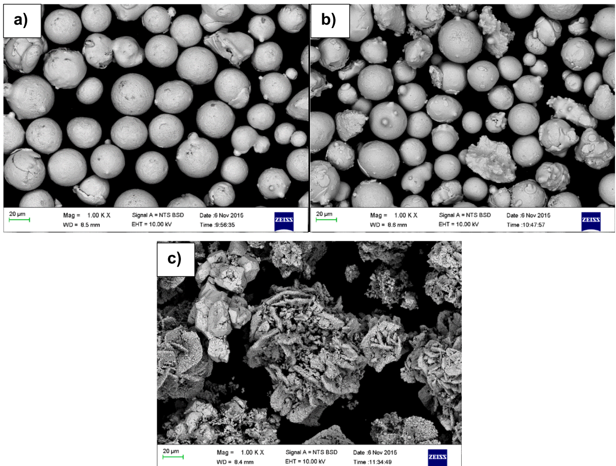
Fig. 2. SEM-BSE images showing powders of: a) ULTIMET™ [33], b) STELLITE™ 6 nominal 0.6 wt% Ru [33], and c) ruthenium [33].
