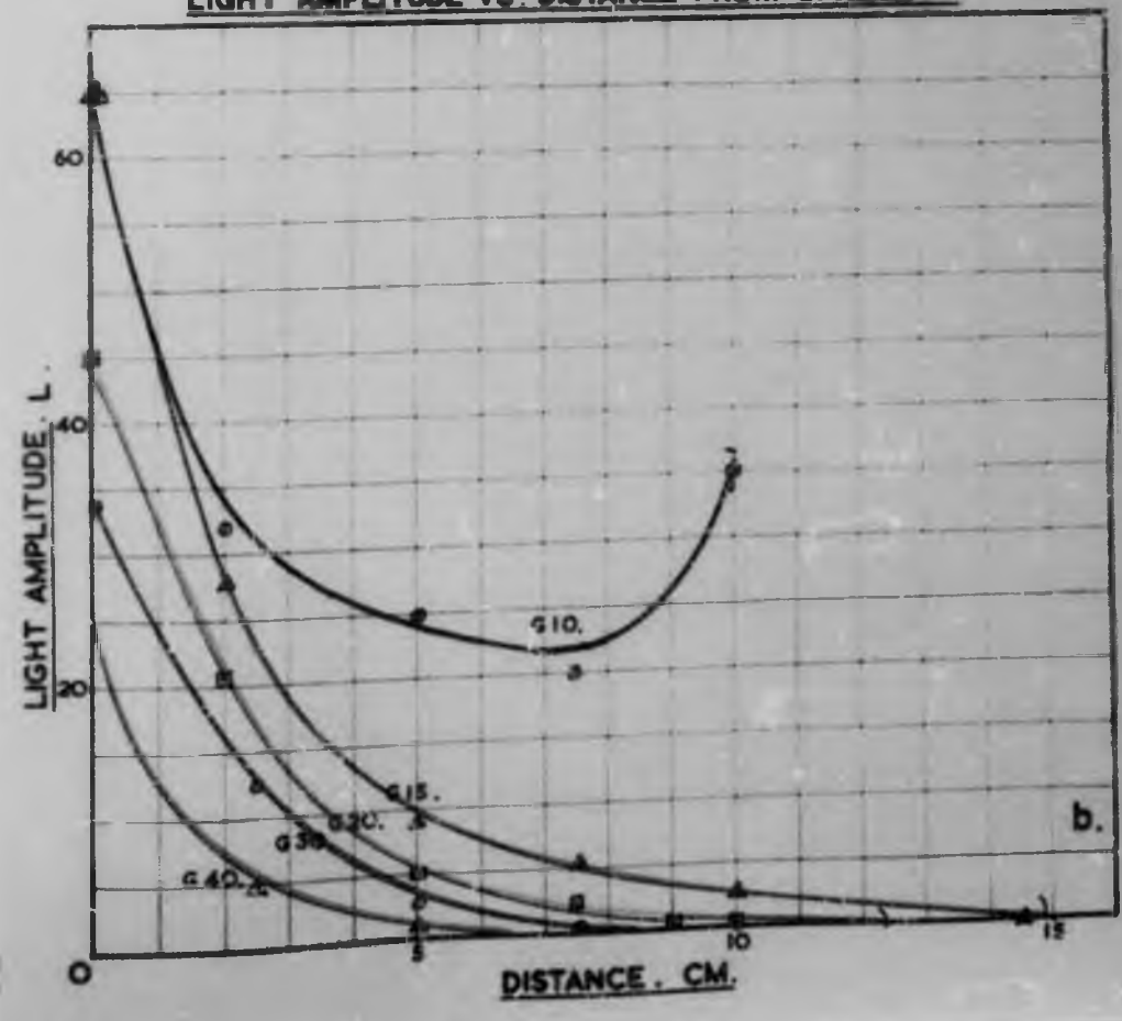
LIGHT AMPLITUDE VS. DISTANCE FROM SPHERE.
