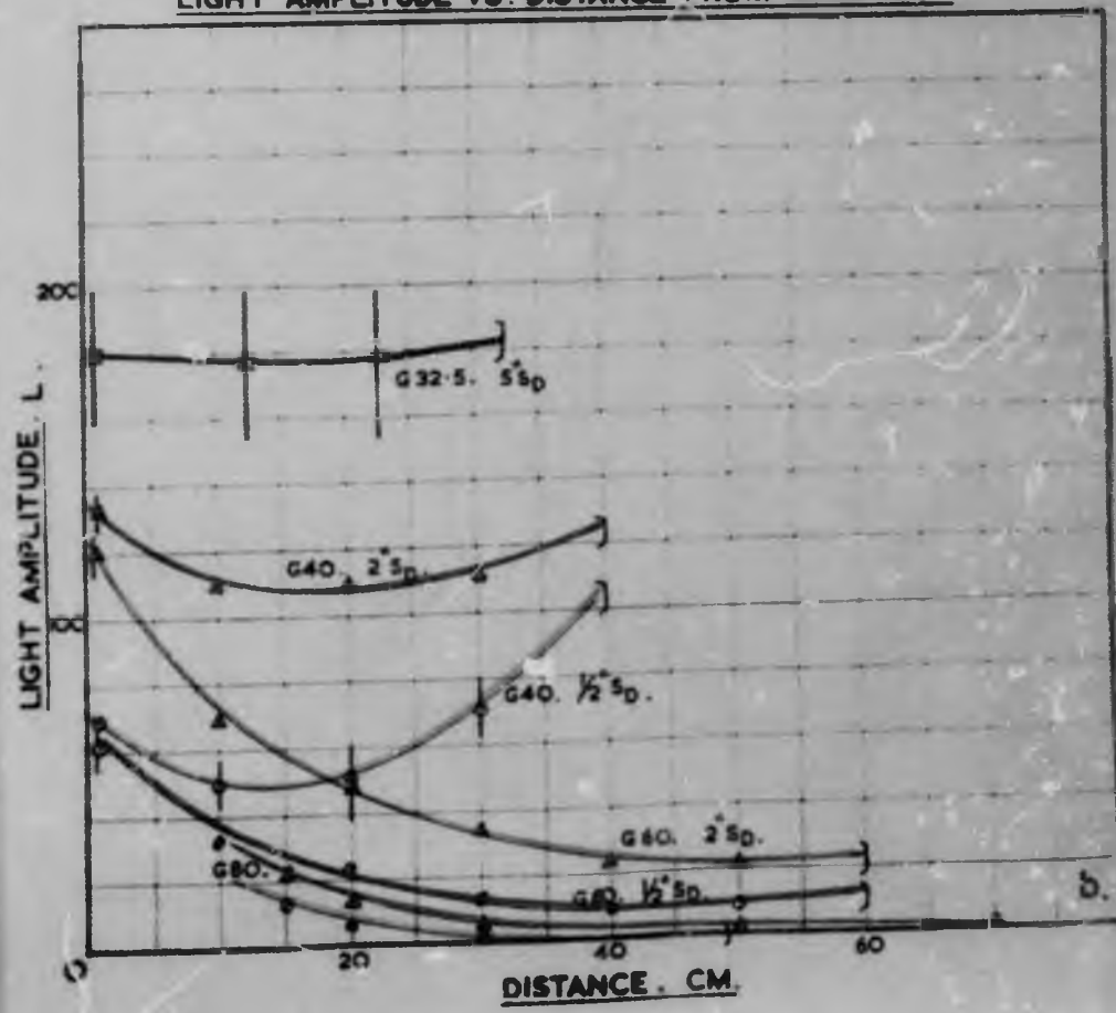
LIGHT AMPLITUDE VS. DISTANCE FROM SPHERE
