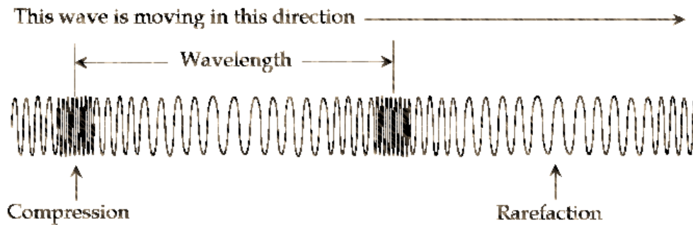
Figure 6.3 Longitudinal Wave from BCSE Science.com 2-Waves
