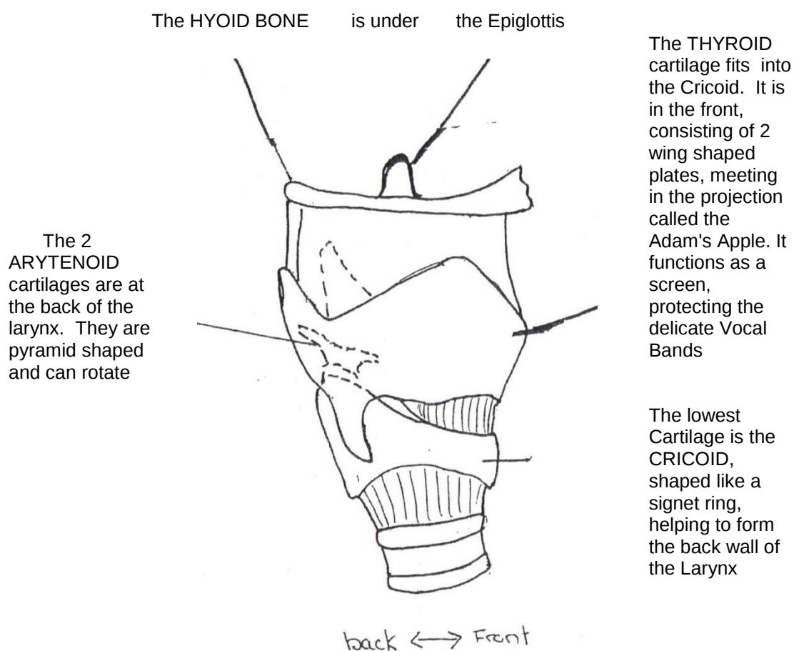
Figure 6.7 Side View of the Larynx
