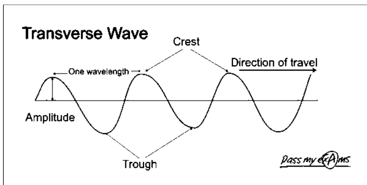
Figure 6.2 A Transverse wave Image from 'Pass my Exams – GCSE Physics
