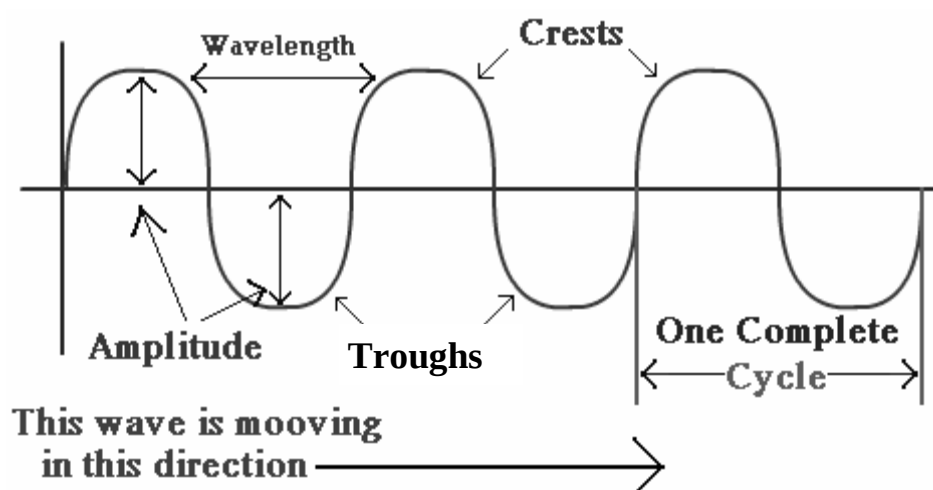
Figure 6.5 Sine curve showing Amplitude (Tutorvista.com)
