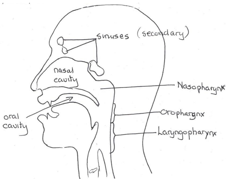
Figure 6.9 The basic areas of resonance (Own composite after Colson, Eisenson.)
