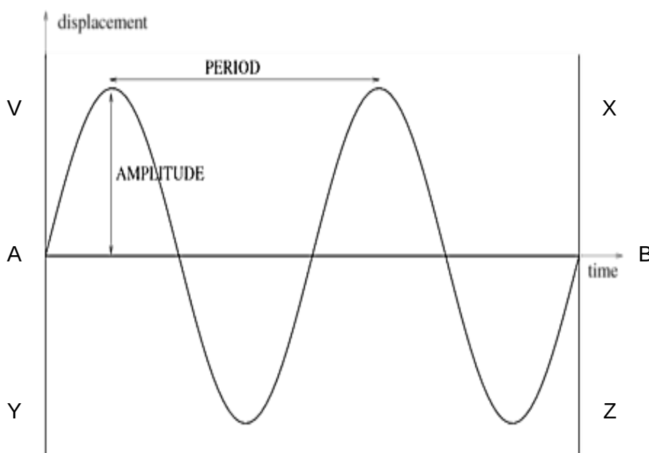
Figure 6.1 Sine Curve, after 'Pass my Exams – GCSE Science- Waves' using lettering added by writer
