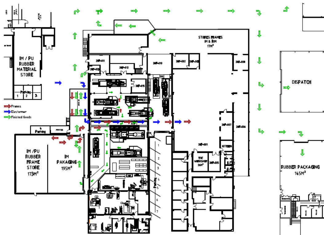
Figure 2 - Factory Layout / Process Flow
