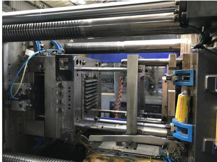
Figure 3 - Mould Showing the Machine Tooling
