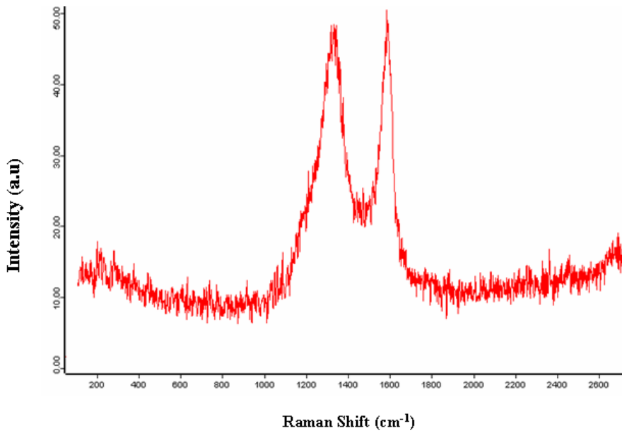
Figure 4.4: Raman Spectra of pristine MWCNTs
