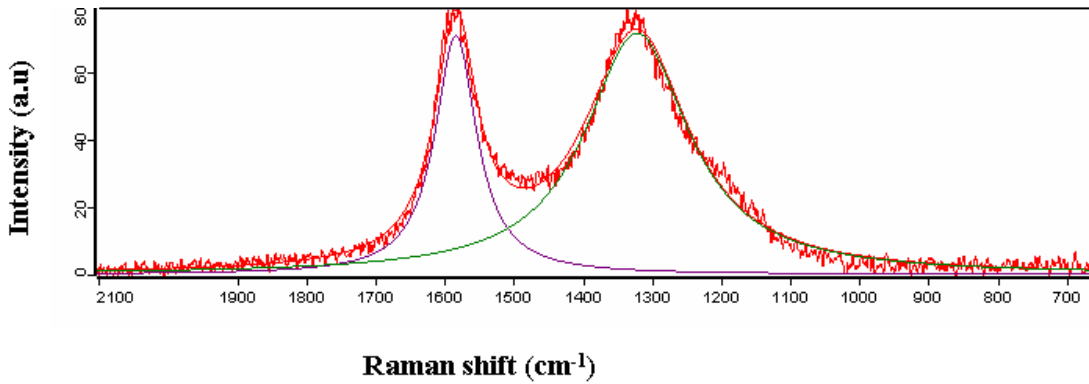
Figure 4.7: Curve fitting results of 30% nitric acid oxidized CNTs
