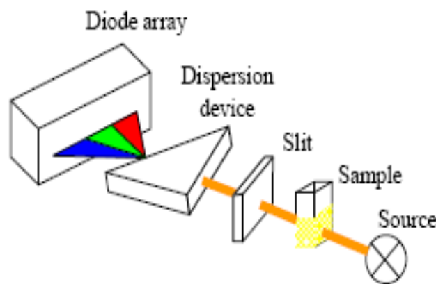
Figure 2.10: Optical density measuring technique (Jomdecha & Prateepasen et al., 2006)
