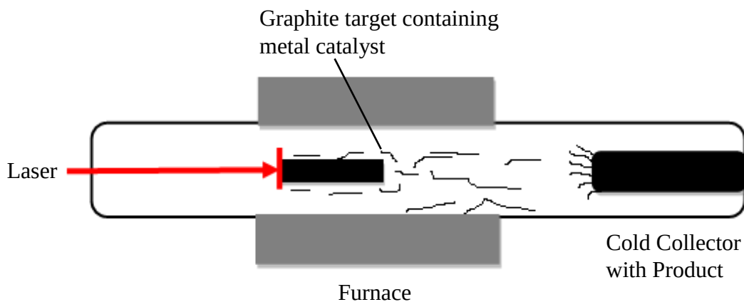
Figure 2.4: A schematic of a pulsed laser deposition reactor (Sinnott & Andrews, 2001)
