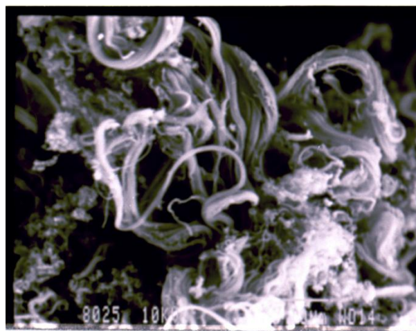
Figure 4.17 SEM Micrograph of 1:3 HNO 3 :H 2 SO 4 oxidised MWCNTs with 10µm scale bar
