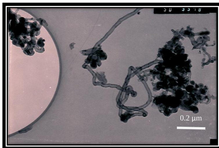
Figure A6.1: TEM micrograph of pristine MWCNTs
