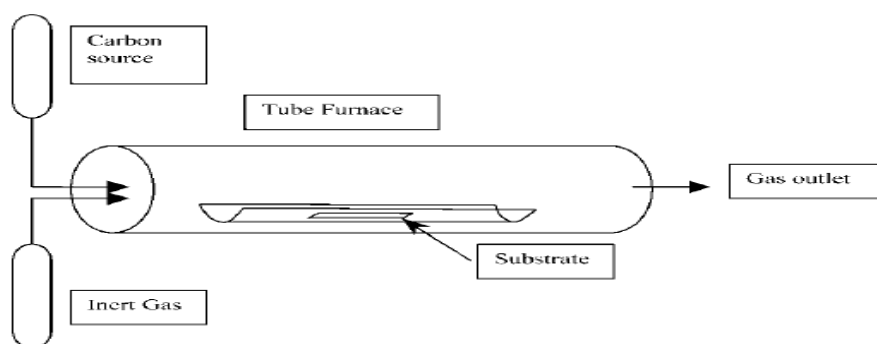
Figure 2.6: Schematic of a typical thermal CVD
