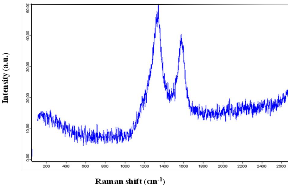
Figure 4.8: Raman spectra of 1:3 HNO 3 :H 2 SO 4 oxidized CNTs
