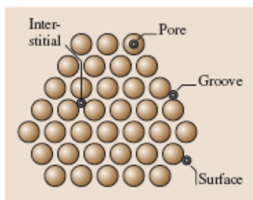
Figure 2.2: Illustration of the four different adsorption sites on a SWCNT bundle (Bhushan, 2004)
