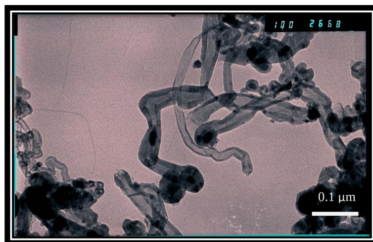
Figure A6.3: TEM micrograph of pristine MWCNTs where scale bar corresponds to 0.1 μm
