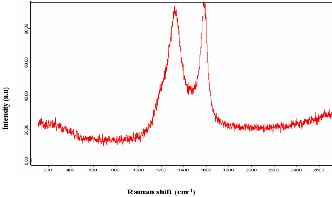
Figure 4.6: Raman spectra of 30% nitric acid oxidised CNTs
