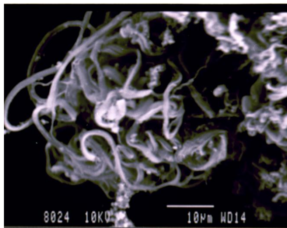
Figure 4.16. SEM Micrograph of 30% HNO 3 oxidised MWCNTs with 10µm scale bar
