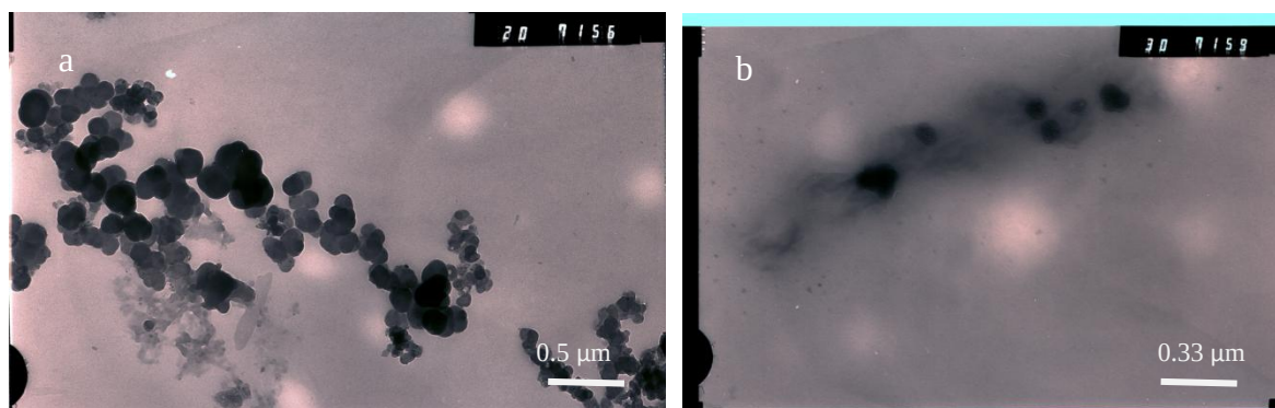
Figure 4.19. Typical TEM image of N-Tritylglycine functionalised MWCNTs. (a) with a 0.5μm scale bar (b) with a 0.33 μm scale bar.
