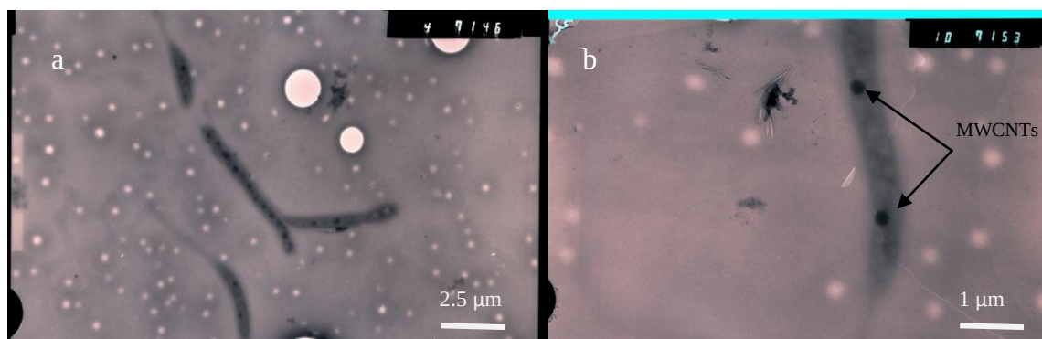
Figure 4.20. Typical TEM micrograph of FITC-MWCNT sample. (a) 2.5 \mu\text{m} scale bar (b) with a 1 \mu\text{m} scale bar.
