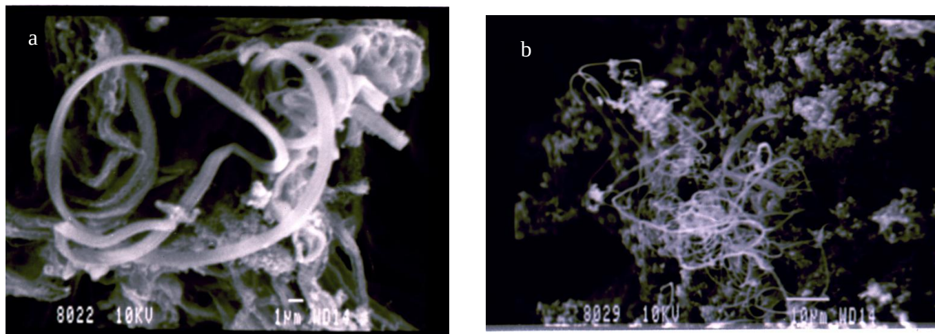
Figure 4.15. Typical SEM Micrograph of pristine MWCNTs. (a) Illustrating MWCNTs with a 1µm scale bar (b) Illustrating MWCNTs with a 10 µm scale bar
