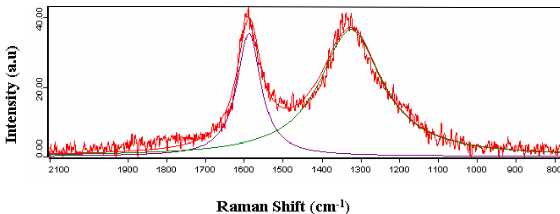
Figure 4.5: Curve fitting results of pristine MWCNTs
