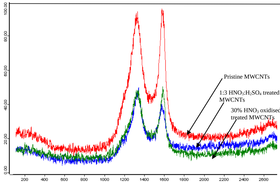
Figure 4.10: Raman spectra of pristine, 30% HNO 3 treated and 1:3 HNO 3 :H 2 SO 4 treated MWCNTs
