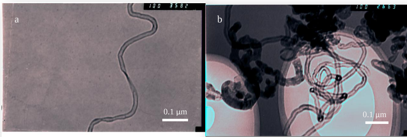
Figure 4.3: Typical TEM micrograph of 30% HNO 3 oxidised MWCNTs. (a) illustrating a single MWCNT with a smooth surface with a 0.1 μm scale bar. (b) illustrating a group of MWCNTs with open ends and smooth surfaces
