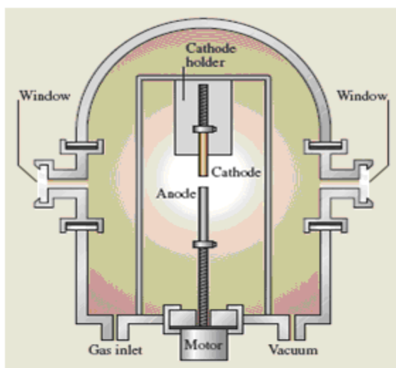
Figure 2.5: Sketch of an electric arc reactor (Bhushan, 2004)
