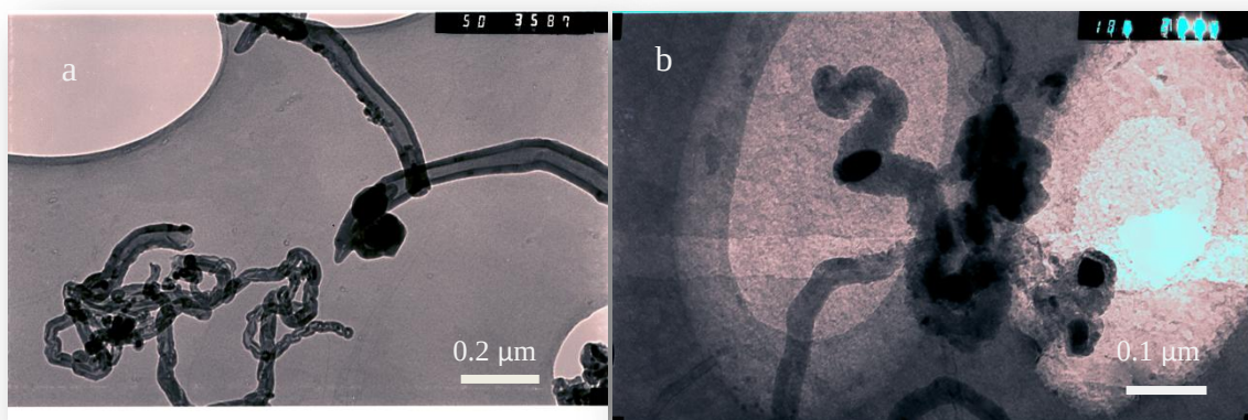
Figure 4.1: Typical TEM micrograph of pristine MWCNTs. (a) illustrating MWCNT with open ends and dark spots indicating metal catalyst at a scale of 0.2 \mu\text{m} . (b) illustrating a MWCNT with metal catalyst at a scale of 0.1 \mu\text{m} .
