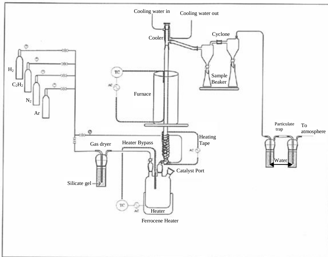
Figure 3.1: Apparatus and SFCCVD Reactor used to produce the MWCNTs (Iyuke, S. S.A. Patent 2101,2005,03438, 2005)
