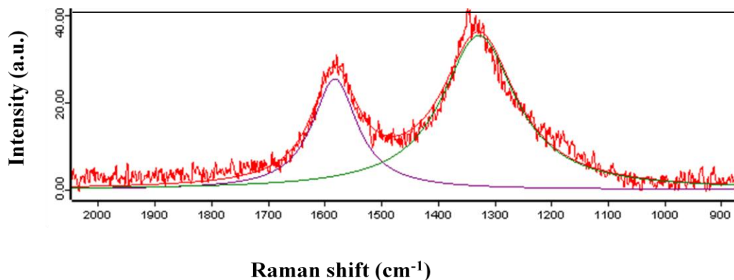
Figure 4.9: Curve fitting results of 1:3 HNO 3 :H 2 SO 4 oxidised MWCNTs
