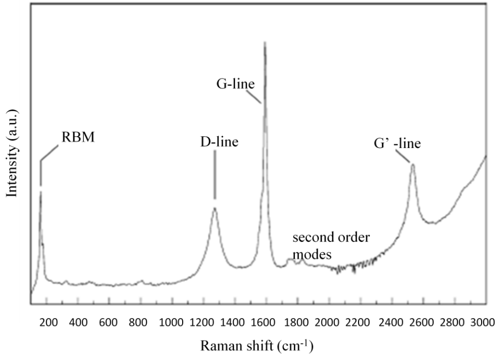
Figure 2.7: Raman spectrum showing characteristic features of CNTs: radial breathing mode (RBM), the D band, G band and G' band (Belin & Epron, 2005)
