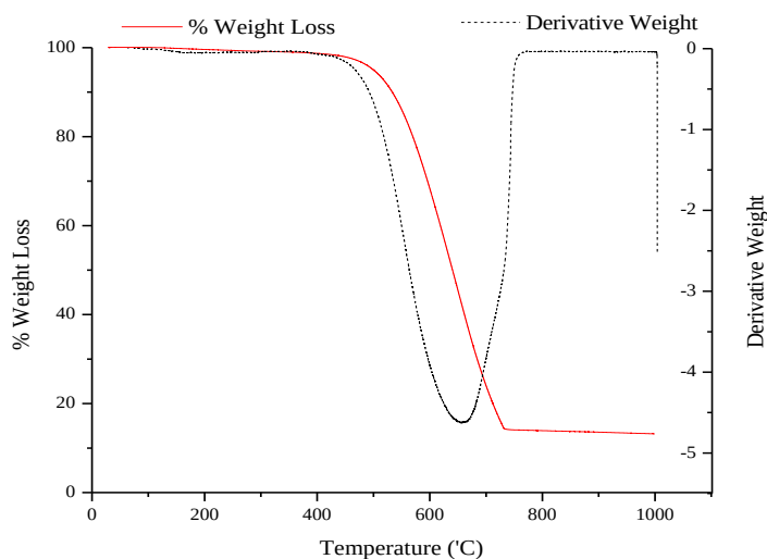
Figure 4.11: Thermal stability of the pristine MWCNTs. The solid line and dashed lines represent TG and DTG curves for the MWCNT samples, respectively
