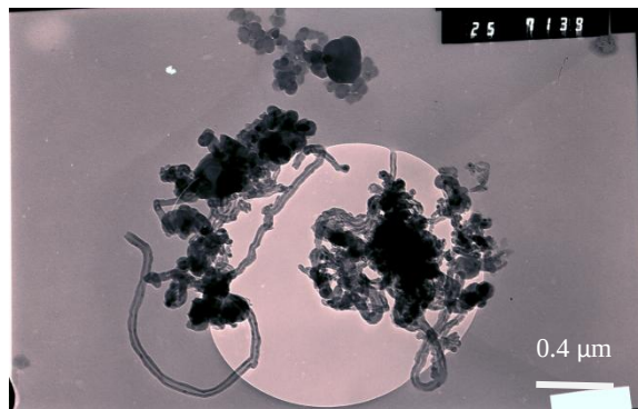
Figure 4.18. Typical TEM image of unreacted MWCNT sample from the 1, 3-dipolar cycloaddition reaction process with 0.4μm scale bar.
