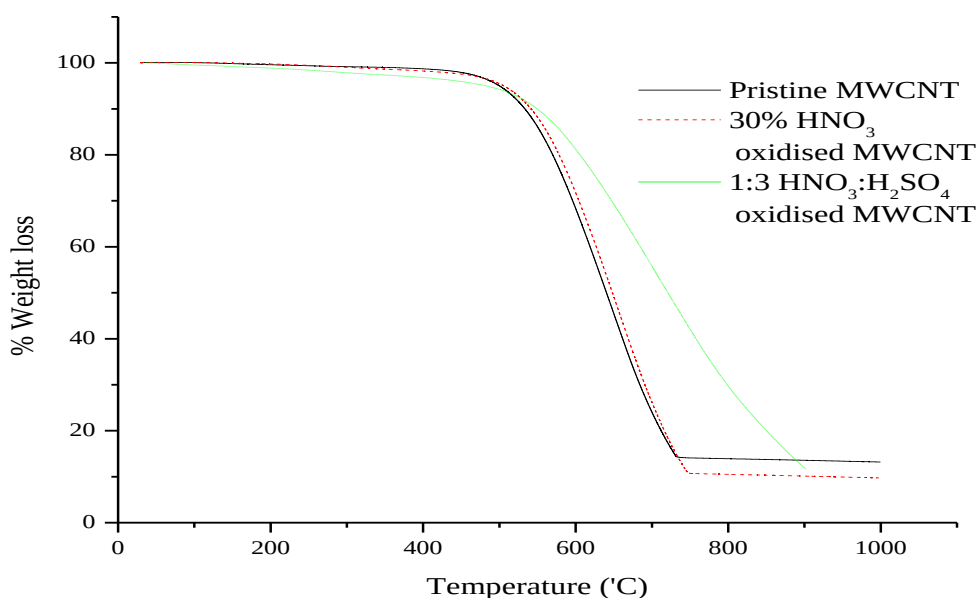
Figure 4.14: Thermal stability of pristine, 30% HNO 3 and 1:3 HNO 3 :H 2 SO 4 oxidised MWCNTs
