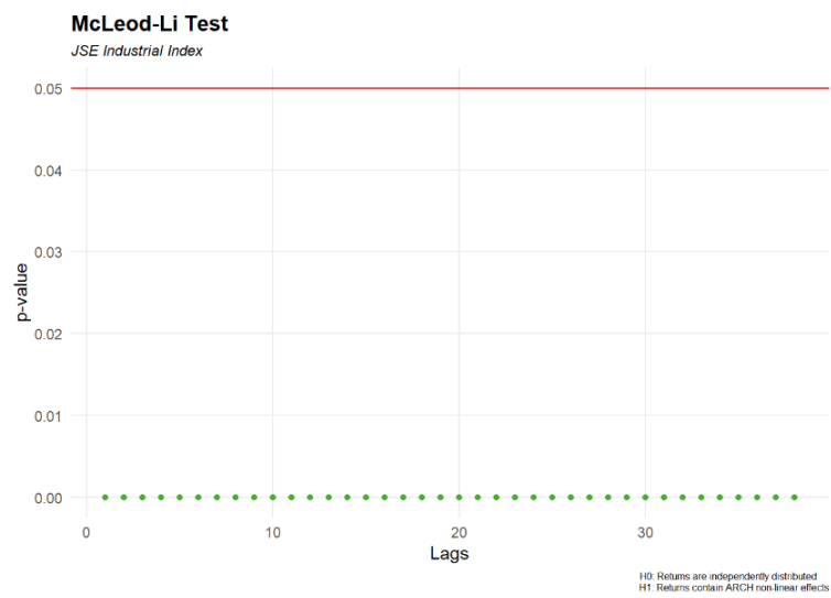
Figure 3: McLeod Li test results on the ind index
