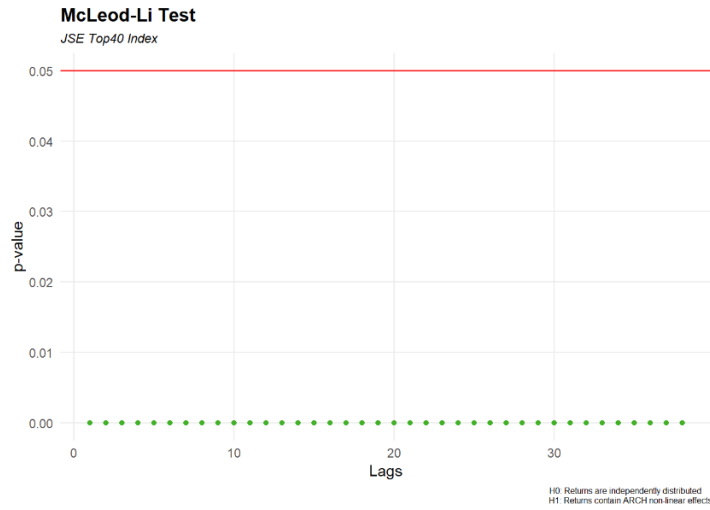
Figure 6: McLeod Li test results on the Top40 index
