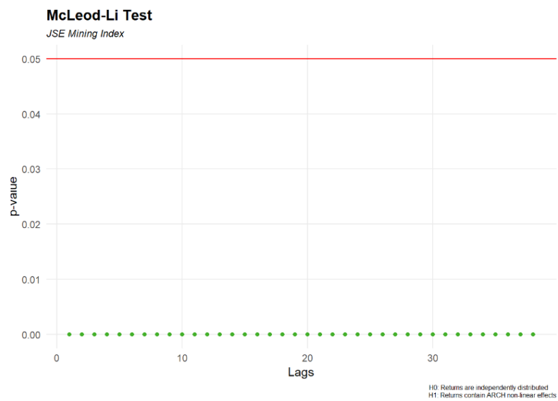
Figure 5: McLeod Li test results on the min index
