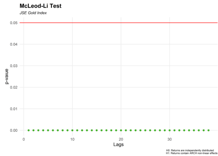
Figure 4: McLeod Li test results on the gold index
