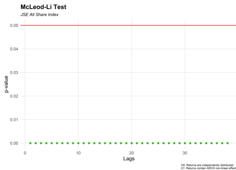
Figure 1: McLeod Li test results on the ALSI
