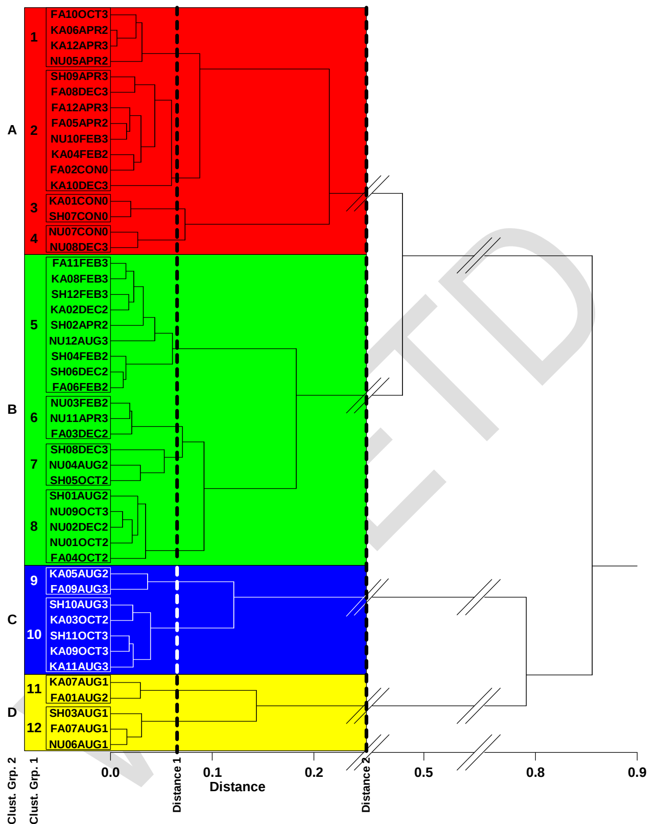
Figure 6-30: Hierarchical cluster tree from a Pearson-Ward cluster analysis on Horn's indices of similarity in structure between Pretoriuskop EBPs in 1996. The codes for the treatment plots are defined in Table 10-1 (p. 214)
