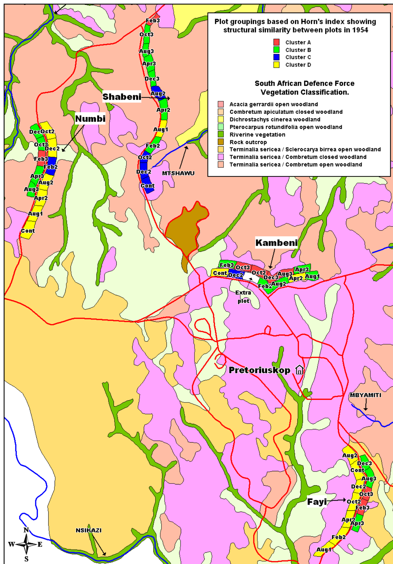
Figure 6-29: Map showing the clustering of the Pretoriuskop EBP plots from a Pearson-Ward cluster analysis on Horn's indices of similarity in structure between plots in 1954 shown in Figure 6-28.
