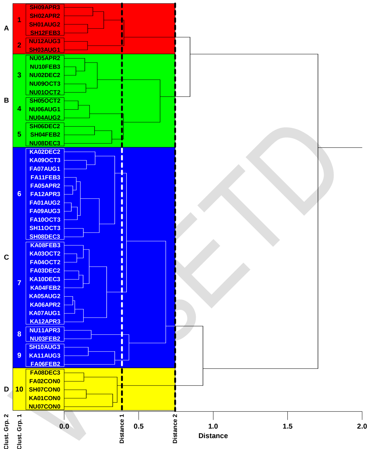
Figure 6-26: Hierarchical cluster tree from a Pearson-Ward cluster analysis on Horn's indices of similarity in species between Pretoriuskop EBPs in 1996. The codes for the treatment plots are defined in Table 10-1 (p. 214)
