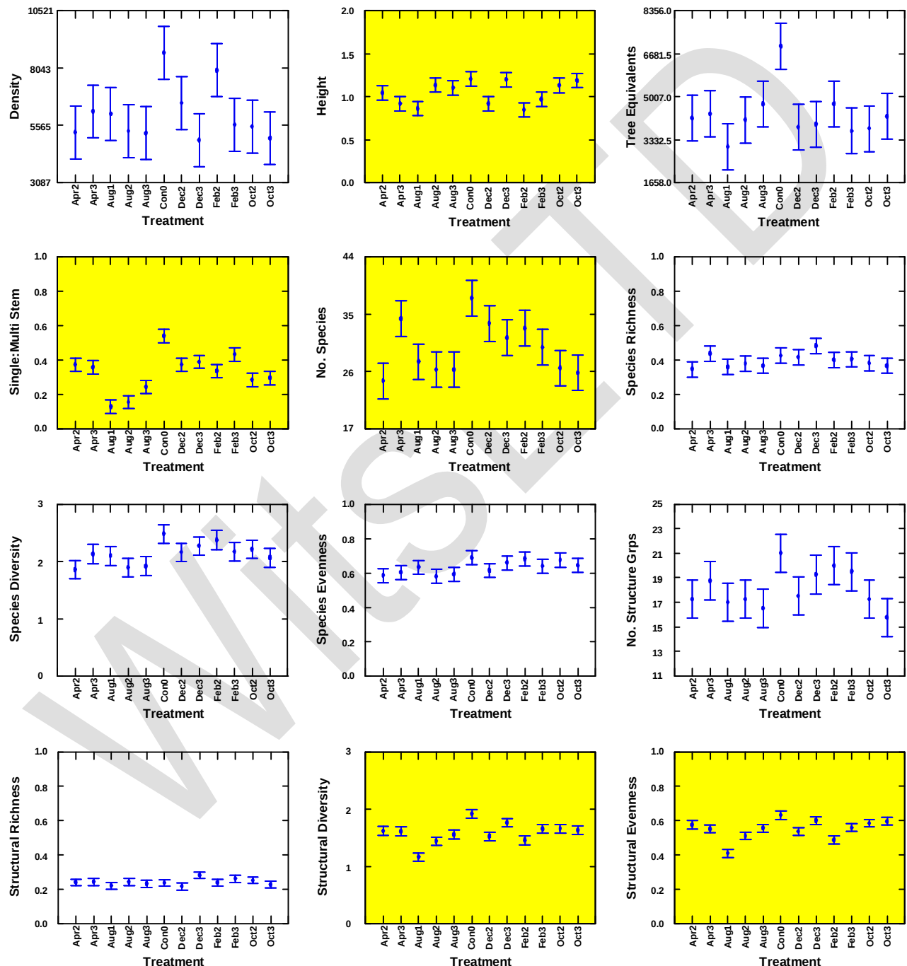
Figure 6-21: The least squares means and standard errors of the vegetation indices from the ANOVA analyses on the 1996 data testing the effect of the different treatments assigned to plots. The colour coding shows the level of the test significance (yellow: \alpha=0.05 , and orange: \alpha = 0.10 ).
