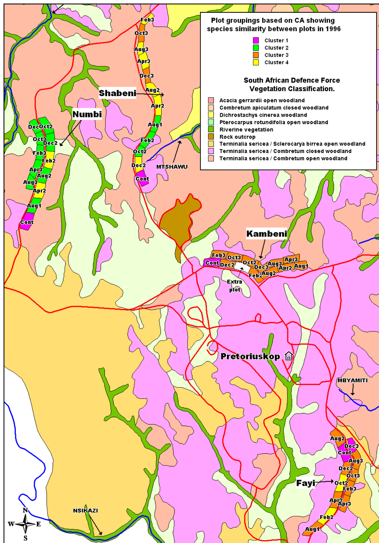
Figure 6-39: Map showing the level 2 groupings of a classification of treatment plots using a stepwise cluster analysis on the first four ordination axes of a CA on the 1996 species by plot data (Figure 6-36). The codes for the treatments are defined in Table 3-1 (p. 15).
