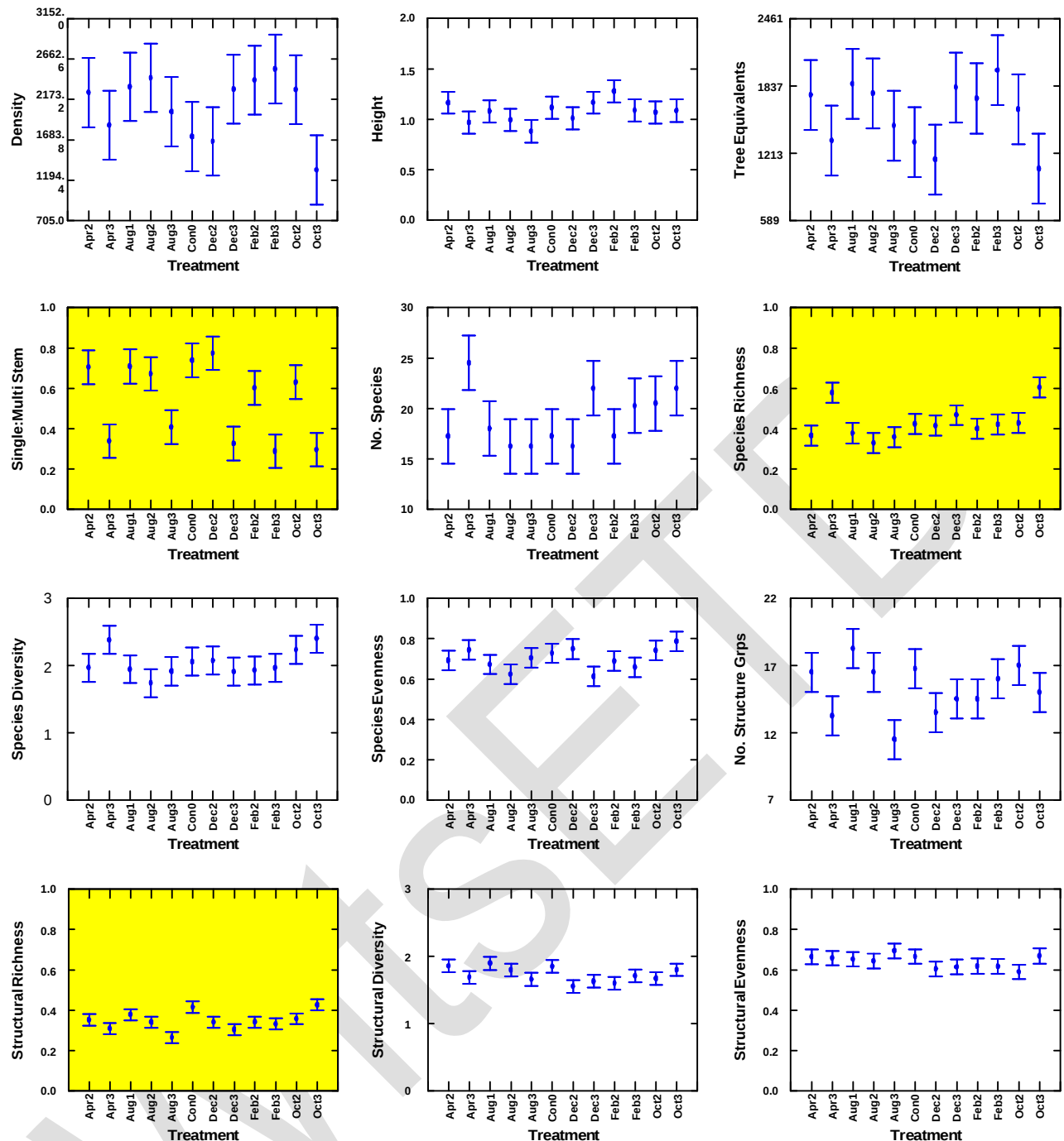
Figure 6-20: The least squares means and standard errors of the vegetation indices from the ANOVA analyses on the 1954 data testing for pre-treatment differences between the plots assigned the different treatments. The colour coding shows the level of the test significance (yellow: \alpha=0.05 , and orange: \alpha = 0.10 ).
