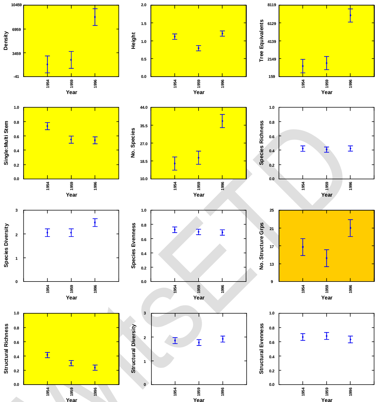
Figure 6-23: The least squares means and standard errors of the vegetation indices from the ANOVA analyses on the 1954, 1959, and 1996 control plot data testing for the effects of not burning. The colour coding shows the level of the test significance (yellow: \alpha=0.05 , and orange: \alpha = 0.10 ).
