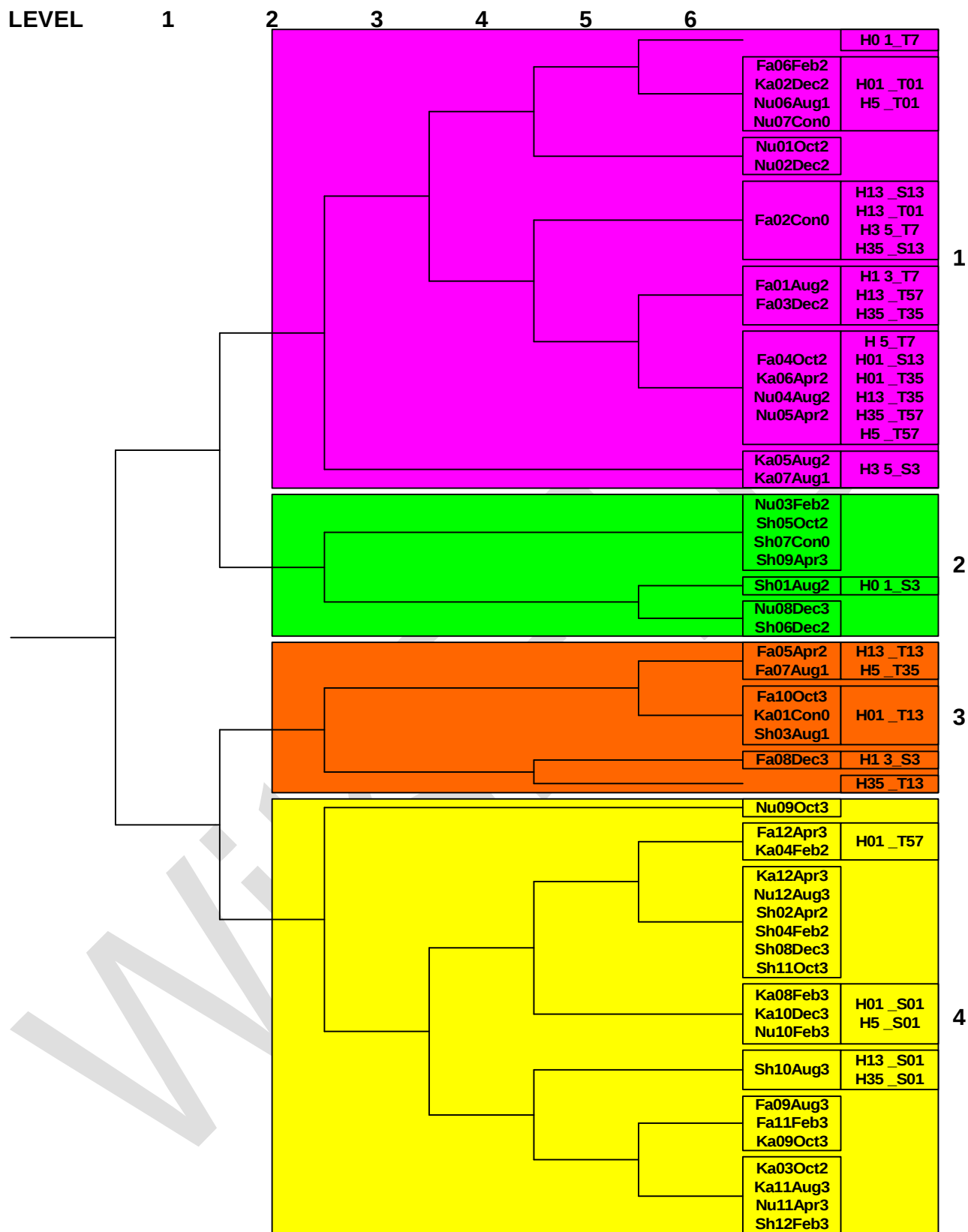
Figure 6-44: Classification of treatment plots and structures using a step-wise Gamma-Ward cluster analysis on the first four ordination axes from the CA on the 1954 structure by plot data. The codes for the treatment plots are defined in Table 10-1 (p. 214) and the codes for the structure groups are defined in Table 5-3 (p. 34).
