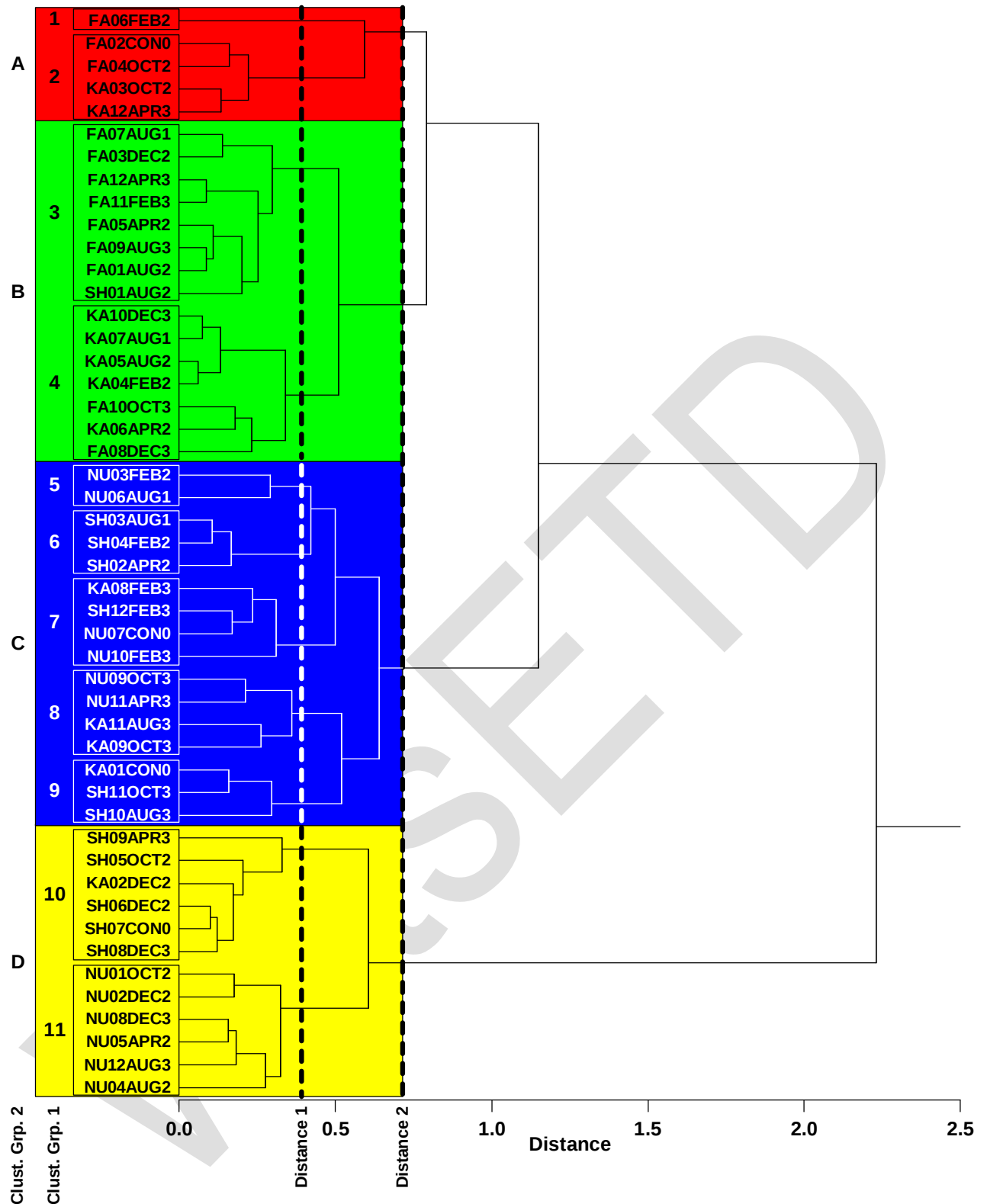
Figure 6-24: Hierarchical cluster tree from a Pearson-Ward cluster analysis on Horn's indices of similarity in species between Pretoriuskop EBPs in 1954. The codes for the treatment plots are defined in Table 10-1 (p. 214).
