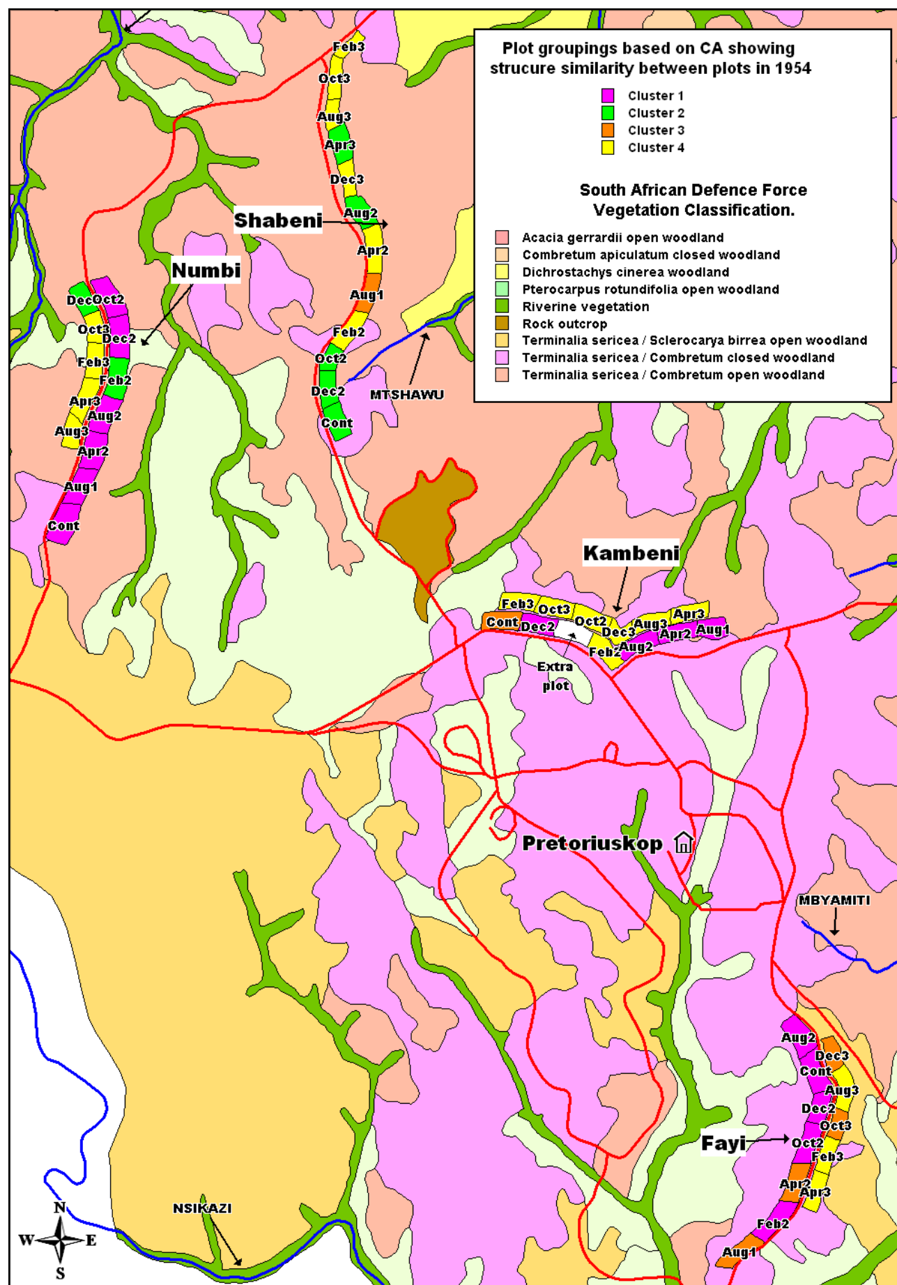
Figure 6-47: Map showing the level 2 clusters from the step-wise Gamma-Ward cluster analysis on the first four ordination axes of the CA on the 1954 structure by plot data (Figure 6-44). The codes for the treatments are defined in Table 3-1 (p. 15).
