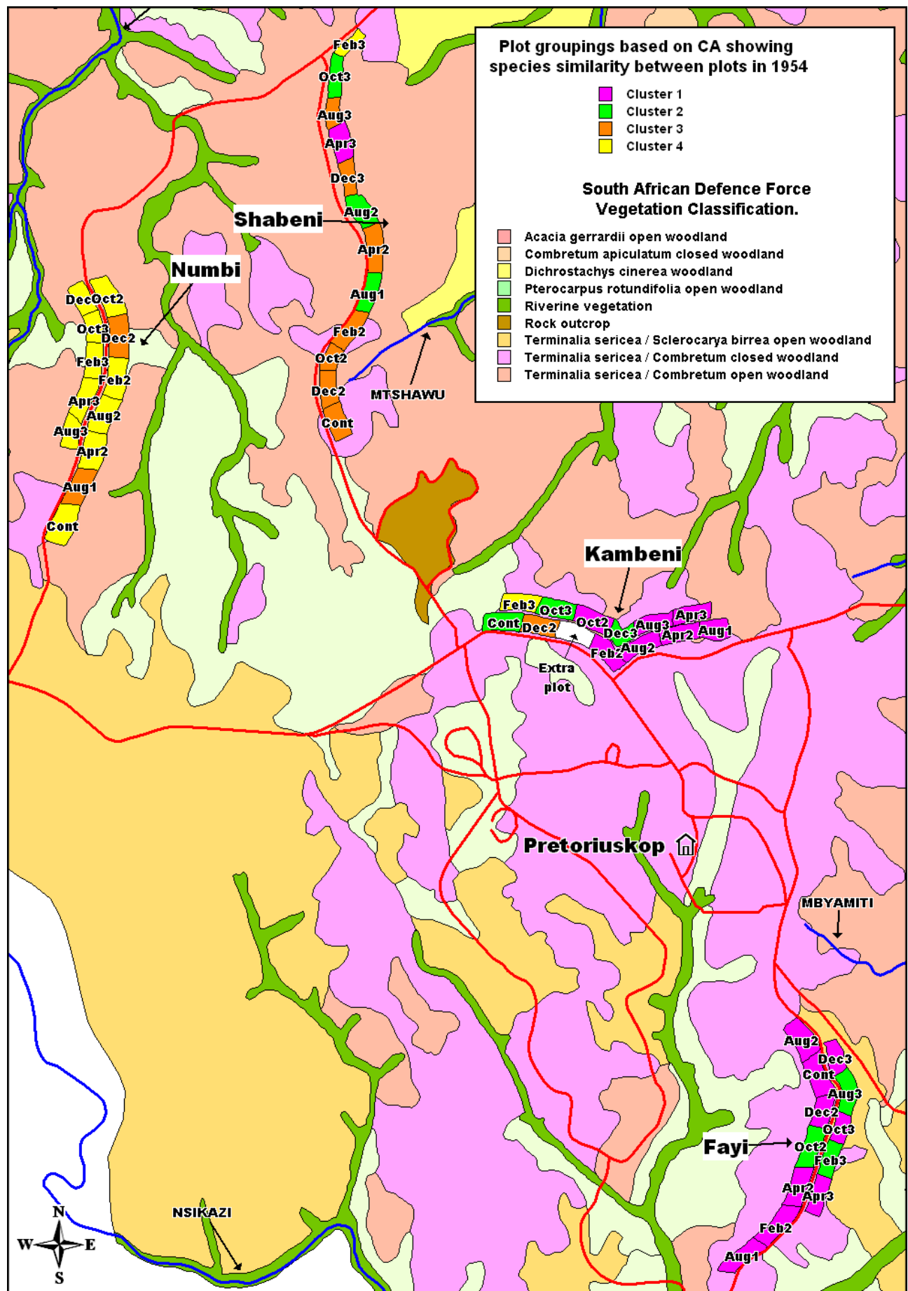
Figure 6-35: Map showing the level 2 clusters from the step-wise Gamma-Ward cluster analysis on the first four ordination axes of the CA on the 1954 species by plot data (Figure 6-32). The codes for the treatments are defined in Table 3-1 (p. 15).
