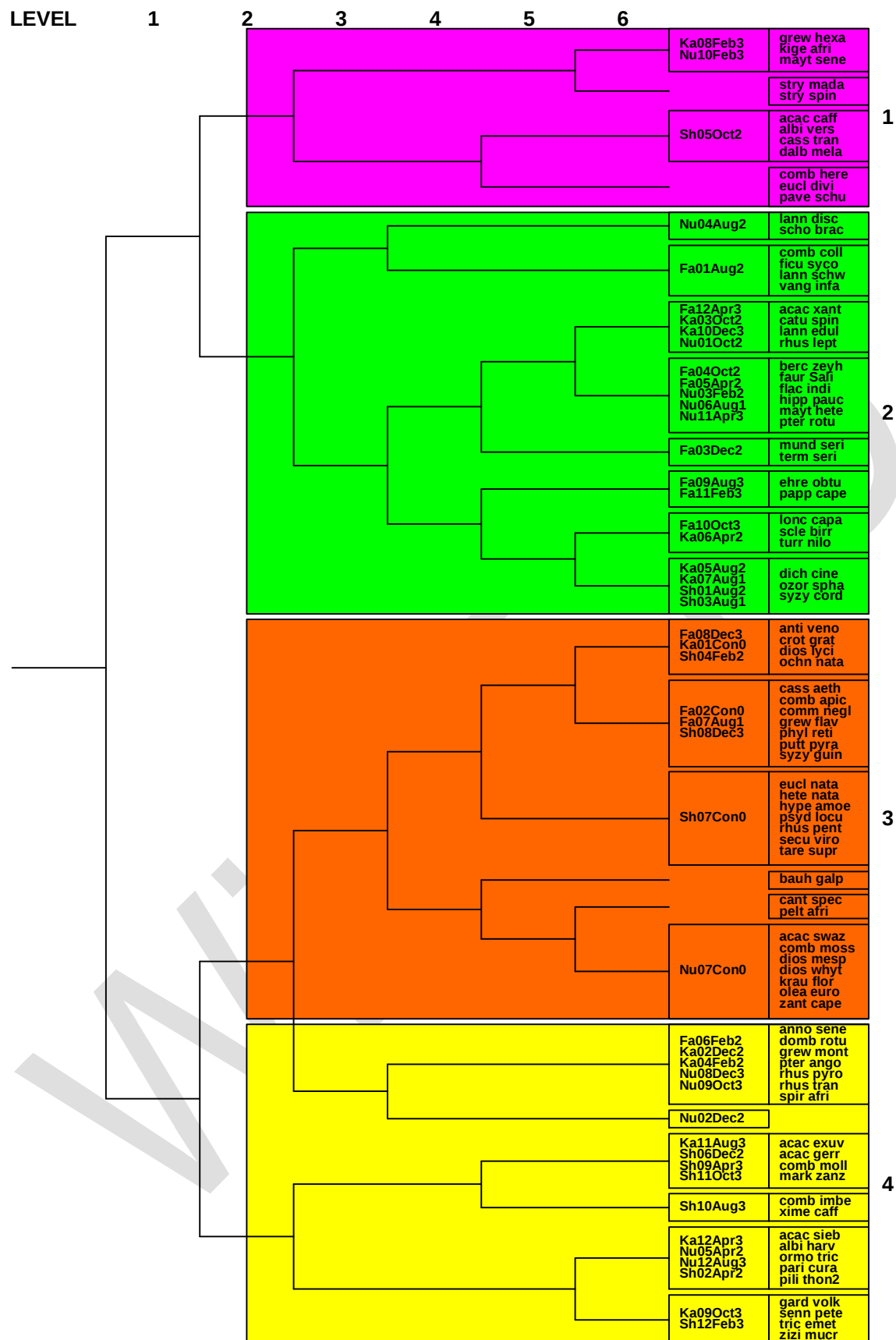
Figure 6-40: Classification of treatment plots and species using a step-wise Gamma-Ward cluster analysis on the first four ordination axes from the CA on the 1996 species by plot data with the first eight ordination axes of the 1954 species by plot CA as covariables. The codes for the treatment plots are defined in Table 10-1 (p. 214) and the codes for the species are defined in Table 9-1 (p. 210).
