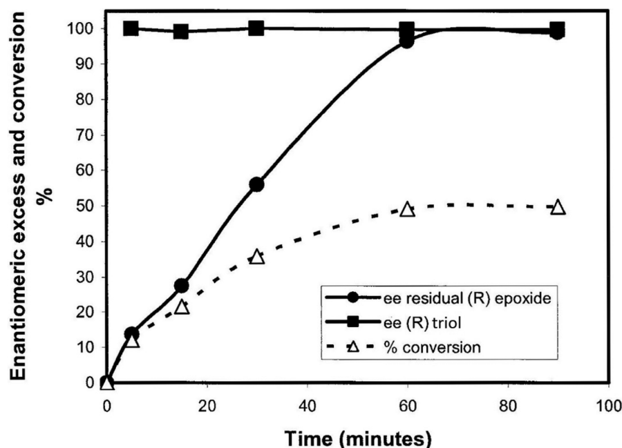
Figure 4. Epoxide ( \pm )- 2 mass % conversion and % enantiomeric excess changes (measured in monoplicate), for both substrate epoxide ( 2 ) and the ( R )-triol product ( 1 ), as observed over time during the scaled up (250 g/L substrate concentration), 80 mL volume biotransformation reaction, conducted at 20 °C, pH 7.0. A Yarrowia lipolytica engineered strain was employed that expresses the EH enzyme originally sourced from Rhodospiridium toruloides (NCYC 3181), at a biomass loading of 5% dry mass/total volume. Another graphic example of this bio-resolution on a 105 g scale of racemic ( \pm )- 2 , as performed in duplicate experiments, is given in Table S1 and graph S1 (supporting information).
