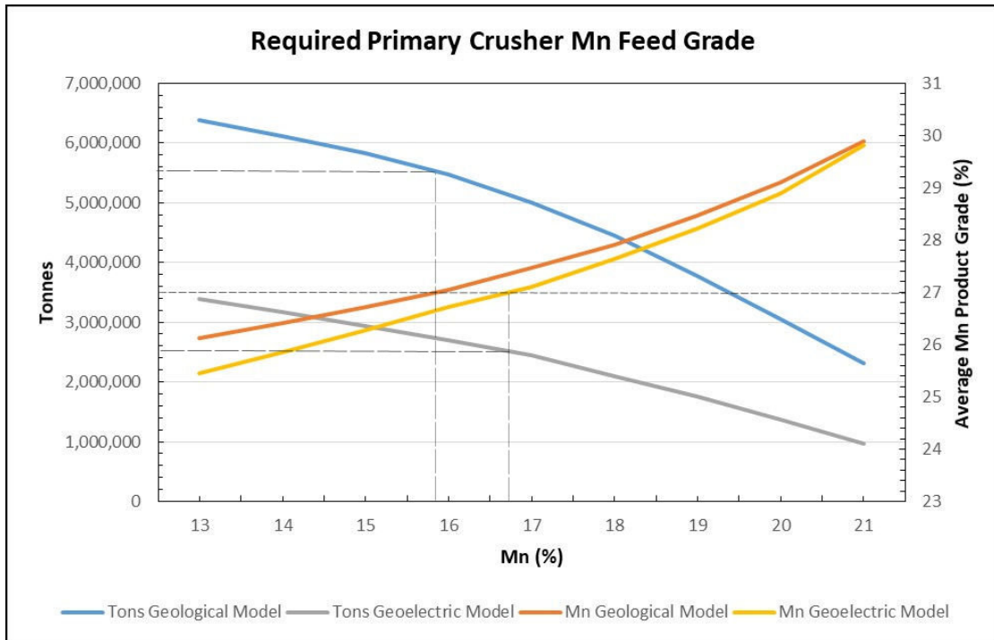
Figure 23. Comparative grade-tonnage curves for the geological and geoelectric models (Created by author).
