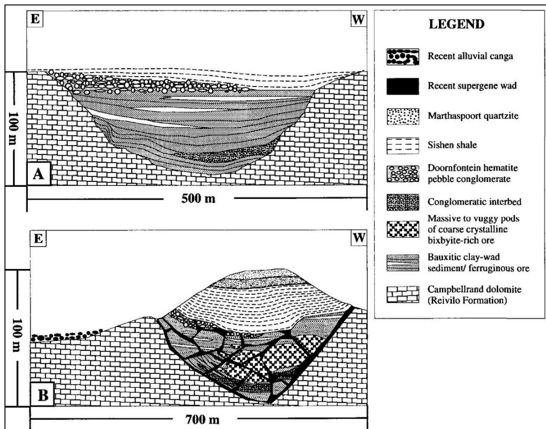
Figure 11. Model for the origin of the ferruginous manganese ores of the Western Belt (Gutzmer, 1996; Gutzmer and Beukes, 1997).
