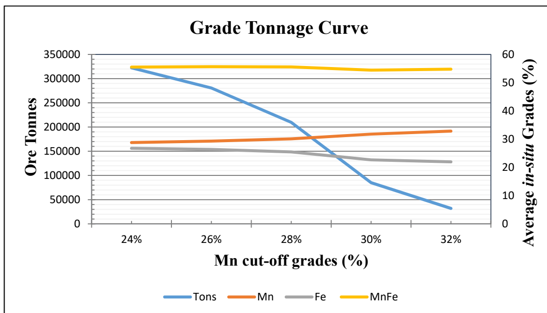
Figure 26. Mn grade-tonnage curve for the mangalore domain. (Created by author).
