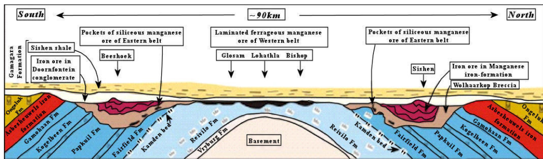
Figure 8. North-south cross-section through the Maremane Dome (Cairncross et al., 1997).
