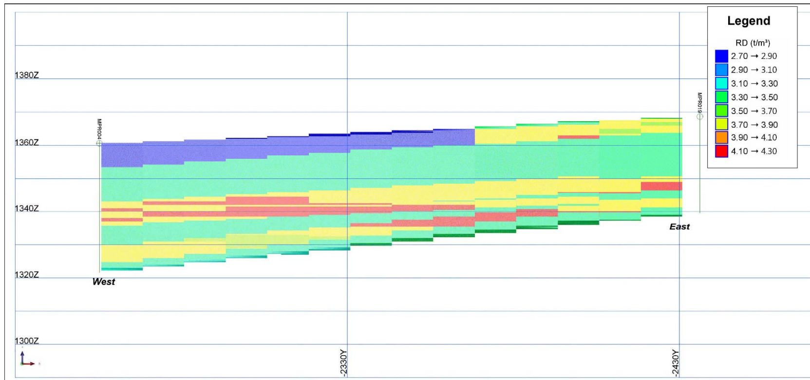
Figure 22. RD dispersion, Section 3, Geological Model (Created by the author.
