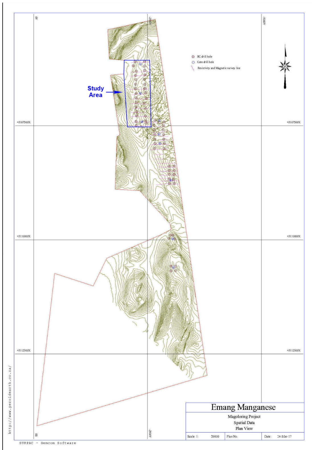
Figure 5. Project spatial data (Created by author).
