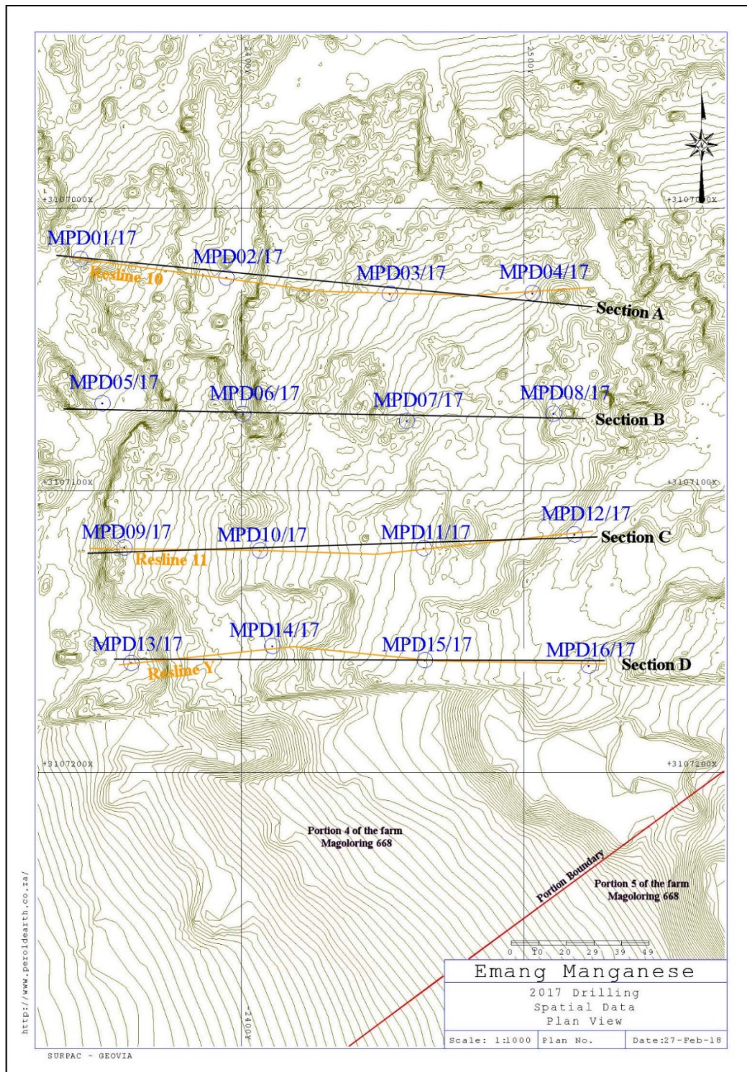
Figure 24. Position of resistivity survey lines to boreholes drilled during 2017, Emang project (Created by author).
