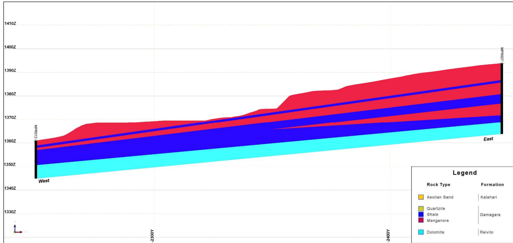
Figure 15. Geological Cross Section 11 (Created by author).
