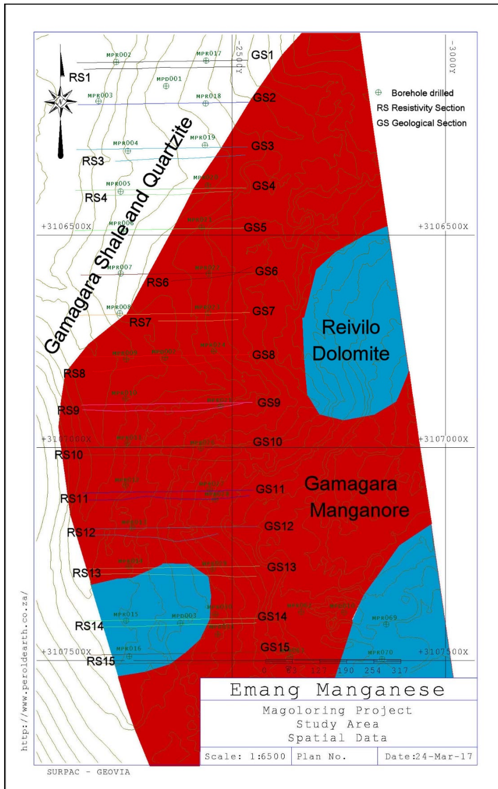
Figure 14. Study Area spatial data (Created by author).
