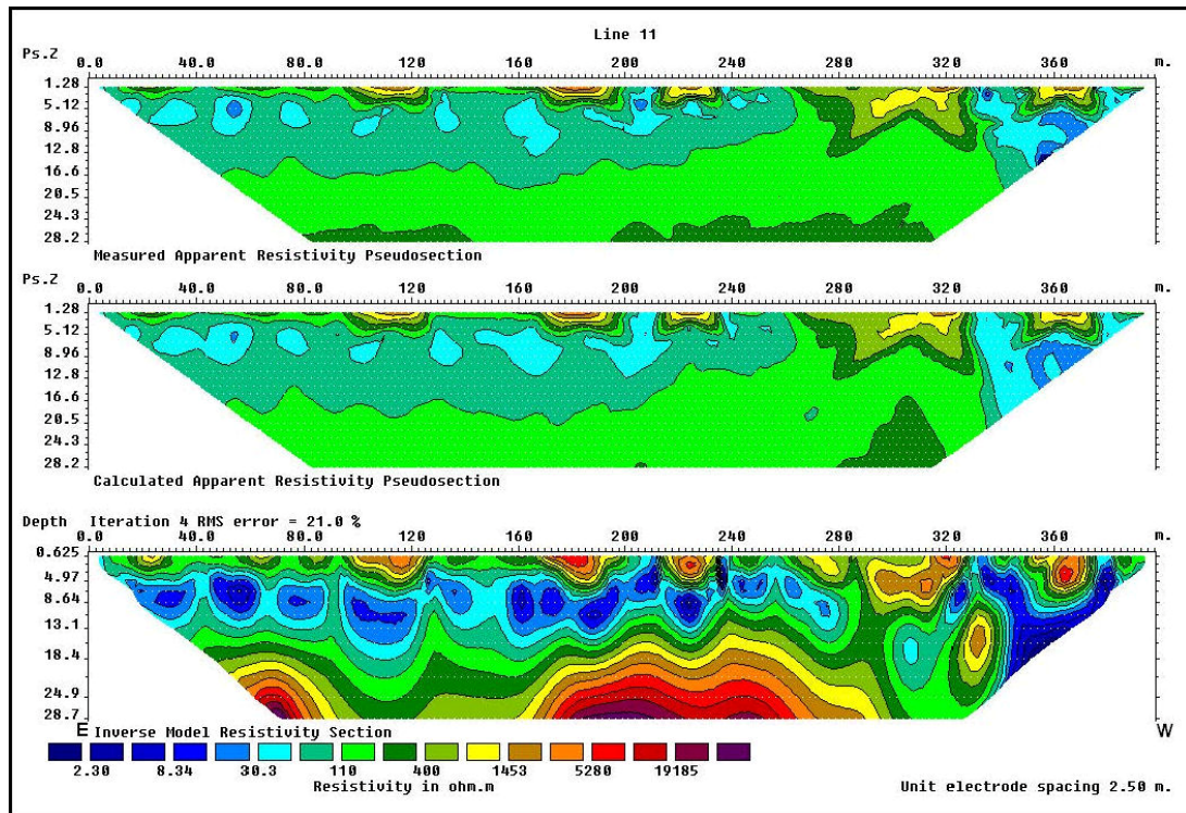
Figure 17. Different graphical resistivity sections, Line 11, received from Vonk (2013).
