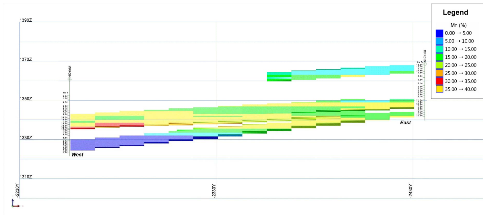
Figure 21. Mn dispersion, Section 3, Geological Model (Created by author).
