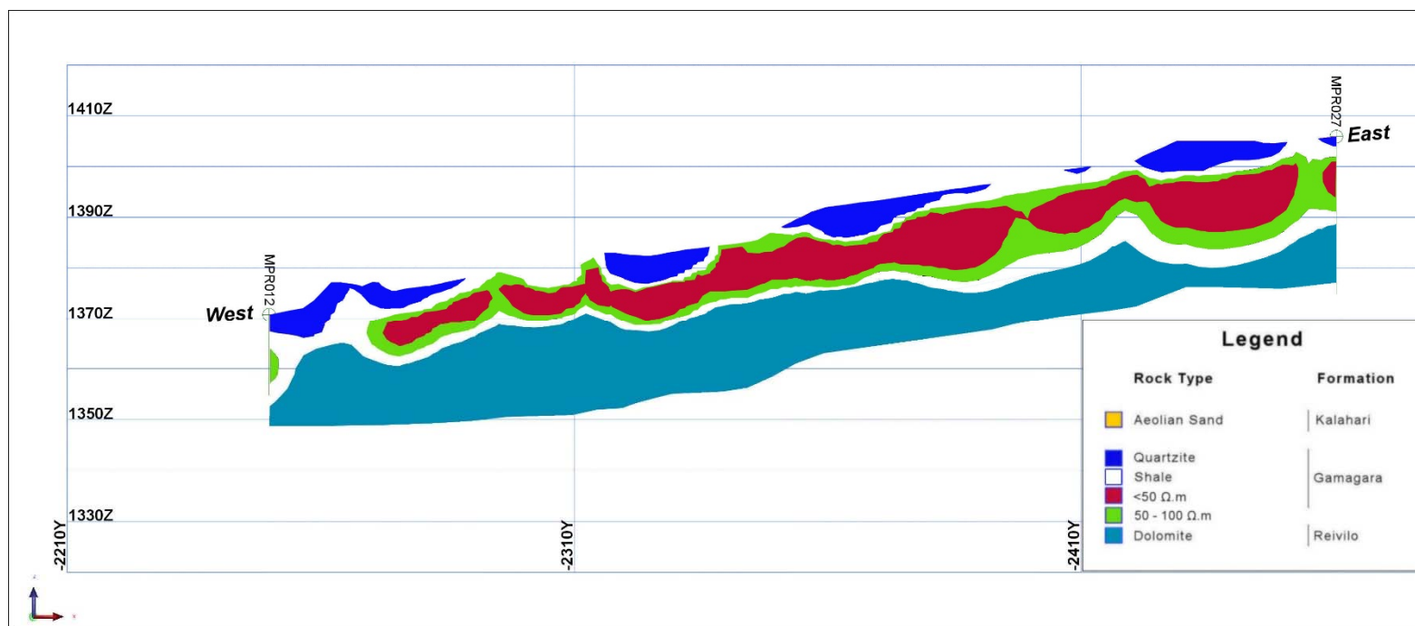
Figure 19. Goelectric Cross Section 11 (Created by author).
