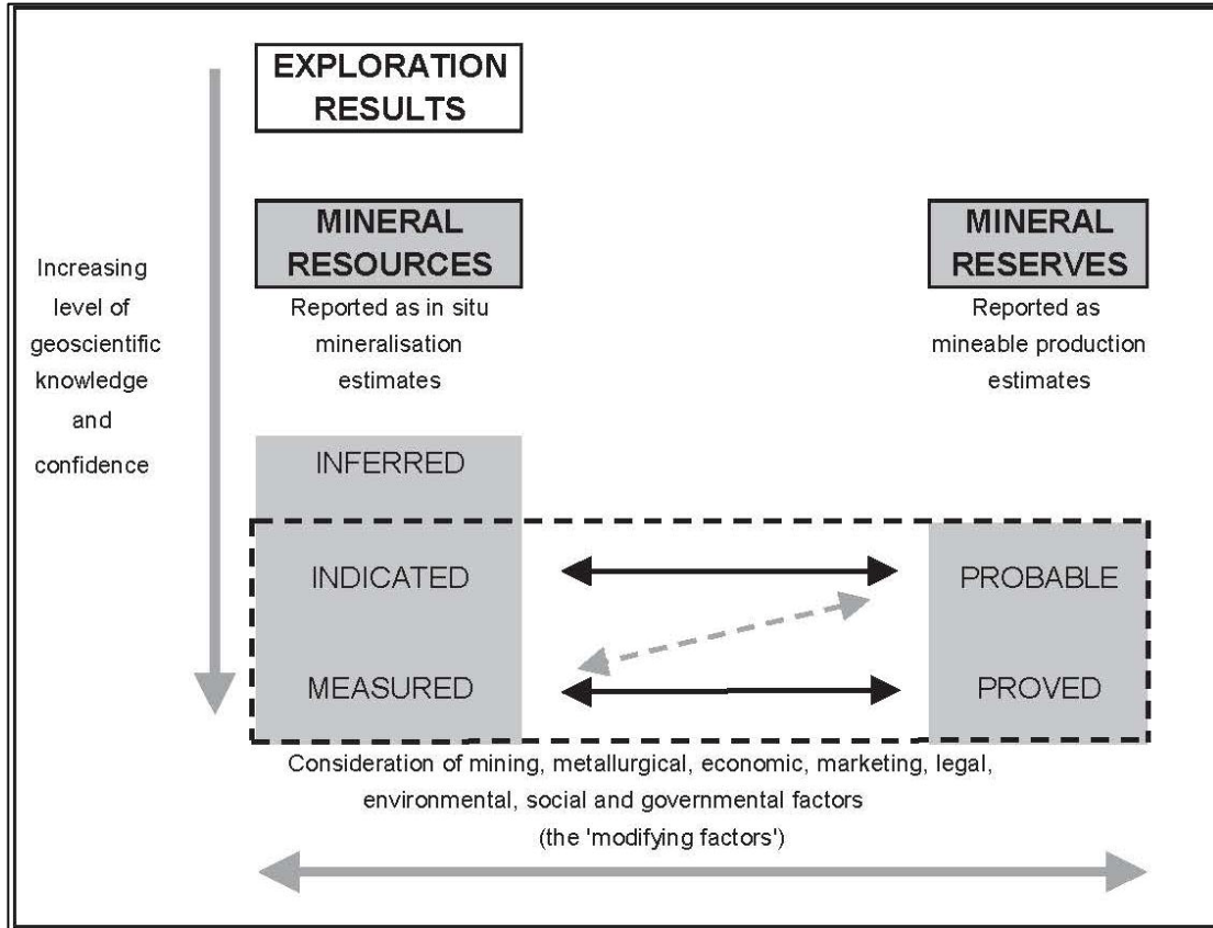
Figure 2. Relationship between Exploration Results, Mineral Resources and Mineral Reserves (Samrec Code, 2016).
