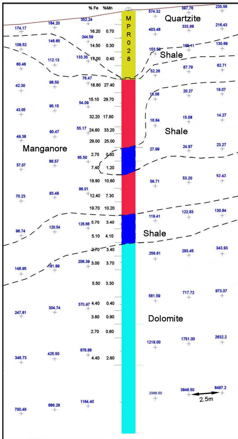
Figure 18. Comparison of logged geology, chemical and resistivity results (blue text) for reverse circulation borehole MPR028 (Created by author).
