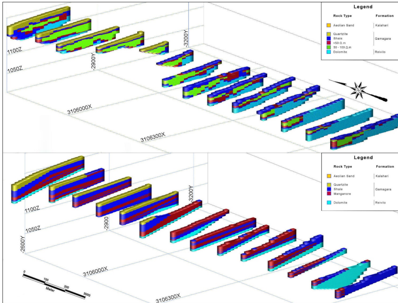
Figure 20. Block model sections from the completed geological and geoelectric models (Created by author).
