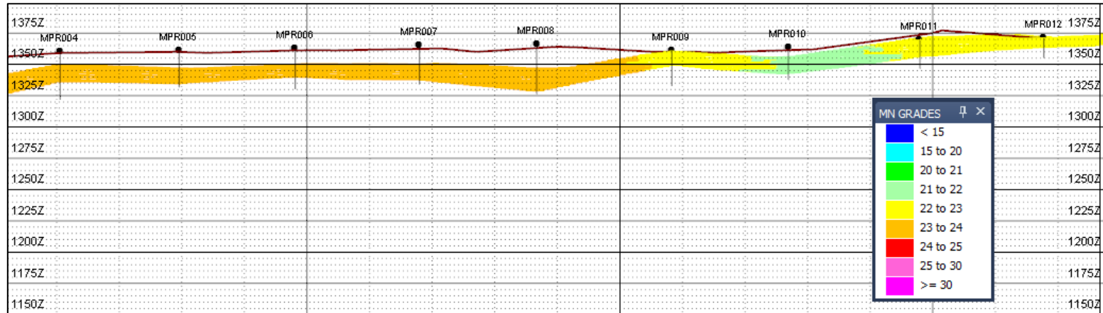
Figure 4. North-south section B (After Upshall and Richards, 2012).
