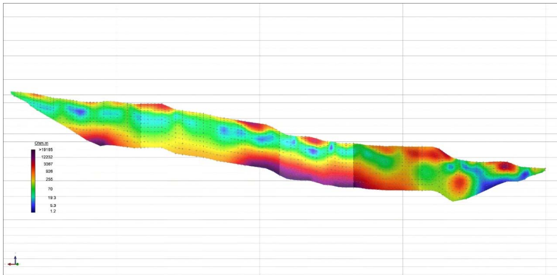
Figure 16. Georeferenced measured apparent resistivity pseudo-section, Line 11(Created by author).
