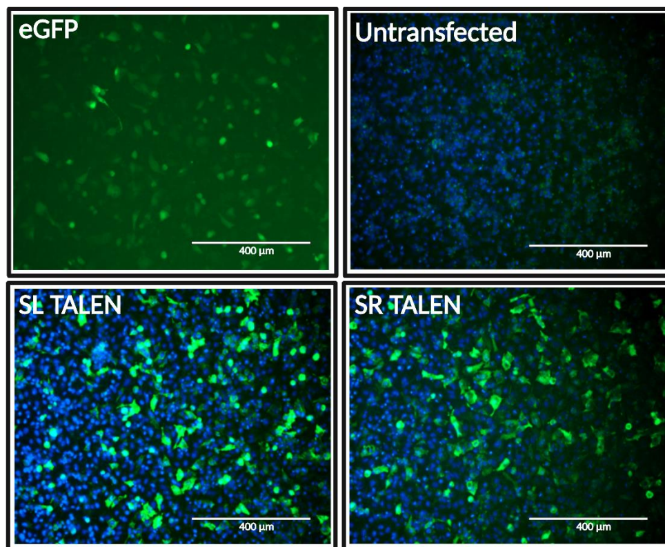
Figure 2.16: Detecting TALEN expression from cellulose-treated cap-1 transcripts using VCE in Huh7 cells.
