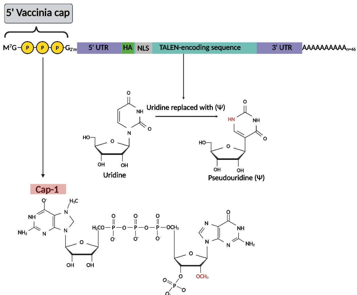
Figure 2.2: TALEN-encoding mRNA with vaccinia cap and Ψ.
