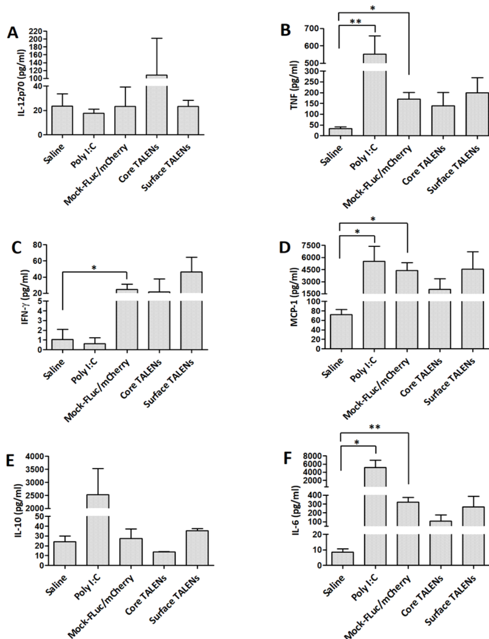
Figure 4.7: LNP-encapsulated TALENs did not illicit significant cytokine induction in transgenic mice.
