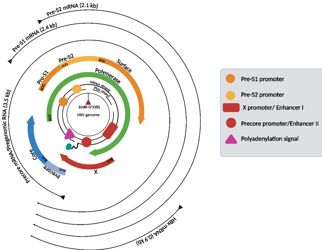
Figure 1.1: The structure of the hepatitis B virus (HBV) genome.
