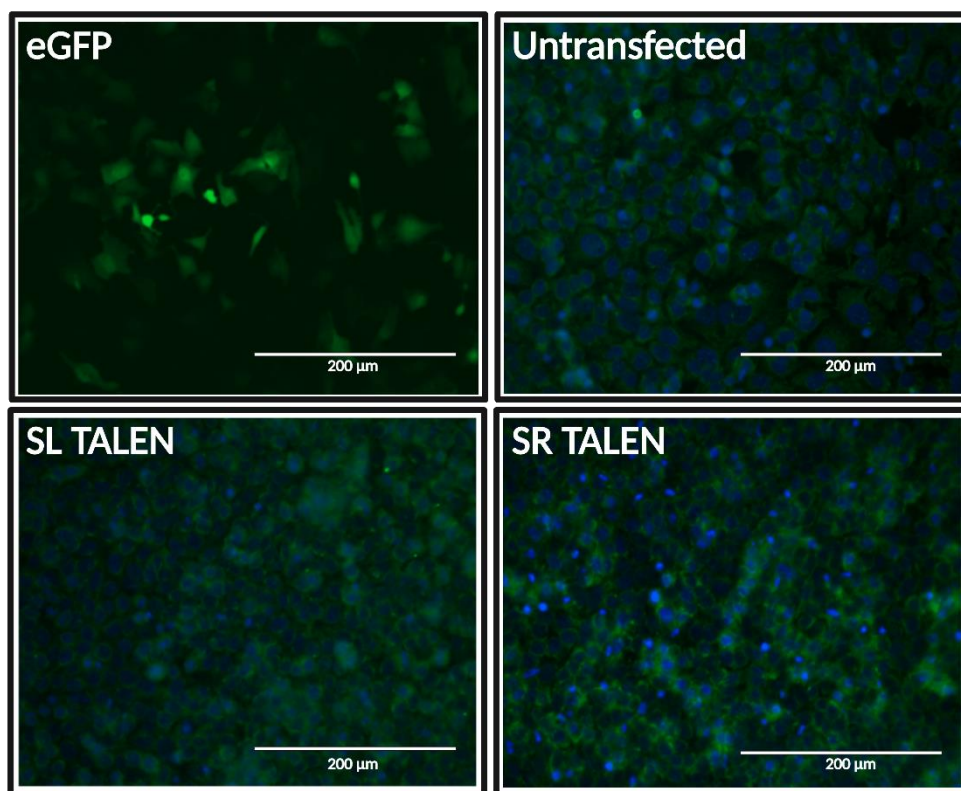
Figure 2.15: Absence of TALEN expression from cap-1 transcripts produced with VCE in Huh7 cells.
