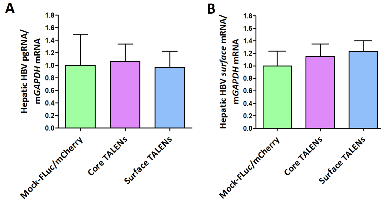
Figure 4.5: Core and Surface TALENs have no impact on hepatic HBV mRNA levels.
