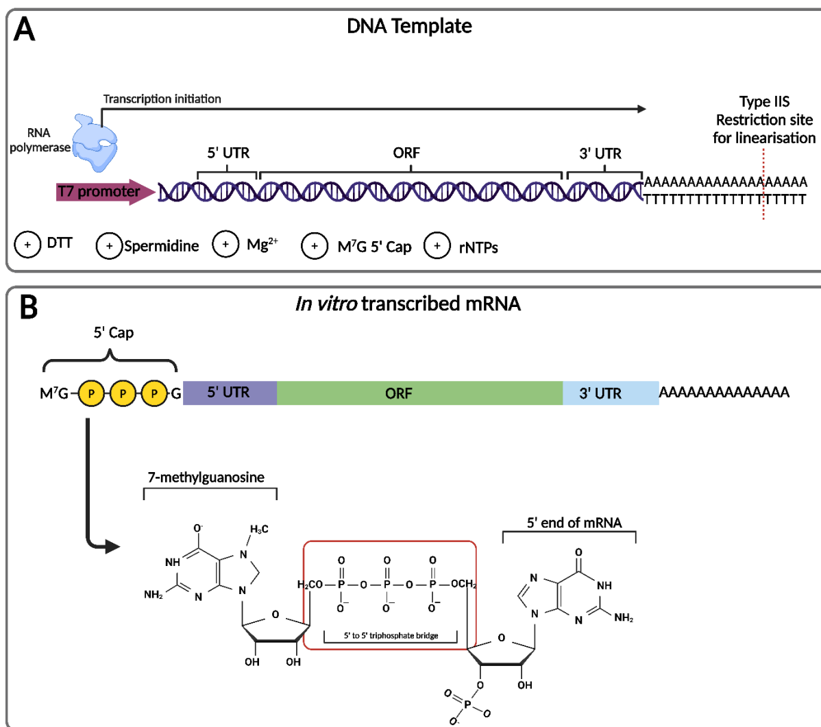
Figure 1.7: Schematic overview of the IVT process from a DNA template.
