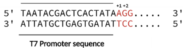
Figure 1.10: CleanCap® AG trinucleotide.
