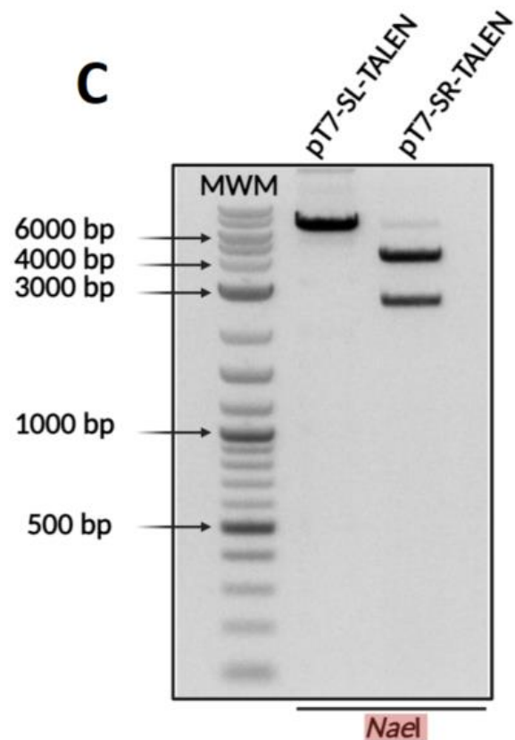
Figure 2.10: Confirmation of left and right FokI domain nucleases in pT7-SL/SR-TALEN plasmids.
