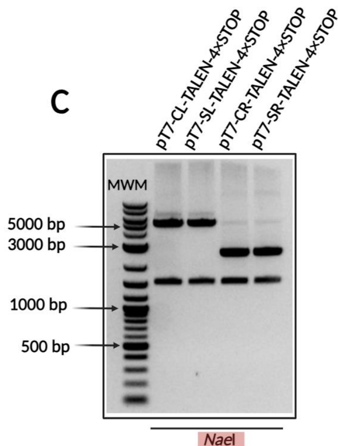
Figure 6.3: Confirmation of left and right FokI nuclease domains in pT7-CL/SL-TALEN and pT7-CR/SR-TALEN plasmids.
