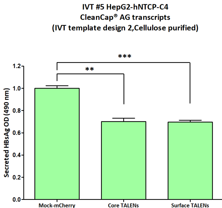
Figure 3.4: TALEN-mediated reduction of HBsAg secretion in HepG2-hNTCP-C4 cells.
