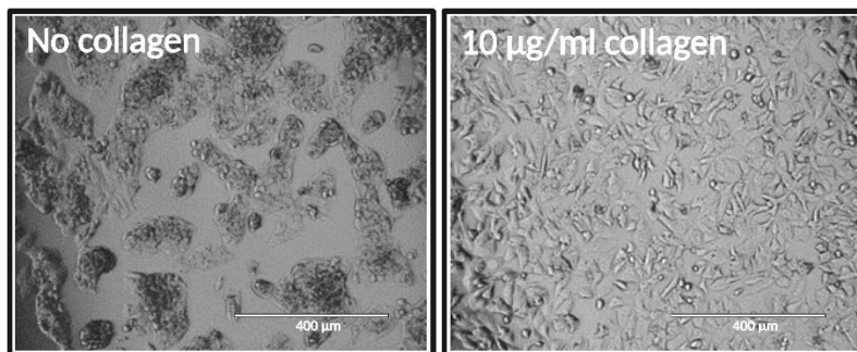
Figure 6.1: Treating culture plates with collagen enhances HepG2-hNTCP-C4 growth.
