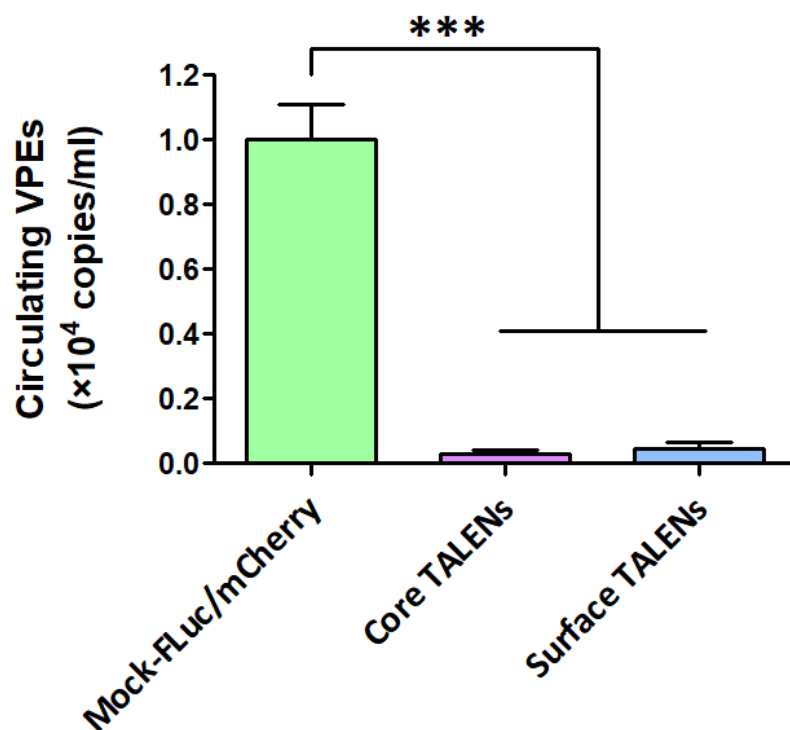
Figure 4.4: TALEN-mediated inhibition of viral replication.
