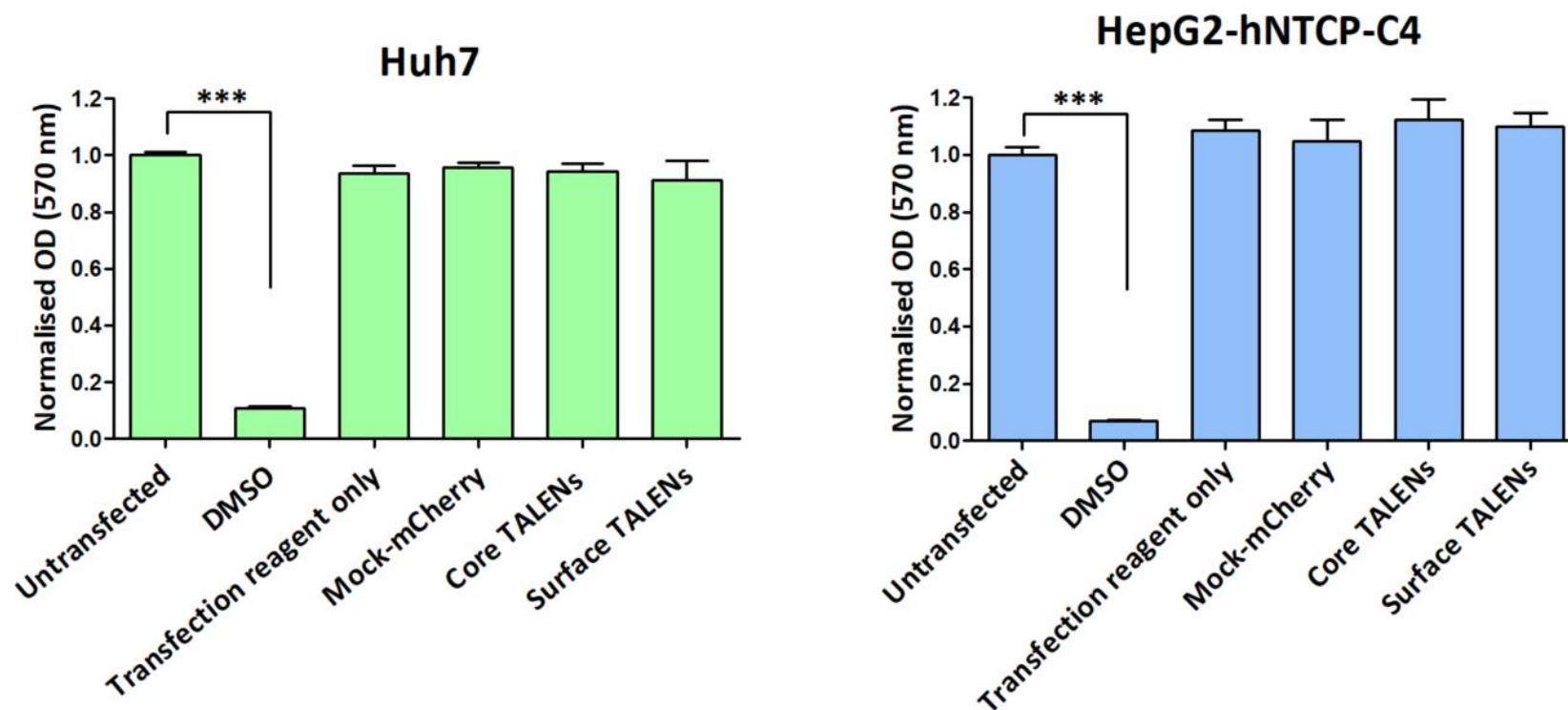
Figure 3.6: Evaluation of TALEN-induced cellular toxicity.
