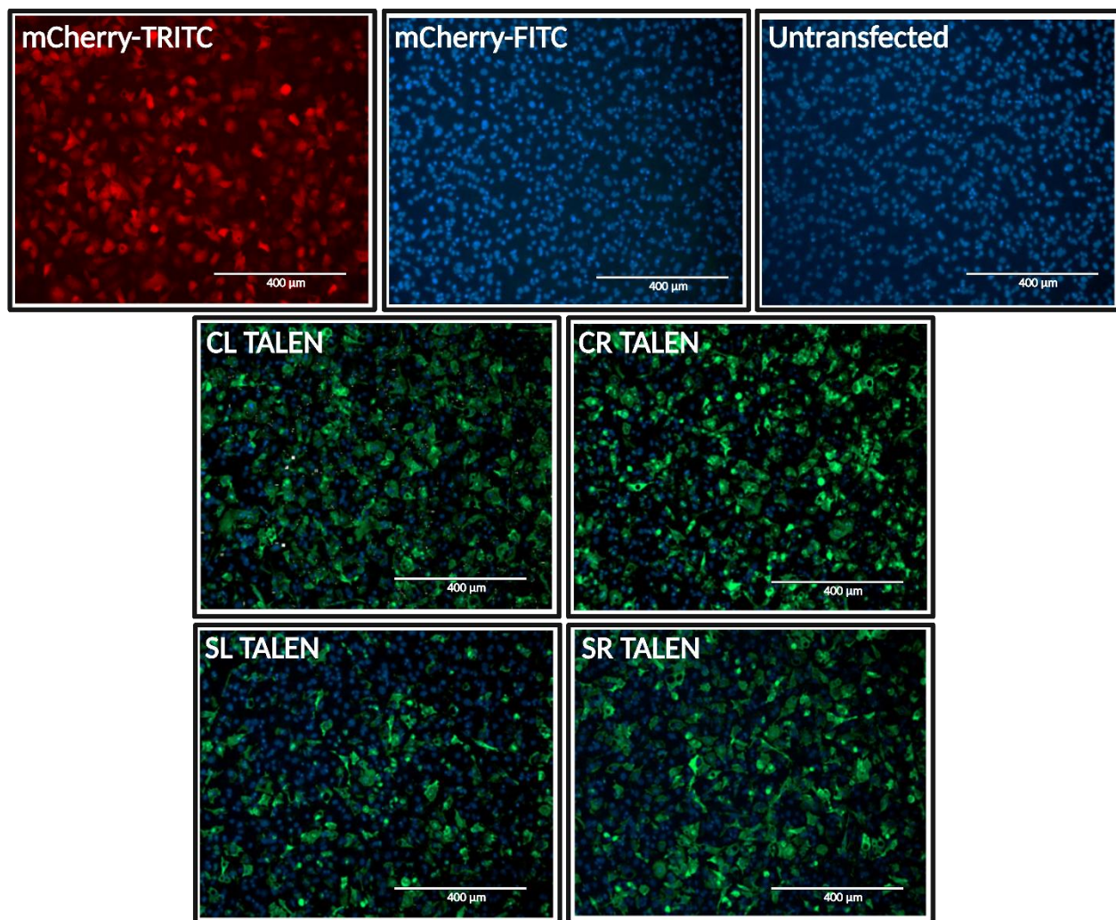
Figure 2.19: Enhanced TALEN expression from cellulose-treated cap-1 transcripts using CleanCap ® AG in Huh 7 cells-IVT template design 2.
