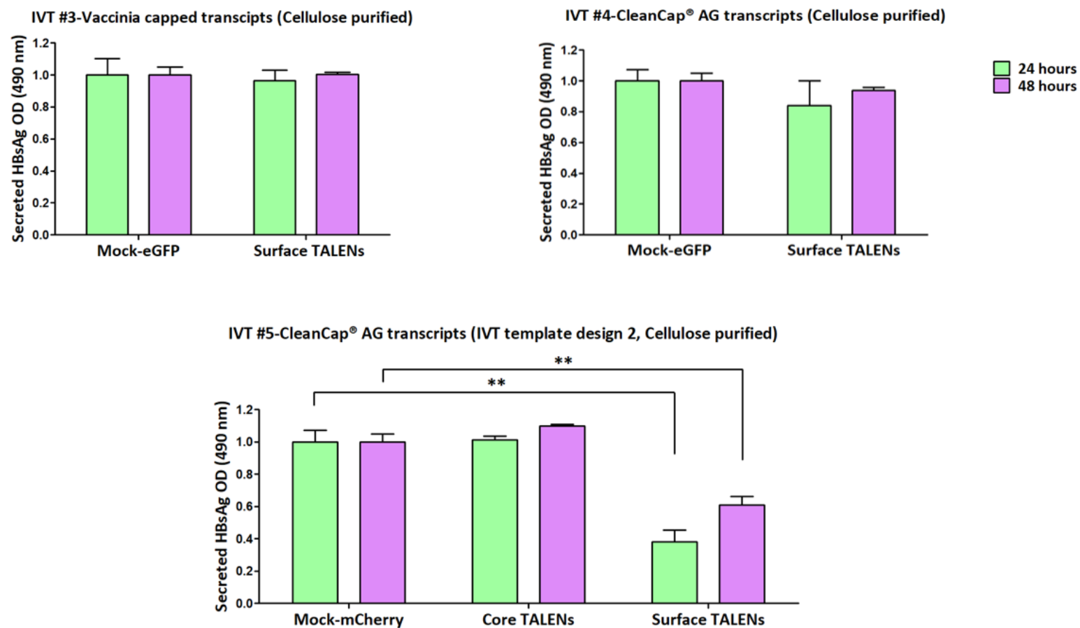
Figure 3.3: Measuring HBsAg secretion in Huh7 cells transfected with pCH-9/3091- IVT #3 to IVT #5.
