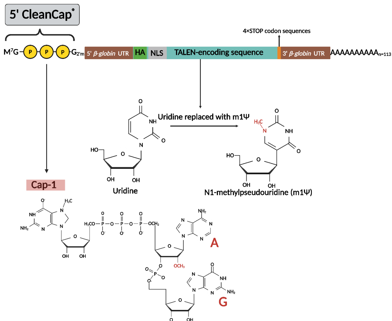
Figure 2.3: TALEN-encoding mRNA with CleanCap® AG and m1Ψ.
