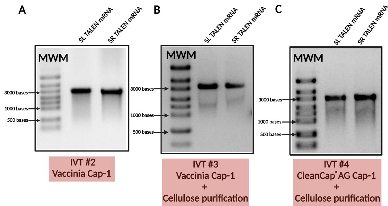
Figure 2.14: Confirmation of in vitro transcribed SL/SR TALEN cap-1 transcripts.
