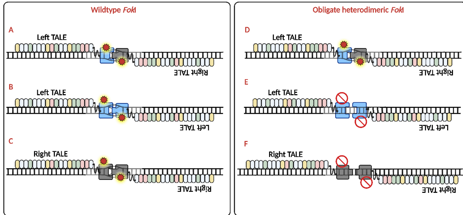
Figure 1.5: Enhanced specificity achieved by obligate heterodimeric Transcription Activator-Like Effector Nucleases (TALENs).
