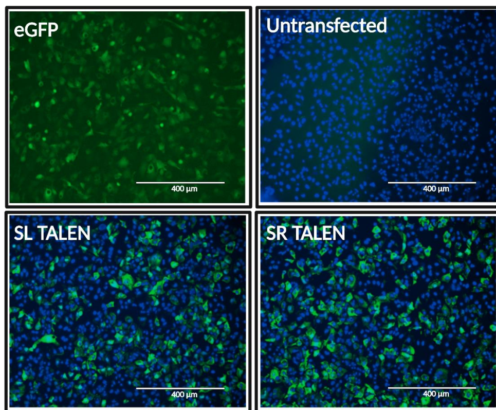
Figure 2.17: Detecting TALEN expression from cellulose-treated cap-1 transcripts using CleanCap ® AG in Huh 7 cells.
