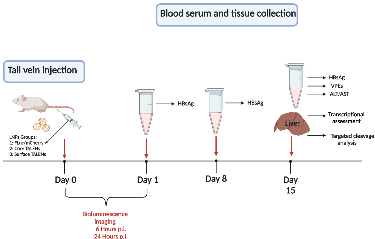
Figure 4.1: Experimental Timeline for TALEN-Treated Mice.
