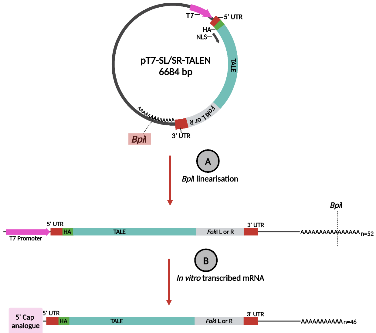
Figure 2.5: Linear templates for IVT of TALEN-encoding mRNA -IVT template design 1.
