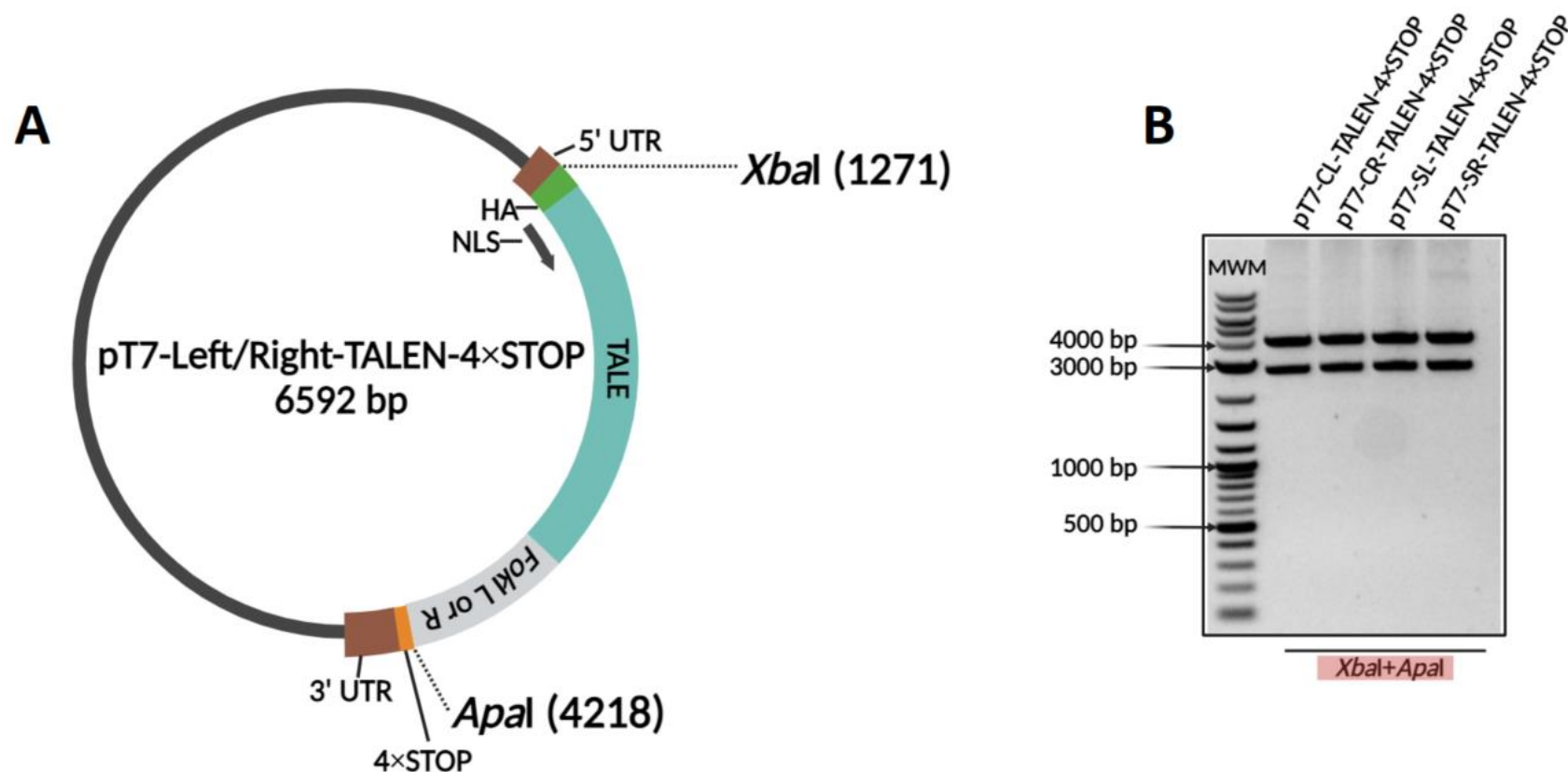
Figure 6.2: Confirmation of pT7-Left/Right-TALEN plasmids.
