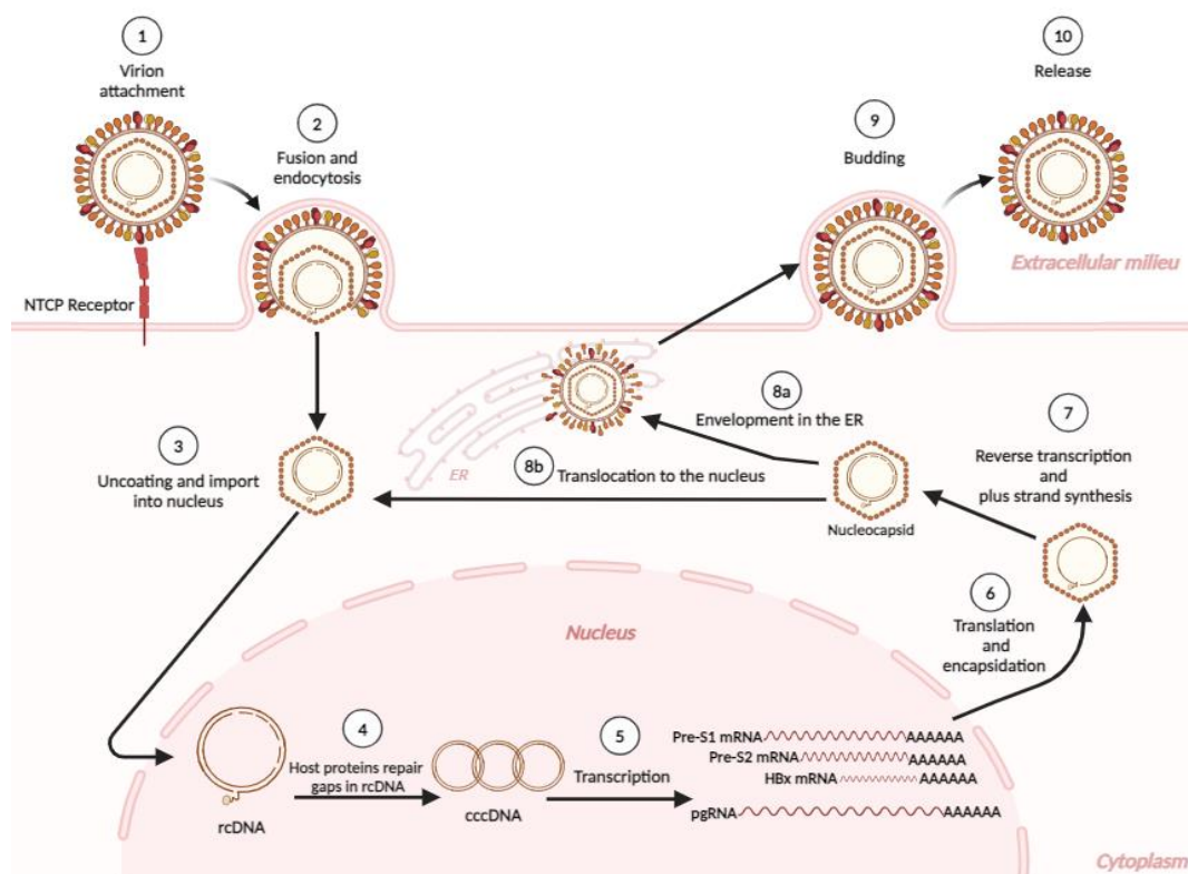
Figure 1.2: The replication cycle of the hepatitis virus (HBV).
