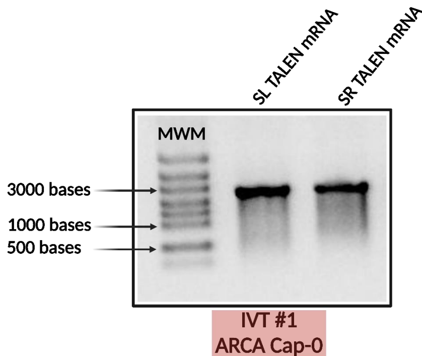
Figure 2.12: Confirmation of in vitro transcribed SL/SR TALEN transcripts with ARCA cap-0.
