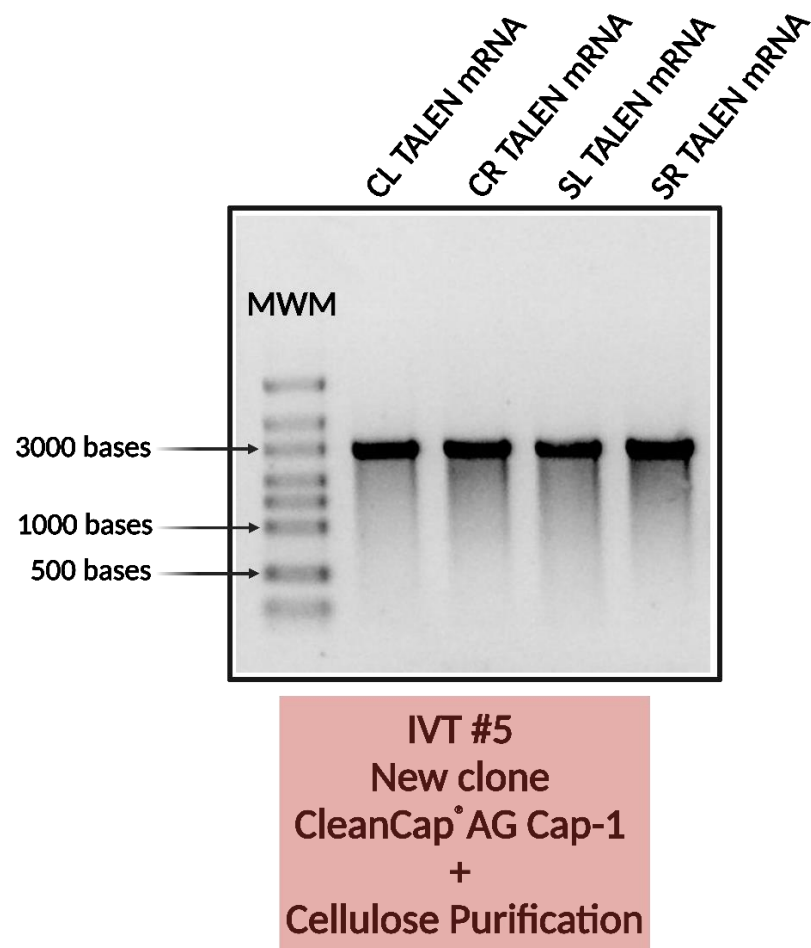
Figure 2.18: Confirmation of in vitro transcribed Core and Surface TALEN transcripts with CleanCap® AG analogues.
