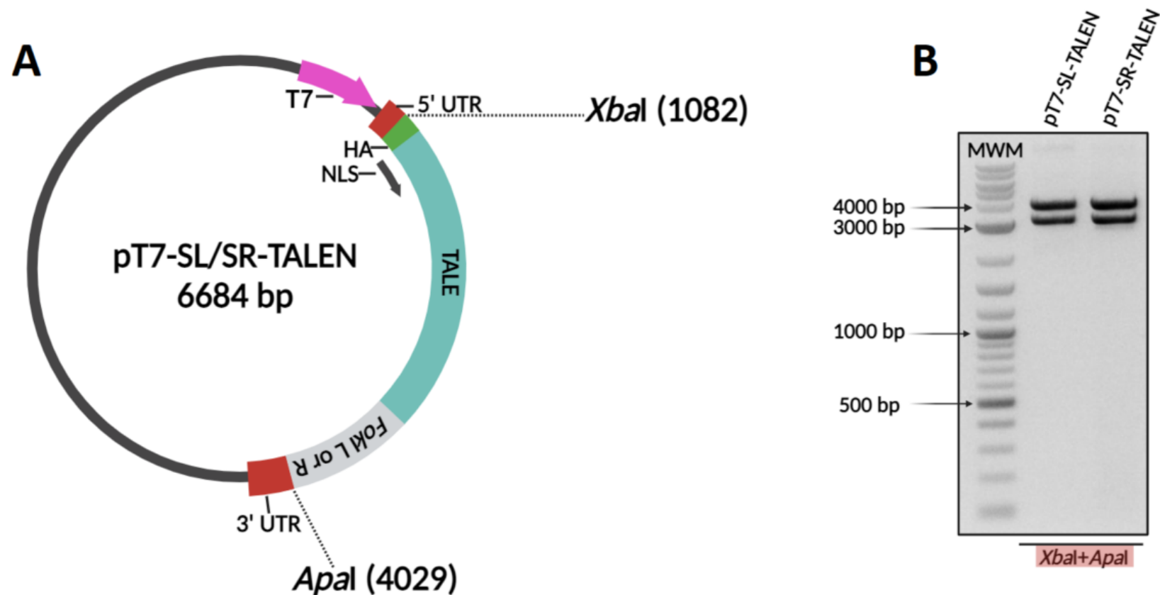
Figure 2.9: Confirmation of pT7-SL/SR-TALEN plasmids.
