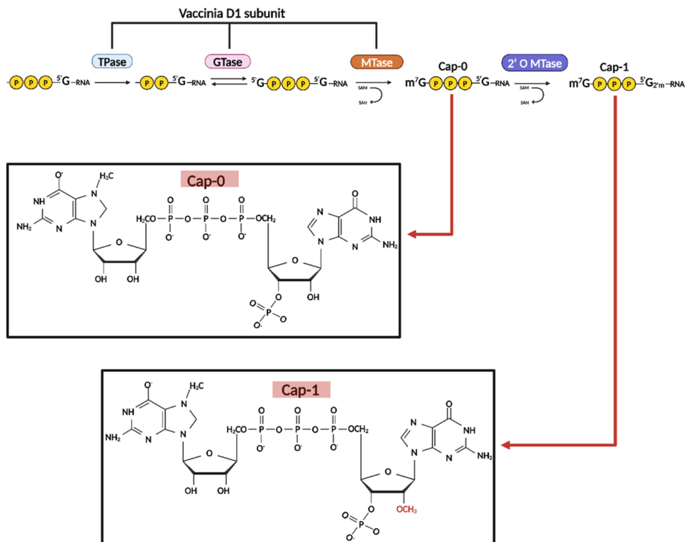
Figure 1. 9: The enzymatic conversion from uncapped to cap-0 and cap-1 transcripts using VCEs.
