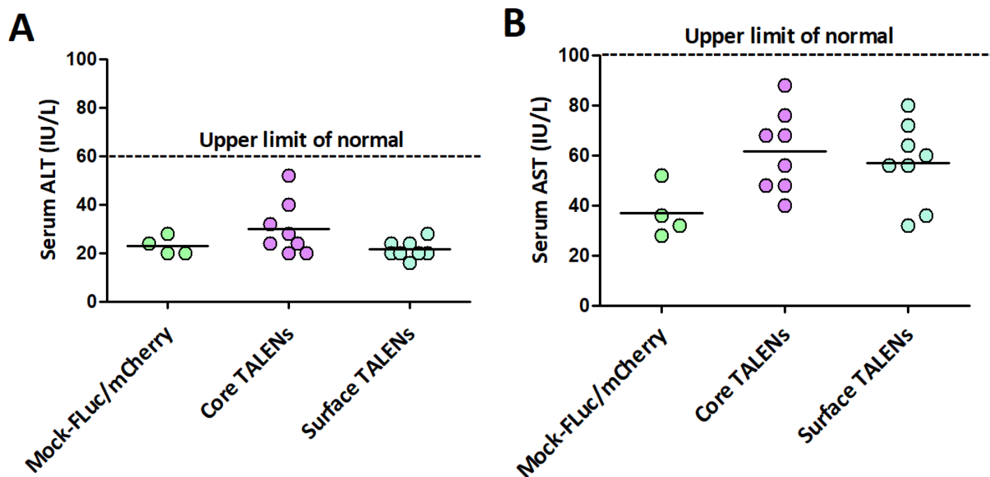
Figure 4.8: Absence of hepatic toxicity in transgenic mice.
