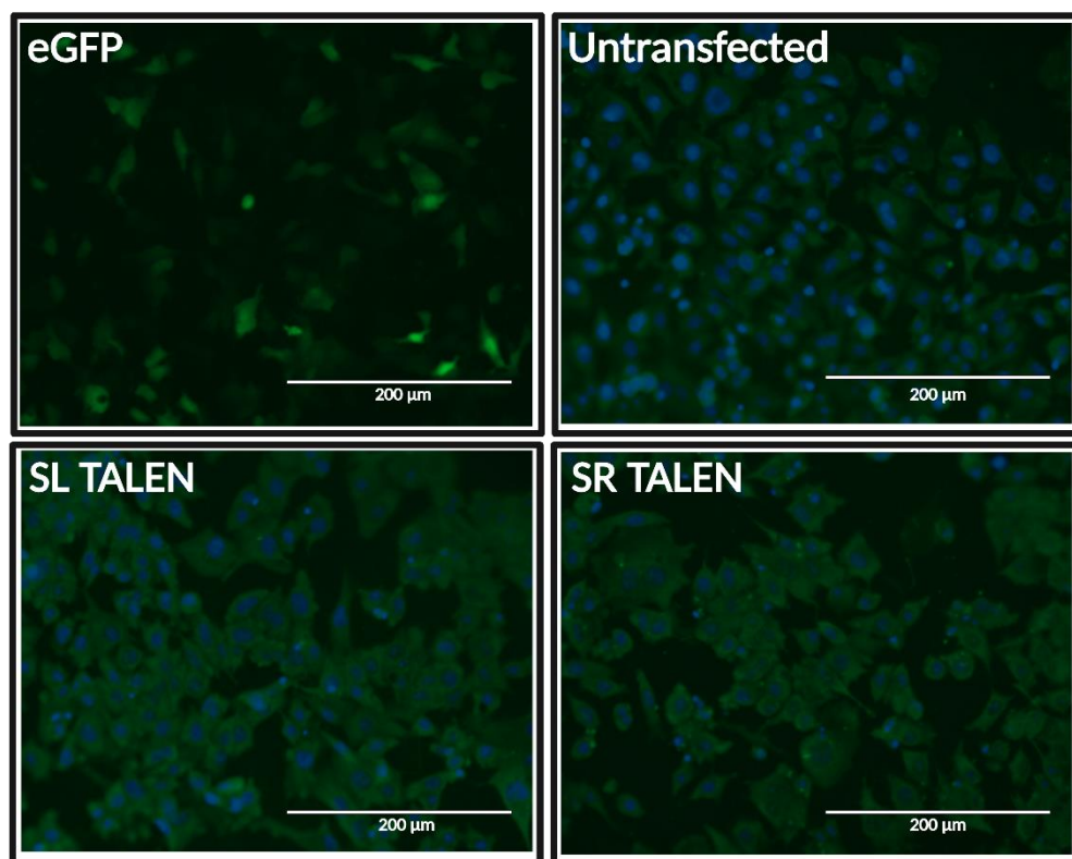
Figure 2.13: Absence of TALEN expression from cap-0 transcripts in Huh7 cells.
