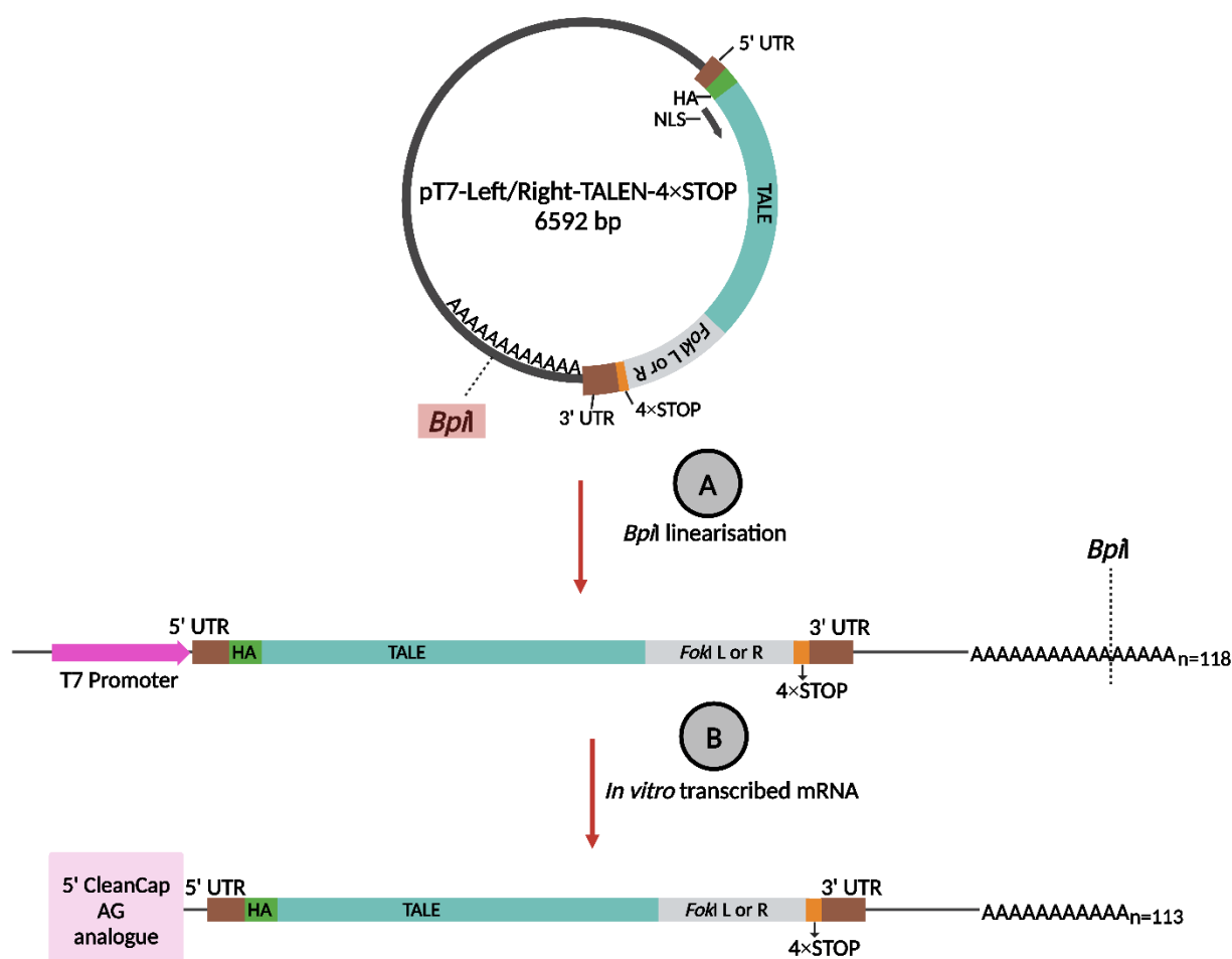
Figure 2.8: Linear templates for IVT of TALEN-encoding mRNA - IVT template design 2.
