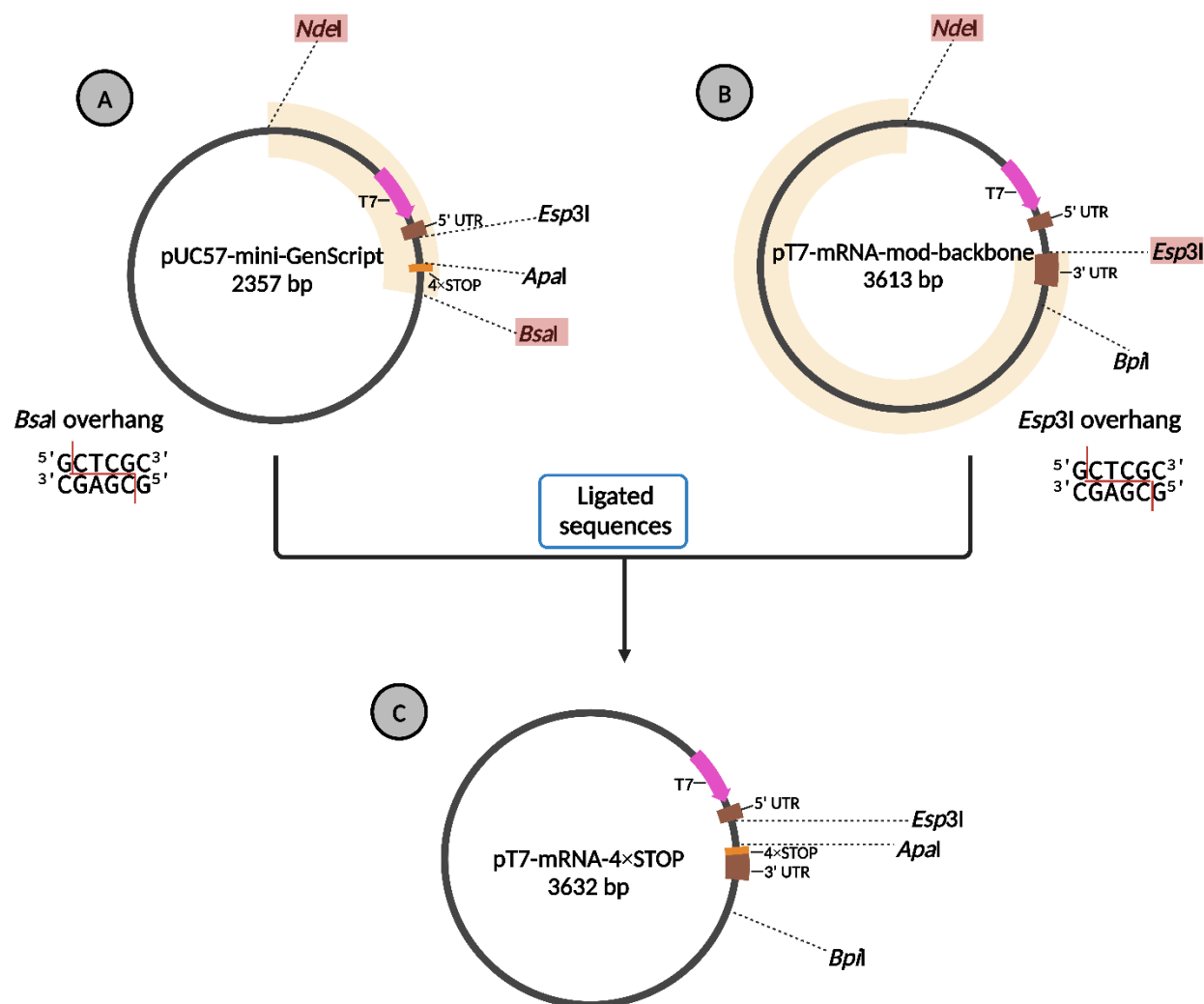
Figure 2.6: Producing modified vector for in vitro transcription- IVT template design 2.
