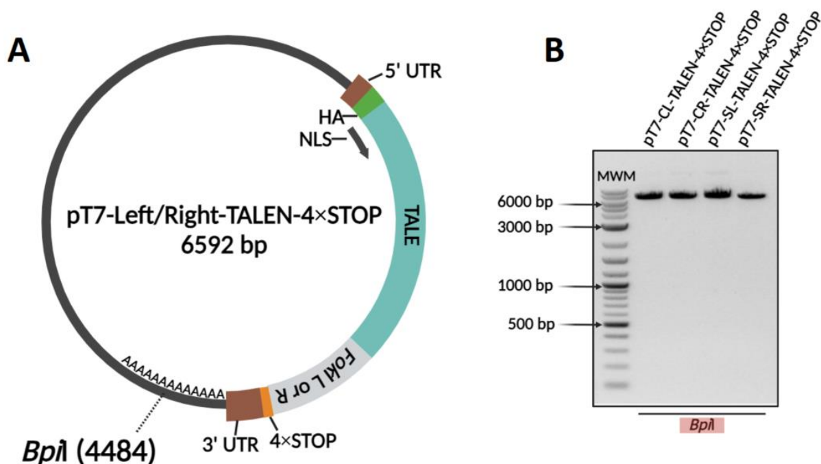
Figure 6.4: Linearised pT7-Left/Right-TALEN templates.
