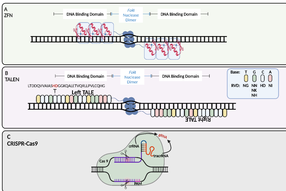
Figure 1.4: Designer nucleases induce double-stranded breaks at target sites.
