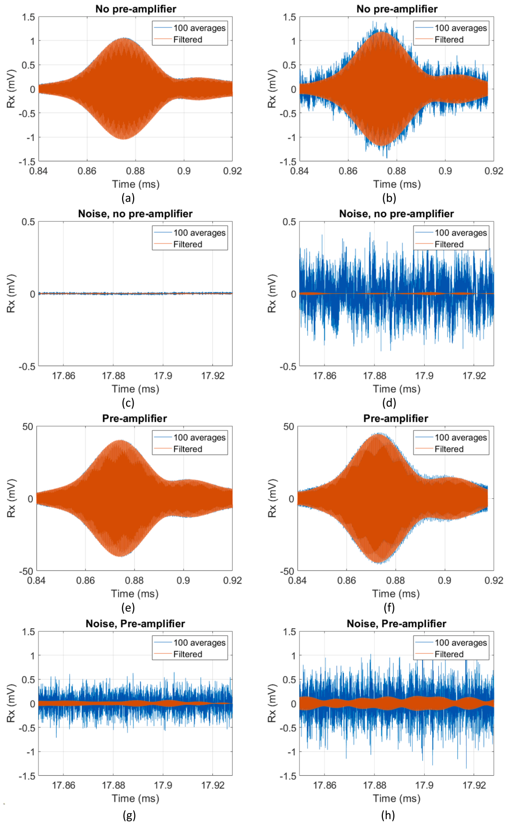
Fig. 8. Influence of pre-amplifier with gain of 33 dB on signals (200 cycles excitation signal) measured using bench-top instruments (a, c, e, g, I, k) and USB oscilloscope (b, d, f, h, j, l). All measurements performed with 100 averages and influence of bandpass filtering shown. (a, b) third arrival, no pre-amplifier; (c, d) noise, no pre-amplifier; (e, f) third arrival, pre-amplifier; (g, h) noise, pre-amplifier; (i, j) third arrival, matching and pre-amplifier; (k, l) noise, matching and the pre-amplifier.
