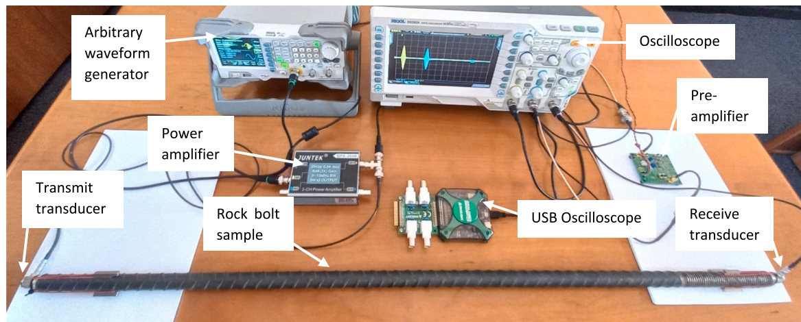
Fig. 3. Photograph of equipment used in measurements.
