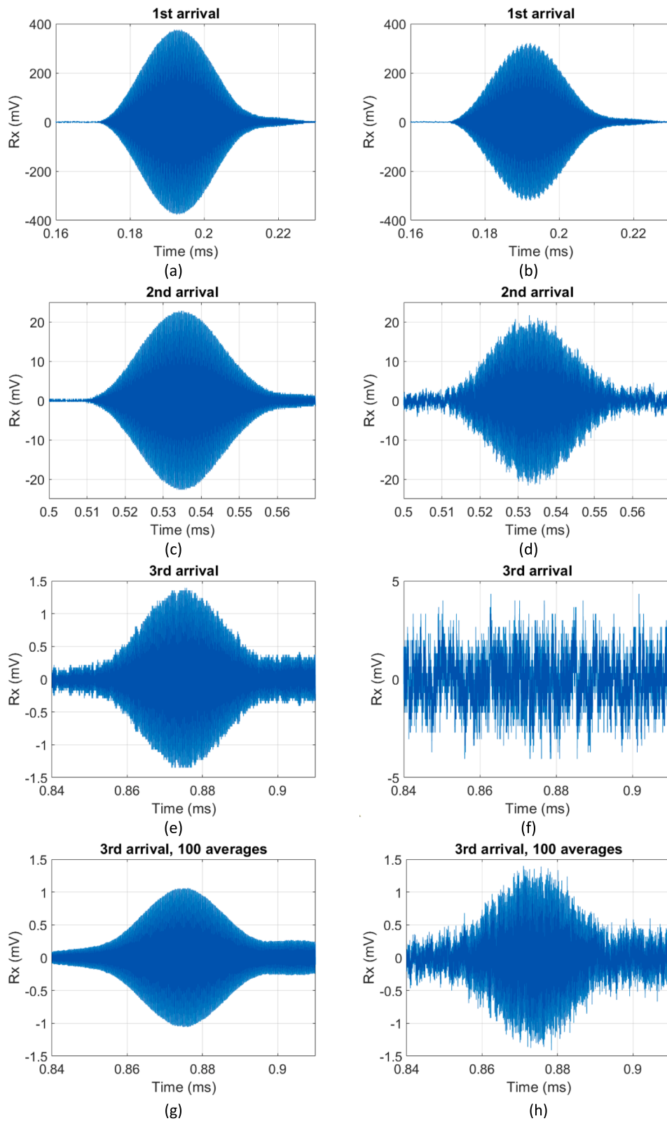
Fig. 7. Comparison of first three arrivals (200 cycles excitation signal) measured with bench-top instruments and USB oscilloscope. (a), (c), and (e) 1st, 2nd and 3rd arrivals with bench-top instruments, (b), (d), and (f) 1st, 2nd and 3rd arrivals with USB oscilloscope, (g) 3rd arrival and 100 averages with bench-top instruments, (h) 3rd arrival and 100 averages with USB oscilloscope.
