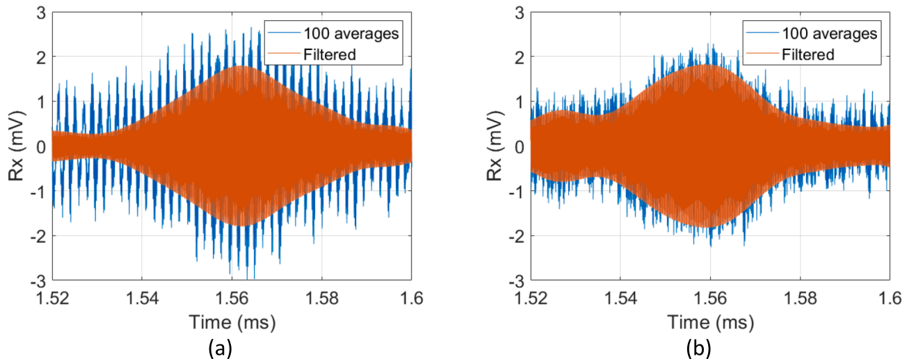
Fig. 9. Comparison of the two oscilloscopes for measuring the 5th arrival: (a) bench-top instruments (b) USB oscilloscope.
