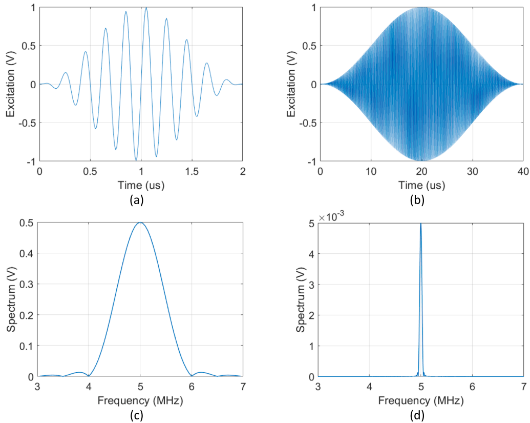
Fig. 2. Tone burst excitation signals with 5 MHz center frequency: (a) 10 cycles; (b) 200 cycles; frequency spectrum of signal with: (c) 10 cycles (bandwidth 2 MHz); (d) 200 cycles (bandwidth 0.1 MHz).
