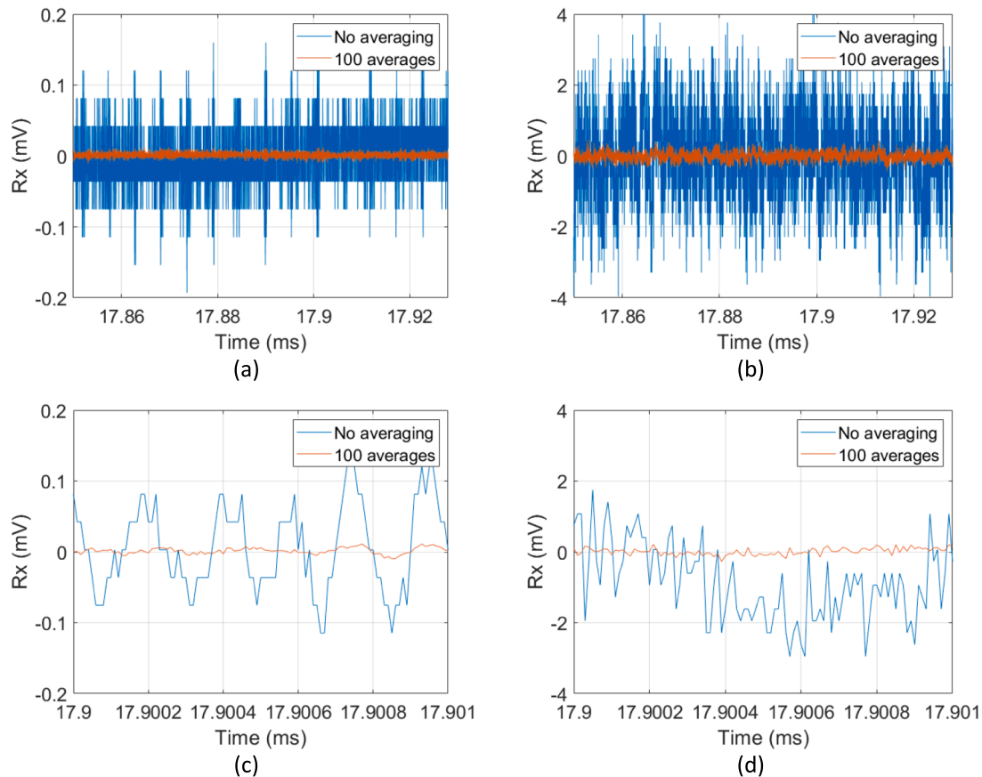
Fig. 5. Comparison of noise measured by (a) bench-top oscilloscope, (b) USB oscilloscope, (c) zoomed view of noise measured by bench-top oscilloscope, (d) zoomed view of noise measured by USB oscilloscope.
