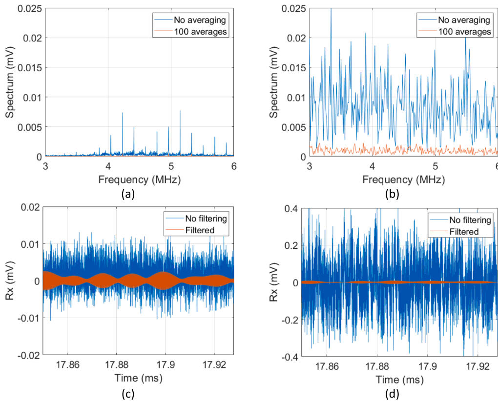
Fig. 6. Frequency content of noise signals (a) measured with bench-top oscilloscope and (b) measured with USB oscilloscope. Influence of bandpass filtering on signals from (c) bench-top oscilloscope and (d) USB oscilloscope.
