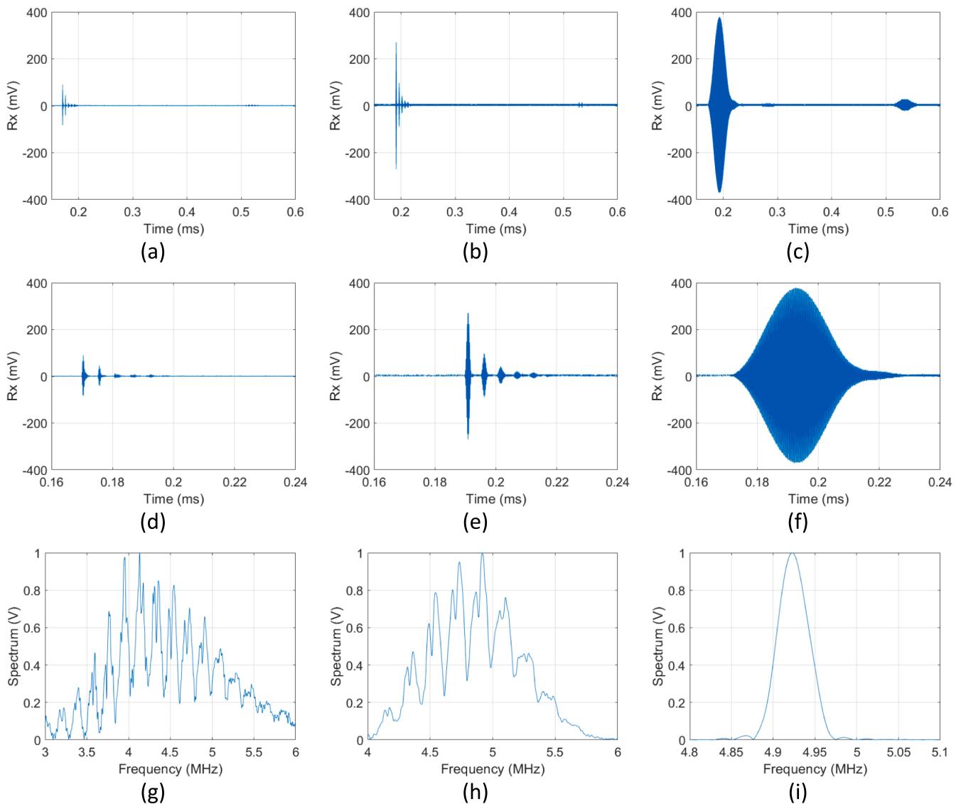
Fig. 4. Influence of number of cycles excitation signal on response signal, (a) rectangular pulse, 1st two arrivals, (b) 10 cycles, 1st two arrivals, (c) 200 cycles, 1st two arrivals, (d) rectangular pulse zoomed view, (e) 10 cycles zoomed view, (f) 200 cycles zoomed view, (g) frequency spectrum of 1st arrival for rectangular pulse excitation signal, (h) frequency spectrum of 1st arrival for 10-cycle excitation signal, (i) frequency spectrum of 1st arrival for 200-cycle excitation.
