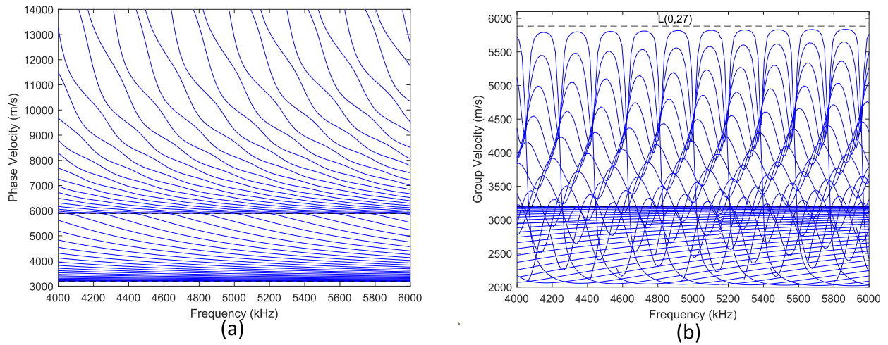
Fig. 1. (a) Phase and (b) group velocity dispersion curves of axisymmetric modes of propagation in a 20 mm diameter steel rod.
