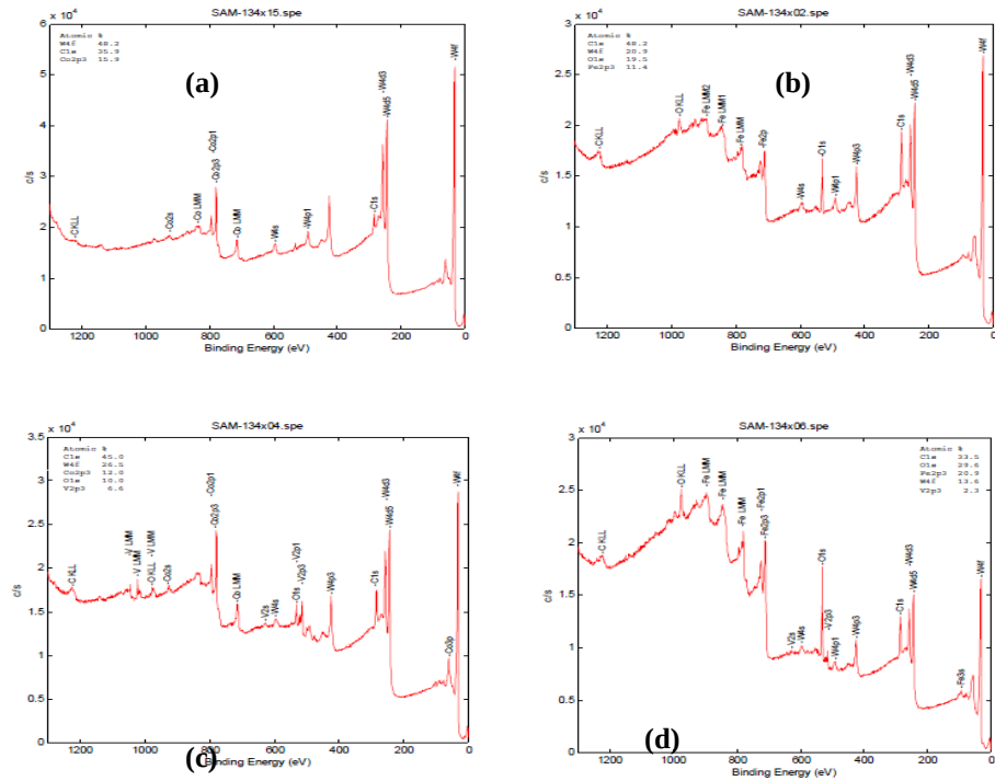
Figure 4. 19 Selected XPS spectra against the 100Cr steel ball for the (a) un-worn track (b) WC-12wt%Co, (c) WC-12wt%Co-10wt%VC, and (c) WC-17wt%Co-10wt%VC coatings.
