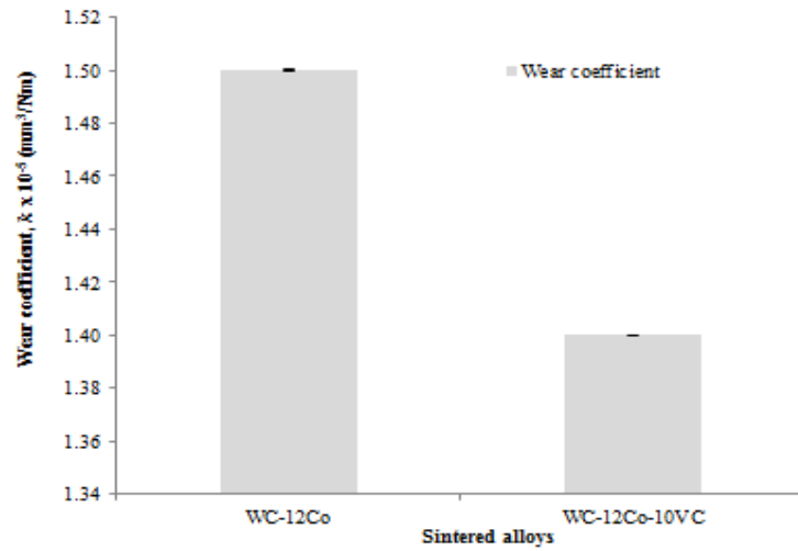
Figure 6. 8 Comparison of the wear coefficients of the sintered alloys against the 100Cr steel balls.
