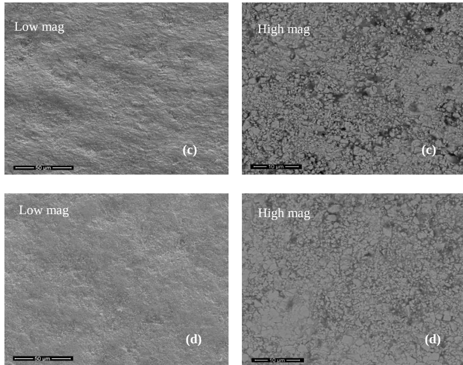
Figure 4. 23 SEM images of the eroded surface of the WC-12wt%Co at (a) 90°, (b) 75°, (c) 60°, and (d) 45°.
