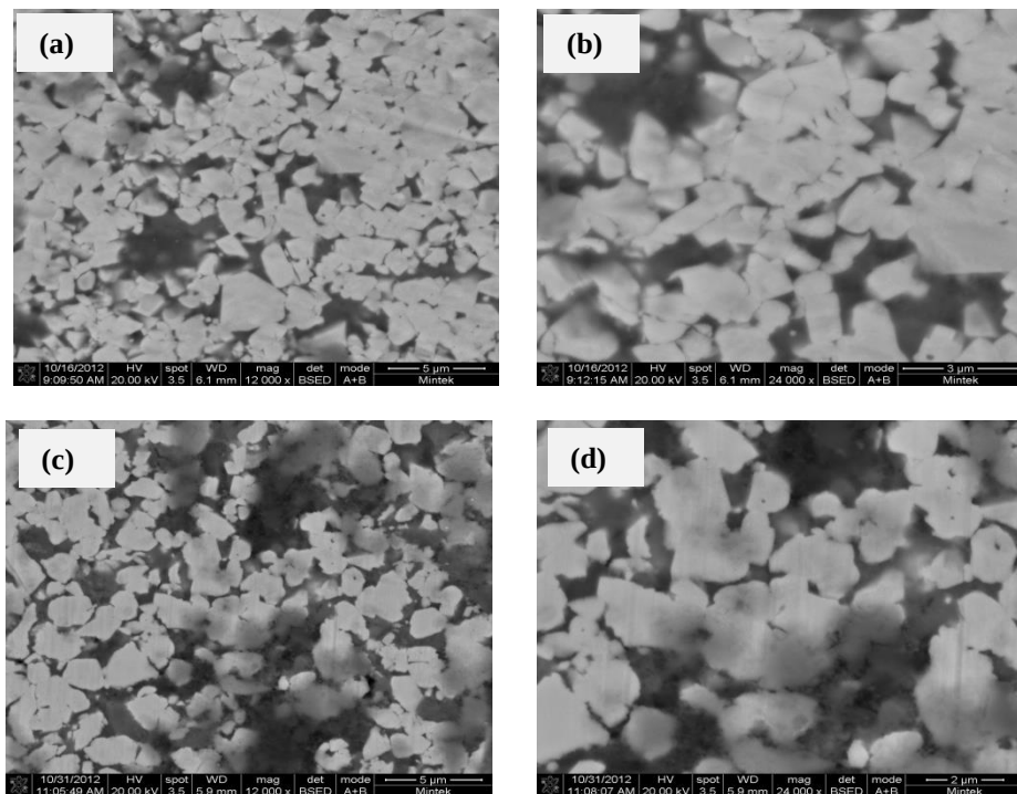
Figure D2. 1 High magnification SEM images of the wear surfaces after sliding against 100Cr steel ball for (a) WC-12wt%Co, and (b) WC-12wt%Co-10wt%VC alloys.
