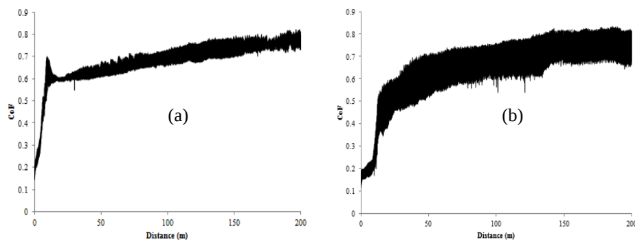
Figure 5. 6 Friction behavior against 100Cr ball for (a) WC-12wt%Co and (b) WC-12wt%Co-10wt%VC alloys.
