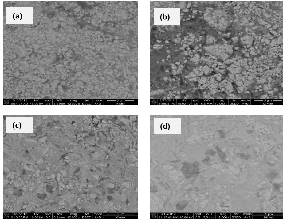
Figure B4B. 1 SEM images of the eroded surface of (a) WC-12wt%Co, (b) WC-12wt%Co-10wt%VC, (c) WC-17wt%Co-10wt%VC (Run 38), and WC-17wt%Co-10wt%VC (Run 39) coatings at 90°.
