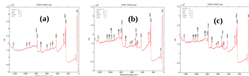
Figure B3B. 1 Wide XPS scan of the wear tracks on the (a) WC-12wt%Co, (b) WC-12wt%Co-10wt%10VC and (c) WC-17wt%Co-10wt%VC coatings
