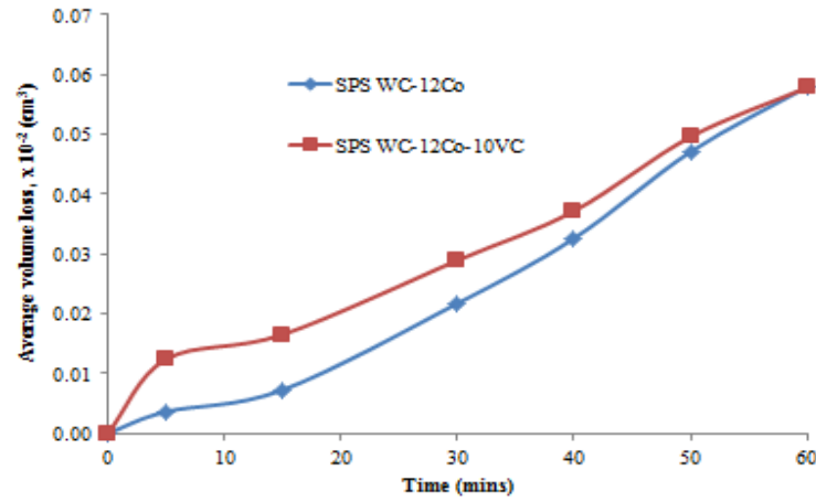
Figure 6. 12 Comparison of the average volume loss against time curves of both alloys at 90°.
