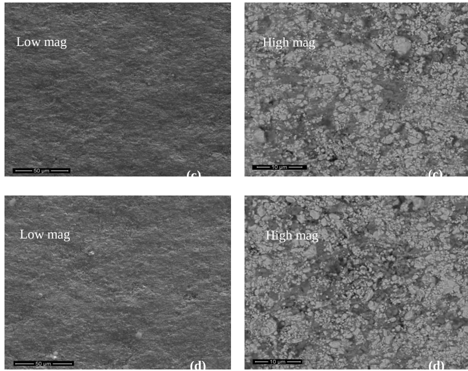
Figure 4. 24 SEM images of the eroded surface of the WC-12wt%Co-10wt%VC at (a) 90°, (b) 75°, (c) 60°, and (d) 45°.
