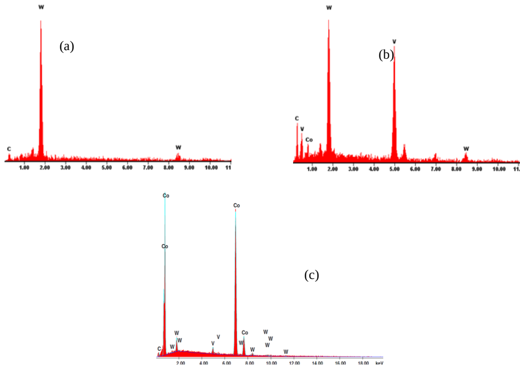
Figure 5. 4 EDS analysis of the (a) white phase showing WC angular grains and (b) dark grey regions showing irregularly shaped (W,V)C grains, and (c) continuous matrix.
