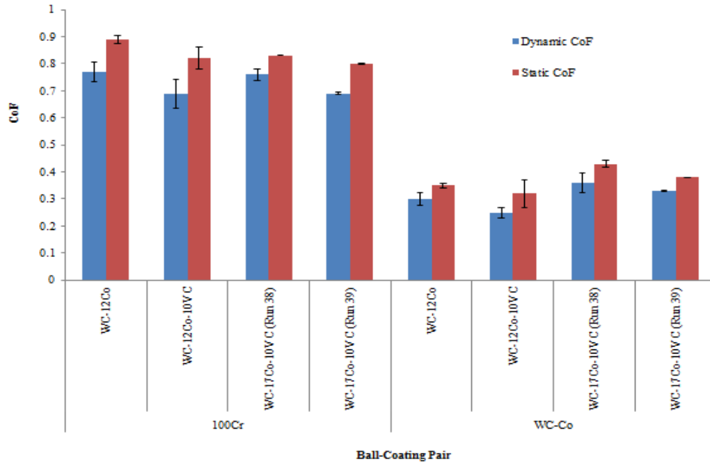
Figure 4. 12 Friction coefficients for the ball-coating pairs.
