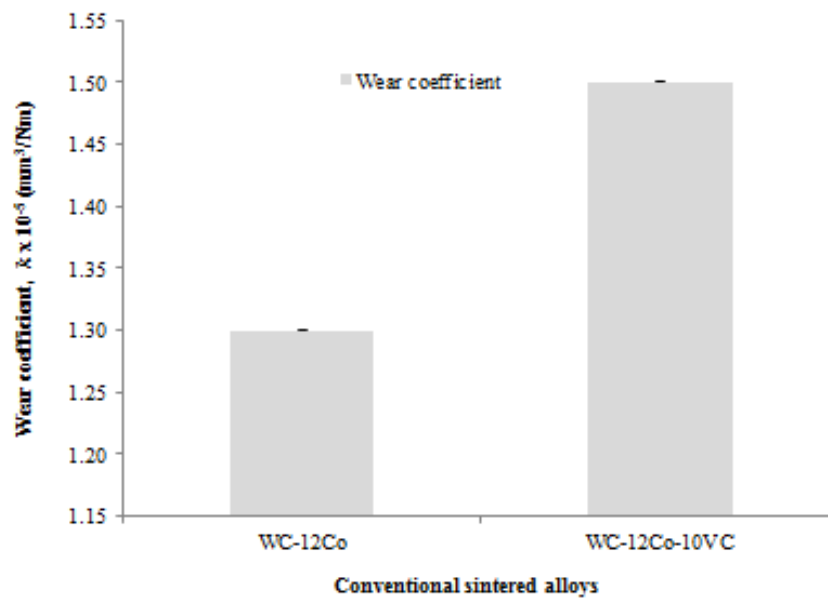
Figure 5. 9 Wear coefficients comparison for the sintered alloys.
