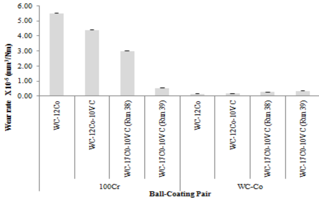
Figure 4. 13 Wear coefficients comparison for the coatings.
