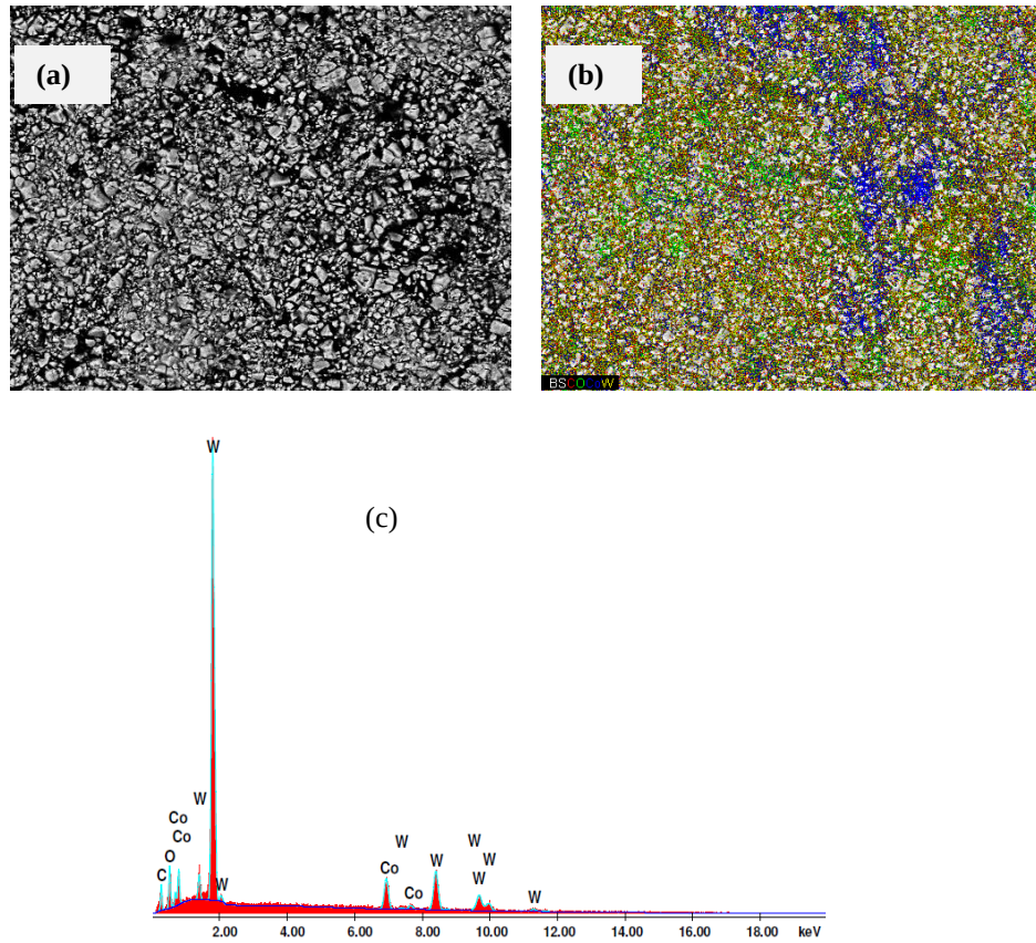
Figure 4. 27 (a) BSE SEM image, (b) EDAX maps overlay and (c) EDX analysis on the eroded surface of the WC-12wt%Co coatings (Brown = C; Blue = Co; Green = O; Yellow = W).
