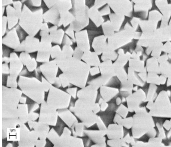
Figure 2. 1 Typical microstructure of sintered WC-12Co alloy (This study).
