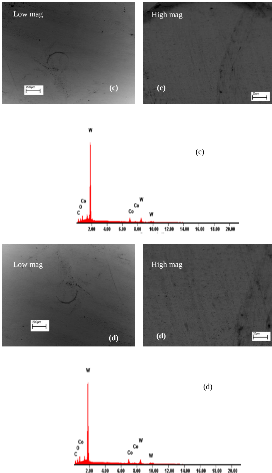
Figure 4. 18 SEM images with EDX analysis of the wear tracks of the WC-Co ball against (a) WC-12wt%Co, (b) WC-12wt%Co-10wt%VC, (c) WC-17wt%Co-10wt%VC (Run 38), and (d) WC-17wt%Co-10wt%VC (Run 39) coatings.
