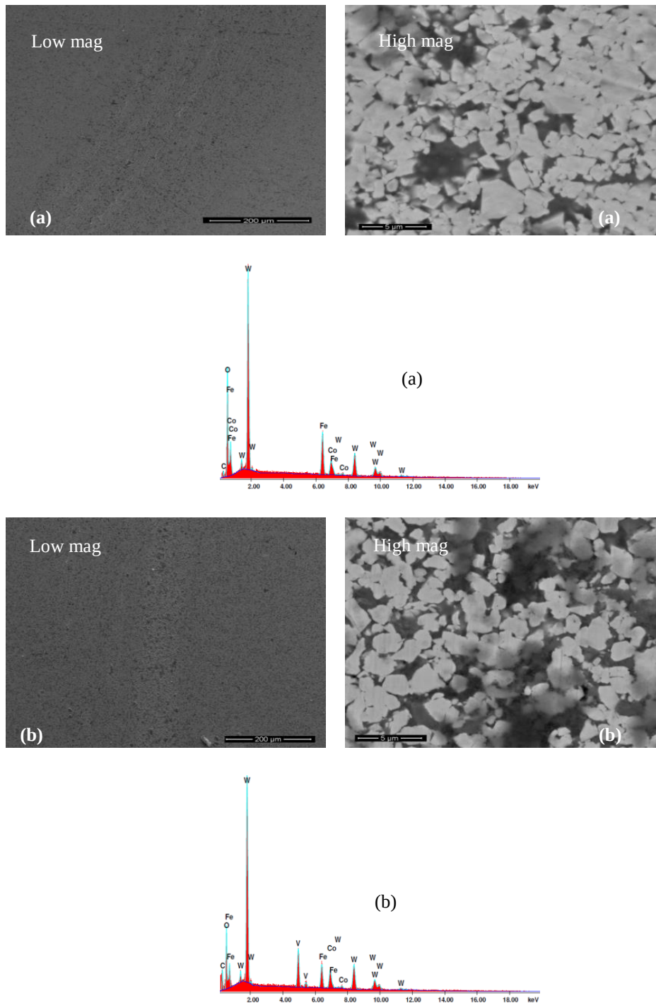
Figure 6. 10 SEM images with EDX analysis of the wear tracks against 100Cr ball for (a) WC-12wt%Co and (b) WC-12wt%Co-10wt%VC alloys.
