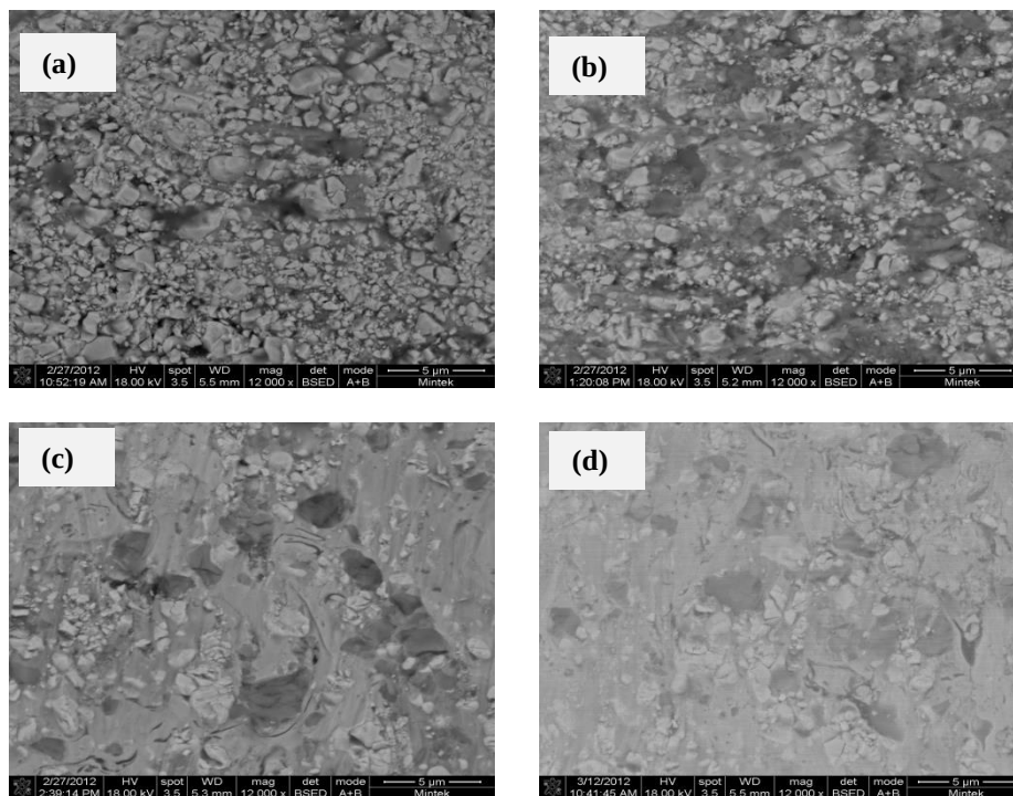
Figure B4B. 3 SEM images of the eroded surface of (a) WC-12wt%Co, (b) WC-12wt%Co-10wt%VC, (c) WC-17wt%Co-10wt%VC (Run 38), and WC-17wt%Co-10wt%VC (Run 39) coatings at 60°.
