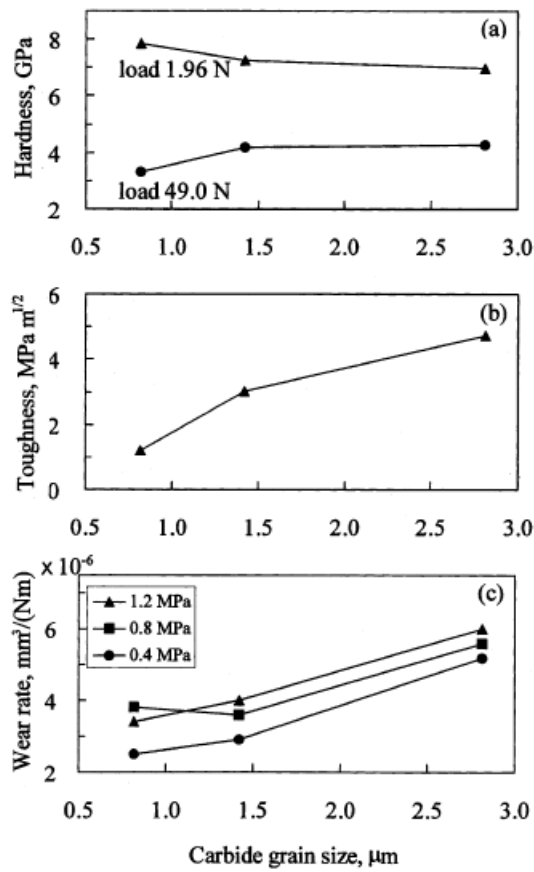
Figure 2. 9 (a) Hardness, (b) fracture toughness, and (c) specific wear rate of WC–Co coatings as a function of carbide grain size. [101].
