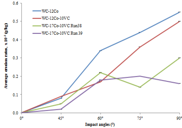
Figure 4. 22 Comparison of the average erosion rate against impact angles.
