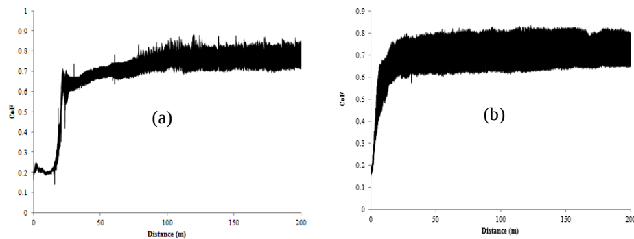
Figure 6. 6 Friction behavior against 100Cr ball for (a) WC-12wt%Co and (b) WC-12wt%Co-10wt%VC alloys.
