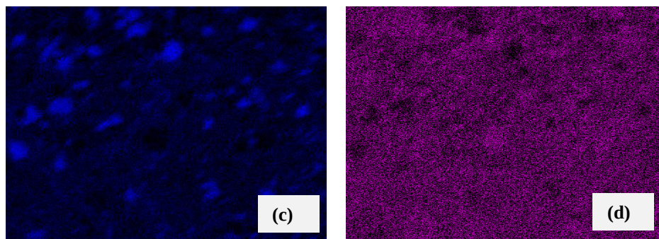
Figure 4. 8 EDAX maps showing the elemental distribution in the WC-17wt%Co-10wt%VC (Run 39) coatings. (a) SEM image (b) Co (c) V and (d) W.
