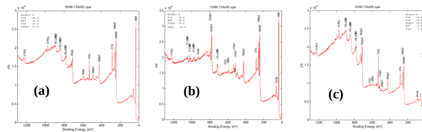
Figure B3A. 1 Wide XPS scan of the wear tracks on the (a) WC-12wt%Co, (b) WC-12wt%Co-10wt%VC and (c) WC-17wt%Co-10wt%VC coatings.
