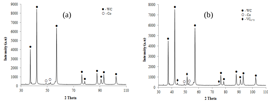
Figure 5. 2 XRD patterns for (a) WC-12wt%Co and (b) WC-12wt%Co-10wt%VC powders.
