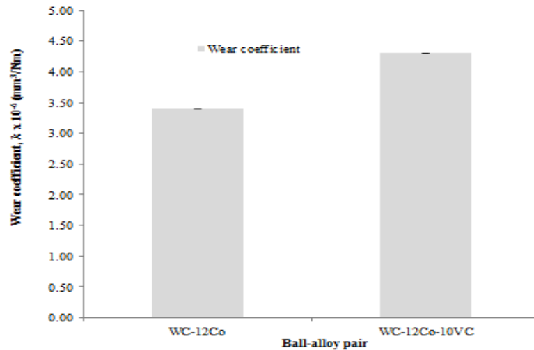
Figure 6. 9 Comparison of the wear coefficients of the 100Cr steel balls sliding pairs against the alloys.
