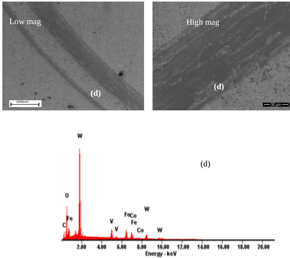
Figure 4. 15 SEM images of the wear tracks against 100Cr ball for (a) WC-12wt%Co, (b) WC-12wt%Co-10wt%VC, (c) WC-17wt%Co-10wt%VC (Run 38), and (d) WC-17wt%Co-10wt%VC (Run 39) coatings.
