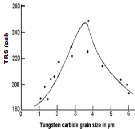
Figure 2. 4 Influence of WC grain size on the transverse rupture strength of WC-6Co hardmetals [35].
