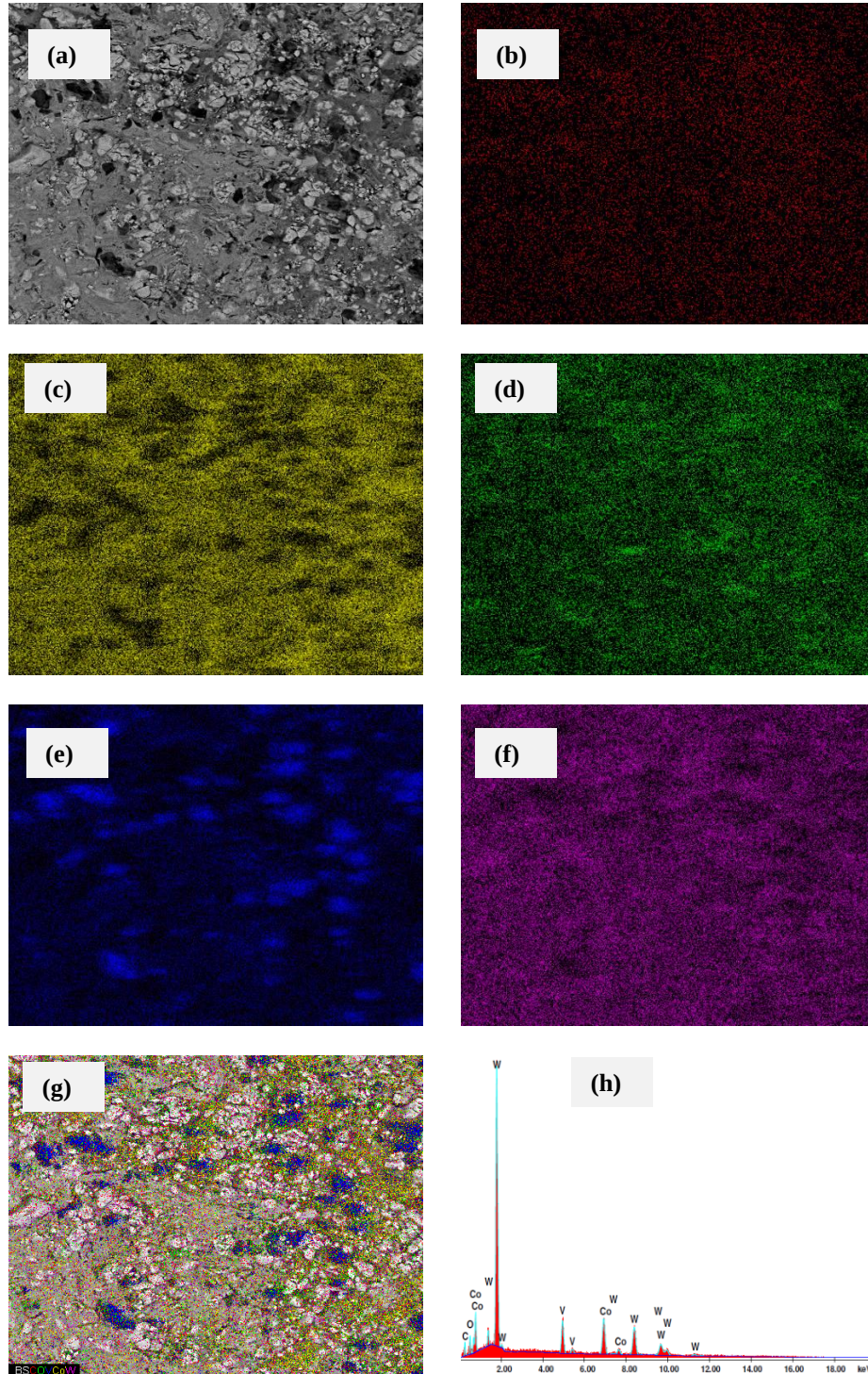
Figure B5. 1 EDAX maps showing the elemental distribution on the eroded surface of the WC-17wt%Co-10wt%VC Run 38 coating (a) BSE SEM image (b) carbon distribution, (c) cobalt distribution, (d) oxygen distribution, (e) vanadium distribution, (f) tungsten distribution, (g) the overlay, and (h) the EDX analysis.
