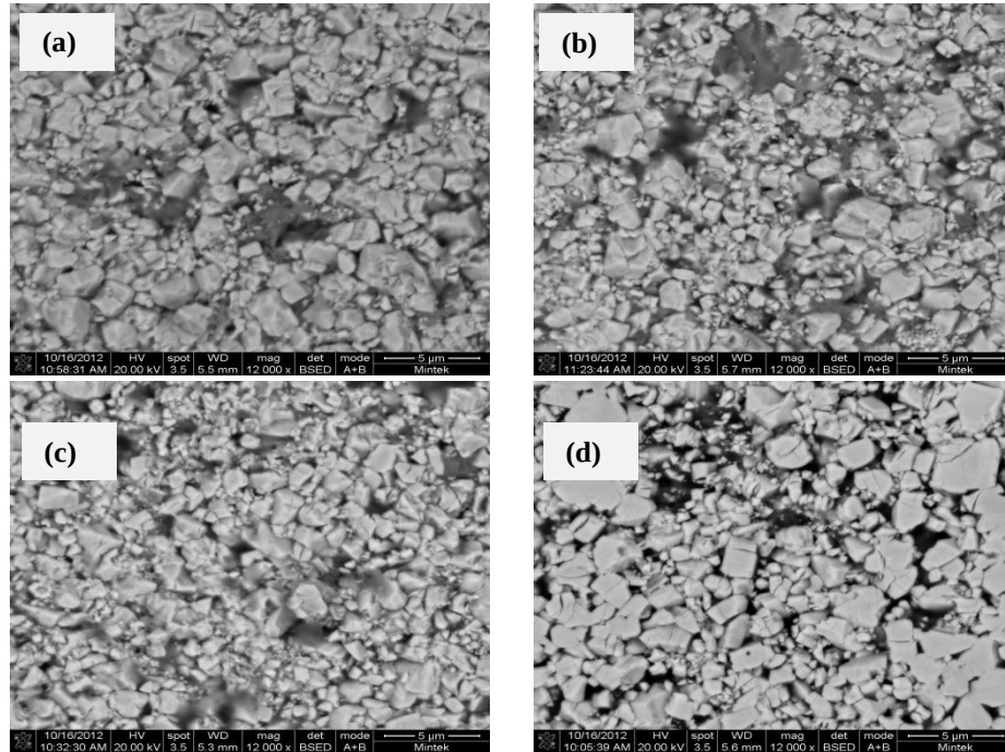
Figure D3B. 1 SEM images of the eroded surface of WC-12wt%Co alloy at (a) 90°, (b) 75°, (c) 60°, and (d) 45°.
