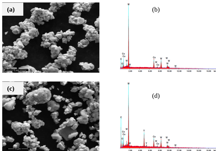
Figure 6. 1 Morphology and EDX analysis of (a) and (b) WC-12wt%Co powder, (b) and (c) WC-12wt%Co-10wt%VC powder.
