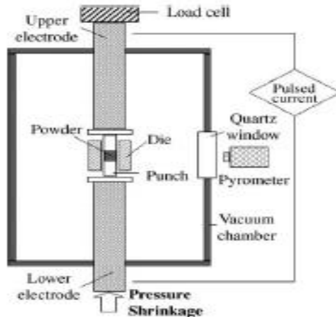
Figure 2. 6 Schematic diagram of a SPS system [54].
