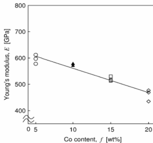
Figure 2. 3 Relationship between Young's modulus and Co content for samples with a WC grain size of 20 \mu\text{m} [34].
