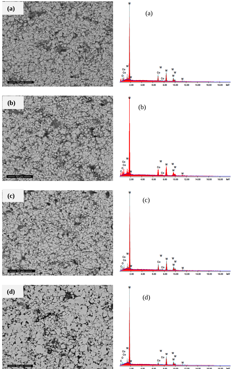
Figure 6. 14 SEM images of the eroded surface of the WC-12wt%Co alloy at (a) 90°, (b) 75°, (c) 60°, and (d) 45°.
