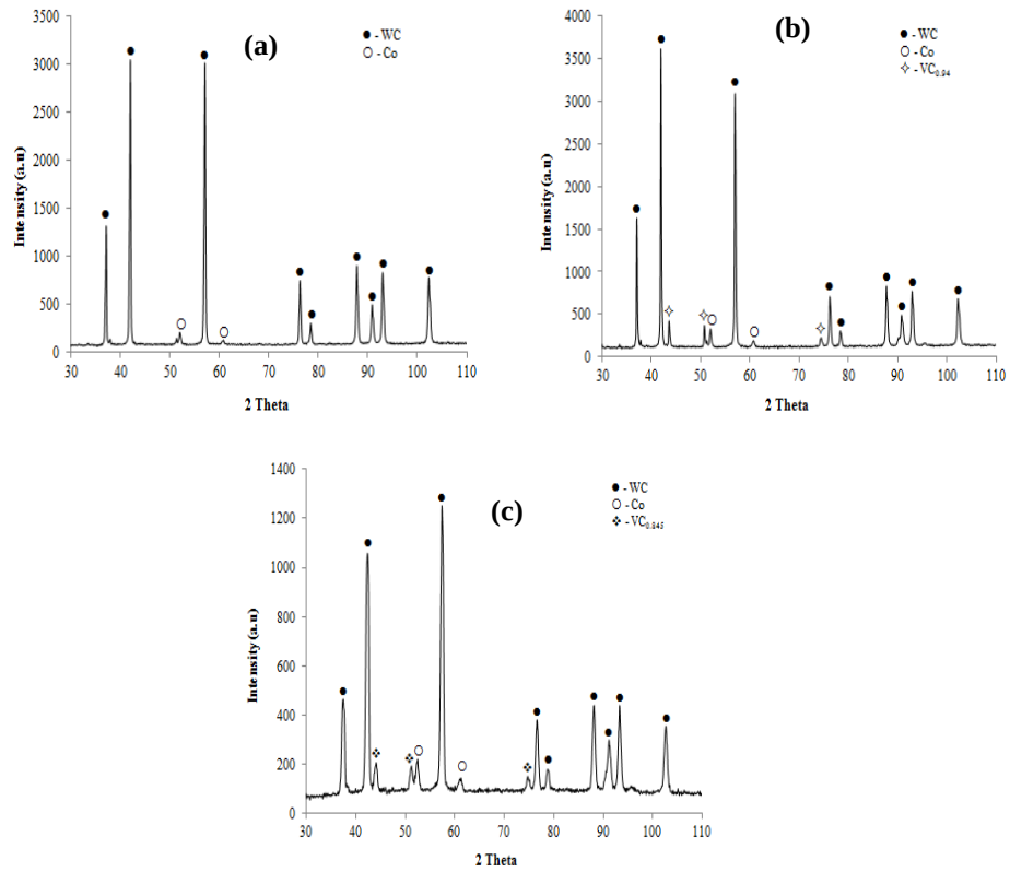
Figure 4. 2 XRD patterns for (a) WC-12wt%Co, (b) WC-12wt%Co-10wt%VC, and (c) WC-17wt%Co-10wt%VC powders.
