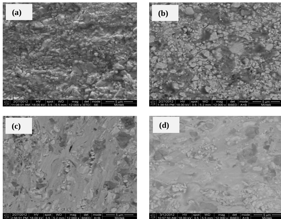
Figure B4B. 2 SEM images of the eroded surface of (a) WC-12wt%Co, (b) WC-12wt%Co-10wt%VC, (c) WC-17wt%Co-10wt%VC (Run 38), and WC-17wt%Co-10wt%VC (Run 39) coatings at 75°.
