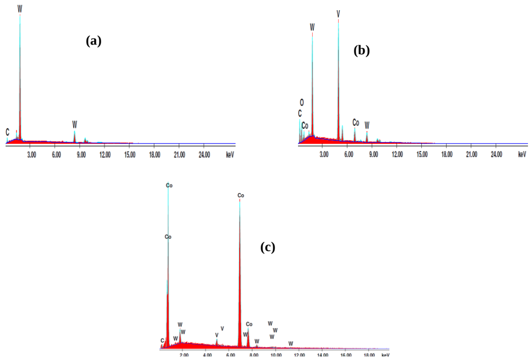
Figure 4. 5 EDS analysis of the (a) white phase showing WC roundish grains and (b) dark grey regions showing irregularly shaped (W,V)C grains, and (c) continuous matrix.
