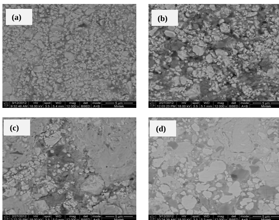
Figure B4B. 4 SEM images of the eroded surface of (a) WC-12wt%Co, (b) WC-12wt%Co-10wt%VC, (c) WC-17wt%Co-10wt%VC (Run 38), and WC-17wt%Co-10wt%VC (Run 39) coatings at 45°.
