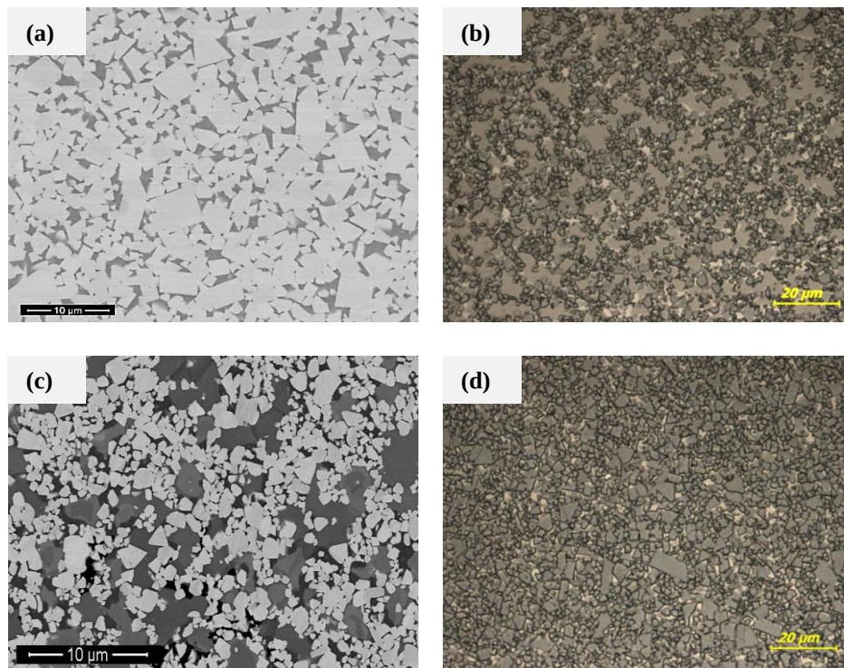
Figure 5. 3 SEM and optical images of the (a) un-etched WC-12wt%Co, (b) etched WC-12wt%Co, (c) un-etched WC-12wt%Co-10wt%VC, and (d) etched WC-12wt%Co-10wt%VC alloys. WC grains appear as white particles; Co binder phase as continuous region; and (W,V)C grains as irregularly shaped dark grey regions. The black regions/spots are pores.
