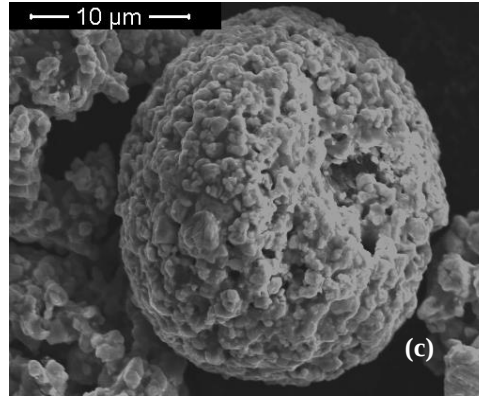
Figure 4. 1 Morphologies of the (a) WC-12wt%Co, (b) WC-12wt%Co-10wt%VC and (c) WC-17wt%Co-10wt%VC powders.
