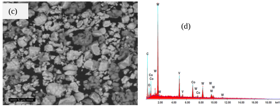
Figure 5. 1 Morphology and EDX analysis of (a) and (b) WC-12wt%Co powder, (b) and (c) WC-12wt%Co-10wt%VC powder.
