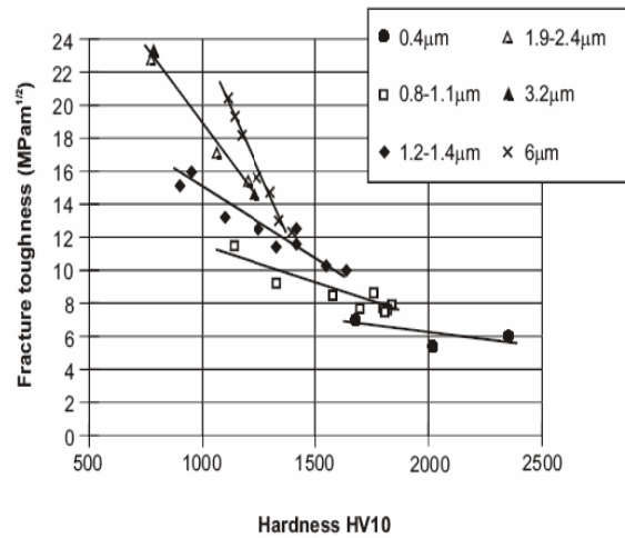
Figure 2. 2 Fracture toughness against hardness for a range of WC-Co hardmetals with differing grain sizes and binder contents [32].
