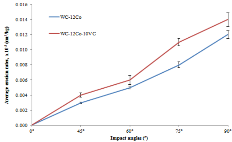
Figure 6. 13 Comparison of the average erosion rate against impact angles.
