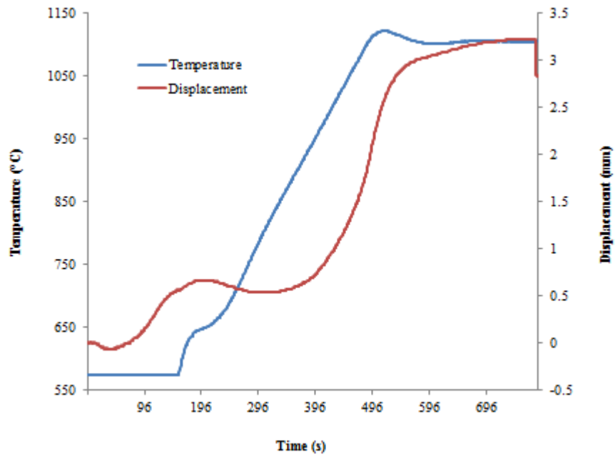
Figure 3. 2 Sintering profile for WC-12wt%Co-10wt%VC SPS alloy.
