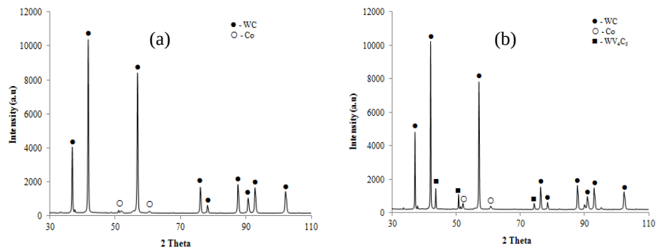
Figure 5. 5 XRD patterns for (a) WC-12wt%Co and (b) WC-12wt%Co-10wt%VC alloys.
