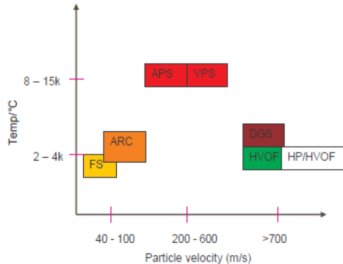
Figure 2. 7 Flame temperature-particle velocity combinations of various thermal spray techniques. FS: flame spray; ARC: arc spray; APS/VPS: air/vacuum plasma spraying; DGS: detonation gun spray; HP/HVOF: high pressure, high velocity oxy-fuel spraying [73].
