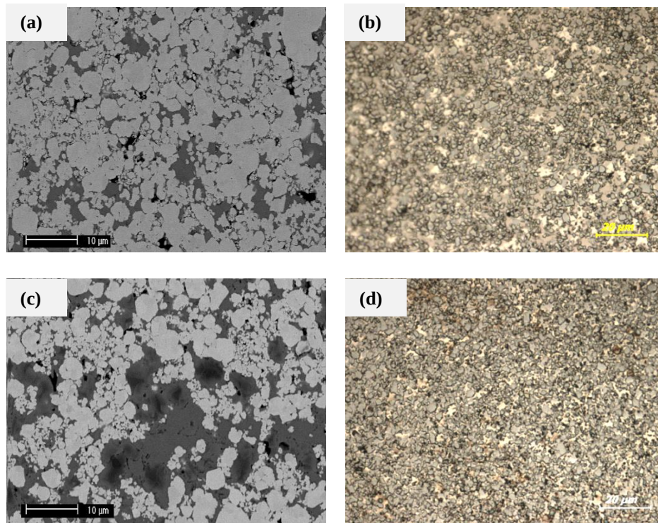
Figure 6. 3 SEM and optical images of the (a) un-etched WC-12wt%Co, (b) etched WC-12wt%Co, (c) un-etched WC-12wt%Co-10wt%VC, and (d) etched WC-12wt%Co-10wt%VC alloys. WC grains appear as white particles; Co binder phase as continuous region; and (W,V)C grains as irregularly shaped dark grey regions. The black regions/spots are pores.
