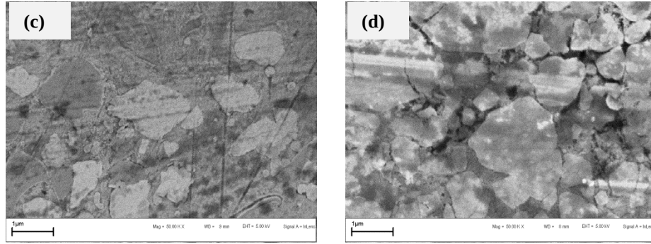
Figure B2. 2 High magnifications SEM images against the 100Cr steel ball on the wear tracks of (a) WC-12wt%Co, (b) WC-12wt%Co-10wt%VC, (c) WC-17wt%Co-10wt%VC (Run 38), and (d) WC-17wt%Co-10wt%VC (Run 39) coatings.
