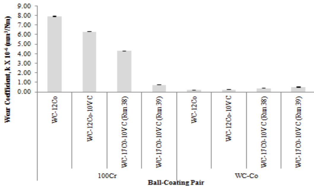
Figure 4. 14 Wear coefficients comparison for the balls.
