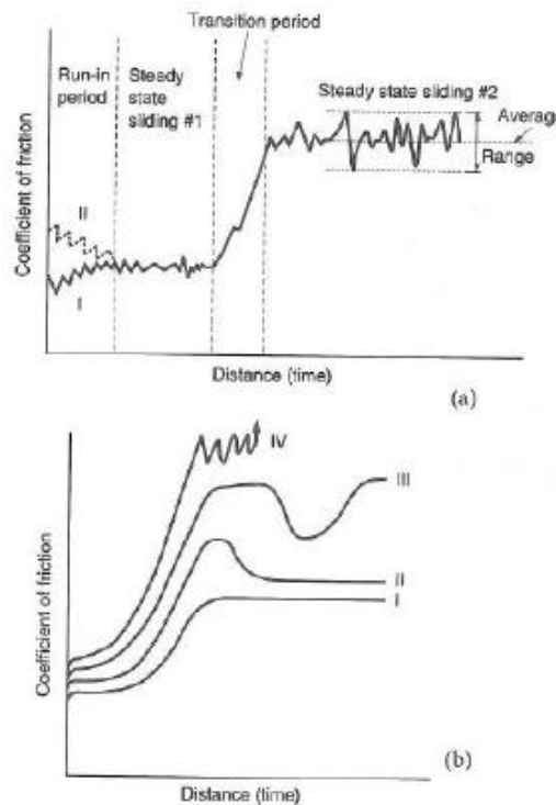
Figure 2. 10 The coefficient of friction as a function of sliding distance. (a) A typical S-shaped curve (b) Four hypothetical friction patterns [112].
