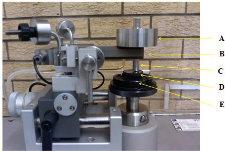
Figure 3. 4 Measurement head of the tribometer (A) Applied load, (B) Elastic blade arm, (C) Ball holder, (D) Sample, (E) Disk mandrel.
