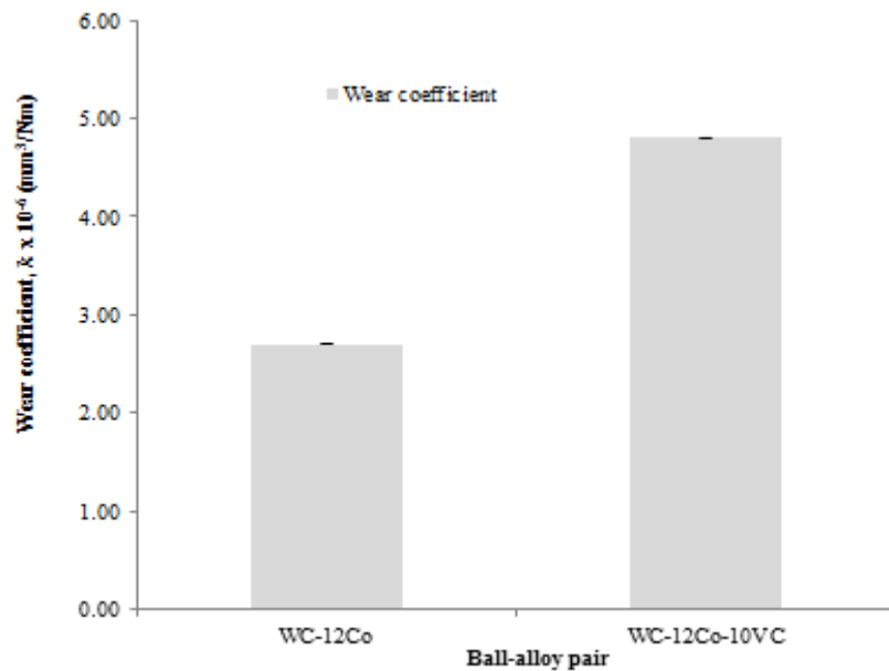
Figure 5. 8 Comparison of the wear coefficients of the 100Cr steel ball-alloy sliding pairs.
