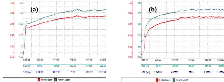
Figure C1. 1 Friction response against the 100Cr steel ball for (a) WC-12wt%Co, and (b) WC-12wt%Co-10wt%VC alloys
