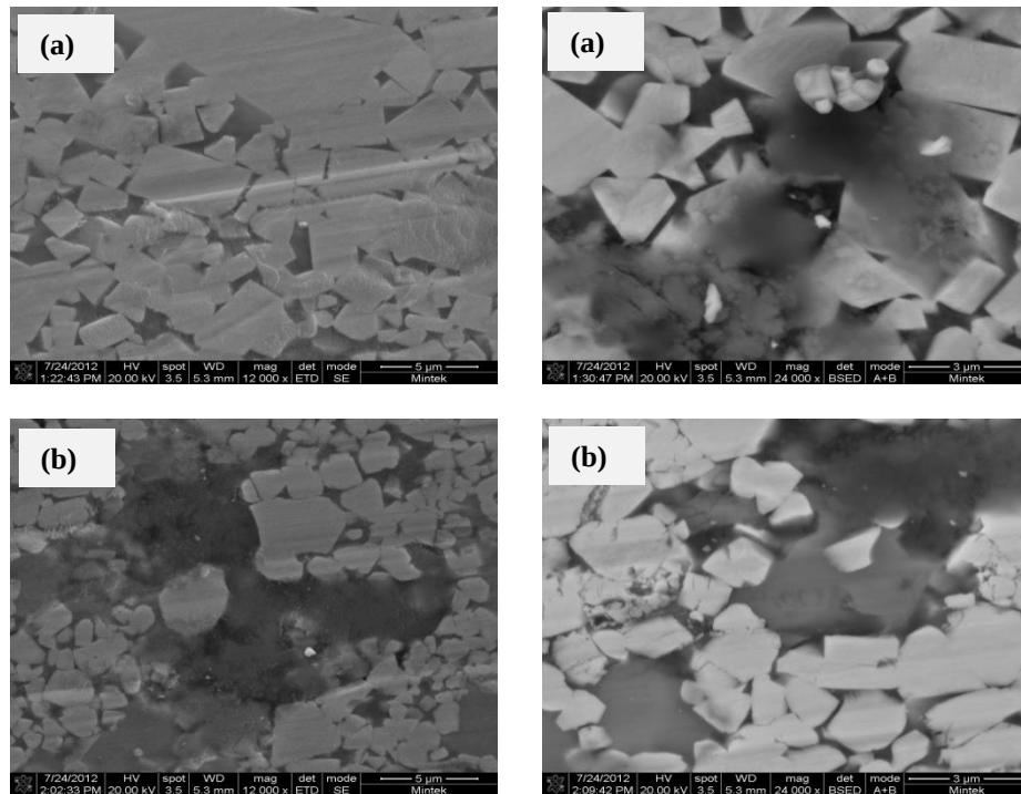
Figure C2. 1 High magnification SEM images of the wear surfaces after sliding against 100Cr steel ball for (a) WC-12wt%Co, and (b) WC-12wt%Co-10wt%VC alloys.
