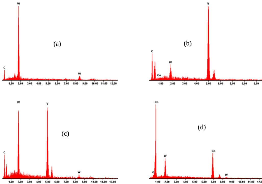
Figure 6. 4 EDS analysis of the (a) white phase showing roundish WC grains and (b & c) light and dark grey regions showing irregularly shaped (W,V)C grains, and (d) continuous matrix.
