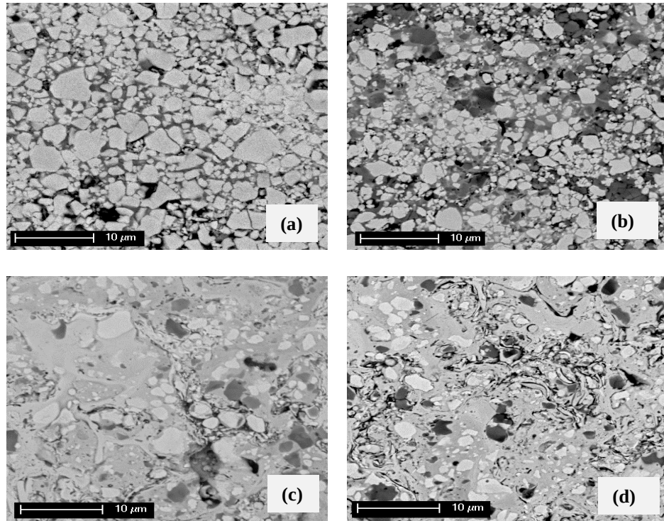
Figure 4. 4 BSE image of (a) WC-12wt%Co, (b) WC-12wt%Co-10wt%VC, (c) WC-17wt%Co-10wt%VC (Run 38) and (d) WC-17wt%Co-10wt%VC (Run 39) coatings. WC grains appear as roundish white particles; Co binder phase as a continuous light grey region; and (W,V)C grains as irregularly shaped dark grey regions. The black regions/spots are pores.
