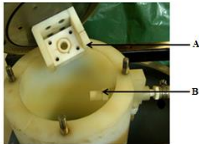
Figure 3. 8 Photograph of the impact chamber showing the sample holder (A) and the exit nozzle (B).
