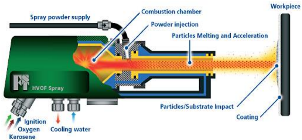
Figure 2. 8 Schematic diagram of HVOF combustion chamber [79].
