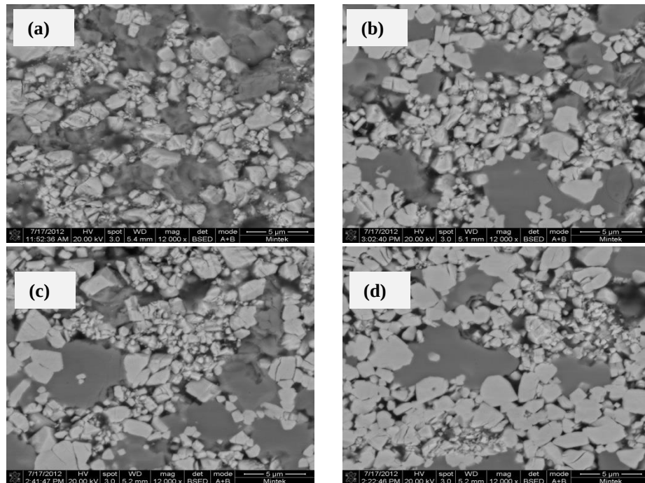
Figure C3B. 2 SEM images of the eroded surface of WC-12wt%Co-10wt%VC alloy at (a) 90°, (b) 75°, (c) 60°, and (d) 45°.
