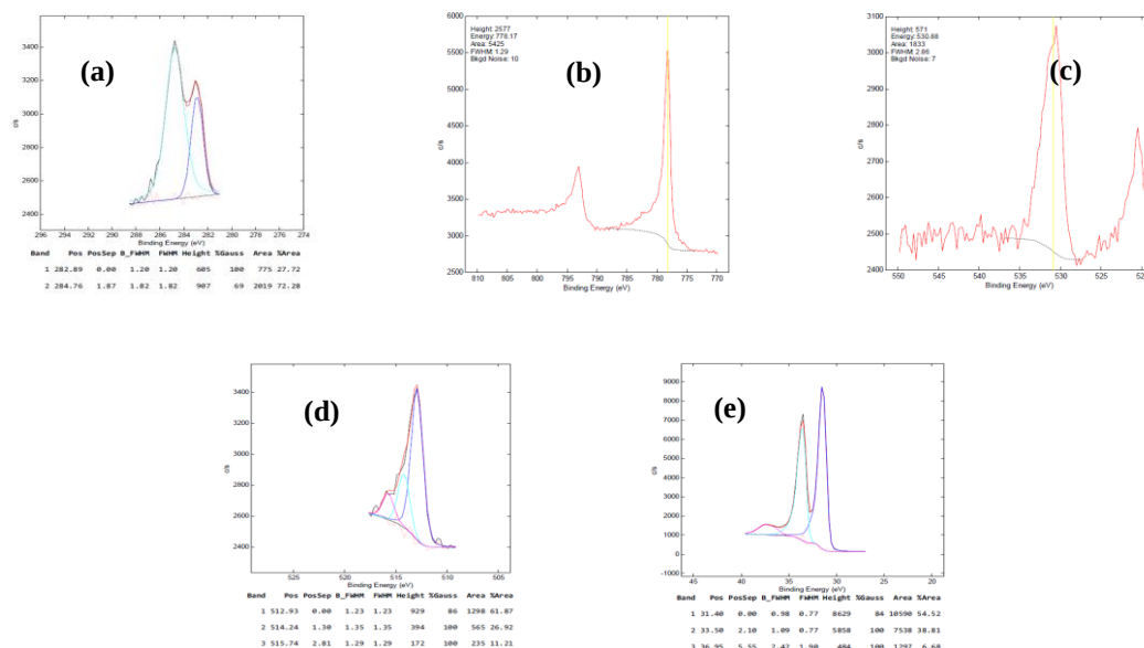
Figure B3A. 3 Narrow XPS of the worn track of the WC-12wt%Co-10wt%VC coating showing (a) carbon (b) cobalt (c) oxygen (d) vanadium and (e) tungsten peaks. The inserted tables show the de-convolution of peaks.
