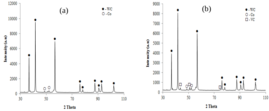
Figure 6. 2 XRD patterns for (a) WC-12wt%Co (b) WC-12wt%Co-10wt%VC powders.
