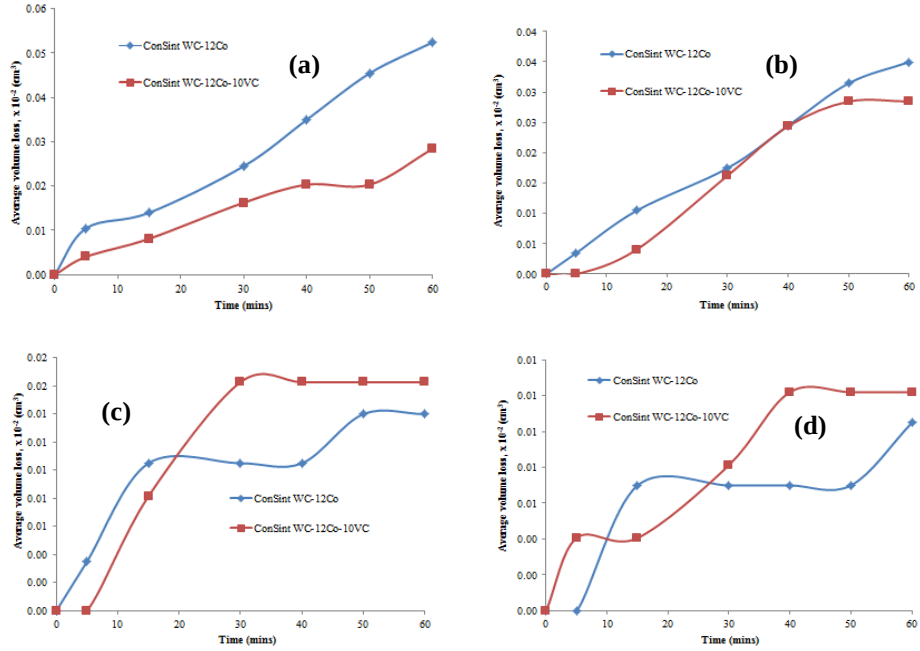
Figure C3A. 1 Average mass losses against time curves for (a) 90°, (b) 75°, (c) 60°, and (d) 45°.
