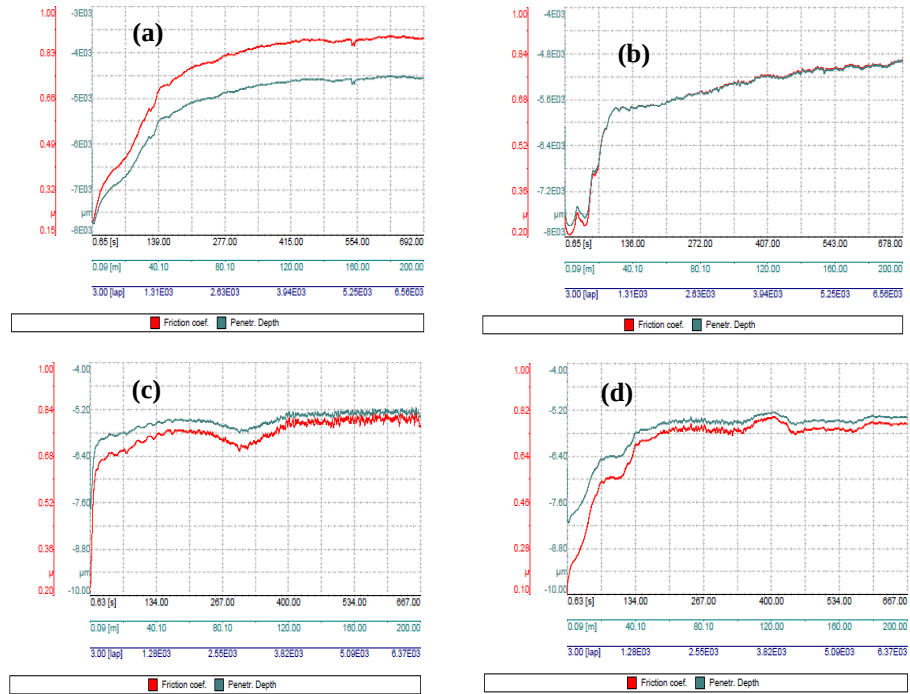
Figure B1. 1 Friction response against 100Cr steel ball against (a) WC-12wt%Co, (b) WC-12wt%Co-10wt%VC, (c) WC-17wt%Co-10wt%VC (Run 38), and (d) WC-17wt%Co-10wt%VC (Run 39) coatings.
