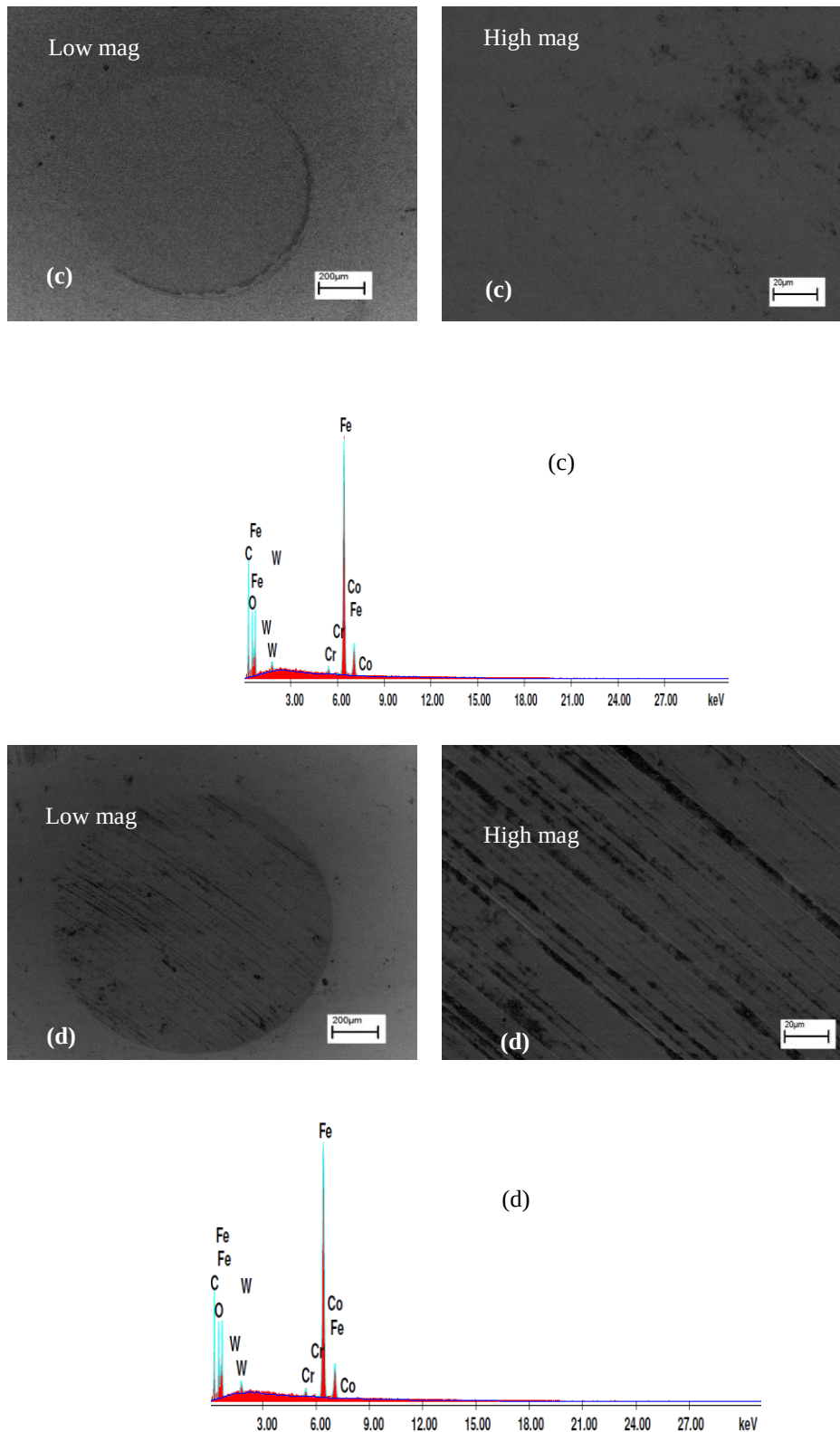
Figure 4. 17 SEM image with EDX analysis of the wear tracks on the 100Cr steel ball against (a) WC-12wt%Co, (b) WC-12wt%Co-10wt%VC, (c) WC-17wt%Co-10wt%VC (Run 38), and (d) WC-17wt%Co-10wt%VC (Run 39) coatings.
