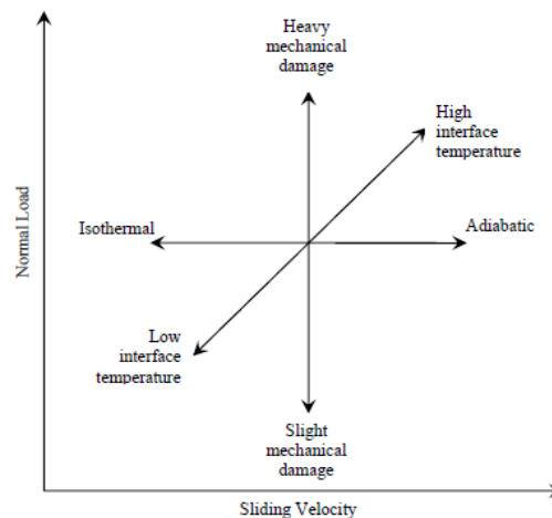
Figure 2. 12 Diagram illustrating the combined influences of load and sliding speed on the sliding wear process [113].
