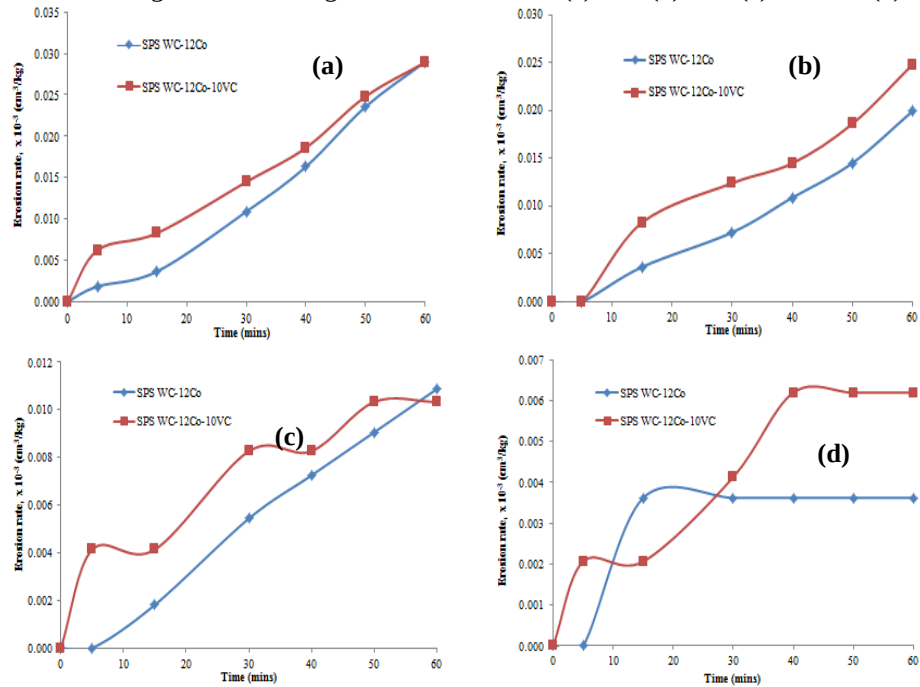
Figure D3A. 2 Average mass losses against time curves for (a) 90°, (b) 75°, (c) 60°, and (d) 45°.
