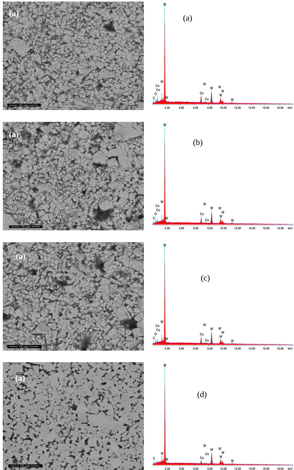
Figure 5 14 SEM images of the eroded surface of the WC-12wt%Co at (a) 90°, (b) 75°, (c) 60°, and (d) 45°.
