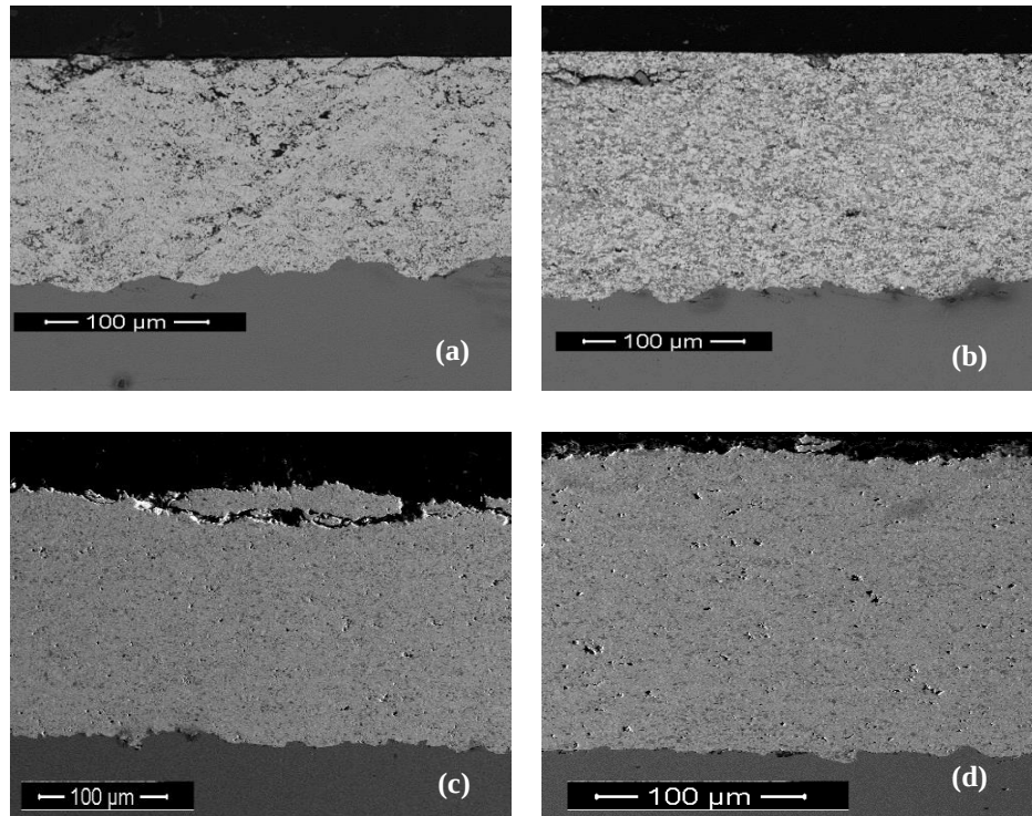
Figure 4. 3 Optical images showing the cross-section of the coating-substrate interface for (a) WC-12wt%Co, (b) WC-12wt%Co-10wt%VC, (c) WC-17wt%Co-10wt%VC (Run 38) and (d) WC-17wt%Co-10wt%VC (Run 39) coatings.
