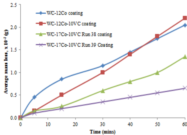
Figure 4. 21 Comparison of the average mass loss against time curves of the coatings at 90° impact angle.
