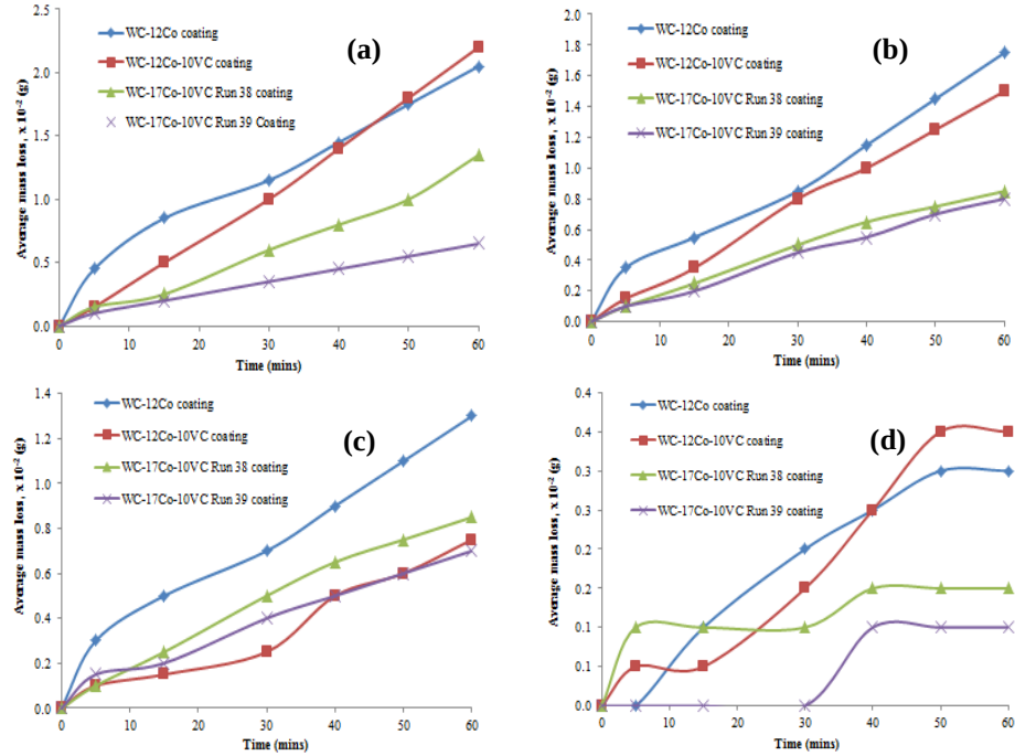
Figure B4A. 1 Average mass losses against time curves for (a) 90°, (b) 75°, (c) 60°, and (d) 45°.
