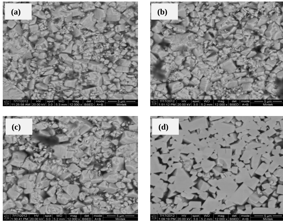
Figure C3B. 1 SEM images of the eroded surface of WC-12wt%Co alloy at (a) 90°, (b) 75°, (c) 60°, and (d) 45°.
