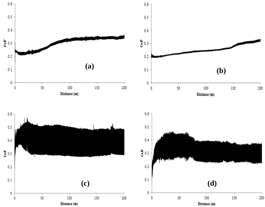
Figure 4. 11 Friction behavior against WC-Co ball for (a) WC-12wt%Co, (b) WC-12wt%Co-10wt%VC, (c) WC-17wt%Co-10wt%VC (Run 38), and (d) WC-17wt%Co-10wt%VC (Run 39) coatings.
