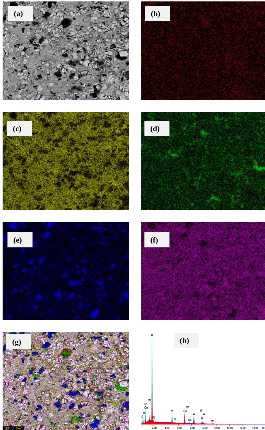
Figure B5. 2 EDAX maps showing the elemental distribution on the eroded surface of the WC-17wt%Co-10wt%VC Run 39 coating (a) BSE SEM image (b) carbon distribution, (c) cobalt distribution, (d) oxygen distribution, (e) vanadium distribution, (f) tungsten distribution, (g) the overlay, and (h) the EDX analysis.
