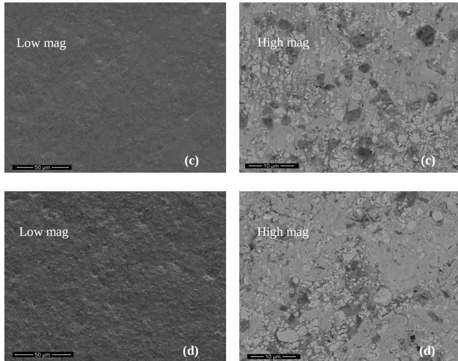
Figure 4. 25 SEM images of the eroded surface of the WC-17wt%Co-10wt%VC Run 38 at (a) 90°, (b) 75°, (c) 60°, and (d) 45°.
