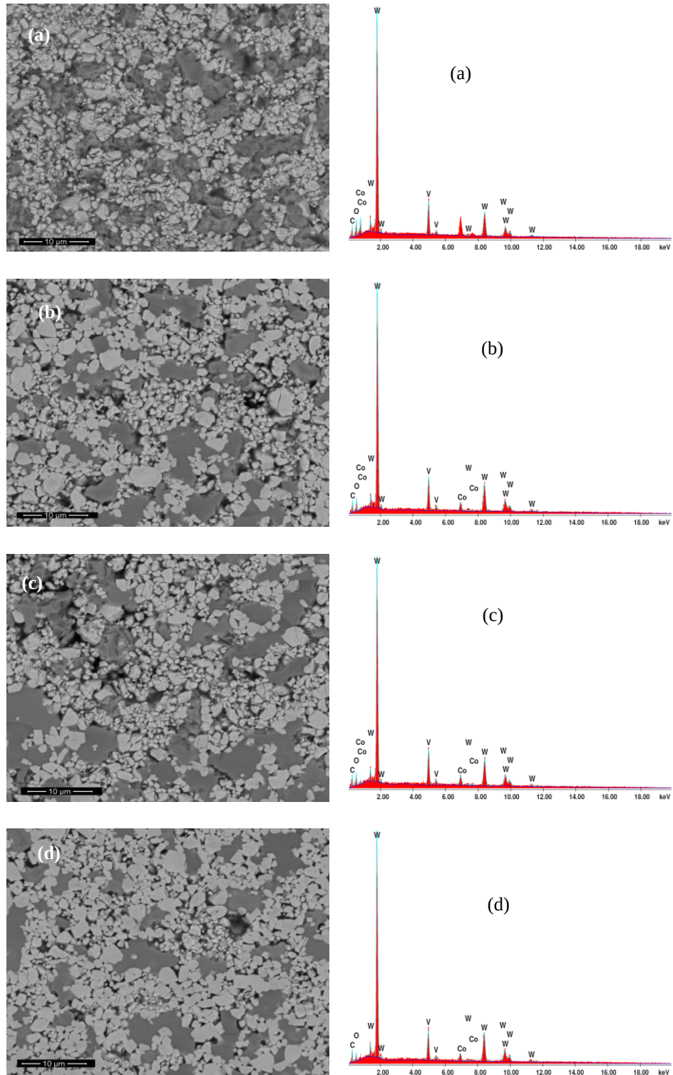
Figure 5. 15 SEM images of the eroded surface of the WC-12wt%Co-10wt%VC at (a) 90°, (b) 75°, (c) 60°, and (d) 45°.
