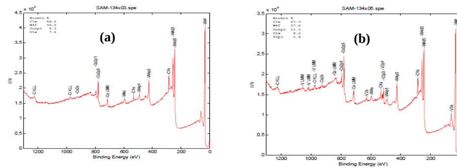
Figure 4. 20 Selected XPS spectra against the WC-Co ball for the (a) WC-12wt%Co, and (b) WC-12wt%Co-10wt%VC coatings.
