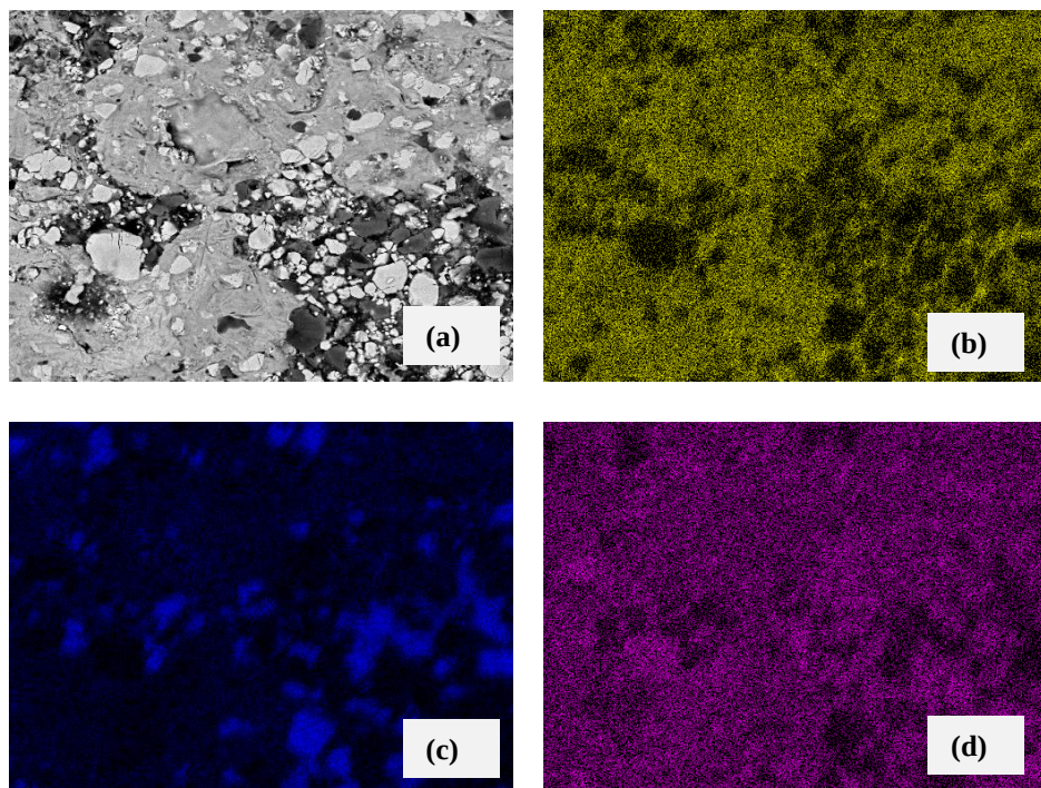
Figure 4. 7 EDAX maps showing the elemental distribution in the WC-17wt%Co-10wt%VC (Run 38) coatings. (a) SEM image (b) Co (c) V and (d) W.
