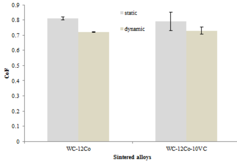
Figure 6. 7 Friction coefficients for the alloy-ball pairs.
