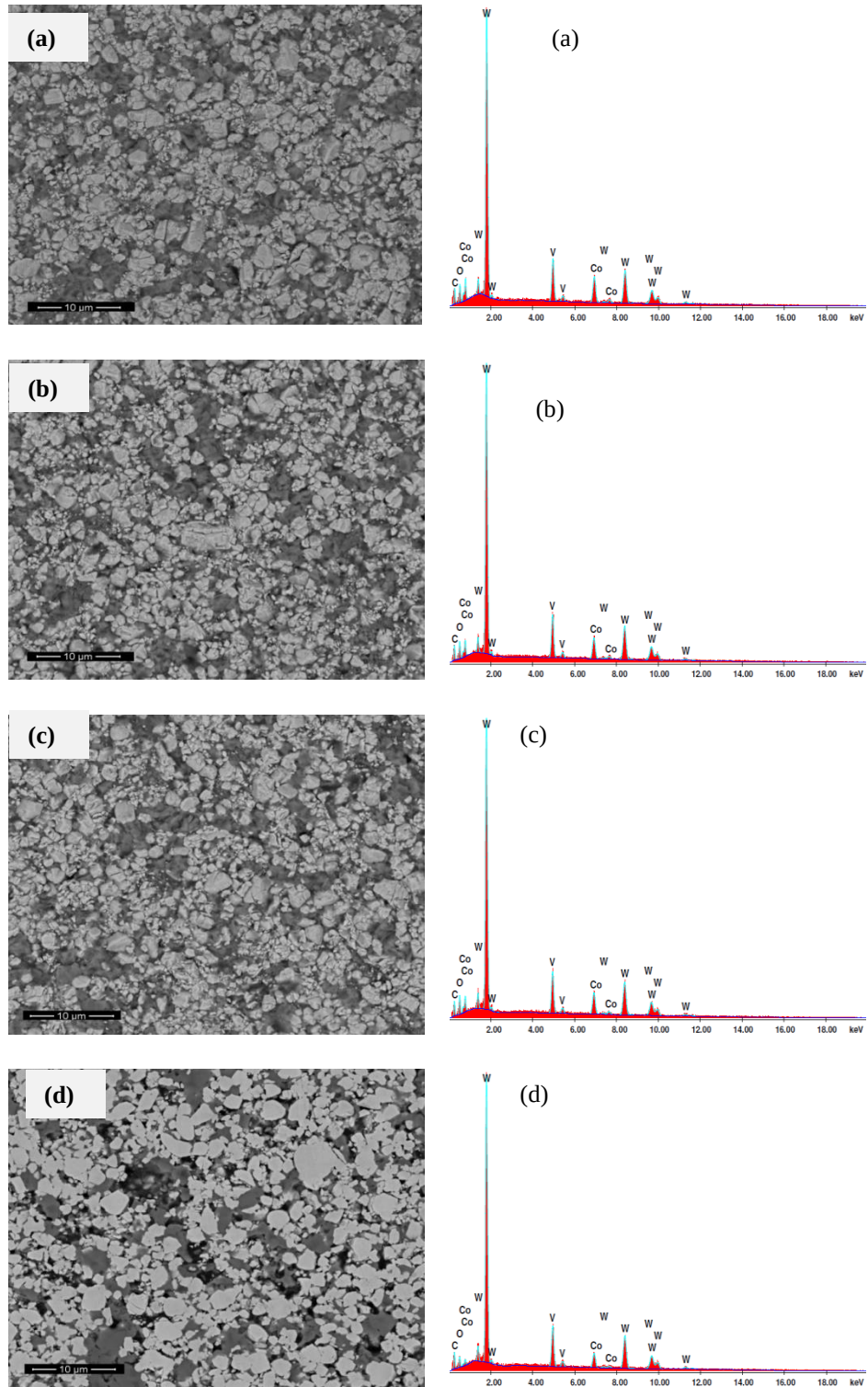
Figure 6. 15 SEM images of the eroded surface of the WC-12wt%Co-10wt%VC alloy at (a) 90°, (b) 75°, (c) 60°, and (d) 45°.
