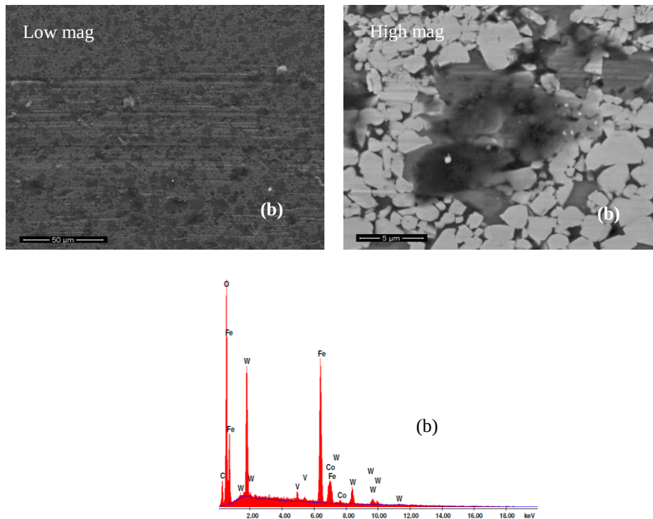
Figure 5. 10 SEM images with EDX analysis of the wear tracks against 100Cr ball for (a) WC-12wt%Co and (b) WC-12wt%Co-10wt%VC alloys.
