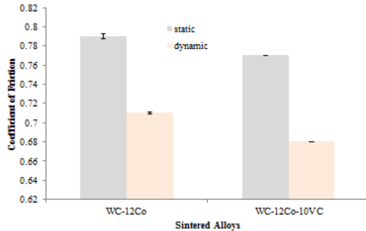
Figure 5. 7 Friction coefficients for the alloy-ball pairs sliding against the 100Cr steel balls.
