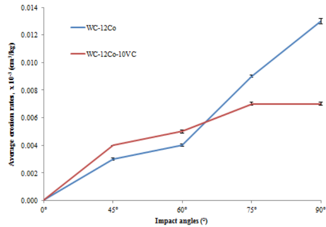
Figure 5. 13 Comparison of the average erosion rate against impact angles.
