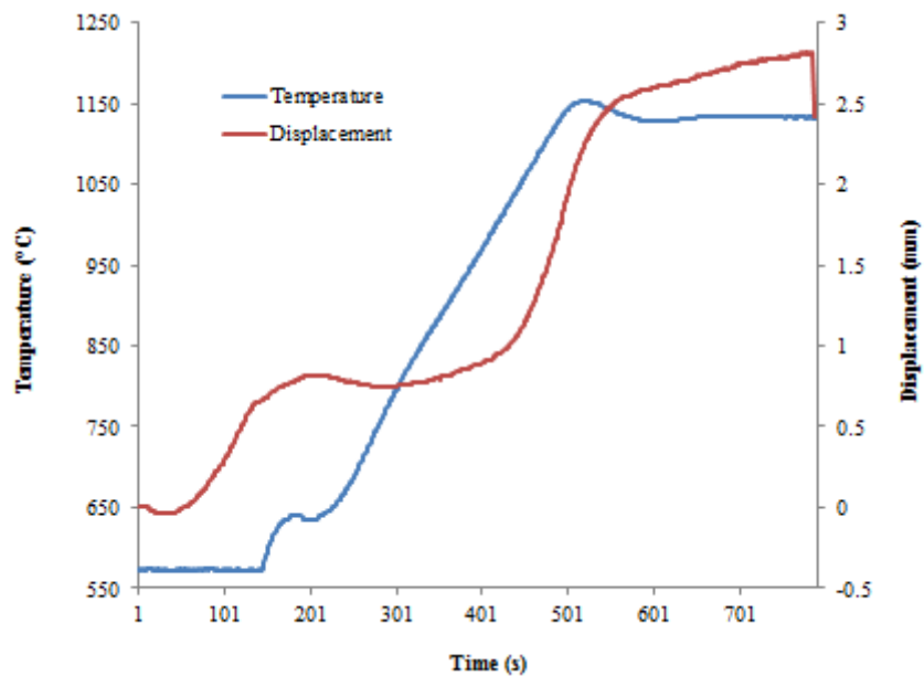
Figure 3. 1 Sintering profile for WC-12wt%Co SPS alloy.
