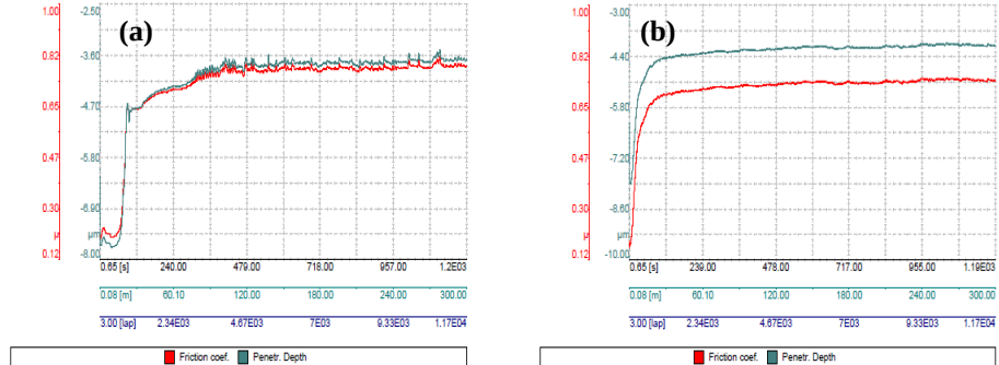
Figure D1. 1 Friction response against the 100Cr steel ball for (a) WC-12wt%Co, and (b) WC-12wt%Co-10wt%VC alloys.
