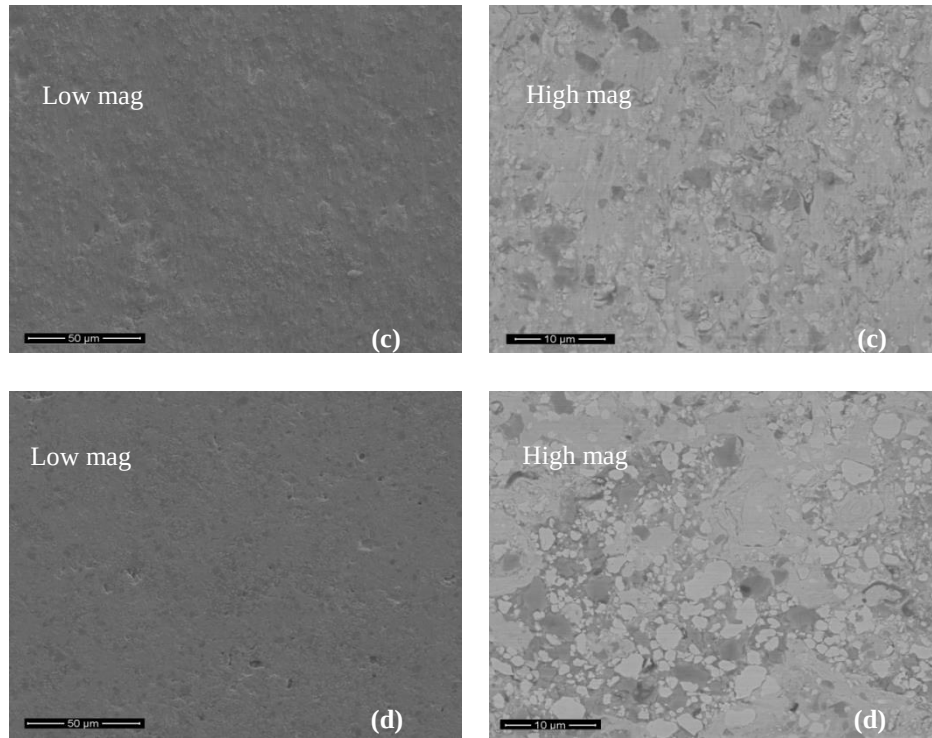
Figure 4. 26 SEM images of the eroded surface of the WC-17wt%Co-10wt%VC Run 39 at (a) 90°, (b) 75°, (c) 60°, and (d) 45°.
