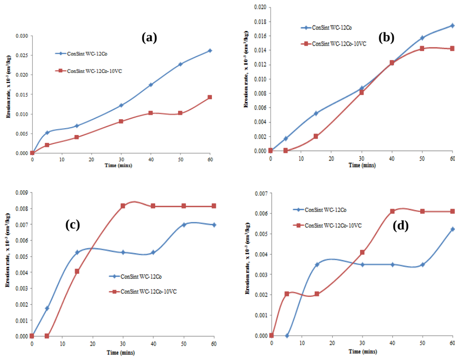
Figure C3A. 2 Average erosion rate against time curves for (a) 90°, (b) 75°, (c) 60°, and (d) 45°.
