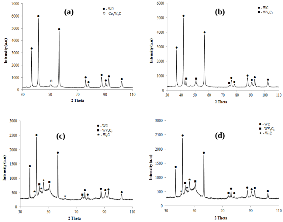
Figure 4. 9 XRD pattern of (a) WC-12wt%Co, (b) WC-12wt%Co-10wt%VC, (c) WC-17wt%Co-10wt%VC (Run 38), and (d) WC-17wt%Co-10wt%VC (Run 39) coatings.
