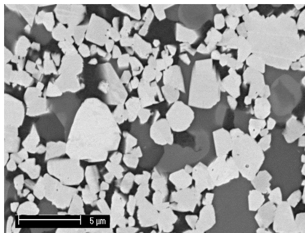
Figure 2. 5 Typical microstructure of sintered WC-12Co-10VC alloy (This study).
