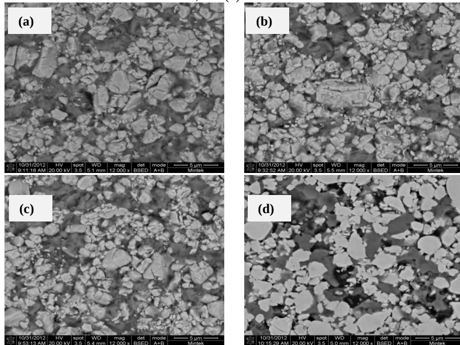
Figure D3B. 2 SEM images of the eroded surface of WC-12wt%Co 10wt%VC alloy at (a) 90°, (b) 75°, (c) 60°, and (d) 45°.
