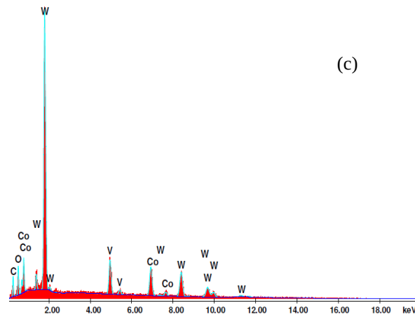
Figure 4. 28 (a) BSE SEM image, (b) EDAX maps overlay and (c) EDX analysis on the eroded surface of the WC-12wt%Co-10wt%VC coatings (Brown = C; Blue = Co; Green = O; Yellow = W; Purple = V).
