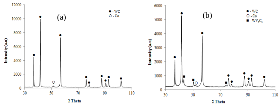
Figure 6. 5 XRD patterns for (a) WC-12wt%Co (b) WC-12wt%Co-10wt%VC alloys.
