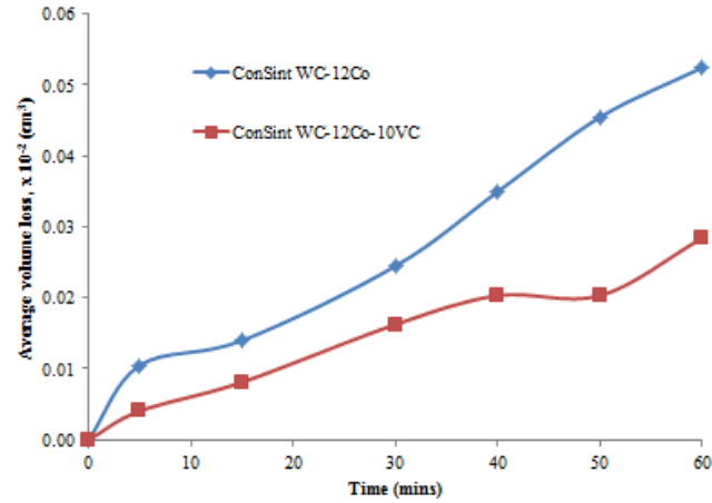
Figure 5. 12 Comparison of the average volume loss against time curves of both alloys at 90°.
