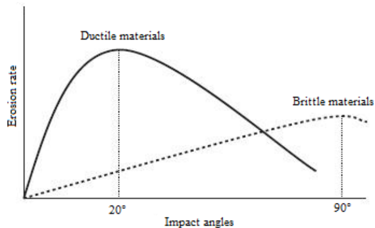
Figure 2. 14 Variation of erosive wear with impact angle for ductile and brittle materials [119].
