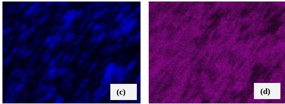
Figure 4. 6 EDAX maps showing the elemental distribution in the WC-12wt%Co-10wt%VC coatings. (a) SEM image (b) Co (c) V and (d) W.
