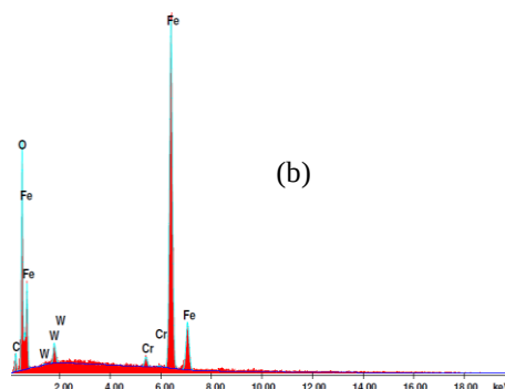
Figure 6. 11 SEM images with EDX analysis of the wear tracks against 100Cr ball for (a) WC-12wt%Co and (b) WC-12wt%Co-10wt%VC alloys.
