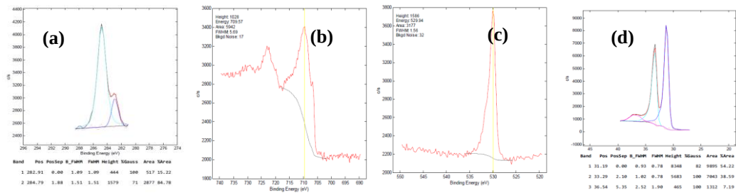
Figure B3A. 2 Narrow XPS scans of the wear track of the WC-12wt%Co coating showing (a) carbon (b) iron (c) oxygen and (d) tungsten peaks. The inserted tables show the de-convolution of peaks.
