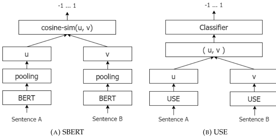
FIGURE 6.1: SBERT [Reimers et al. 2019] and USE regression architectures
