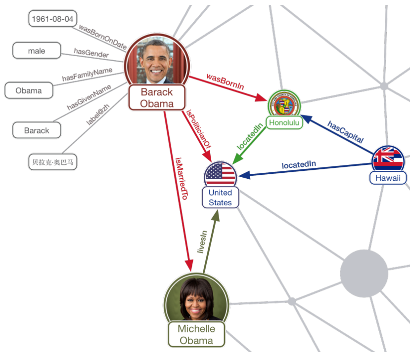
FIGURE 2.1: Example of Knowledge Graph from [Zhou et al. 2019] showing entity nodes in circles, with labels directly underneath. Directed edges represent relationships between entities. Each entity may have one or more properties associated with it, such as gender or given name if the entity is a person.
