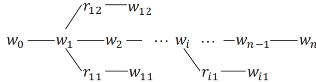
FIGURE 2.10: Sentence Tree structure [Liu et al. 2020]
