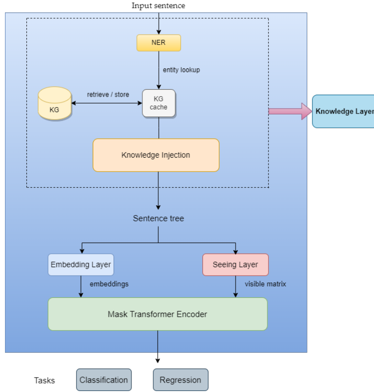
FIGURE 5.1: K-BERT architecture
