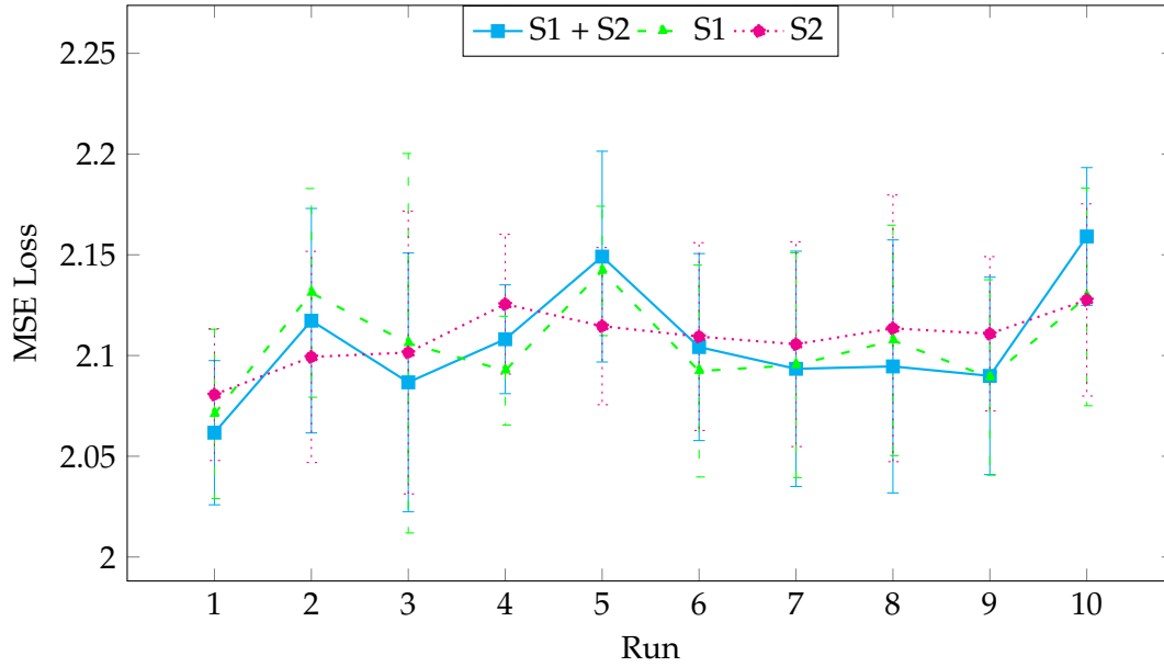
FIGURE 8.1: Mean MSE test loss with standard deviation error bars on best performing model per run. Mean is taken across ten trails.
