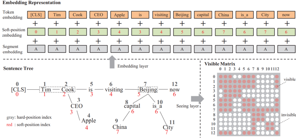
FIGURE 2.11: The processing of converting a sentence tree to an embedding representation with a visible matrix [Liu et al. 2020].
