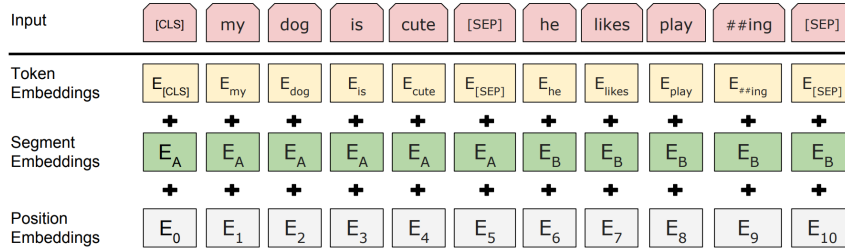
FIGURE 2.9: BERT input representation [Devlin et al. 2019]
