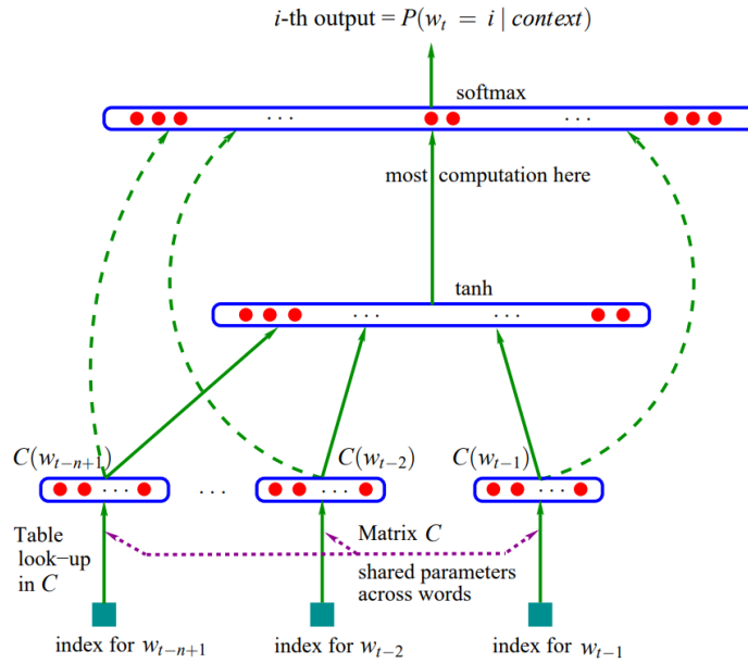
FIGURE 2.4: Bengio et al. [2003] neural architecture f depicted by Equation 2.3, where g is the neural network.
