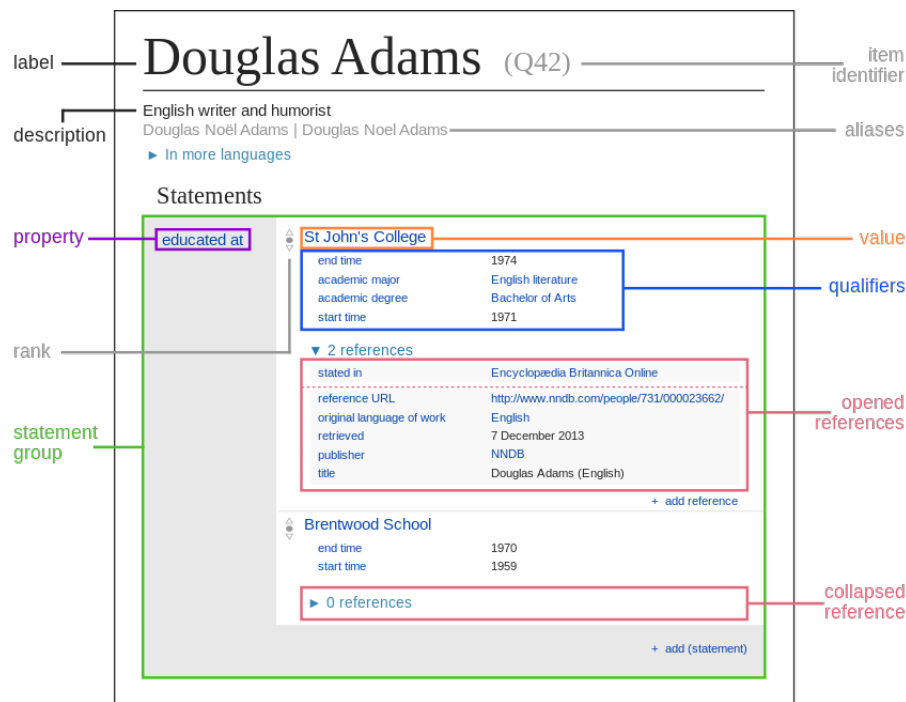
FIGURE 4.1: Wikidata information on English writer Douglas Adams [wik 2016a]
