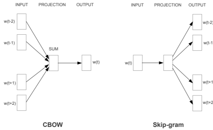
FIGURE 2.5: CBOW and Skip-gram models [Mikolov et al. 2013a]. CBOW predicts the current word based on the context. Skip-gram predicts the context words given the current word.
