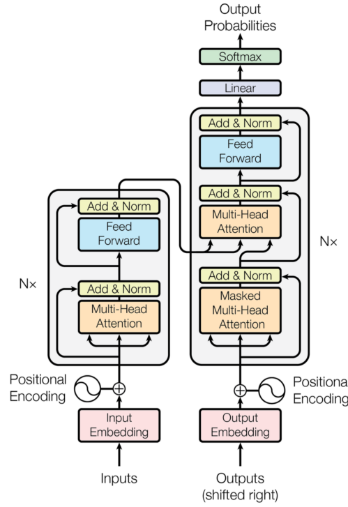
FIGURE 2.8: Transformer architecture from [Vaswani et al. 2017]
