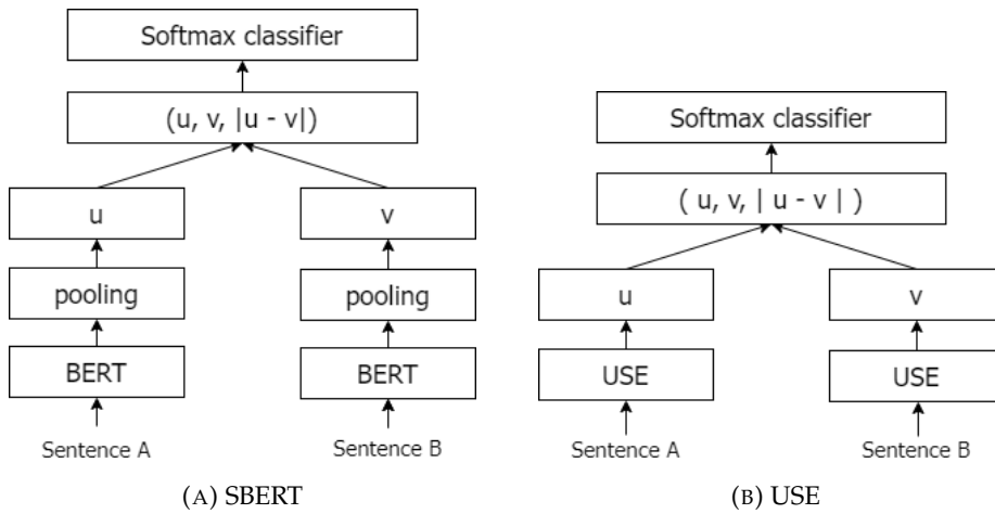
FIGURE 6.2: SBERT [Reimers et al. 2019] and USE classification architectures
