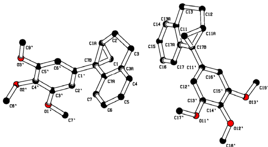
Figure 1: X-ray crystal structure of 7b-(3,4,5-trimethoxyphenyl)-1a,2,3,7b-tetrahydro-1 H -cyclopropa[ a ]naphthalene ( 125 ) showing both molecules in the asymmetric unit. Hydrogen atoms are omitted for clarity.
