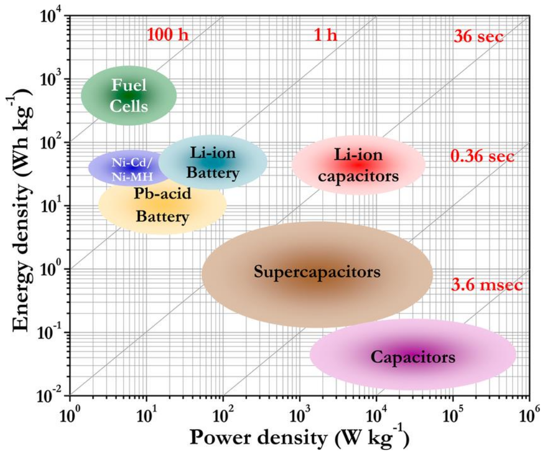
Figure 1.1: Ragone plot of numerous storage devices [4].
