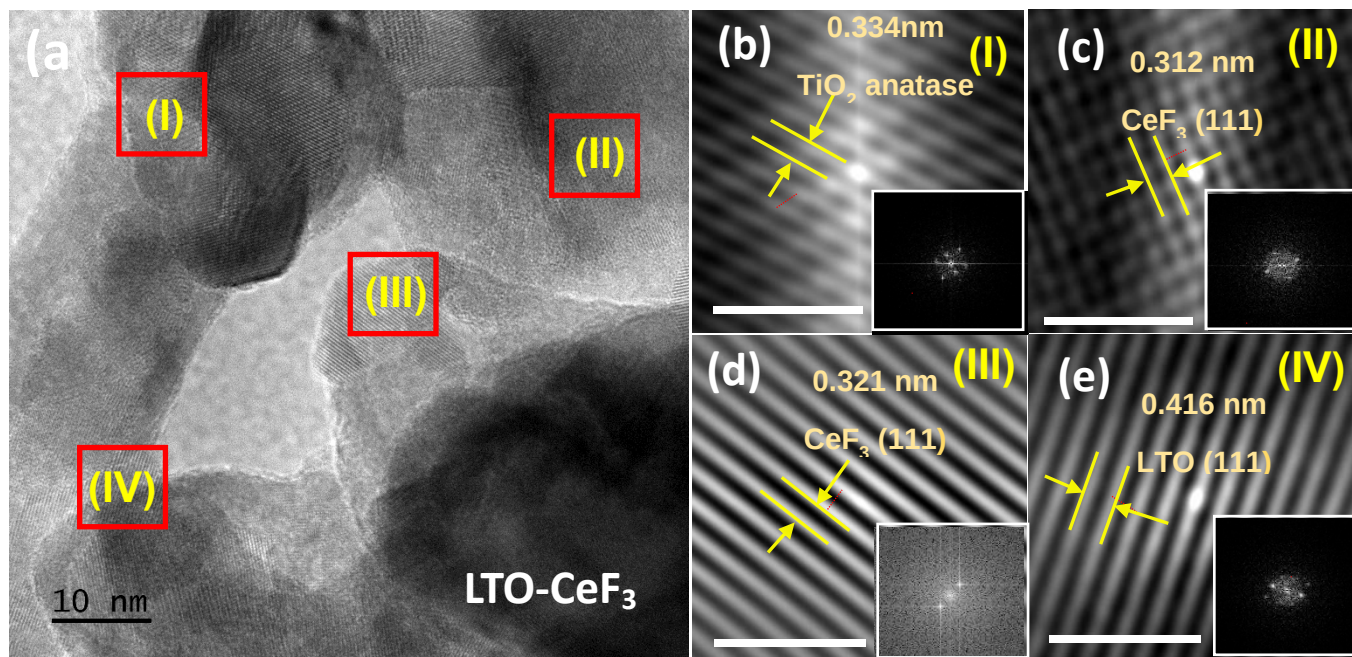
Figure 4.6: HRTEM image of (a) LTO-CeF 3 region and SAED image of (b) TiO 2 anatase (101), (c) CeF 3 (111), (d) CeF 3 (111), and (e) LTO (111) lattice plane on LTO- CeF 3 .
