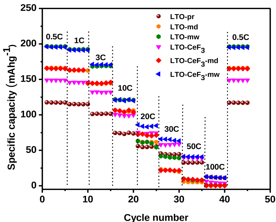
Figure 4.22: Rate capability of the LTO-p, LTO-CeF 3 , LTO-md, LTO-CeF 3 -md, LTO-mw, and LTO-CeF 3 -mw.
