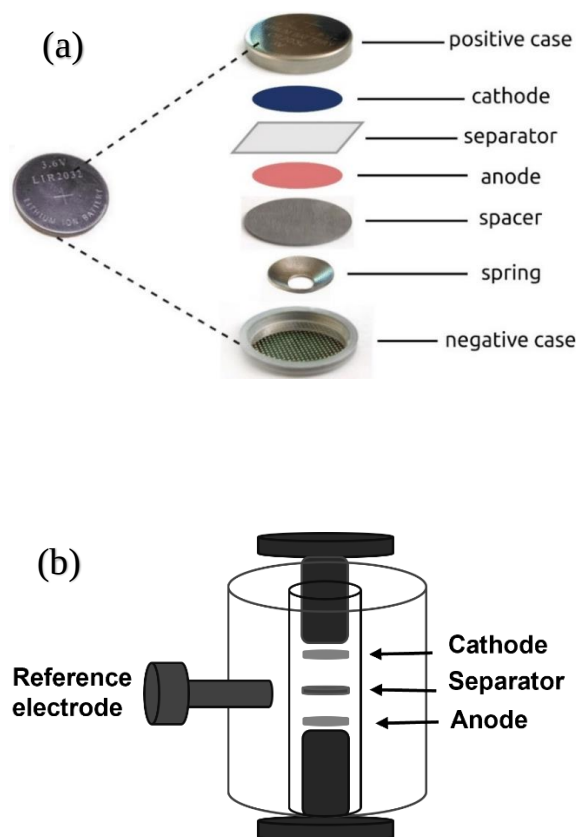
Figure 3.3: (a) Coin cell components [3], (b) Schematic of T-type Swagelok cell.
