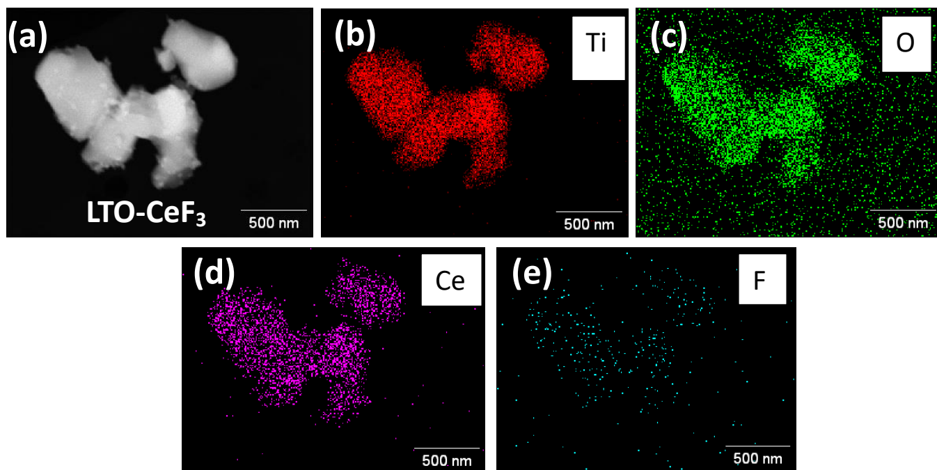
Figure 4.10: SEM micrograph of (a) LTO-CeF 3 , with its associated (b) Ti, (c) O, (d) Ce, and (e) F elemental mapping.
