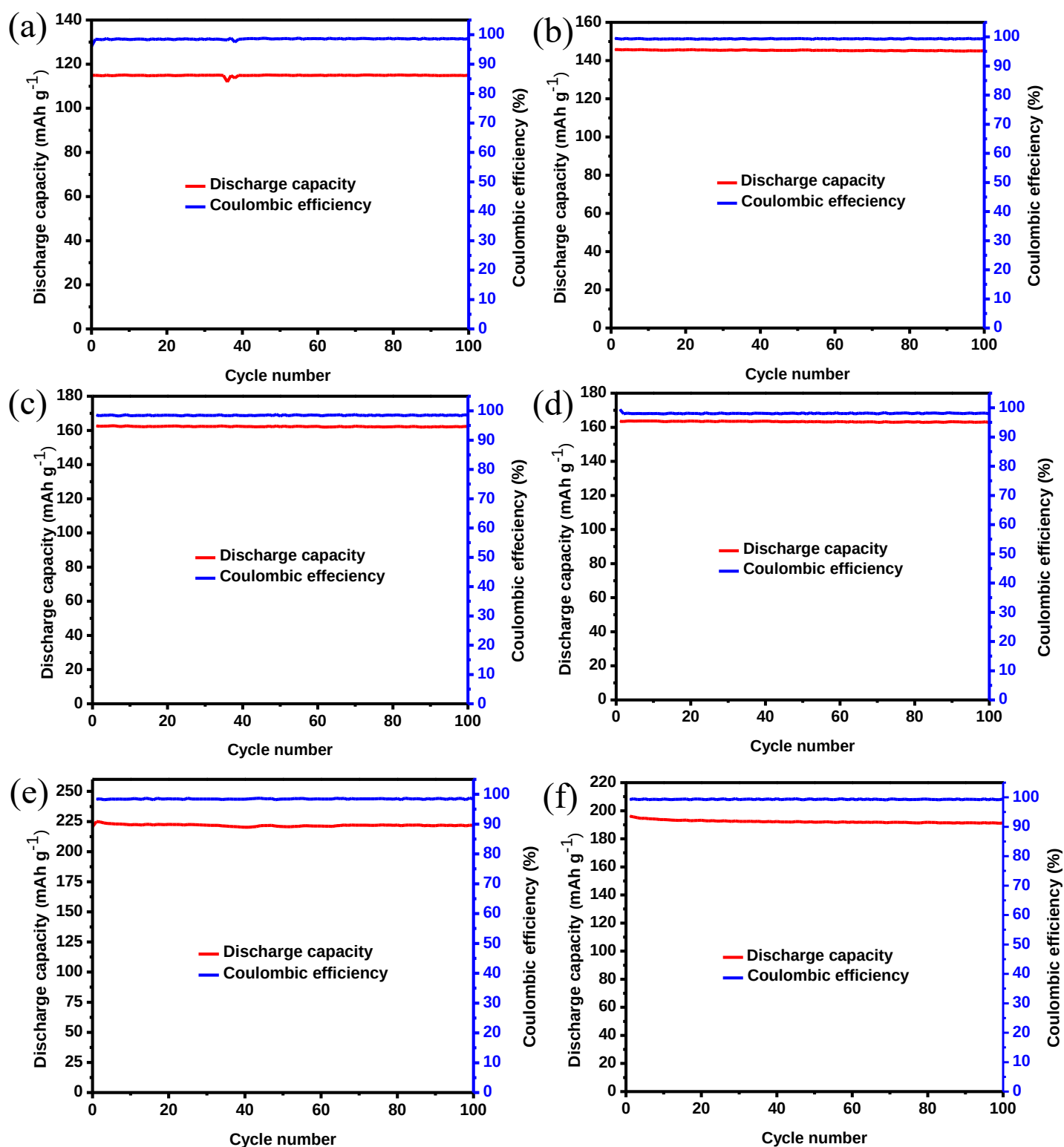
Figure 4.19: Discharge capacity and coulombic efficiency of (a) LTO-p, (b) LTO-CeF 3 , (c) LTO-md, (d) LTO-CeF 3 -md, (e) LTO-mw, and (f) LTO-CeF 3 -mw at 1C for 100 cycles.
