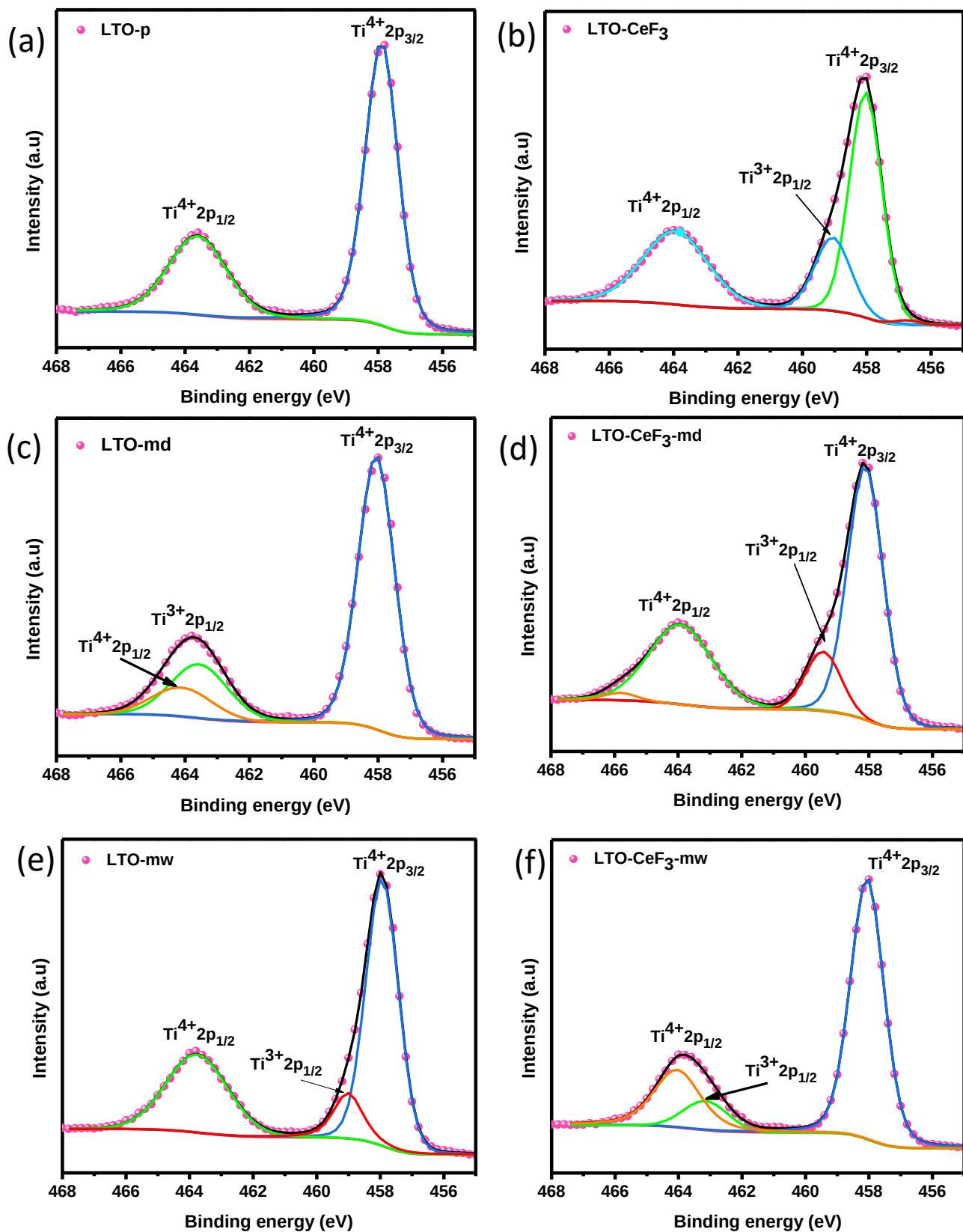
Figure 4.14: Deconvolution of Ti2p on (a) LTO-p, (b) LTO- CeF_3 , (c) LTO-md, (d) LTO- CeF_3 -md, (e) LTO-mw, and (f) LTO- CeF_3 -mw material.
