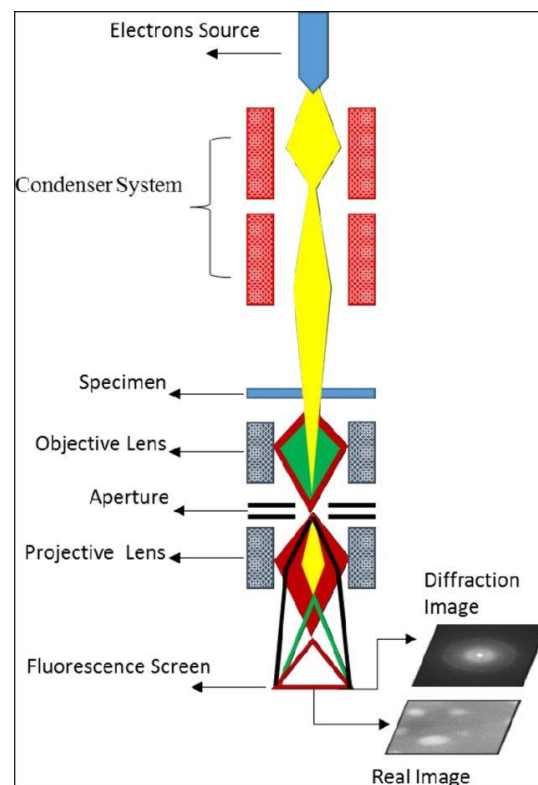
Figure 2.9 : Transmission Electron Microscopy working principle [38].
