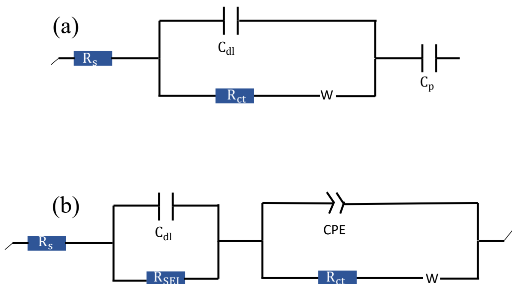
Figure 4.24: Equivalent circuit of the materials (a) before cycling and only after cycling for LTO-p, and (b) After cycling.
