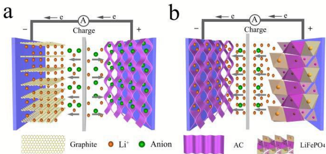
Figure 2.6: Storage mechanisms of LICs, (a) electrolyte-consumption and (b) lithium-ion transport [26].
