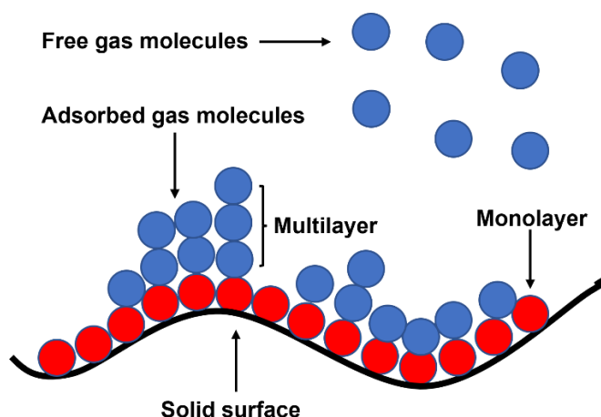
Figure 2.13: BET working principle.
