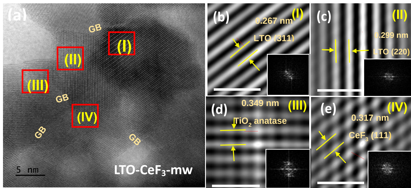
Figure 4.7: HRTEM image of (a) LTO-CeF 3 -mw region and SAED image of (b) LTO (311), (c) LTO (220) (d) TiO 2 anatase (101), and (e) CeF 3 (111) lattice plane on LTO- CeF 3 -mw.
