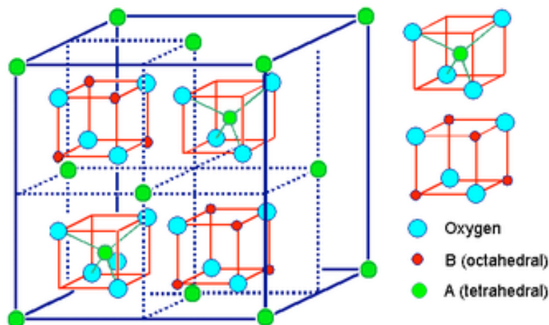
Figure 2.18: Spinel structure diagram [58].
