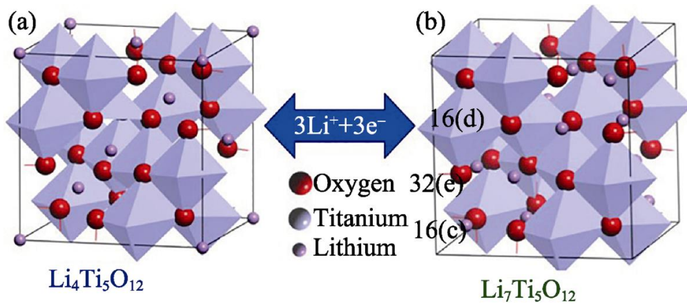
Figure 2.19: (a) LTO in Spinel structure, (b) LTO in rock-salt structure [67].
