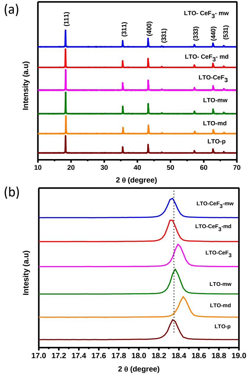
Figure 4.1: (a) XRD patterns, (b) 111 peaks of LTO-p, LTO-md, LTO-mw, LTO-CeF 3 , LTO-CeF 3 -md, and LTO-CeF 3 -mw
