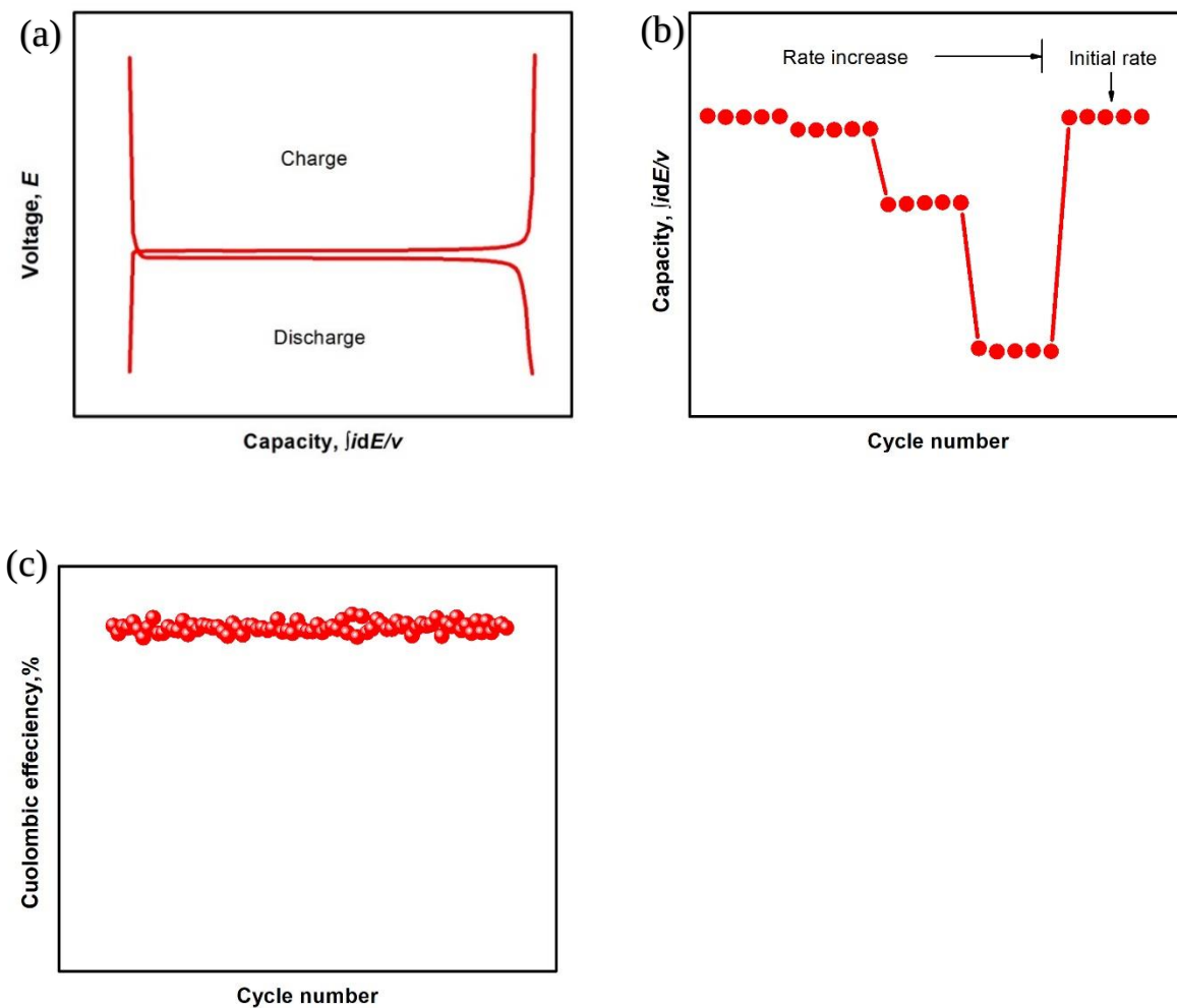
Figure 2.17: (a) Charge and discharge curves, (b) rate capability performance, (c) Coulombic efficiency plot.
