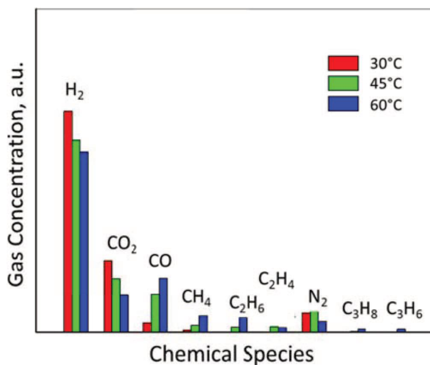
Figure 2.22: Concentration of decomposed chemical species at different temperatures [95].
