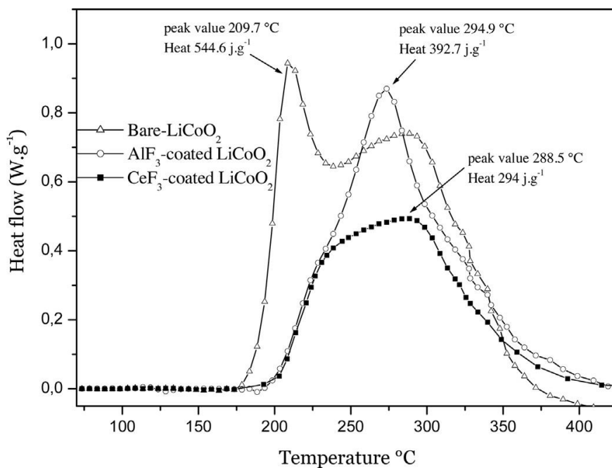
Figure 2.23: DSC plots of the bare-LiCoO 2 and coated -LiCoO 2 cathodes at fully charged state. [103].
