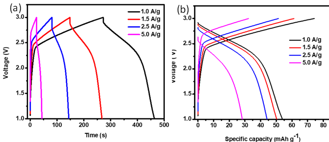
Figure 5.6: Charge-discharge of LTO-CeF 3 //CB full cell at several current densities.
