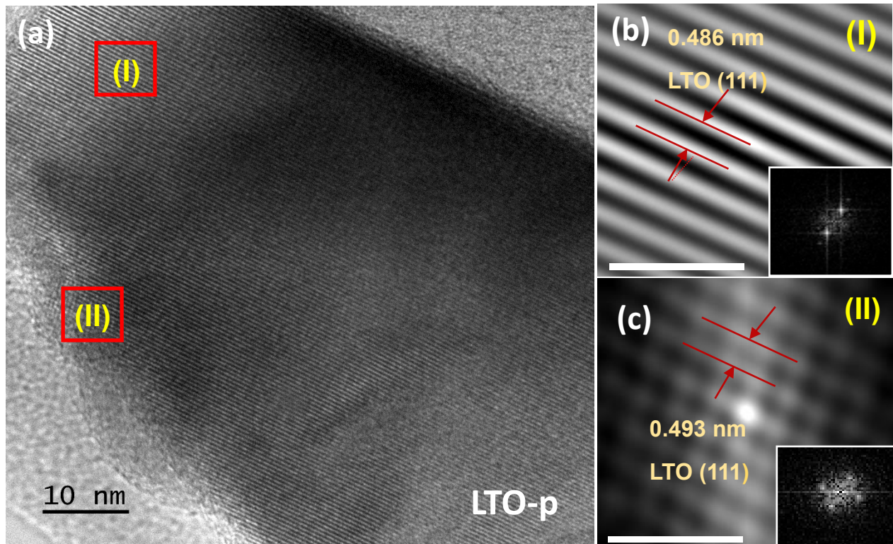
Figure 4.4: HRTEM image of (a) LTO-p, region and SAED image of (b) LTO (111) and (c) LTO (111) lattice plane on LTO-p.
