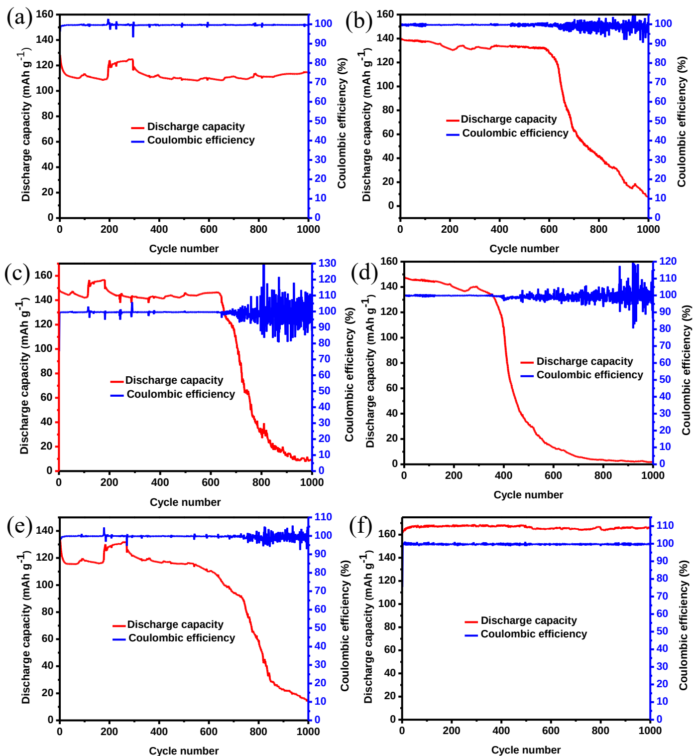
Figure 4.21: Discharge capacity and coulombic efficiency of (a) LTO-p, (b) LTO-CeF 3 , (c) LTO-md, (d) LTO-CeF 3 -md, (e) LTO-mw, and (f) LTO-CeF 3 -mw at 5C for 1000 Cycles.
