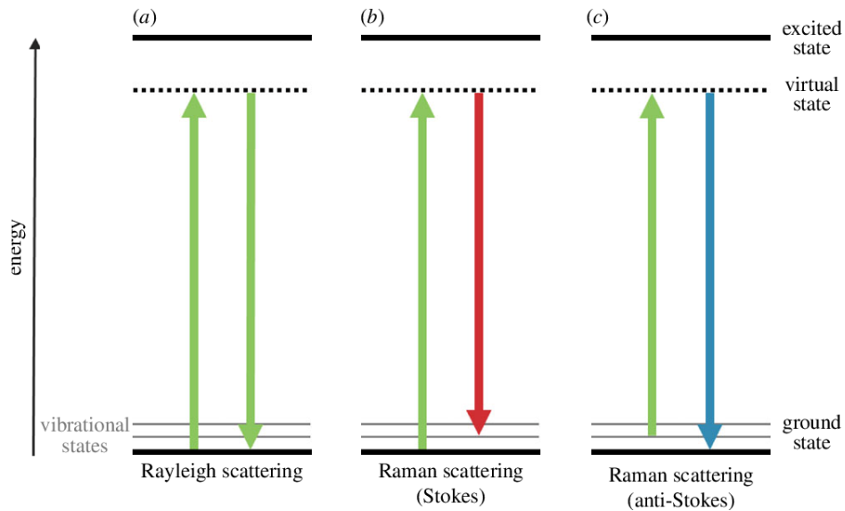
Figure 2.8: Raman scatterings [34].
