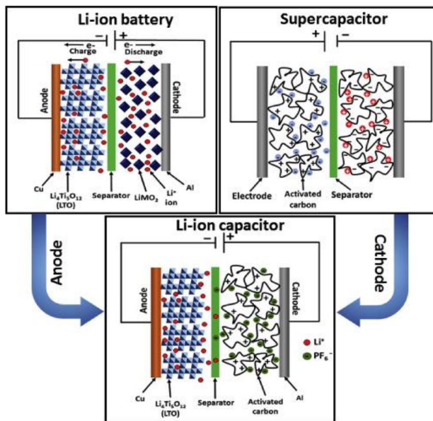
Figure 2.5: Diagrams of LIB, supercapacitor and LIC [28].
