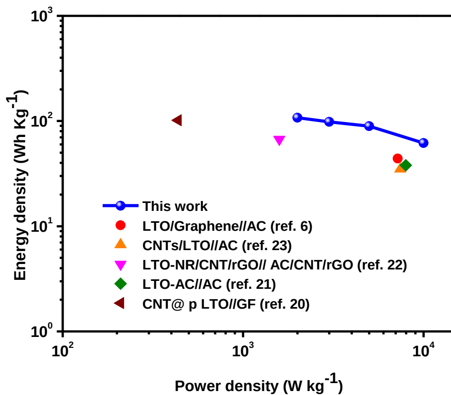
Figure 5.9: Ragone plot for LIC full cell made up of LTO anode and CB cathode, compared with the literature.
