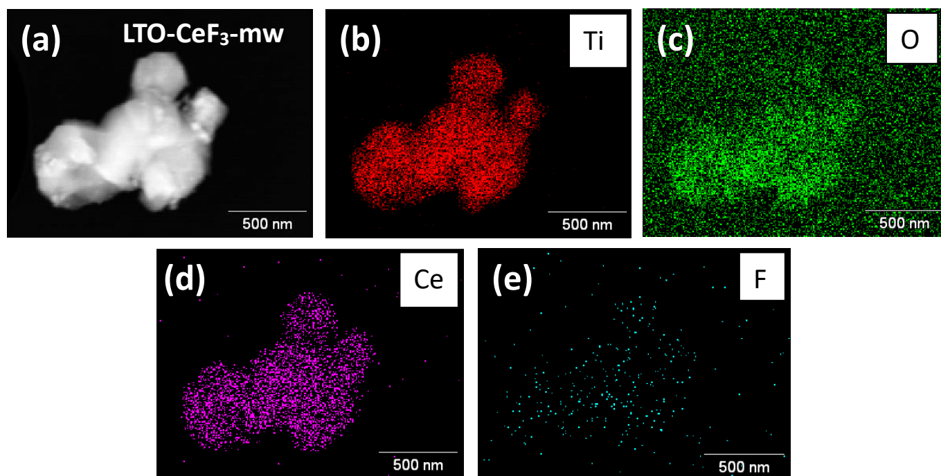
Figure 4.11: SEM micrographs of (a) LTO-CeF 3 -mw, with its associated (b) Ti, (c) O, (d) Ce, and (e) F elemental mapping.
