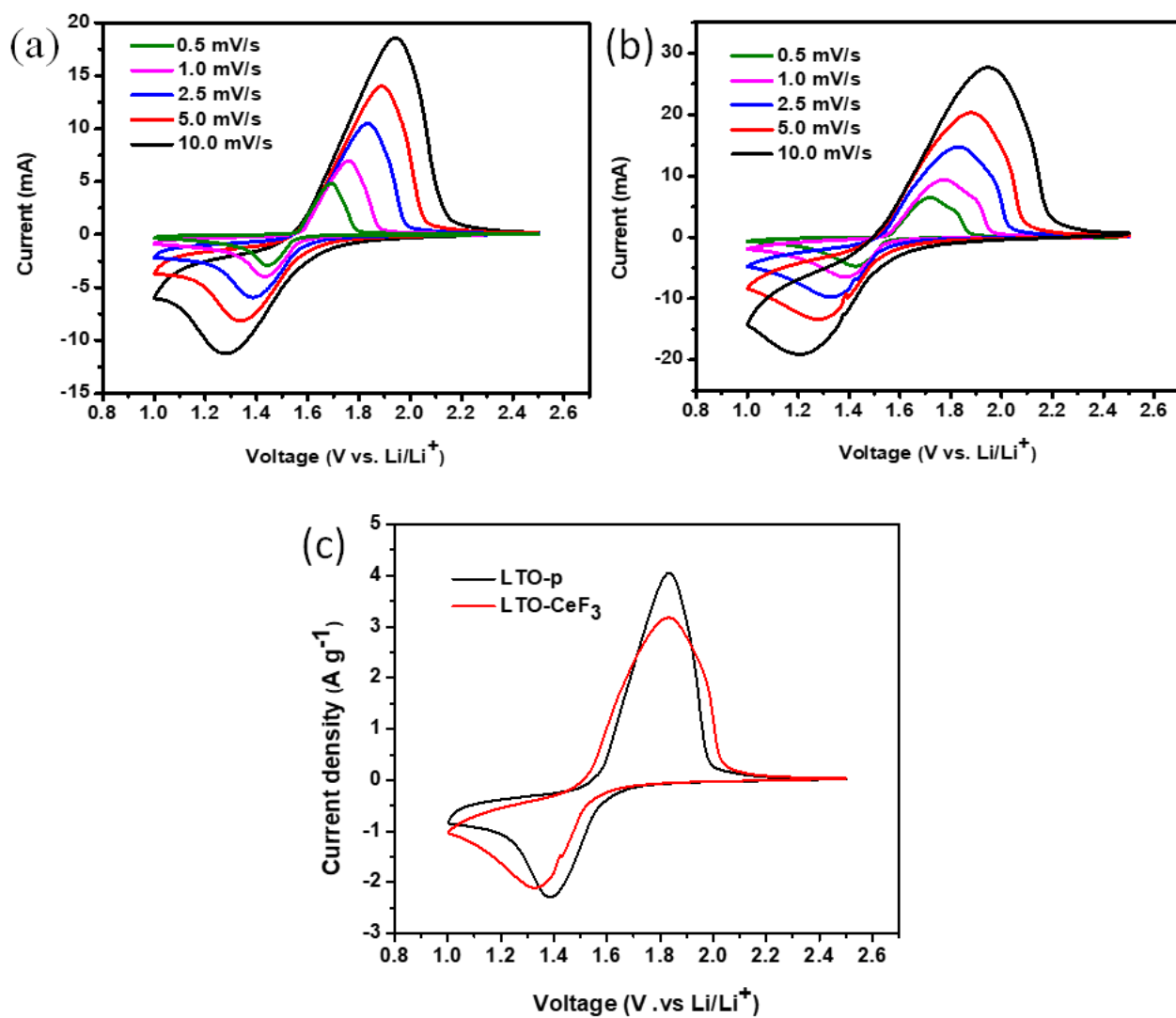
Figure 5.1: Half-cell CV plots at numerous scan rates: (a) LTO-p, (b) LTO-CeF 3 , and (c) comparison of LTO-P and LTO-CeF 3 at 2.5 mV s -1 .
