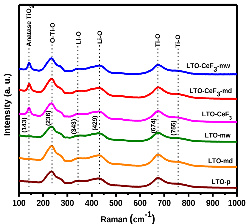
Figure 4.2: Raman spectra of the materials.
