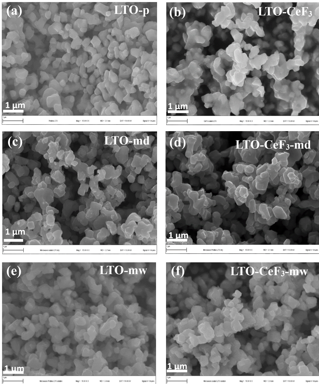
Figure 4.16: SEM image of (a) LTO-p, (b) LTO-CeF 3 , (c) LTO-md, (d) LTO-CeF 3 -md, (e) LTO-mw, and (f) LTO-CeF 3 -mw.
