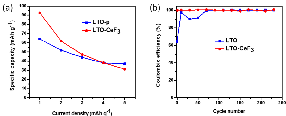
Figure 5.3: (a) Specific capacity at several current densities, (b) Coulombic efficiency of LTO-p and LTO-CeF 3 .
