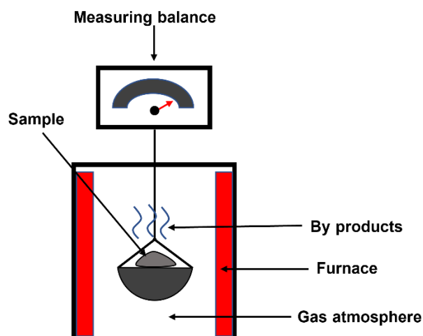
Figure 2.14: Working principle of TGA.
