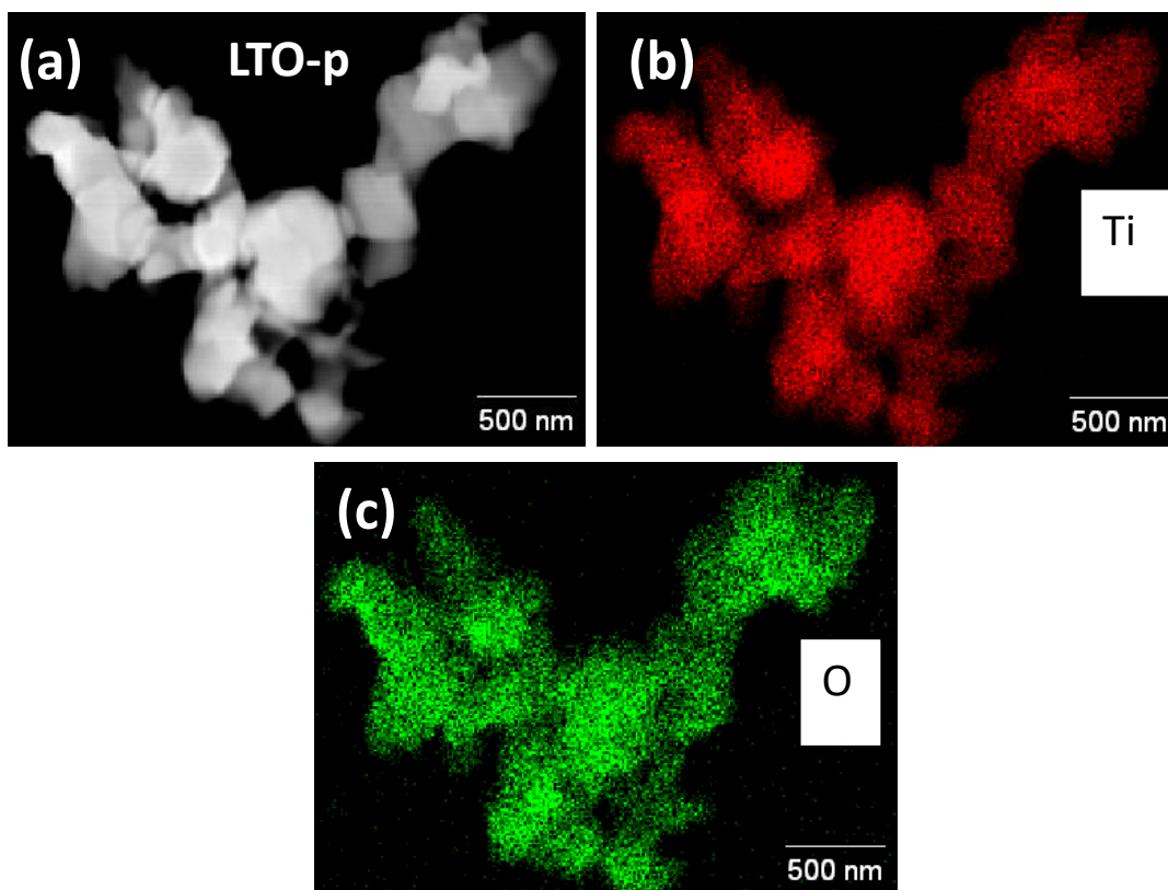
Figure 4.8: SEM micrographs of (a) LTO-p, with its associated (b) Ti and (c) O elemental mapping.
