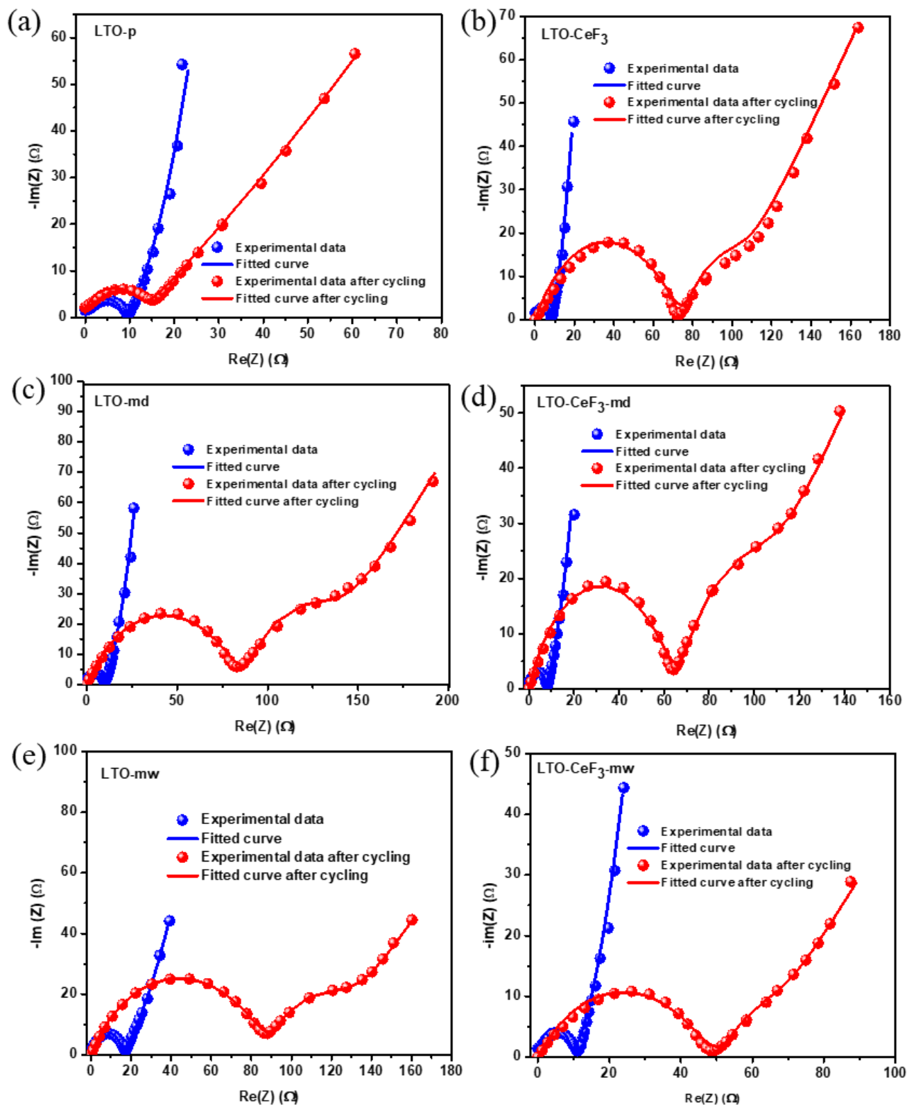
Figure 4.23: Nyquist plots before and after 1000 cycles of (a) LTO-p, (b) LTO-CeF 3 , (c) LTO-md, (d) LTO-CeF 3 -md, (e) LTO-mw, and (f) LTO-CeF 3 -mw.
