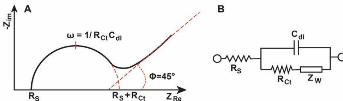
Figure 2.16: Nyquist plot and the equivalent Randles circuit.
