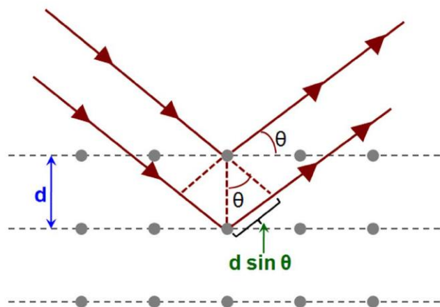
Figure 2.7: X-ray diffraction schematic of 2 dimensional crystal [32].
