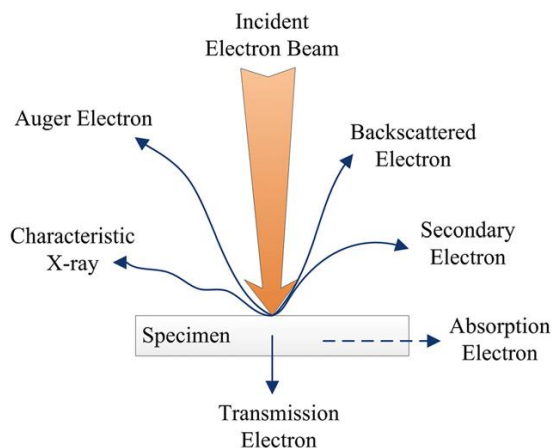
Figure 2.10: Working principle depiction of SEM [41].
