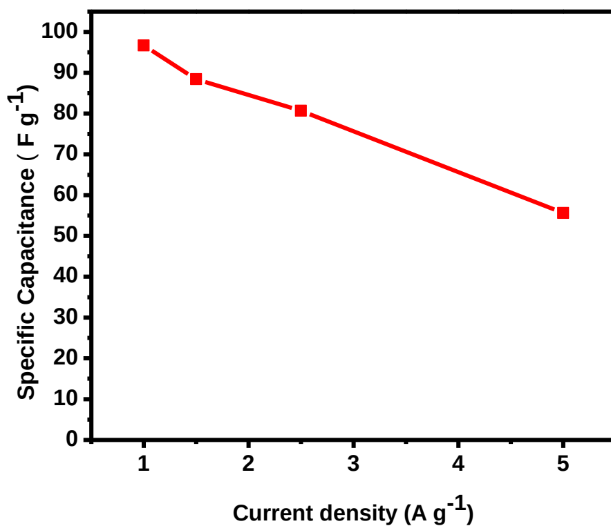
Figure 5.7: Specific capacitance at various current density.
