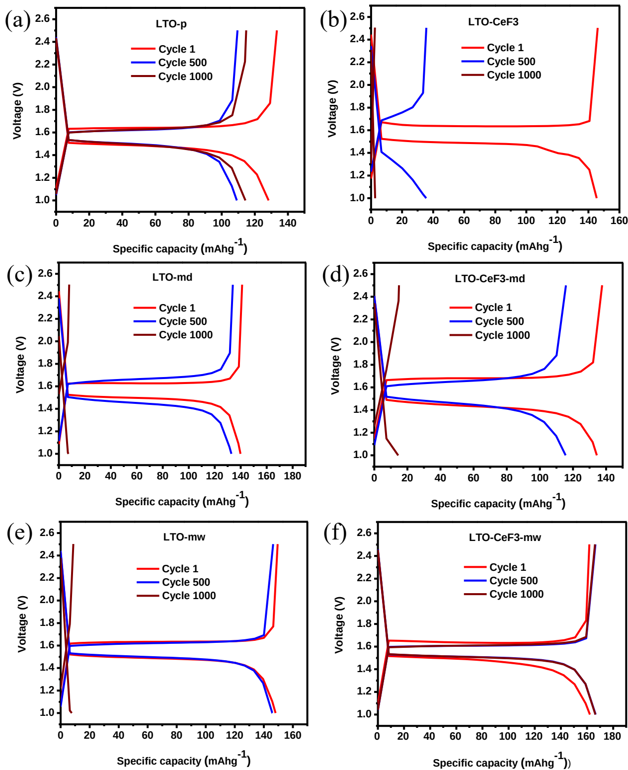
Figure 4.20: Charge/discharge plots of (a) LTO-p, (b) LTO-CeF 3 , (c) LTO-md, (d) LTO-CeF 3 -md, (e) LTO-mw, and (f) LTO-CeF 3 -mw at 5C for 1000 Cycles.
