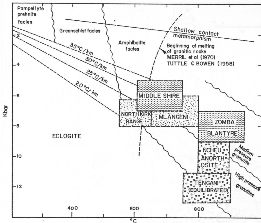
Fig.51. P-T conditions for certain areas in southern Malawi; shown in relation to metamorphic facies and other relevant metamorphic subdivisions and geothermal gradients (after Green and Ringwood, 1967; Winkler, 1974).
