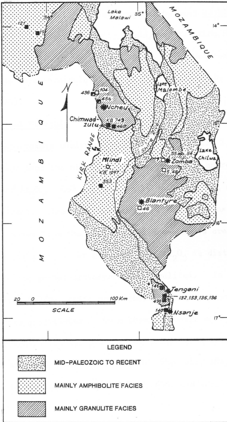
Fig.9. Locality map for samples of mineral analyses. Orthopyroxene granulite and associated amphibolite (□); garnet-two-pyroxene granulite (◐); garnet-clinopyroxene granulite and associated amphibolite (■); orthogneiss (○)(modified after Bloomfield, 1968).
