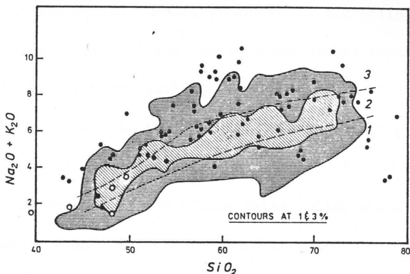
Fig.54. Alkali-silica diagram for the southern Malawi granulites (●) and for the Kirk Range amphibolites and metadolerites (○) superimposed on the field of 240 hypersthene-bearing rocks of African charnockite-granulite suites (after Clifford, 1974). Dashed lines separate the fields of: (1) alkali olivine basalt, (2) high alumina basalt, and (3) tholeiite (after Kuno, 1968).
