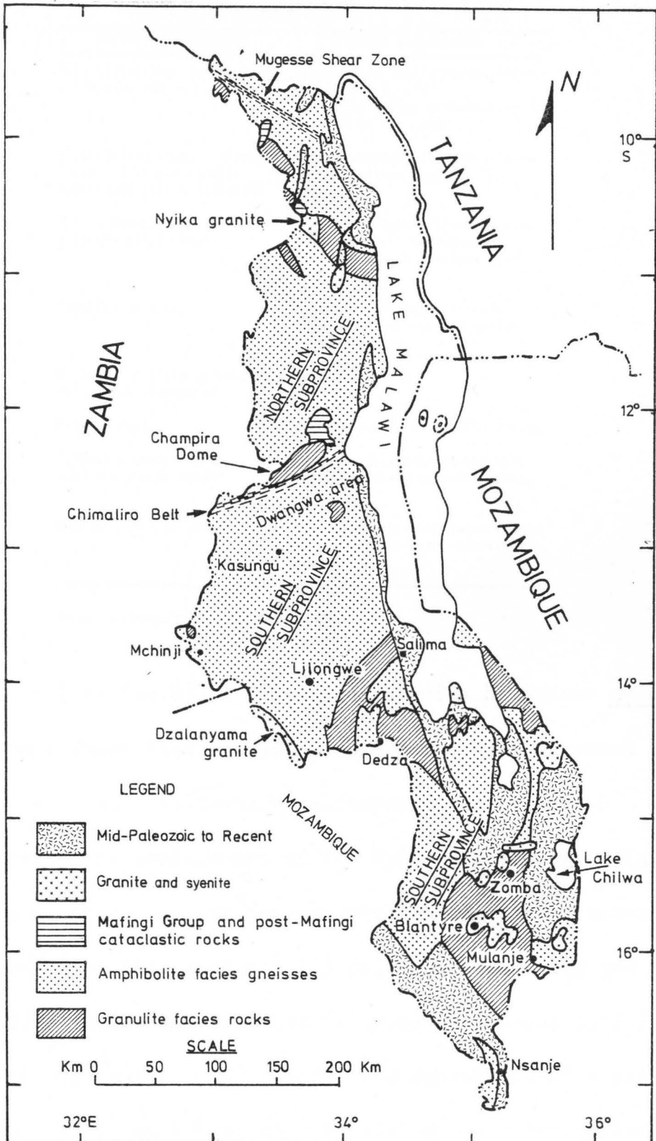
Fig.3. Major geological units of Malawi (modified after Carter and Bennett, 1973).
