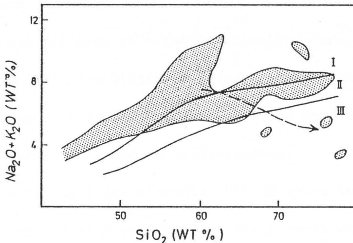
Fig.44. Alkali-silica diagram illustrating the distribution of the southern Malawi granulites (shaded area; see Fig.22) in relation to fields of (I), alkali-olivine basalt; (ii) high-alumina basalt; and (III), tholeiite (given by Kuno, 1968). The arrow defines the trend of pelitic rocks from Japanese Paleozoic geosynclinal deposits ( ibid. ).
