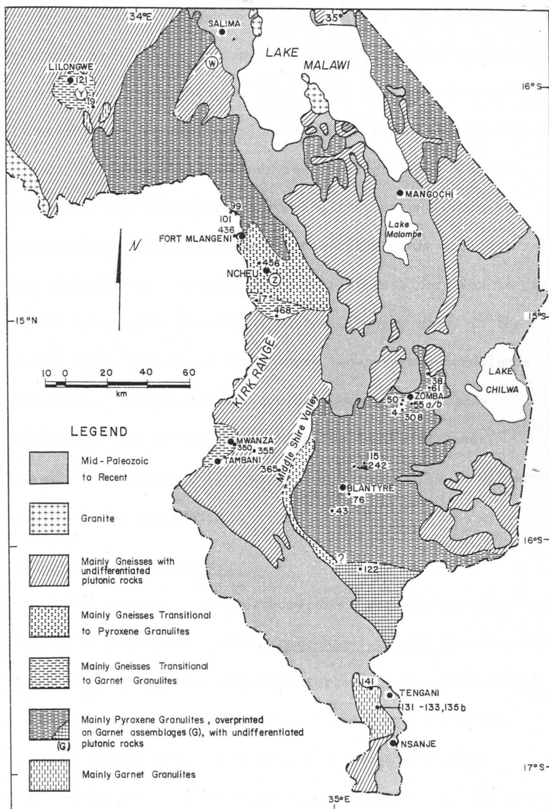
Fig.35. Generalized map of localities referred to in Chapter 5 (see also Maps 1 to 4 in the pocket at the back of the thesis; modified after Bloomfield, 1968; Morel, 1961a).
