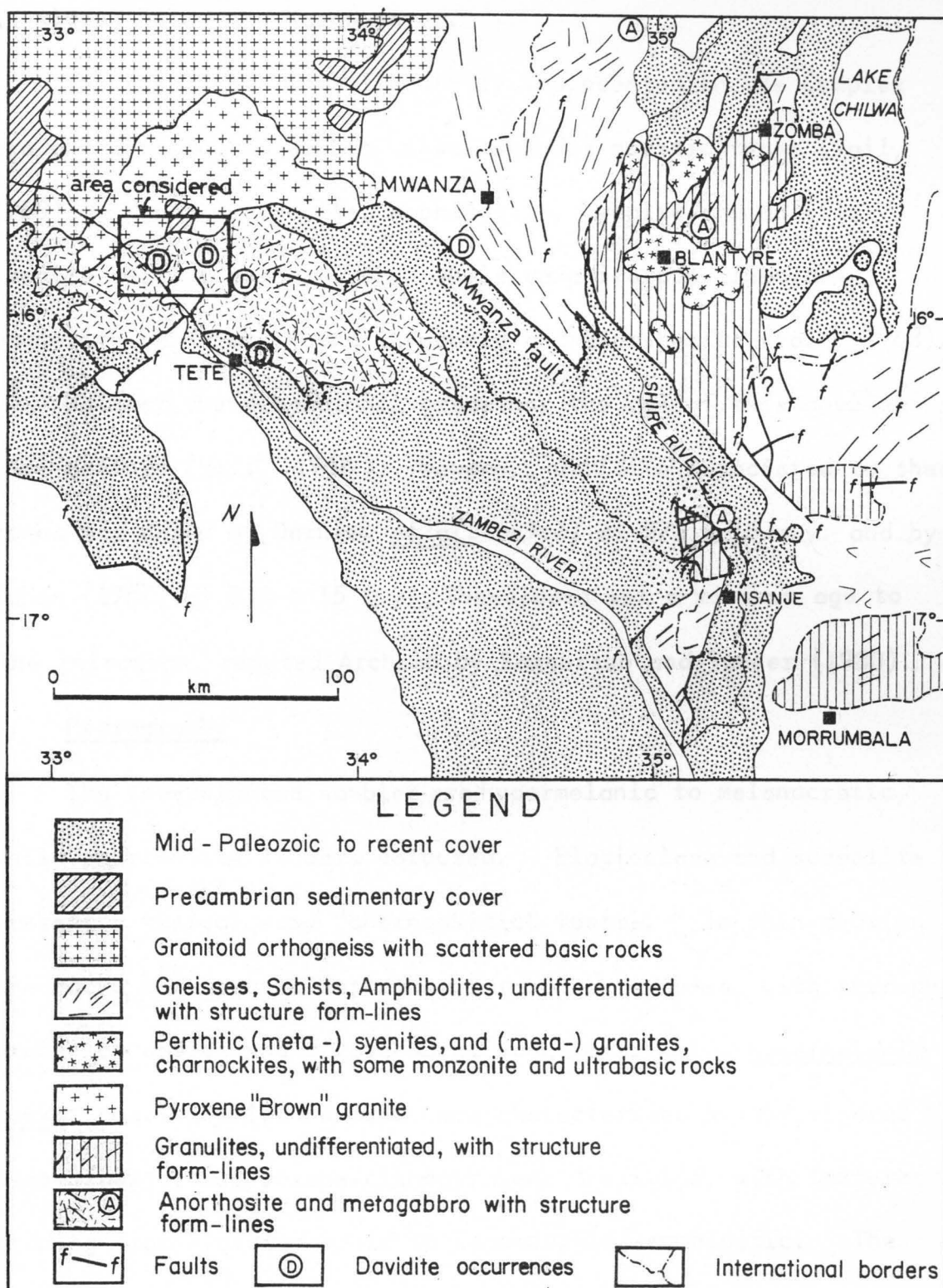
Fig.VII-A. Generalized geology of southern Malawi and the adjacent Tete area of north-west Mozambique (after Davidson and Bennett, 1950, Freitas, 1956; Oberholzer 1968, Bloomfield, 1968; and Vail 1968).
