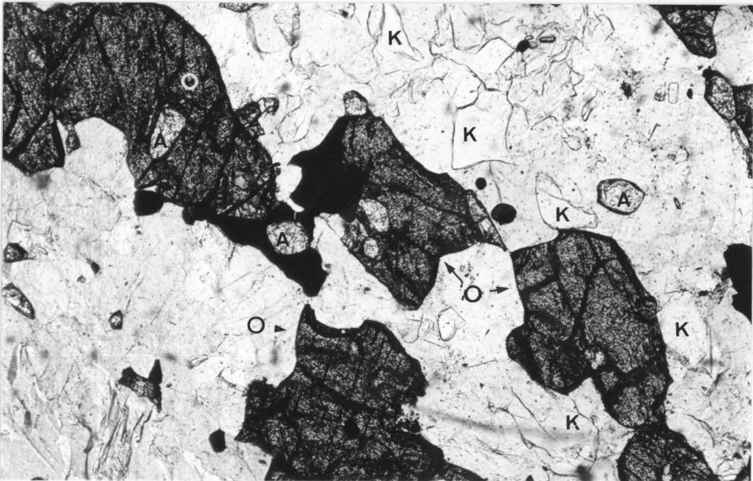
Plate 2. Mesocratic granulite, rich in orthopyroxene(o), perthite (K), and apatite (A). X50, Ncheu, (see locality 441, Map 3).
