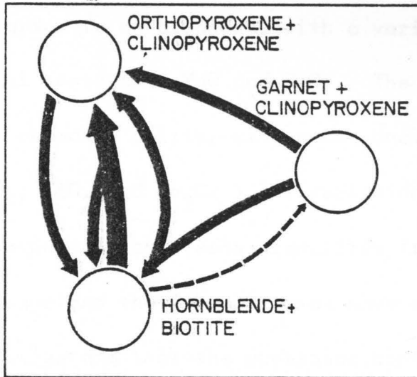
Fig.50. Mineral relationships amongst southern Malawi amphibolite and granulite facies parageneses (see text for explanation).
