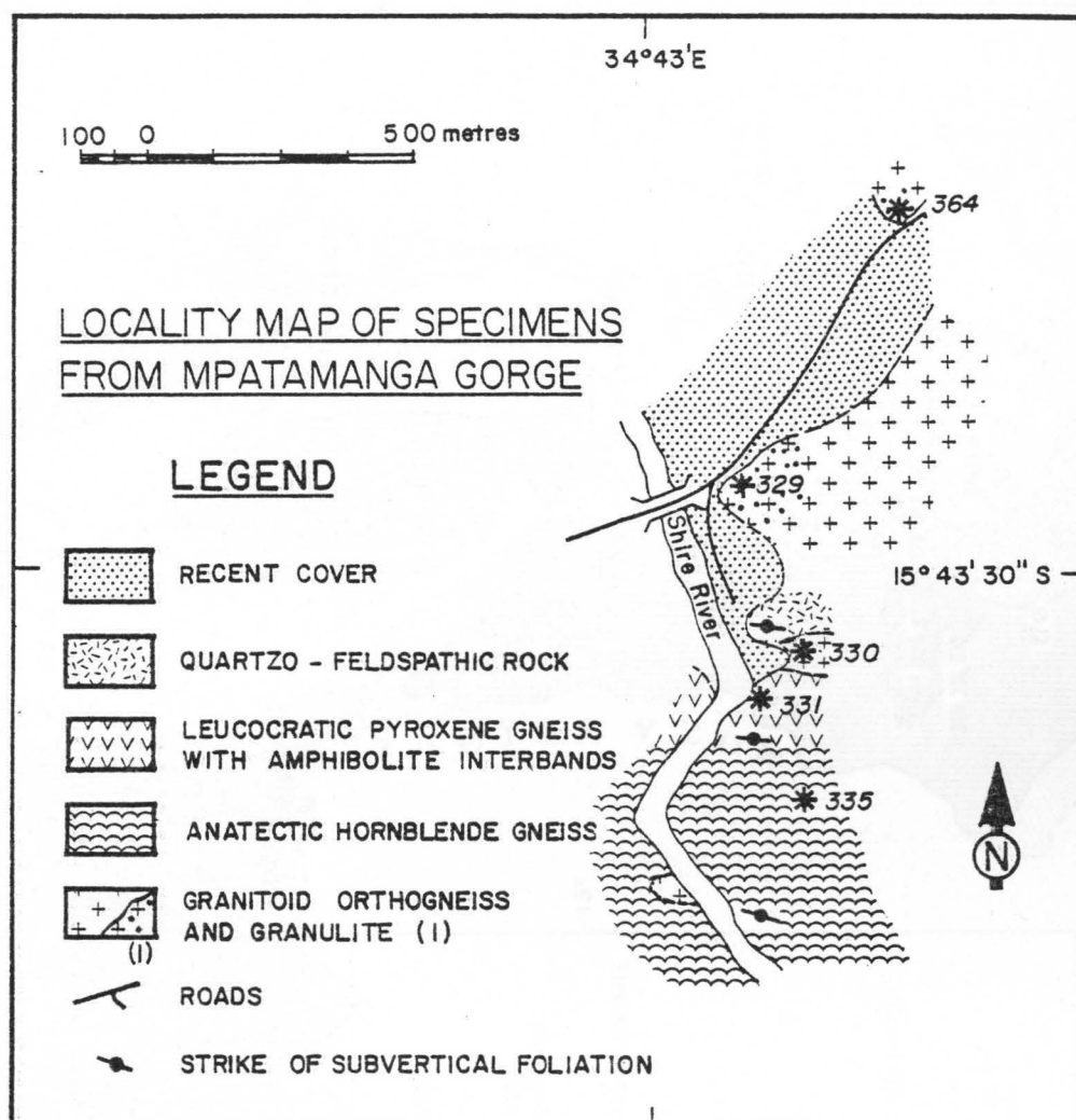
Fig.VI-A. Geological map of the Mpatamanga Gorge in the Middle Shire transition zone with localities of samples used in age determinations.
