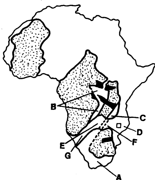
Fig.58. Major structural units of Africa with Archean-lower Proterozoic ( \geq 2\ 000 m.y. old) mobile belts (black), stable continental crust since 1\ 500 m.y. ago (stippled), and mobile belts younger than 1\ 500 m.y. (blank)(after Onstott and Hargraves, 1981). (A) to (G) are mobile belts discussed in the text and (□) is position of southern Malawi.
