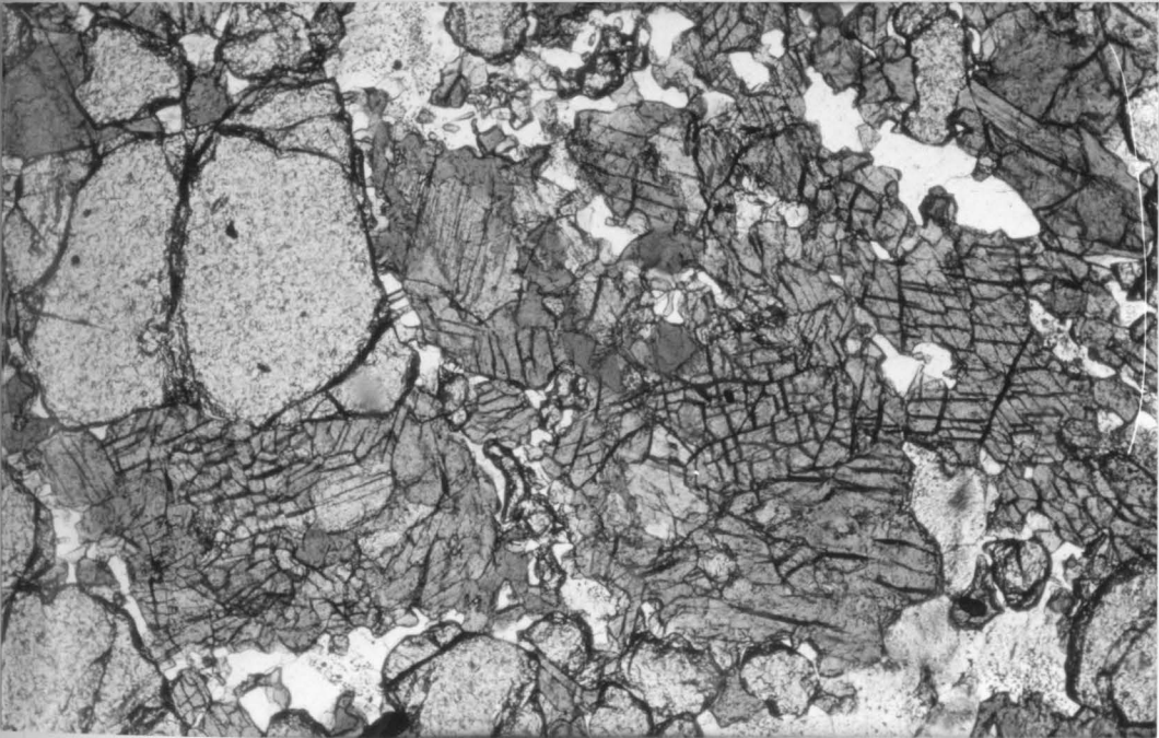
Plate 4. Melanocratic garnet-clinopyroxene-hornblende granulite. X50, Tengani area (see Locality 132, Map 1).
