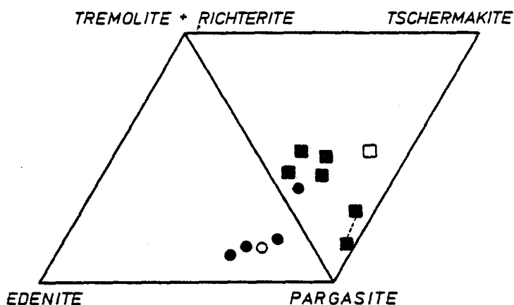
Fig.17. End members distribution in hornblendes. Two-pyroxene granulite (●), and an associated amphibolite (○); garnet-clinopyroxene granulite (■), and a related amphibolite (□). Dashed line joins analyses from the same sample.
