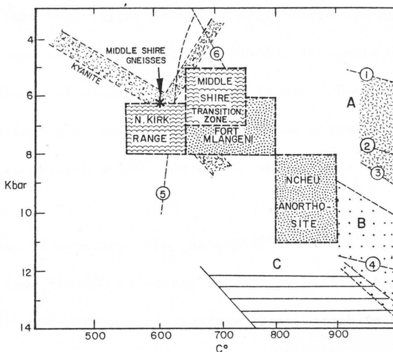
Fig.37. Some experimental data relevant to the determination of the P-T conditions in parts of southern Malawi. The fields of Al-silicates, the shaded areas A, B and C and the numbered curves 1 to 4 are the same as in Fig.36; curve 5 is beginning of melting in granitic rocks (Merril et al. , 1970; Tuttle and Bowen, 1958); and 6 is the high-temperature stability limit of muscovite + quartz (Althaus et al. , 1970).
