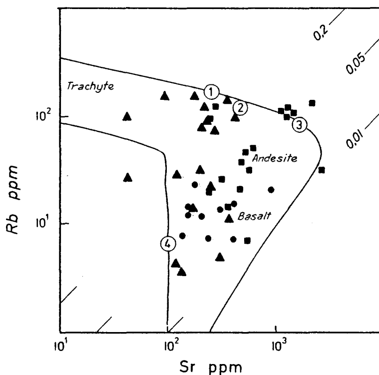
Fig.46. Distribution of Rb and Sr in southern Malawi melanocratic (●), mesocratic (■) and leucocratic (▲) granulites in relation to the basalt-rhyolite/trachyte trend (given by Hedge, 1966). Numbers indicate: (1), granite ( ibid. ); (2), rhyolite and rhyodacite (Groome and Hall, 1974); (3), latite (Nockolds and Allen, 1954); and (4), Fiji keratophyre (Gill, 1970).
