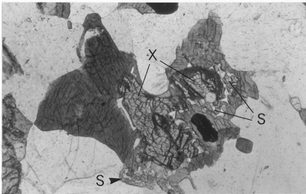
Plate 12. Type III retrograde geometry: detail of an orthopyroxene relict (x) rimmed by a hornblende-quartz symplectite (S). X50, Zomba area (see Locality 38, Map 2).
