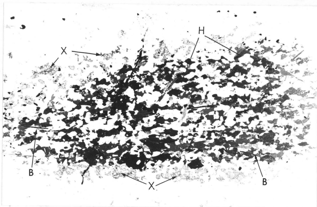
Plate 14. Photomicrograph of an amphibolite stripe from the sample of Plate 13, showing a Type I prograde geometry; note pyroxenes (X), hornblende (H) and biotite (B). X6, Blantyre area (see Locality 242, Map 2).
