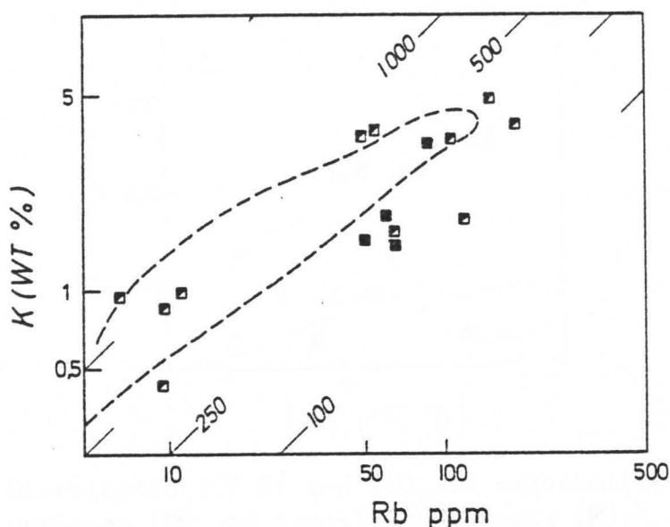
Fig.30. Distribution of K and Rb in all amphibolite facies gneisses (■) and transitional rocks (▤) listed in Table 29. The outlined area is the field of the granulites in Fig.23.
