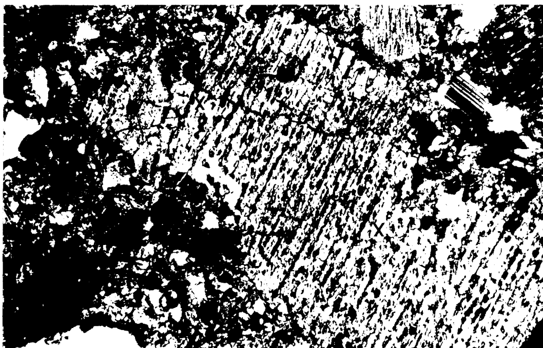
Plate 27. Metagabbro; detail of clinopyroxene (X) with regularly distributed grains of plagioclase, sphene and hornblende. X50, Tete area (sample no.T201; Coelho, 1969).
