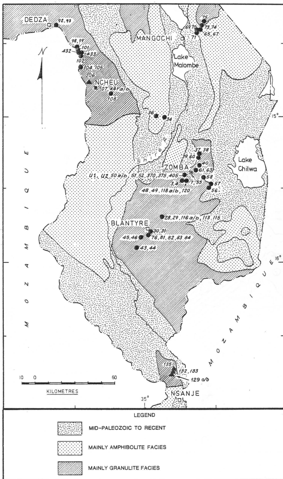
Fig.19. Locality map for analysed rock samples: orthopyroxene granulites (•); garnet-clinopyroxene granulites (▲); (modified after Bloomfield, 1968).
