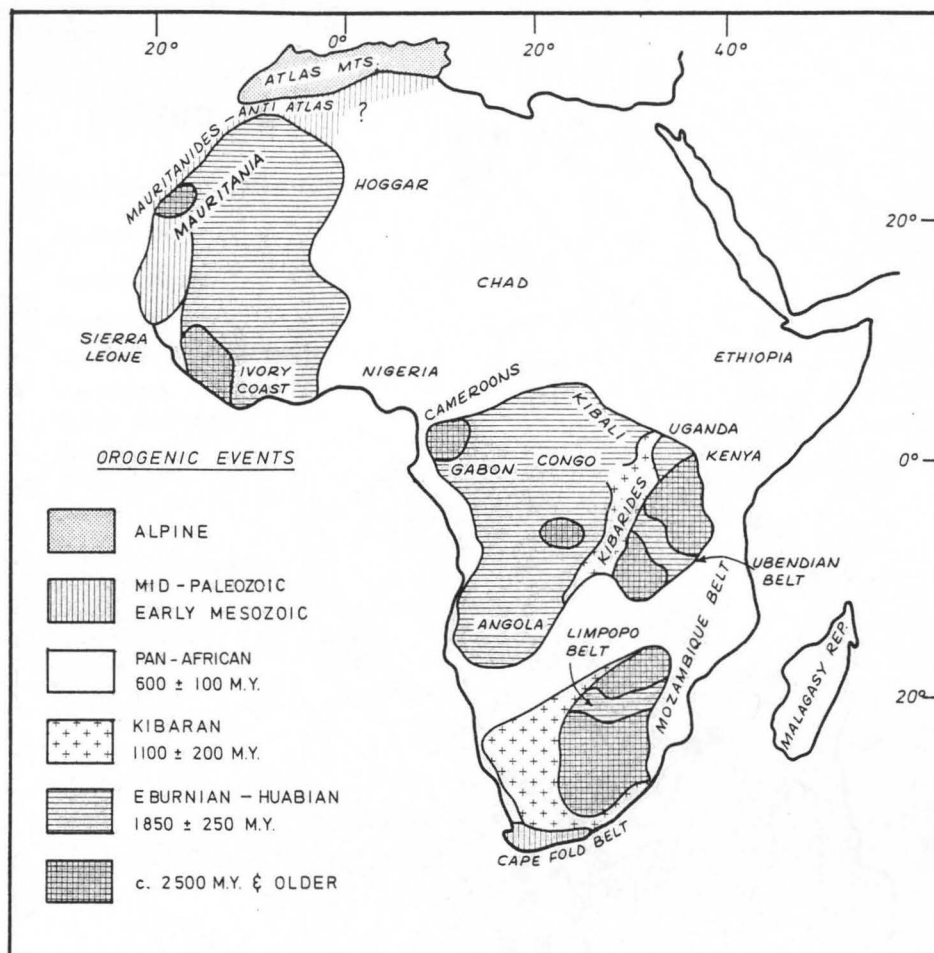
Fig.1. Generalized map of major structure units of Africa undisturbed by subsequent events (after Clifford, 1974).
