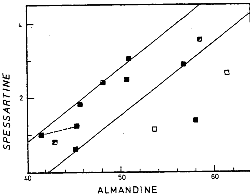
Fig.14. Distribution of almandine and spessartine end-members in garnets. Garnet-orthopyroxene granulites ( \square ); garnet-clinopyroxene granulites ( \blacksquare ); and garnet-two pyroxene granulites ( \square ). Broken line joins analyses of zoned garnet; for the field between lines, see text.
