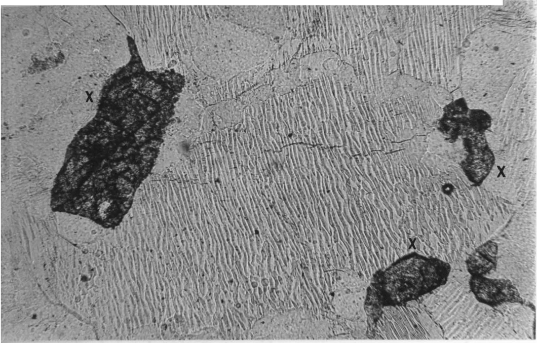
Plate 3. Leucocratic granulite rich in mesoperthite; note stable xenoblastic orthopyroxene (x). X120, Ncheu (see Locality 458, Map 3).
