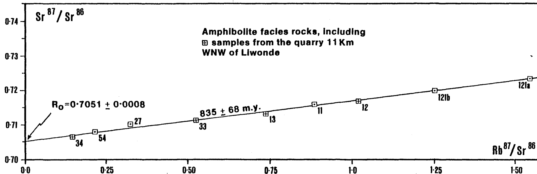
Fig.VI-E. Rb-Sr whole-rock isochron diagram, after Clifford et al. (in prep.), for the southern Malawi regional amphibolite facies gneisses (see Appendices VI-B and VI-2 for sample localities and Appendix II-3 for petrographic descriptions).
