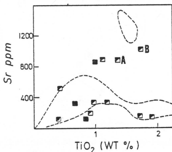
Fig.31. Distribution of Sr and \text{TiO}_2 in amphibolite facies gneisses (■) and transitional rocks (▤). A and B are samples from localities nos. 30 and 31 (see Fig. 19). The outlined areas are the fields of granulites in Fig.24.
