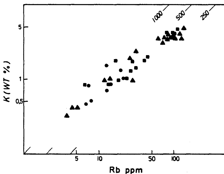
Fig.23. Distribution of K and Rb in melanocratic (•), mesocratic (■), and leucocratic (▲) orthopyroxene-bearing granulites listed in Tables 24 to 26.
