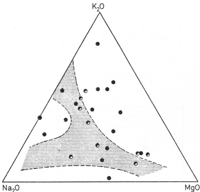
Fig.28. \text{Na}_2\text{O} - \text{K}_2\text{O} - \text{MgO} diagram (weight per cent) of all amphibolite facies gneisses (●) and amphibolite to granulite facies transitional rocks (◐) listed in Tables 27 and 28, in relationship to the field (shaded) of granulites in Fig.21(a).
