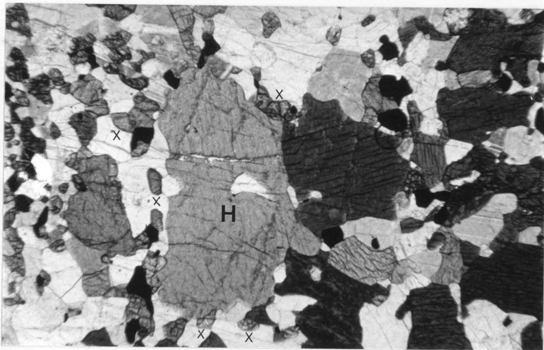
Plate 10. Type I prograde geometry: detail of interface between granulite (left) and amphibolite (right). Note the incipient growth of small orthopyroxene (X) from a large hornblende (H). X120, Middle Shire Valley transition zone (see Locality 322, Map 2).
