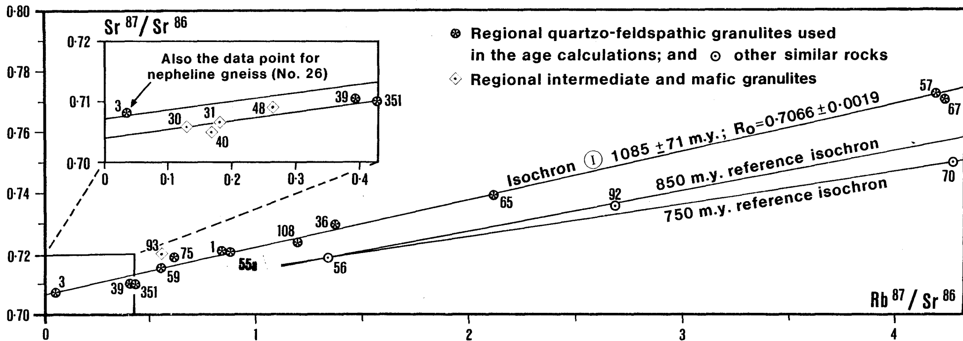
Fig.VI-C. Rb-Sr whole-rock isochron diagram, after Clifford et al. (in prep.), for the regional quartzo-feldspathic granulites of southern Malawi (see Appendices VI-B and VI-2 for sample localities and Appendix II-3 for petrographic descriptions).
