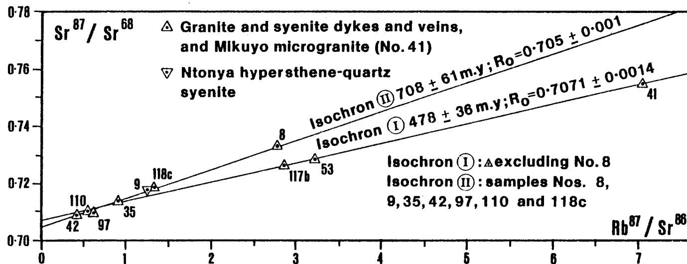
Fig.VI-G. Rb-Sr whole-rock isochron diagram, after Clifford et al. (in prep.), for the southern Malawi granite and syenite dykes and veins (see Appendices VI-B and IV-2 for sample localities and Appendix II-3 for petrographic descriptions).
