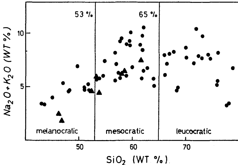
Fig.22. Distribution of (\text{Na}_2\text{O}+\text{K}_2\text{O}) and \text{SiO}_2 in all granulites listed in Tables 20 2 to 22 2 . Two-pyroxene granulites, (●); and garnet-clinopyroxene granulites, (▲).
