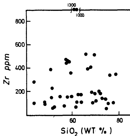
Fig.26. Plot of Zr and \text{SiO}_2 in orthopyroxene granulites listed in Tables 24 to 26.
