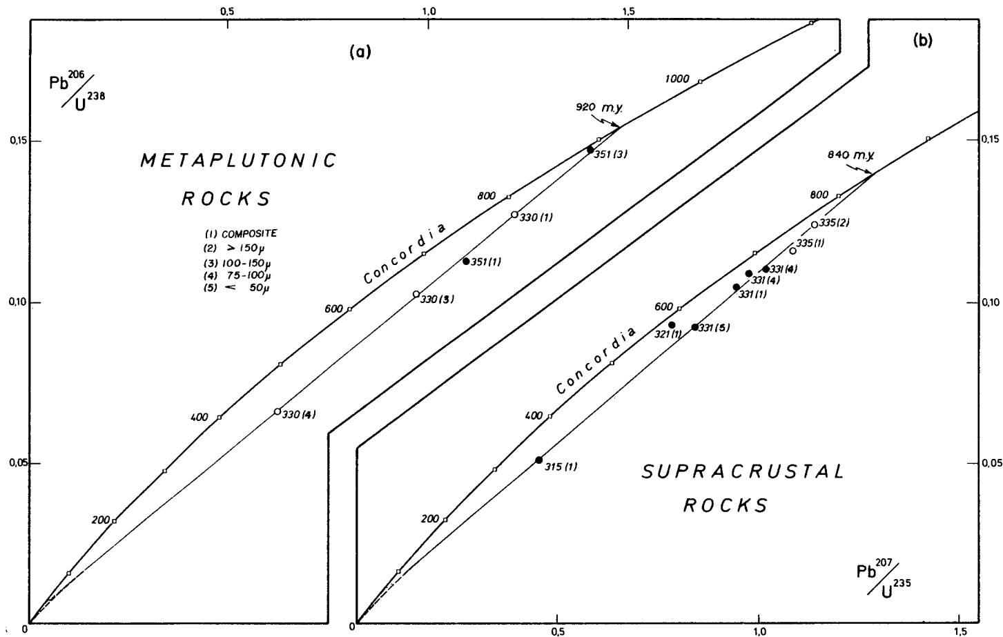
Fig.49(a). Concordia plot for zircon fractions from metaplutonic rocks of the Middle Shire area; (●) hypersthene-bearing rocks, and (○) gneisses and orthogneisses (see note 1 to Table 42). Fig.49(b). Concordia plot for zircon fractions from supracrustal rocks of the Middle Shire area (the symbols are the same as in Fig.49(a); see note 1 to Table 42).
