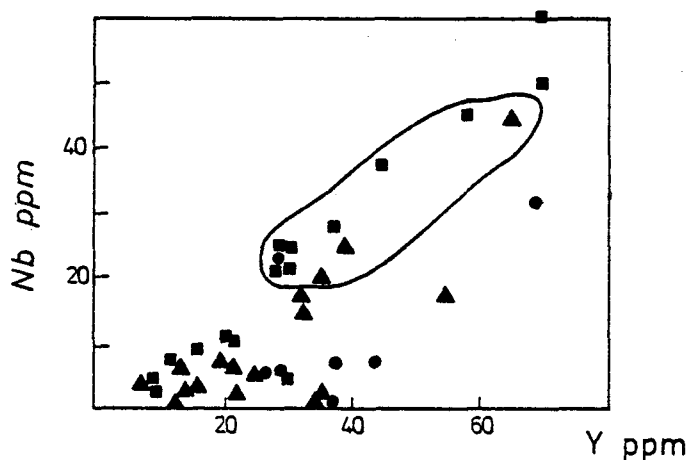
Fig.27. Distribution of Y and Nb in melanocratic ( \bullet ), mesocratic ( \blacksquare ), and leucocratic ( \blacktriangle ) orthopyroxene granulites listed in Tables 24 to 26. The outlined field is discussed in the text.
