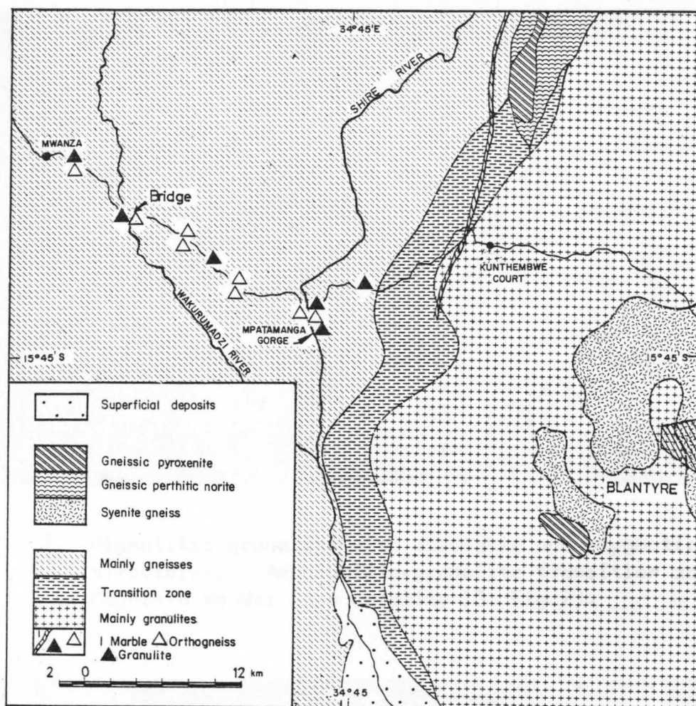
Fig.8. Geology of the Middle Shire area (after Morel, 1961a).
