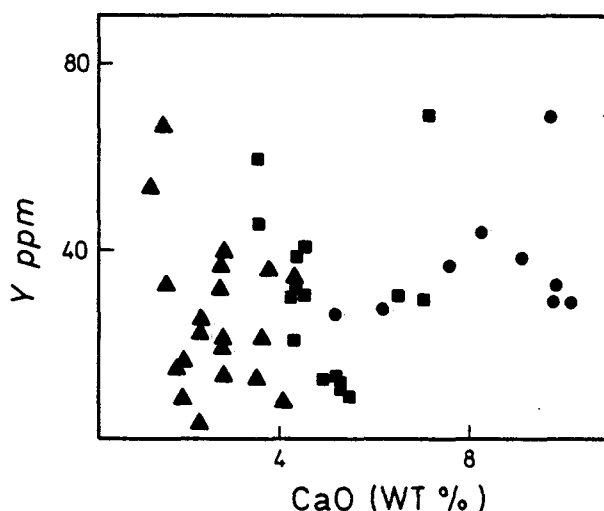
Fig.25. Distribution of Y and CaO in melanocratic (•), mesocratic (■), and leucocratic (▲) orthopyroxene granulites listed in Tables 24 to 26.
