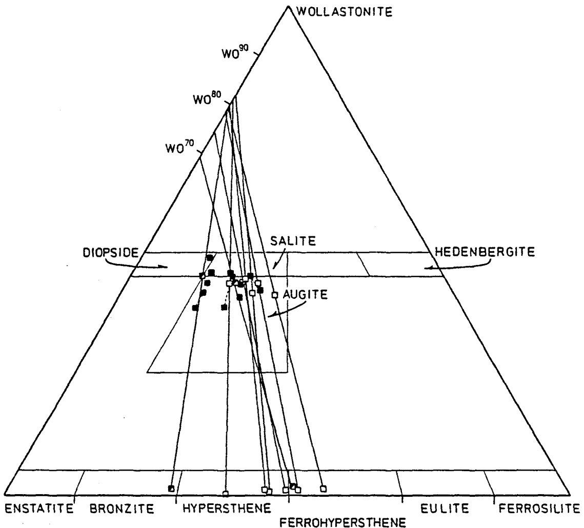
Fig.10. Distribution of wollastonite-enstatite-ferrosilite end-members in pyroxenes. Two-pyroxene granulites (□); garnet-clinopyroxene granulites (■); and garnet-two-pyroxene granulites (▤). Broken lines join analyses from zoned minerals and tie-lines join coexisting ortho- and clinopyroxenes.
