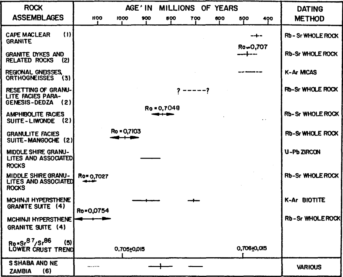
Fig.55. Age determinations in southern Malawi and other relevant areas. (1) Snelling (1963); (2) Clifford et al. (in prep.); (3) Bloomfield (1970); (4) Brewer et al. , (1979); (5) Clifford (1974); and (6) Cahen (1970).
