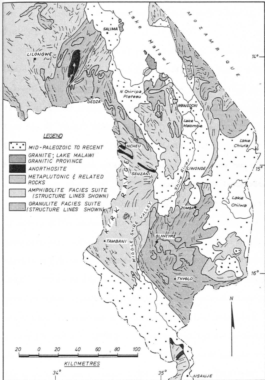
Fig.4. Geology of southern Malawi (after Bloomfield, 1968).
