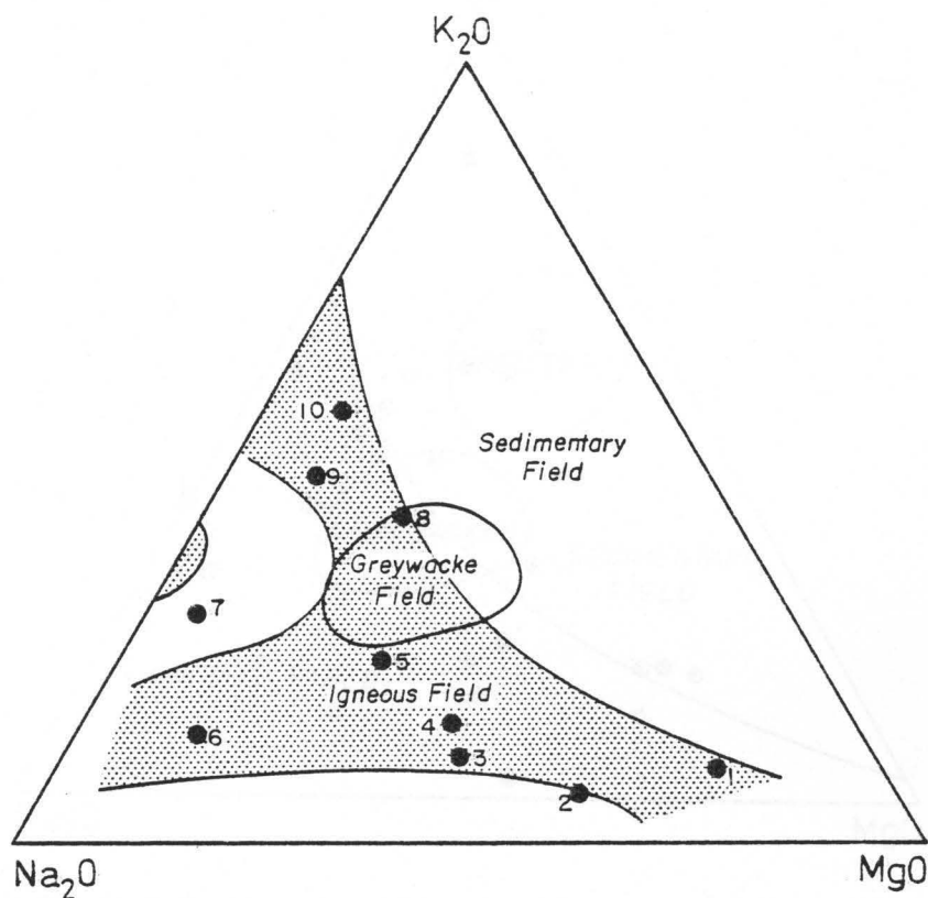
Figs.39. K_2O - Na_2O - MgO diagram illustrating the distribution of the southern Malawi granulites (shaded area; see Fig. 21(a) in relation to sedimentary and igneous fields (given by de La Roche, 1966). Dots (●) 1 to 10 are average plots of: (1), alkali gabbro; (2), Ural spilite; (3), spilite; (4), and (5), andesite; (6), Fiji (low-K) rhyodacite; (7), New Zealand quartz-keratophyre; (8), monzonite; (9), alkali syenite; (10), calc-alkali granite. Sources of data are: (1), (4), (5), (8), (9), and (10), Nockolds (1954); (2), Sharfman (1968); (3) Sundius (1930, p.9); (6), Gill and Gordon (1973); and (7), Bartrum (1936, p.417, n.1).
