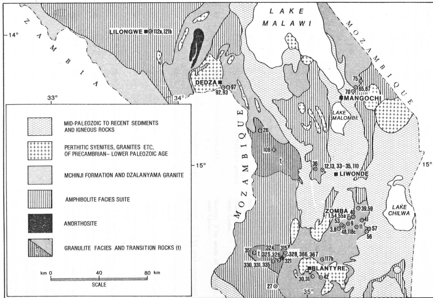
Fig.VI-B. Generalised locality map for samples used in age determinations (after Clifford et al. , in prep.; Bloomfield, 1968).
