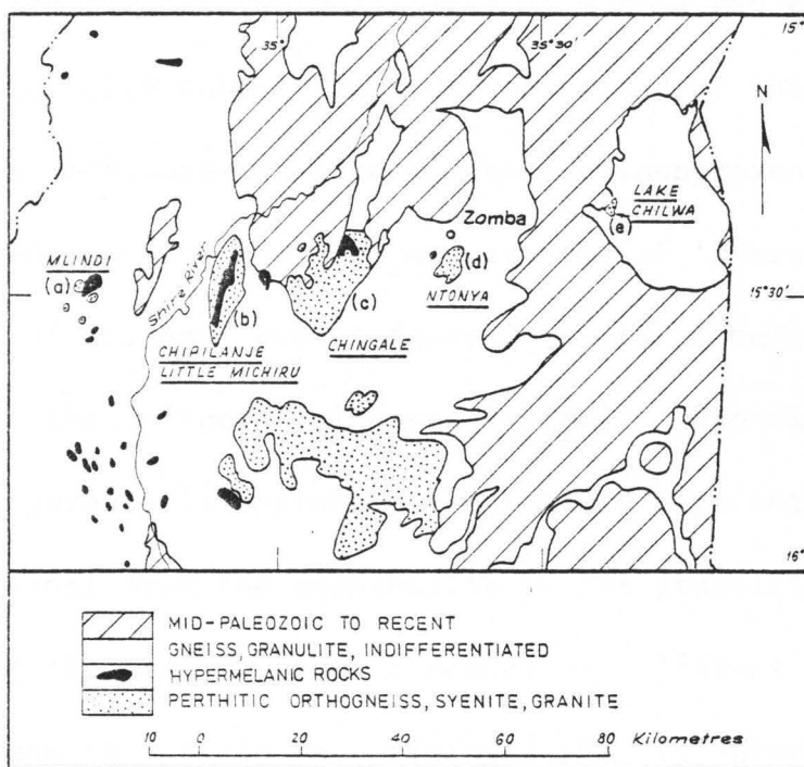
Fig.5. Geology of part of southern Malawi showing five plutonic Ring Complexes indicated by letters (a) to (e) and with their names underlined (after Bloomfield, 1965b).
