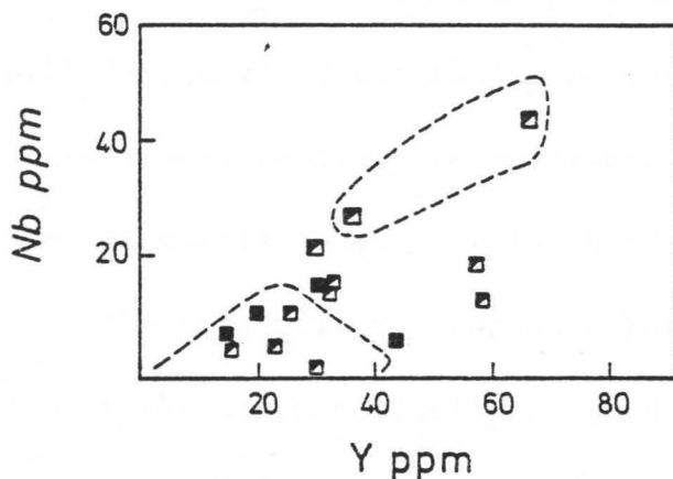
Fig.32. Distribution of Nb and Y in amphibolite facies gneisses (■) and transitional rocks (▤). The outlined areas are fields of granulites in Fig.27.
