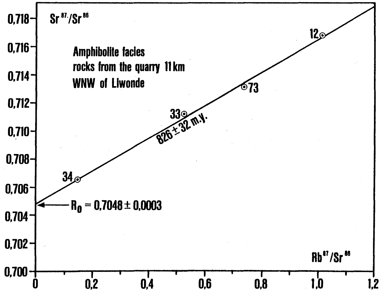
Fig.VI-F. Rb-Sr whole-rock isochron diagram for the Liwonde quarry gneisses and amphibolite (see Appendices VI-B and VI-2 for sample localities and Appendix II-3 for petrographic descriptions).
