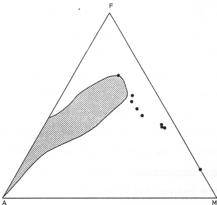
Fig.34. AFM diagram of all amphibolite, metadolerite, metagabbro and related rocks (•), listed in Appendix IV-11. Shaded area is the field of pyroxene granulites in Fig.21(b).
