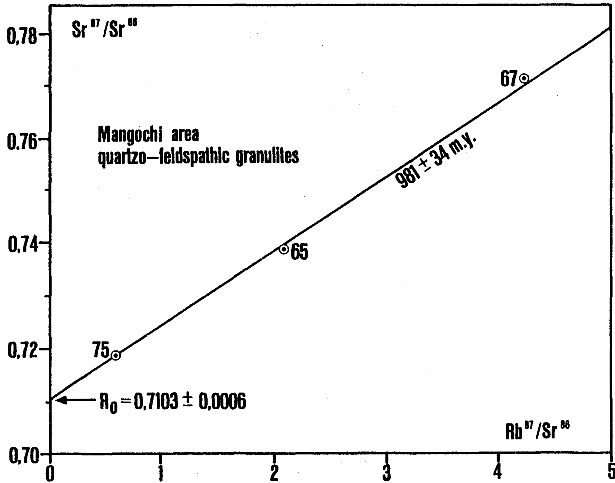
Fig.VI-D. Rb-Sr whole-rock isochron diagram for the Mangochi area granulites and related rocks (see Appendices VI-B and VI-2 for sample localities and Appendix II-3 for petrographic descriptions).
