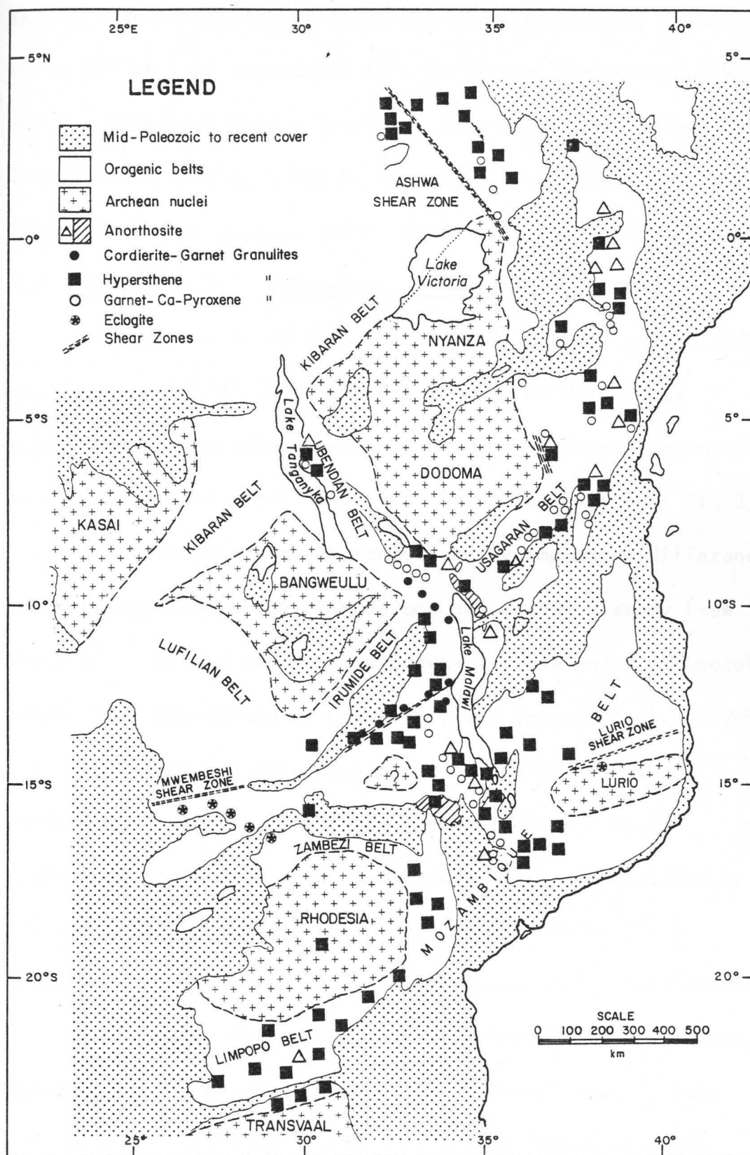
Fig.2. Main structural units in East Africa (modified after Vail, 1965; Saggerson, 1973; Saggerson and Turner, 1980).
