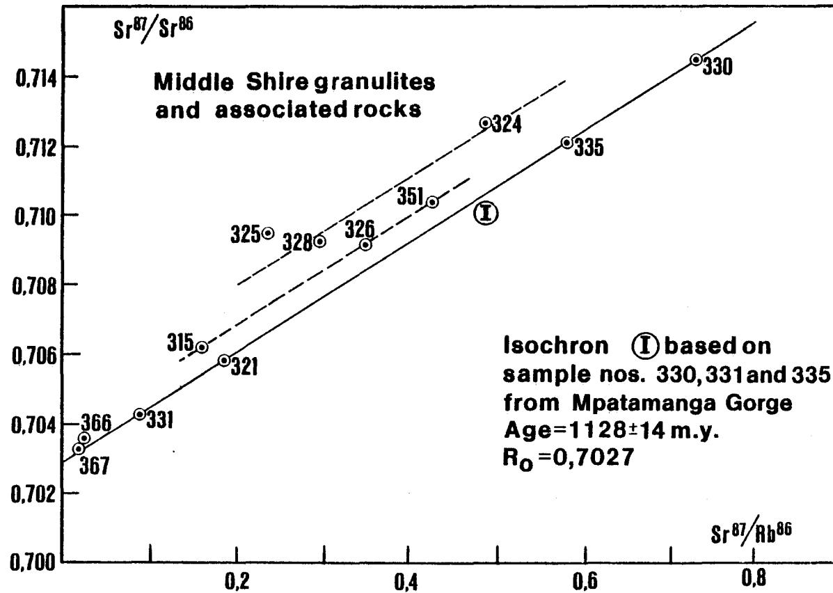
Fig.48. Rb-Sr whole-rock isochron diagram (after York, 1969) for the Middle Shire granulites, and associated rocks (see Fig.47 and Appendices VI-A, VI-B and VI-2 for localities and Appendix II-3 for petrographic data).
