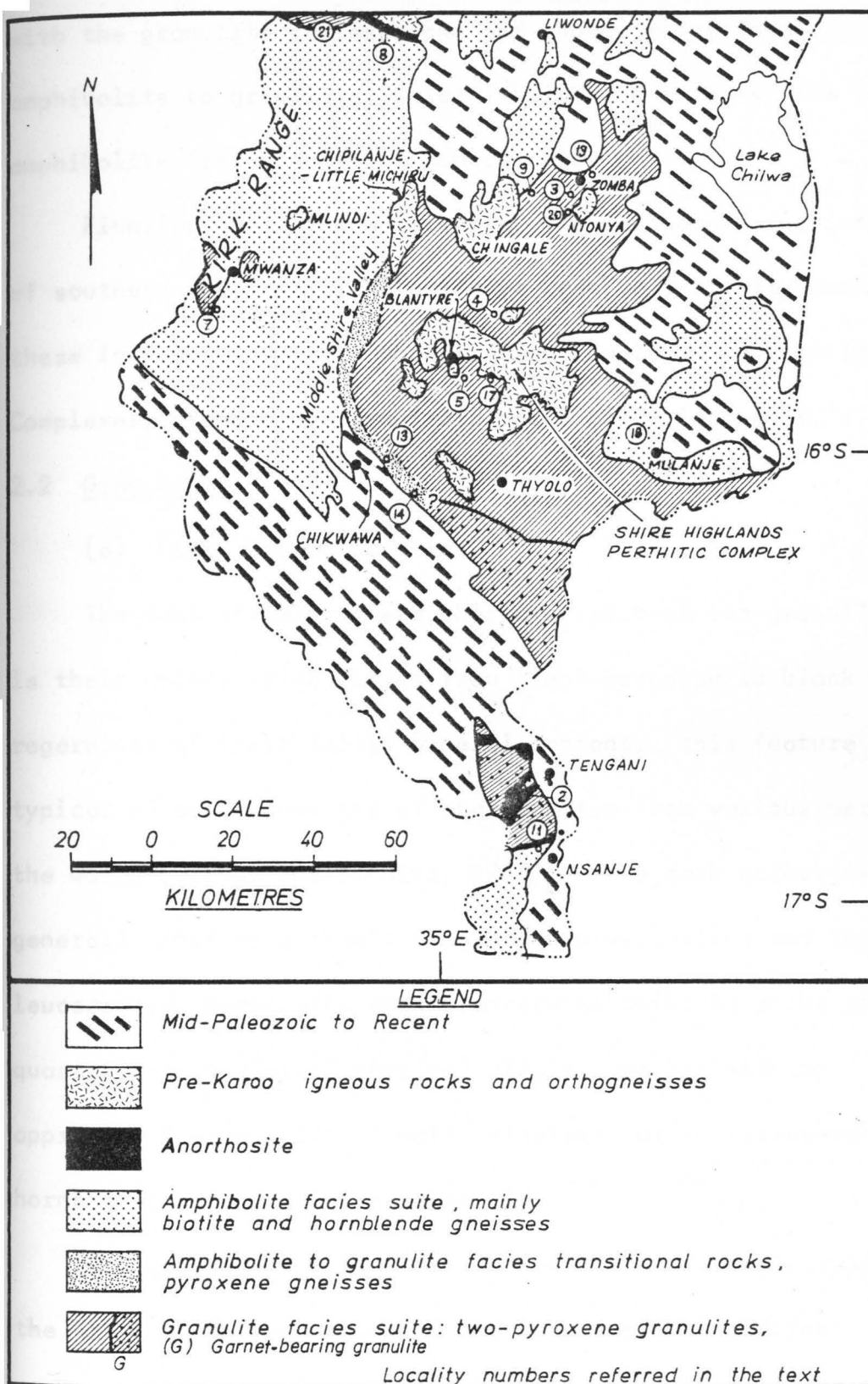
Fig.7. Locality map for southern Malawi (modified after Bloomfield, 1968; Morel, 1958).
