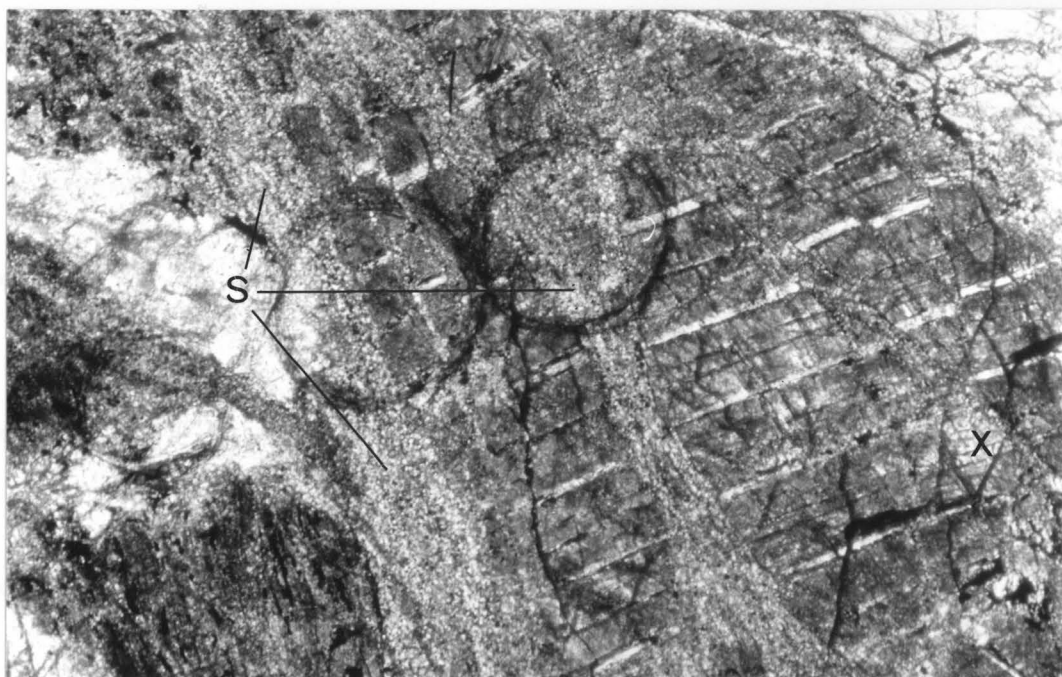
Plate 24. Pyroxenite, detail of clinopyroxene (X), with scapolite-hornblende-microshears (S) off-setting exsolution lamellae of orthopyroxene. X50, Tete area (sample no.T117; Coelho, 1969).
