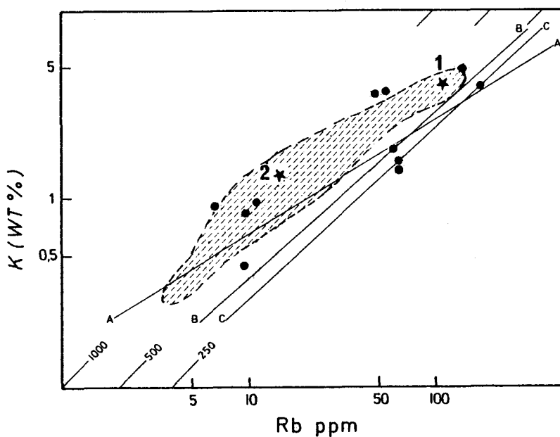
Fig.45. Distribution of K and Rb in southern Malawi granulites (shaded area; see Fig.23) and in gneisses and transitional rocks (dots (•); see Fig.30), in relation to igneous trends of: (A), island-arc igneous suites (given by Jakés and White, 1970); (b), lower crust granulite and charnockite suites (given by Lewis and Spooner, 1973); and (c), high-level igneous rocks (given by Shaw, 1968). Stars (★) are: (1), average of five rhyolites (Groome and Hall, 1974); and (2), Saipan dacite (Taylor et al. , 1969).
