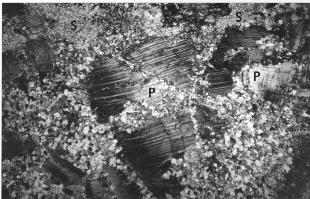
Plate 25. Anorthosite, detail of sheared plagioclase (P); note scapolite (S), and size breakdown of feldspar along cross-cutting shears. X10, crossed nicols, Tete area (sample no.T11; Coelho, 1969).
