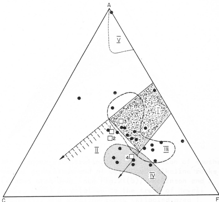
Fig.42. ACF diagram illustrating the distribution of southern Malawi amphibolite facies gneisses and amphibolite to granulite facies transitional rocks (●) listed in Tables 27 and 28, in relation to the sedimentary and igneous fields and average composition of igneous rocks referred to in Fig.41. Field (V): Al-rich clay and shale (given by Winkler, 1967, p.56).
