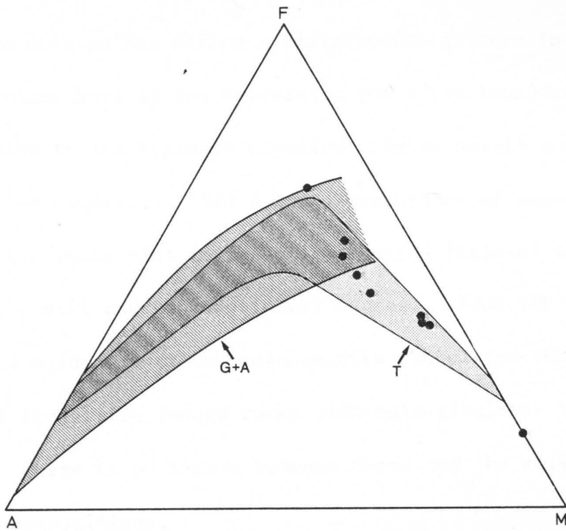
Fig.43. AFM diagram illustrating the distribution of southern Malawi granulites and of world calc-alkaline rocks (shaded area G+A; see Fig.21(b); Robinson and Leake, 1975) in relation to the trend of Hawaii tholeiitic and alkaline rocks (stippled area T, given by MacDonald, 1968). Dots (•) are plots of northern Kirk Range amphibolite, metagabbro and peridotite (see Fig.34 and Appendix IV-11).
