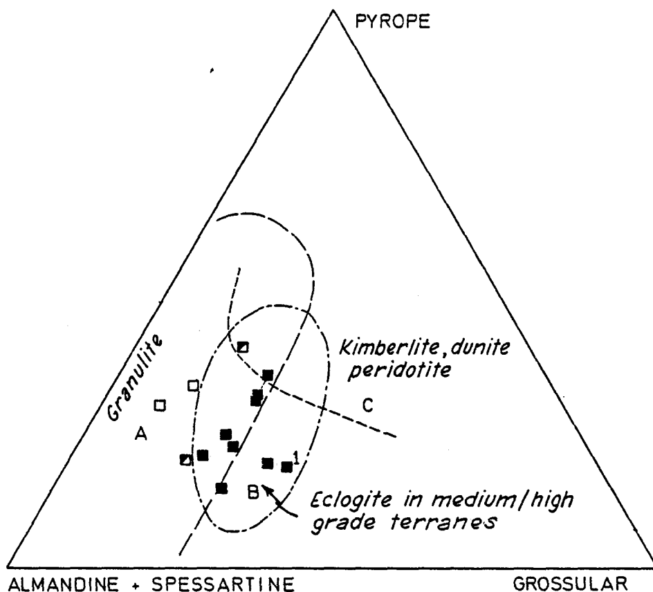
Fig.15. Distribution of end-members in garnet, showing the fields of garnet from granulite, eclogite, etc. from Winkler (1974, p.269). Garnet-orthopyroxene granulites (□); garnet-clinopyroxene granulites (■); and garnet-two-pyroxene granulites (◐). Broken line joins analyses of zoned garnet; for sample no.1 see text.
