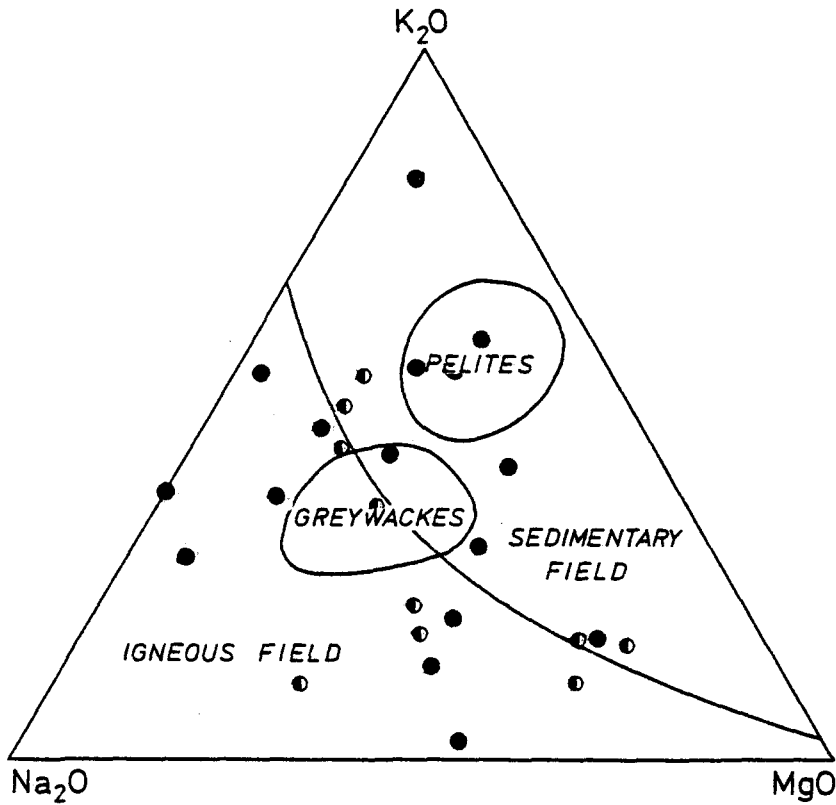
Fig.40. K_2O - Na_2O - MgO diagram illustrating the distribution of the southern Malawi amphibolite facies gneisses (●), and amphibolite to granulite facies transitional rocks (⊙) (see Fig.28), in relation to sedimentary and igneous fields (given by de La Roche, 1966).
