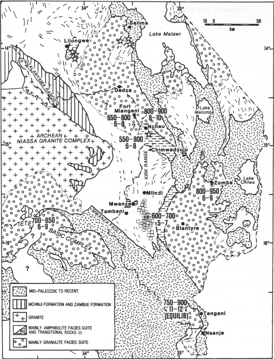
Fig.52. Regional distribution of P-T conditions in southern and central Malawi showing T in °C and P in kbar ; (□) biotitite and (☆) garnet-olivine rocks (after Freitas, 1956; Coelho, 1956, Assuncao and Coelho, 1956; Morel, 1961a; Bloomfield, 1968; Oberholzer, 1968; Saggerson and Turner, 1980 ; see Appendix VII).
