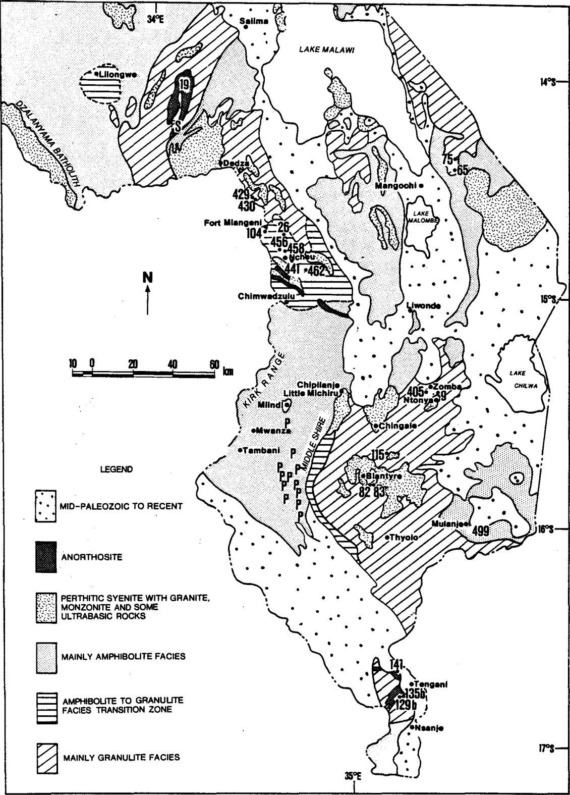
Fig.38. Generalized map of localities referred to in Chapter 6; P: biotitite rocks(modified after Bloomfield, 1968; Morel, 1961a).
