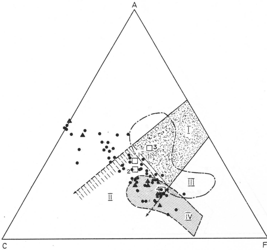
Fig.41. ACF diagram illustrating the distribution of all southern Malawi two-pyroxene granulites (●) and garnet-clinopyroxene granulites (▲) listed in Tables 20 to 22, in relation to sedimentary and igneous fields of: (I), clays and shales with up to 35 per cent carbonate; (II), marls; (III), greywacke; (IV), basaltic and andesitic rocks (given by Winkler, 1967, p.56). Squares (□) 1 to 4 are average plot of: (1), granodiorite; (2), tonalite; (3), calc-alkali granite; (4), basalt (Nockolds, 1954).
