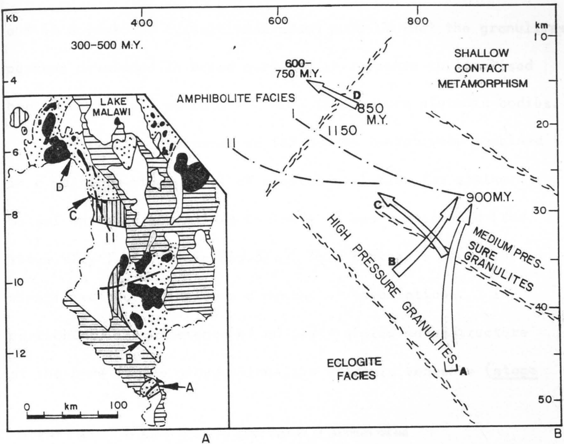
Fig.56(a). Generalised map of metamorphic assemblages in southern Malawi. Horizontal ruling, mid-Paleozoic to Recent; black, metamorphosed plutonic rocks; blank, gneisses; vertical ruling, transitional rocks; and stippled, granulites. Curves (I) and (II) are thermal profiles and (A), (B), (C) and (D) are polymetamorphic terranes shown in Fig.56(b).
