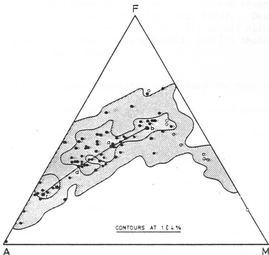
Fig.53. AFM diagram for the southern Malawi granulite facies rocks (●), and Kirk Range amphibolite and metadolerite (○) superimposed on field of 240 hypersthene-bearing rocks of African charnockite-granulite suites (after Clifford, 1974), in relation to Daly's (1933) average rhyolite (r), dacite (d), andesite (a) and basalt (b).
