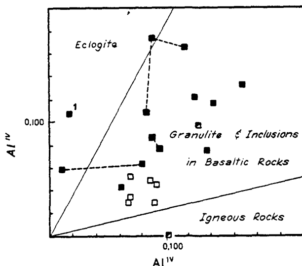
Fig.11. Distribution of Al^{iv} and Al^{vi} in clinopyroxenes. Two-pyroxene granulites (□); garnet-clinopyroxene granulites (■) and garnet-two-pyroxene granulites (◐). Labelled fields after Aoki and Kushiro (1968). See text for data on no.1.
