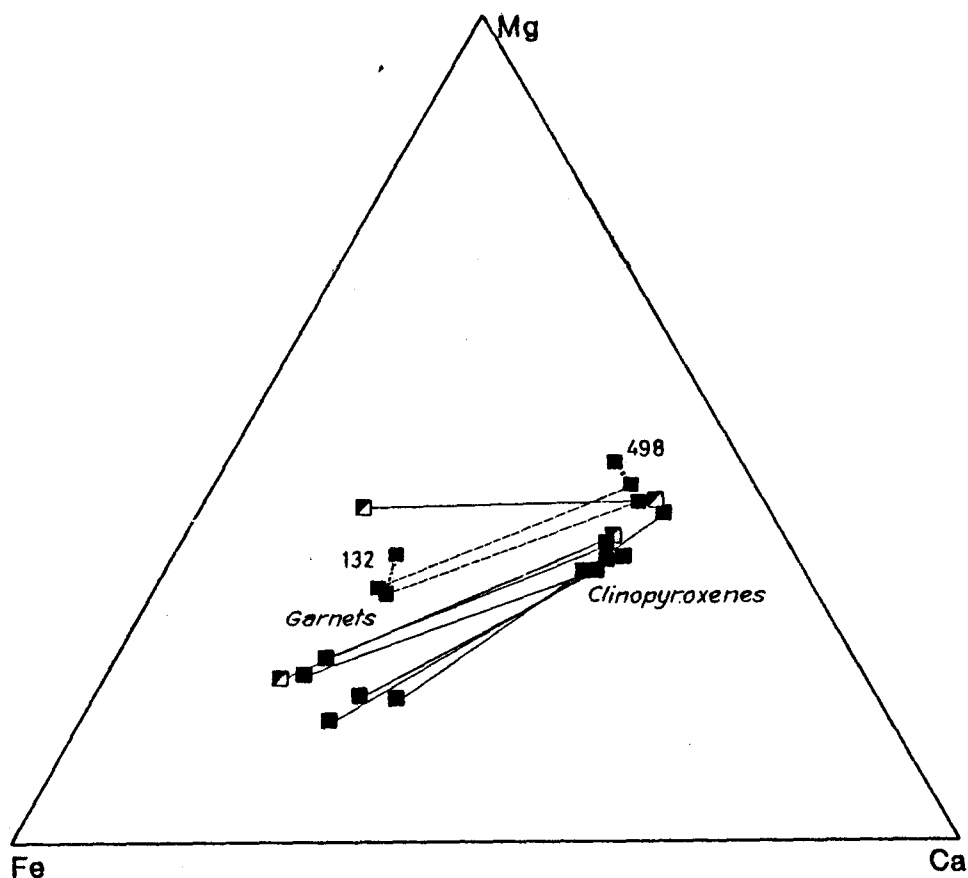
Fig.16. Distribution of Ca, Mg, Fe in coexisting garnet and clinopyroxenes from garnet-clinopyroxene granulites (■) and garnet-two-pyroxene granulites (□); broken tie-lines link minerals nos. 132 and 498 from Tengani (see Fig.9); dotted lines join analyses of zoned minerals.
