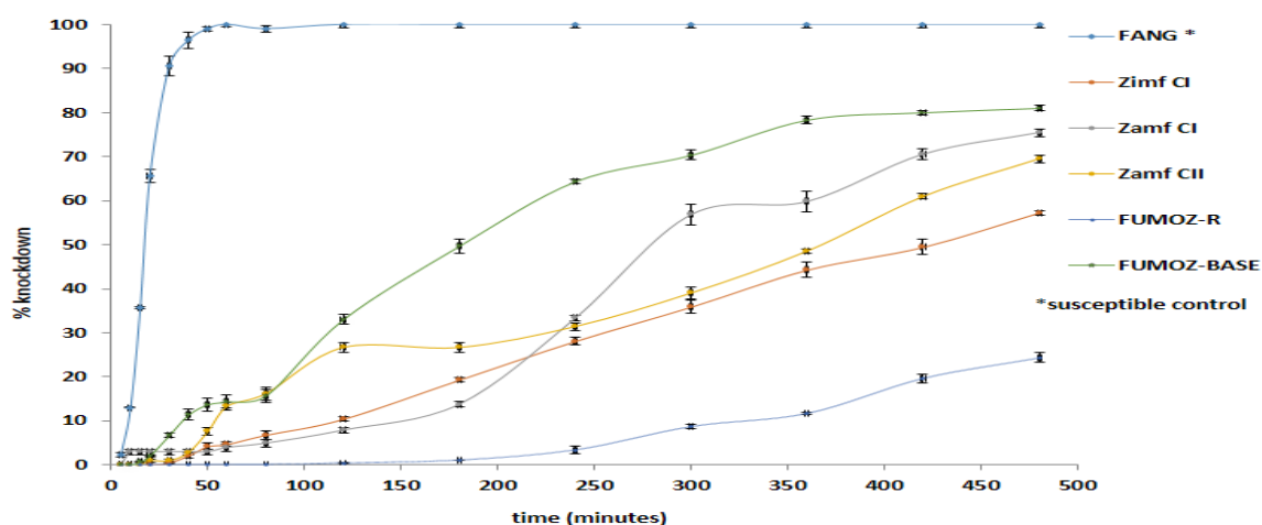
Figure 3.2: Deltamethrin induced knockdown trends in wild caught and laboratory An. funestus over an 8 hour exposure period. The susceptible FANG strain reached 100% knockdown within 1 hour, while none of the other (i.e. resistant strains) test strains were fully knocked down by 8 hours. The FUMOZ-R strain showed the lowest knockdowns over time. Wild-caught strains (Zimf CI, Zamf CI, Zamf CII) displayed knockdown rates lower than the unselected FUMOZ-BASE strain.
