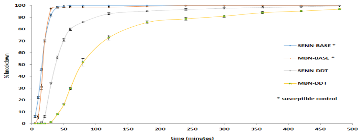
Figure 3.4: Deltamethrin induced knockdown trends in laboratory An. arabiensis over 8 hour exposure period. Susceptible laboratory strains (SENN-BASE and MBN-BASE) portrayed similar knockdown trends and 100% knockdown was reached in 1 hour. SENN-DDT displayed higher deltamethrin knockdown trend than MBN-DDT. However, the two resistant strains showed no difference to susceptible strains post the 6 th hour of exposure.
