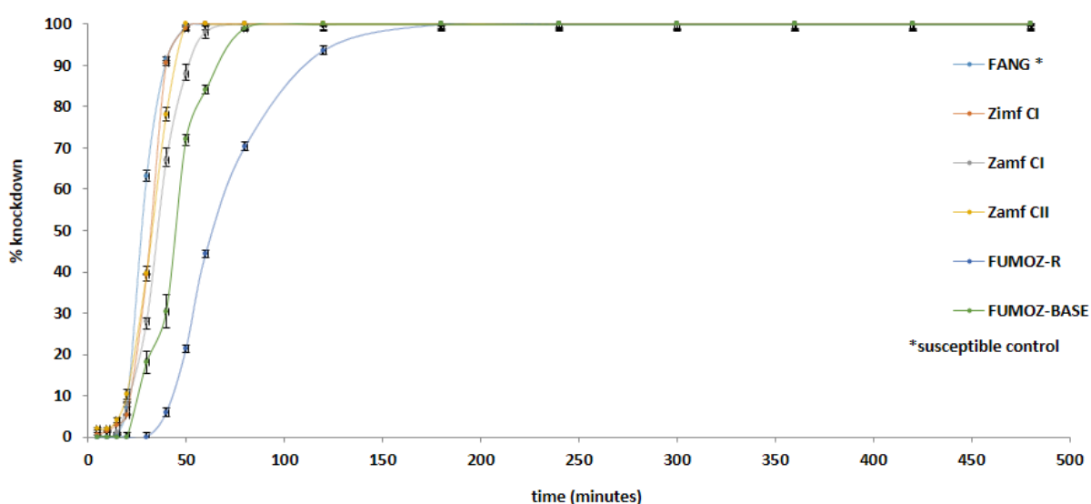
Figure 3.3: Bendiocarb induced knockdown trends in wild caught and laboratory Anopheles funestus over an 8 hour exposure period. All the strains reached 100% knockdown by 3.33 hours. The FUMOZ-R strain displayed the slowest knockdown rates, followed by FUMOZ-BASE, while the wild strains (Zimf CI, Zamf CI, Zamf CII) displayed knockdown rates similar to the susceptible FANG strain.
