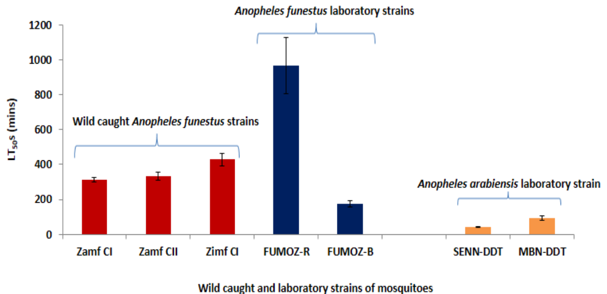
Figure 3.9: Deltamethrin lethal times of wild caught and laboratory Anopheles strains. Wild caught An. funestus strains dark red are compared to laboratory An. funestus strains dark blue and laboratory An. arabiensis strains represented with orange bars. The Zimbabwe wild An. funestus strain (Zimf CI) had higher deltamethrin induced lethal times than Zambia strains (Zamf CI and Zamf CII). There was no difference in deltamethrin induced lethal times between the Zambia strains (Zamf CI and Zamf CII). FUMZ-R had higher deltamethrin induced lethal time than FUMZ-BASE and An. funestus wild caught
