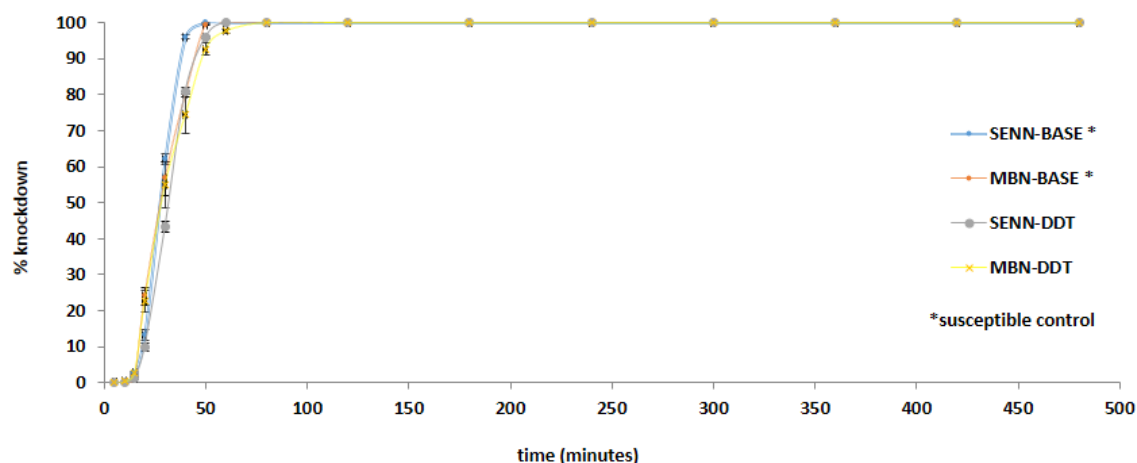
Figure 3.5: Bendiocarb induced knockdown trends in laboratory An. arabiensis over 8 hour exposure period. Pyrethroid susceptible laboratory strains (SENN-BASE and MBN-BASE) showed similar knockdown trends. Even though MBN-DDT has cross resistance to bendiocarb (Nardini et al. , 2012), its resistance intensity knockdown trends do not show difference to bendiocarb susceptible strains.
