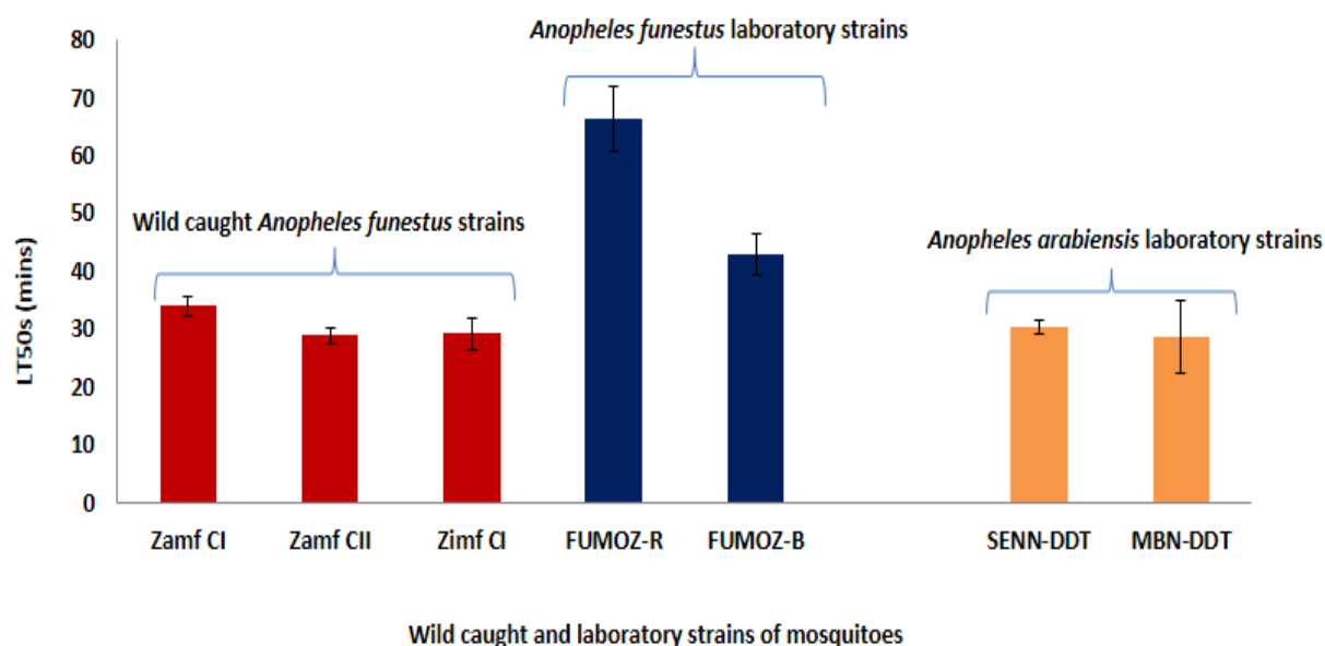
Figure 3.8: Bendiocarb lethal times of wild caught and laboratory Anopheles strains.
