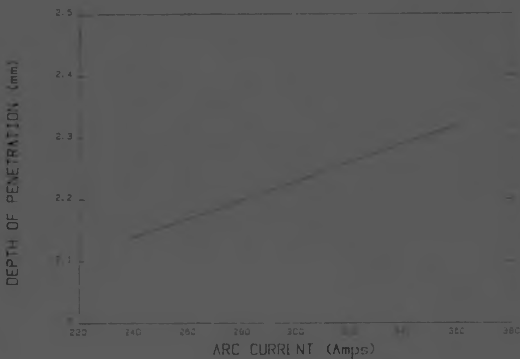
Figure 7.18 Relationship of Depth of penetration vs arc current.
