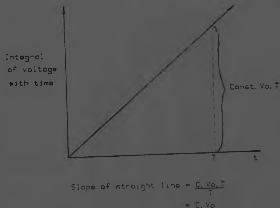
Figure 3.3 Representation of output from the chart recorder.
