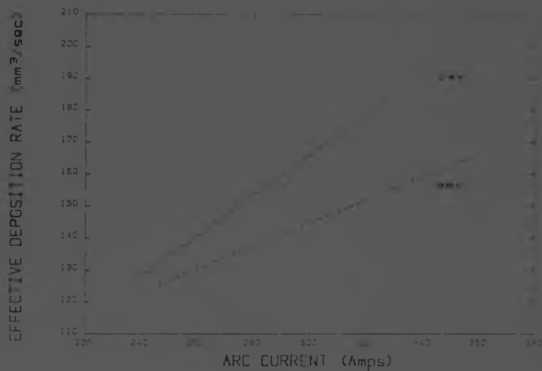
Figure 5.8 Graphical representation of effective deposition rate vs arc current and voltage.
