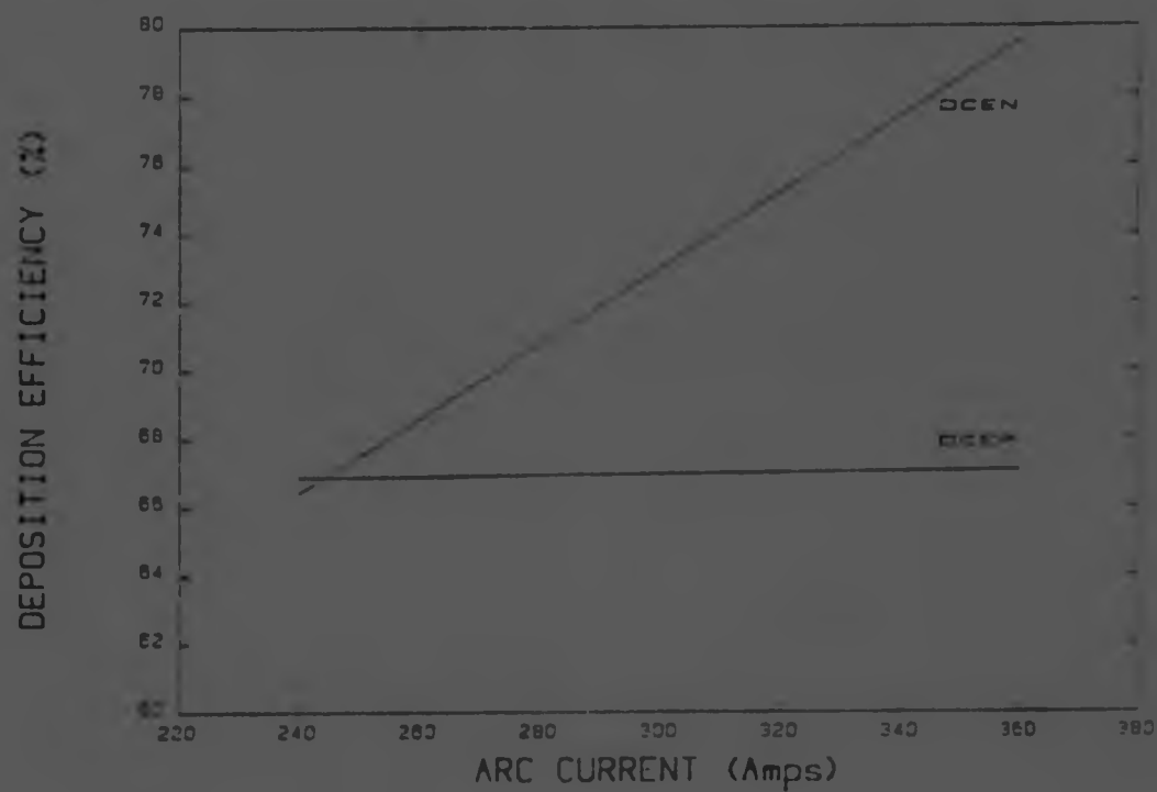
Figure 5.3 Graphical representation of deposition efficiency vs arc current and polarity.
