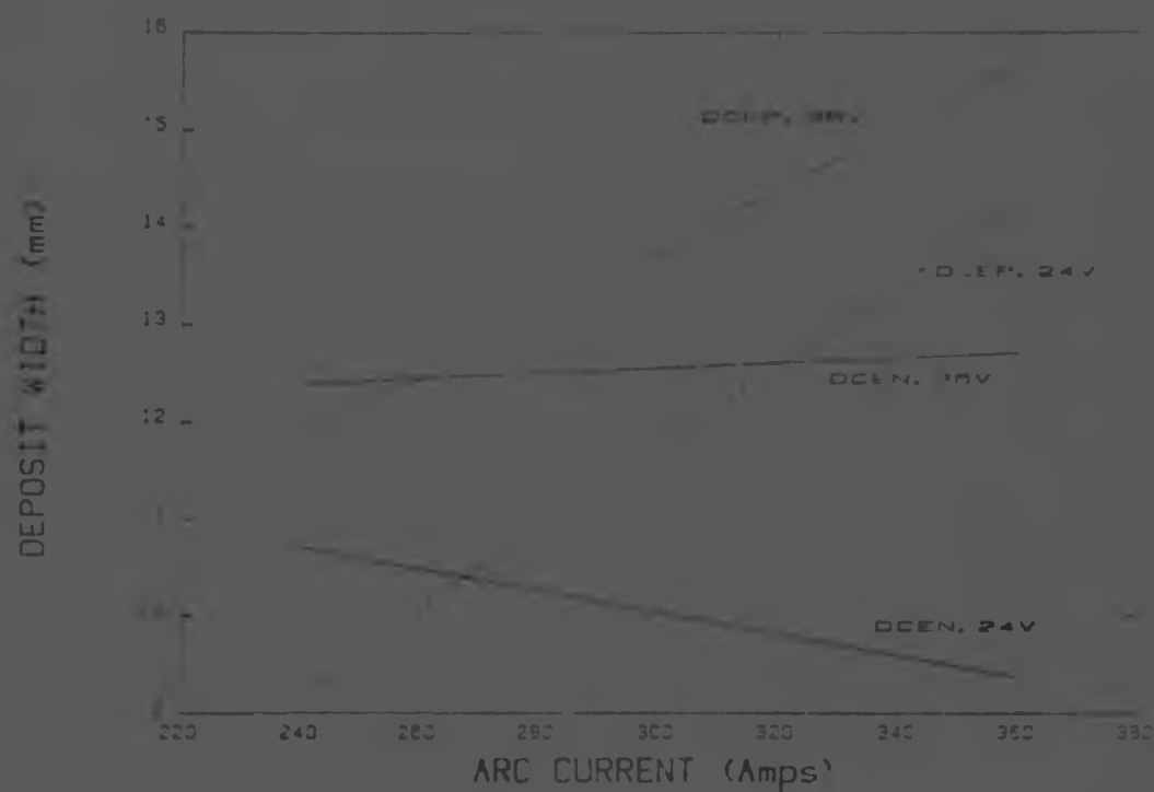
Figure 5.13 Graphical representation of deposit width vs arc current, arc voltage and polarity.
