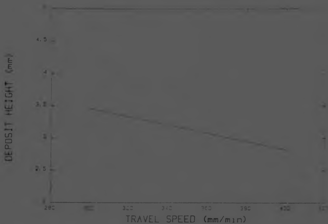
Figure 7.17 Relationship of Deposit Height Travel Speed
