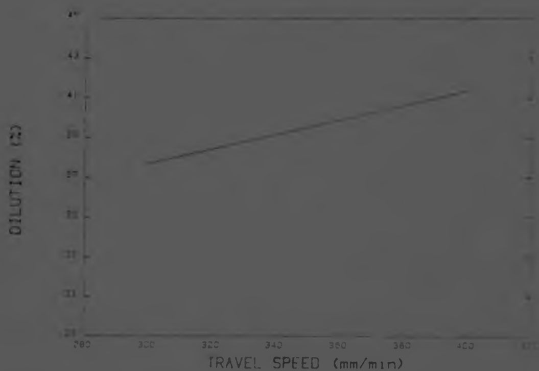
Figure 5.23 Graphical representation of deposit dilution vs travel speed.
