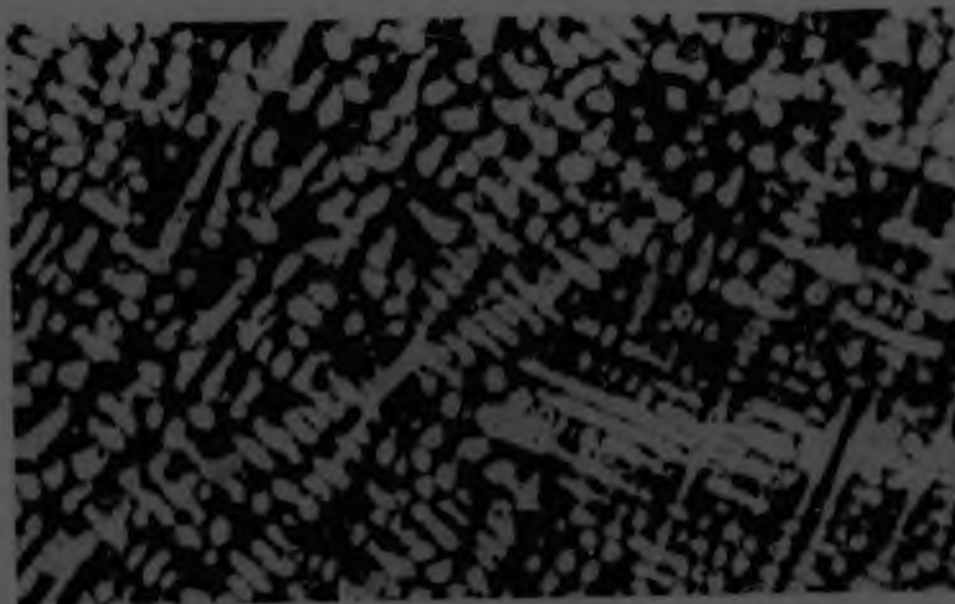
Figure 4.1 Photomicrograph of the dendritic microstructure of the weld bead with the lowest percentage dilution. Magnification 500X.
