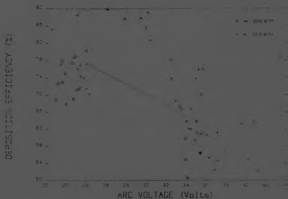
Figure 5.1 Graph showing all data points of deposition efficiency vs arc voltage for the discussion of factorial experiments.
