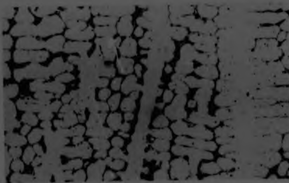
Figure 4.2 Photomicrograph of the dendritic microstructure of the weld deposit with the highest percentage dilution. Magnification 500X.
