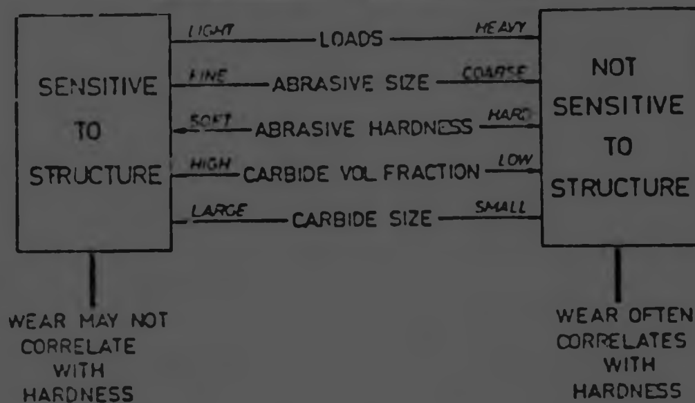
Figure 2.1 Model showing relationship between abrasive wear parameters and microstructure.
