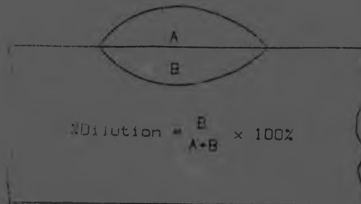
Figure 2.4 Schematic representation of the percentage dilution of a weld deposit.
