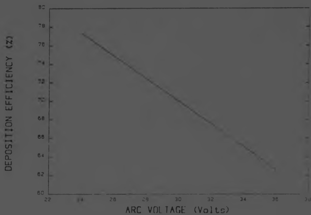
Figure 5.4 Graphical representation of deposition efficiency vs arc voltage.
