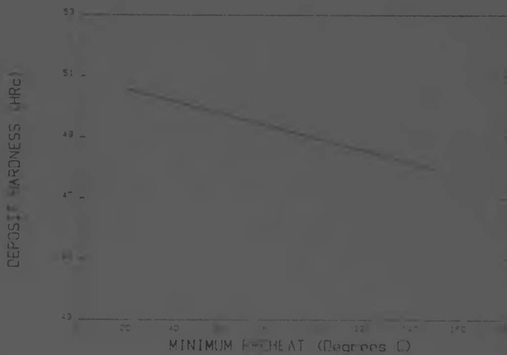
Figure 2.26 Graphical representation of deposit hardness vs minimum preheat.
