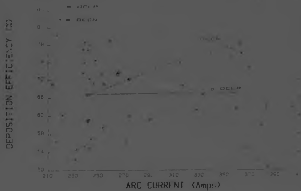
Figure 5.2 Graph showing all data points of deposition efficiency vs arc current and polarity for the discussion of interactions in factorial experiments.
