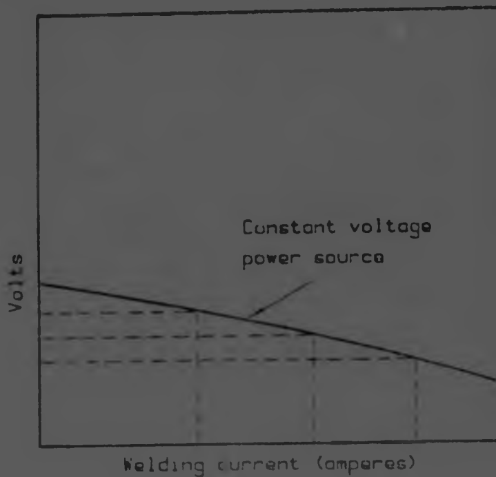
Figure 2.7 Characteristic arc current Versus voltage curve for a constant voltage power supply.
