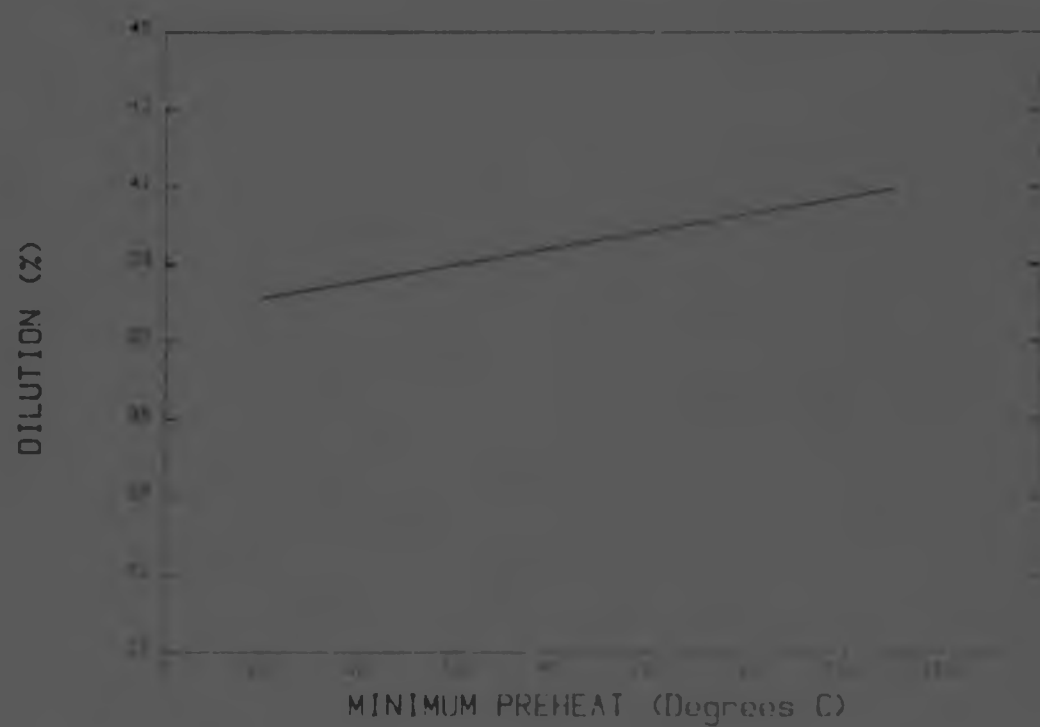
Figure 5.24 Graphical representation of deposit dilution vs minimum preheat.
