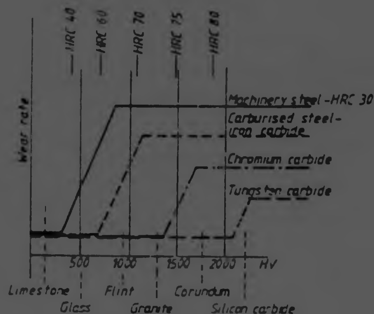
Figure 2.2 Idealized diagram of abrasive wear rate of materials versus mineral hardness.
