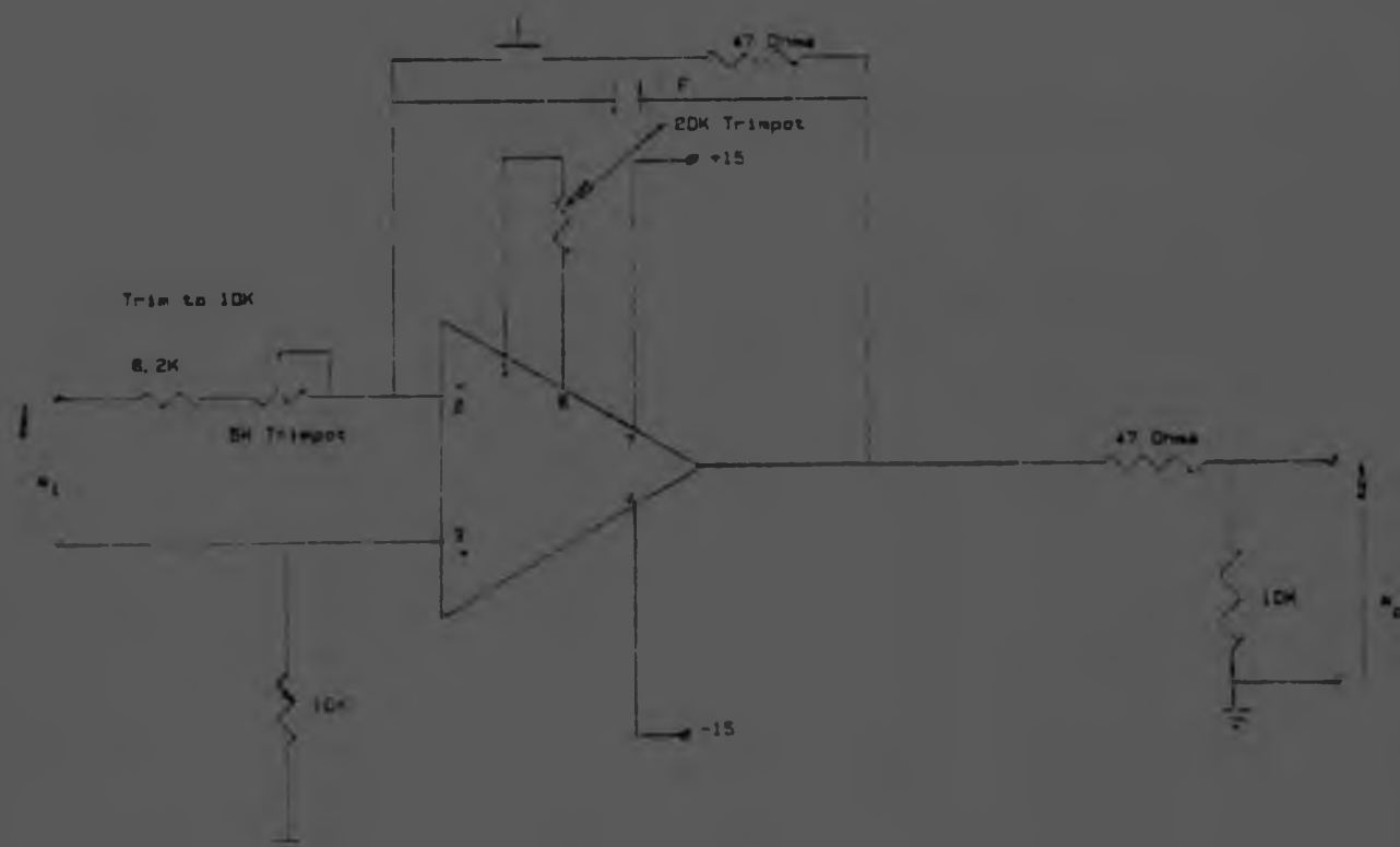
Figure B1 Diagram of the electronic integrating circuit used in the measurement of arc current and arc voltage.
