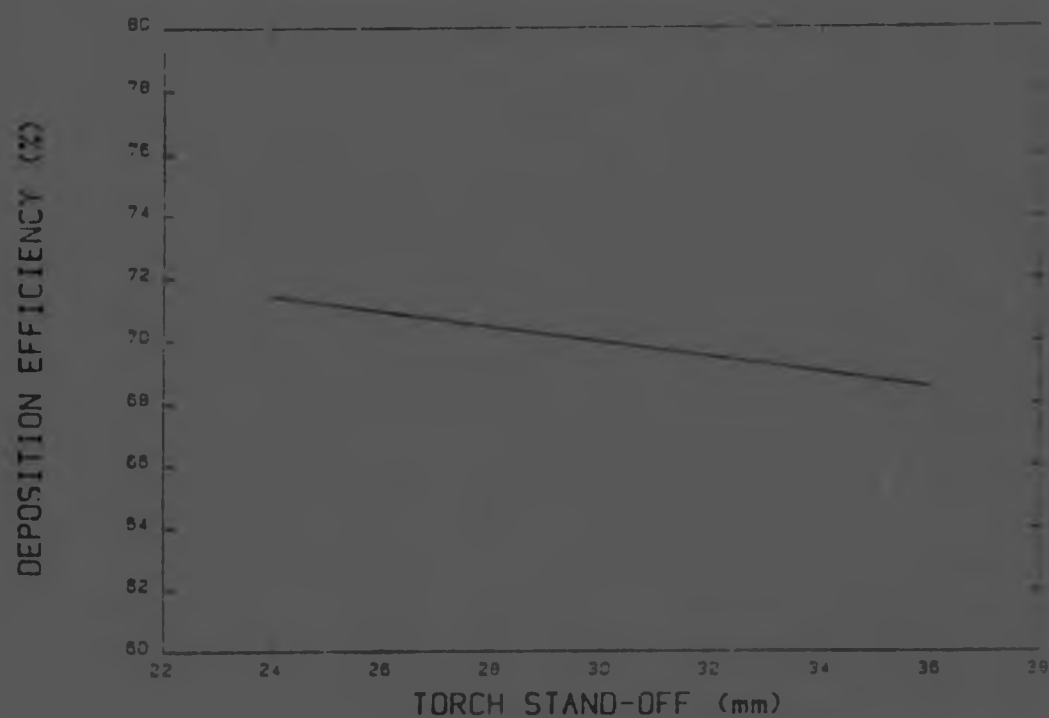
Figure 5.5 Graphical representation of deposition efficiency vs torch stand-off.
