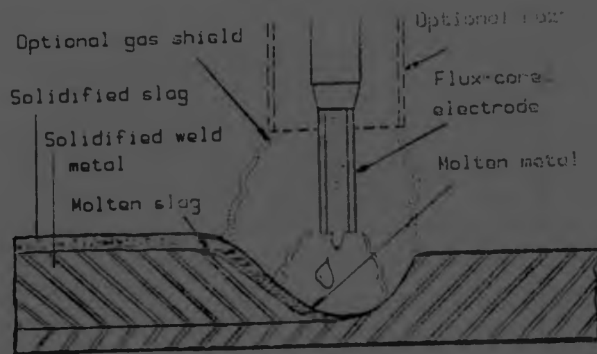
Figure 2.6 Schematic representation of the principles involved in flux-cored arc welding.
