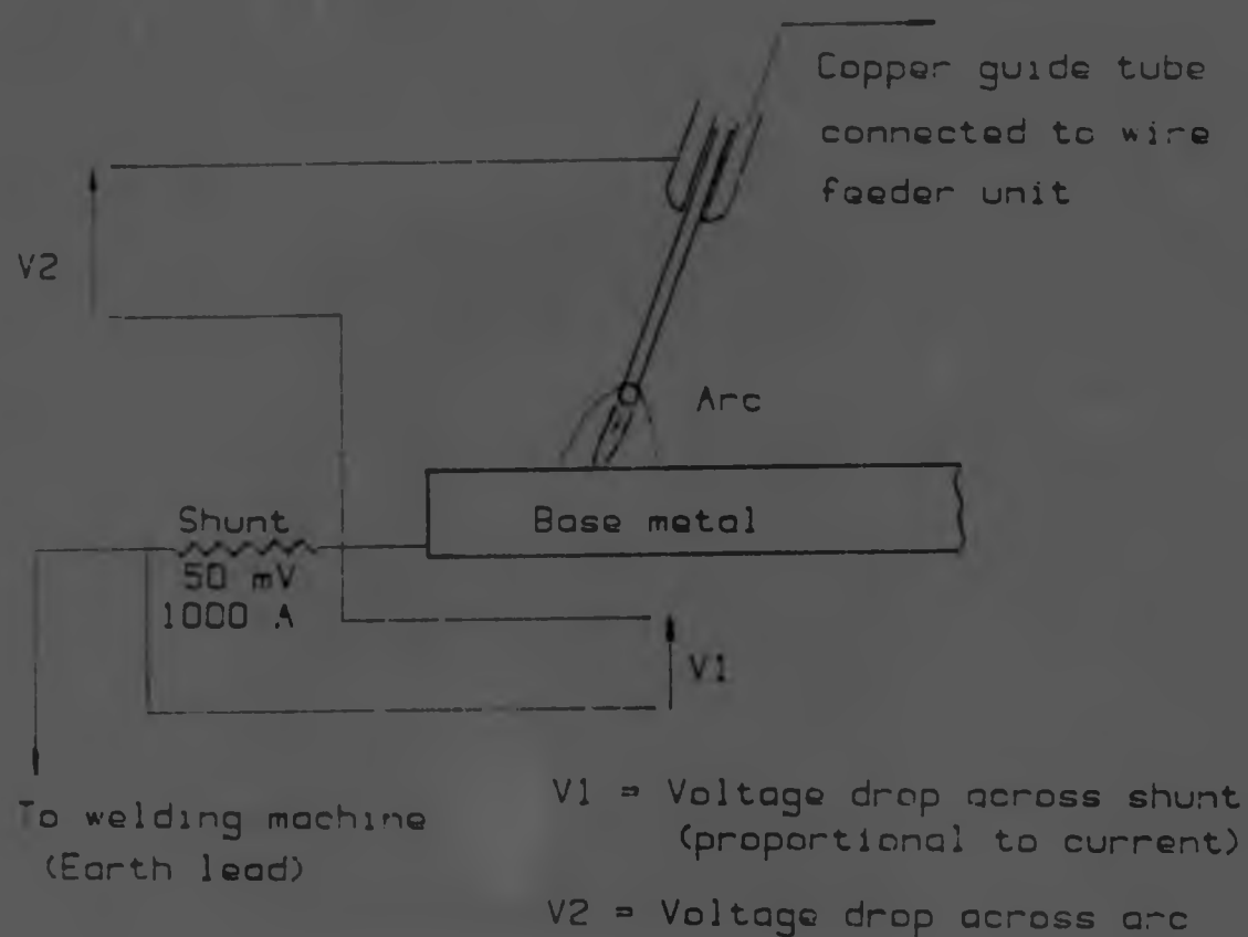
Figure 3.2 Schematic representation of the system used for the measurement of arc current and voltage.
