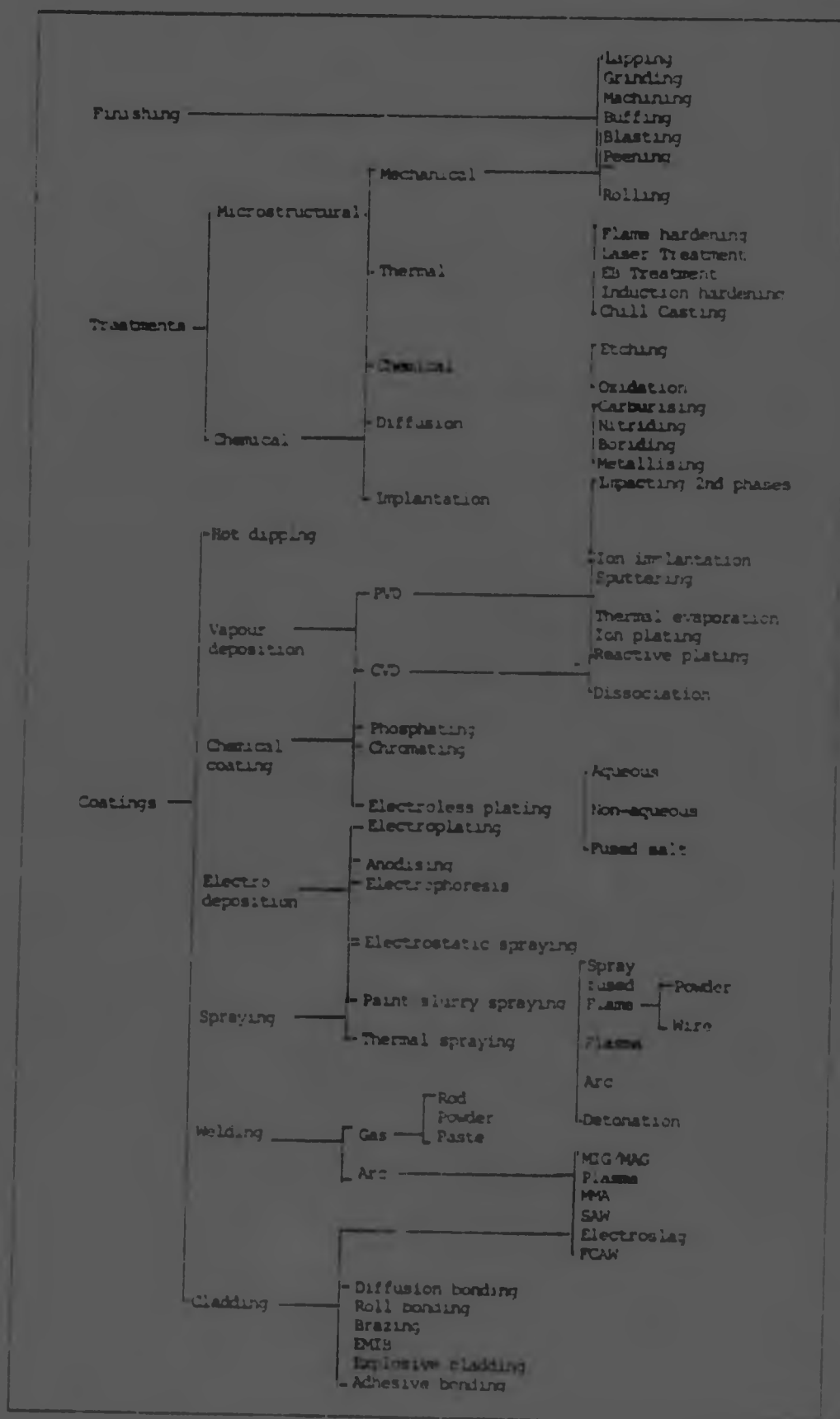
Figure 2.3 Classification of surface modification processes available in industry today.
