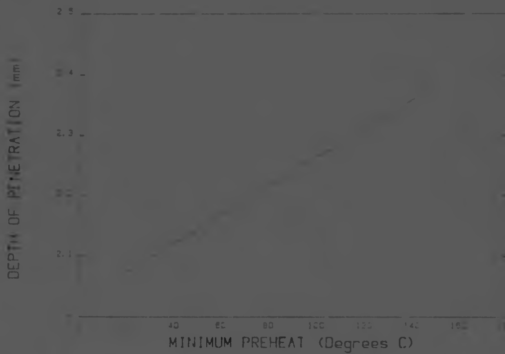
Figure 5.14 Graphical representation of depth of penetration vs. minimum preheat.
