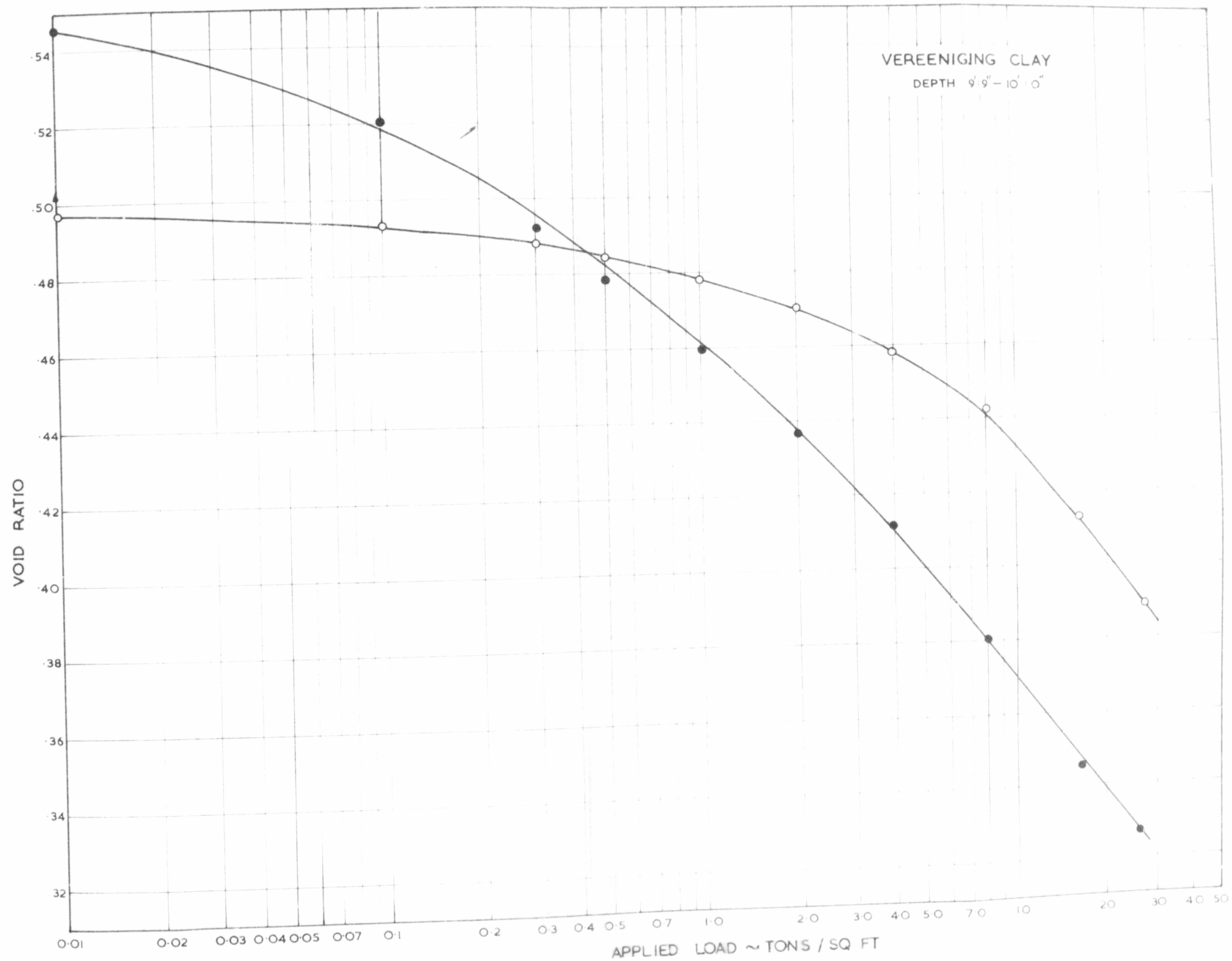
TYPICAL DOUBLE OEDOMETER CURVES FOR VEREENIGING EXPANSIVE CLAY
