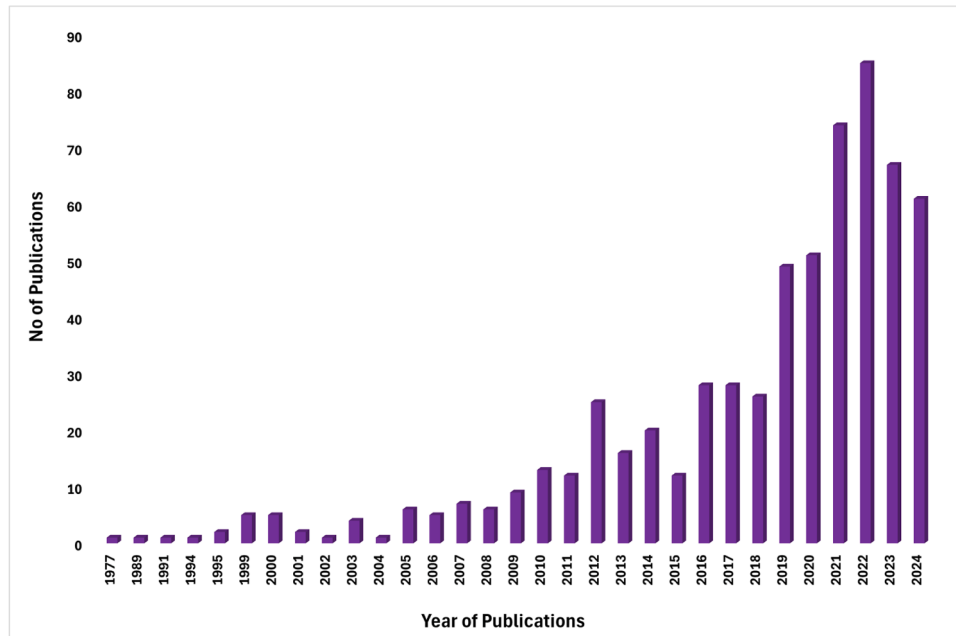
Fig. 2. Publication trend.
