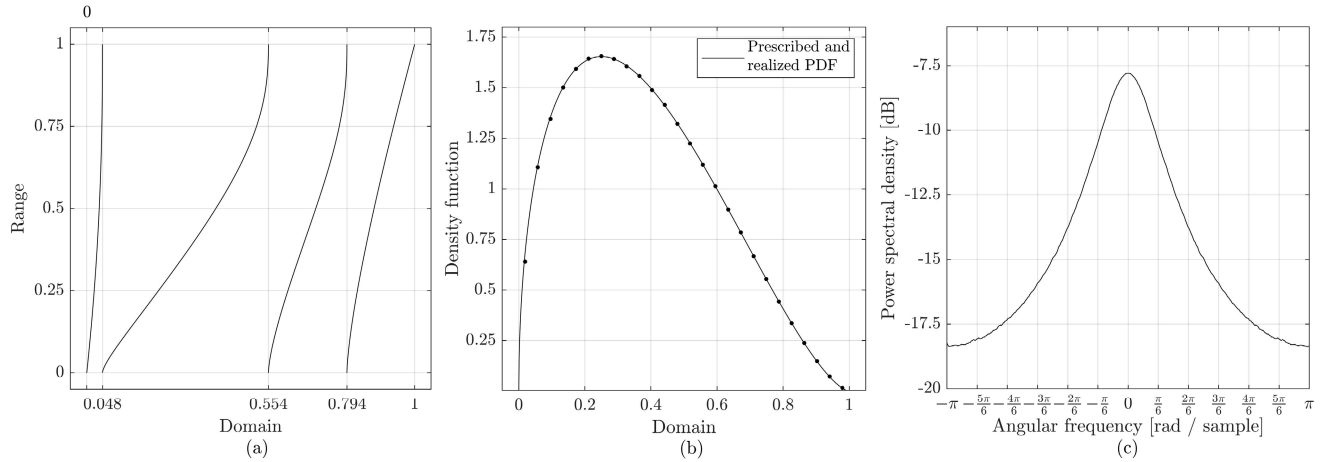
FIGURE 12. Plots associated with the system designed using the topological conjugation method of [12]. These plots are (a) the map used by the system, (b) the prescribed and realized response PDF associated with the system, and (c) the PSD of the system response, computed numerically. In (b), dots represent values computed using numerical simulation to verify the results predicted by theory.
