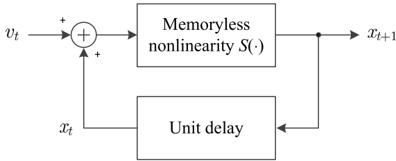
FIGURE 1. Diagram of a recursive, discrete-time and one-dimensional dynamical system configured to use the memoryless nonlinearity S as its evolution rule.
