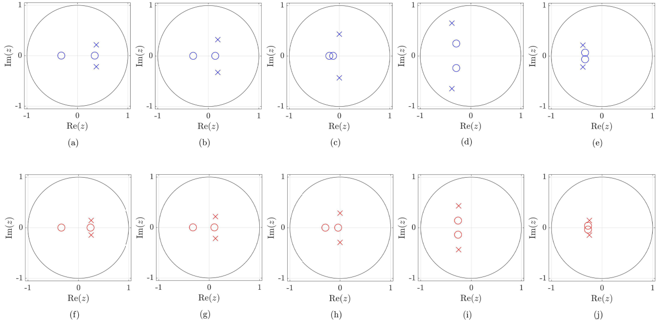
FIGURE 9. Pole-zero plots associated with the systems of the second set. In these plots, crosses represent poles and circles represent zeros. Plots (a) to (e) and plots (f) to (j) are associated with eigenvalues \lambda_2 denoted by the blue and red markers of Fig. 8(a), respectively. From left to right, the pole-zero plots of each row correspond to \arg(\lambda_2) = \pi/6, 2\pi/6, \dots, 5\pi/6 .
