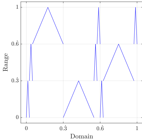
FIGURE 10. Plot of the hat map associated with the second set of systems that realizes an order-zero FPM with eigenvalue \lambda_2 = 0.75 \exp(i4\pi/6) .
