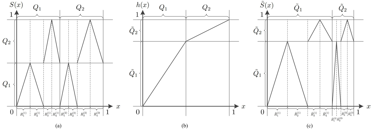
FIGURE 4. Plots of (a) a PWL hat map S , (b) a conjugating transform h , and (c) the corresponding topological conjugate \tilde{S} = h \circ S \circ h^{-1} of the map S .
