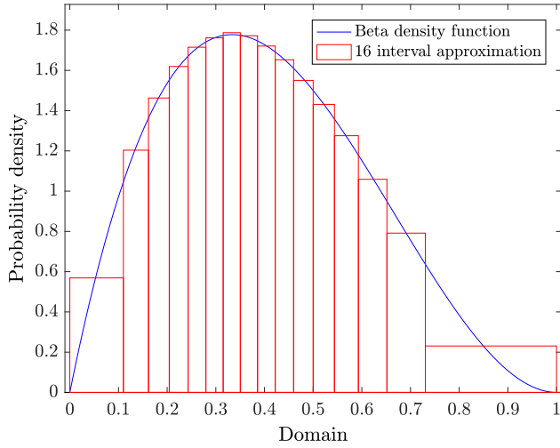
FIGURE 13. Prescribed zero-input response PDF (plotted in blue) and the response PDF realized with the first system of the example of section VI-C (plotted in red), for a Markov partition of 16 intervals [40].
