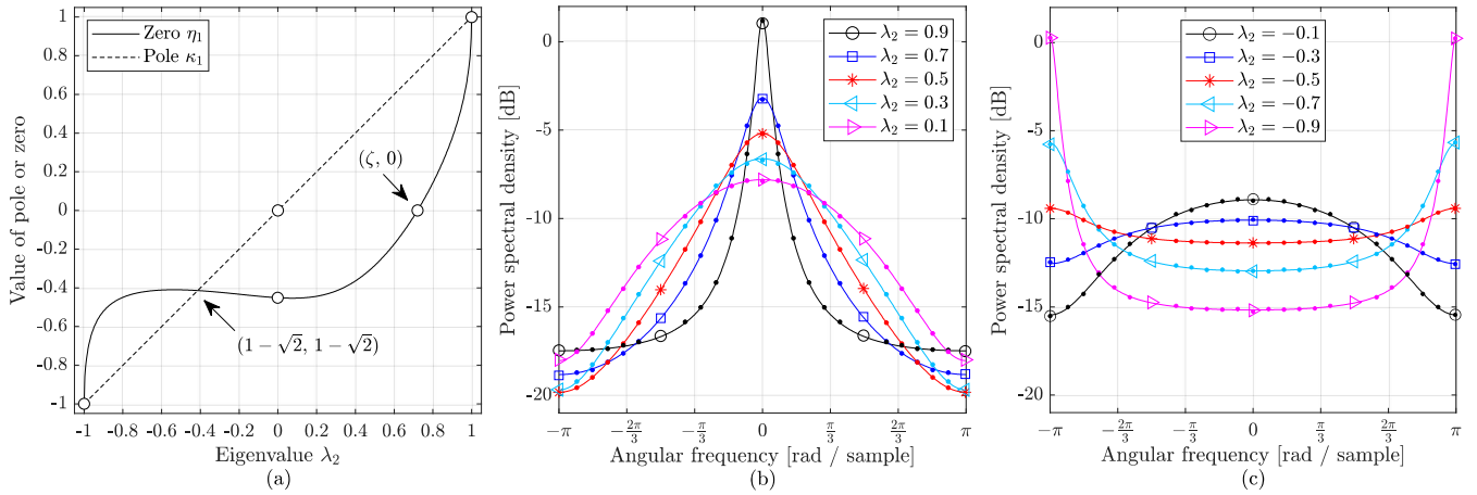
FIGURE 5. Plots of (a) the PSD pole and zero of the systems belonging to the first set, as a function of eigenvalue \lambda_2 , where circles represent excluded values, and (b) and (c) the PSDs of the systems from this set, for positive and negative eigenvalues \lambda_2 , respectively. In (b) and (c), solid lines represent values computed by evaluating the theoretical expressions and dots represent values computed using numerical simulation to verify the results predicted by theory.
