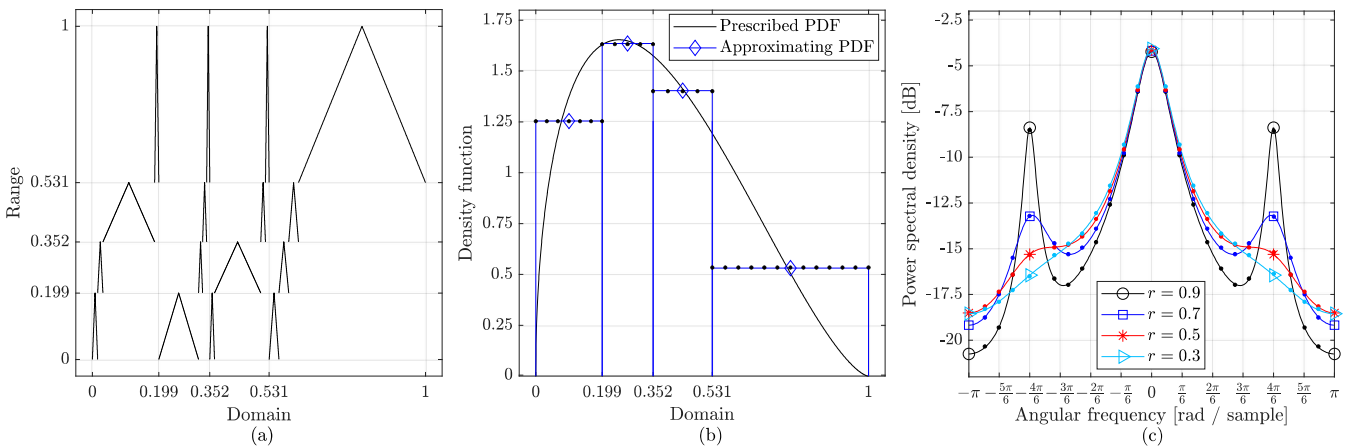
FIGURE 11. Plots associated with the examples of section VI-A. These plots are (a) the conjugate map \tilde{S} associated with r = 0.7 , (b) the prescribed response PDF (black) and the response PDF shared by all systems that use the conjugate maps \tilde{S} (blue), and (c) the PSDs of the systems that use the conjugate maps \tilde{S} . In (b) and (c), solid lines represent values computed by evaluating the theoretical expressions and dots represent values computed using numerical simulation to verify the results predicted by theory.
