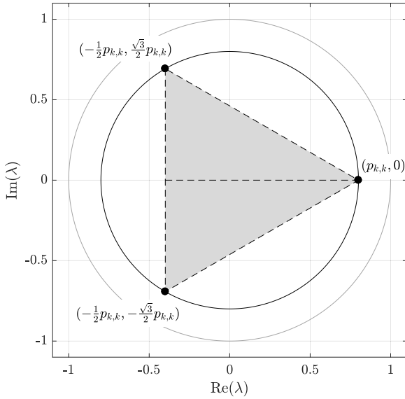
FIGURE 3. Complex plane with shaded region representing the permissible values for eigenvalue \lambda = re^{i\theta} when applying the novel disaggregation technique. The parameter p_{k,k} = 0.8 was used in the figure. Reproduced with permission from [43].
