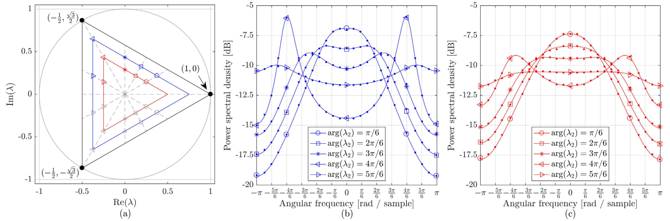
FIGURE 8. Plots of (a) the region of permissible eigenvalues \lambda_2 associated with the systems of the second set, where blue and red markers denote those eigenvalues selected, and (b) and (c) the PSDs of the systems from this set, for eigenvalues \lambda_2 denoted by the blue and red markers in (a), respectively. In (b) and (c), solid lines represent values computed by evaluating the theoretical expressions and dots represent values computed using numerical simulation to verify the results predicted by theory.
