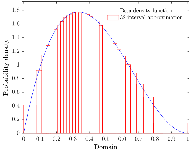
FIGURE 14. Prescribed zero-input response PDF (plotted in blue) and the response PDF realized with the second system of the example of section VI-C (plotted in red), for a Markov partition of 32 intervals [40].
