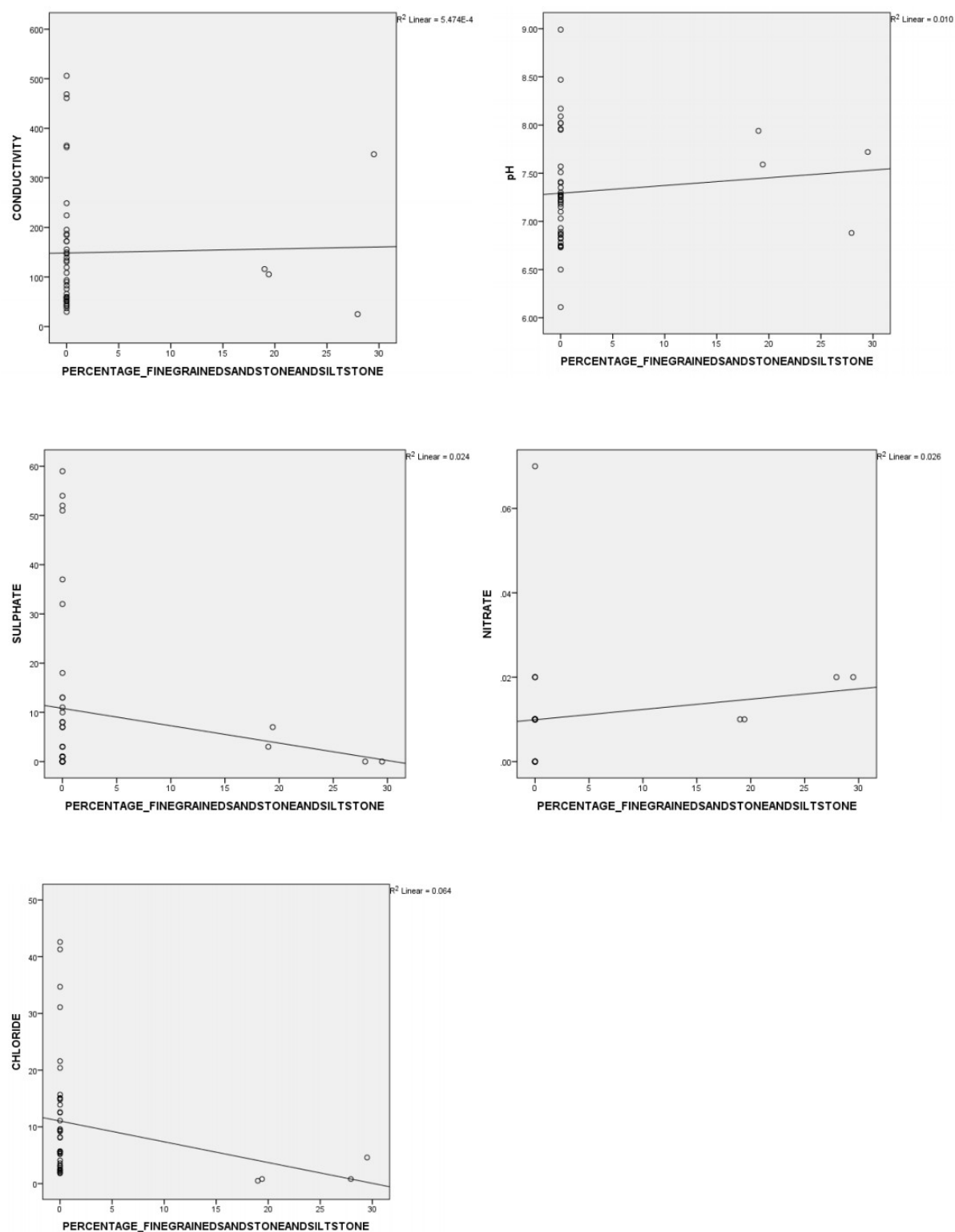
Figure 15 Scatterplots of fine grained sandstone geology with conductivity ( \mu S\ cm^{-1} ), pH, sulphate ( mg\ l^{-1} ), nitrate ( mg\ l^{-1} ) and chloride ( mg\ l^{-1} ).
