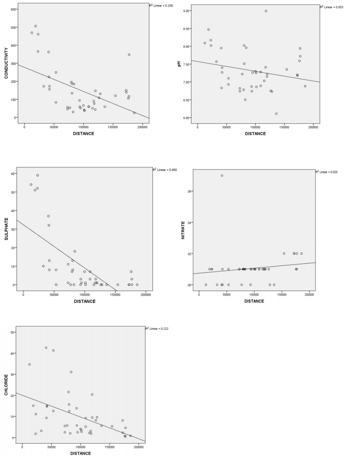
Figure 19 Scatterplots of linear distance (m) of study catchments from Majuba with conductivity ( \mu S cm^{-1} ), pH, sulphate ( mg l^{-1} ), nitrate ( mg l^{-1} ) and chloride ( mg l^{-1} ).
