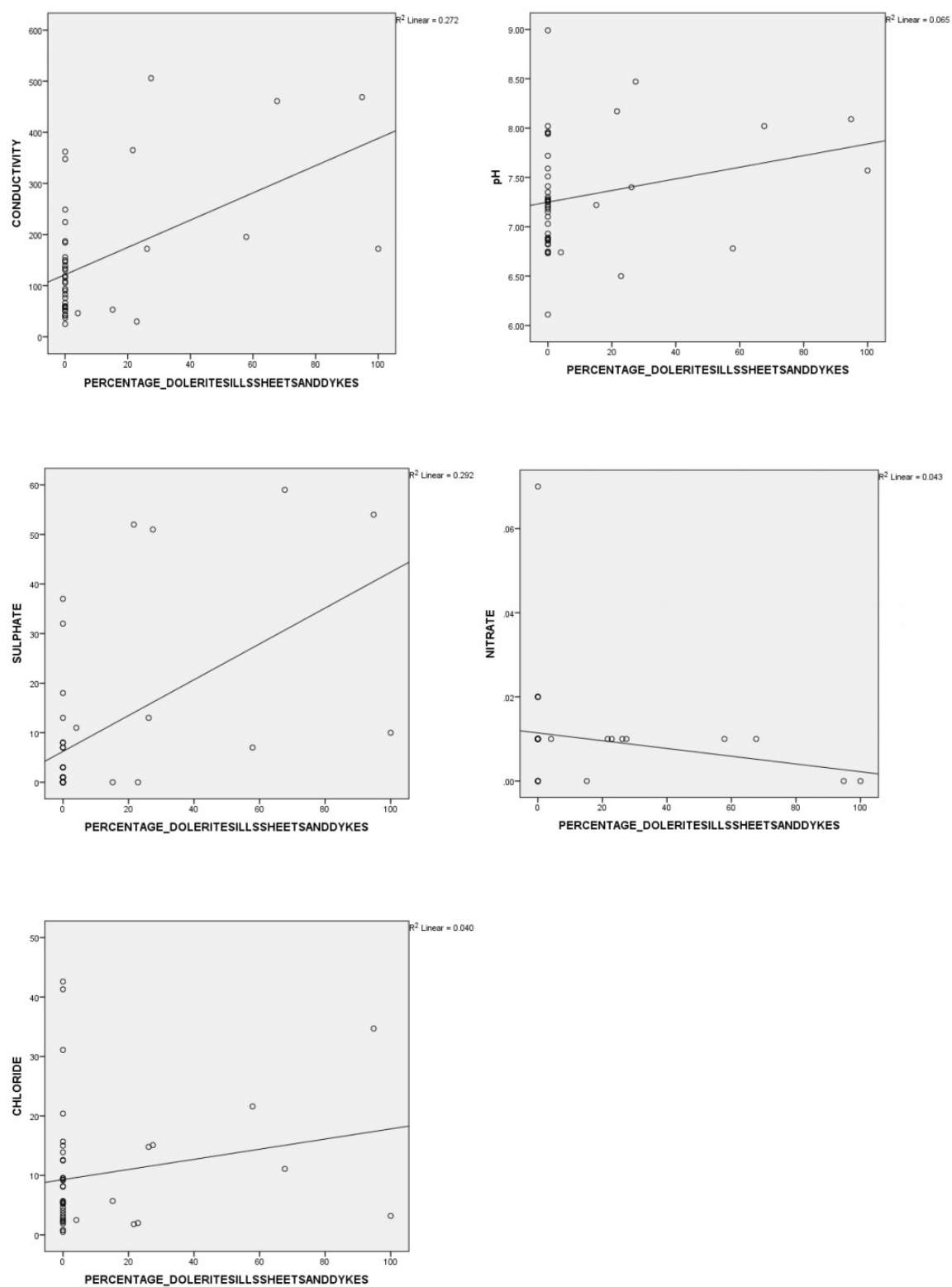
Figure 17 Scatterplots of dolerite geology with conductivity ( \mu\text{S cm}^{-1} ), pH, sulphate ( \text{mg l}^{-1} ), nitrate ( \text{mg l}^{-1} ) and chloride ( \text{mg l}^{-1} ).
