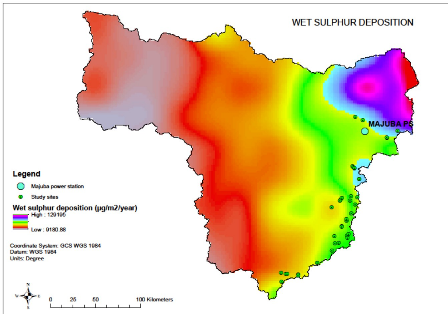
Figure 13 modelled annual wet sulphur deposition rates for 2014, with location of study sites.
