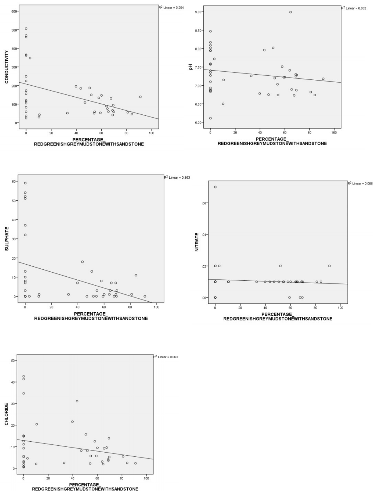
Figure 16 Scatterplots of red greenish grey mudstone with sandstone geology with conductivity ( \mu S cm^{-1} ), pH, sulphate ( mg l^{-1} ), nitrate ( mg l^{-1} ) and chloride ( mg l^{-1} ).
