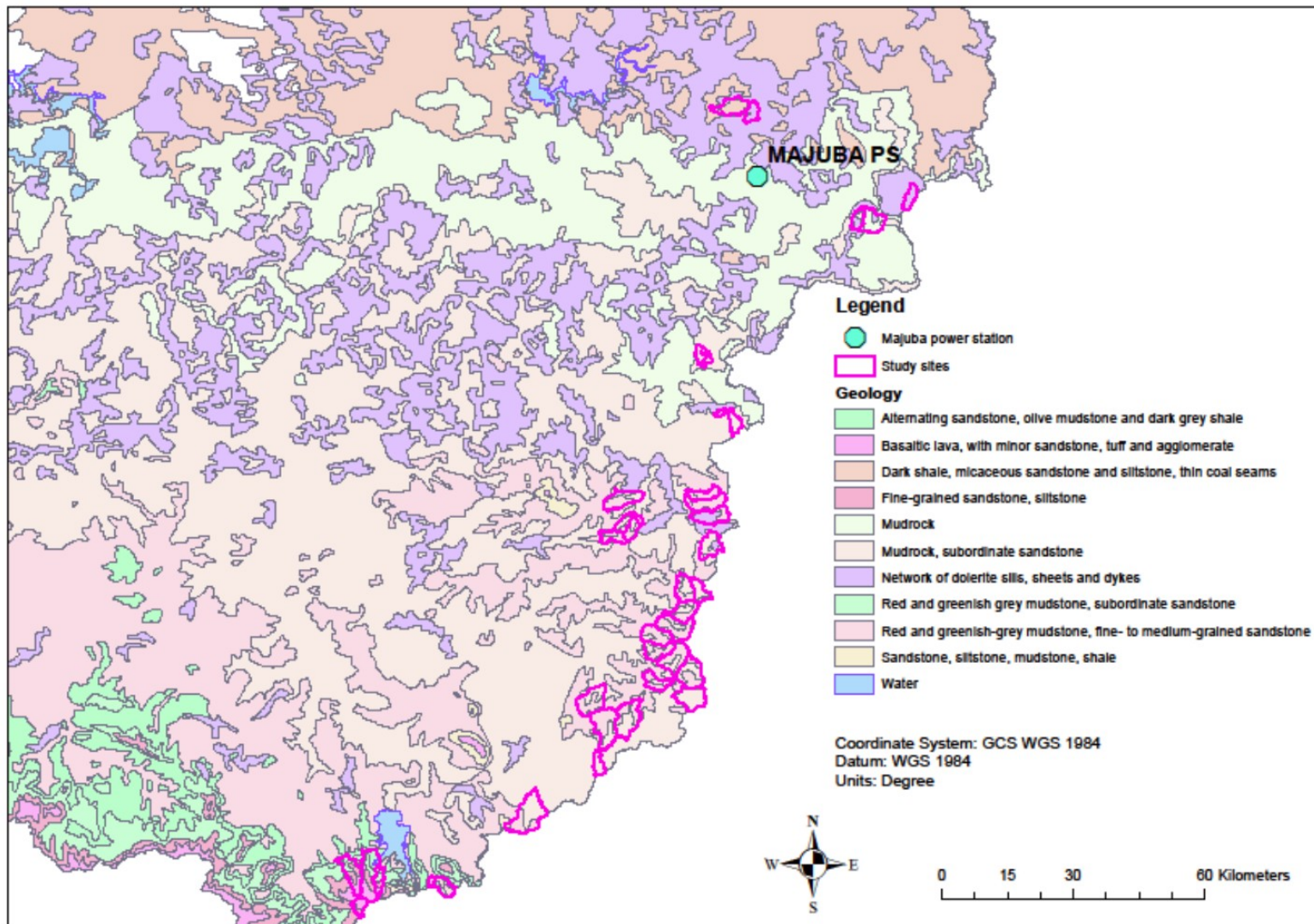
Figure 12 Distribution of various rock types in the 42 study catchments
