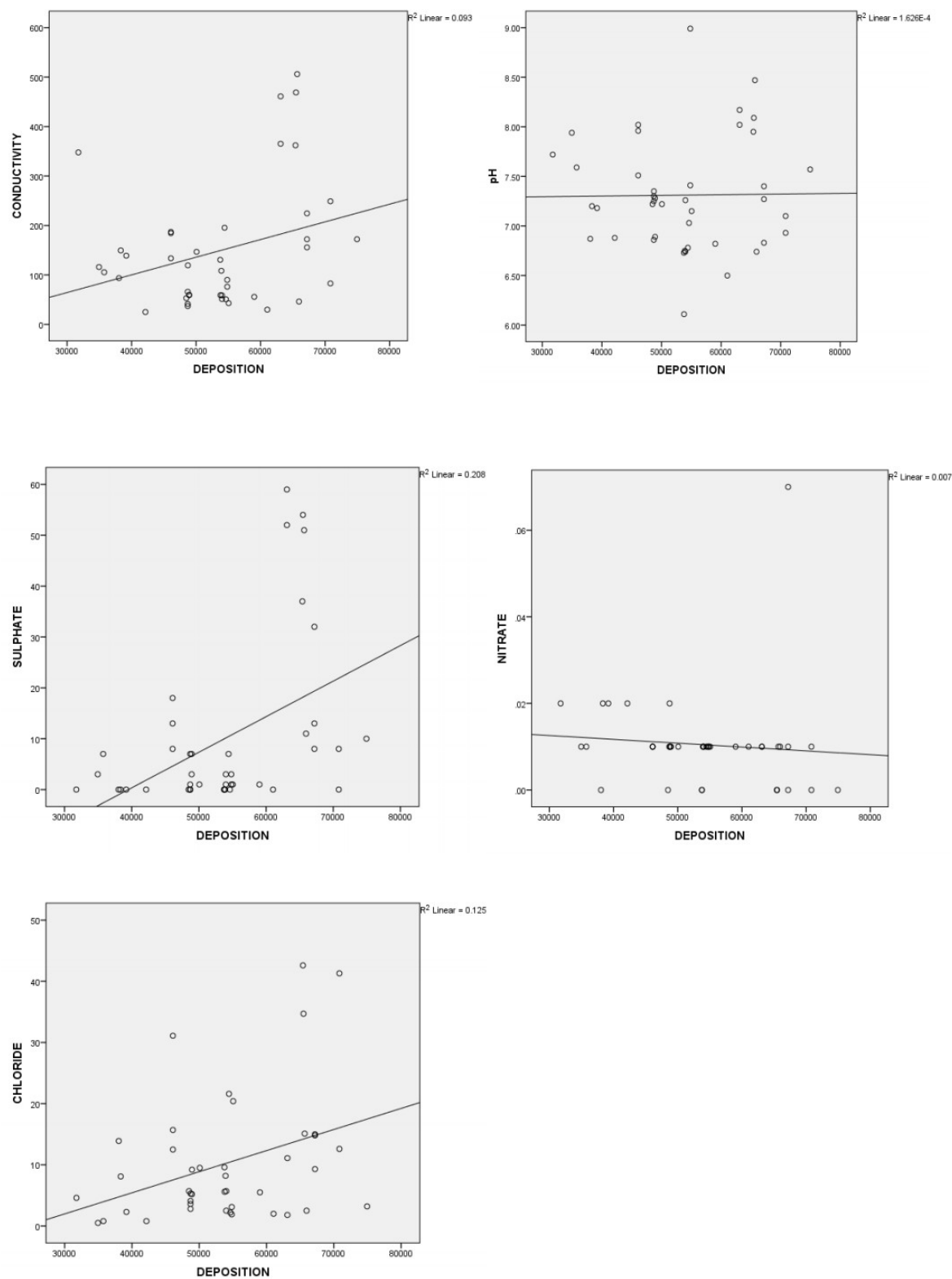
Figure 18 Scatterplots of modelled wet sulphur deposition rates ( \mu\text{g m}^{-2} \text{ year}^{-1} ) with conductivity ( \mu\text{S cm}^{-1} ), pH, sulphate ( \text{mg l}^{-1} ), nitrate ( \text{mg l}^{-1} ) and chloride ( \text{mg l}^{-1} ).
