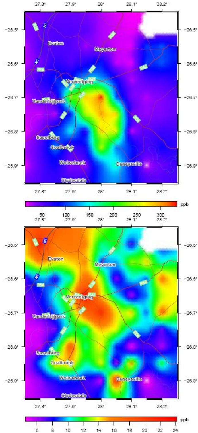
Figure 2.4: The spatial distribution of \text{SO}_2 over the Vaal Triangle area and surrounding towns as measured by the aircraft. The top figure shows the maximum values and the bottom figure the median values gridded on a 0.05 by 0.05 degree resolution (Piketh et al. , 2006).
