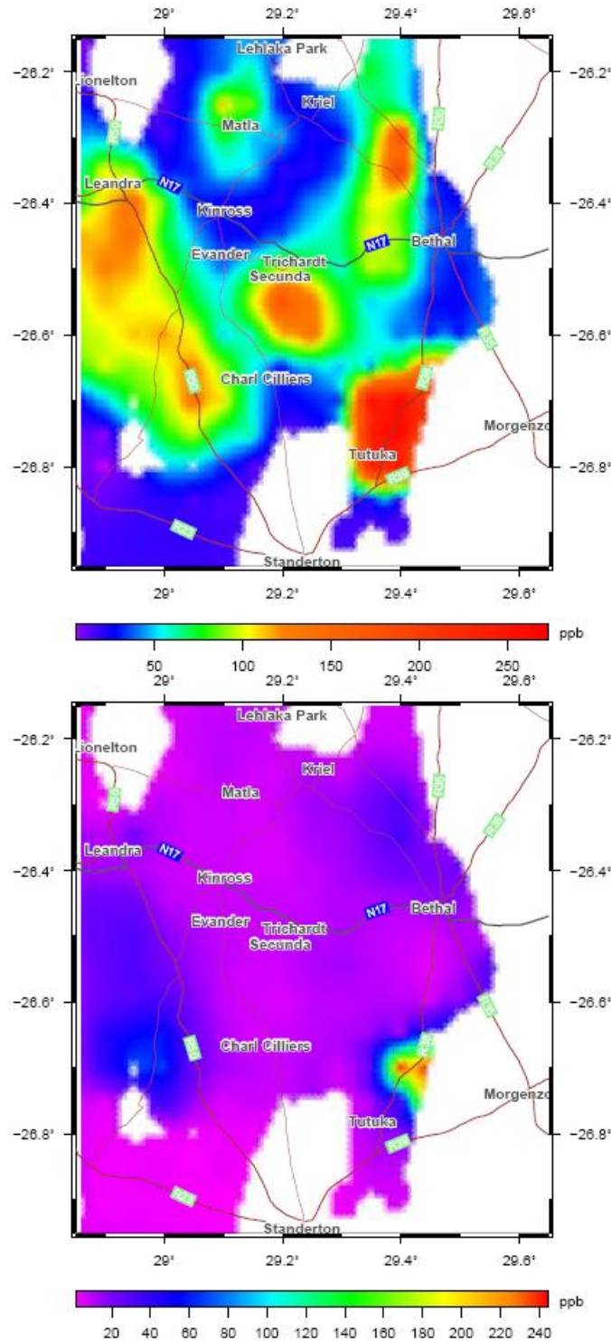
Figure 2.2: The spatial distribution of \text{SO}_2 over Secunda and surrounding towns as measured by the aircraft. The top figure shows the maximum values and the bottom figure the median values gridded on a 0.05 by 0.05 degree resolution (Piketh et al. , 2006).
