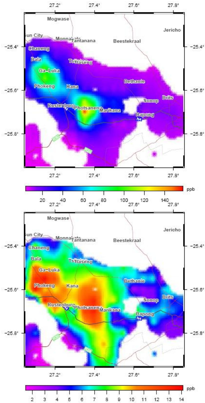
Figure 2.3: The spatial distribution of \text{SO}_2 over Rustenburg and surrounding towns as measured by the aircraft. The top figure shows the maximum values and the bottom figure the median values gridded on a 0.05 by 0.05 degree resolution (Piketh et al. , 2006).
