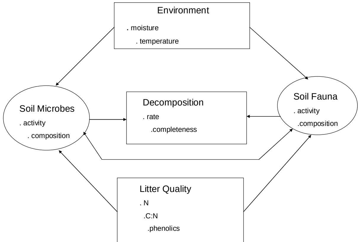
Figure 2.1 Factors that control the rate and completeness of decomposition. Source: Prescott et al. (2000).
