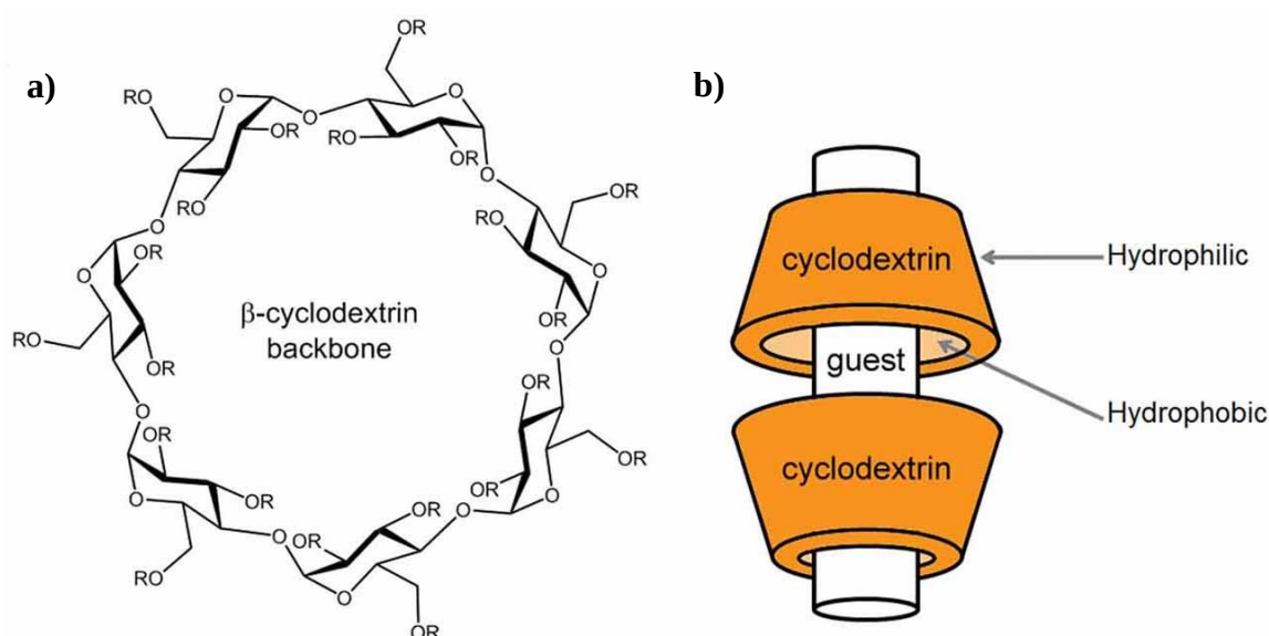
Figure 4: Basic structure of a \beta -cyclodextrin and formation of a complex with a guest compound. (a) The chemical structure of a \beta -cyclodextrin backbone with chemical substitution groups depicted as R, which are replaced with different chemical groups during the modification process (b) Illustration of the interaction between cyclodextrins and guest compounds modelled from the interaction between hydroxypropyl-beta-cyclodextrin (HP \beta CD) and cholesterol. One cholesterol molecule is encapsulated in the hydrophobic interior of a cyclodextrin dimer, and the hydrophilic exterior allows for solubilisation. [Source: Crumline et al. , 2017, accessed 20 February 2023].
