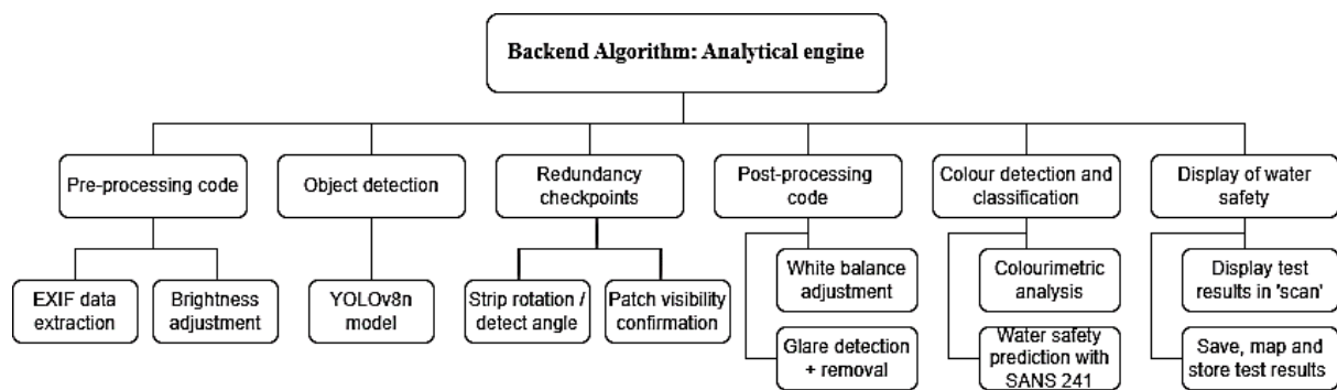
Fig. 3.3 Overview of software architectural hierarchy
