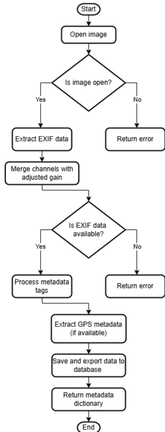
Fig. 3.4 EXIF data flowchart
