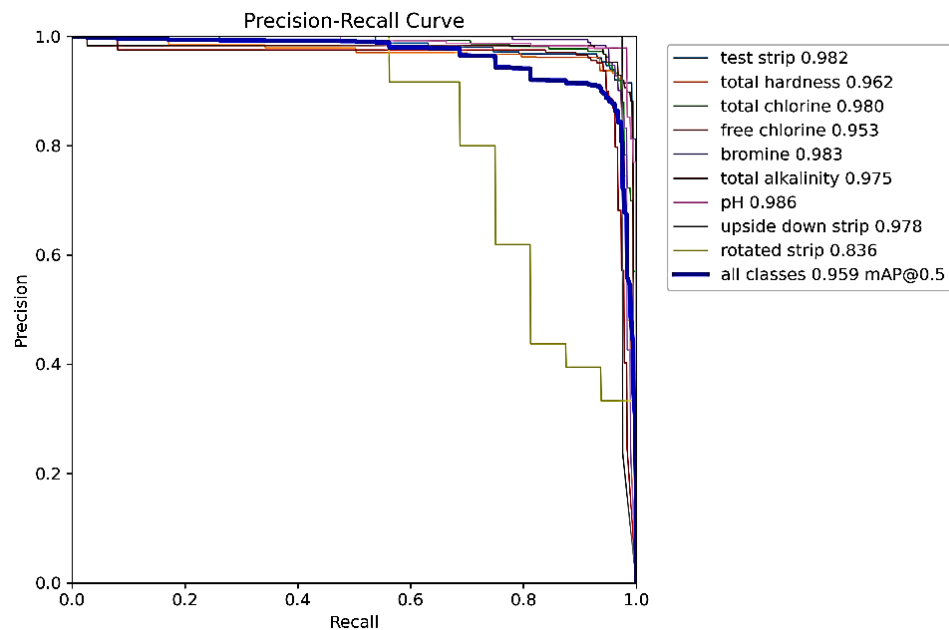
Fig. 4.6 Precision-recall curve for custom-trained YOLOv8n model
