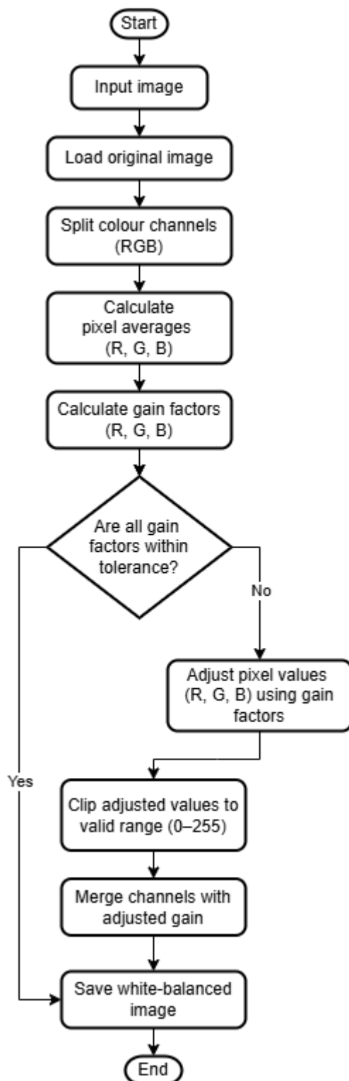
Fig. 3.8 White balance code flowchart
