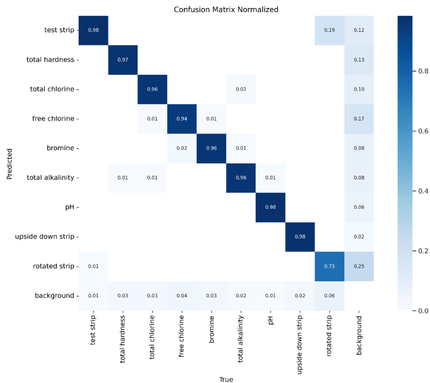
Fig. 4.5 Confusion matrix for custom-trained YOLOv8 nano model
