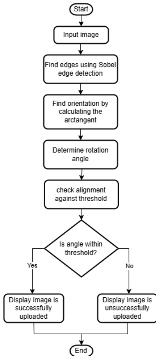
Fig. 3.6 Rotation angle detection code flowchart
