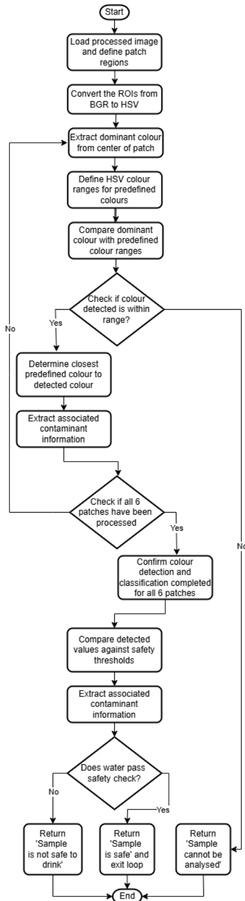
Fig. 3.10 Flowchart of the colour classification code segment
