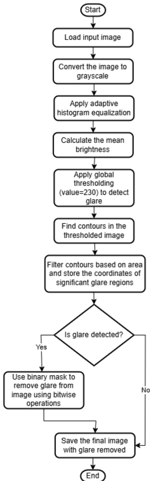
Fig. 3.9. Glare detection and removal code flowchart
