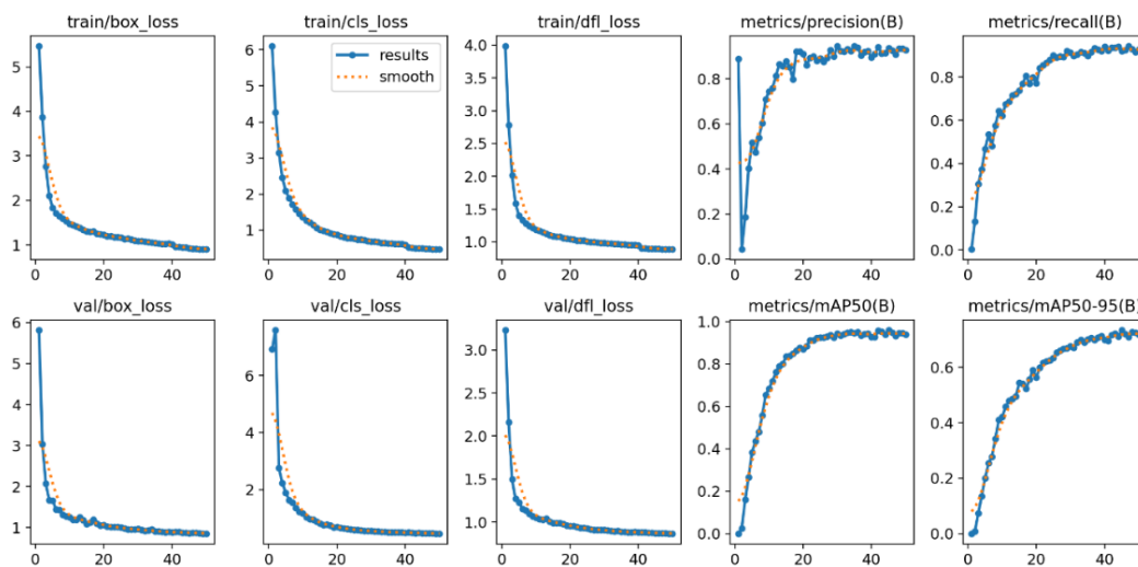
Fig. 4.4 Training and validation metrics and losses over 50 epochs
