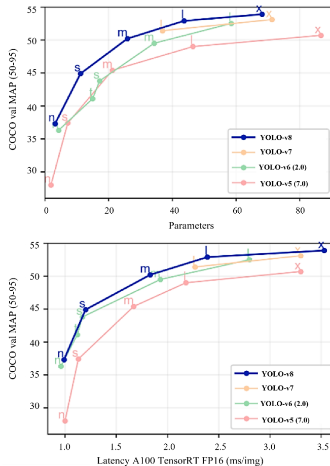
Fig. 2.4 Graph of YOLOv8 compared with predecessors [115]
