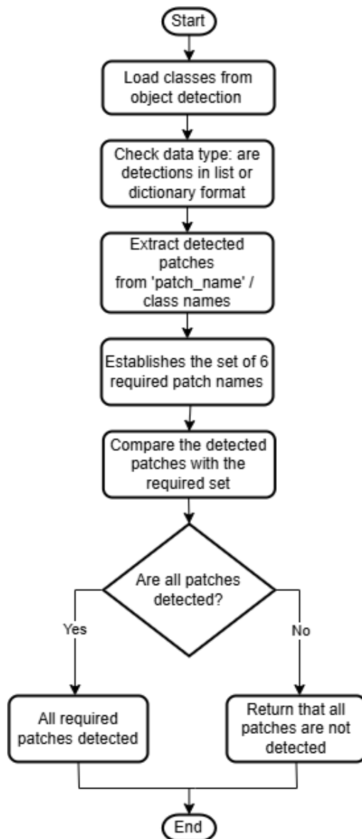
Fig. 3.7 Patch visibility code flowchart
