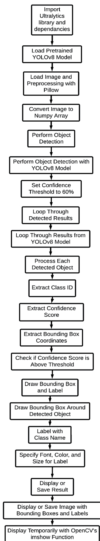
Fig. 3.5 YOLO model framework and implementation
