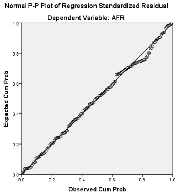
Figure 12. AFR Model 2: Normal P-Plot of Regression
