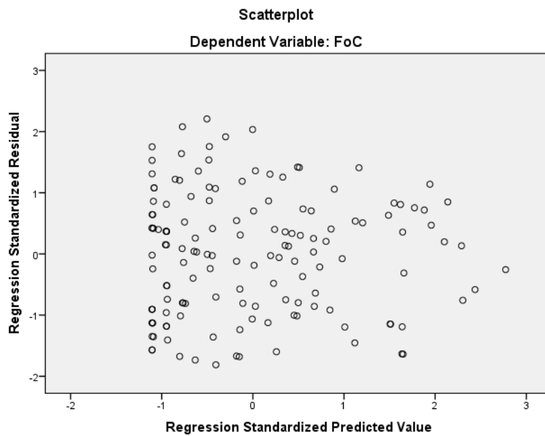
Figure 7. FoC Model 1: Scatterplot of the Standardized Residuals and Standardized Predicated Values
