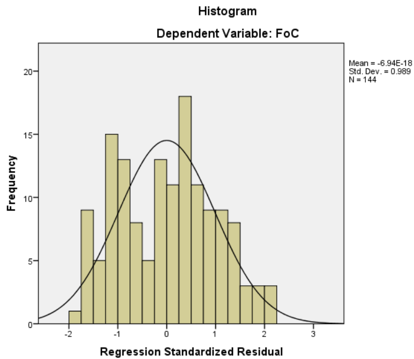
Figure 5. FoC Model 2: Histogram
