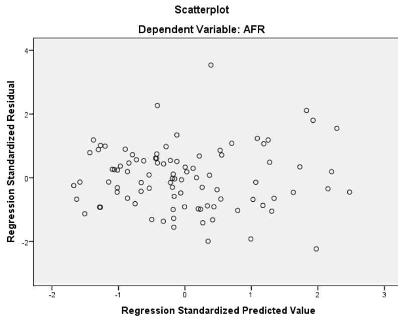
Figure 10. AFR Model 1: Scatterplot of the Standardized Residuals and Standardized Predicated Values
