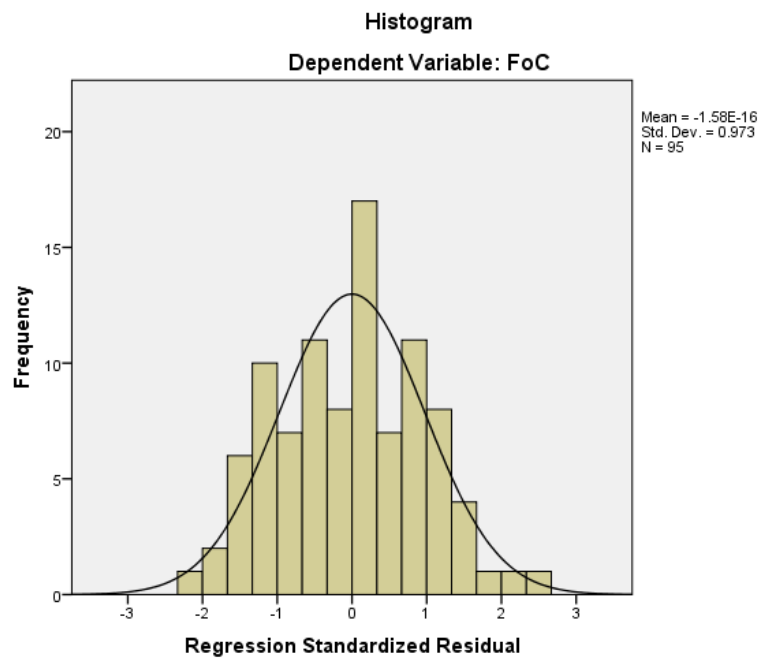
Figure 2. FoC Model 1: Histogram
