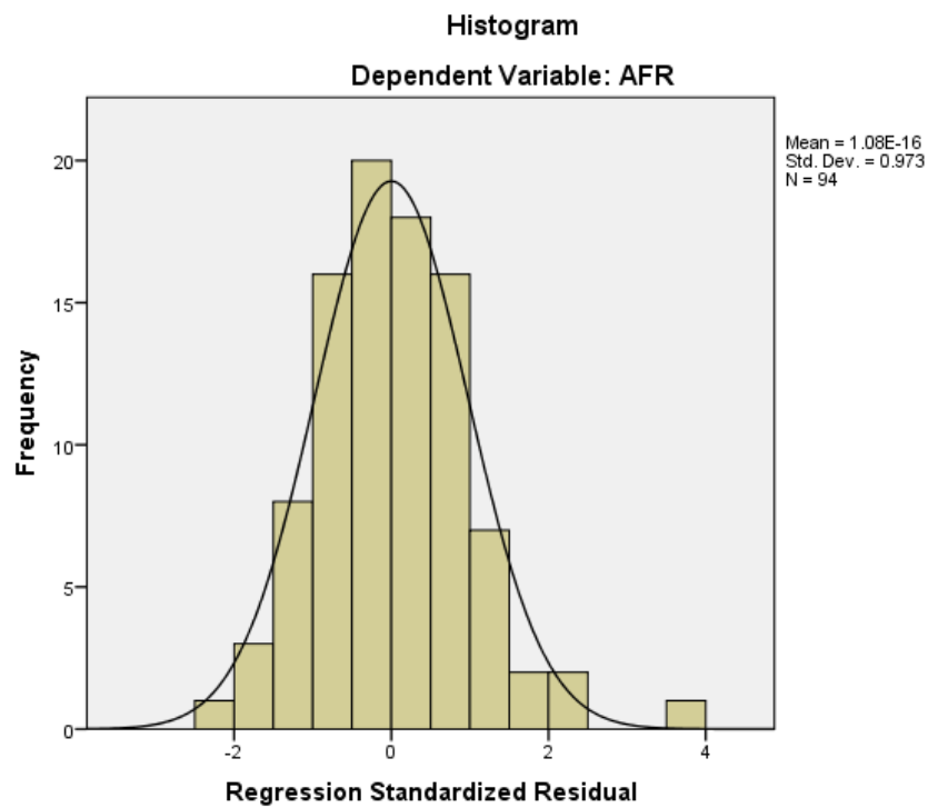
Figure 8. AFR Model 1: Histogram
