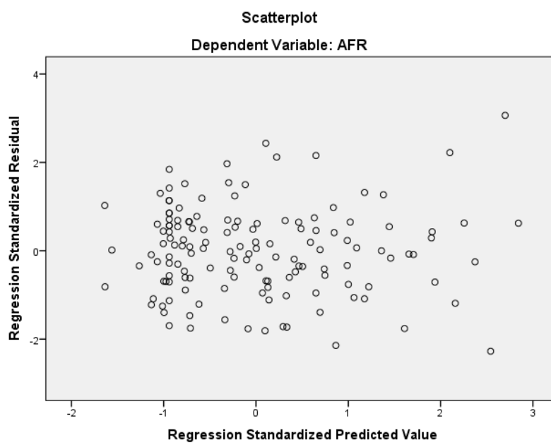
Figure 13. AFR Model 2: Scatterplot of the Standardized Residuals and Standardized Predicated Values
