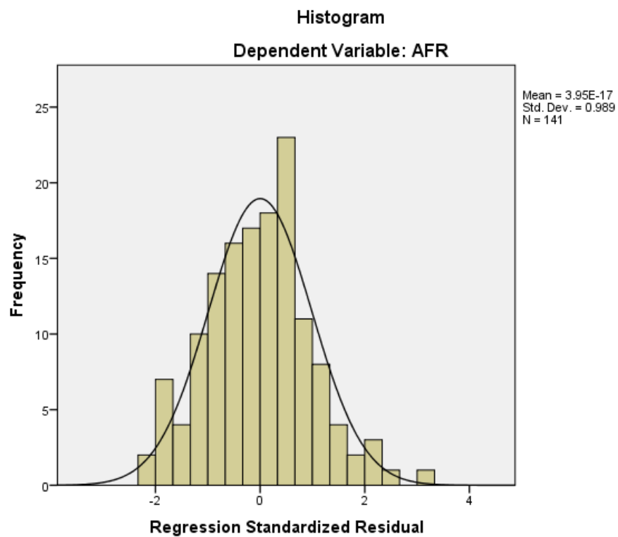
Figure 11. AFR Model 2: Histogram
