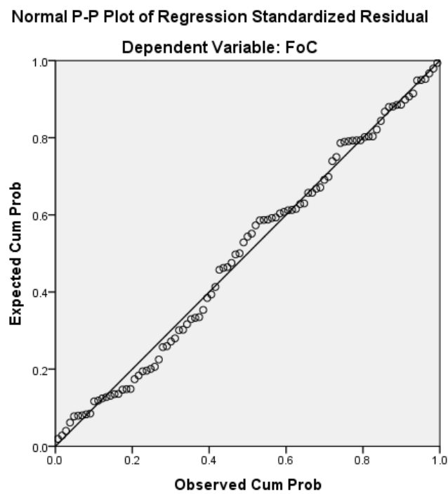
Figure 3. FoC Model 1: Normal P-Plot of Regression
