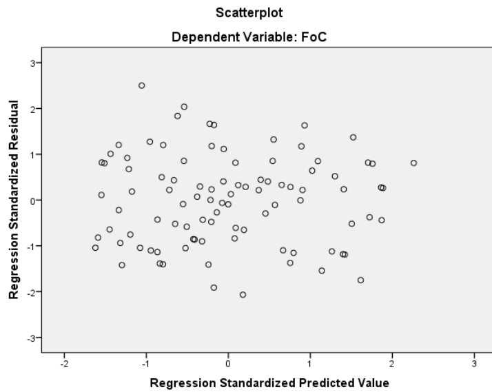
Figure 4. FoC Model 1: Scatterplot of the Standardized Residuals and Standardized Predicated Values
