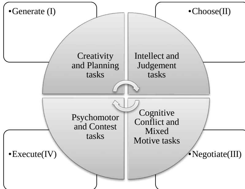
Figure 6. McGrath group task circumplex
