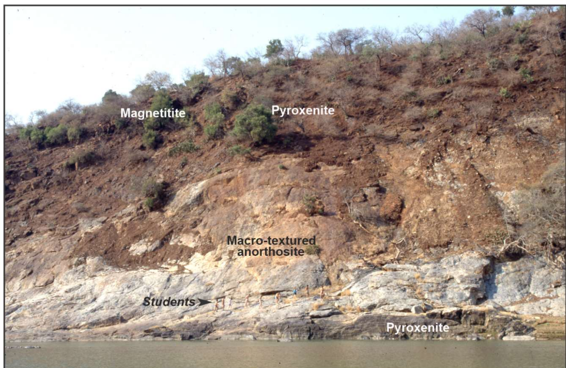
Anorthosite and magnetitite layers where the Tugela River cuts through the Mambula Complex
