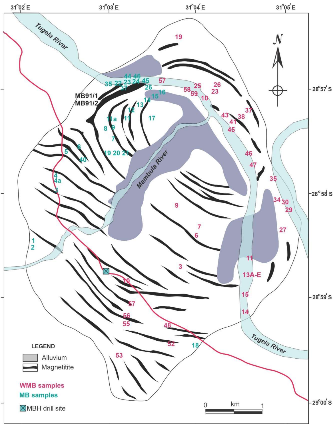
Sample sites in the Mambula Complex
