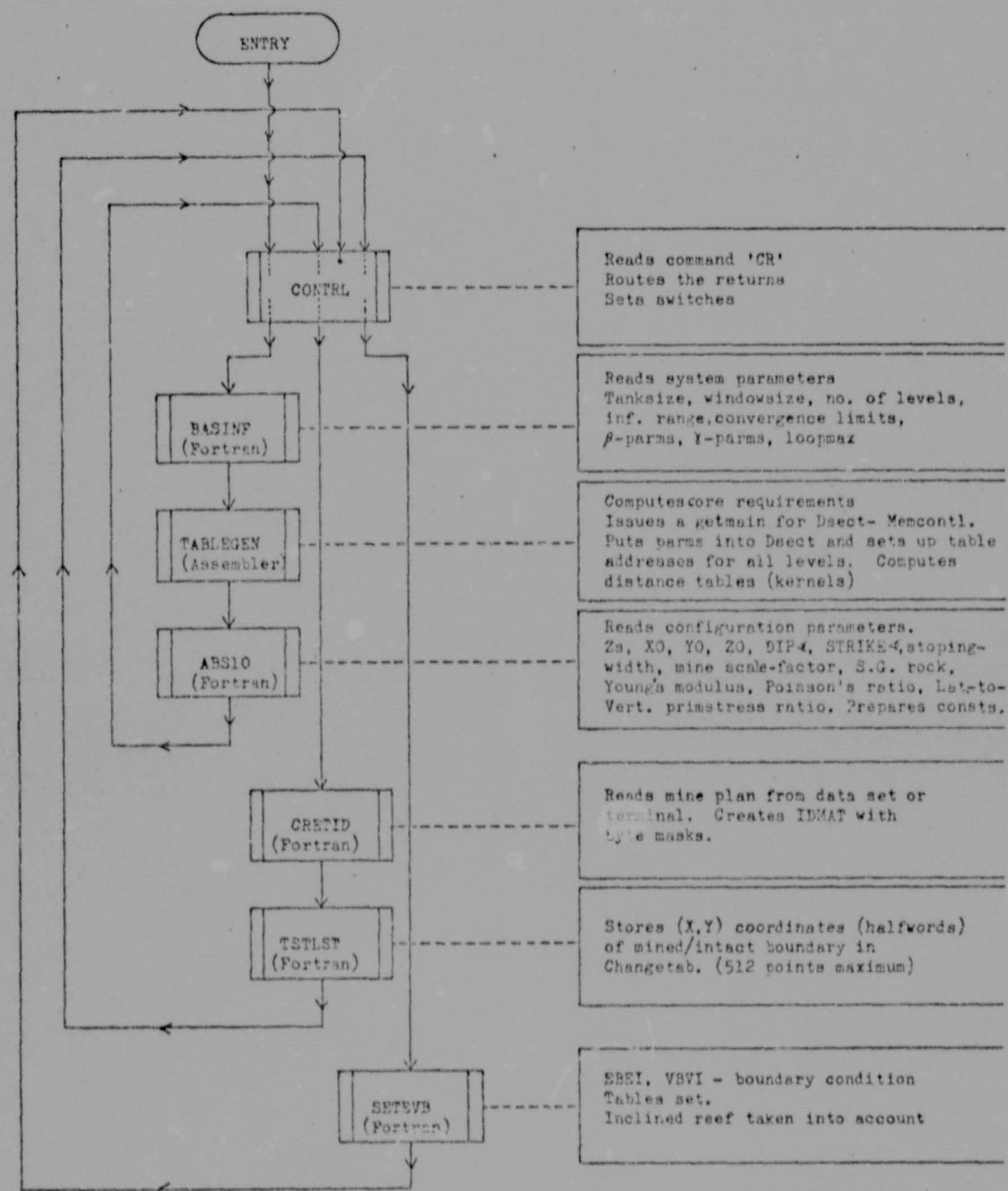
Figure 5.2 Flowchart of Create-Mode Routines
