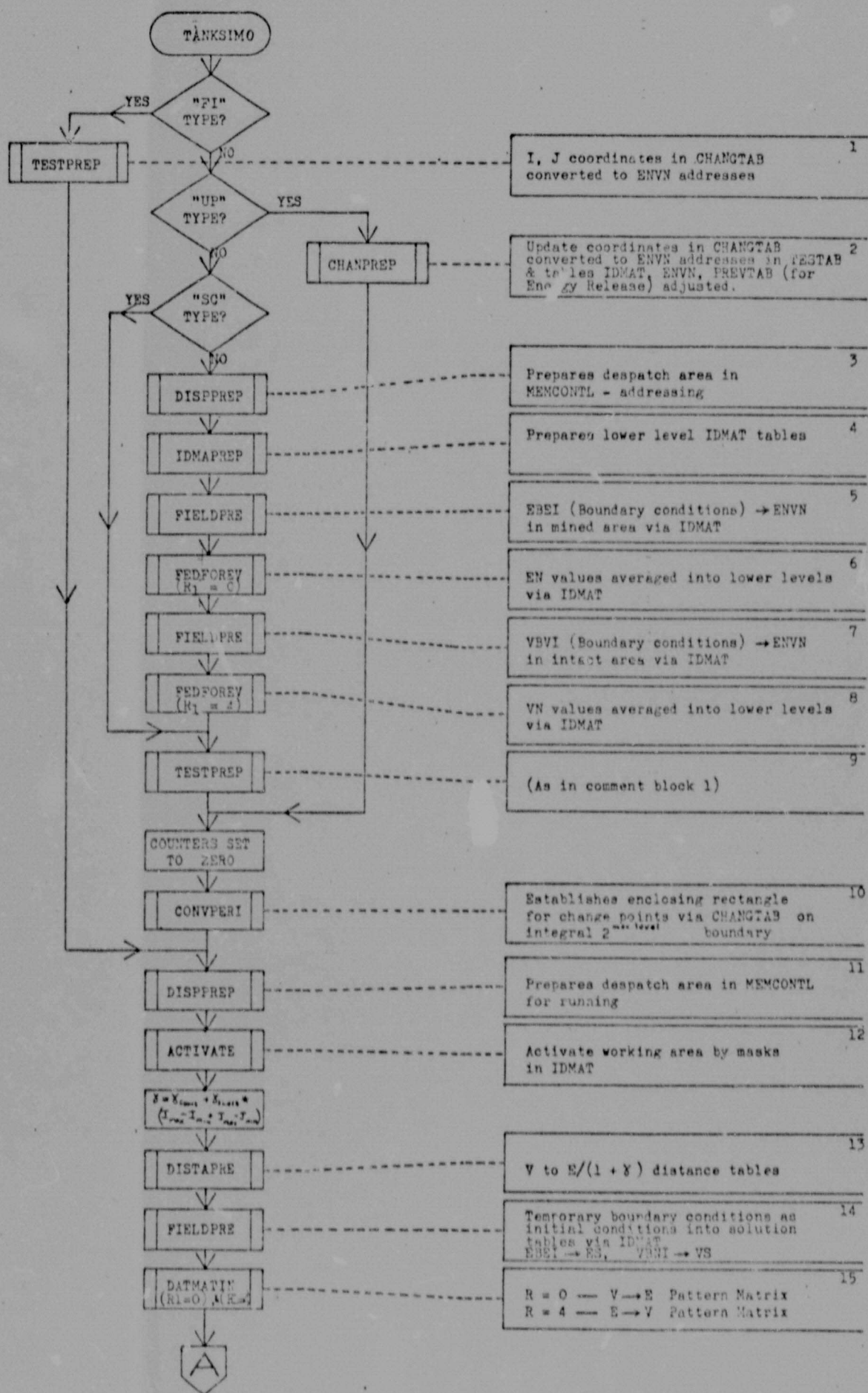
Figure 5.6 Flow Chart of TANKSIMO
