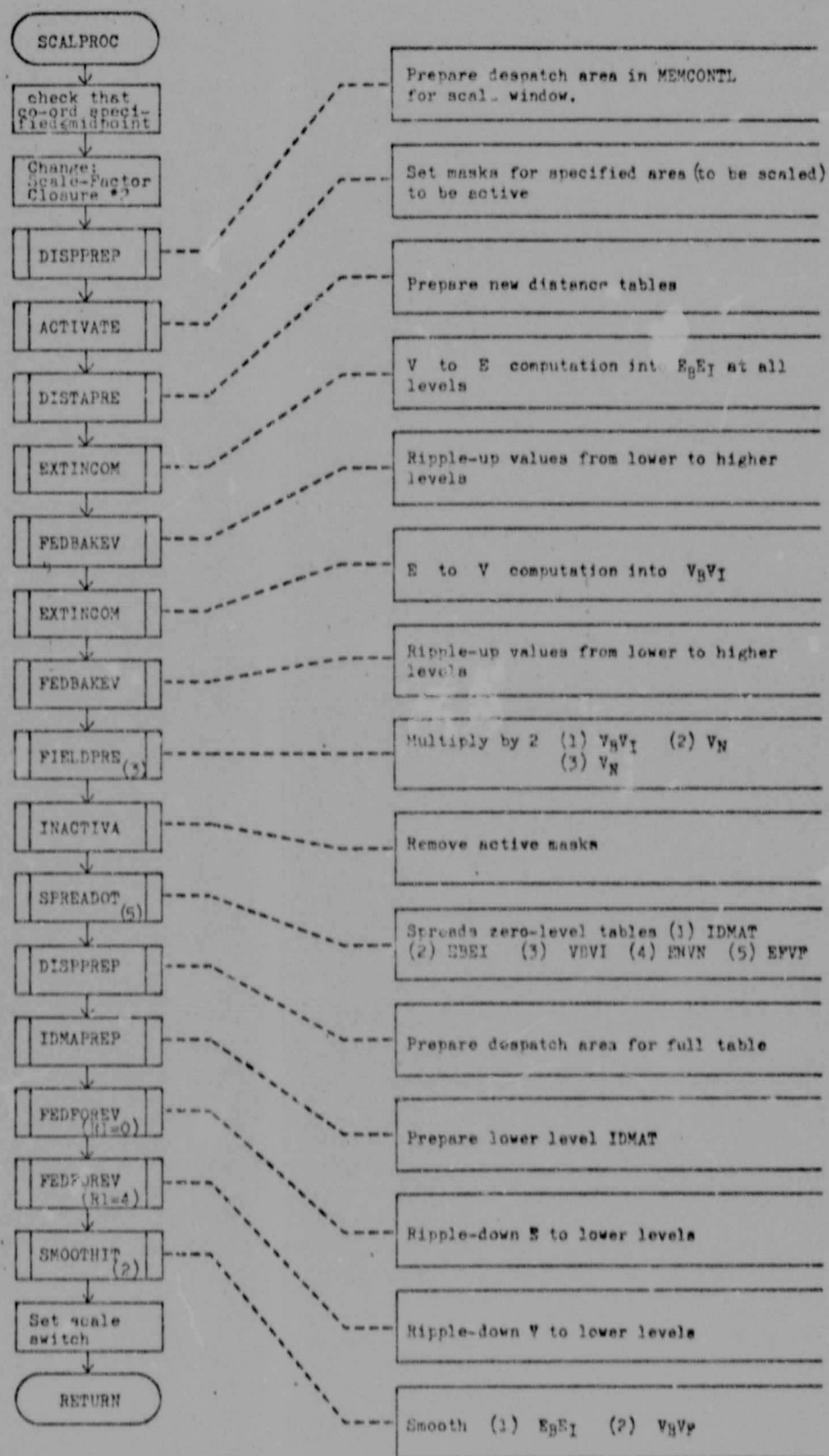
Figure 5.5 Flow Chart of SCALPROC
