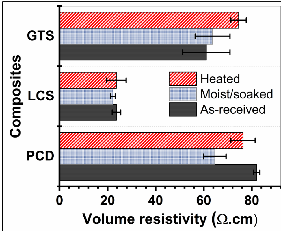
Figure 6-10 Measured volume electrical resistivity of the composites (GTS – Greenside tailing slurry; LCS – Likeflow coal slurry; PCD – Proteas coal discard)
