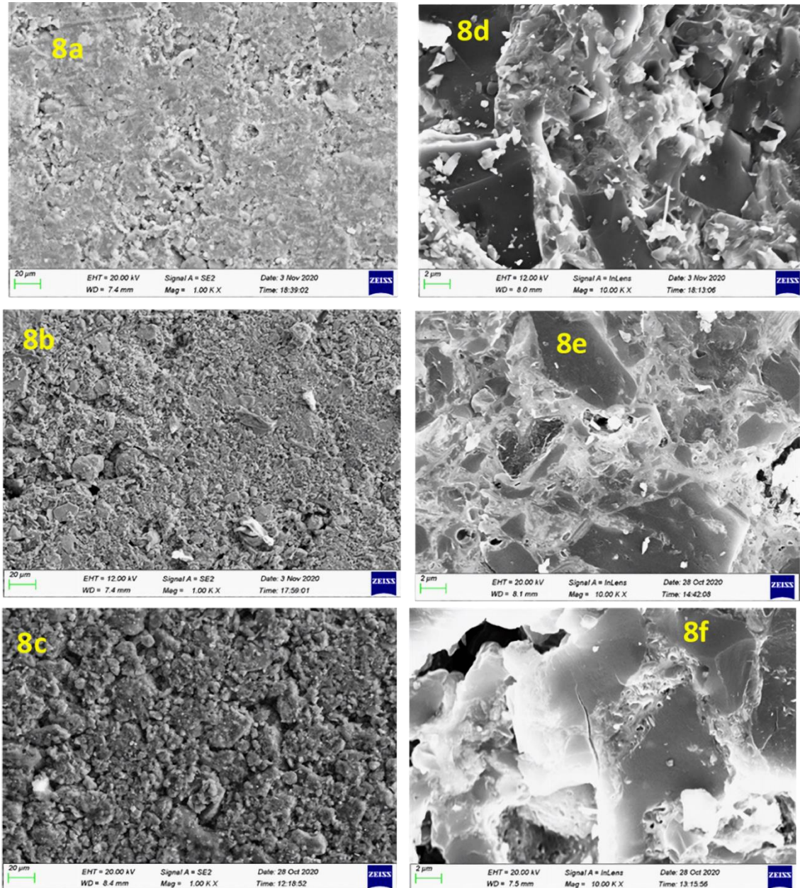
Figure 4-8 Microstructure of the top surface of coal composite specimens (a) Likeflow coal slurry (LCS), (b) Greenside tailing slurry (GTS) and (c) Proteas coal discard (PCD), and the fractured surface of (d) LCS, (e) GTS and (f) PCD
