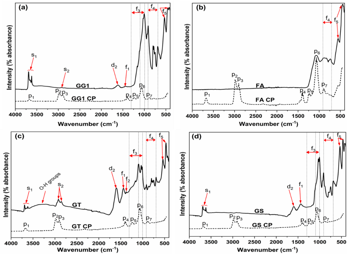
Figure 7-3 Fourier Transform Infrared spectra of the coal waste and their corresponding composites (CP – composite; GG1 – discard from washing plant; FA – fly ash; GT – fine waste; GS – coal waste from Witbank coalfield)
