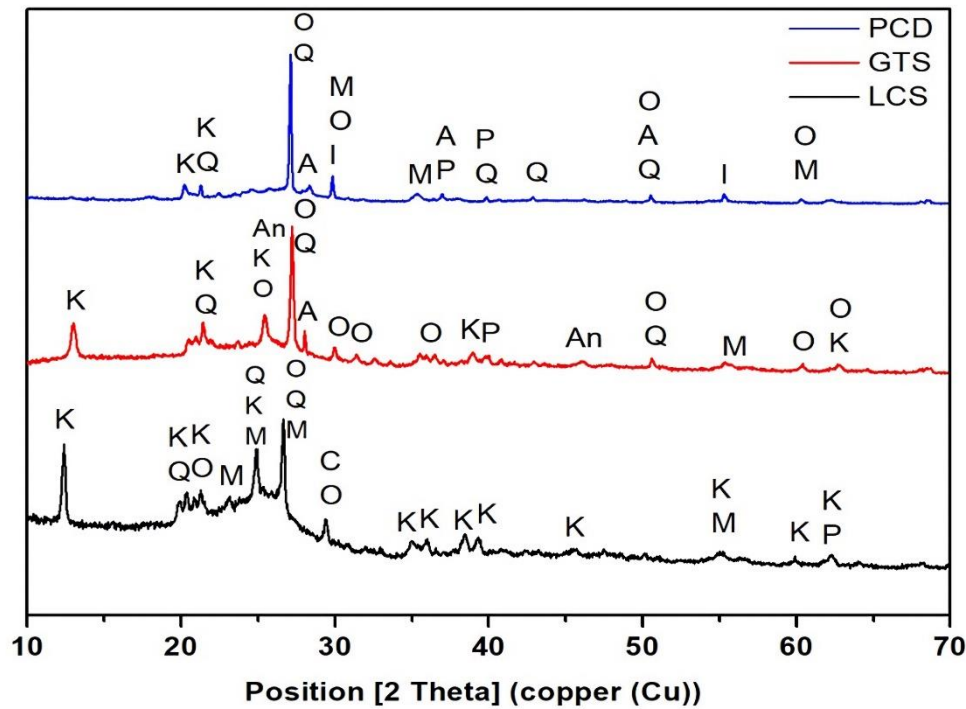
Figure 4-5 X-ray diffraction patterns of pulverised coal discard samples (K – kaolinite; Q – quartz; M – muscovite; O – orthoclase; P – pyrite; Q – quartz; C – calcite; A – anorthite; An – anatase; I – illite; GTS – Greenside tailing slurry; LCS – Likeflow coal slurry; PCD – Proteas coal discard)
