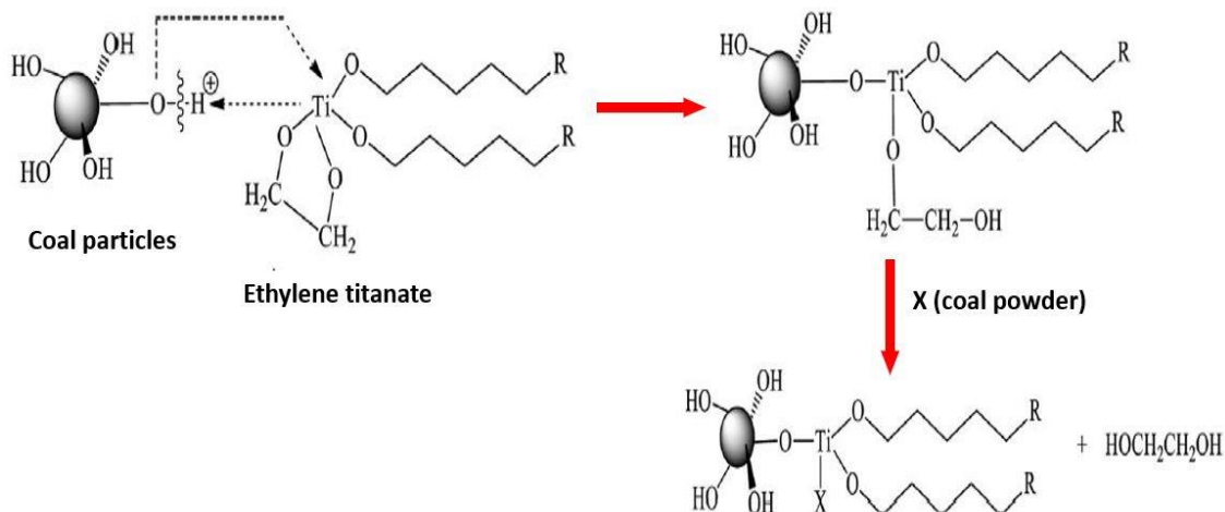
Figure 2-9 Reaction scheme of coal particles and titanate coupling agent (Adapted from Cheng et al. (2014))
