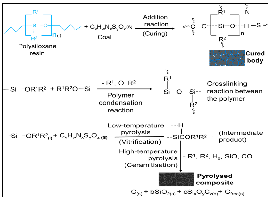
Figure 6-5 Hypothetical mechanisms of the curing and pyrolysis of coal waste and the polysiloxane preceramic polymer
