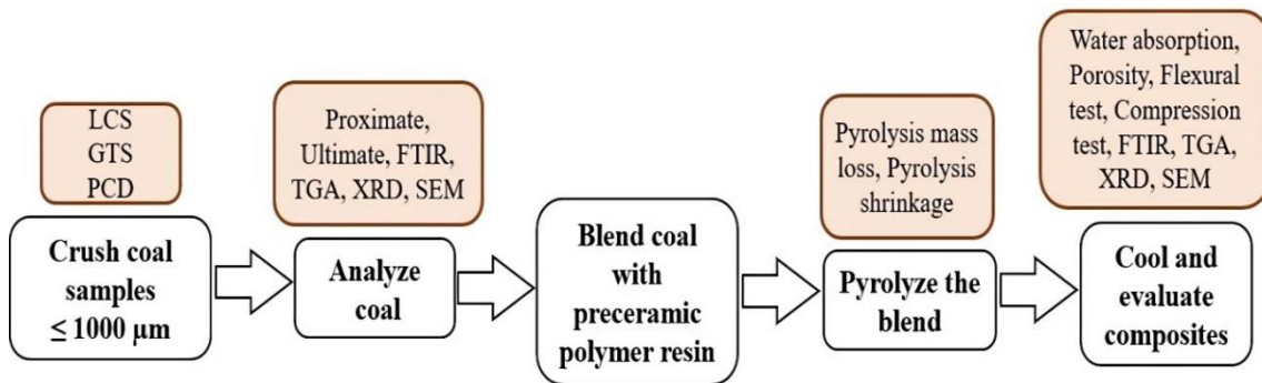
Figure 4-1 A schematic representation of the experimental procedure for producing coal composites
