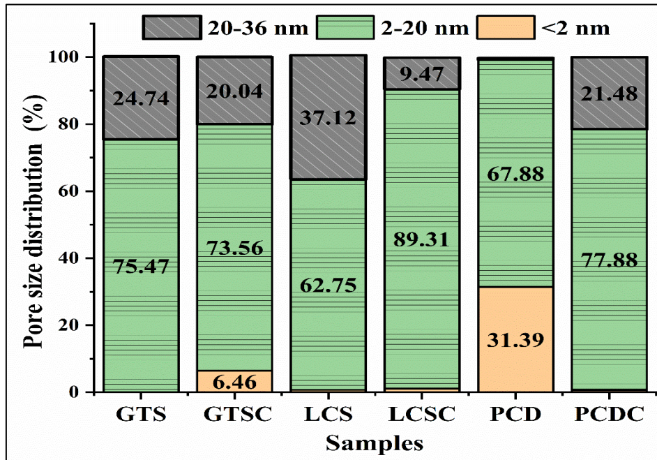
Figure 6-6 Comparison of the pore size distributions of the coal samples and the carbon/ceramic composites
