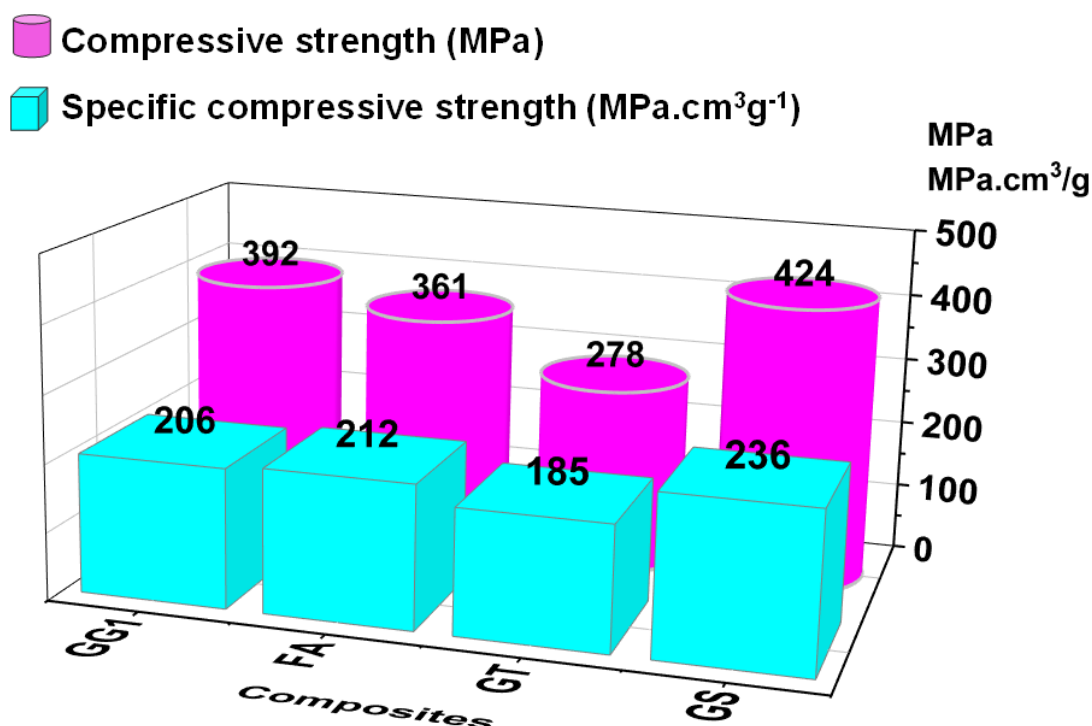
Figure 7-12 Average ultimate compressive stress and specific compressive strength of the composites
