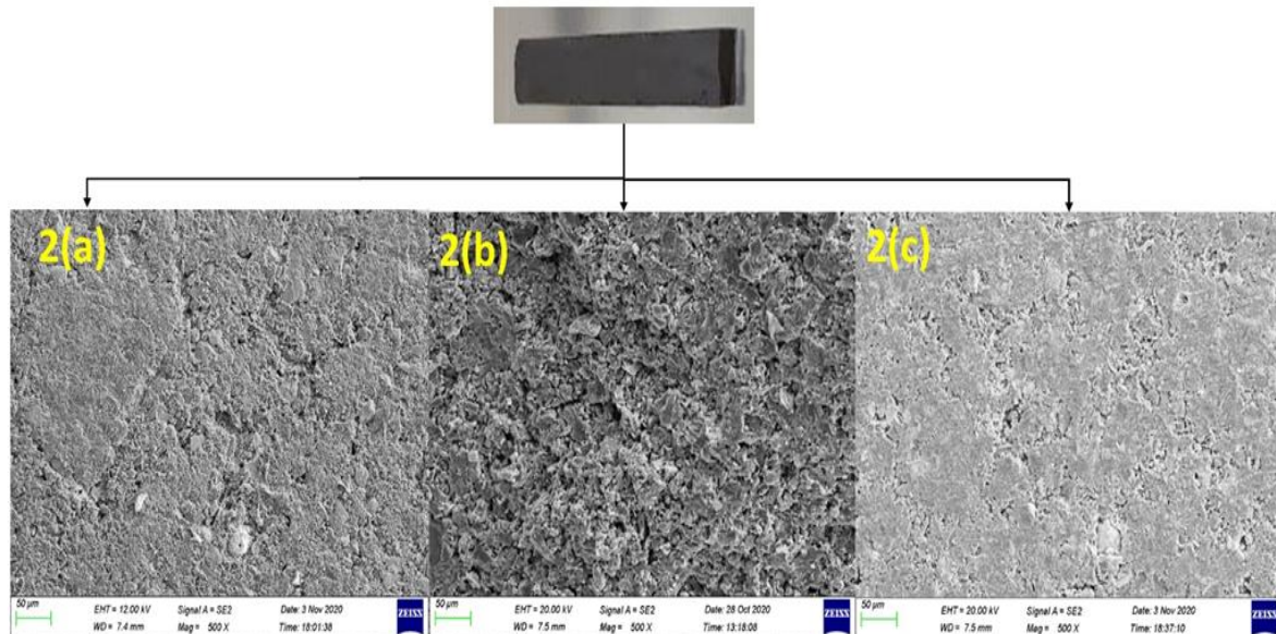
Figure 5-2 Scanning electron microscopy images of the (a) Greenside tailing slurry, (b) Proteas coal discard and (c) Likeflow coal slurry composites
