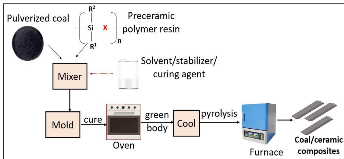
Figure 2-11 Schematic of coal/ceramic composite preparation
