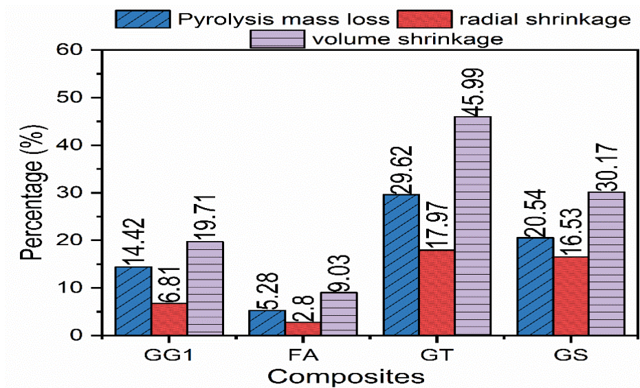
Figure 7-8 Average pyrolysis mass loss and shrinkage of the composites (GG1 – discard from washing plant; FA – fly ash; GT – fine waste; GS – coal waste from Witbank coalfield)
