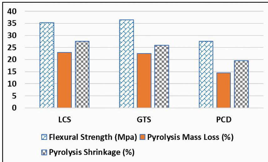
Figure 4-9 Summary of flexural strength, pyrolysis mass loss and pyrolysis shrinkage of coal composite specimens
