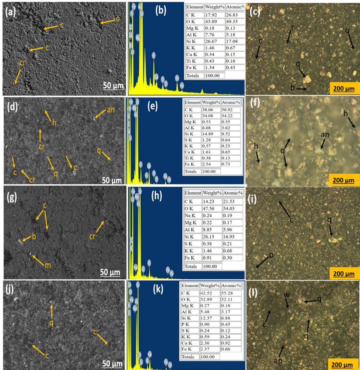
Figure 7-5 Scanning electron microscopy secondary electron image (a), back-scattered images (d, g, j), energy dispersive X-ray spectroscopy analysis (b, e, h, k) and optical micrographs (c, f, i, l) of the as-fabricated composites. (a, b, c) GG1; (d, e, f) FA; (g, h, i) GT; (j, k, l) GS composites. (an – anorthite; b – aluminium phosphate; c – carbon; cr – crack; h – hematite; m – monetite; q – quartz)
