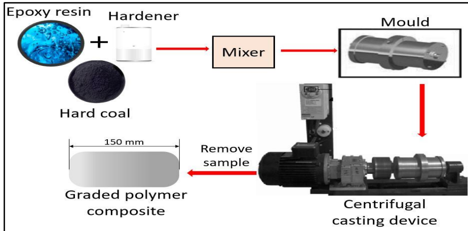
Figure 2-5 Schematic of coal/polymer gradient composite preparation based on the centrifugal casting method (Adapted from Stabik and Chomiak (2011))
