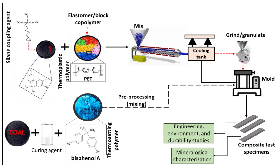
Figure 2-4 Schematic representation for the fabrication of coal/polymer composites
