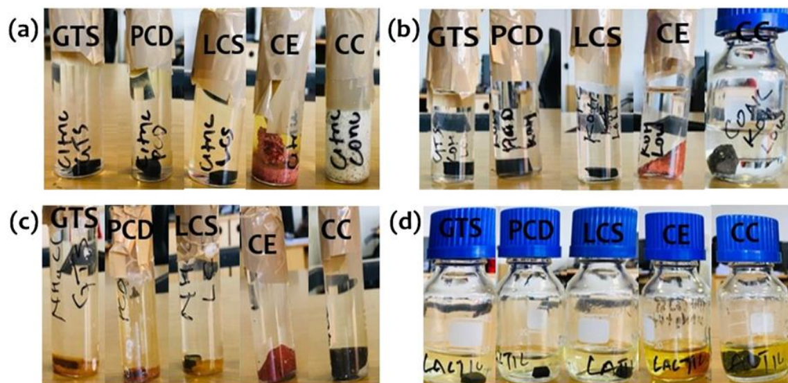
Figure 5-6 Coal composites and conventional roof tiles exposed to different chemicals: (a) citric acid, (b) potassium hydroxide, (c) ammonium chloride and (d) lactic acid solution
