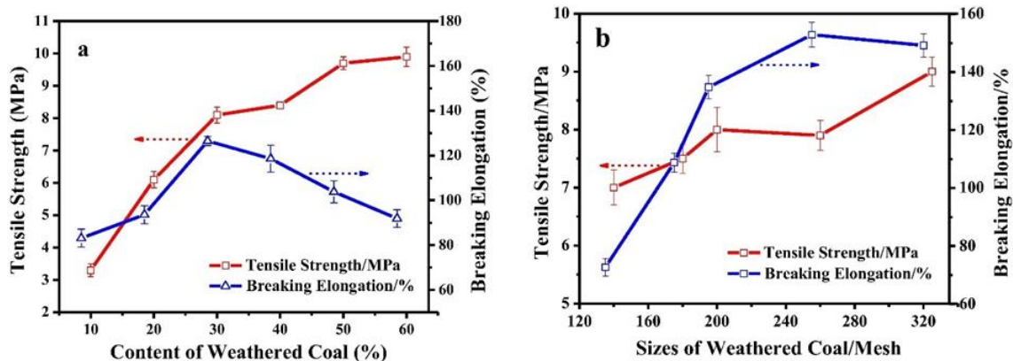
Figure 2-7 Mechanical properties as a function of (a) the percentage mass of coal and (b) the particle size (Hu et al., 2017, reproduced with permission from Elsevier)
