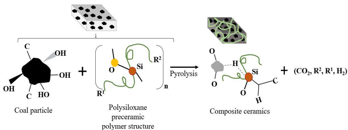
Figure 4-10 Mechanism of the binding scheme between discard coal particles and the preceramic polymer resin
