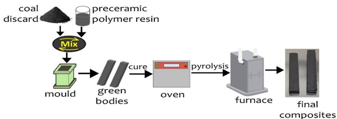
Figure 5-1 Schematic of coal/ceramic composites production
