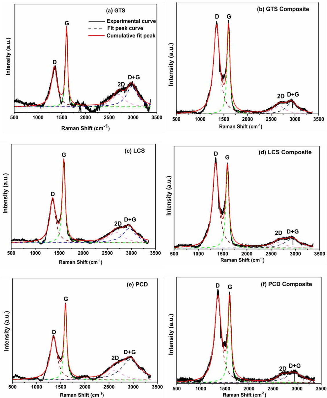
Figure 6-8 Raman spectra of the coal waste and the carbon/ceramic composites with their corresponding curve-fitting bands
