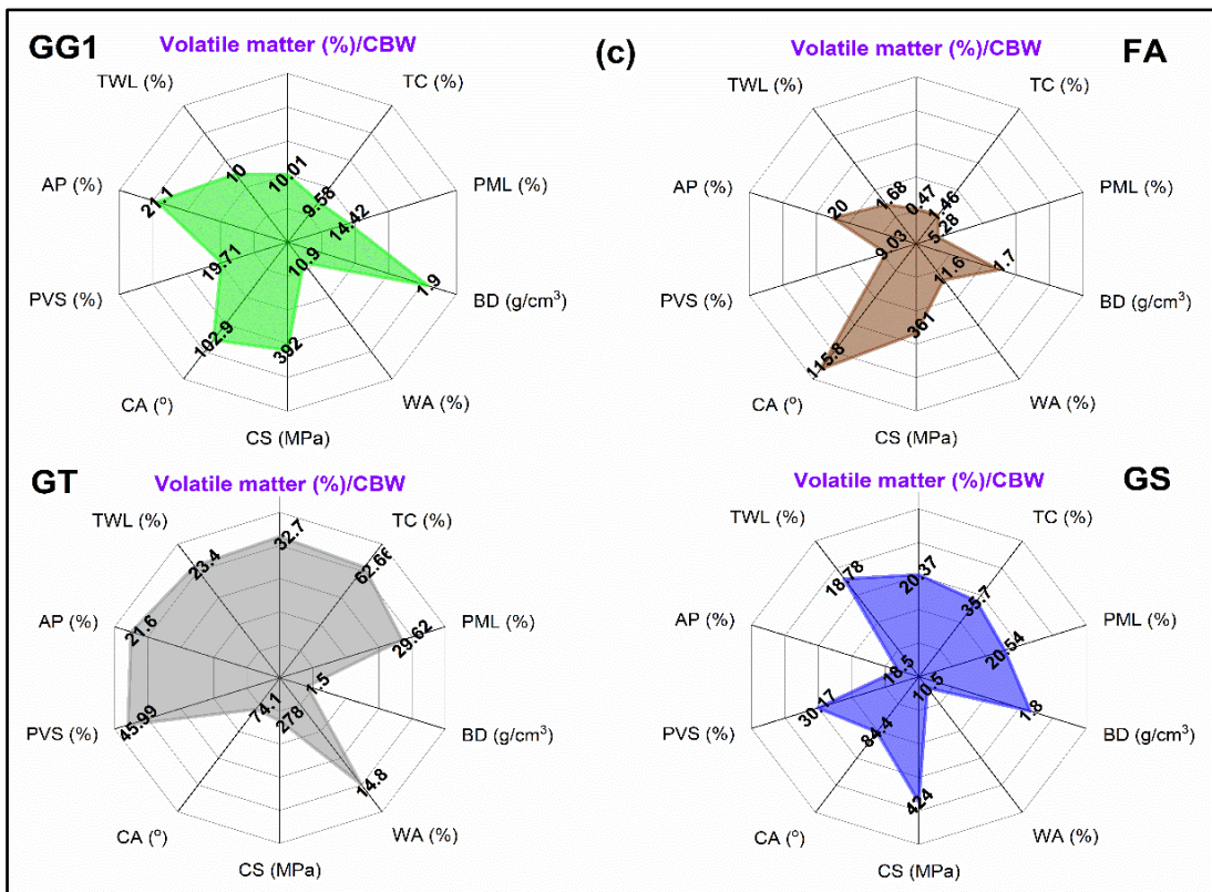
Figure 7-13 The correlation between (a) hydrogen/carbon ratio (b) ash content (c) volatile matter of CBW on the key performance properties of the composites
