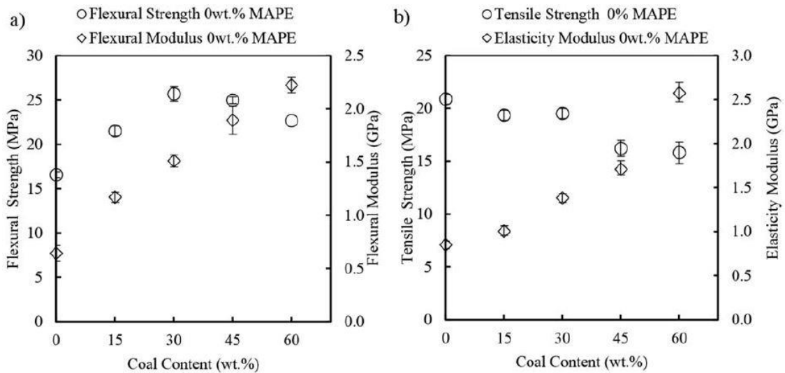
Figure 2-6 (a) Flexure and (b) tensile properties of coal plastic composites composed of 0 to 60 weight percent (wt.%) of Pittsburgh No. 8 coal (Phillips et al., 2019)
