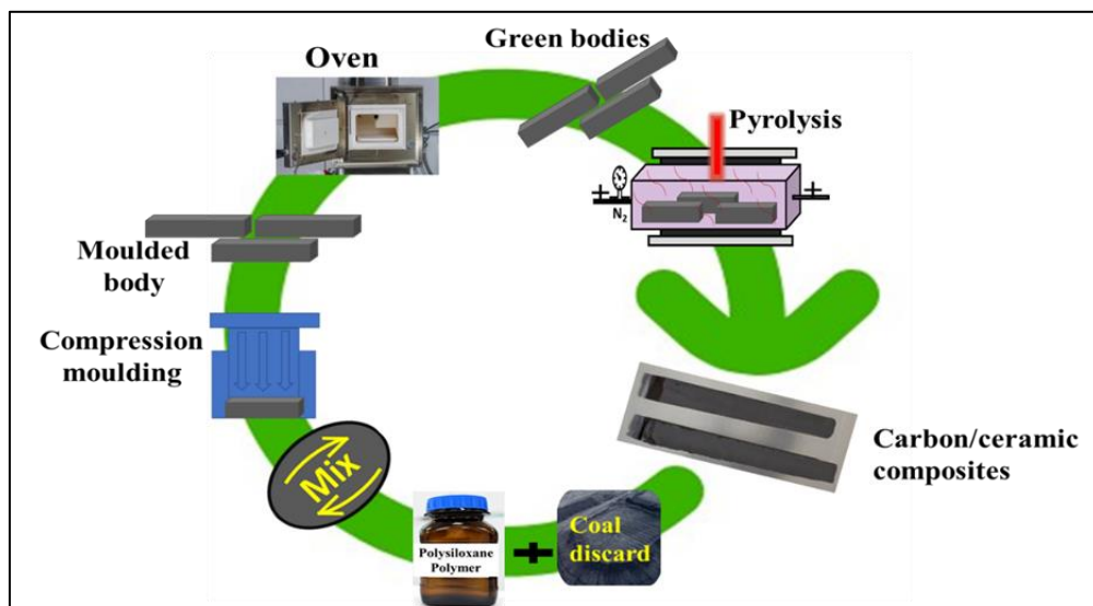
Figure 6-2 A summary of the production of the carbon/ceramic composites
