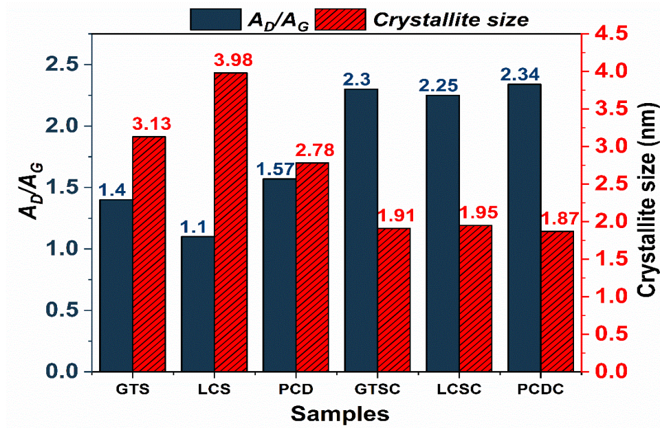
Figure 6-9 Variation in the peak intensity ratio ( A_D/A_G ) and the size of the carbon cluster crystallites of the coal and their composites
