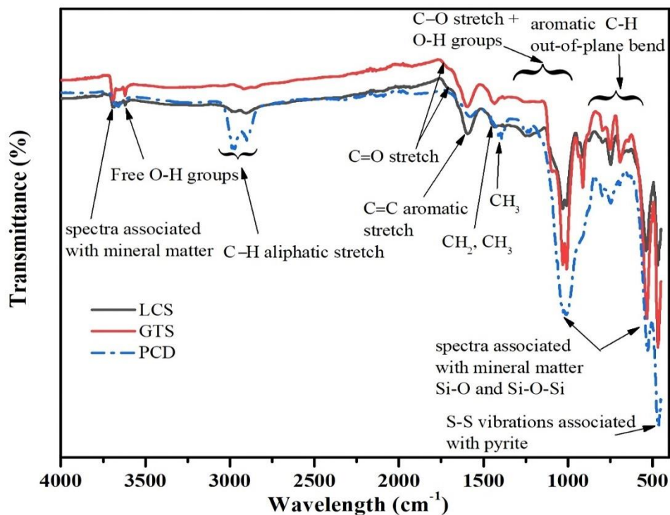
Figure 4-3 Spectra of the raw coal discard samples
