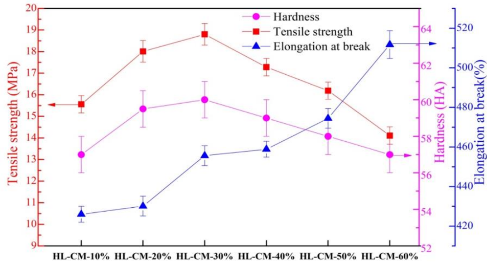
Figure 2-8 Mechanical properties of the SBR1500 rubber filled with coal slime with different ash content (Tan et al., 2019, reproduced with permission from Elsevier)
