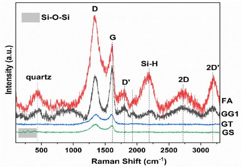
Figure 7-6 Raman spectra of the composites
