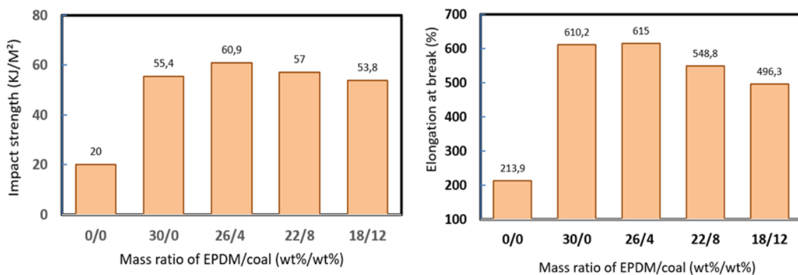
Figure 2-10 (a) impact strength and (b) elongation at break of pure polypropylene (0/0), and polypropylene/ethylene-propylene-diene monomer/coal composites (Adapted and modified from Bai et al. (2019))
