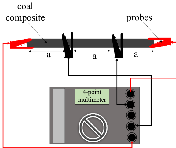
Figure 6-4 Arrangement of the four-point probe resistance measurement of the carbon/ceramic composites
