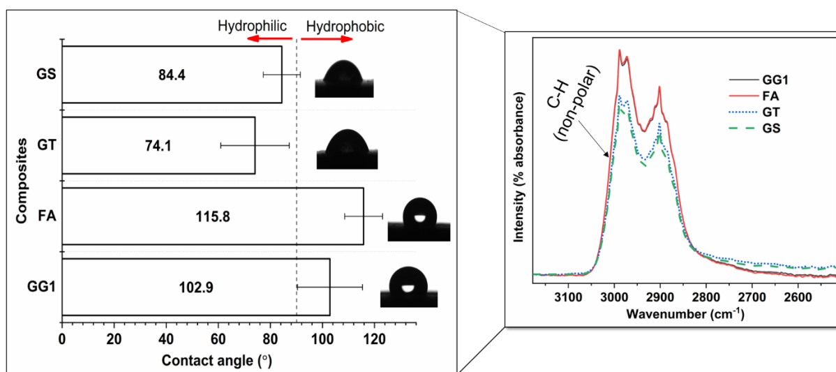
Figure 7-11 The water contact angle of the composites measured by the sessile drop method and FTIR of the nonpolar C-H group (right)
