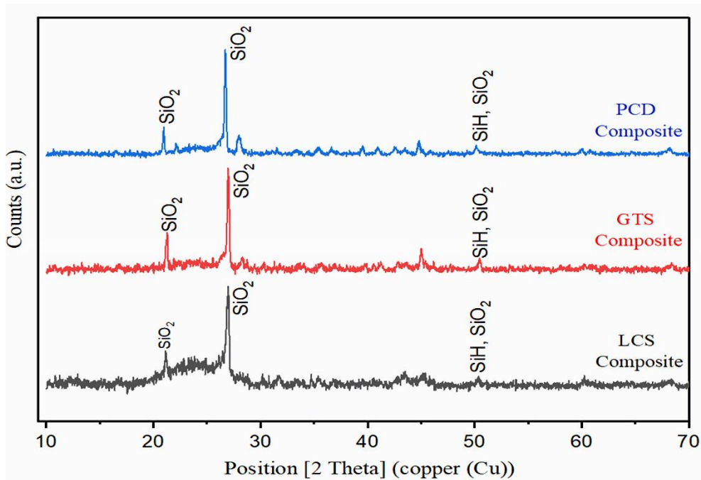
Figure 4-6 X-ray diffraction patterns obtained for coal/ceramic composite specimens (a.u. – arbitrary units; SiH – silicon hydride; \text{SiO}_2 – silicon dioxide; GTS – Greenside tailing slurry; LCS – Likeflow coal slurry; PCD – Proteas coal discard)
