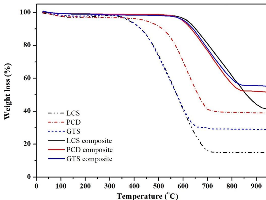
Figure 4-7 Thermogravimetric curves for coal discard samples and coal composite specimens
