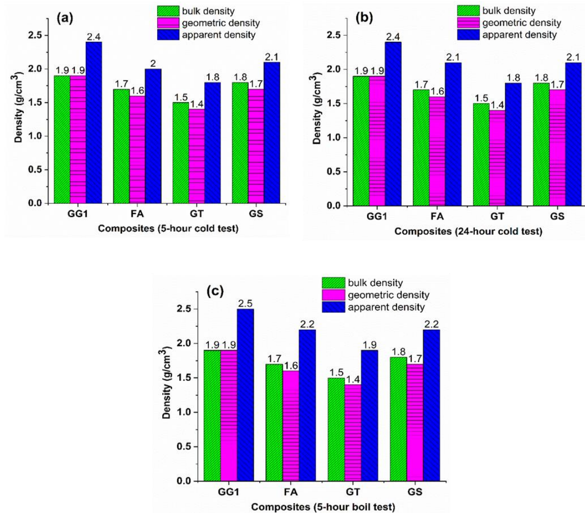
Figure 7-9 Bulk, geometric and apparent densities of the composites (GG1 – discard from washing plant; FA – fly ash; GT – fine waste; GS – coal waste from Witbank coalfield)
