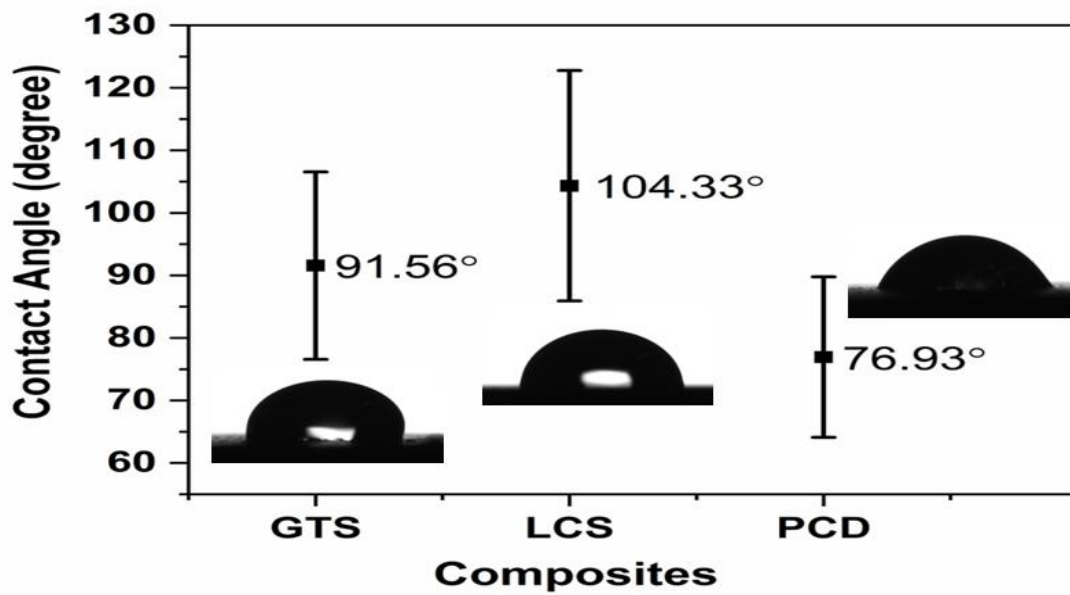
Figure 6-7 The water contact angle of the carbon/ceramic composites at room temperature (GTS – Greenside tailing slurry; LCS – Likeflow coal slurry; PCD – Proteas coal discard)
