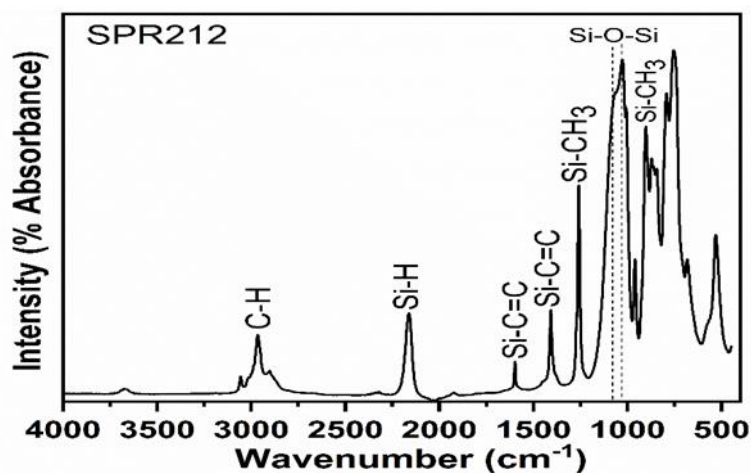
Figure 7-2 Fourier Transform Infrared spectrum of the native polysiloxane SPR-212
