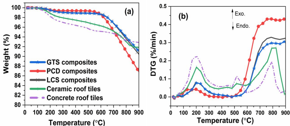
Figure 5-5 (a) Weight loss curves and (b) derivative thermogravimetric (DTG) curves of coal discard composites and conventional roof materials (GTS – Greenside tailing slurry; PCD – Proteas coal discard; LCS – Likeflow coal slurry)
