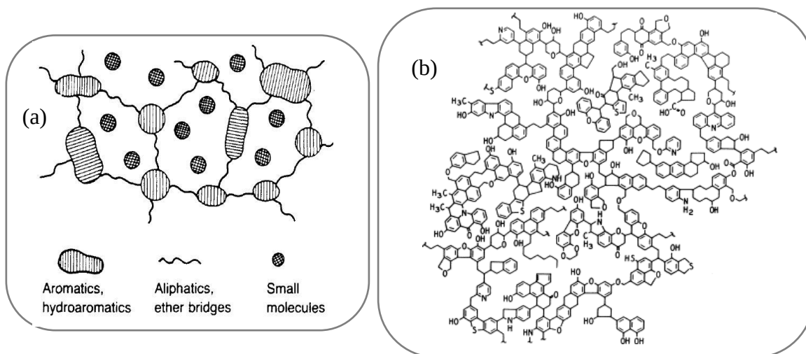
Figure 2-2 (a) Three-dimensional crosslinked two-component macromolecular model of coal (Adapted from Haenel (1992)), (b) Molecular structure model of bituminous coal (Adapted from Shinn (1984))
