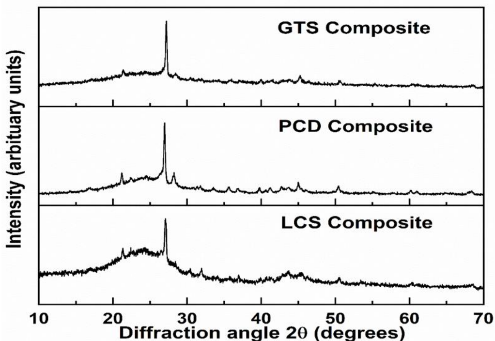
Figure 5-4 X-ray diffraction patterns of the composites (GTS – Greenside tailing slurry; PCD – Proteas coal discard; LCS – Likeflow coal slurry)
