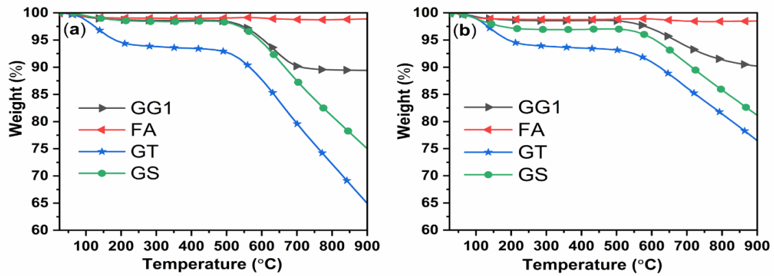
Figure 7-7 Thermal analysis (TGA) profiles of the composites under (a) Oxygen (b) Air environment
