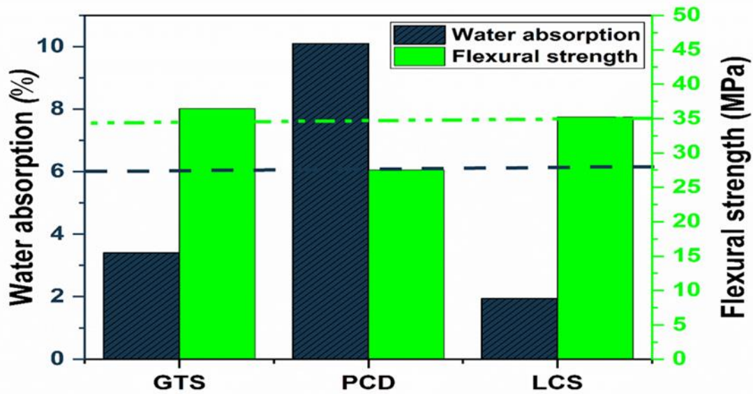
Figure 5-3 Water absorption and flexural strength properties of the composites (GTS – Greenside tailing slurry; PCD – Proteas coal discard; LCS – Likeflow coal slurry; dotted lines represent the standard cut-off)
