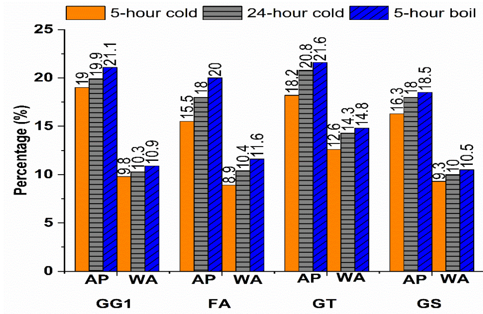
Figure 7-10 Average apparent porosity and water absorption of the composites (AP – average porosity; WA – water absorption; GG1 – discard from washing plant; FA – fly ash; GT – fine waste; GS – coal waste from Witbank coalfield)
