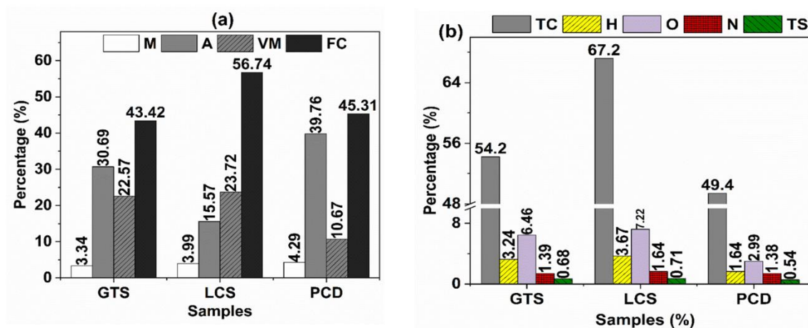
Figure 6-1 Assessment of the physicochemical characteristics of the coal wastes (air-dried) (a) Proximate analysis (b) Ultimate analysis
