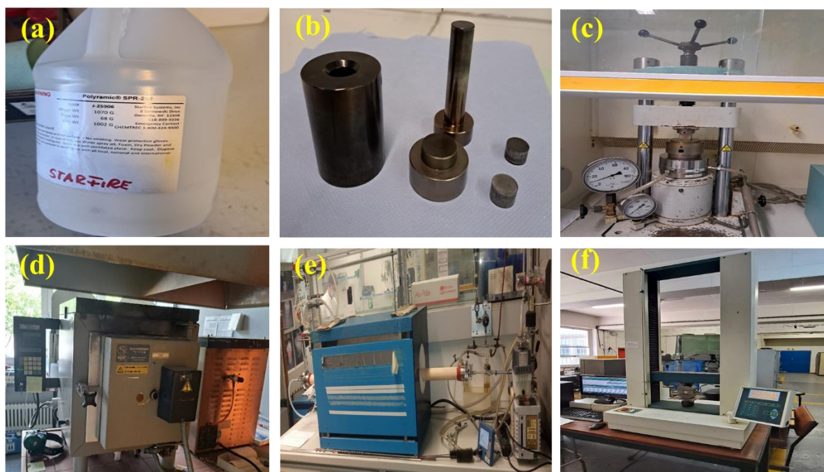
Figure 3-4 Resources used in the fabrication of the coal composites: (a) SPR-212 preceramic polymer, (b) 20 mm diameter moulds for shaping, (c) compression moulding machine, (d) oven for curing the moulded mixture of coal and the preceramic polymer, (e) high temperature furnace for pyrolysis of the cured moulded body and (f) compressive strength test equipment
