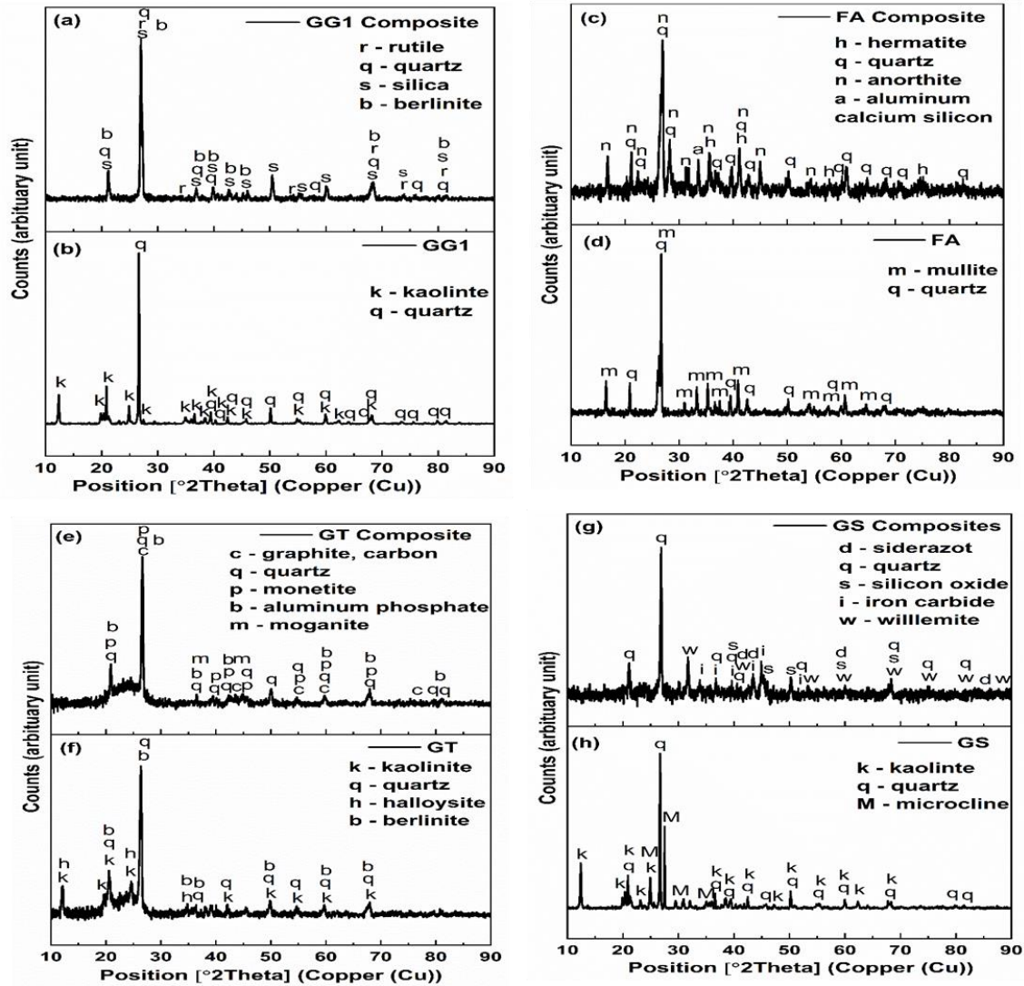
Figure 7-4 A comparison of the X-ray diffraction patterns of the coals and coal composites
