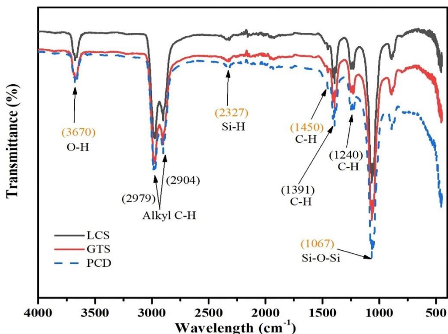
Figure 4-4 Spectra of the coal composites (GTS – Greenside tailing slurry; LCS – Likeflow coal slurry; PCD – Proteas coal discard)
