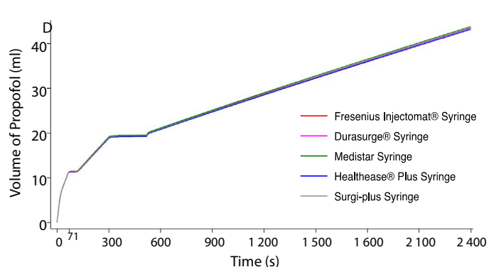
Figure 4D: Volume versus time plot of non-programmed syringes versus Fresenius Injectomat® option
