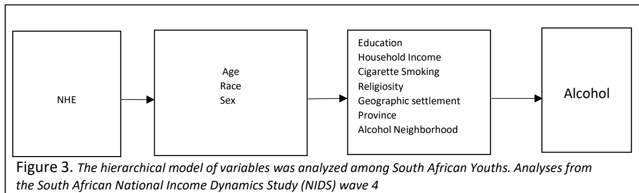
Figure 3: Hierarchical model used in the analysis
