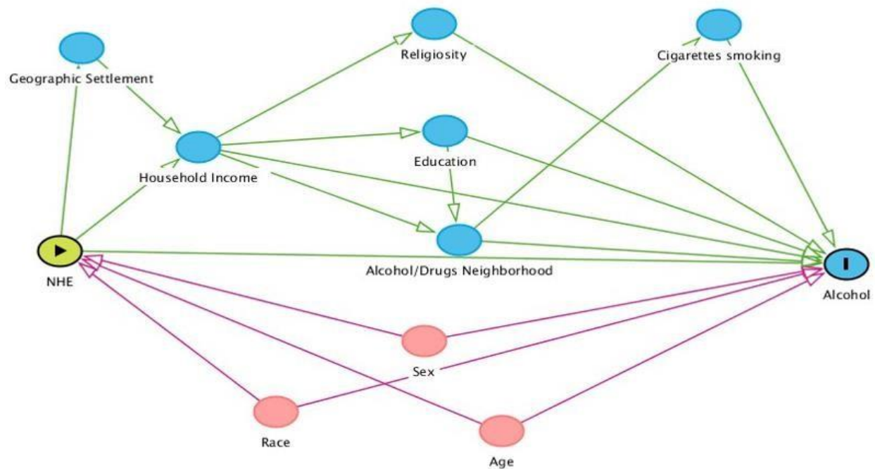
Figure 2: Directed acyclic graph
