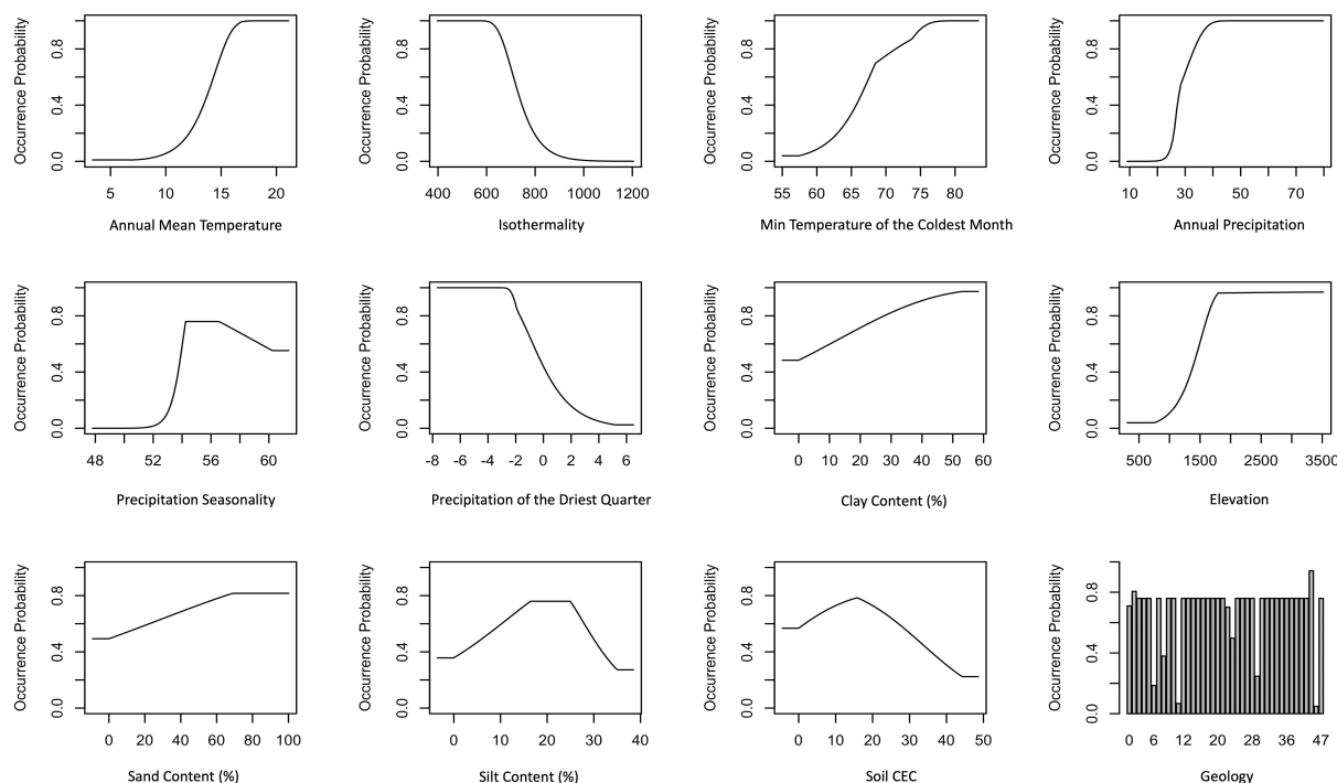
FIGURE 2 Response curves of the bioclimatic and environmental variables for the sungazer ENM. The x-axis of each graph represents each variable, and the y-axis indicates the probability of occurrence (cloglog output) for sungazers. The Geology plot is indicative of geology type (categorical data).
