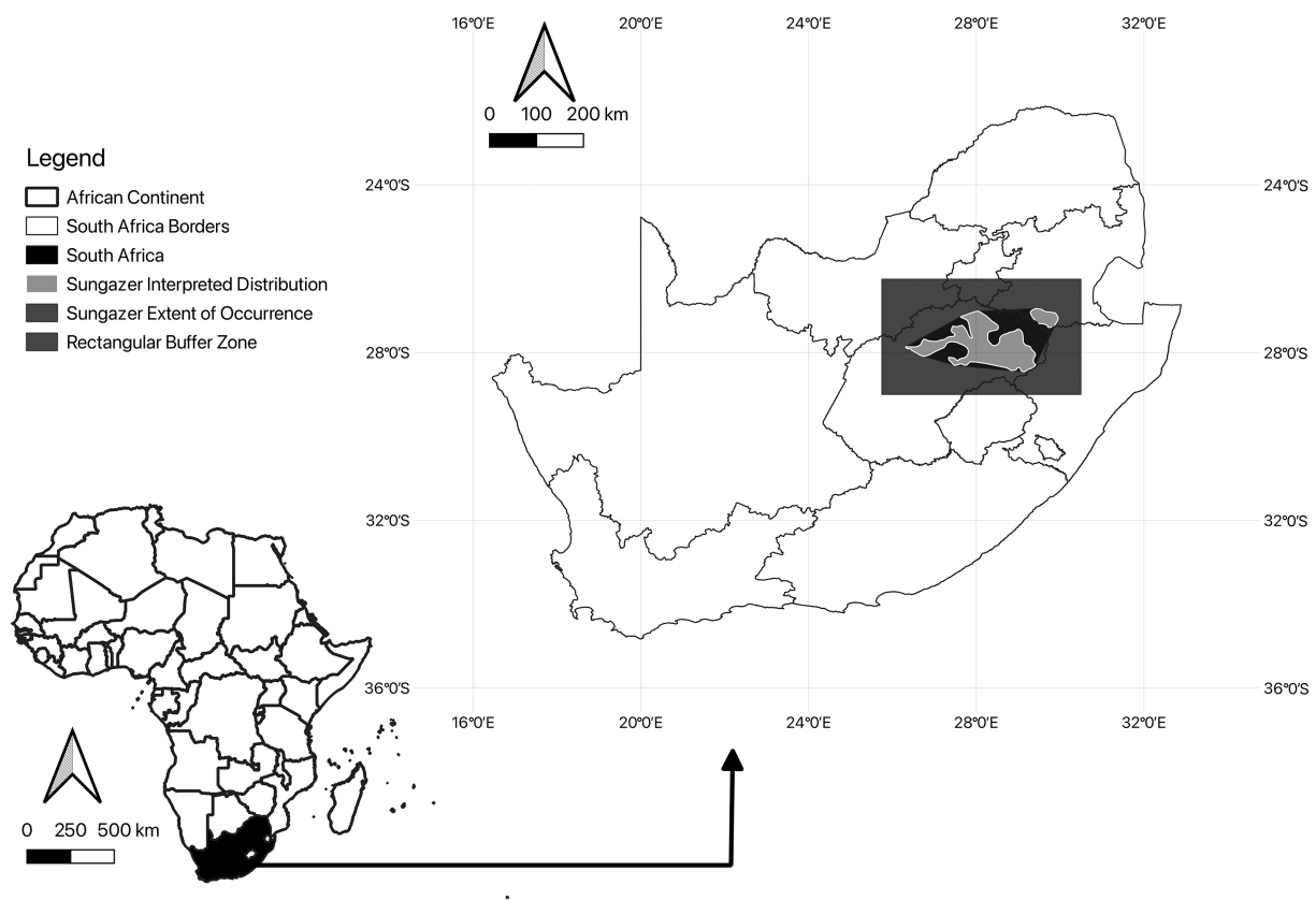
FIGURE 1 Map of Africa zoomed into South Africa that shows the different scales used to predict habitat suitability for sungazers. Dark grey represents the rectangular buffer zone ( 142\,884\text{ km}^2 ) from which current and future sungazer distributions were modelled. Inside the buffer zone is the EOO (black; 40\,573\text{ km}^2 ) and the interpreted distribution (light grey; 21\,985\text{ km}^2 ) for sungazers.
