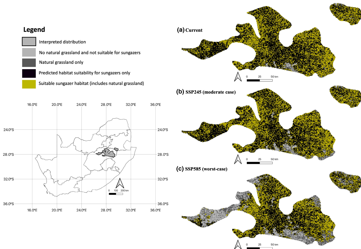
FIGURE 4 Habitat suitability maps showing the predicted distribution of sungazers within their current interpreted distribution. The map shows South Africa zoomed into an overlay of the binary output (suitable/unsuitable) of predicted sungazer occurrence with natural grassland only. The intersection (yellow) between natural grassland and predicted sungazer occurrence is considered suitable sungazer habitat. Maps shown represent current (a), and future 2100 (SSP245 (b) and SSP585 (c)) predictions. SSP, shared socioeconomic pathways.
