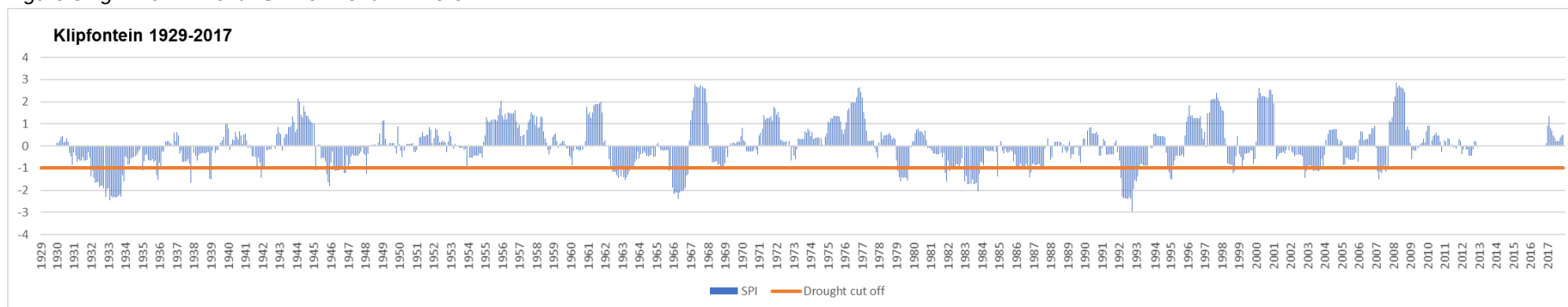
Figure 8.2h: The 12-month SPI for Klipfontein
