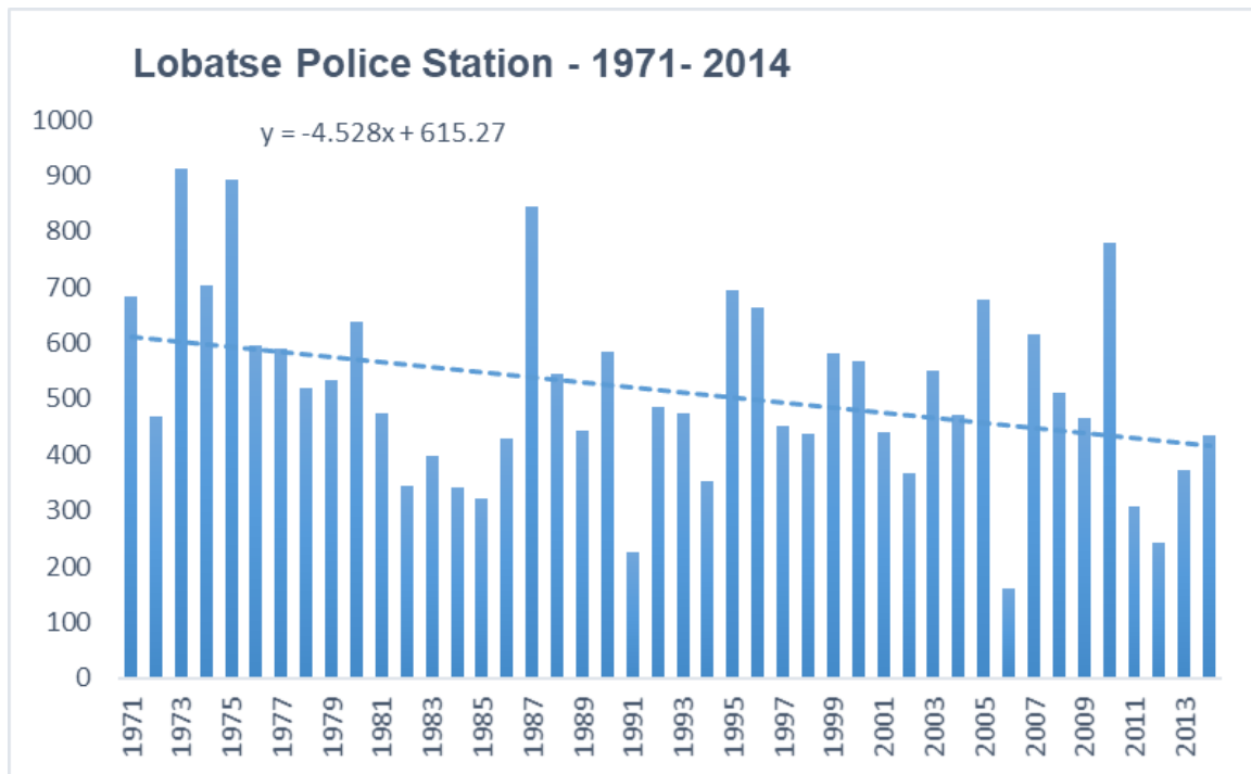
8.1m Rainfall data Lobatse Police Station
