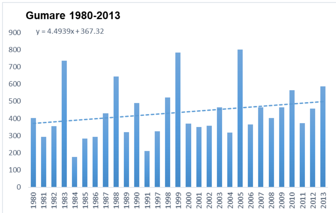
8.1y Rainfall data Gumare
