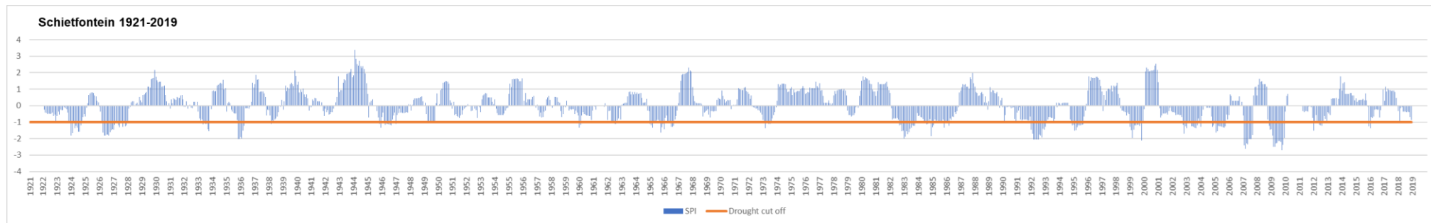
Figure 2: The 12-month SPI for Schietfontein.
