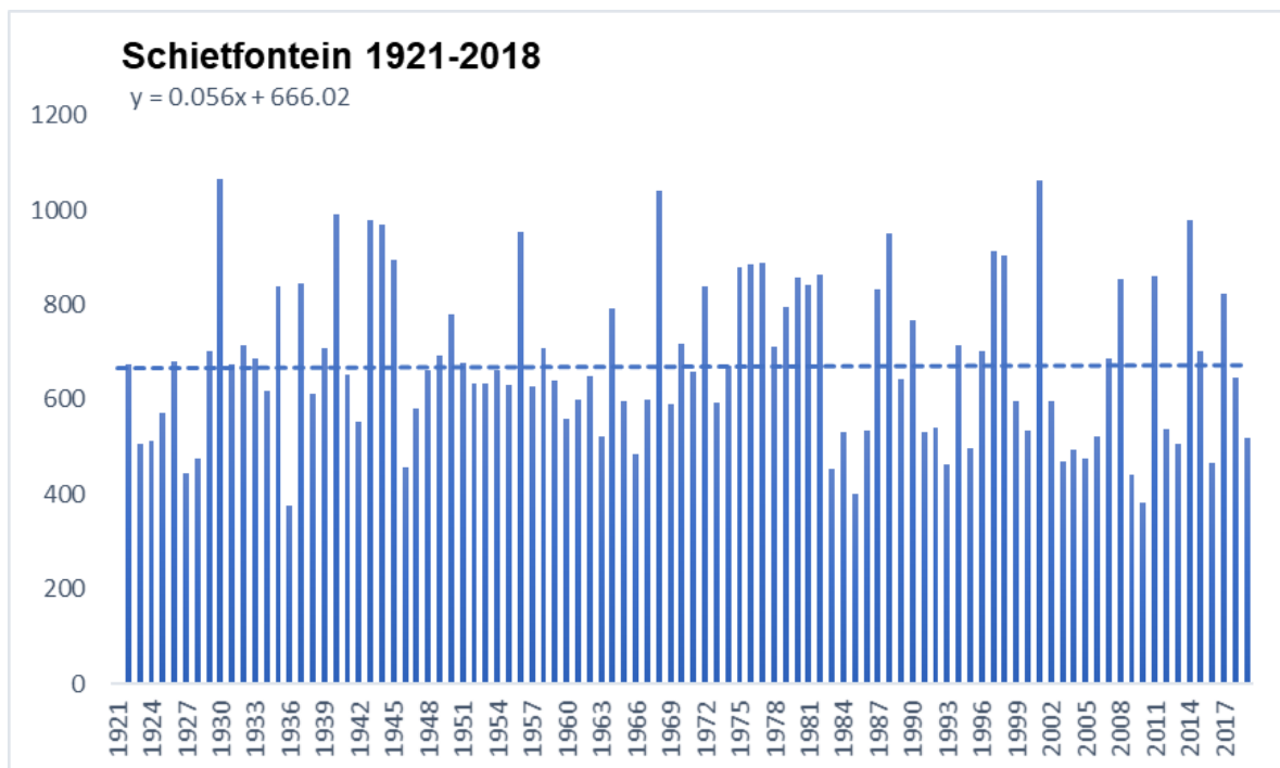
8.1aw Rainfall data Schietfontein
