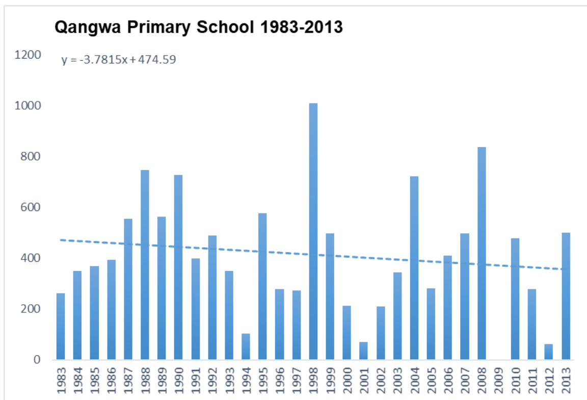
8.1v Rainfall data Qangwa Primary School
