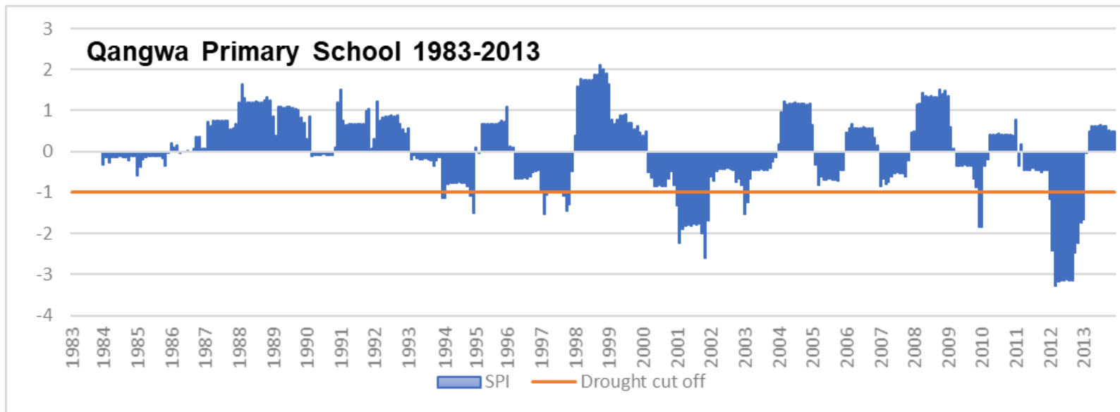
Figure 8.2as: The 12-month SPI for Qangwa Primary School
