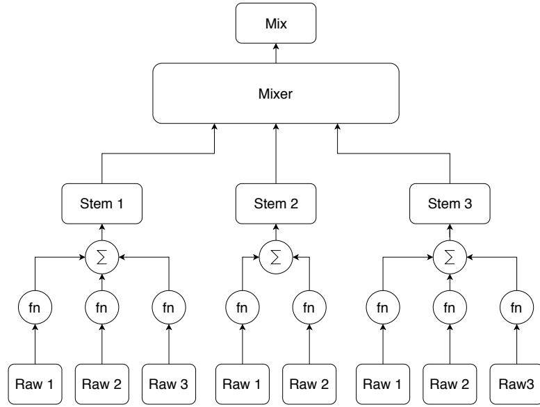
Figure 4.1: Layout of files in dataset
