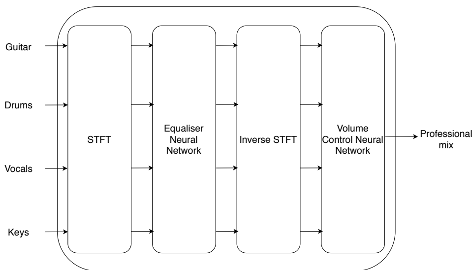
Figure 5.1: System Model - EQ first
