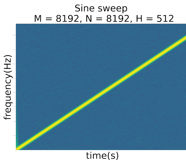
Figure 4.3: High frequency resolution and improved temporal resolution
