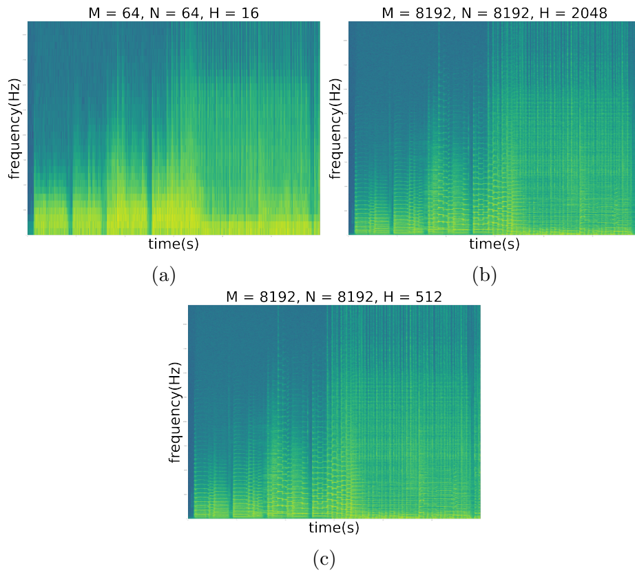
Figure 4.5: Spectrogram comparison between different FFT and hop sizes
