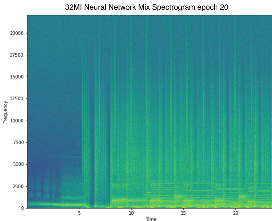
Figure 6.3: Output spectrogram of the 32MI equaliser neural network on test input after 20 epochs of training
