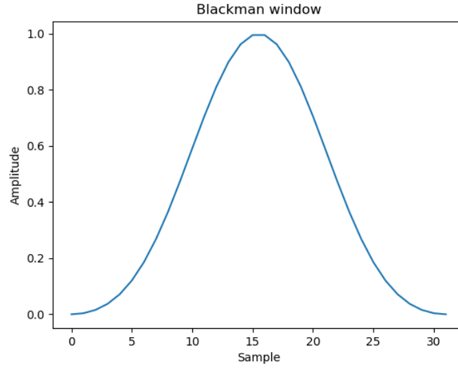
Figure 1.4: Time domain representation of Blackman window
