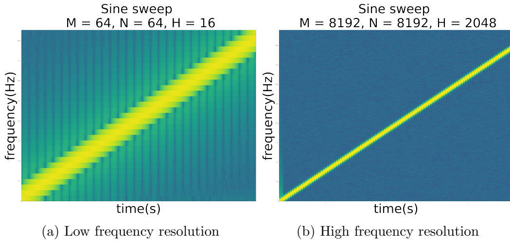
Figure 4.2: Sine sweep spectrogram comparison
