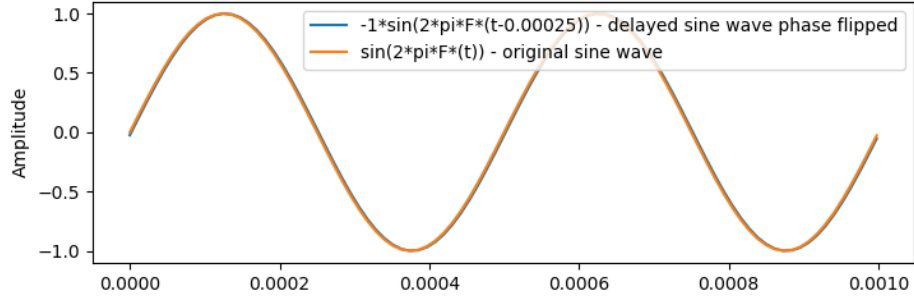
Figure 5.11: Phase cancellation solution example
