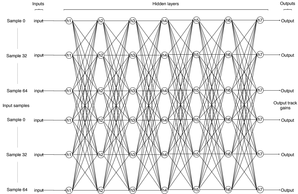
Figure 5.8: Simplified representation of the densely connected 64 sample volume control model used in this paper
