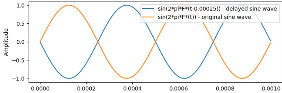
Figure 5.10: Phase cancellation example
