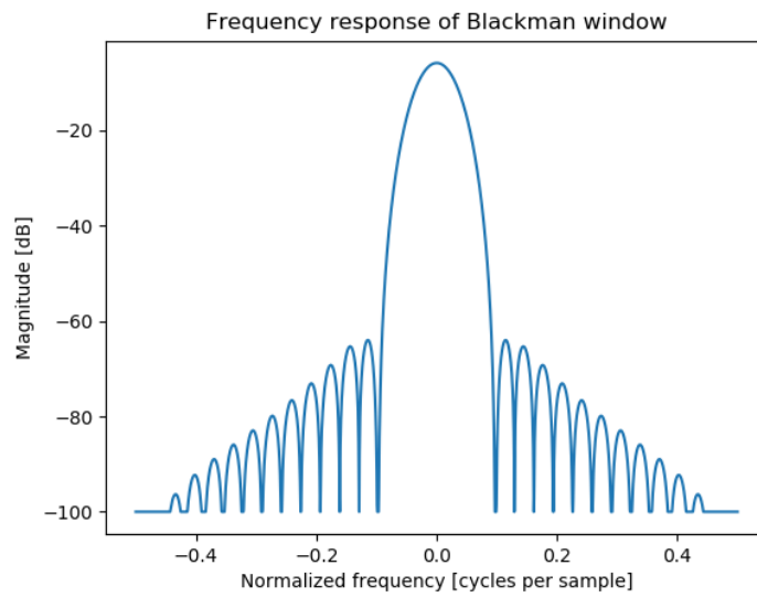
Figure 1.5: Frequency domain representation of Blackman window
