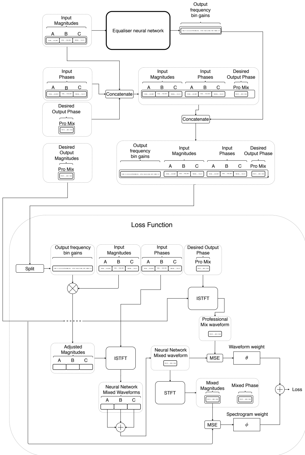
Figure 5.2: Equaliser Loss function explanation
