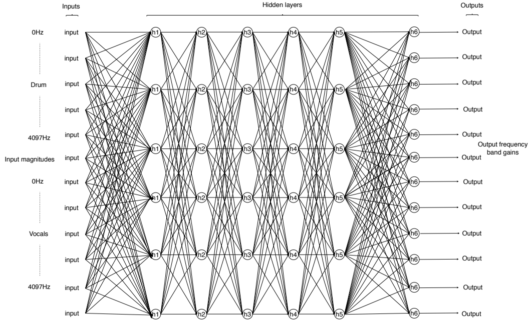
Figure 5.7: Simplified representation of the 4096 band equaliser model used in this paper
