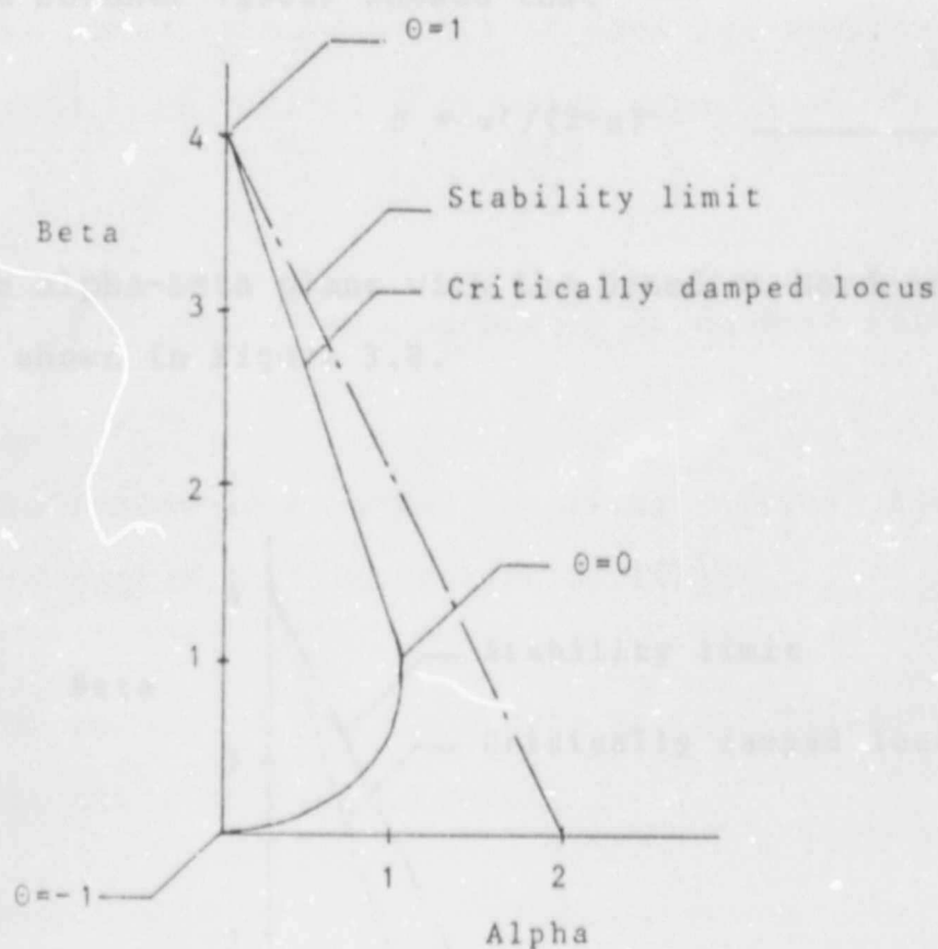
Figure 3.7 Locus for the Critically Damped Alpha-Beta Filter
