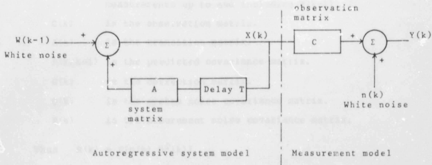
Figure 3.10 A General Form of the Kalman Filter
