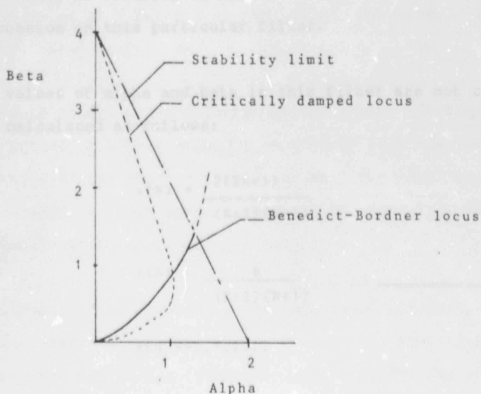
Figure 3.8 Locus for the Benedict-Bordner Condition
