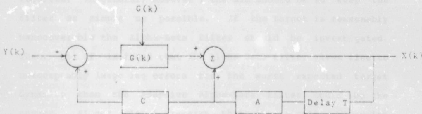
Figure 3.12 Computational Steps in the Kalman Filter
