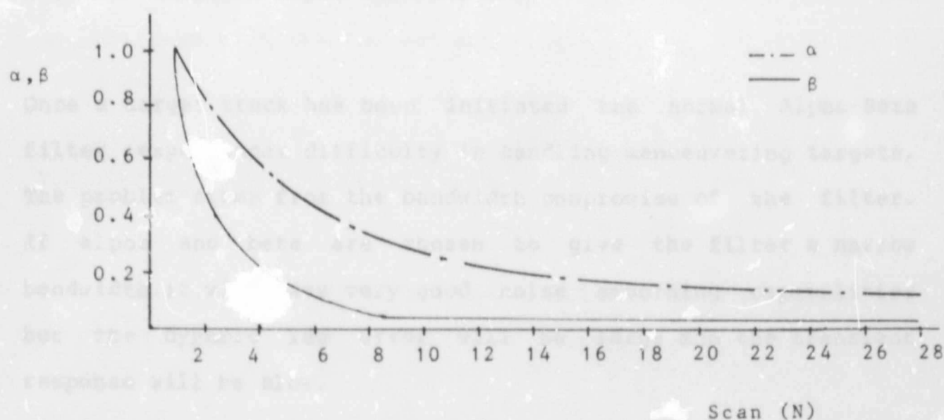
A possible solution to this shortcoming is to adapt the values of \alpha and \beta as a function of the number of scans N . Figure 3.9 Plots of \alpha, \beta Versus N for the Expanding Memory Filter. The gains are not allowed to decrease indefinitely but will be frozen after a predetermined number of iterations so as to ensure that the filter retains a measure of dynamic response in the event of target manoeuvres at a later stage.
