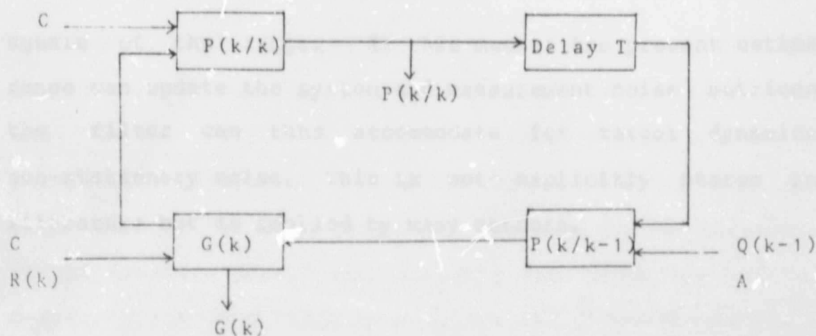
Figure 3.11 Computational Stages in the Kalman Filter
