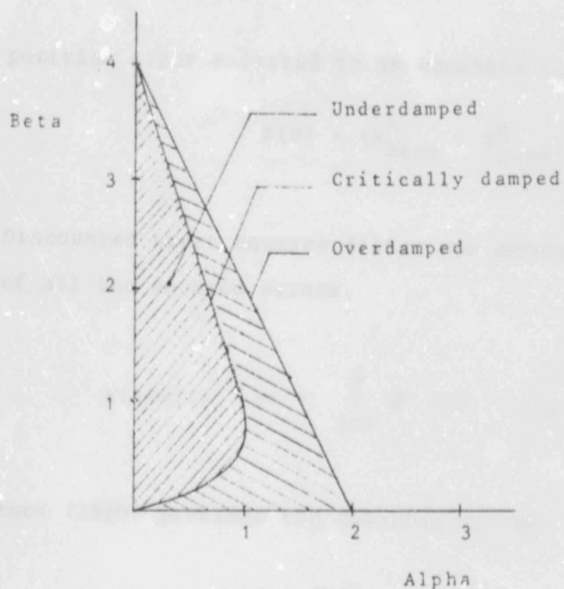
Figure 3.6 The Alpha-Beta Filter Response Regions
