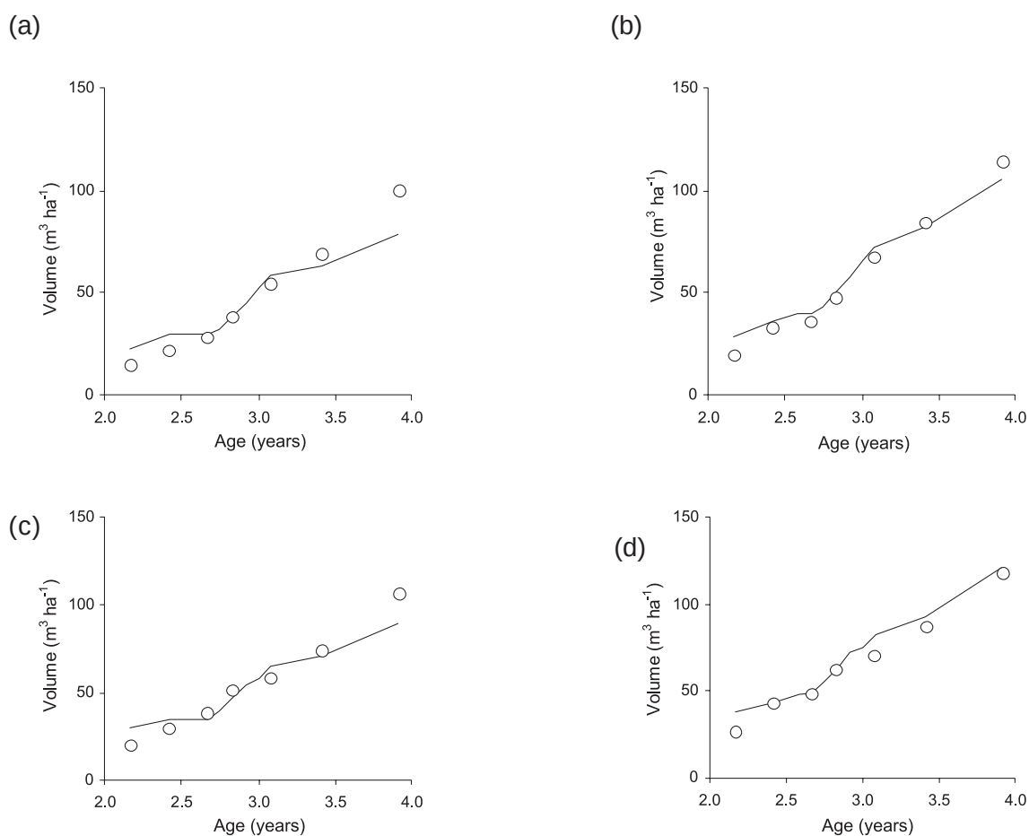
FIGURE 2. Time series of observed (o) and 3-PG model-simulated (—) stand volume in (a) control, (b) irrigated, (c) fertilised and (d) irrigated and fertilised E. grandis trees.
