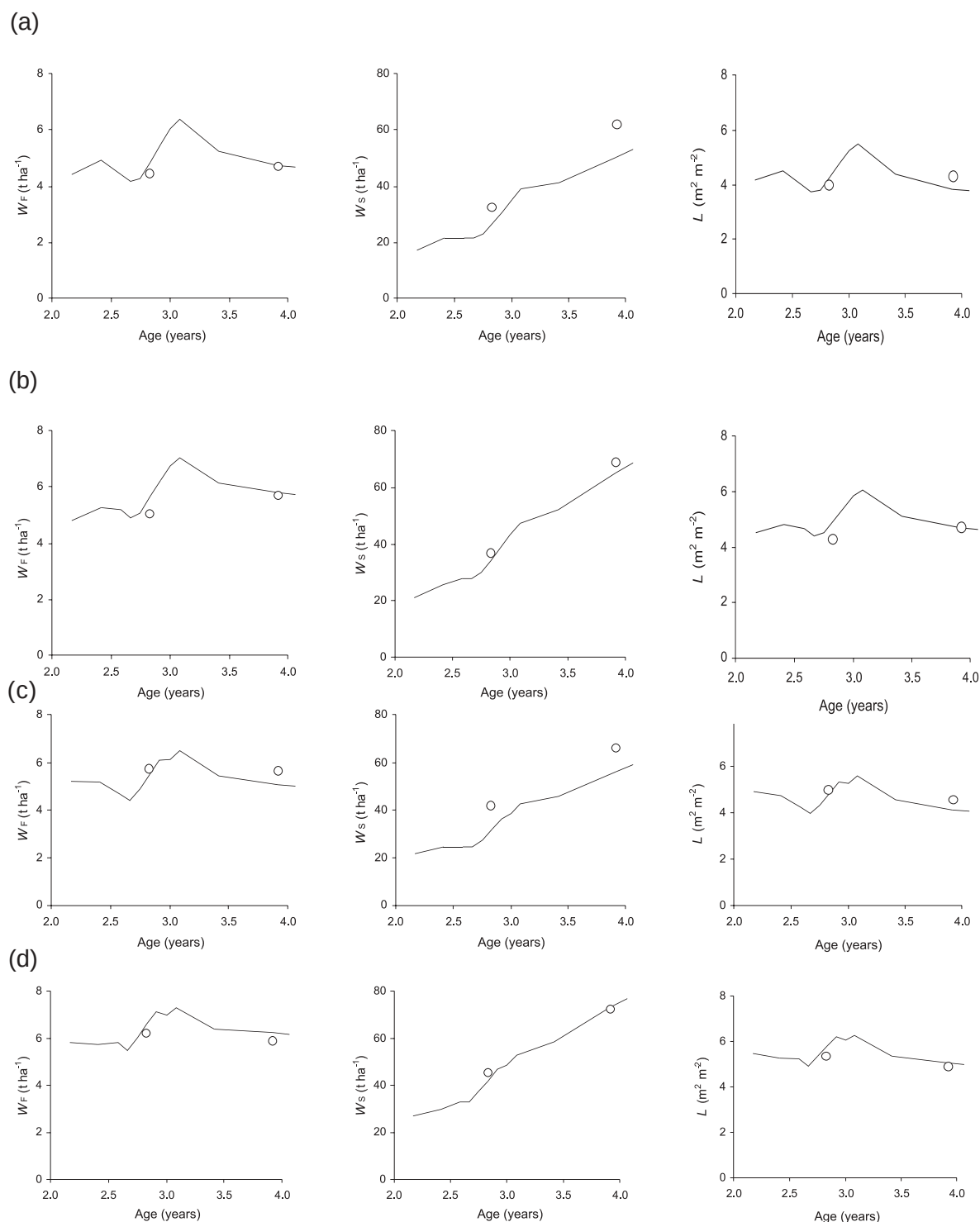
FIGURE 1. Time series of observed (o) and 3-PG model-simulated (—) foliage ( W_F ) and above-ground woody (stem wood plus bark and branches) ( W_S ) biomass, and leaf area index ( L ) in (a) control, (b) irrigated, (c) fertilised and (d) irrigated and fertilised E. grandis trees.
