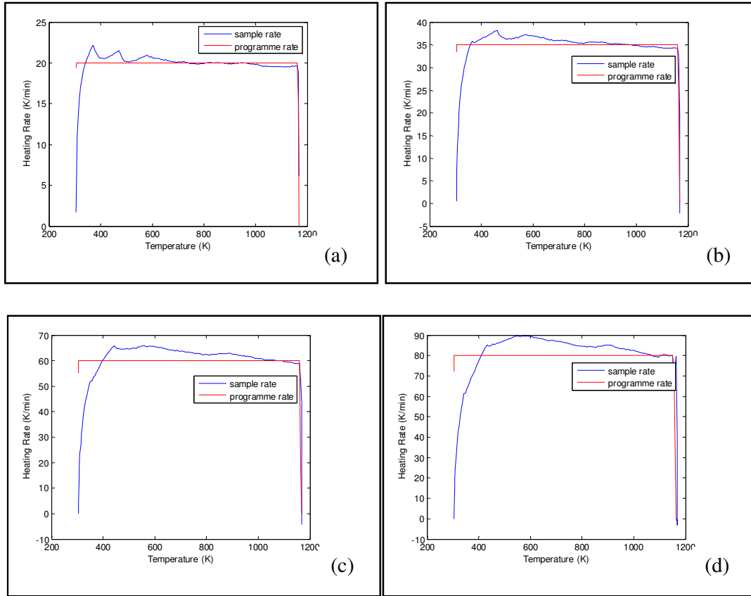
Figure 5.7: Comparison of programme heating rates and actual heating rates of the samples for coal pyrolysis in a Perkin Elmer STA600 TGA
