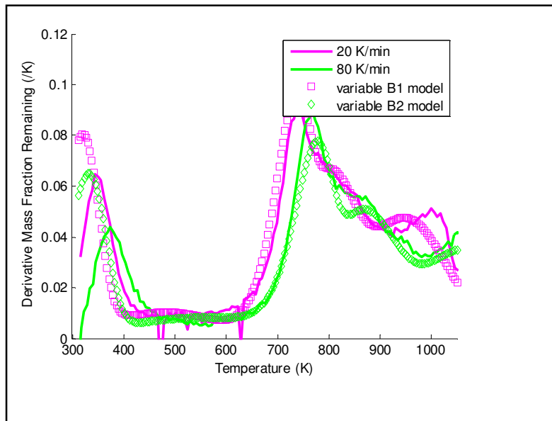
Figure 5.14 (b): DTG curves for coal pyrolysis at heating rates of 20 K/min and 80 K/min with DAEM predictions for actual heating rate profiles using parameters calculated from instantaneous heating rates
