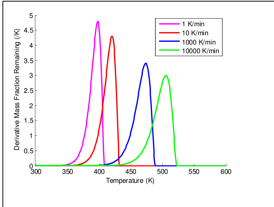
Figure 4.24: Simulated DTG curves for a shrinking core reaction at different heating rates simulated using \Psi^{s,c}
