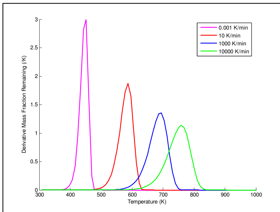
Figure 4.2: Simulated DTG curves for pyrolysis with a single, first-order reaction at different heating rates
