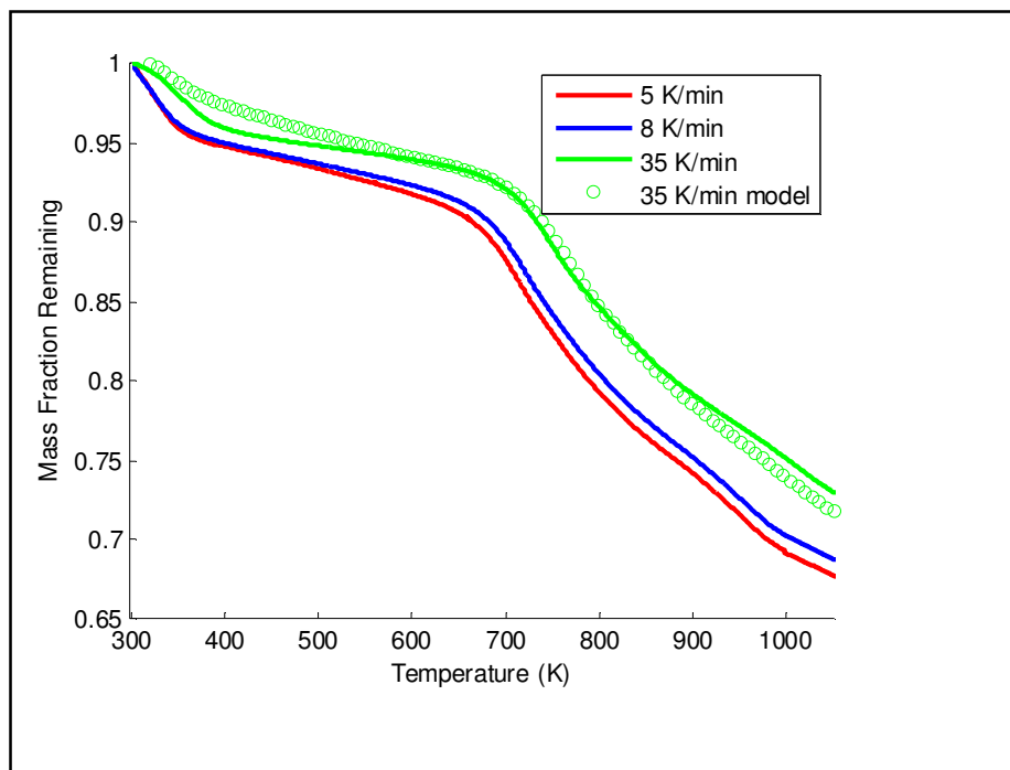
Figure 5.21: Comparison of model curve to experimental curve for 35 K/min using parameters obtained from lower heating rate data
