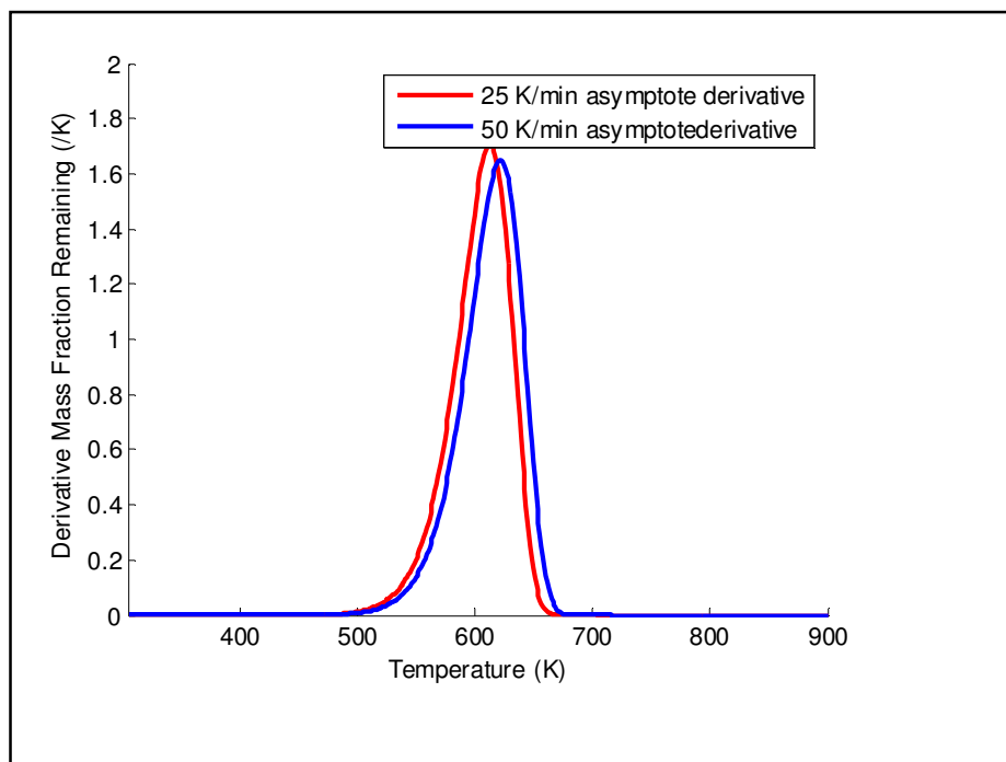
Figure 4.13: Simulated DTG curves for pyrolysis with a single, first-order reaction at variable heating rates
