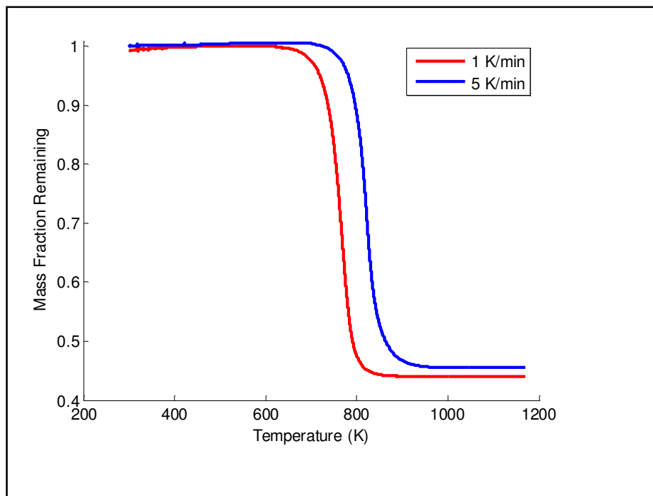
Figure 6.12: TGA curves for the combustion of a South African char at different heating rates in a TA Instruments Q600 TGA
