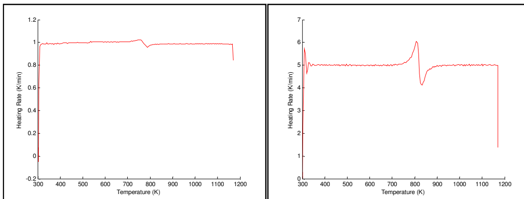
Figure 6.15: Actual heating rates of the samples for char combustion in a TA Instruments Q600 TGA
