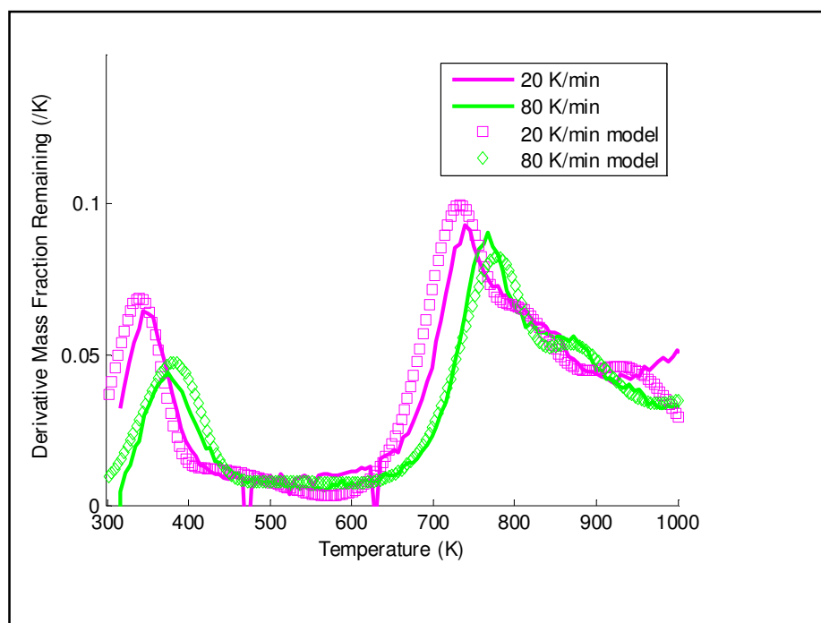
Figure 5.6: DTG curves for coal pyrolysis at heating rates of 20 K/min and 80 K/min with DAEM predictions for each heating rate
