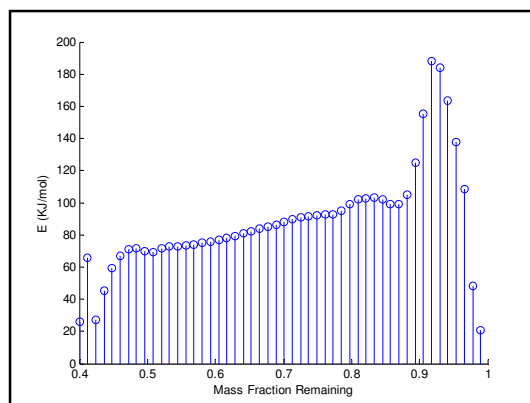
Figure 6.7: Kinetic parameters calculated for char combustion using instantaneous heating rates (a) Initial mass fraction of each component (b) Activation Energy of each reaction
