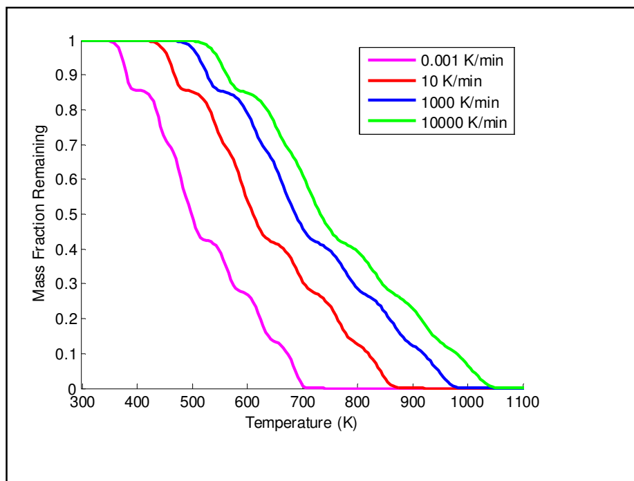
Figure 4.6: Simulated TGA curves for pyrolysis with seven first order reactions at different heating rates
