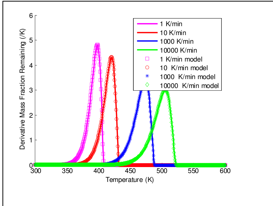
Figure 4.27: Simulated DTG curves for a shrinking core reaction at different heating rates simulated using \Psi^{s,c} , with model predictions for each of these heating rates
