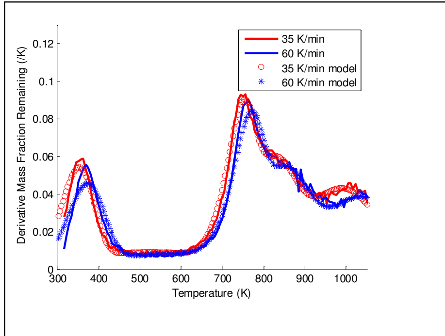
Figure 5.10: DTG curves for coal pyrolysis at heating rates of 35 K/min and 60 K/min with DAEM predictions using parameters calculated from instantaneous heating rates
