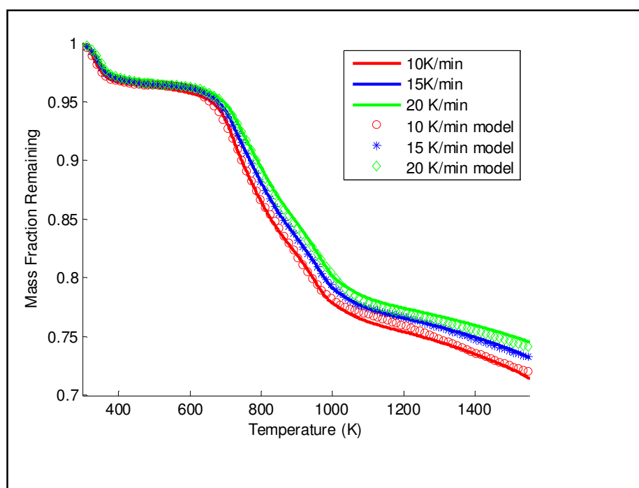
Figure 5.26: TGA curves for the pyrolysis of South African coal at different heating rates in a TA Instruments Q600 TGA, with DAEM predictions for each heating rate
