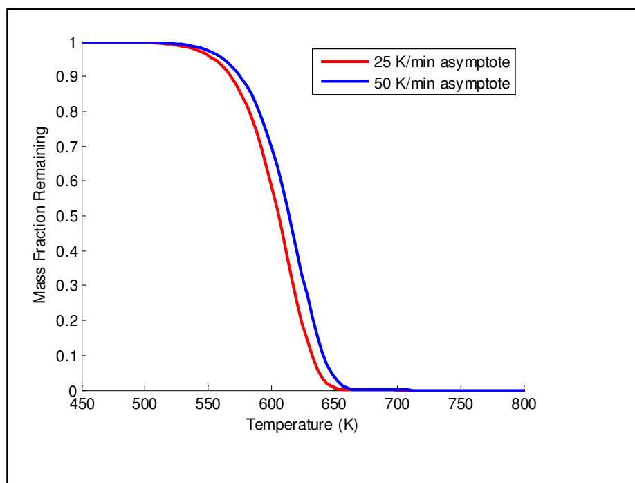
Figure 4.12: Simulated TGA curves for pyrolysis with a single, first-order reaction at variable heating rates
