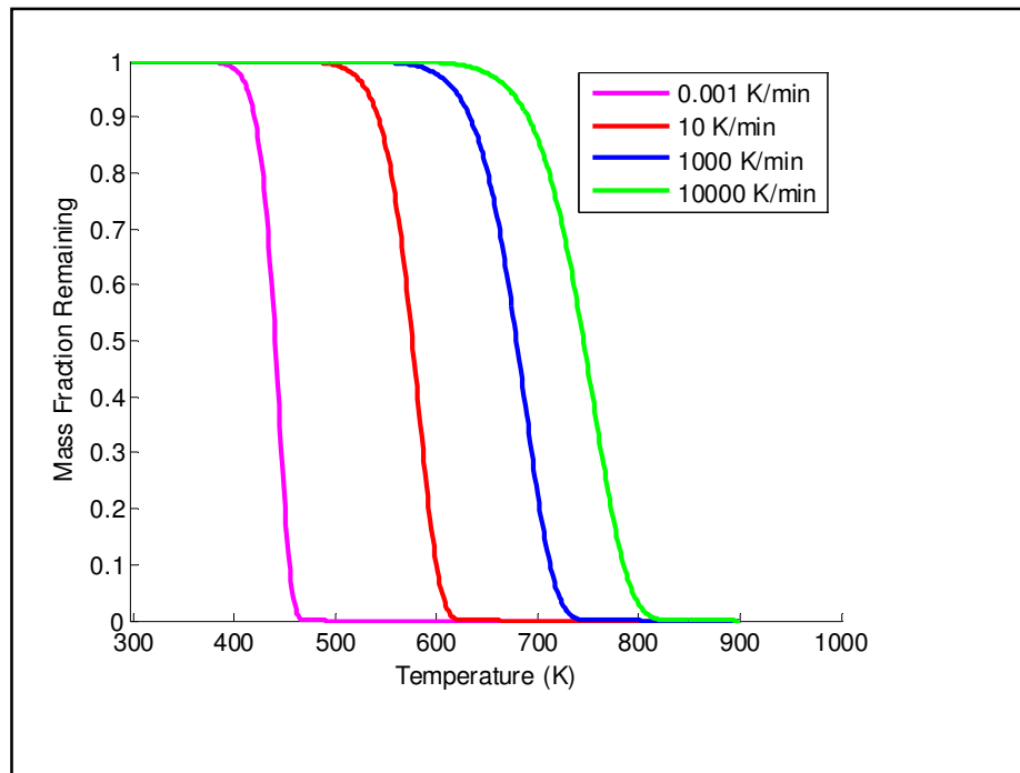
Figure 4.1: Simulated TGA curves for pyrolysis with a single, first-order reaction at different heating rates
