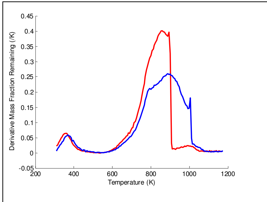
Figure 6.9: DTG curves for the combustion of a South African coal at two different heating rates in a Perkin-Elmer STA600 TGA
