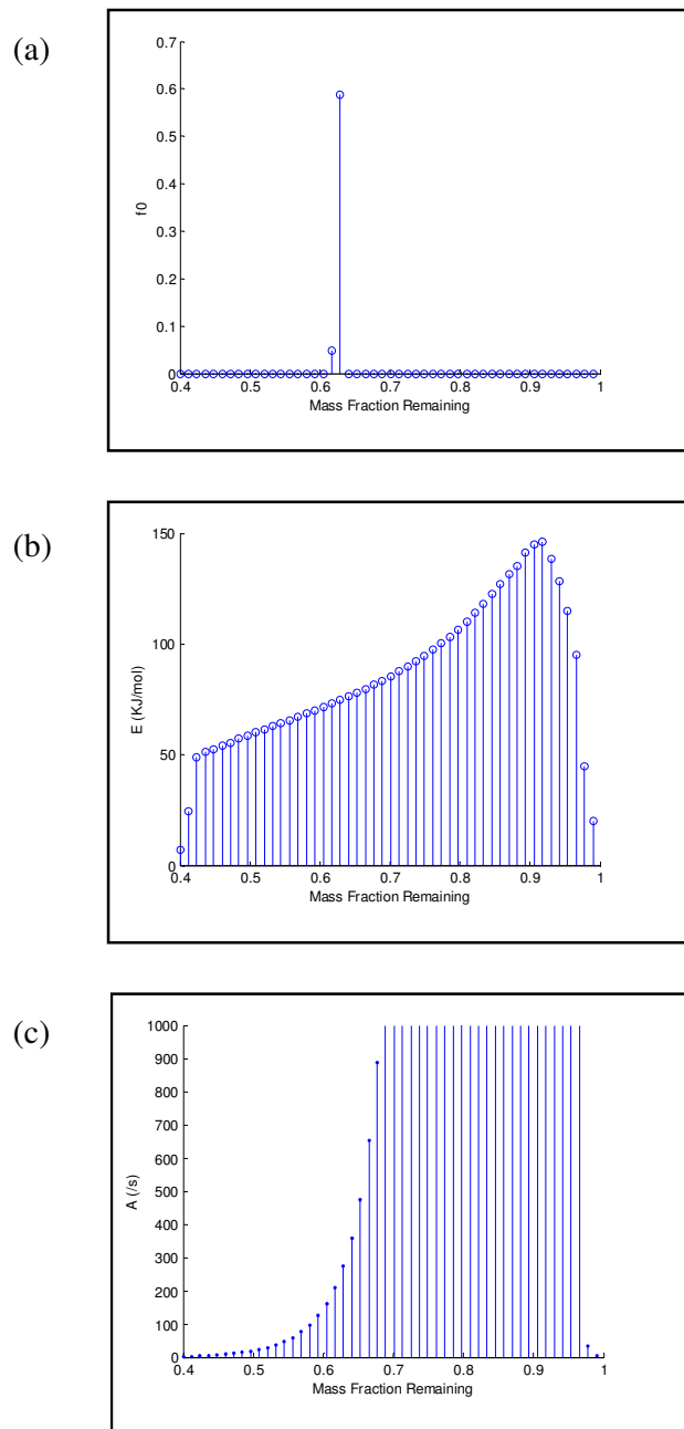
Figure 6.3: Kinetic parameters calculated for char combustion (a) Initial mass fraction of each component (b) Activation Energy of each reaction (c)Pre-exponential factor of each reaction
