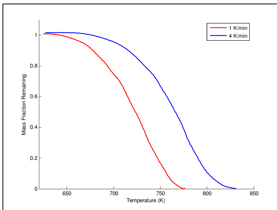
Figure 4.28: TGA curves for char combustion in air reported by Njapha (2003)
