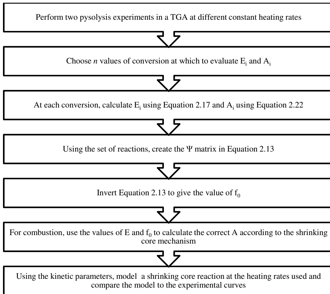
Figure 3.3: Flow Diagram of algorithm steps (Scott et al. , 2006)
