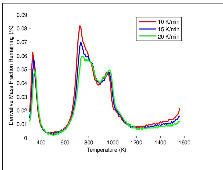
Figure 5.23: DTG curves for the pyrolysis of South African coal at different heating rates in a TA Instruments Q600 TGA
