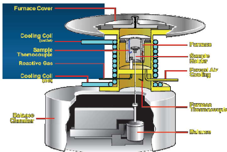
Figure 3.1: Schematic diagram of Perkin-Elmer STA 600 TGA (courtesy of Perkin-Elmer)
