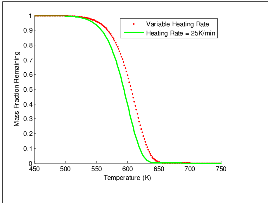
Figure 4.14: Simulated TGA curves for pyrolysis with a single, first order reaction at a variable heating rate and constant heating rate of 25 K/min
