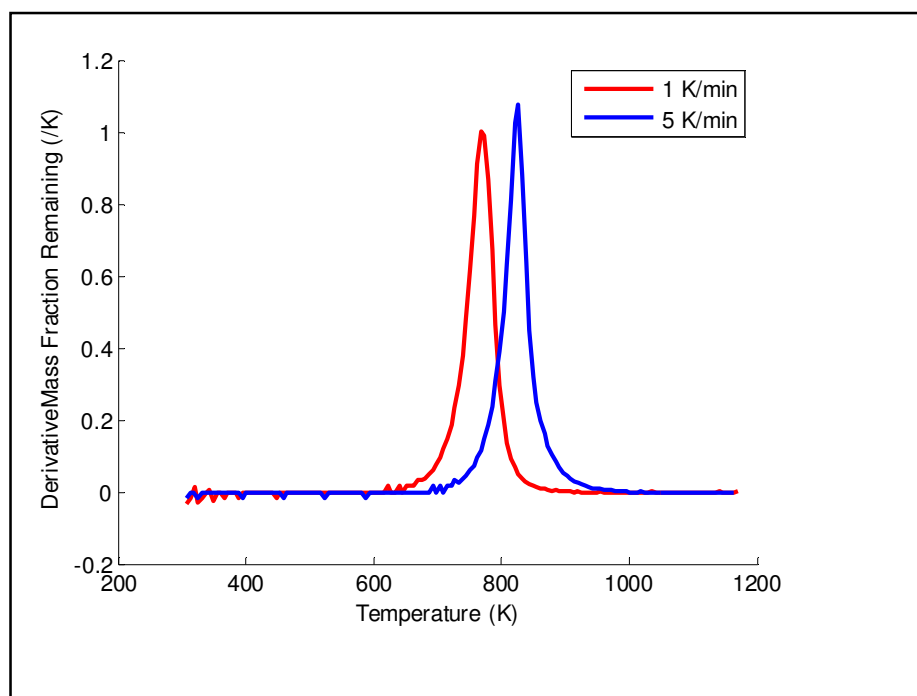
Figure 6.13: DTG curves for the combustion of a South African char at different heating rates in a TA Instruments Q600 TGA
