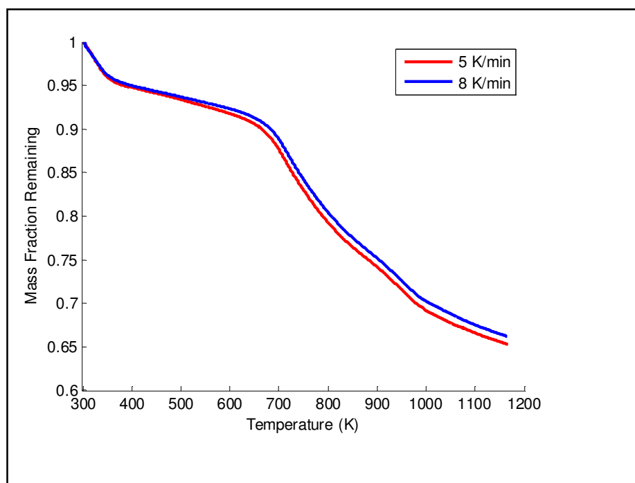
Figure 5.15: TGA curves for the pyrolysis of a South African coal at low heating rates
