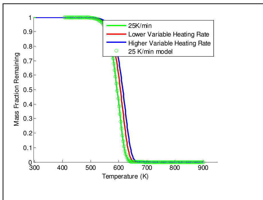
Figure 4.17: Simulated TGA curve pyrolysis with a single, first order reaction at a constant heating rate of 25 K/min, with a DAEM prediction using parameters calculated from variable heating rate curves
