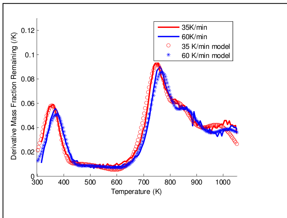
Figure 5.4: DTG curves for coal pyrolysis at heating rates of 35 K/min and 60 K/min, with DAEM predictions for each heating rate
