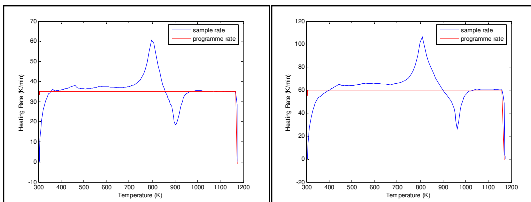
Figure 6.6: Comparison of programme heating rates and actual heating rates of the samples for char combustion in a Perkin Elmer STA600 TGA
