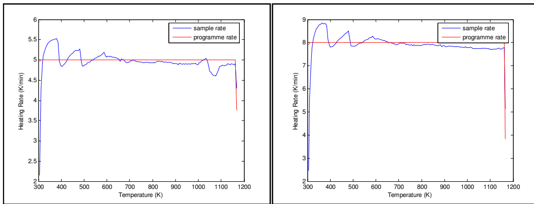
Figure 5.18: Comparison of programme heating rates and actual heating rates of the samples for coal pyrolysis at lower heating rates in a Perkin Elmer STA600 TGA
