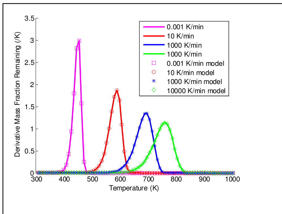
Figure 4.5: Simulated DTG curves for pyrolysis with a single, first order reaction at different heating rates, with DAEM predictions for each of these heating rates
