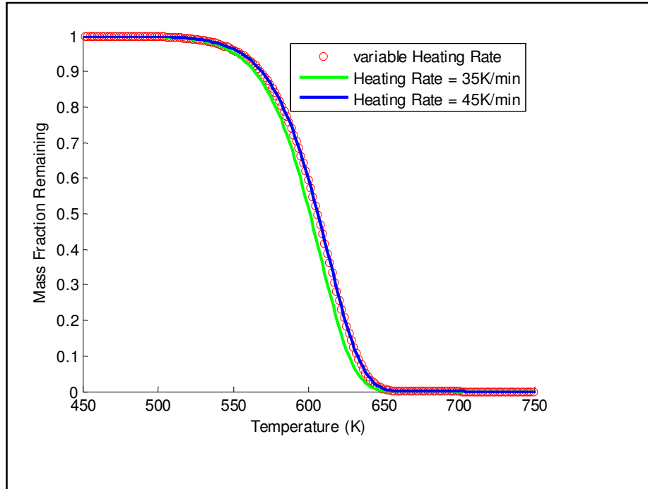
Figure 4.15: Simulated TGA curves for pyrolysis with a single, first order reaction at a variable heating rate and constant heating rates of 35 K/min and 45 K/min
