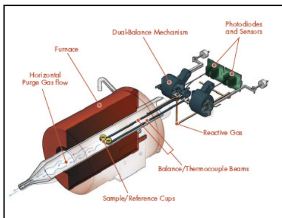
Figure 3.2: TA Instruments Q600 TGA balance and furnace (courtesy of TA Instruments)
