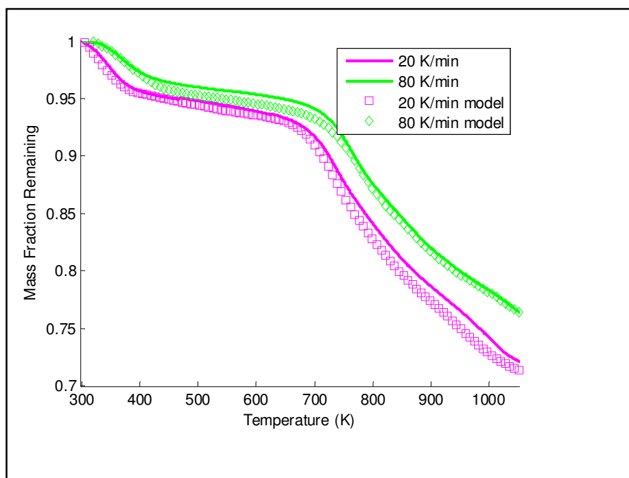
Figure 5.11: TGA curves for coal pyrolysis at heating rates of 20 K/min and 80 K/min with DAEM predictions using parameters calculated from instantaneous heating rates
