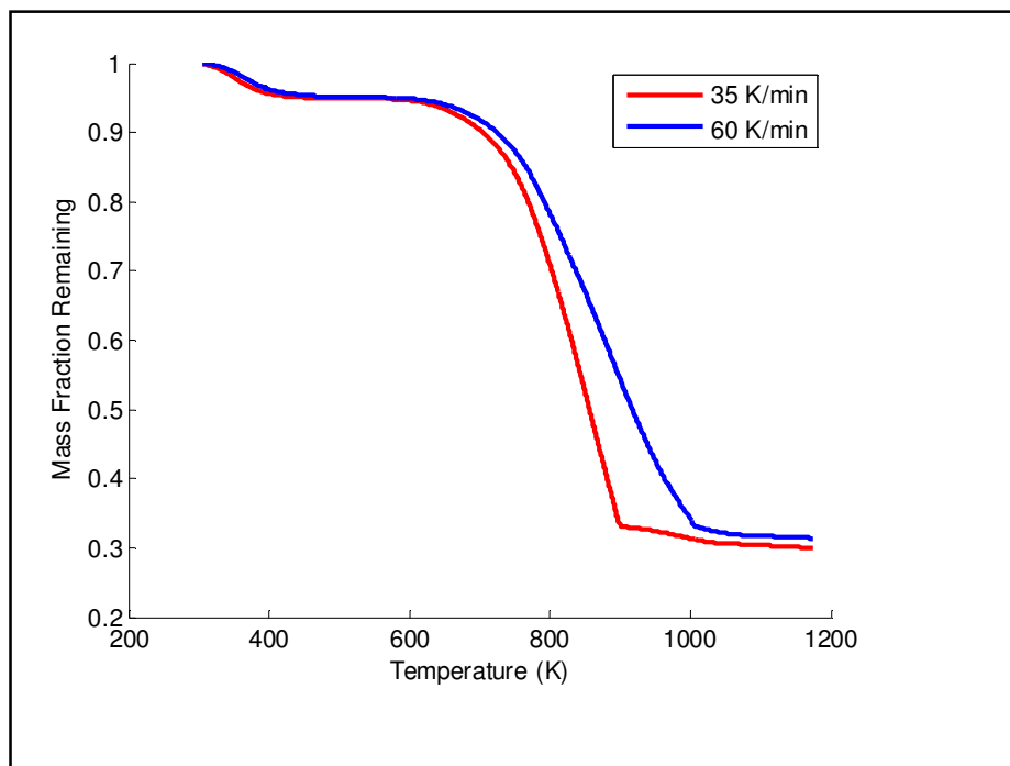
Figure 6.8: TGA curves for the combustion of a South African coal at two different heating rates in a Perkin-Elmer STA600 TGA
