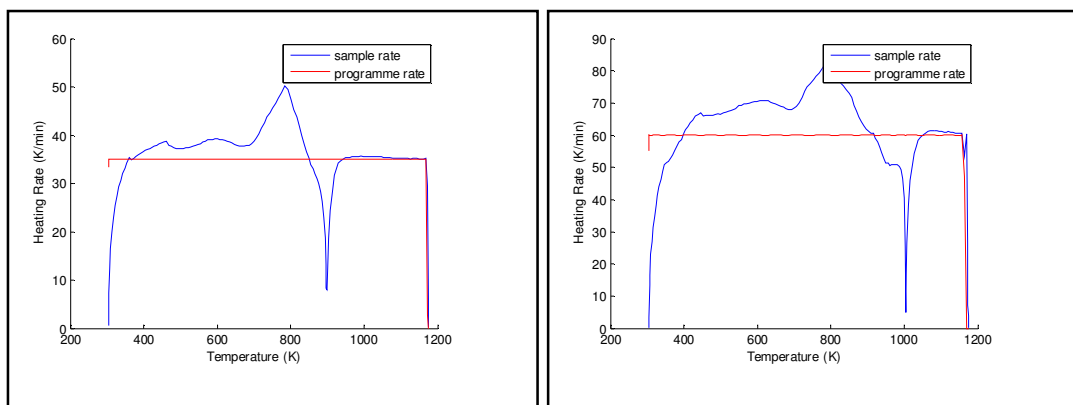
Figure 6.11: Comparison of programme heating rates and actual heating rates of the samples for coal combustion in a Perkin Elmer STA600 TGA
