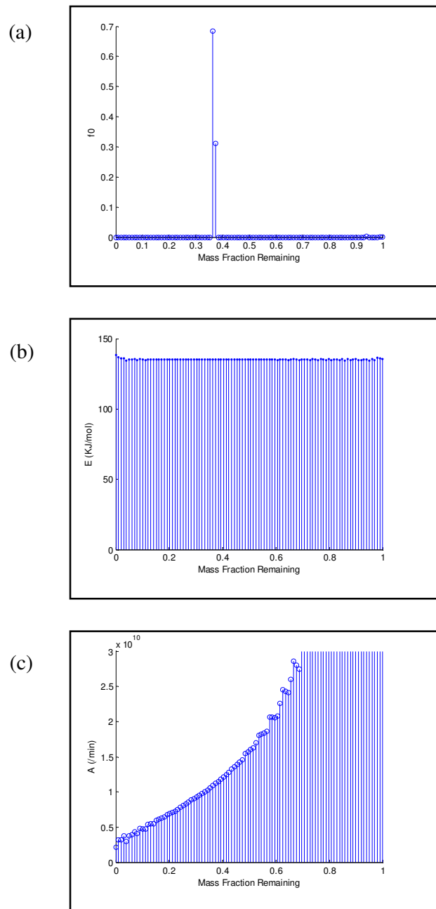
Figure 4.16: Kinetic parameters calculated for simulated single first-order reaction with variable heating rates (a) Initial mass fraction of each component (b) Activation Energy of each reaction (c) Pre-exponential factor of each reaction
