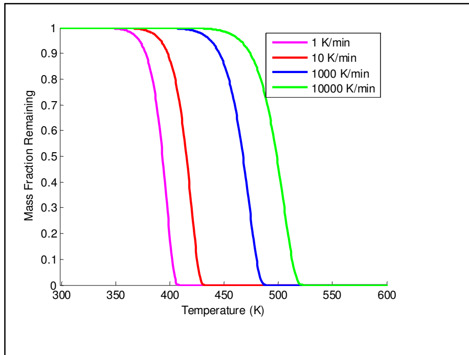
Figure 4.23: Simulated TGA curves for a shrinking core reaction at different heating rates simulated using \Psi^{s.c.}
