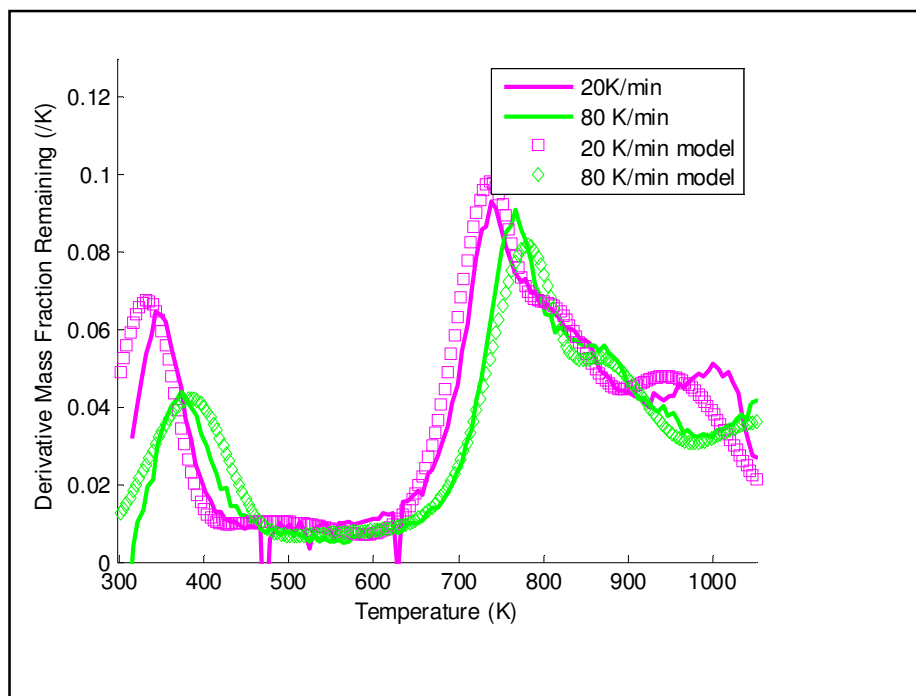
Figure 5.12: DTG curves for coal pyrolysis at heating rates of 20 K/min and 80 K/min with DAEM predictions using parameters calculated from instantaneous heating rates
