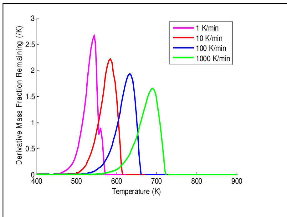
Figure 4.19: Simulated DTG curves for a shrinking core reaction at different heating rates simulated using ode45 solver
