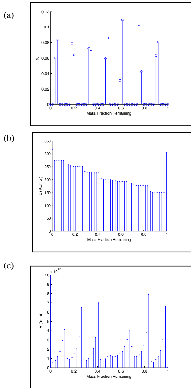
Figure 4.8: Kinetic parameters calculated for seven simulated first-order reactions (a) Initial mass fraction of each component (b) Activation Energy of each reaction (c) Pre-exponential factor of each reaction
