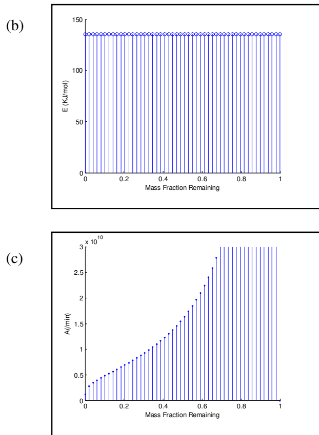
Figure 4.3: Kinetic parameters calculated for simulated single, first-order reaction (a) Initial mass fraction of each component (b) Activation Energy of each reaction (c) Pre-exponential factor of each reaction
