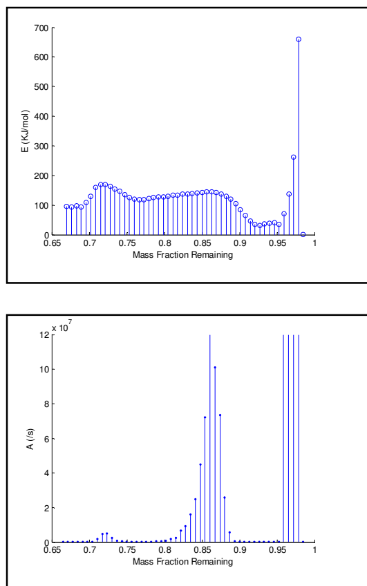
Figure 5.17: Kinetic Parameters calculated for coal pyrolysis at lower heating rates (a) Initial mass fraction of each component (b) Activation Energy of each reaction (c) Pre-exponential factor of each reaction
