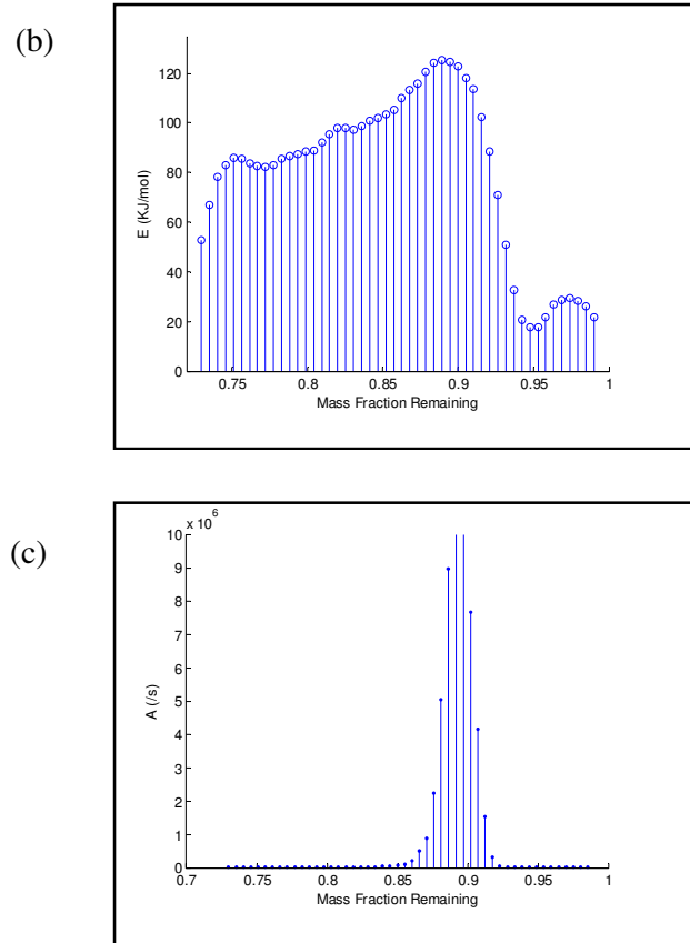
Figure 5.2: Kinetic parameters calculated for coal pyrolysis (a) Initial mass fraction of each component (b) Activation Energy of each reaction (c) Pre-exponential factor of each reaction
