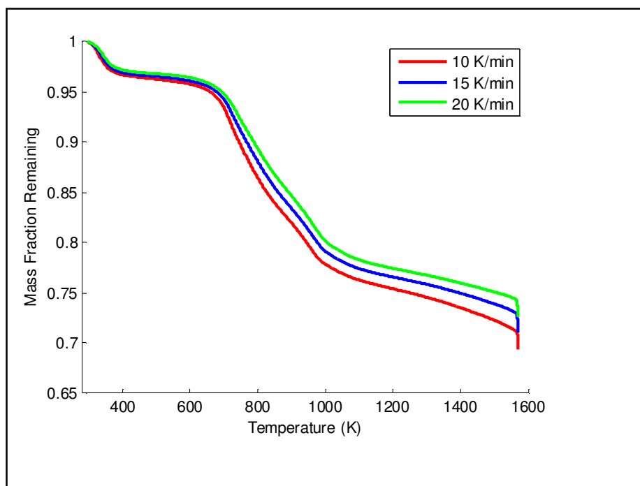
Figure 5.22: TGA curves for the pyrolysis of South African coal at different heating rates in a TA Instruments Q600 TGA
