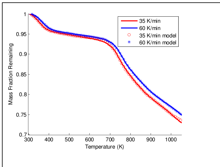
Figure 5.3: TGA curves for coal pyrolysis at heating rates of 35 K/min and 60 K/min, with DAEM predictions for each heating rate
