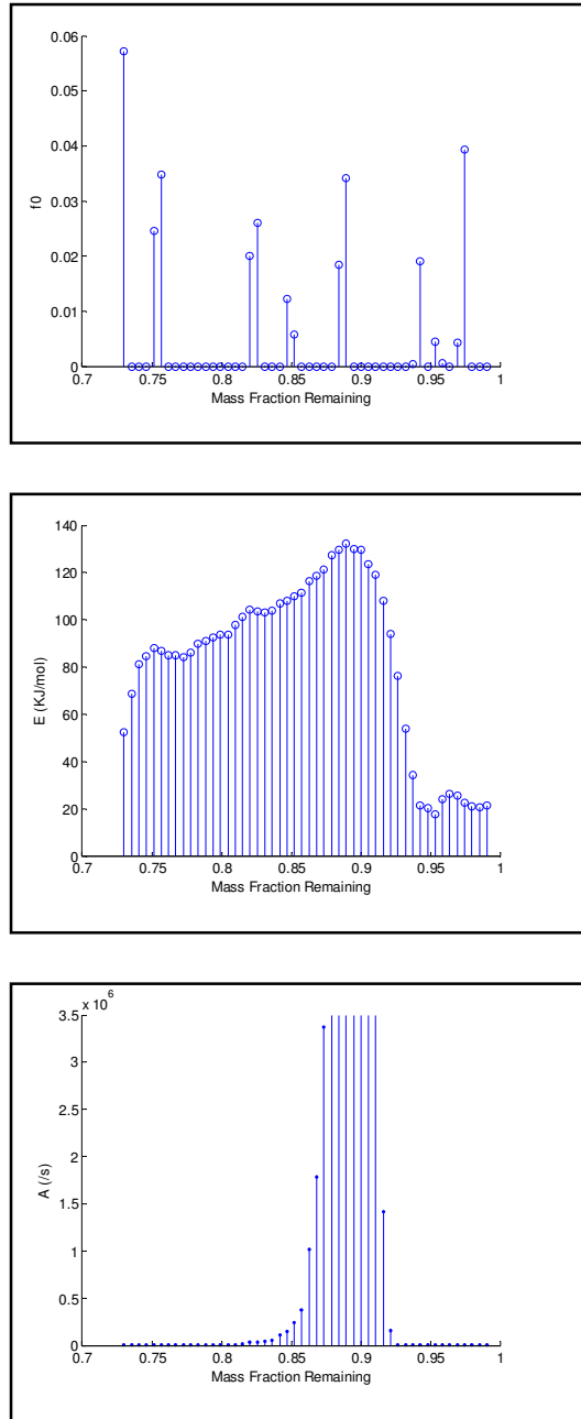
Figure 5.8: Kinetic parameters calculated for coal pyrolysis using instantaneous heating rates (a) Initial mass fraction of each component (b) Activation Energy of each reaction (c) Pre-exponential factor of each reaction
