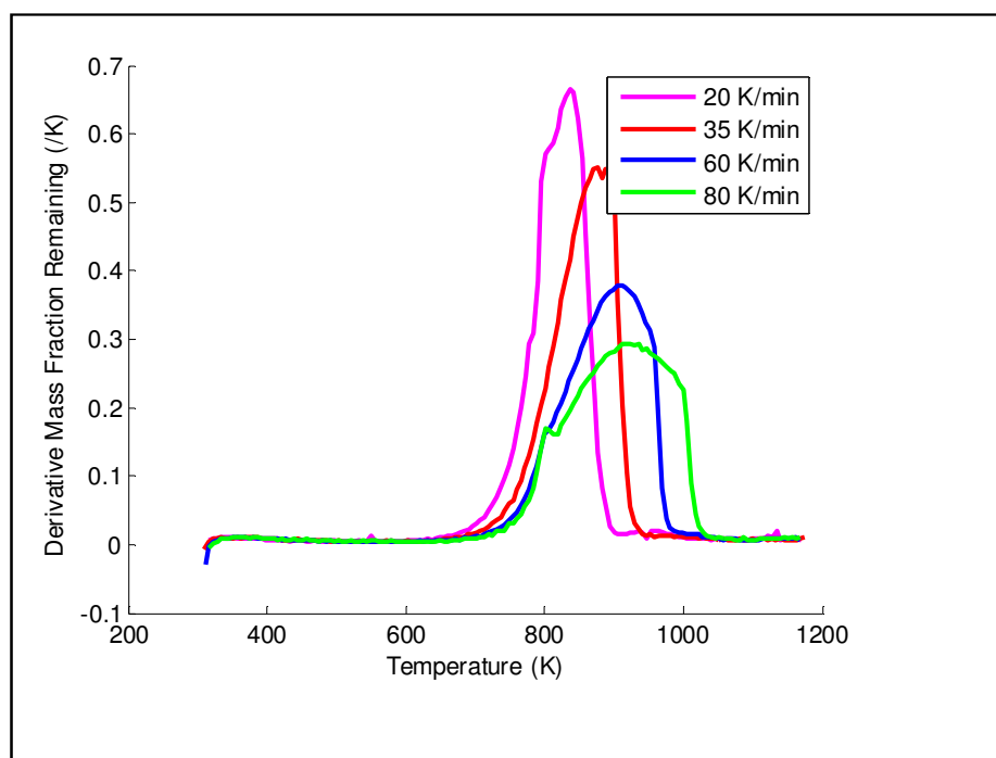
Figure 6.2: DTG curves for the combustion of a South African char at different heating rates in a Perkin-Elmer STA600 TGA
