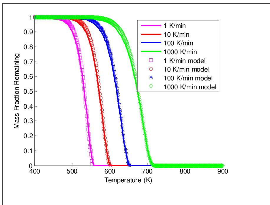
Figure 4.21: Simulated TGA curves for a shrinking core reaction at different heating rates simulated using ode45 solver, with model predictions for each of these heating rates
