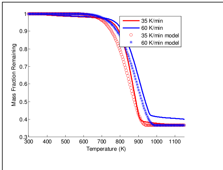
Figure 6.5: TGA curves for the combustion of a South African char at heating rates of 35 K/min and 60 K/min, with shrinking core model predictions for each heating rate
