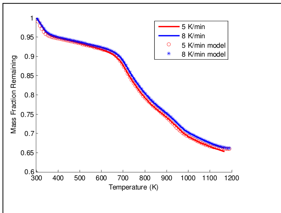
Figure 5.19: TGA curves for coal pyrolysis at heating rates of 5 K/min and 8 K/min with DAEM predictions for each heating rate
