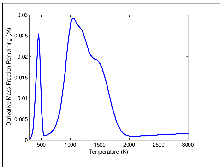
Figure 5.29: DAEM prediction of a DTG curve for a heating rate of 10 000 K/min
