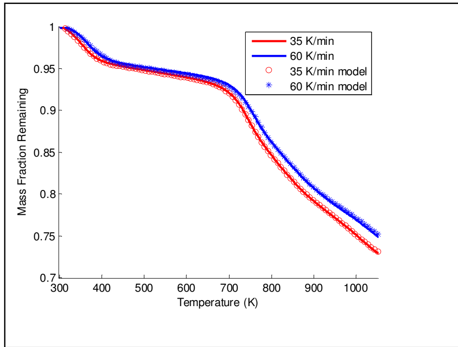
Figure 5.9: TGA curves for coal pyrolysis at heating rates of 35 K/min and 60 K/min with DAEM predictions using parameters calculated from instantaneous heating rates
