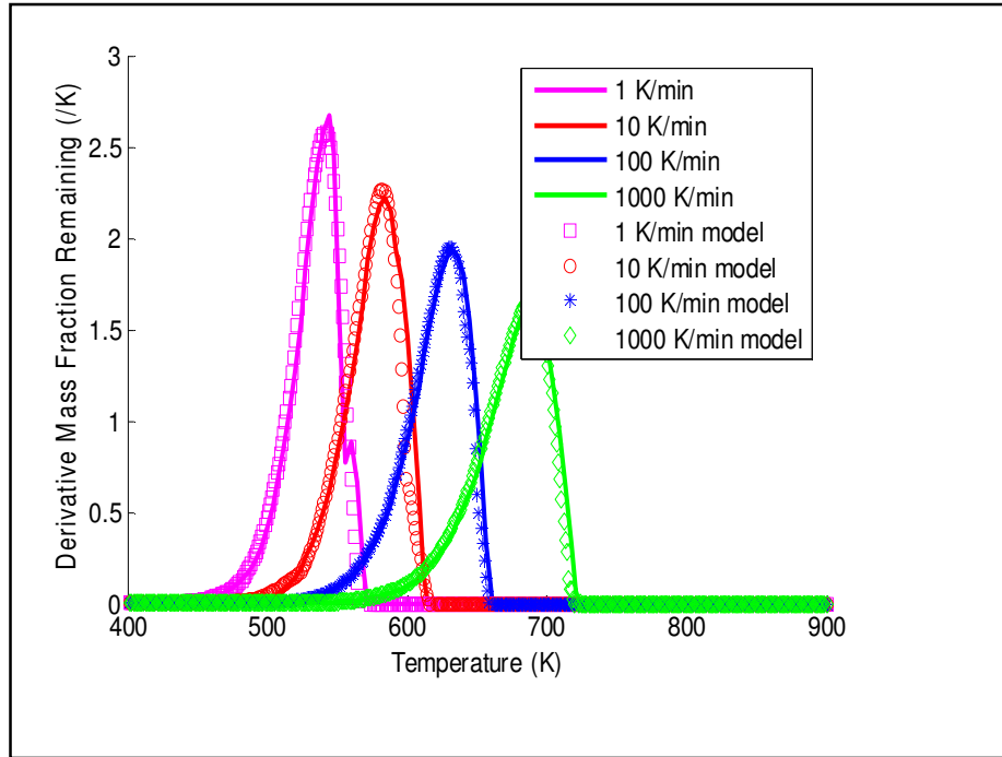
Figure 4.22: Simulated DTG curves for a shrinking core reaction at different heating rates simulated using ode45 solver, with model predictions for each of these heating rates
