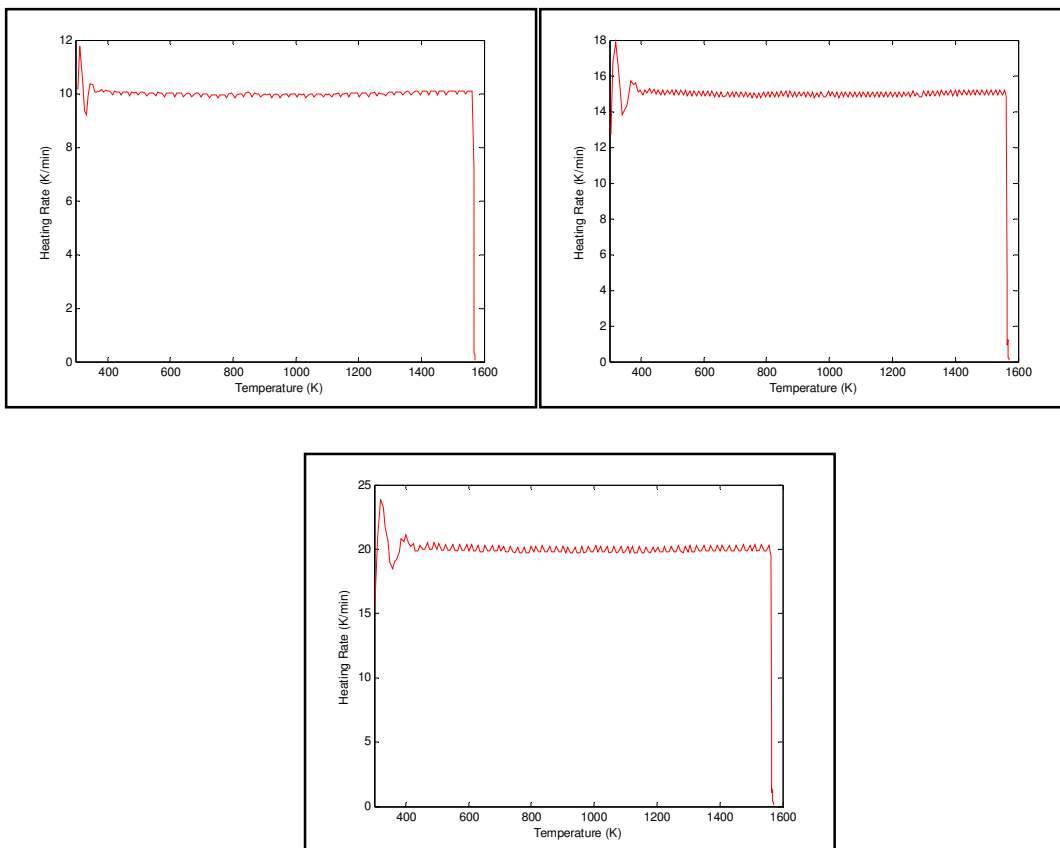
Figure 5.25: Actual heating rates of the samples for coal pyrolysis in a TA instruments Q600 TGA
