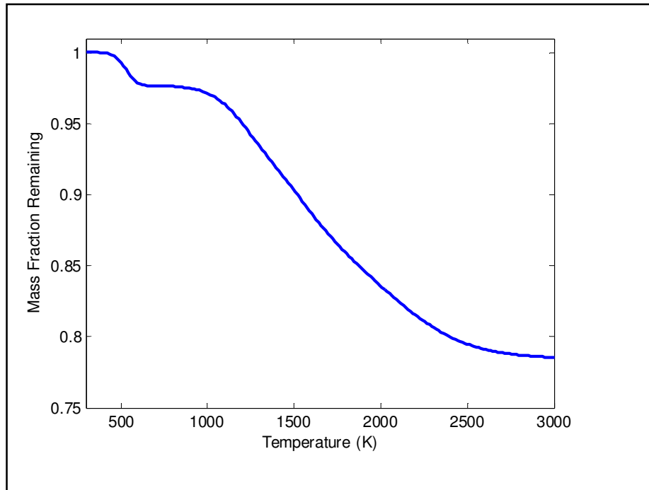
Figure 5.28: DAEM prediction of a TGA curve for a heating rate of 10 000 K/min
