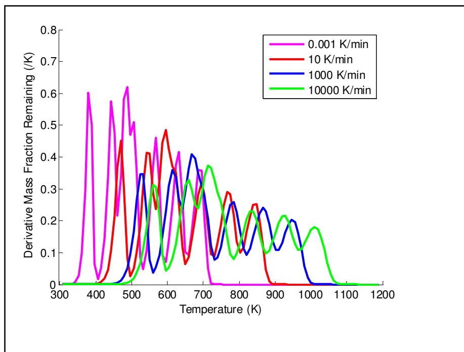
Figure 4.7: Simulated DTG curves for pyrolysis with seven first order reactions at different heating rates
