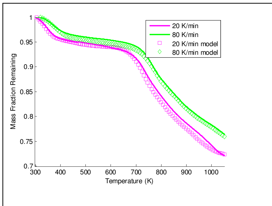
Figure 5.5: TGA curves for coal pyrolysis at heating rates of 20 K/min and 80 K/min with DAEM predictions for each heating rate
