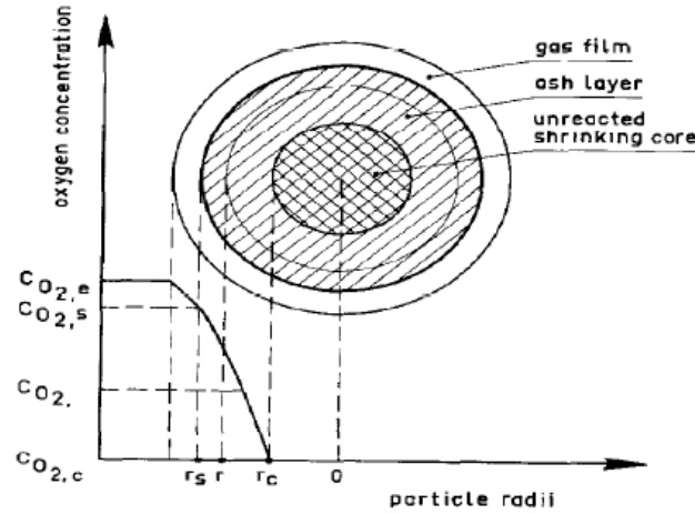
Figure 2.1: Schematic representation of a particle undergoing combustion (Abdel-Hafez, 1988)
