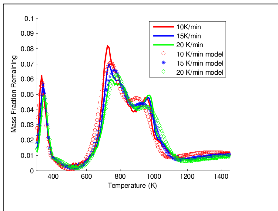
Figure 5.27: DTG curves for the pyrolysis of South African coal at different heating rates in a TA Instruments Q600 TGA, with DAEM predictions for each heating rate
