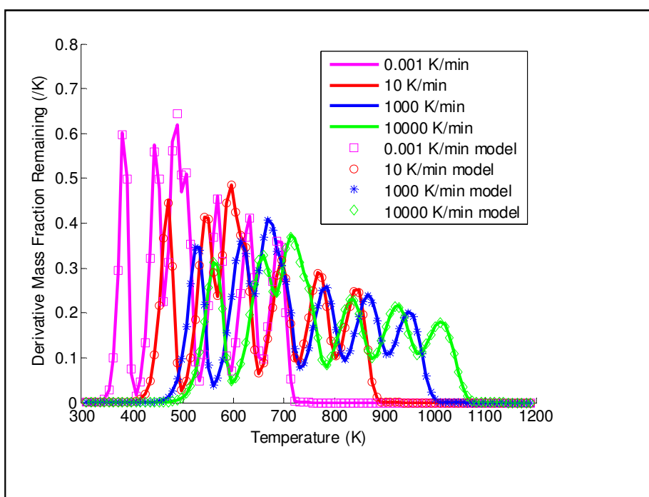
Figure 4.10: Simulated DTG curves for seven first order reactions at different heating rates, with DAEM predictions for each of these heating rates
