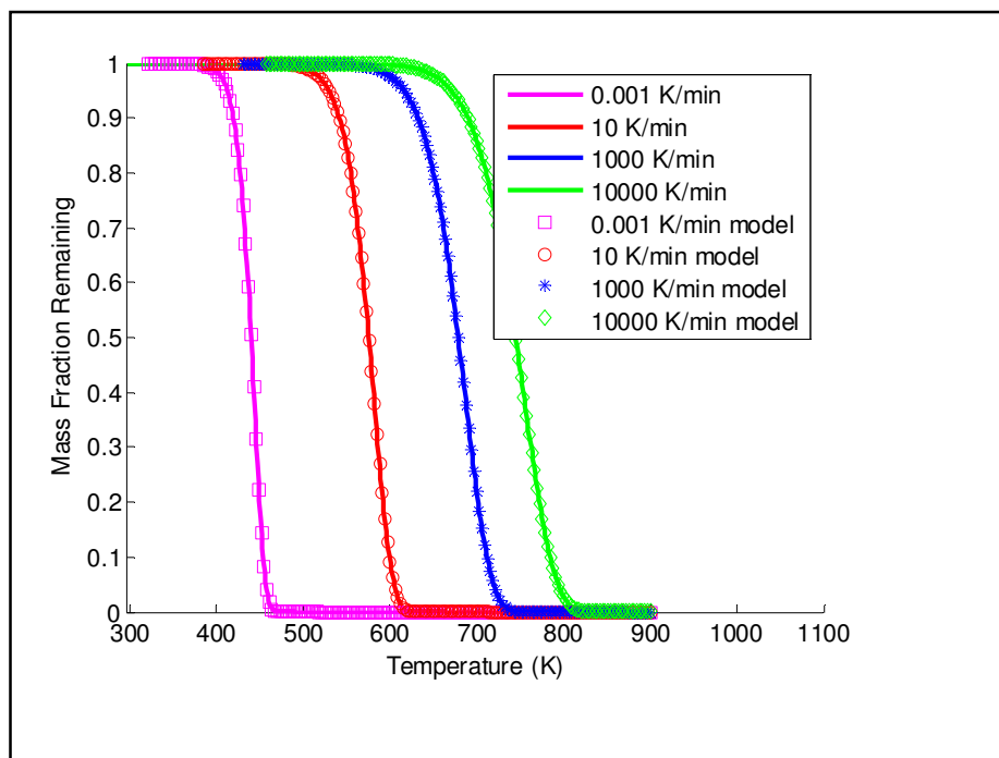
Figure 4.4: Simulated TGA curves for pyrolysis with a single, first-order reaction at different heating rates, with DAEM predictions for each of these heating rates
