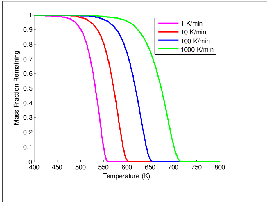
Figure 4.18: Simulated TGA curves for a shrinking core reaction at different heating rates simulated using ode45 solver
