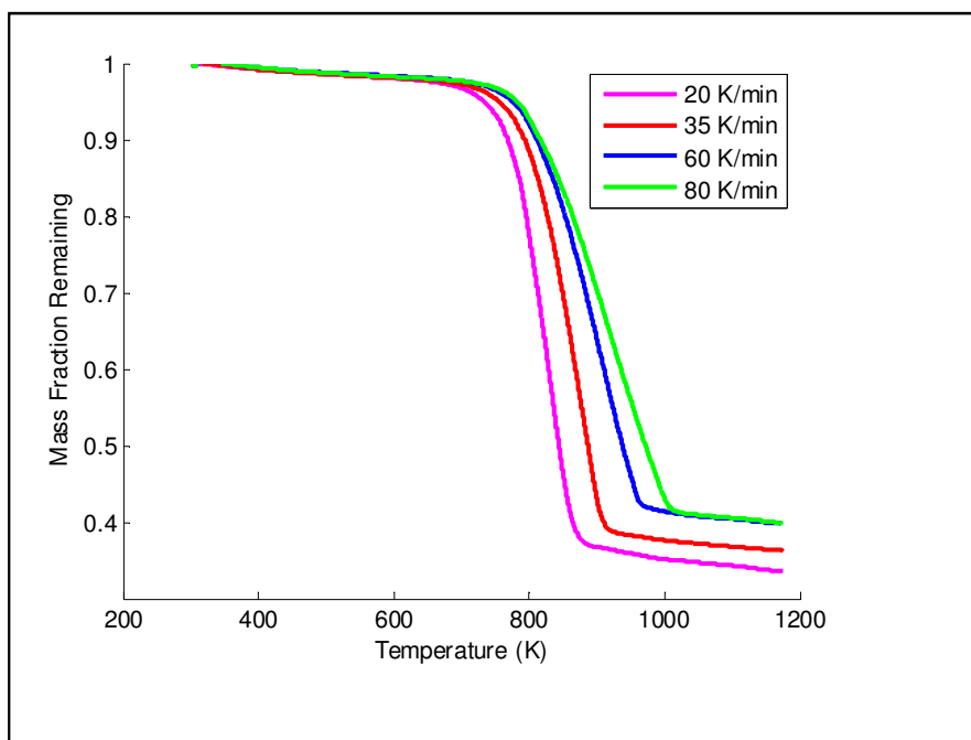
Figure 6.1: TGA curves for the combustion of a South African char at different heating rates in a Perkin-Elmer STA600 TGA
