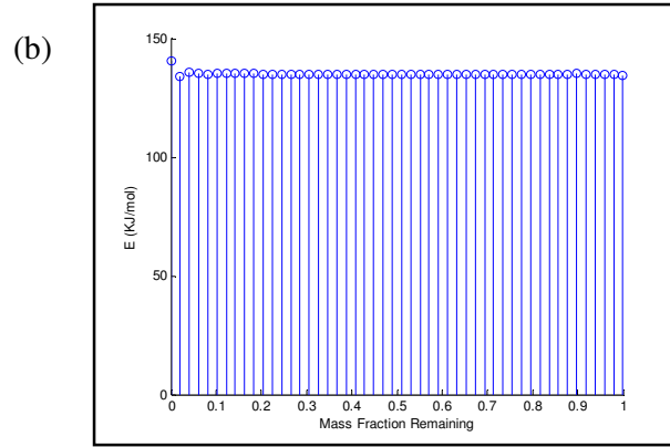
Figure 4.25: Kinetic parameters calculated for a simulated shrinking core reaction using \Psi^{s.c} (a) Initial mass fraction of each component (b) Activation Energy of each reaction
