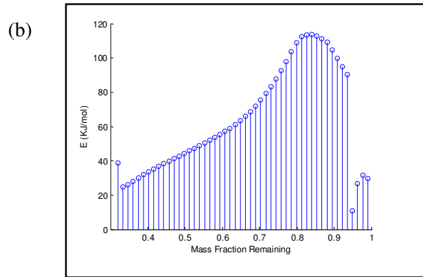
Figure 6.10: Kinetic parameters calculated for coal combustion (a) Initial mass fraction of each component (b) Activation Energy of each reaction
