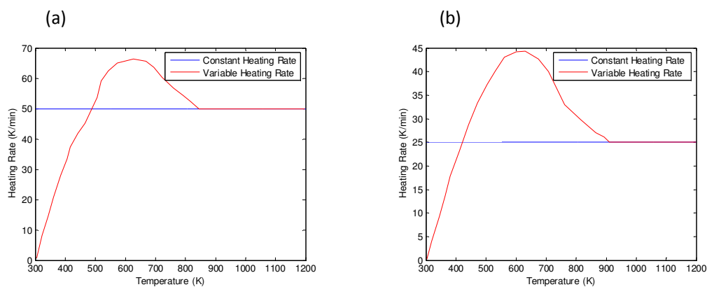
Figure 4.11: Heating rates vs. temperature profiles used for simulation of TGA data
