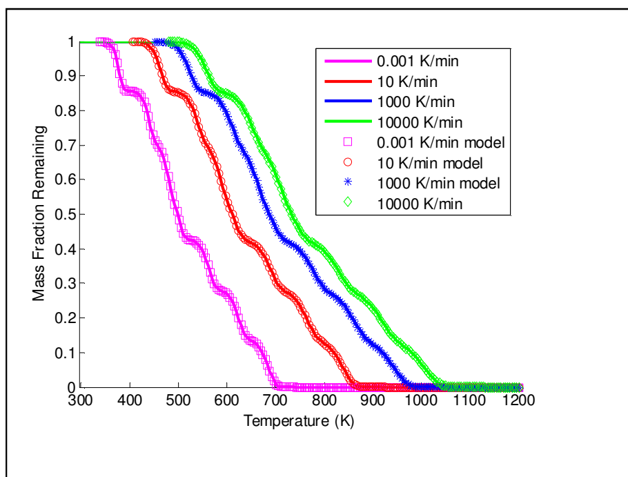
Figure 4.9: Simulated TGA curves for seven first-order reactions at different heating rates, with DAEM predictions for each of these heating rates
