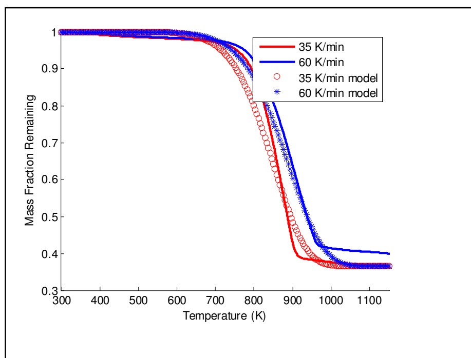
Figure 6.4: TGA curves for the combustion of a South African char at heating rates of 35 K/min and 60 K/min, with DAEM predictions for each heating rate
