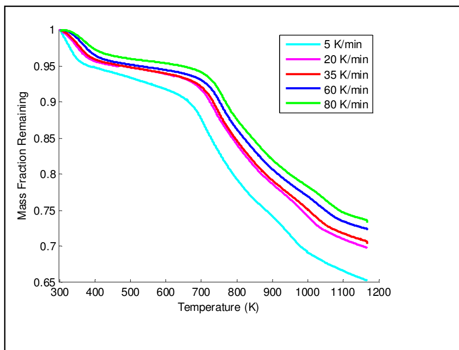
Figure 5.1: TGA curves for the pyrolysis of a South African coal at different heating rates in a Perkin-Elmer STA600 TGA
