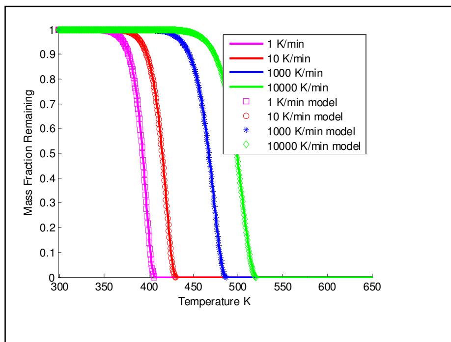
Figure 4.26: Simulated TGA curves for a shrinking core reaction at different heating rates simulated using \Psi^{s,c} , with model predictions for each of these heating rates
