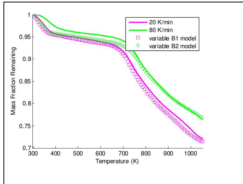
Figure 5.13 (b): TGA curves for coal pyrolysis at heating rates of 20 K/min and 80 K/min with DAEM predictions for actual heating rate profiles using parameters calculated from instantaneous heating rates
