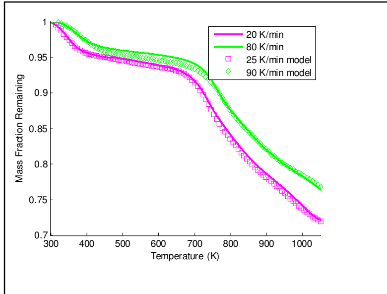
Figure 5.13 (a): TGA curves for coal pyrolysis at heating rates of 20 K/min and 80 K/min with DAEM predictions for constant heating rates of 25 K/min and 90 K/min using parameters calculated from instantaneous heating rates
