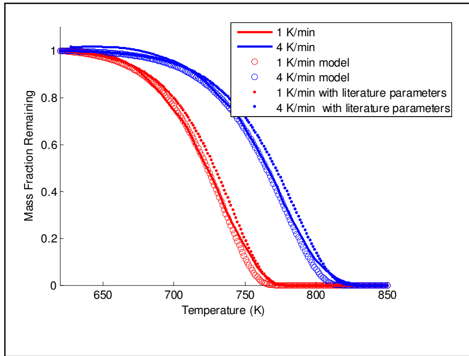
Figure 4.29: TGA curves for char combustion in air reported by Njapha (2003) with model predictions using calculated parameters and parameters reported by Njapha (2003)
