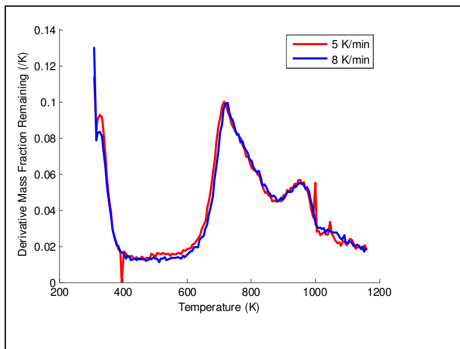
Figure 5.16: DTG curves for the pyrolysis of a South African coal at low heating rates
