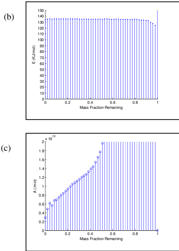
Figure 4.20: Kinetic parameters calculated for a simulated shrinking core reaction using ode45 solver (a) Initial mass fraction of each component (b) Activation Energy of each reaction (c) Pre-exponential factor of each reaction
