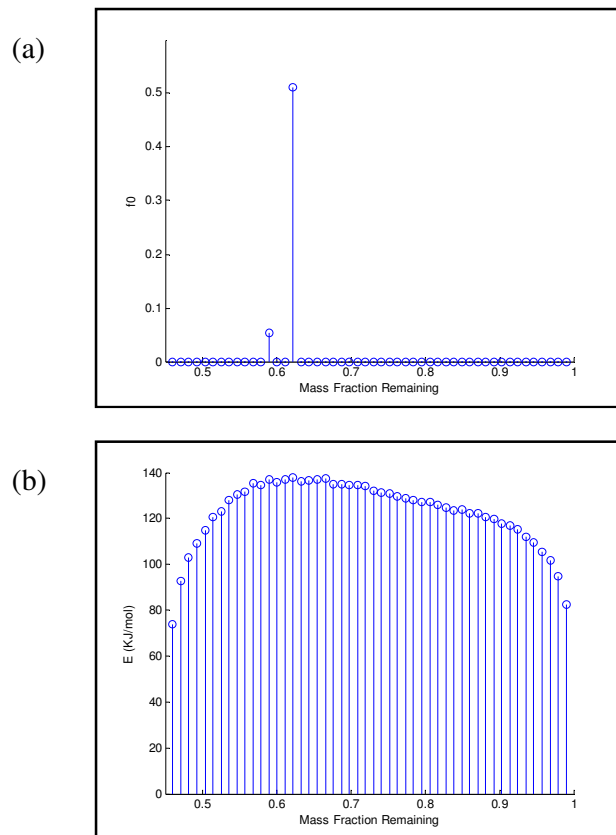
Figure 6.14: Kinetic parameters calculated for char combustion in a TA Instruments Q600 TGA (a) Initial mass fraction of each component (b) Activation Energy of each reaction
