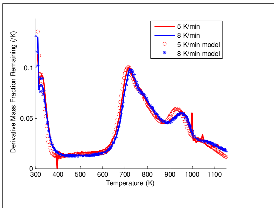
Figure 5.20: DTG curves for coal pyrolysis at heating rates of 5 K/min and 8 K/min with DAEM predictions for each heating rate
