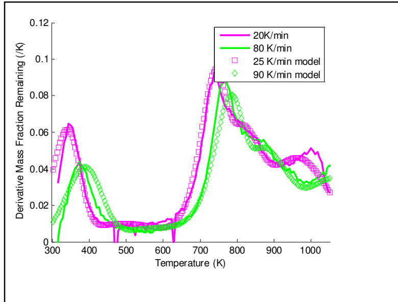
Figure 5.14 (a): DTG curves for coal pyrolysis at heating rates of 20 K/min and 80 K/min with DAEM predictions for constant heating rates of 25 K/min and 90 K/min using parameters calculated from instantaneous heating rates
