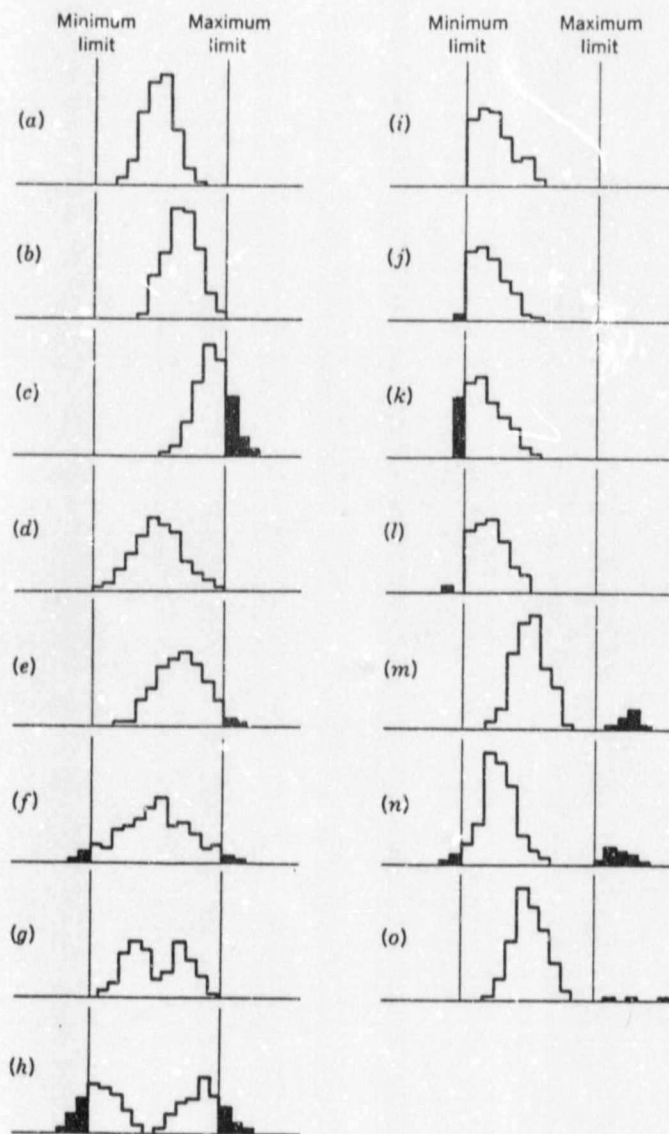
Figure 18. 15 Examples of Histograms Related to Tolerances
