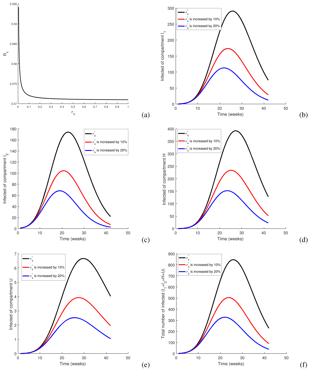
FIG. 8. Variation of \sigma_s . The influence of \sigma_s on \mathcal{R}_c ; I_1, I_2, H, U and (I_1 + I_2 + H + U) . (i) \sigma_s = \sigma_s^* ; (ii) \sigma_s^* is increased by 10%; (iii) \sigma_s^* is increased by 20%. The other parameters are those estimated in Sierra Leone.
