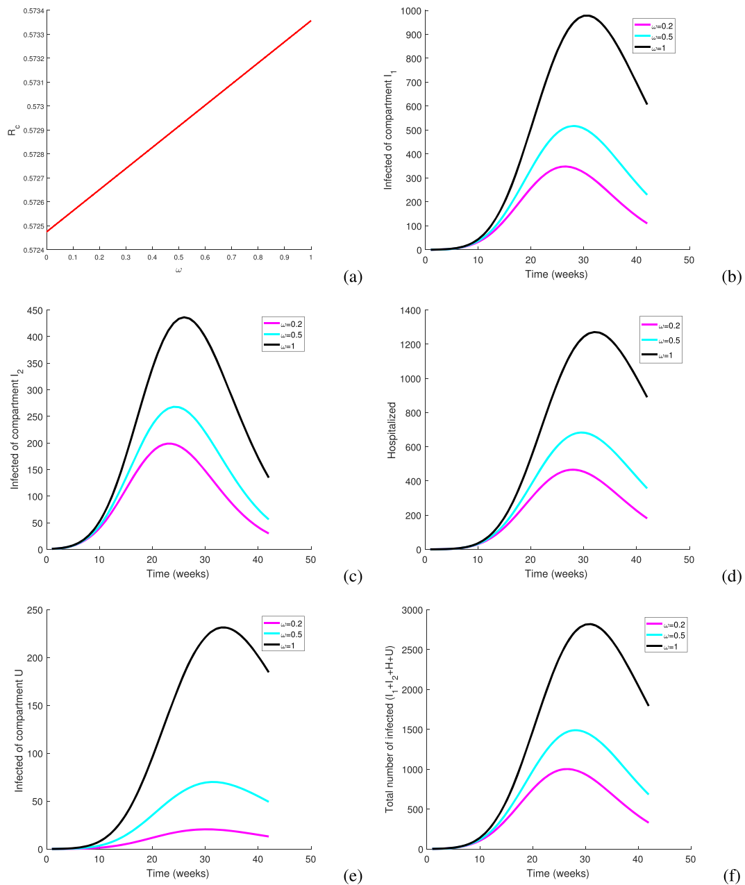
FIG. 4. Place of traditional medicine Figure 4 (a) shows a plot of R_c versus \omega . The rest are plots of the number of infected in compartments I_1 , I_2 , H , U and the infection curve, for (i) \omega = 1 ; (ii) \omega = 0.5 ; (iii) \omega = 0.2 . The other parameters for the simulations are those estimated for Sierra Leone.
