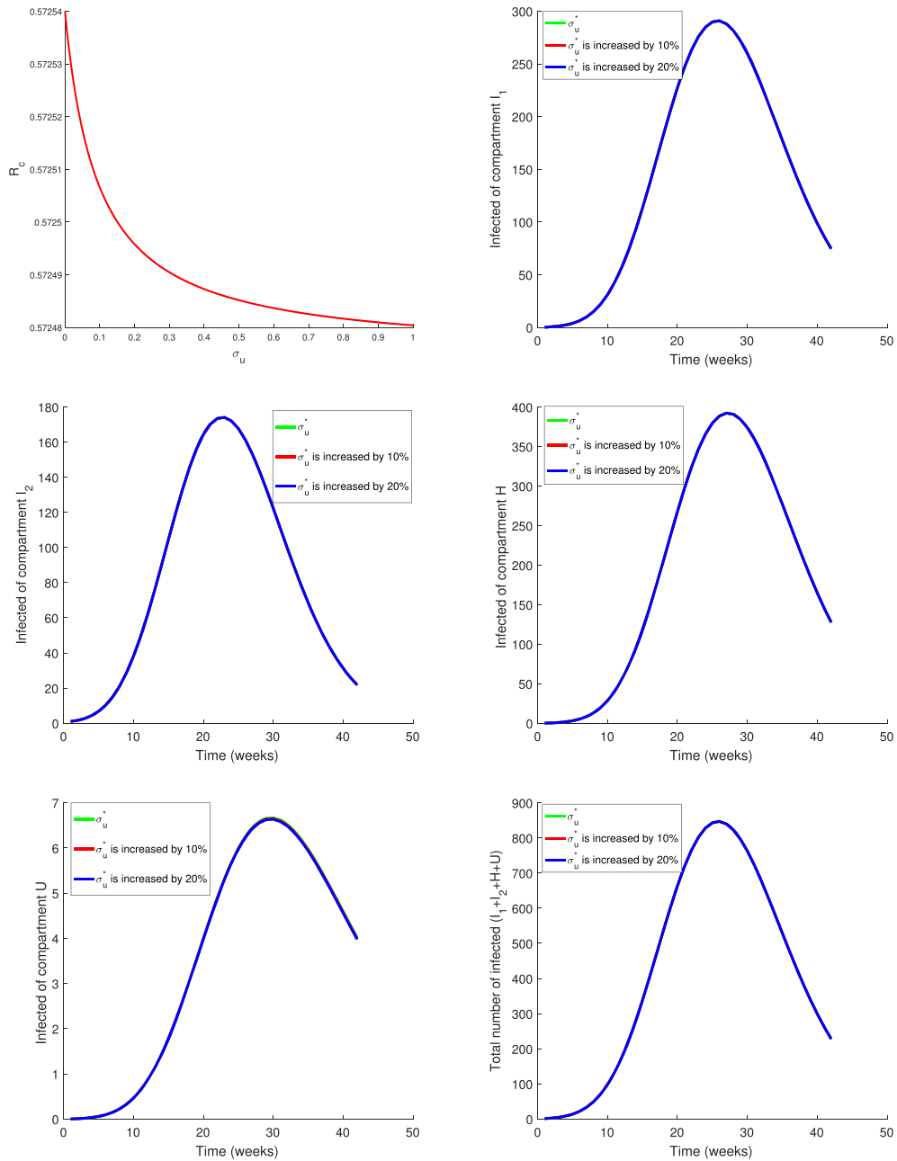
FIG. 6. Variation of \sigma_u Figure 6 (a) is a plot of \mathcal{R}_c versus \sigma_u . The rest are curves of the infected in compartments I_1 , I_2 , H , U as well as the total number of infected ( I_1 + I_2 + H + U ) when the parameter \sigma_u varies: (i) \sigma_u = \sigma_u^* ; (ii) \sigma_u^* is increased by 10%; (iii) \sigma_u^* is increased by 20%. The other parameters are those estimated in Sierra Leone.
