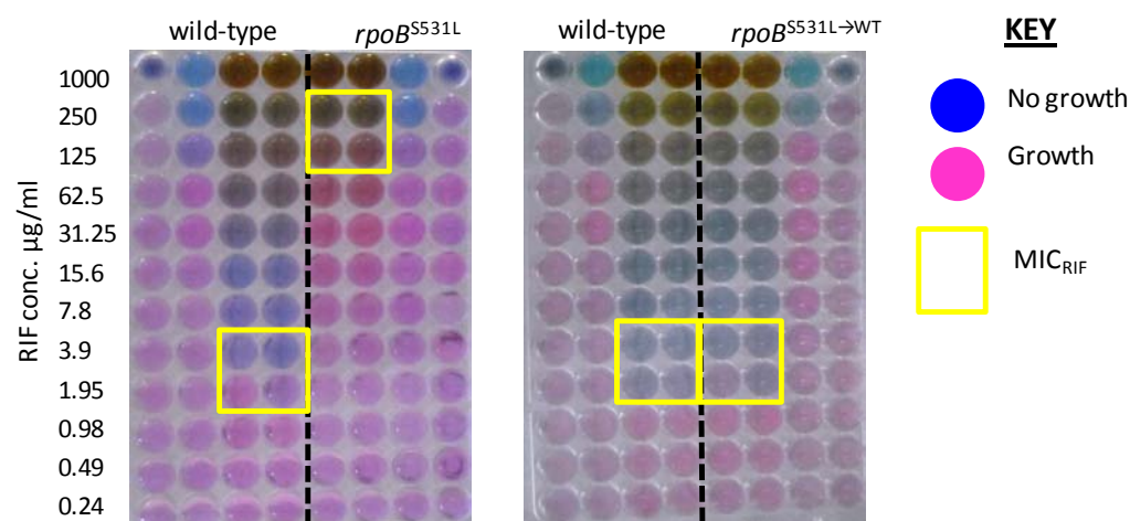
Figure 3.20 Restoration of wild-type rpoB in rpoB S531L restores RIF-susceptibility.
