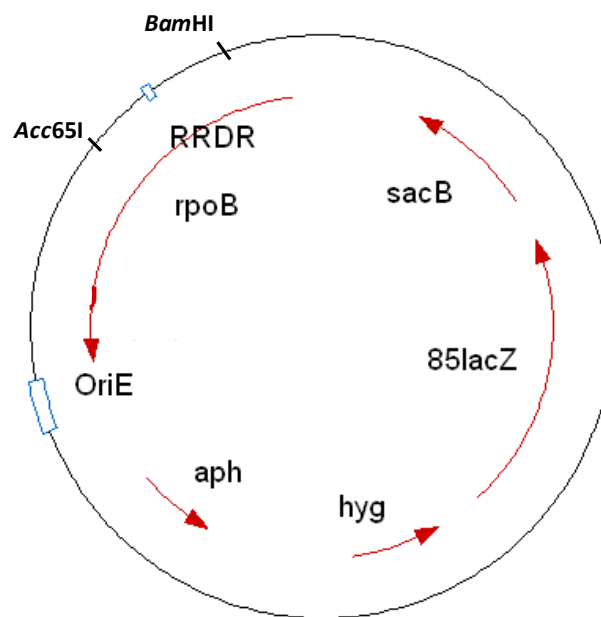
Figure 3.6 Representative suicide vector for allelic exchange.
