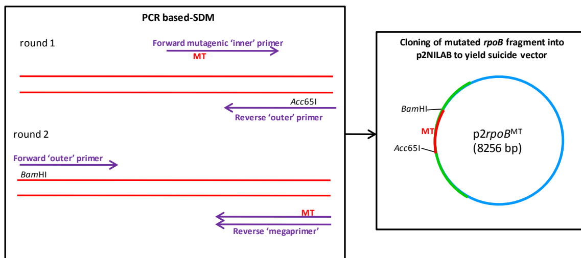
Figure 2.1 Schematic summary of the cloning strategy used in this project.
