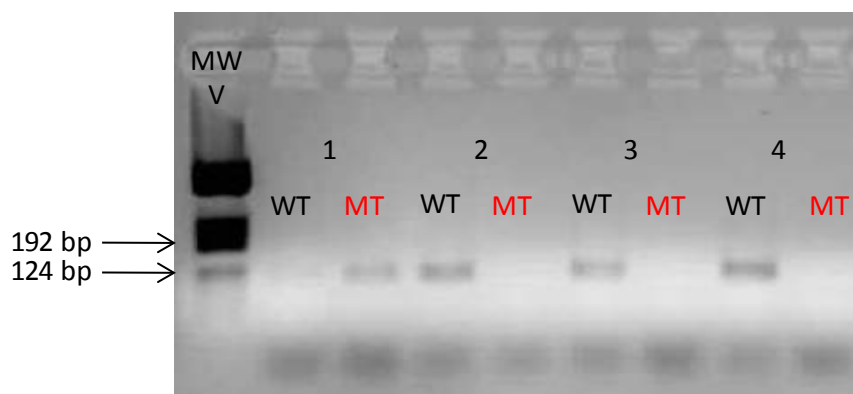
Figure 3.11 Colony one contains an S531L mutation in rpoB and is the rpoB S531L DCO.
