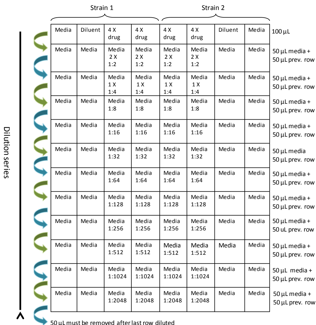
Figure 2.5 Schematic representation of preparation of MABA 96-well plates.
