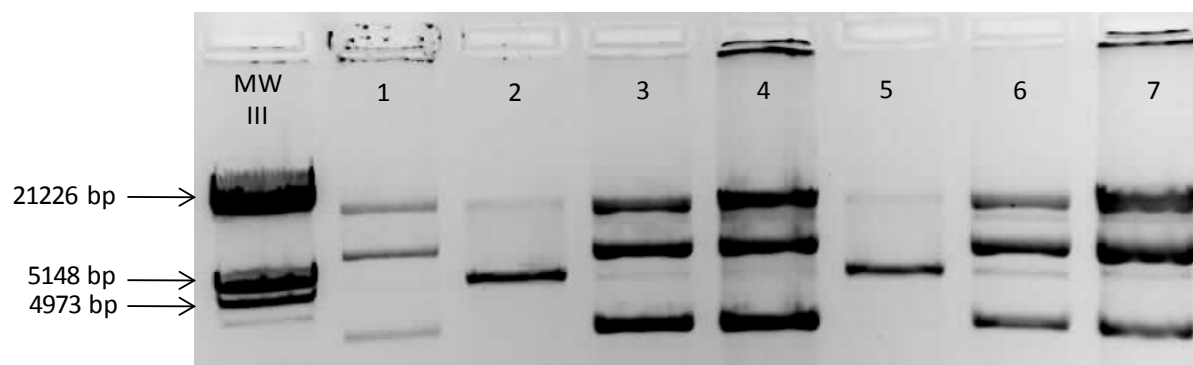
Figure 3.3 Acc65I and Bam HI sites were removed from p2NIL.
