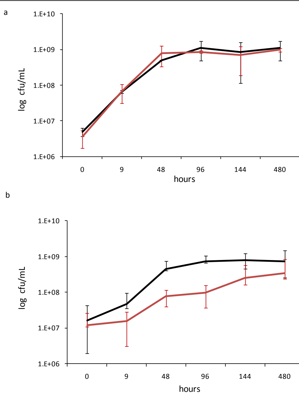
Figure 3.21 The rpoB S531L mutant has a fitness defect when grown in competition with wild-type MSM in 7H9 OADC.
