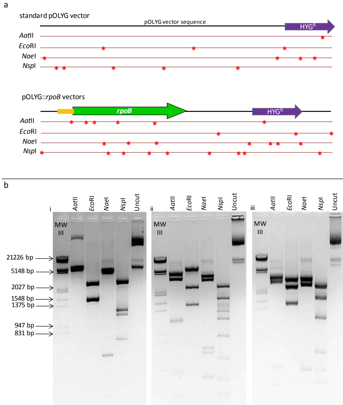
Figure 3.16 Over-expression of rpoB leads to plasmid re-arrangement.
