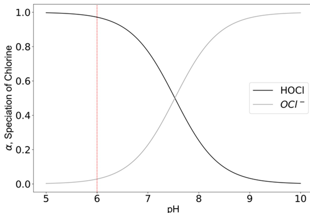
Fig 1. Speciation of aqueous chlorine species (represented by the fractional alpha value) as a function of pH, around circumneutral pH values. In the pH range shown above, the predominant species is hypochlorous acid at the lower end and shifts to the hypochlorite ion at the upper end. The vertical line shown at pH 6 is the target pH value for a disinfectant solution where hypochlorous acid is the predominant species. This figure was produced using published chlorine speciation equations [17]. Alpha represents the fractional concentration of a chlorine species over the total chlorine concentration.
