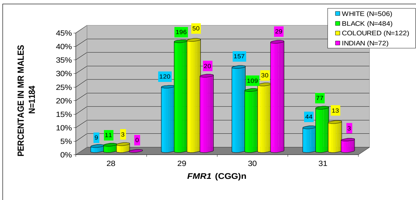
Figure 3.2 Histogram showing the distribution of common FMR1 alleles in the 4 different ethnic groups and their frequencies within each ethnic group tested.
