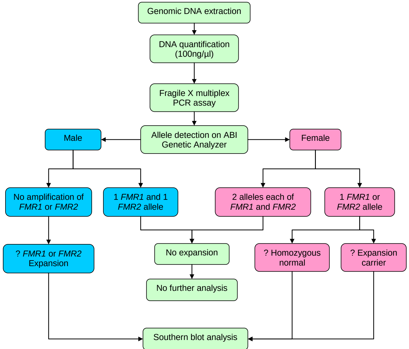
Figure 2.1 An overview of the procedure used for fragile X syndrome testing. The PCR is set up as a multiplex PCR reaction to detect FMR1 and FMR2 repeat and the flow diagram shows the steps followed for each locus.
