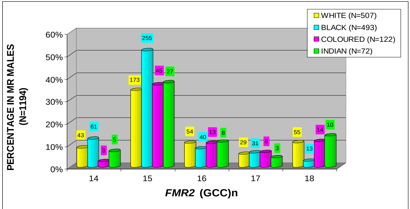
Figure 4.4 Histogram showing the common FMR2 GCC repeats and its frequency within each ethnic group tested
