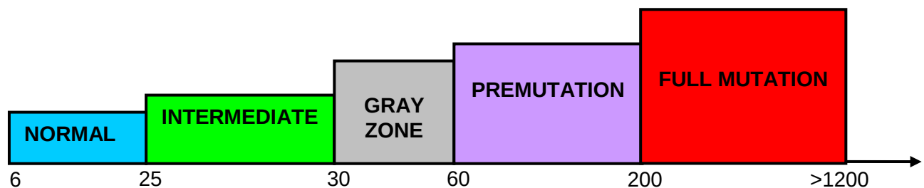
Figure 1.6 Range of FMR2 GCC repeats in the FMR2 gene.
