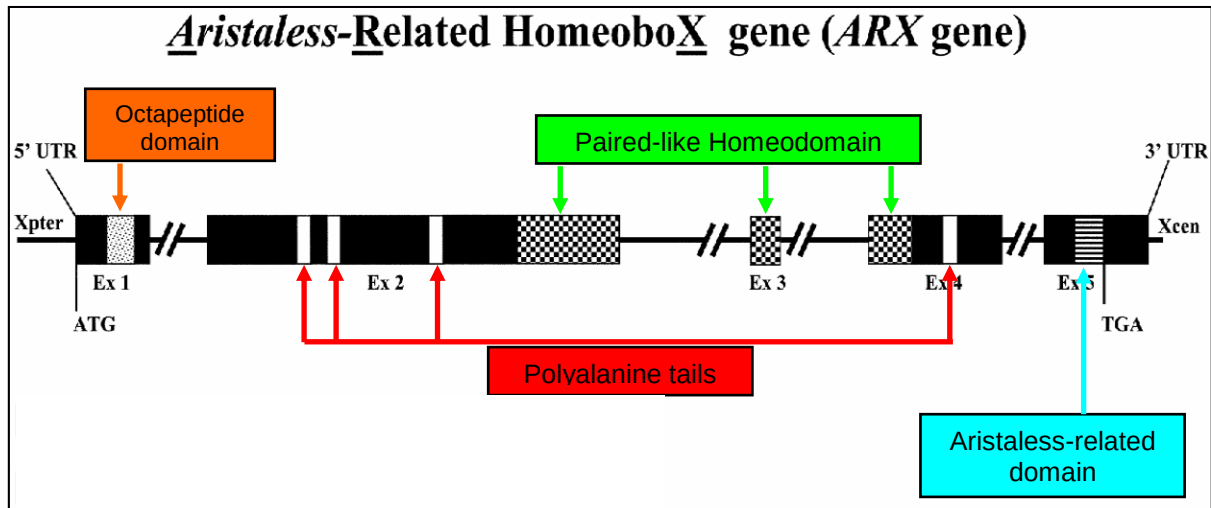
Figure 1.10 Schematic representation of the genomic organization of the ARX gene and the corresponding protein domains (Chiurazzi, et al., 2004)
