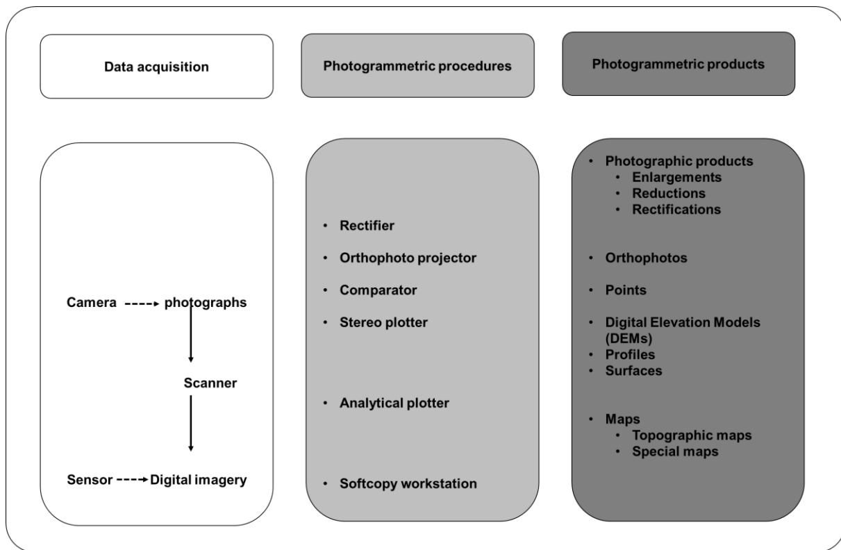
Figure 4-4: Overview of systems within photogrammetry (after Schenk, 2005)
