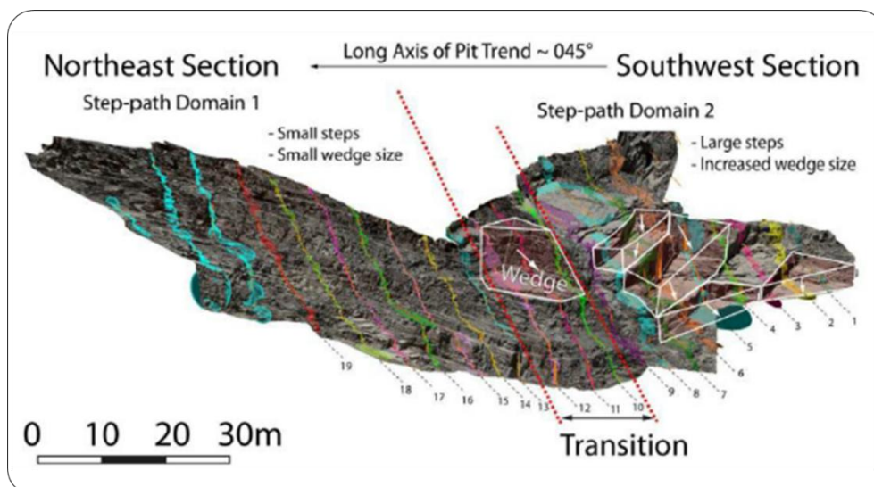
Figure 4-5: Photogrammetry model of east wall ( f=100\text{mm} ; distance= 50\text{m} ) showing a step path characterisation approach for evaluating existing slope geometry at Jwaneng mine, Botswana (Lupogo et al. 2014)
