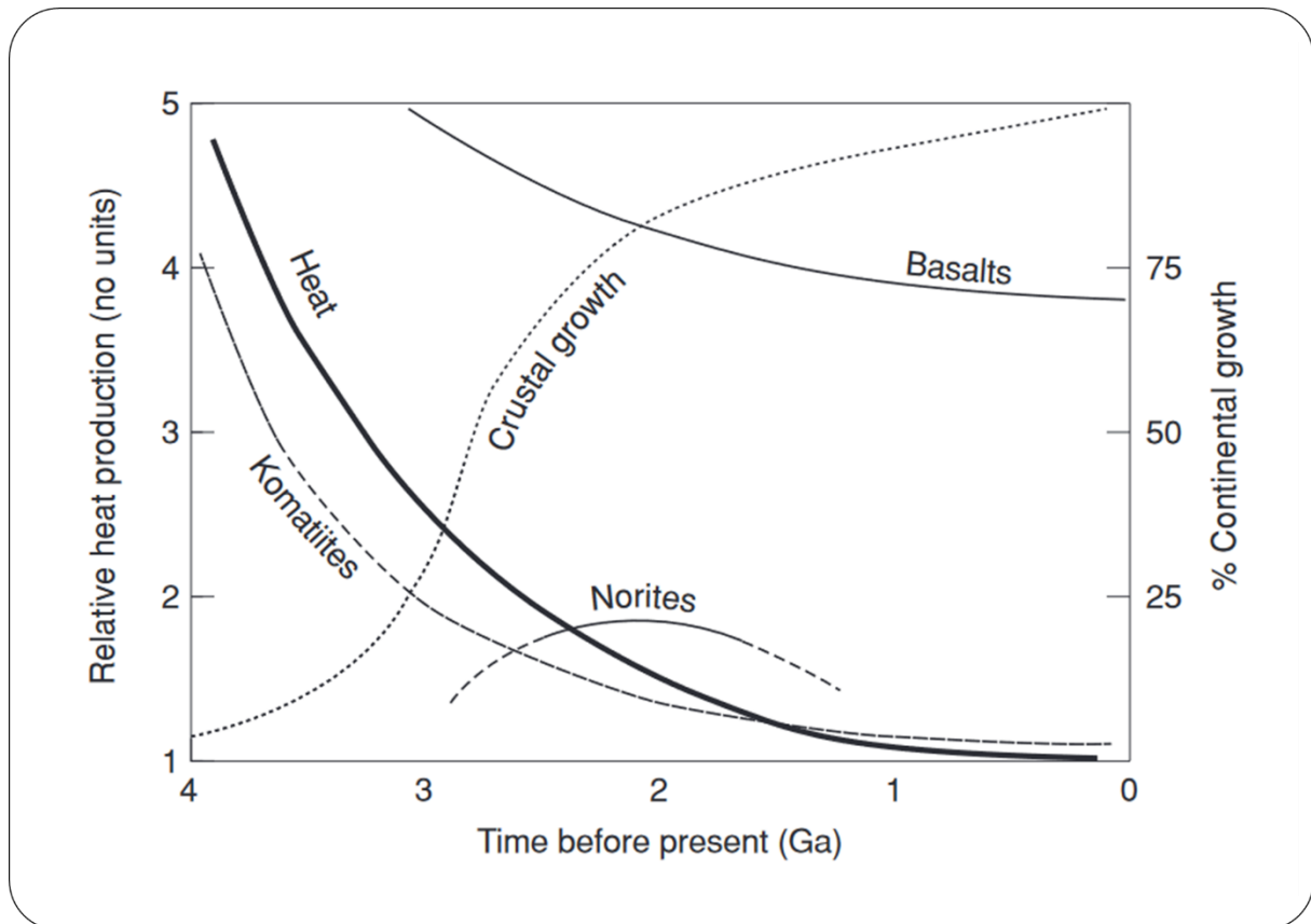
Figure 4-9: Schematic diagram showing the exponential decline in global heat production with time and the matching decline in production of komatiite volcanism (after Hall and Hughes, 1993, in Robb, 2006)
