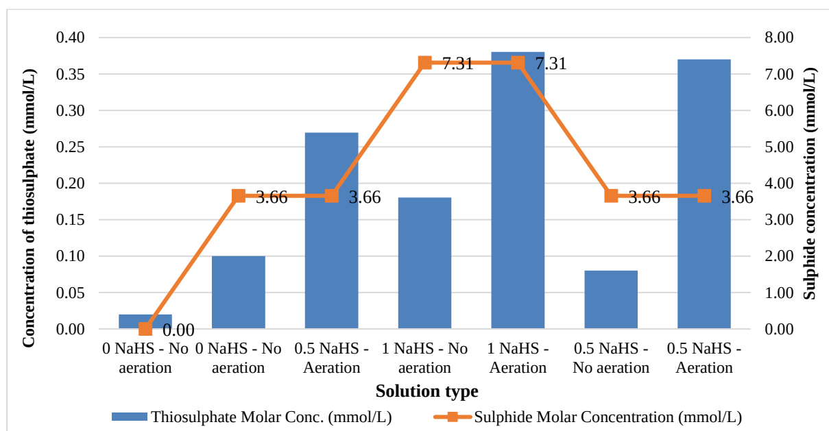
Figure 4.4 The relation of the thiosulphate with change in aeration and sulphide
