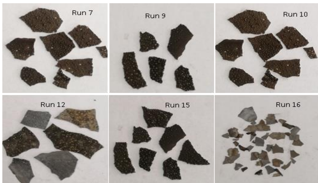
Figure 4.17 Sample photographs for SEM analysis
