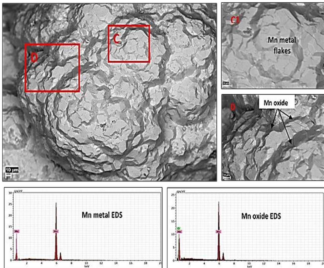
Figure 4.18 BSE images and EDS spectrum of manganese metal flakes and manganese oxide in run 7
