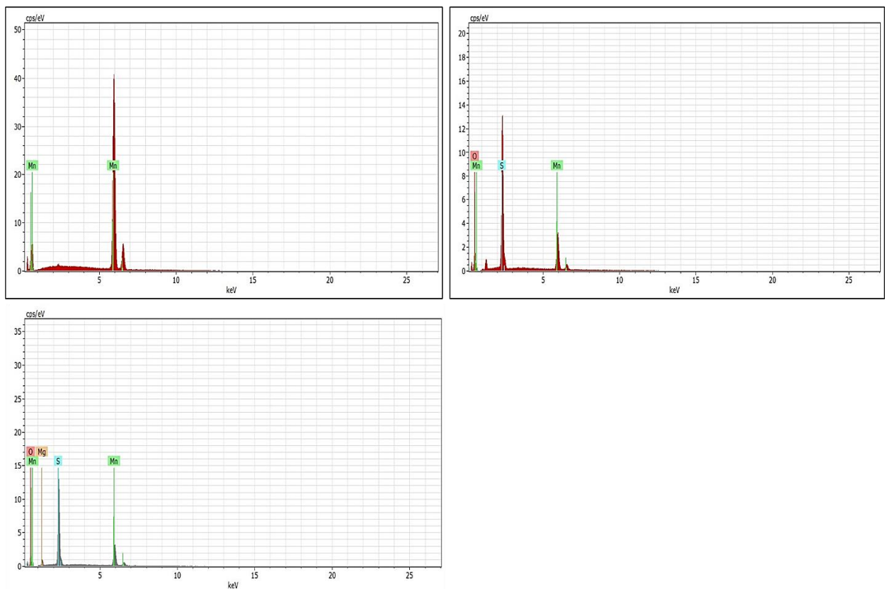
Figure 4.28 EDS spectrum of manganese sulphur agglomerates in Run 12
