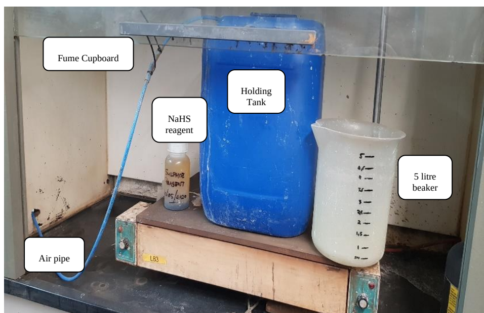
Figure 3.2 Test setup for solution preparation
