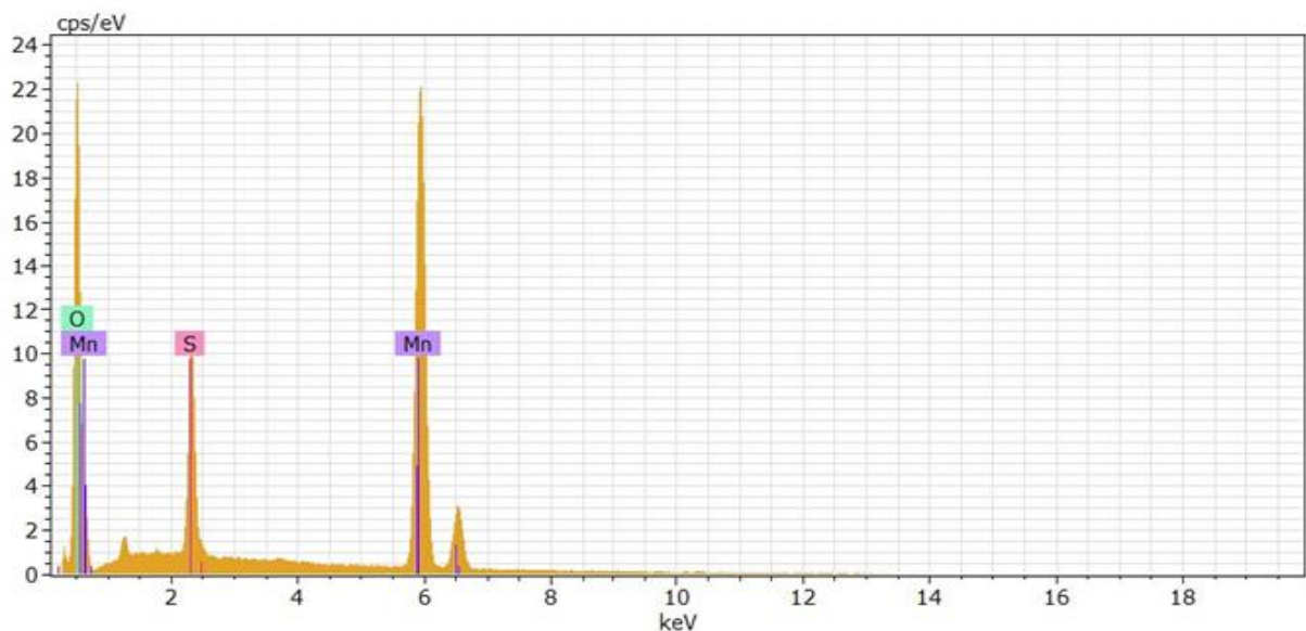
Figure 4.20 EDS spectrum of manganese sulphur agglomerates in Run 9
