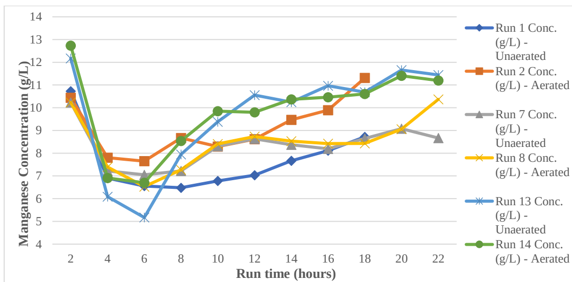
Figure 4.9 The catholyte concentration for runs at fresh feed and aeration
