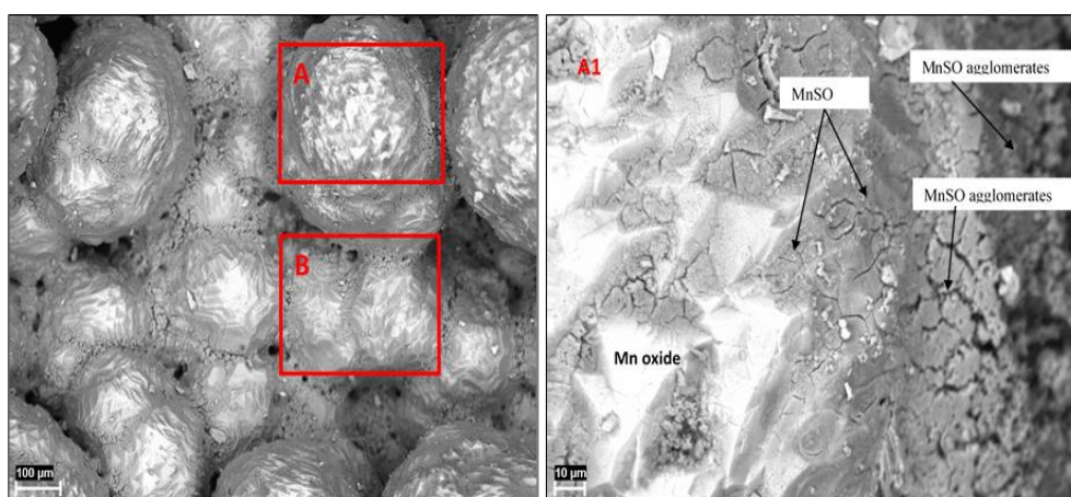
Figure D.12 BSE images of manganese oxide prisms and manganese sulphate agglomerates in Run 9 at a resolution of 100 and 10 µm
