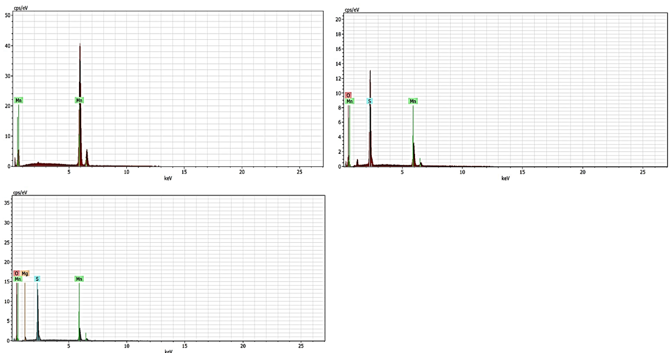
Figure 4.22 EDS spectrum of manganese sulphur agglomerates in Run 10
