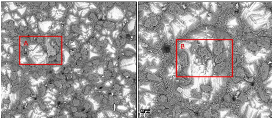
Figure D.14 Overview BSE images of well-developed manganese metal prisms with the surface coated by fibrous manganese sulphate particles in Run 16 at a resolution of 20 and 10 \mu\text{m} .
