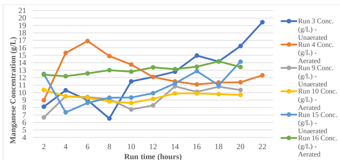
Figure 4.12 The catholyte concentration for runs at 0.5 NaHS and aeration
