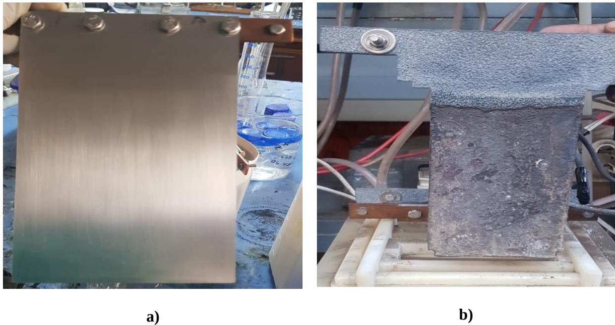
Figure 3.6 Types of electrodes used in the lab cells a) Stainless Cathode Plate b) Anode Plate
