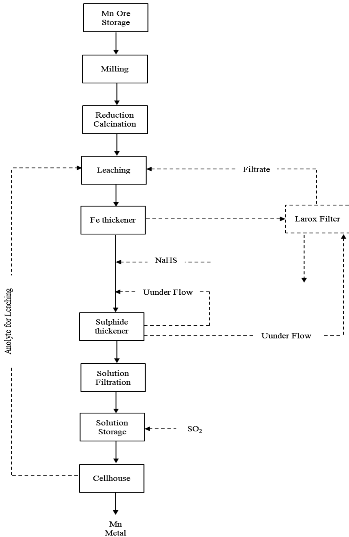
Figure 1.1 Typical flow diagram of manganese production at Manganese Metal Company
