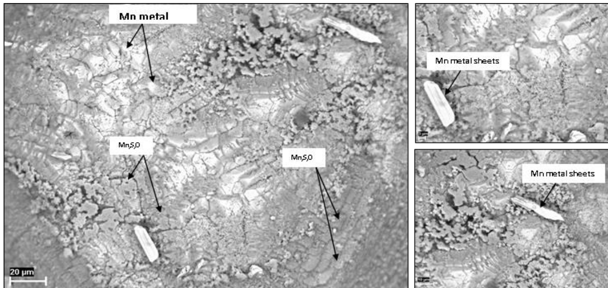
Figure 4.21 BSE images of developing Mn metal prisms with surface coated by manganese sulphide and fine discrete manganese metal sheets in Run 10
