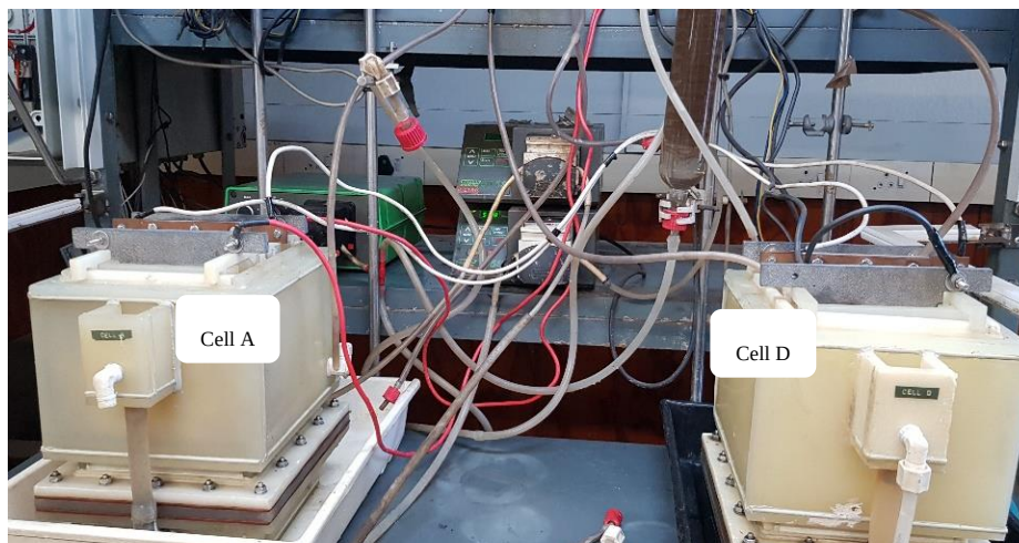
Figure 3.5 Laboratory electrowinning cells A and D
