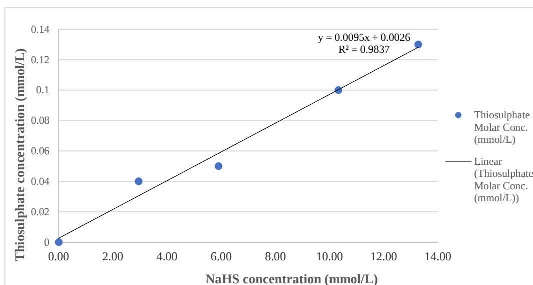
Figure 4.2 Thiosulphate and NaHS concentration for T102 solution
