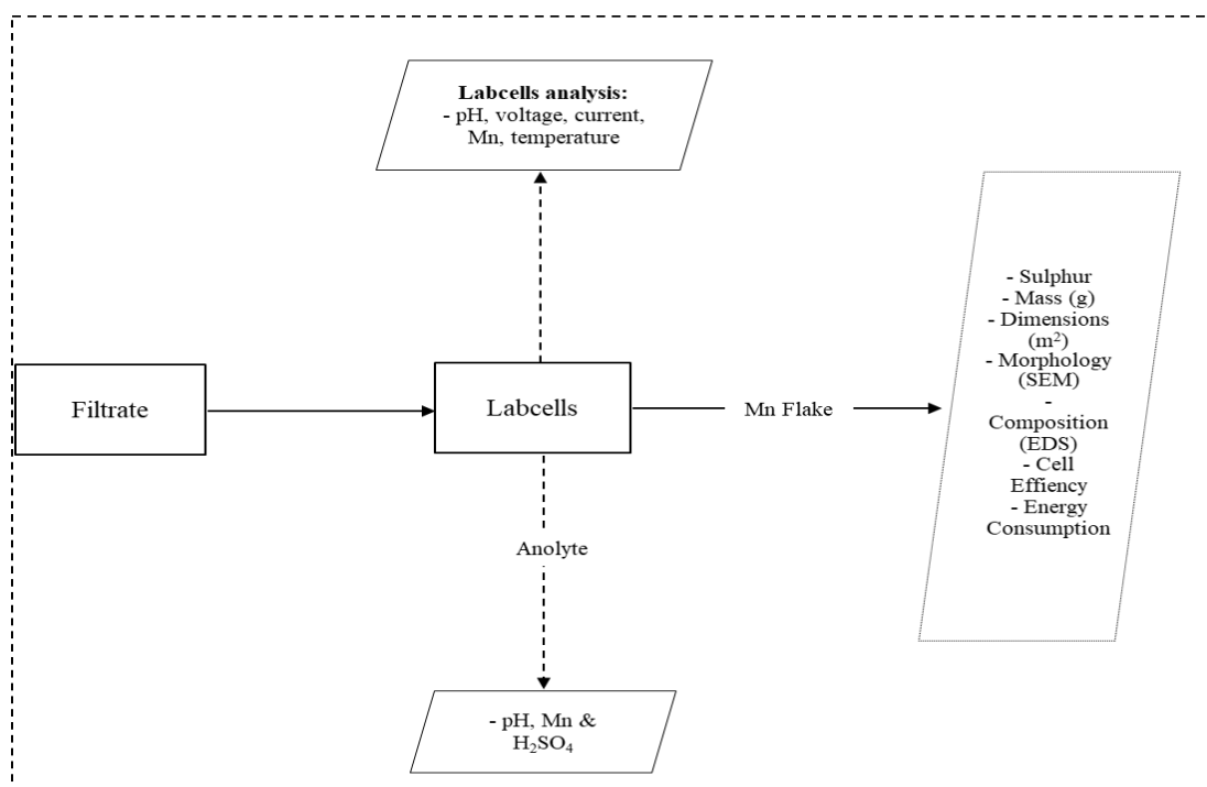
Figure 3.15 Flow diagram for the labcells operations
