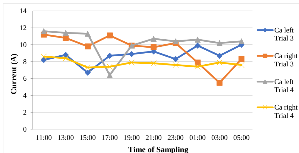
Figure C.2 The current readings on the cathode for trial 3 and 4
