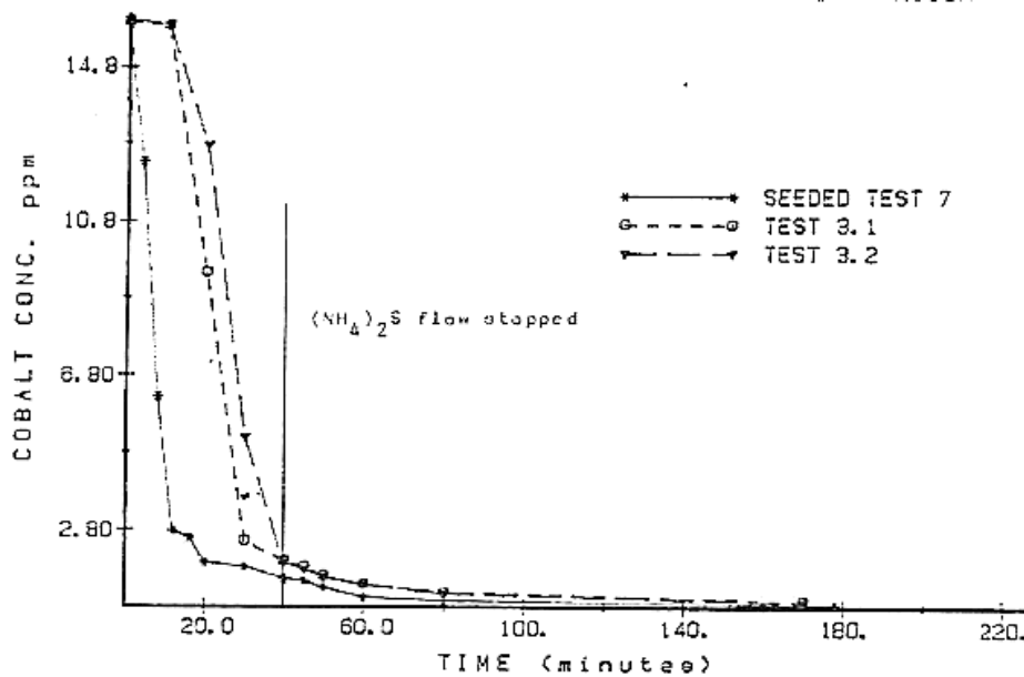
Figure 2.2 Seeded and unseeded test comparison for cobalt in a reaction vessel (Bijsterveld, 1984)
