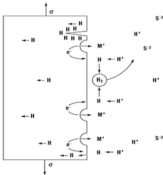
Figure 2.6 Schematic Showing the Generation of Hydrogen Producing SSC (NACE, 2002)
