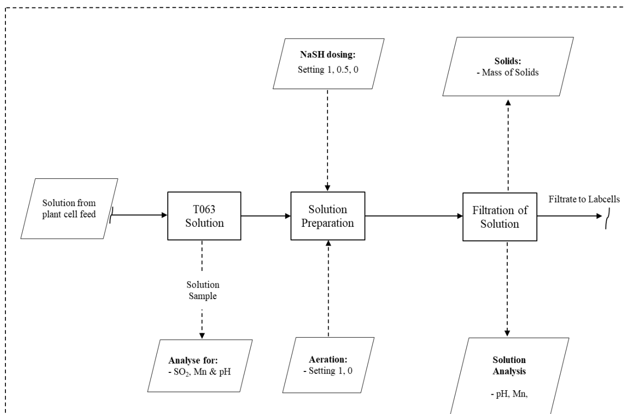
Figure 3.12 Flow diagram for the solution preparation experiments
