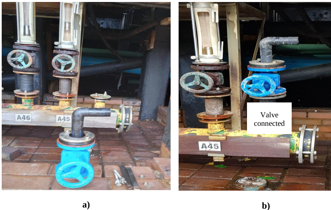
Figure 3.1 Solution collection point a) Valve at F-bank rotameter. b) Installed valve for solution collection
