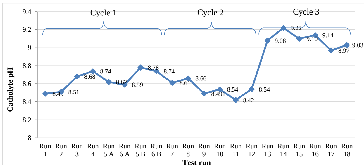
Figure 4.8 The average catholyte pH of the test runs
