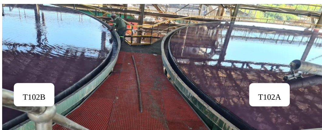
Figure D.4 Sulphide thickeners number 102-A (T102A) and 102-B (T102B) used for the purification of the solution by removal of the precipitate or solid particles
