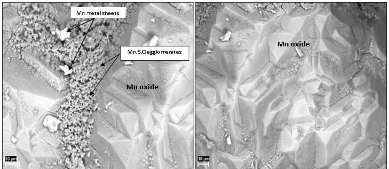
Figure 4.19 BSE images of fine discrete manganese metal sheets, manganese oxide prisms and manganese sulphide agglomerates in Run 9
