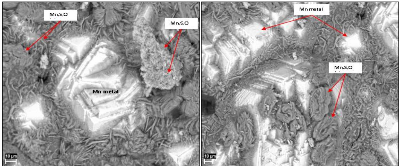
Figure 4.25 Detailed BSE images of well-developed manganese metal prisms with the surface and ridges coated by fibrous manganese sulphide particles in Run 16
