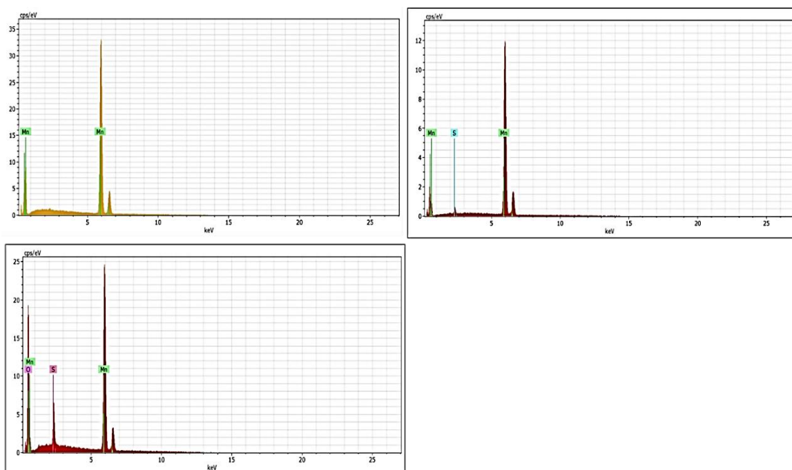
Figure 4.24 EDS spectrum of manganese sulphur agglomerates in Run 15
