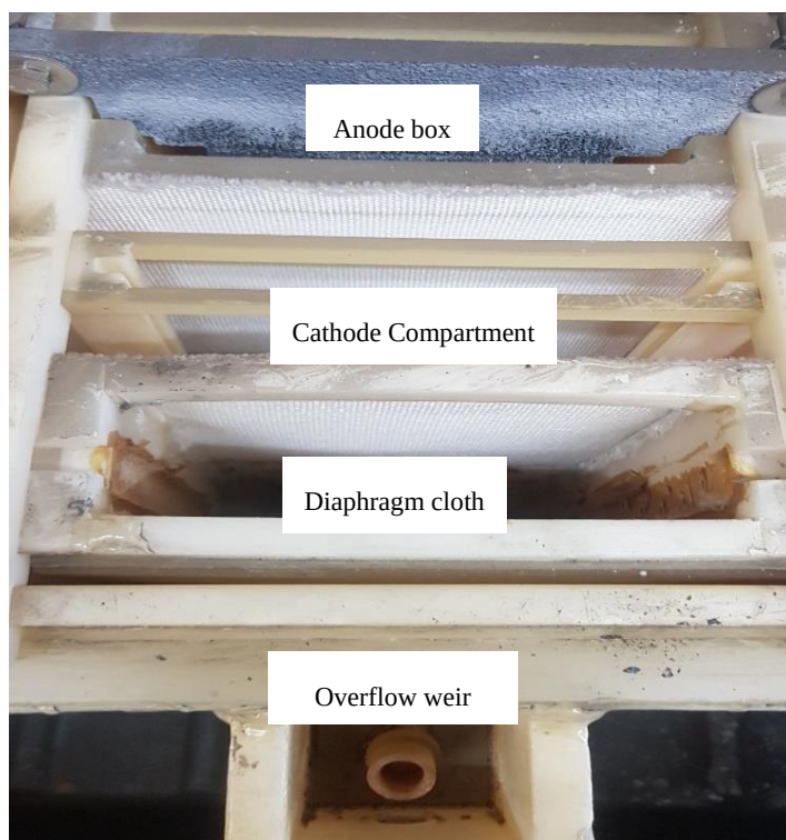
Figure 3.9 The top-view of the lab-cells section
