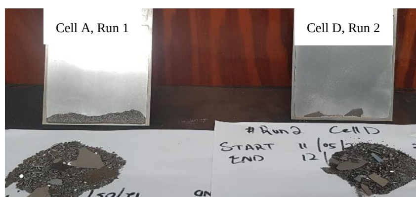
Figure 4.11 Physical characteristics of metal run 1 and run 2 after stripping
