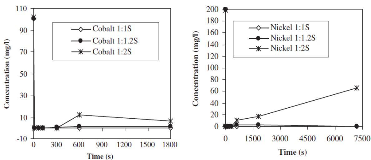
Figure 2.3 Nickel and cobalt concentrations in the batch experiments using an aqueous sulphide source (Lewis and van Hille, 2005)
