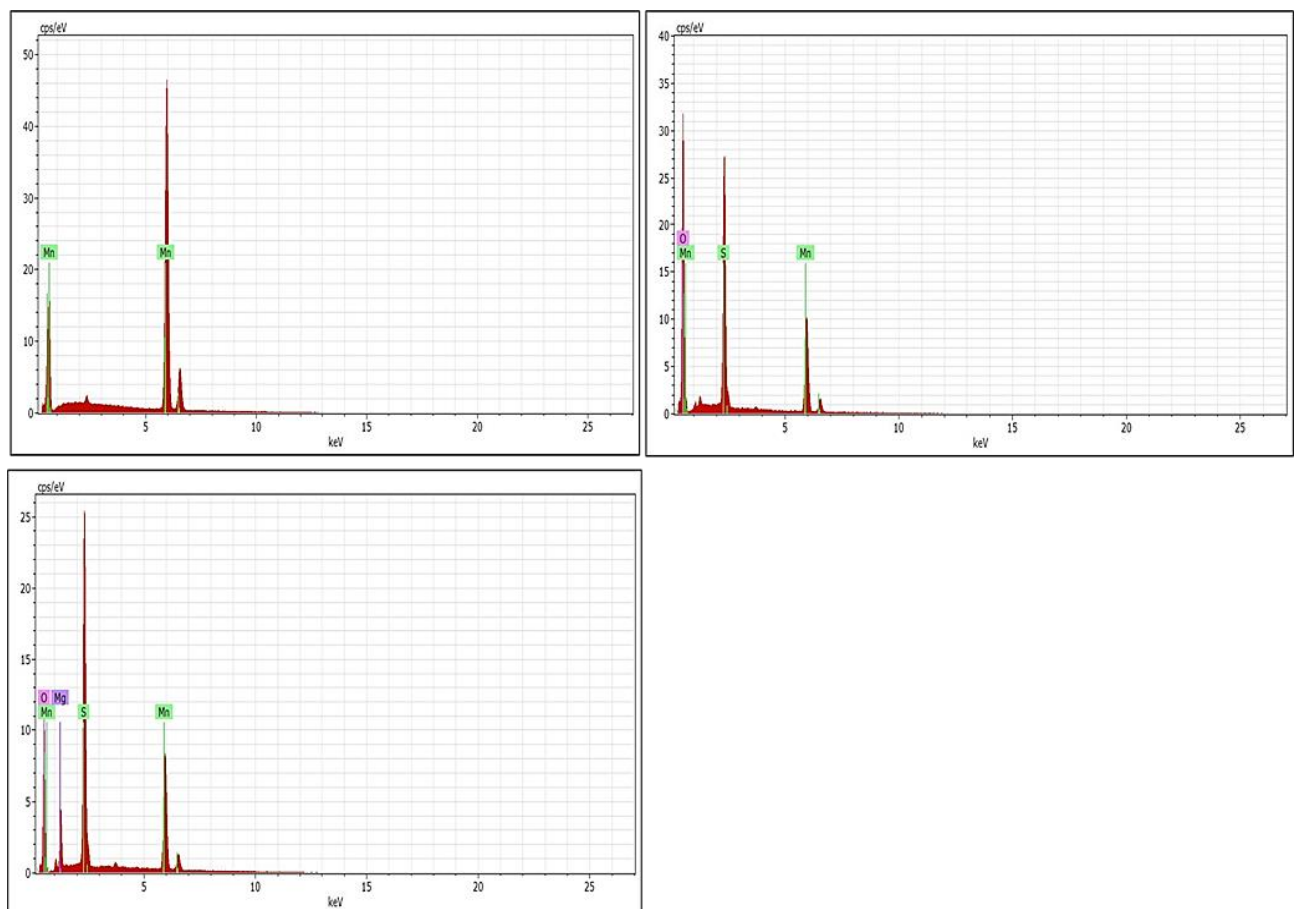
Figure 4.26 EDS spectrum of manganese sulphur agglomerates in Run 16
