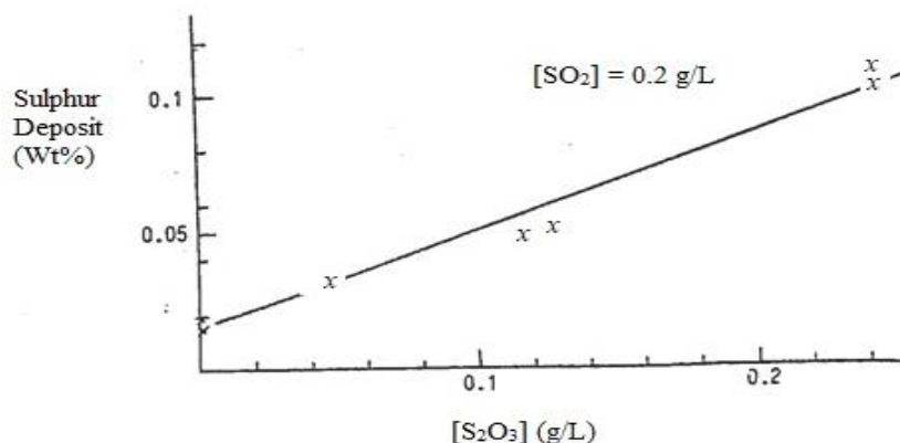
Figure 2.5 The concentration of thiosulphate vs sulphur in metal (Saunders and Ribane, 1986)
