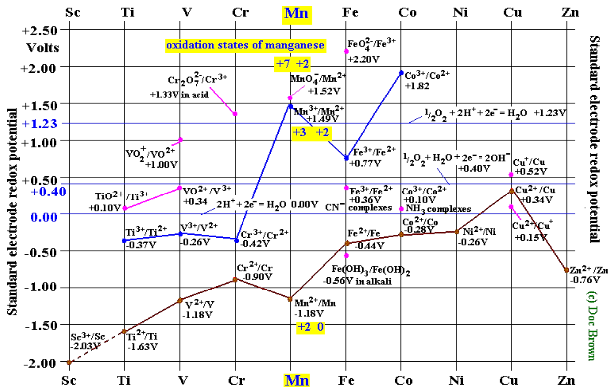
Figure 2.1 Standard electrode potential chart diagram for the 3d-block elements (Brown, 2020: Appendix, para.2)
