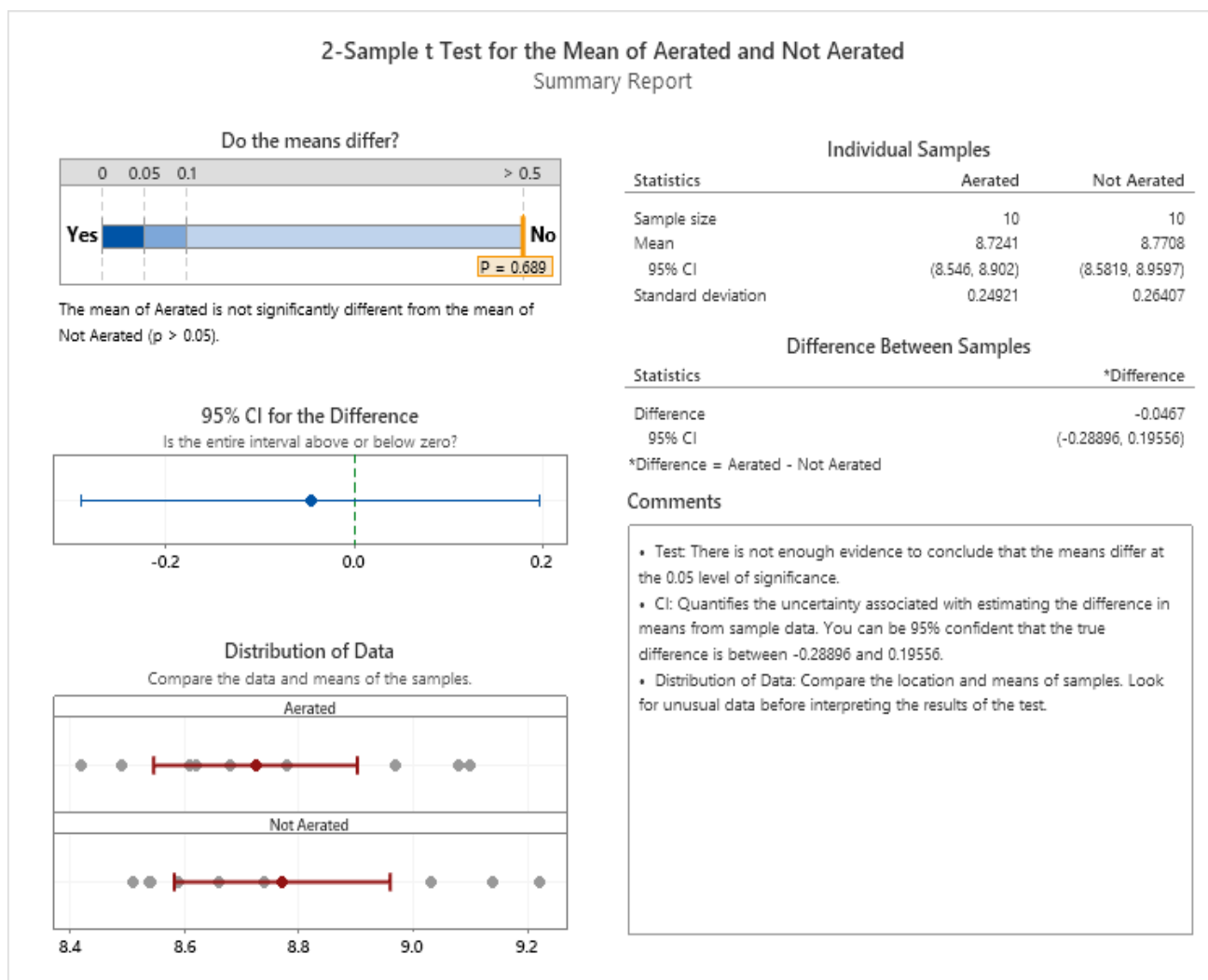
Figure D.5 The two-sample t-test conducted to compare the difference between the catholyte pH of the aerated and not aerated solution
