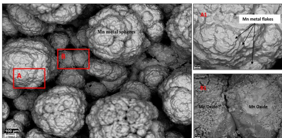
Figure D.11 BSE images of manganese metal flakes and manganese oxide in Run 7 at a resolution of 100 and 10 µm
