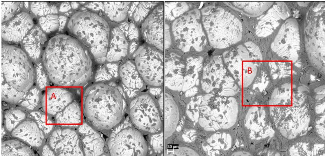
Figure D.13 Overview BSE images of well-developed manganese oxide spheres, and the cementing material in Run 12 at a resolution of 100 and 30 \mu\text{m}
