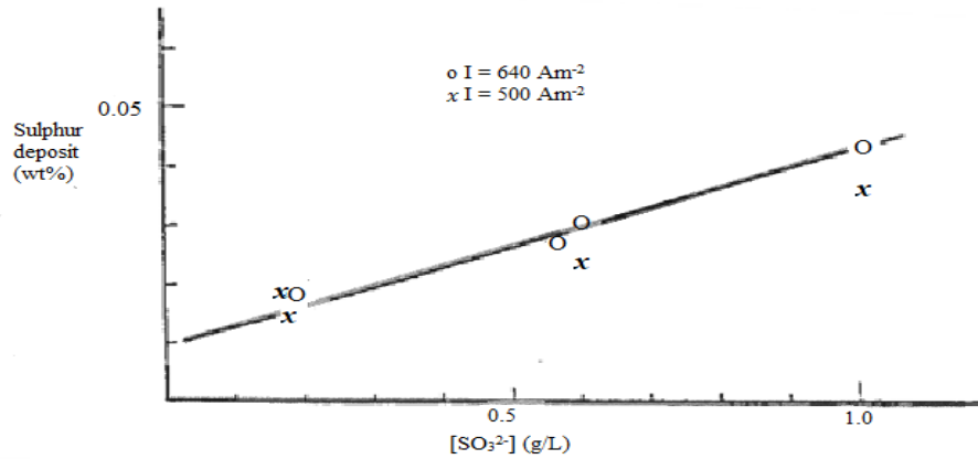
Figure 2.4 The concentration of sulphite vs sulphur in metal (Saunders and Ribane, 1986)
