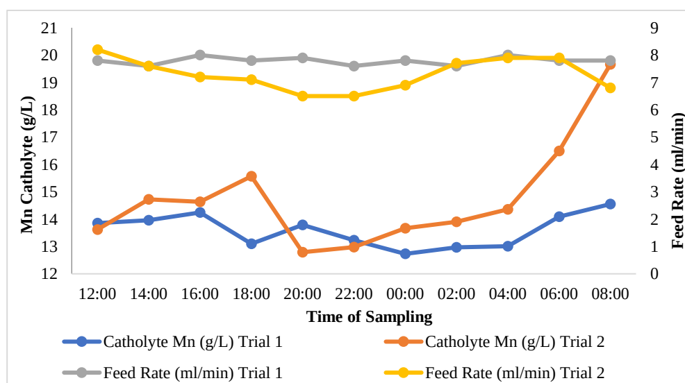
Figure C.3 Catholyte Mn concentration and flow rate
