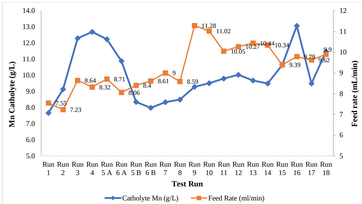
Figure 4.7 The average manganese catholyte of the test programme
