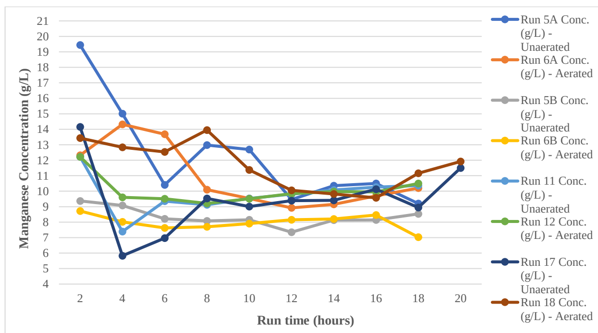
Figure 4.14 The catholyte concentration for runs at 1.0 NaHS and aeration
