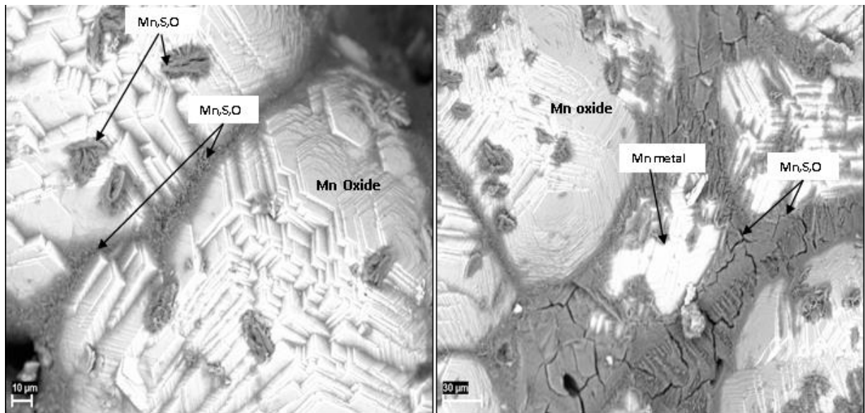
Figure 4.27 Detailed BSE images of well-developed manganese oxide spheres, and the cementing material manganese sulphide, in Run 12
