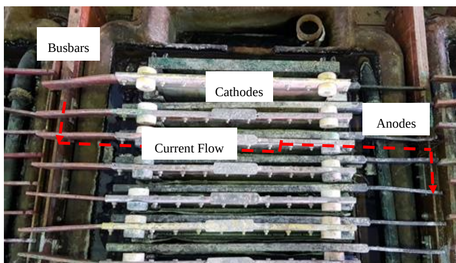
Figure A.1 Cell Design and Current Flow
