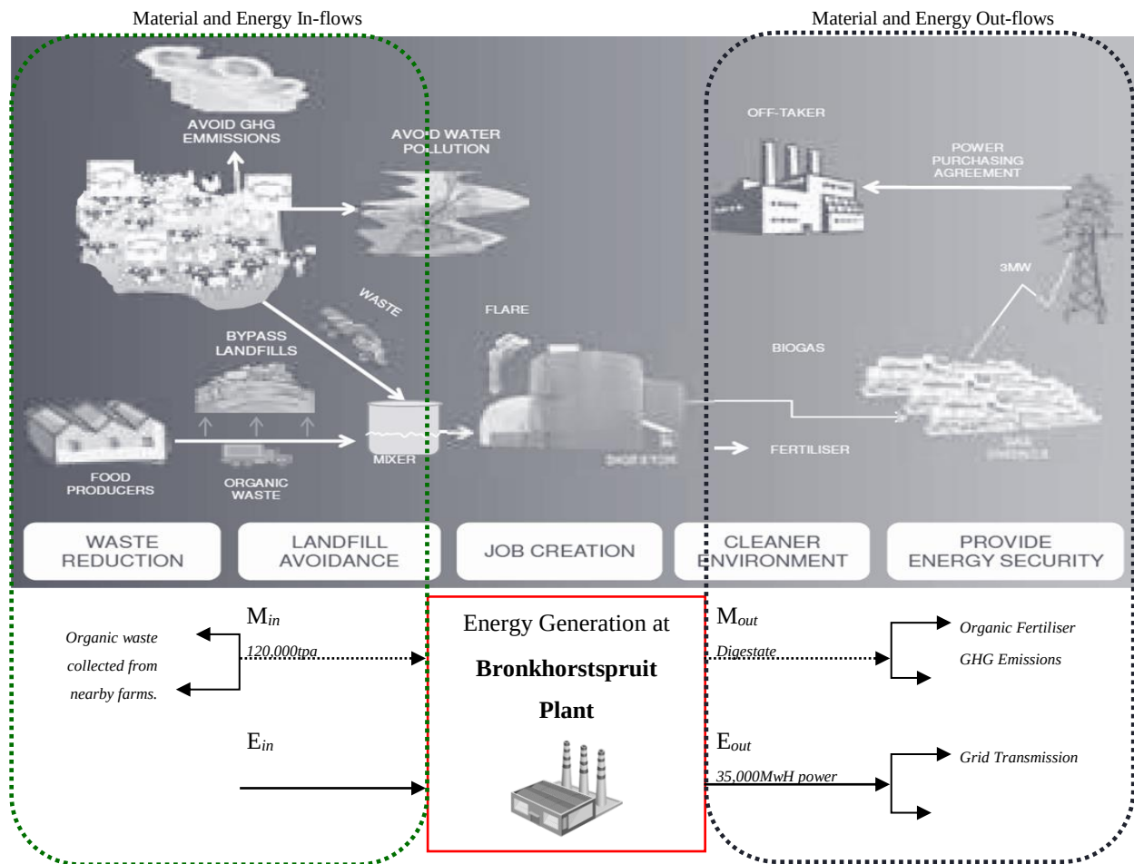
Figure 4.5: Bronkhorstspuit Biogas Plant - Energy and Waste Flows Schematic
