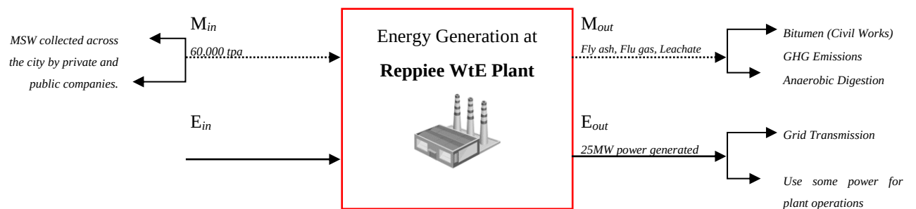
Figure 4.3: Reppie WtE Plant – Energy and Waste Flows Schematic
