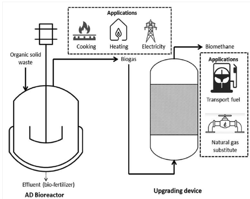
Figure 2.19: Typical Design of an AD Plant and its by-products
