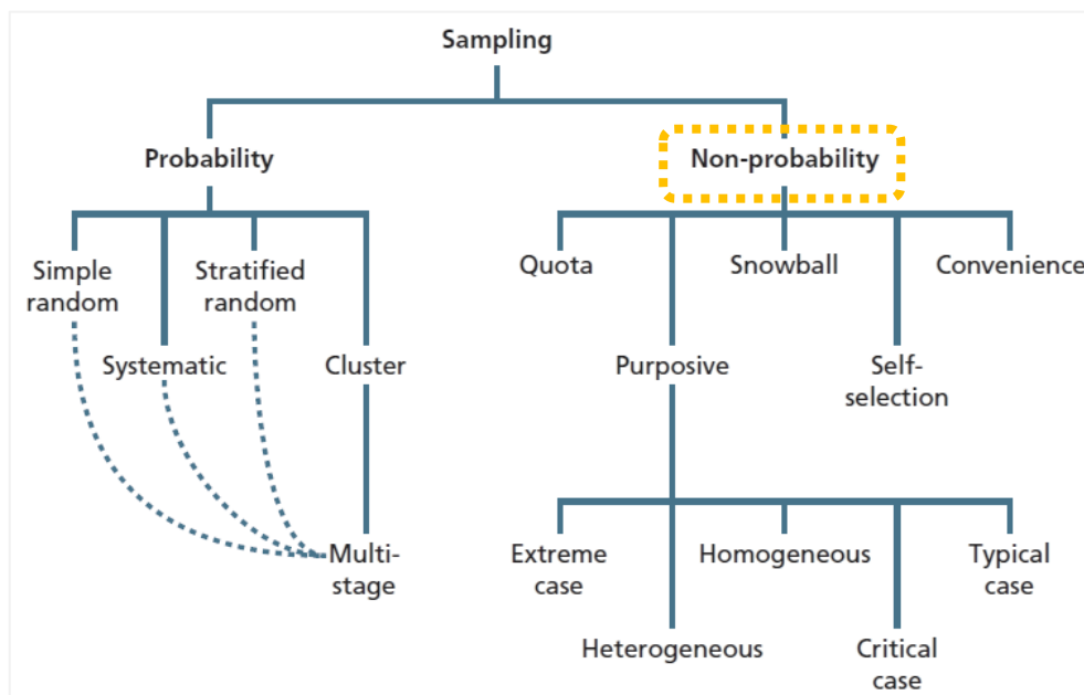
Figure 3.7: Sampling Techniques
