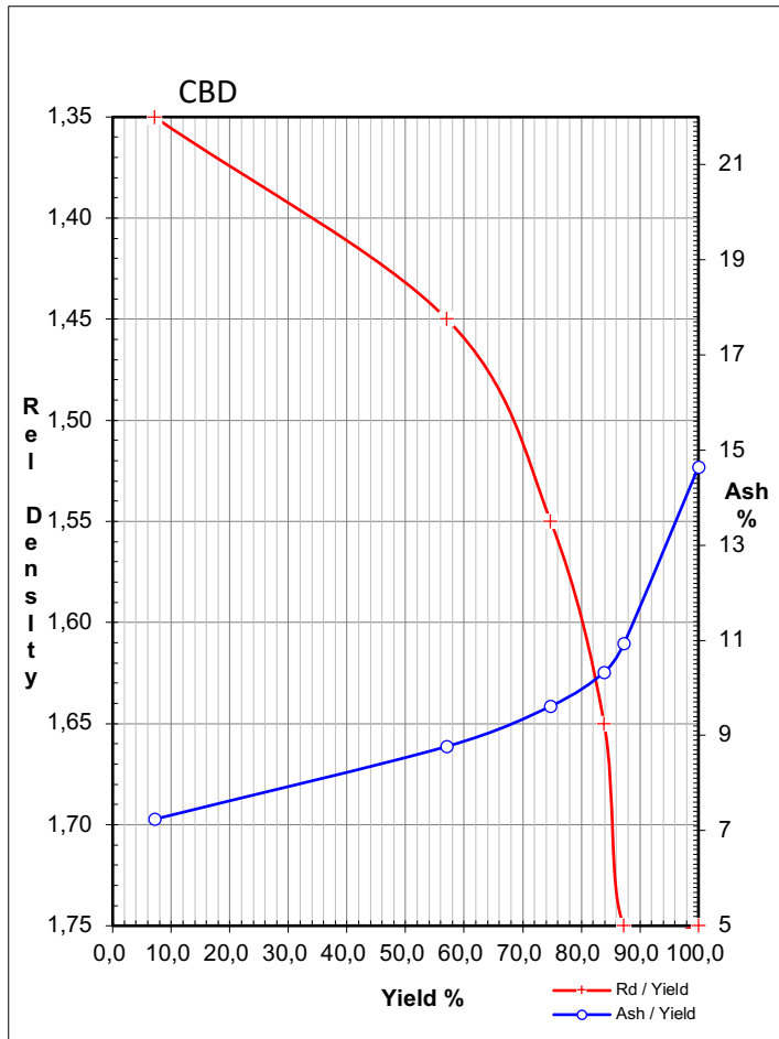
Figure 28: Graphical representation of the Ash Yield and densimetric washability curves of the CBD ply of the CS30AI. Ash and RD are directly proportional to the yield of the CBD ply.
