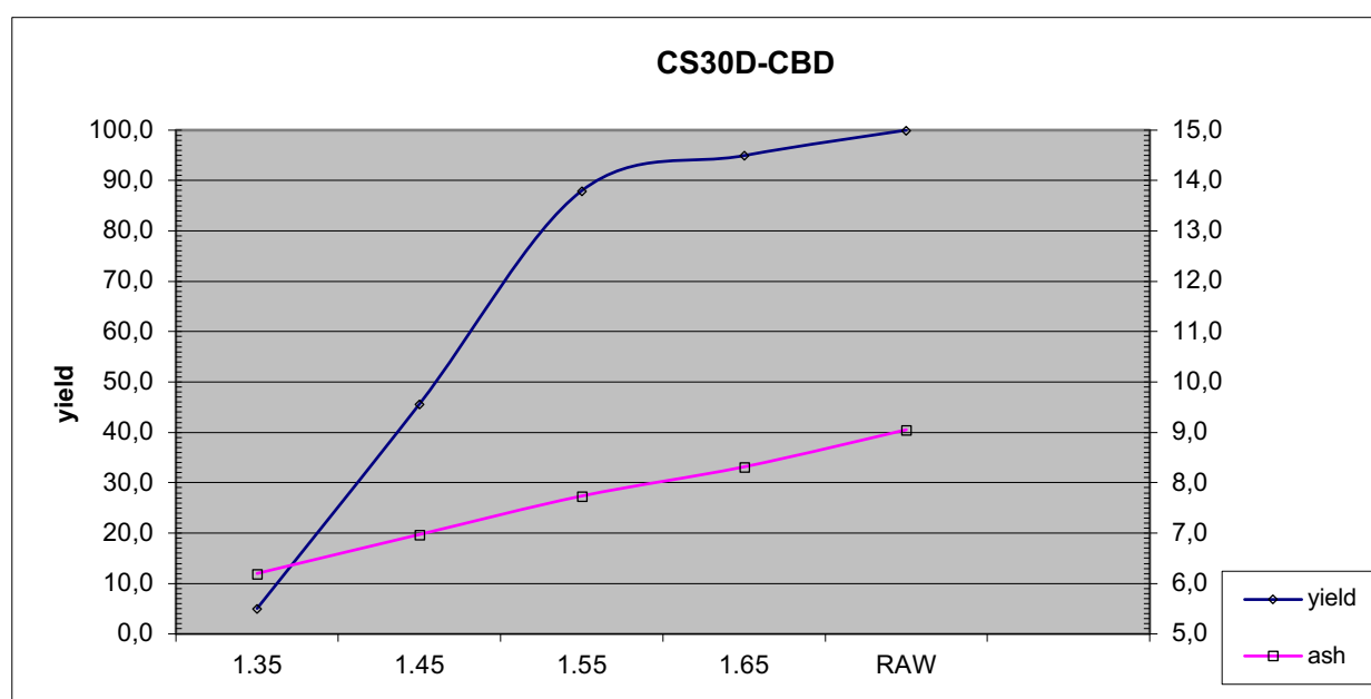
Figure 37: The densimetric and ash yield curves of the prime product of the CBD ply of the Channel Sample 30D showing a relationship between Ash Yield and RD Yield.
