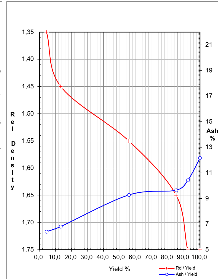
Figure 24: Graphical representation of the Ash Yield and densimetric washability curves of the CB ply of the CS30B. Ash and RD are directly proportional to the yield of the CB ply.
