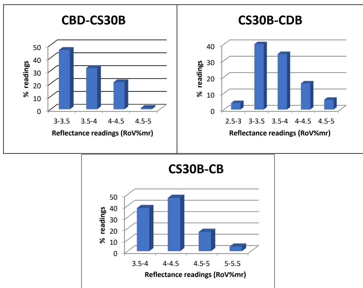
Figure 41: Unimodal distribution of the vitrinite reflectance of the CBD, CDB, and CB plies of the Main Seam
