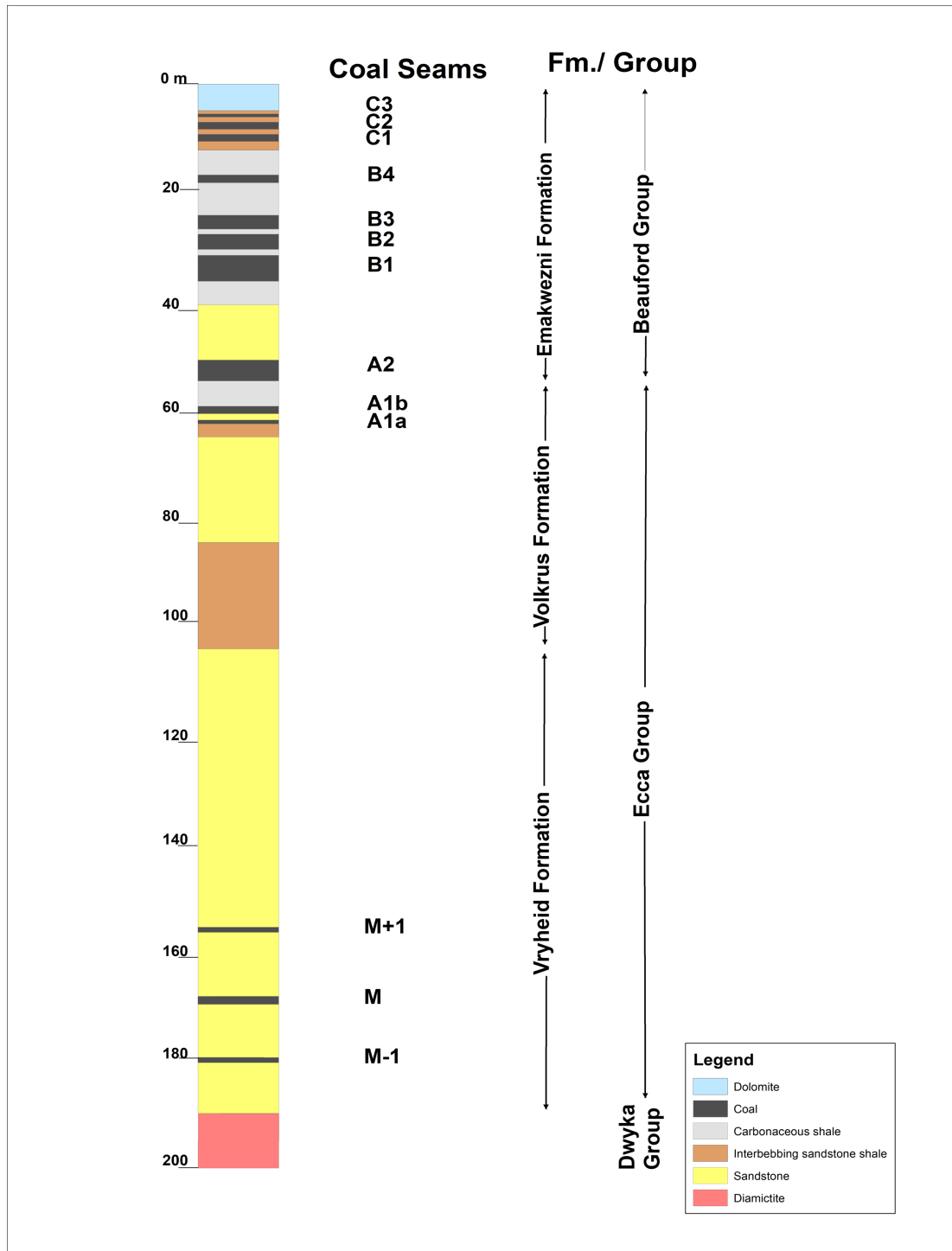
Figure 4: Generalised stratigraphic sequence of the Karoo Supergroup fill of the Nongoma Graben in the Msebe area, Nongoma Coalfield (Hatherly and Sexton, 2013).
