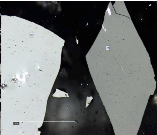
B. Collotelinite in bright coal (left) and dull coal (right)
