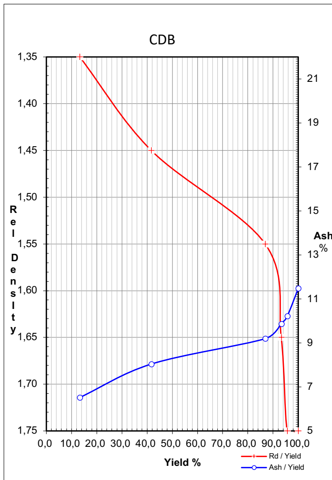
Figure 35: Graphical representation of the Ash Yield and densimetric washability curves of the CDB ply of the CS30D. Ash and RD are directly proportional to the yield of the CDB ply.
