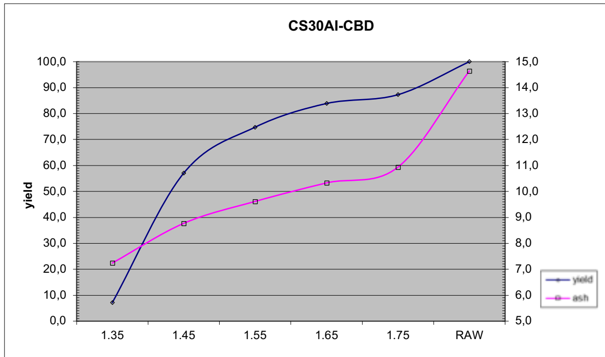
Figure 31: The densimetric and ash yield curves of the prime product of the CBD ply of the Channel Sample 30AI showing a relationship between Ash Yield and RD Yield.
