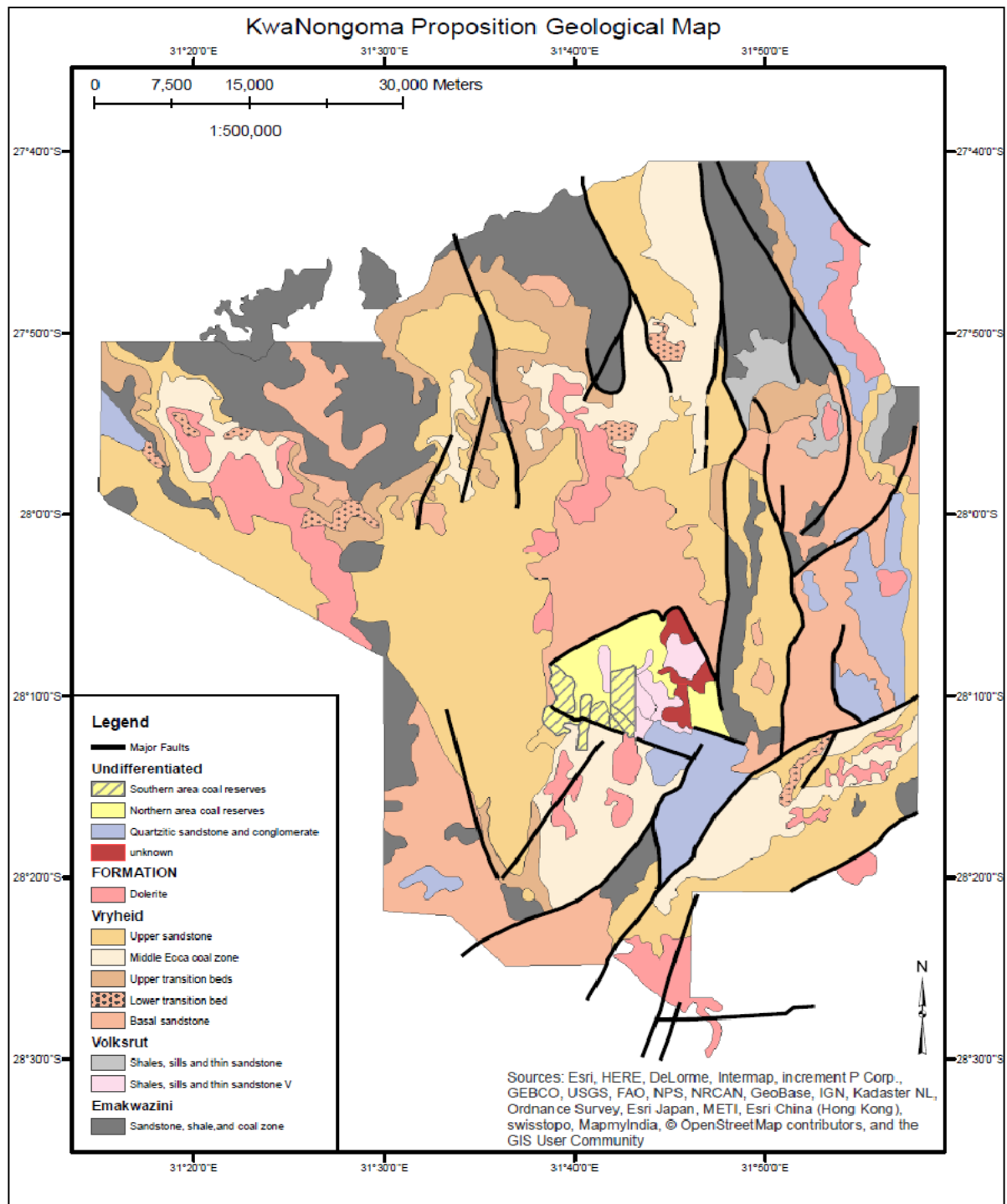
Figure 5: Geologic map depicting the structural setting of the Nongoma Coalfield (ZAC geologists).
