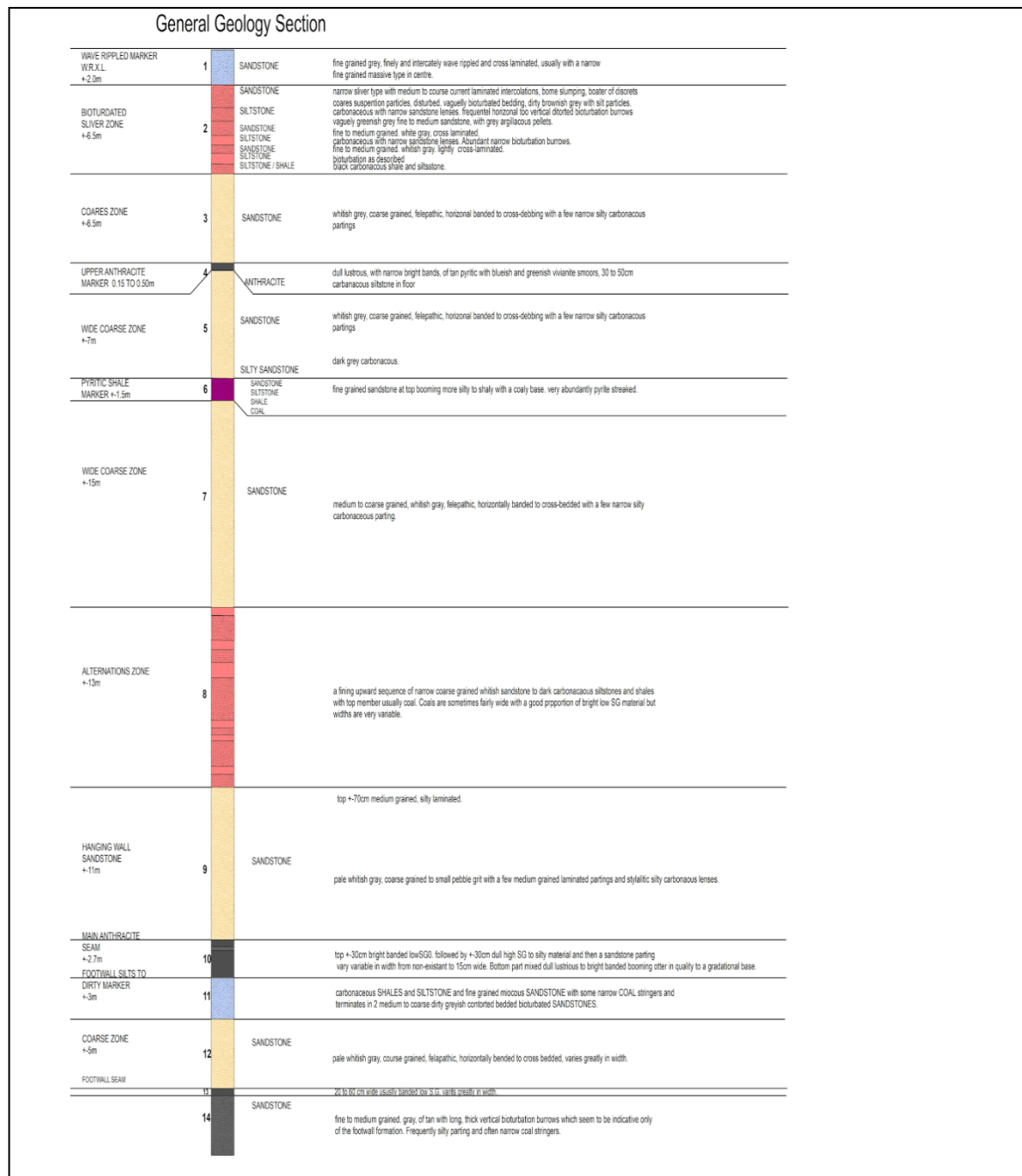
Figure 6: Generalised geological section of the ZAC mines showing the 14 lithological units (ZAC geologists).
