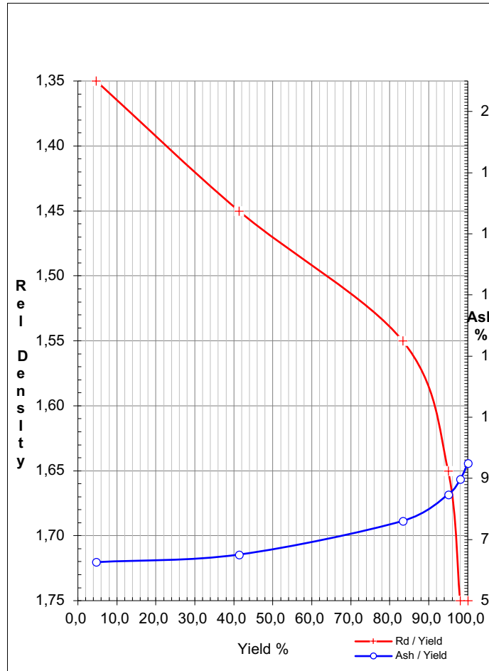
Figure 23: Graphical representation of the Ash Yield and densimetric washability curves of the CBD ply of the CS30B. Ash and RD are directly proportional to the yield of the CBD ply.
