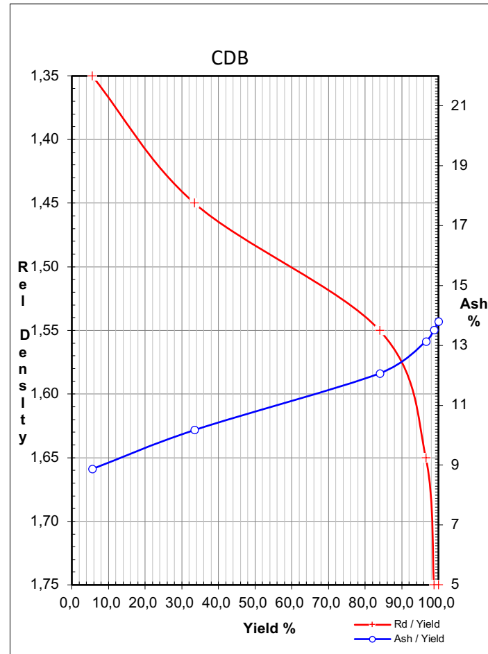
Figure 29: Graphical representation of the Ash Yield and densimetric washability curves of the CDB ply of the CS30AI. Ash and RD are directly proportional to the yield of the CDB ply.
