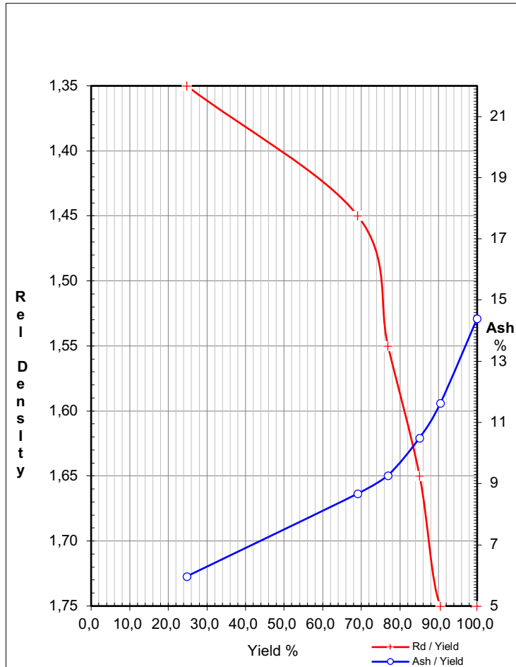
Figure 22: Graphical representation of the Ash Yield and densimetric washability curves of the CBD ply of the CS30B. Ash and RD are directly proportional to the yield of the CBD ply.
