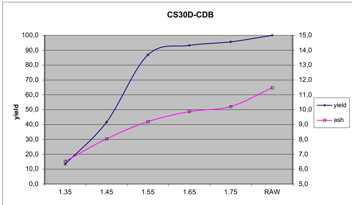
Figure 38: The densimetric and ash yield curves of the prime and middlings product of the CDB ply of the Channel Sample 30D showing a relationship between Ash Yield and RD Yield.
