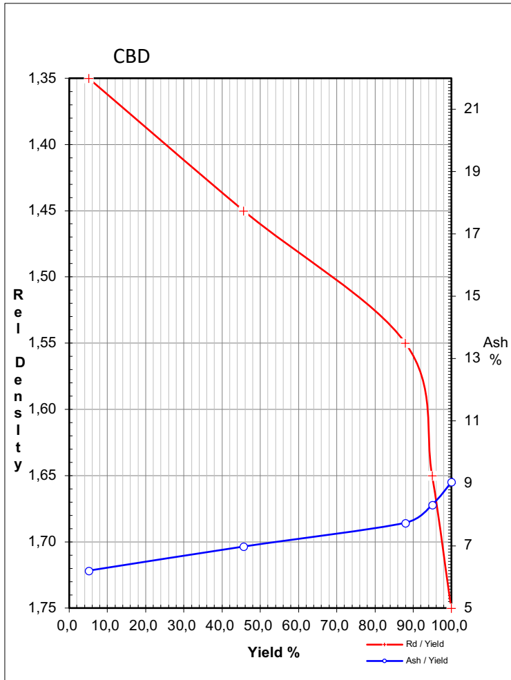
Figure 34: Graphical representation of the Ash Yield and densimetric washability curves of the CBD ply of the CS30D. Ash and RD are directly proportional to the yield of the CBD ply.
