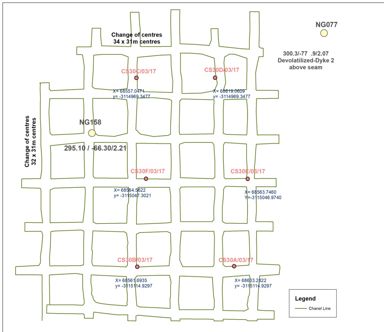
Figure 20: Ngwabe Shaft Section 30 layout showing where the channel sampling was conducted.
