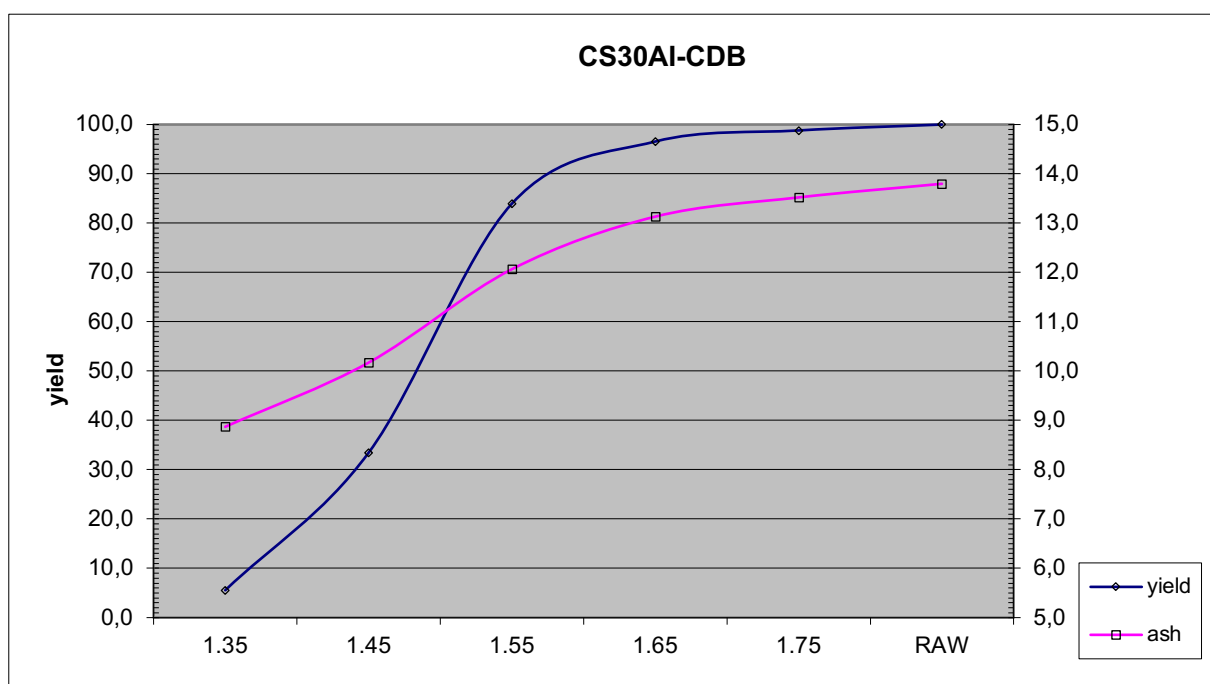
Figure 32: The densimetric and ash yield curves of the prime product of the CDB ply of the Channel Sample 30AI showing a relationship between Ash Yield and RD Yield.
