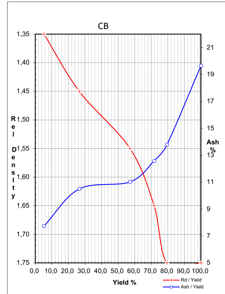
Figure 30: Graphical representation of the Ash Yield and densimetric washability curves of the CB ply of the CS30AI. Ash and RD are directly proportional to the yield of the CB ply.
