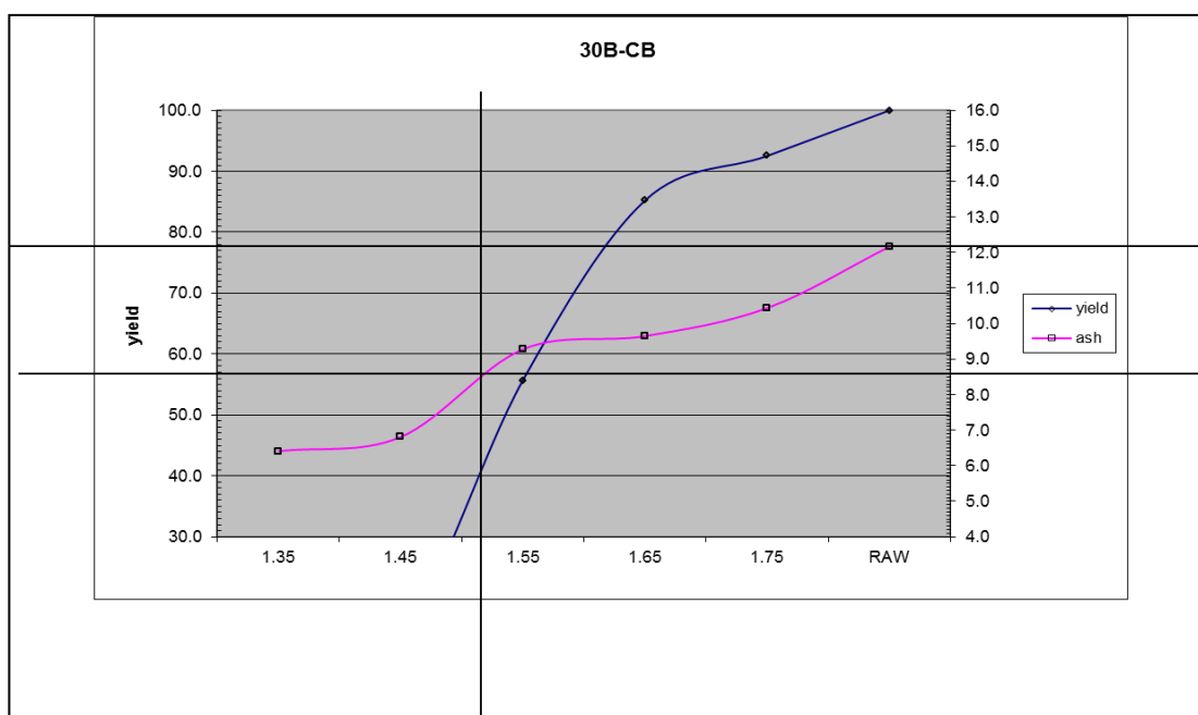
Figure 27: The densimetric and ash yield curves of the prime product of the CB ply of the Channel Sample 30B showing a relationship between Ash Yield and RD Yield.
