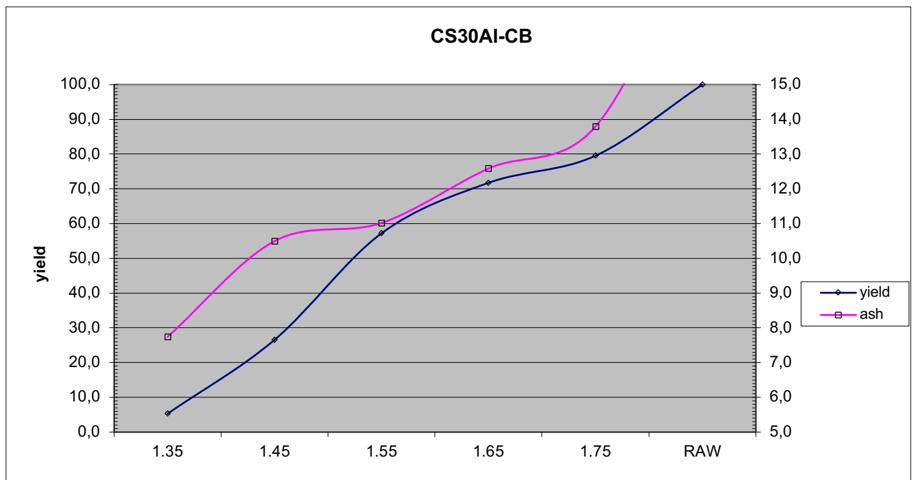
Figure 33: The densimetric and ash yield curves of the prime product of the CB ply of the Channel Sample 30AI showing a relationship between Ash Yield and RD Yield.
