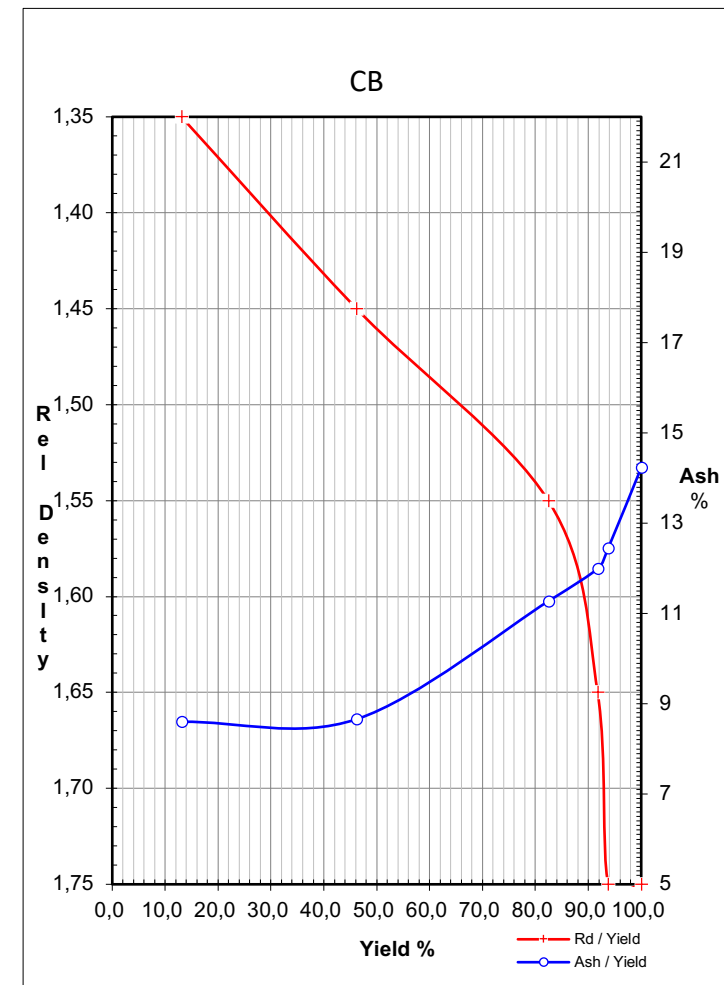
Figure 36: Graphical representation of the Ash Yield and densimetric washability curves of the CB ply of the CS30D. Ash and RD are directly proportional to the yield of the CB ply.
