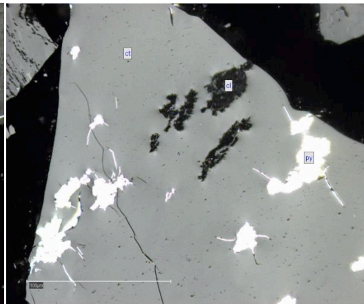
D. Collotelinite, clay (cl) and pyrite (py)
