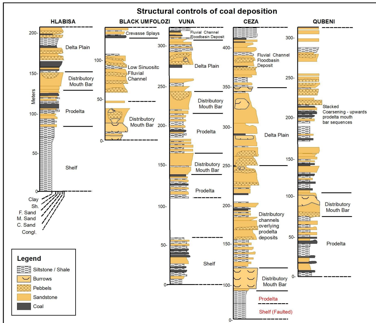
Figure 11: Measured stratigraphic profiles of the Karoo Supergroup showing coarsening-upward and fining-upward depositional trends and interpreted depositional environment (Turner and Whateley, 1983).
