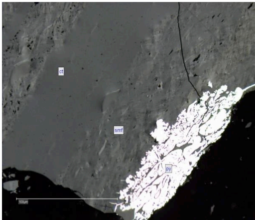
C. Collotelinite (ct), semifusinite (smf) pyrite (py)
