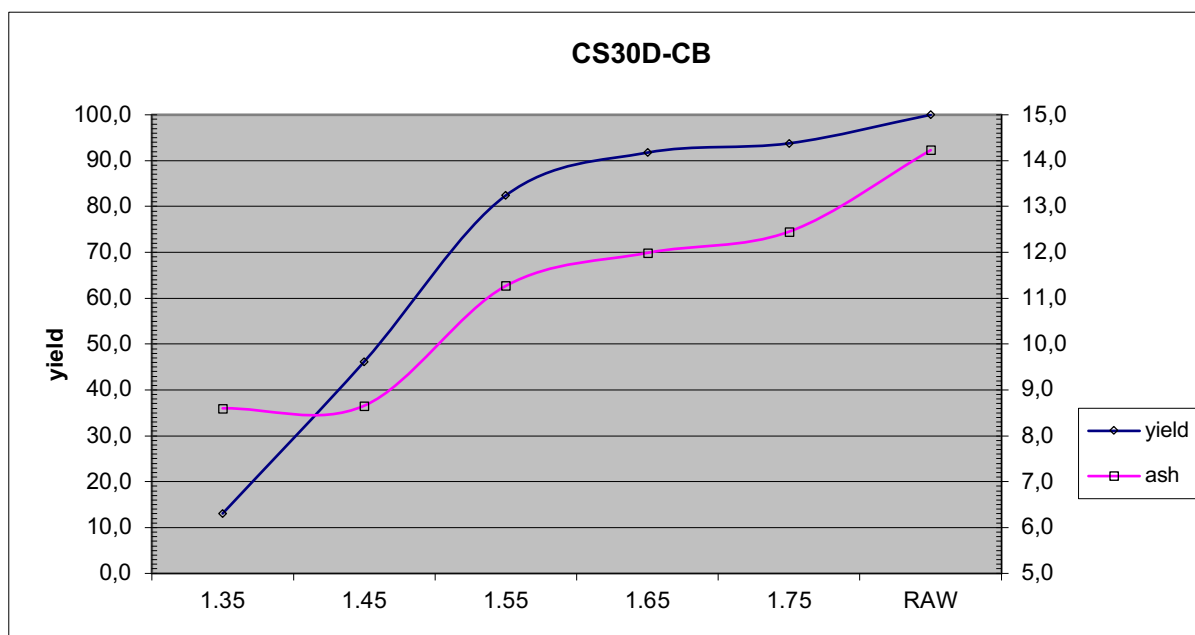
Figure 39: The densimetric and ash yield curves of the middlings product of the CB ply of the Channel Sample 30D showing a relationship between Ash Yield and RD Yield.
